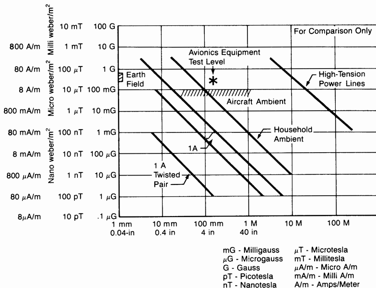
Figure 4.1-12 Magnetic Fields
