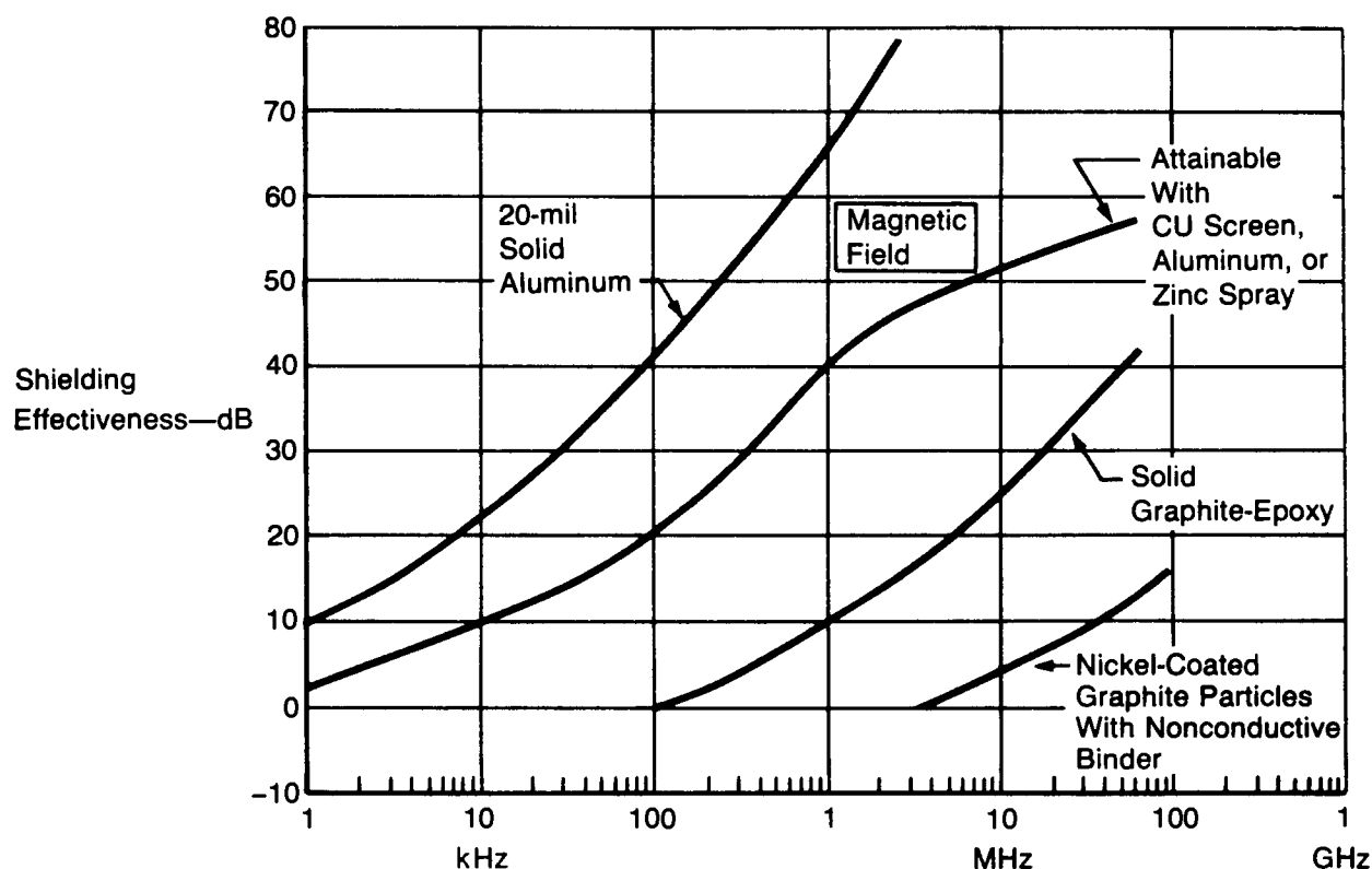
Figure 3.5-8 SE Comparison
