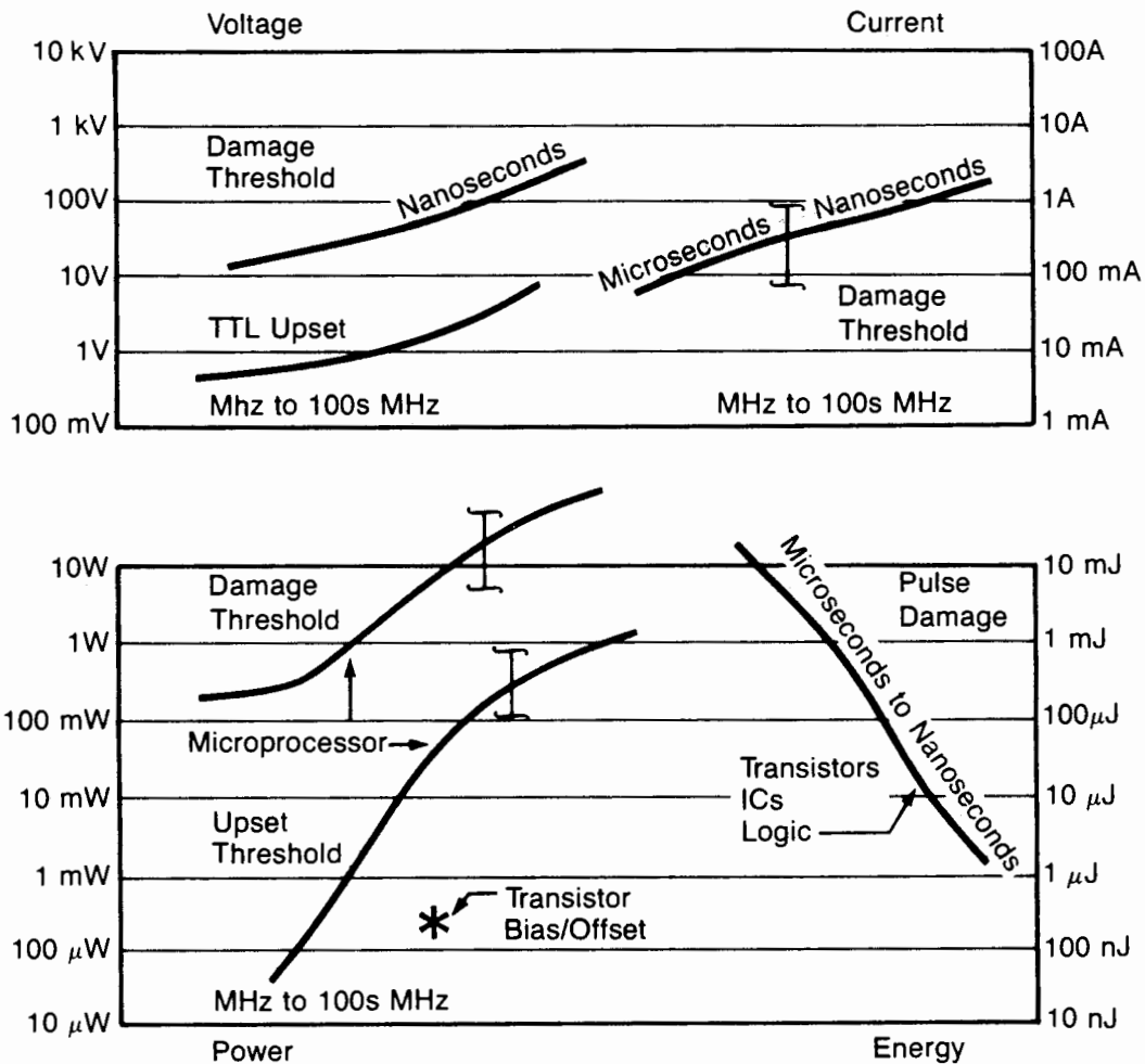
Figure 3.1-1 Microcircuit Tolerance
