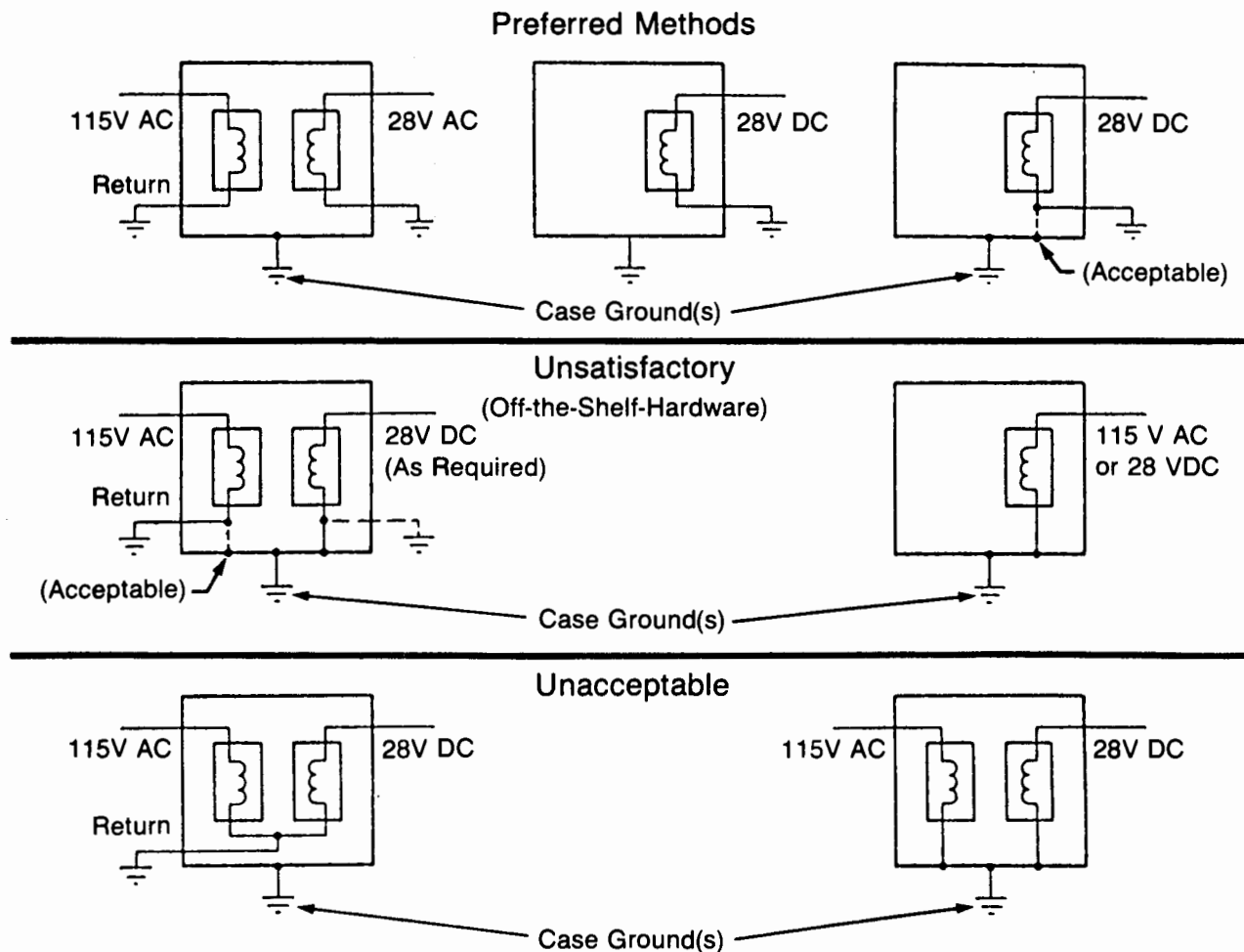
Figure 3.5-11 Power Returns
