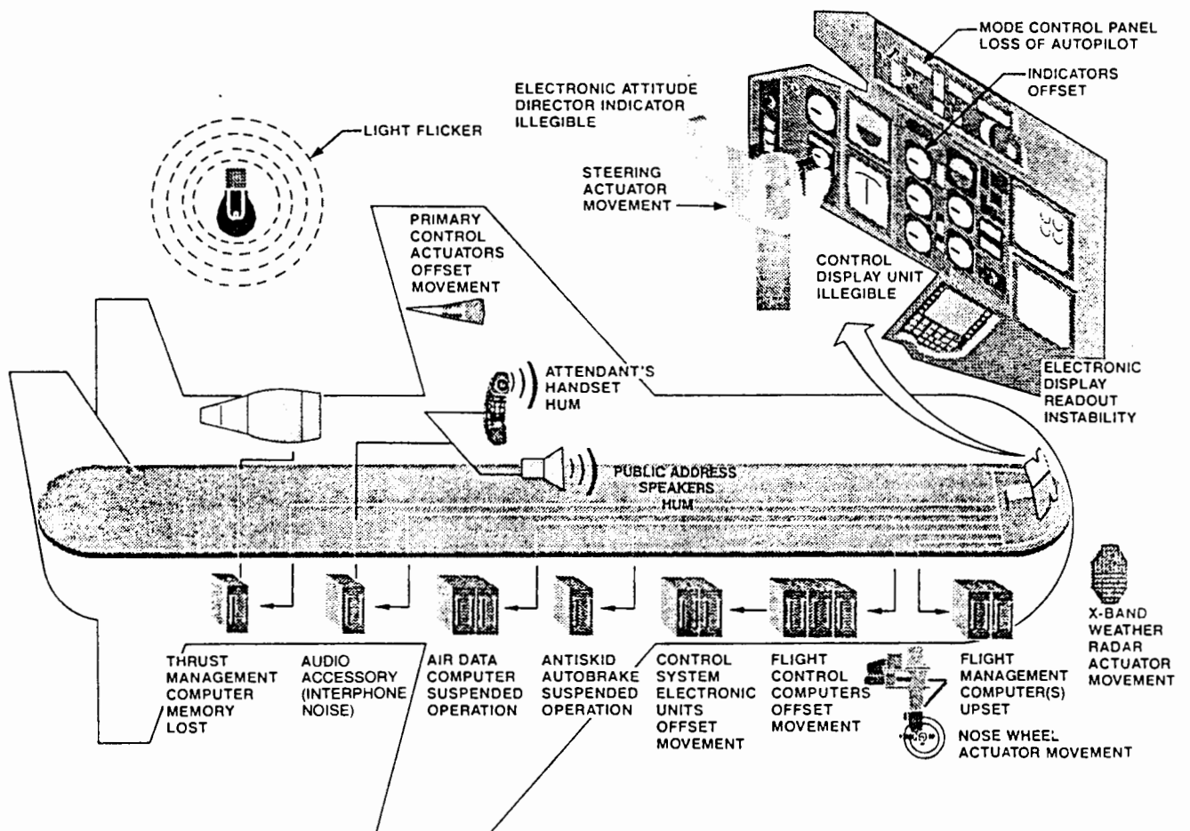
Figure 1.1-4 Electromagnetic Interference Effects
