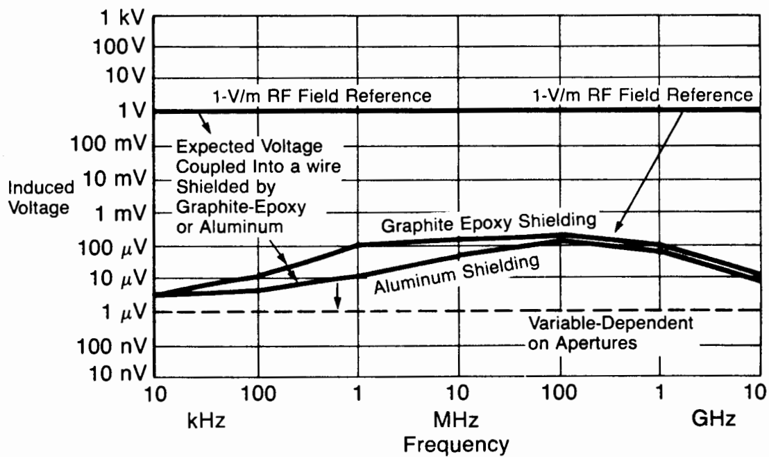
Figure 4.1-8 Graphite-Epoxy or Al Shielding Added
