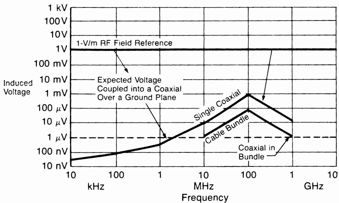
Figure 4.1-6 Representative Coax Voltage Coupling
