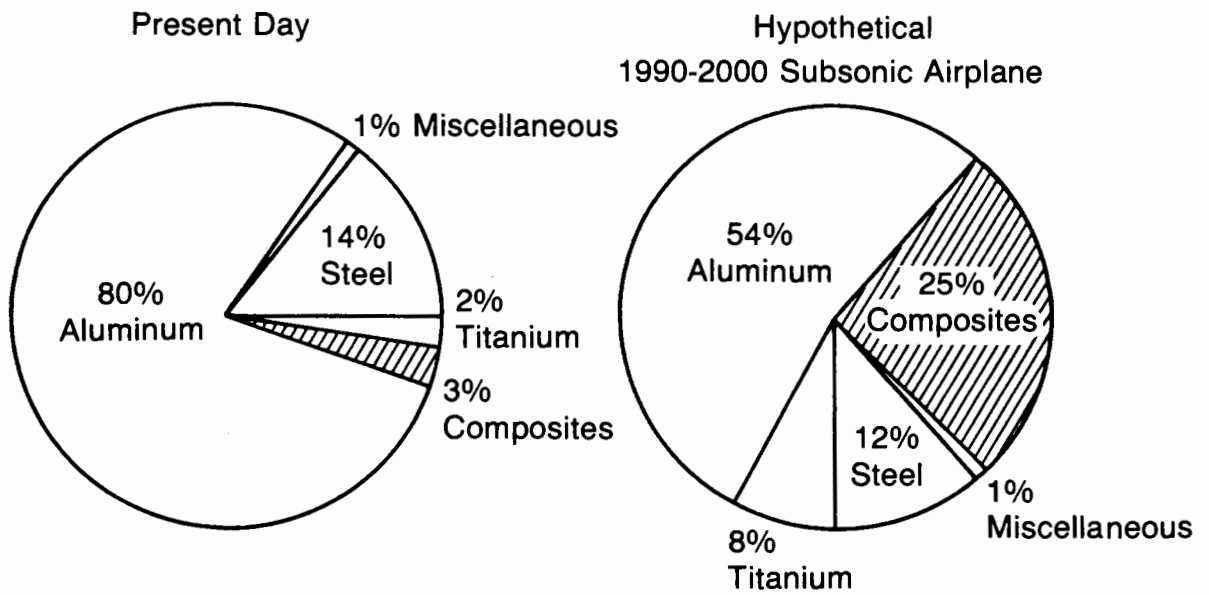
Figure 2.2-10 Materials Distribution
