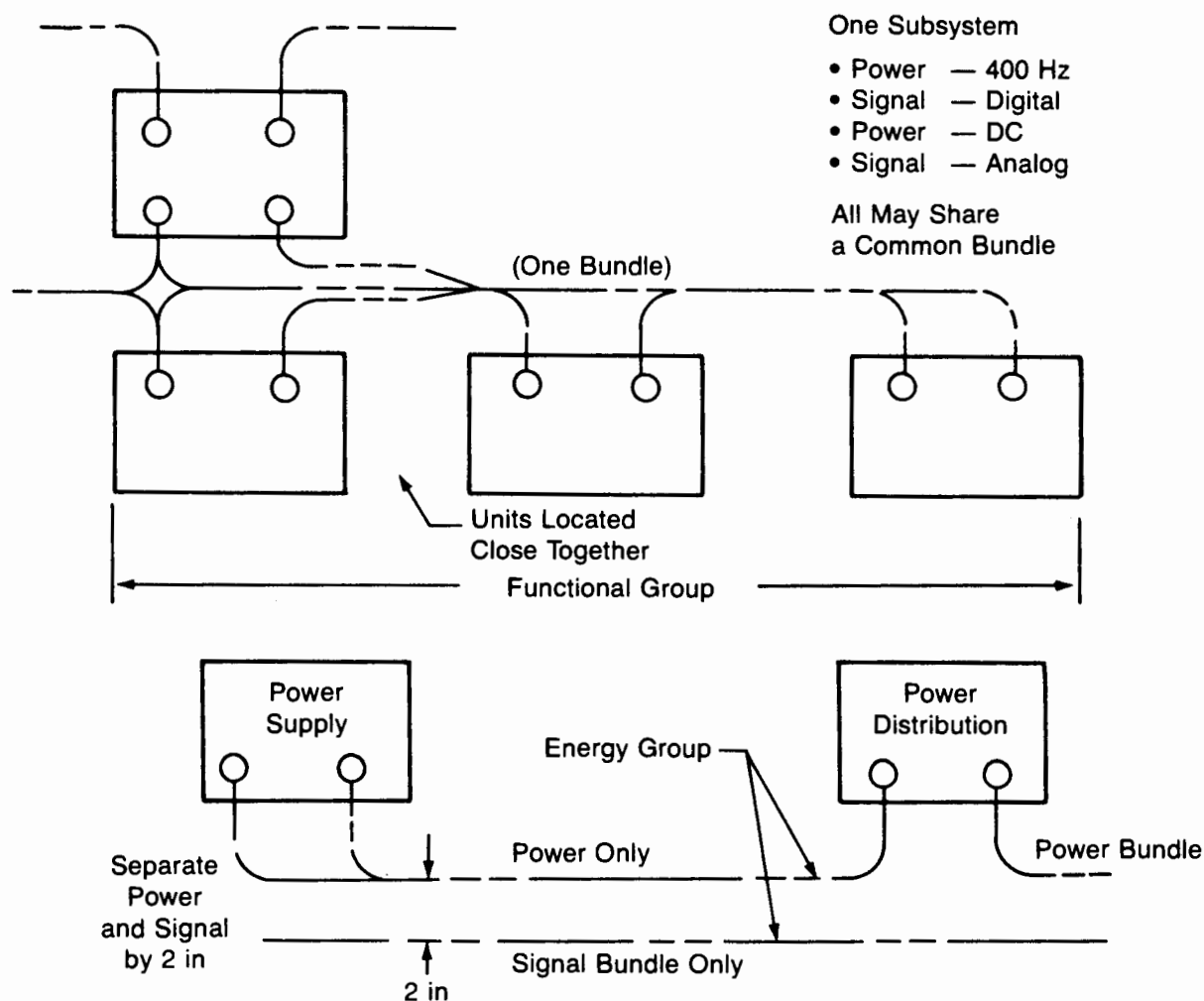
Figure 3.4-2 Wiring Categories
