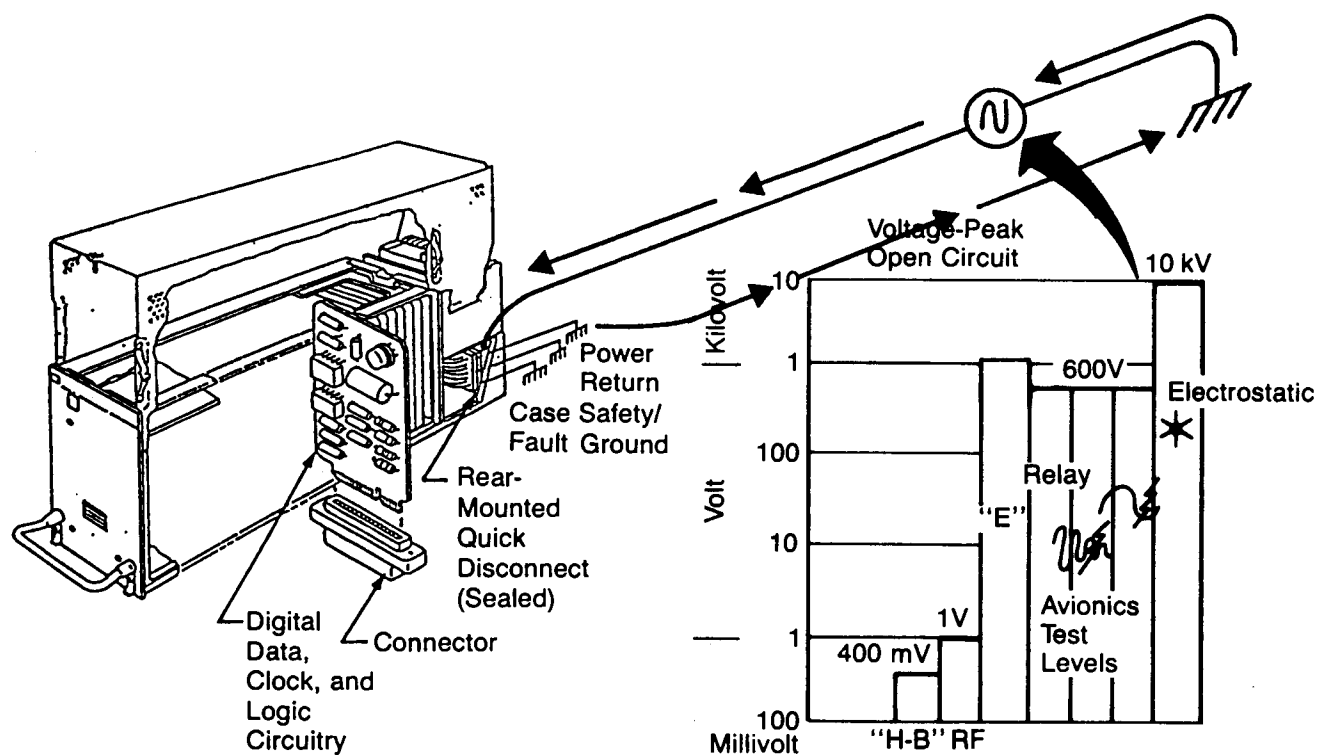
Figure 2.1-7 Noise Voltages
