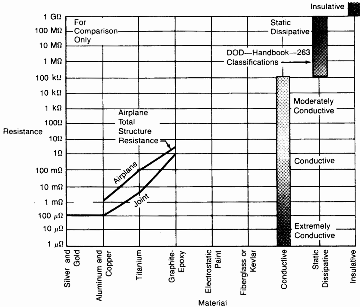
Figure 3.5-13 Configuration/Resistance Overview
