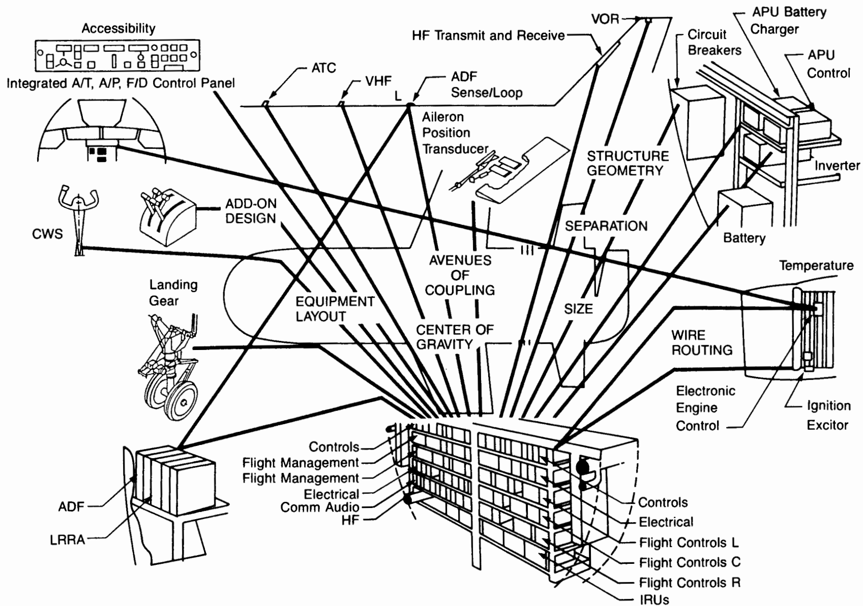
Figure 2.1-19 Equipment/Wiring Location Complexities
