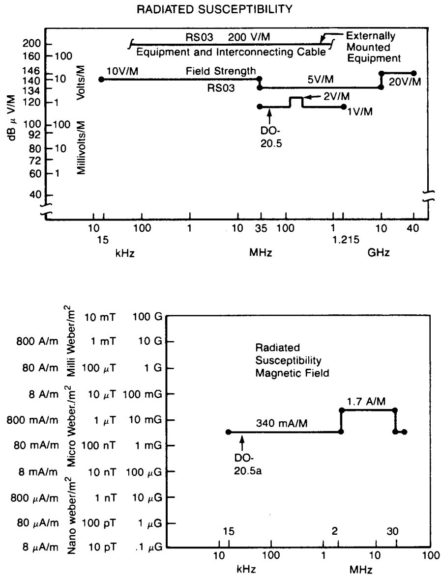
Figure B1. EMI Test Limits (Continued)
