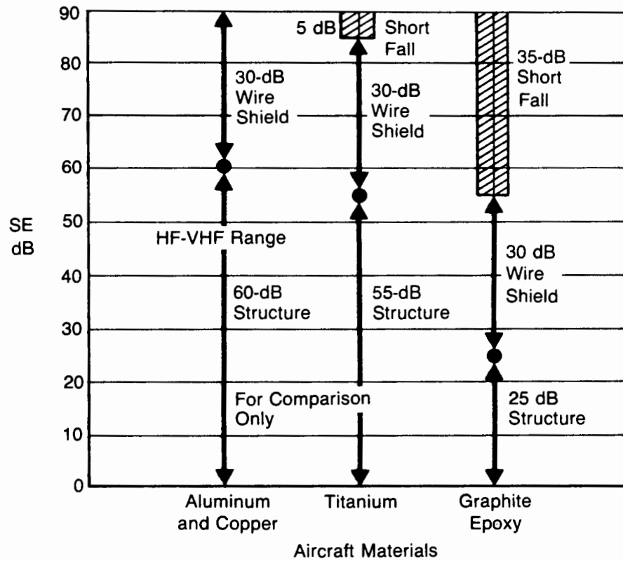
Figure 3.6-3 Graphite-Epoxy SE Shortfall
