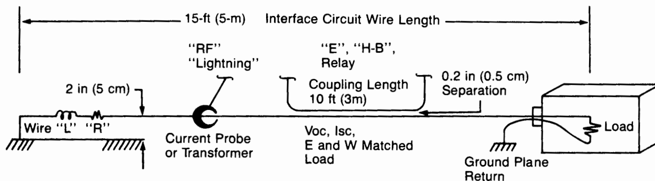
Figure 3.4-5 Laboratory Test Setup
