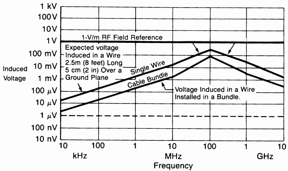
Figure 4.1-3 Expected Wire Voltage—Eight Feet
