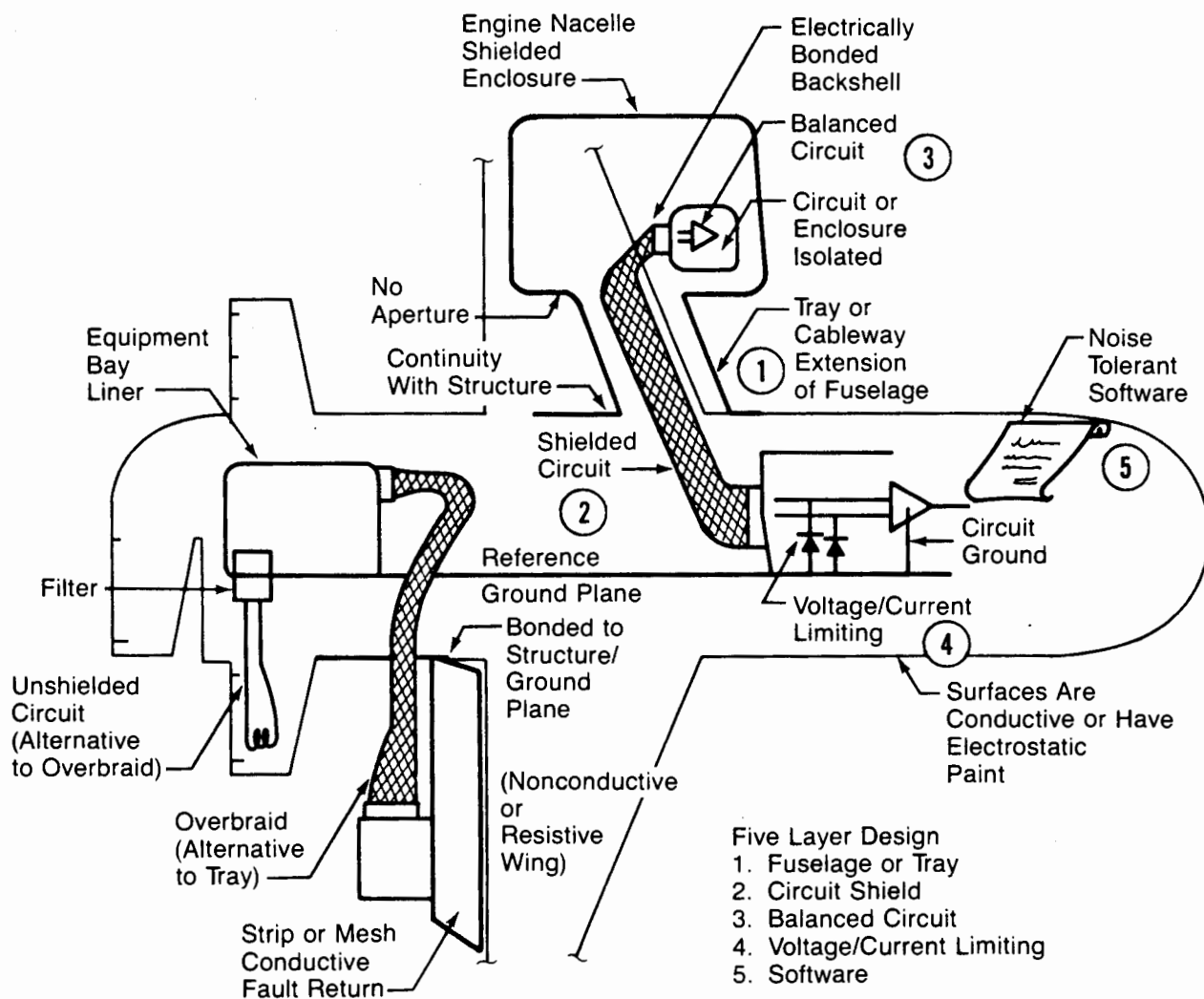
Figure 4.2-1 Layered Design
