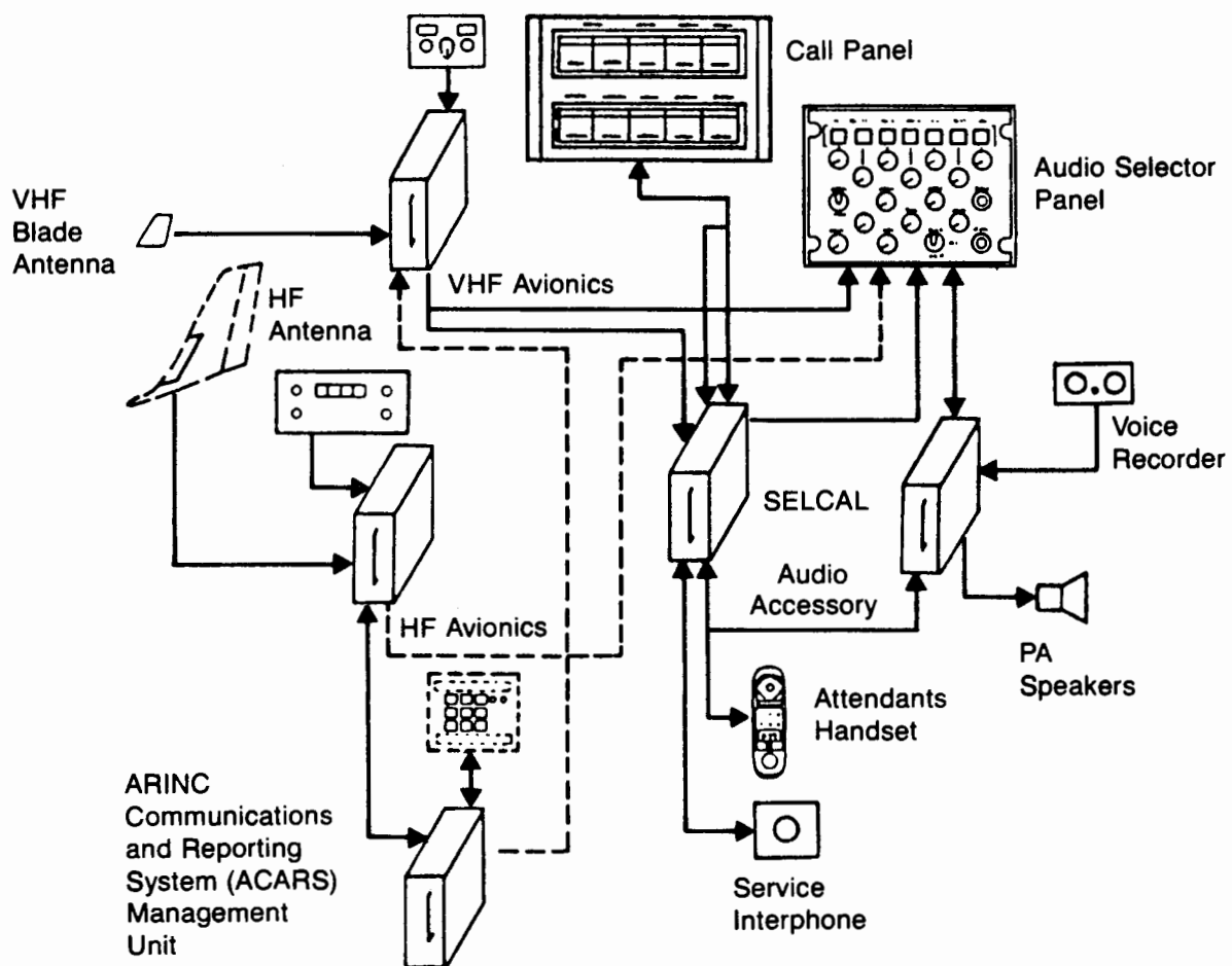
Figure 2.1-16 Communication
