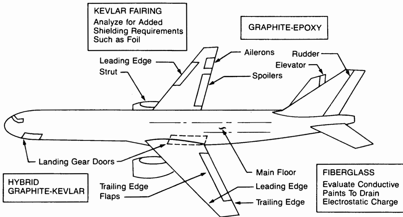
Figure 3.6-1 Typical Nonmetallic Applications
