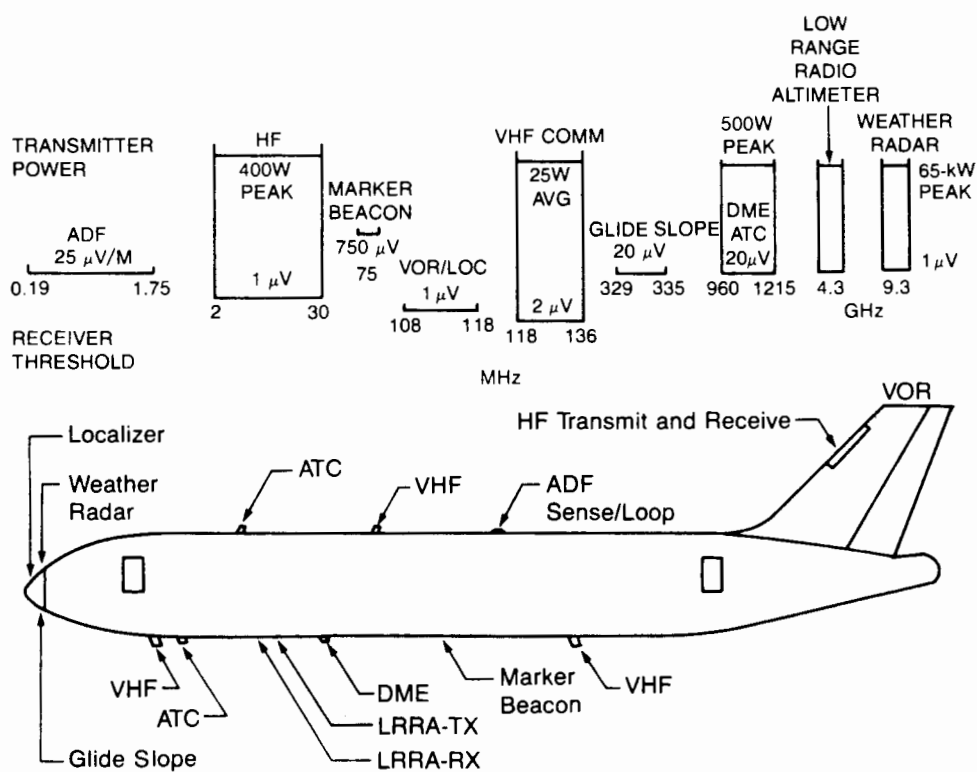
Figure 2.1-12 Transmitters-Receivers
