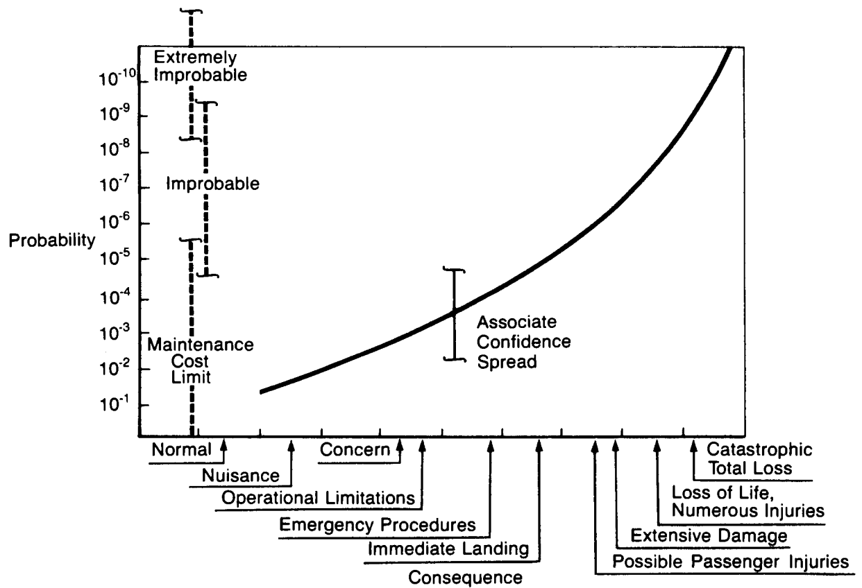
Figure 2.3-1 Probability Versus Consequence
