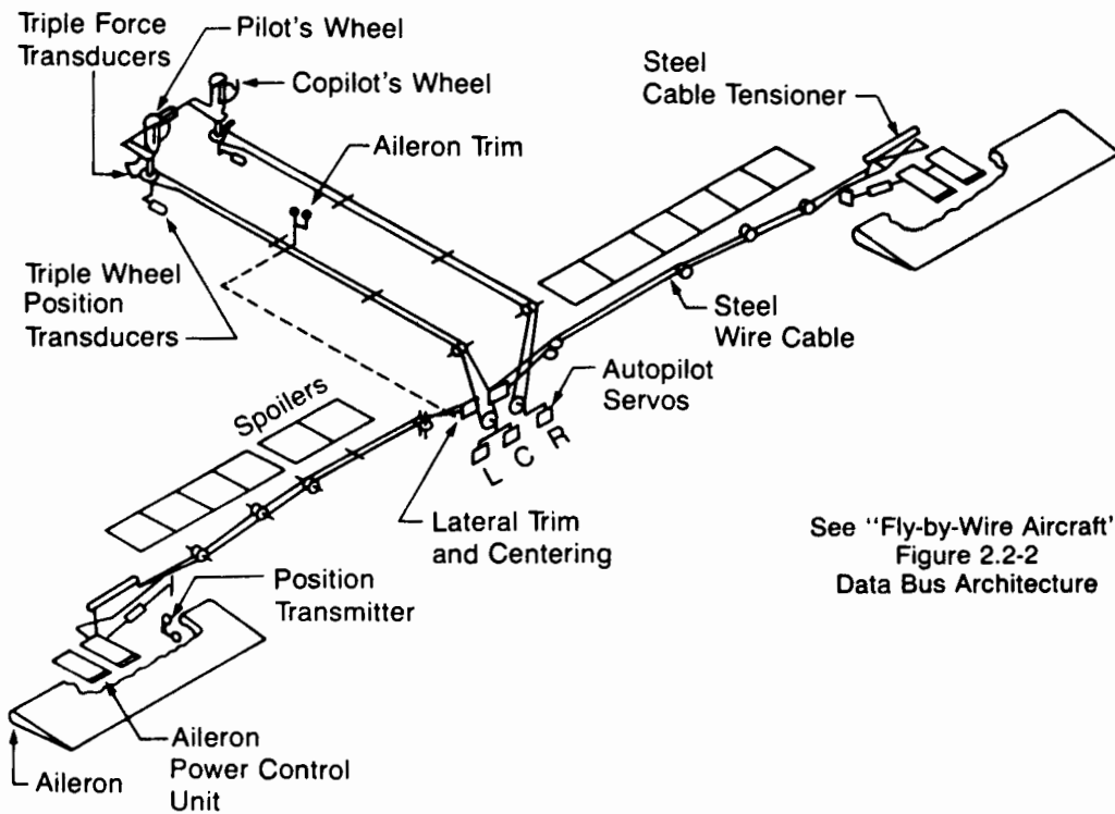
Figure 2.1-14 Roll Control System
