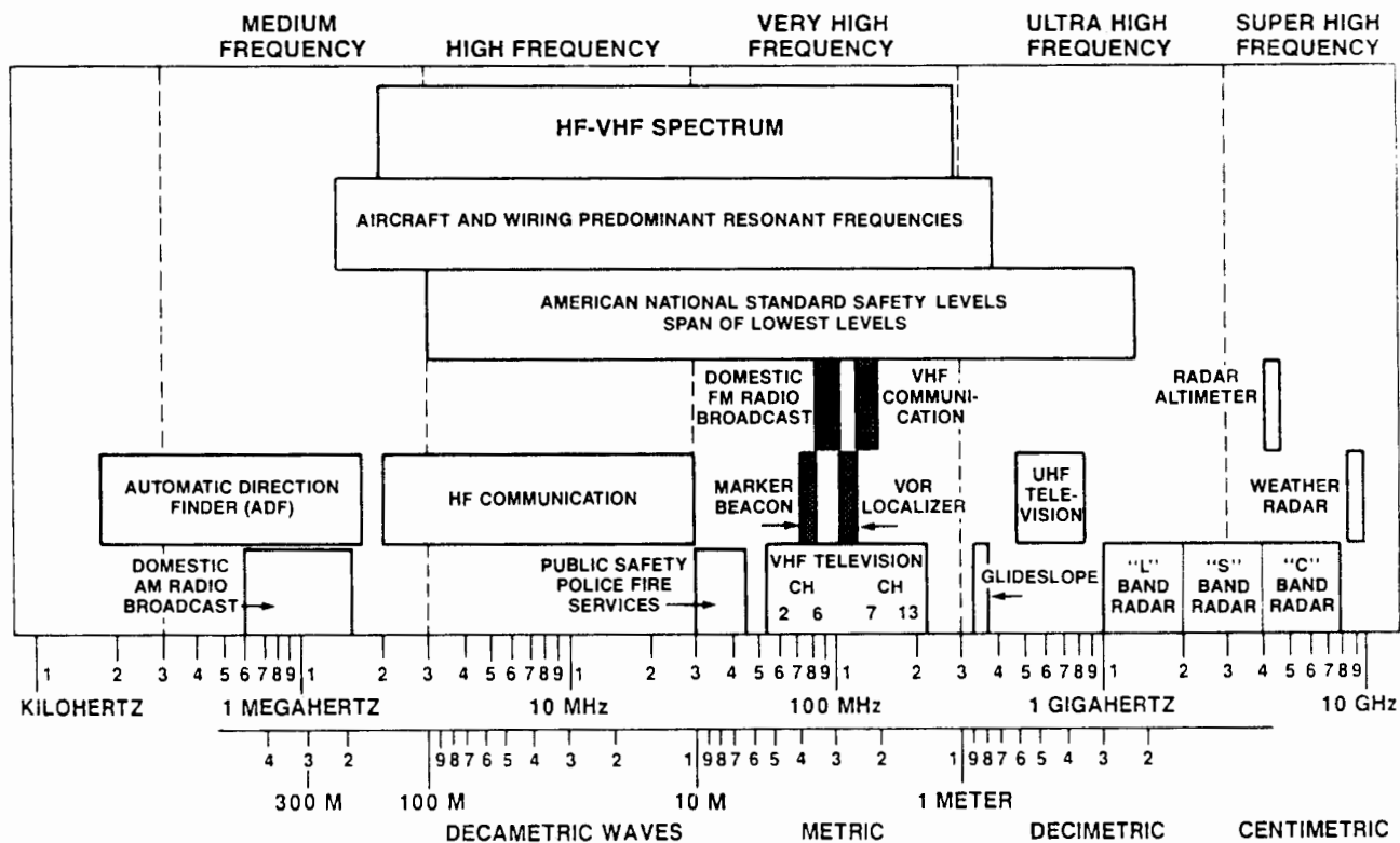
Figure 4.1-1 HF-VHF Range
