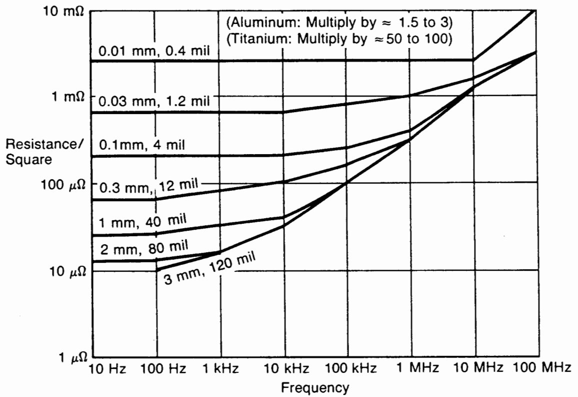
Figure 3.5-14 Resistance Plot—Copper Plane
