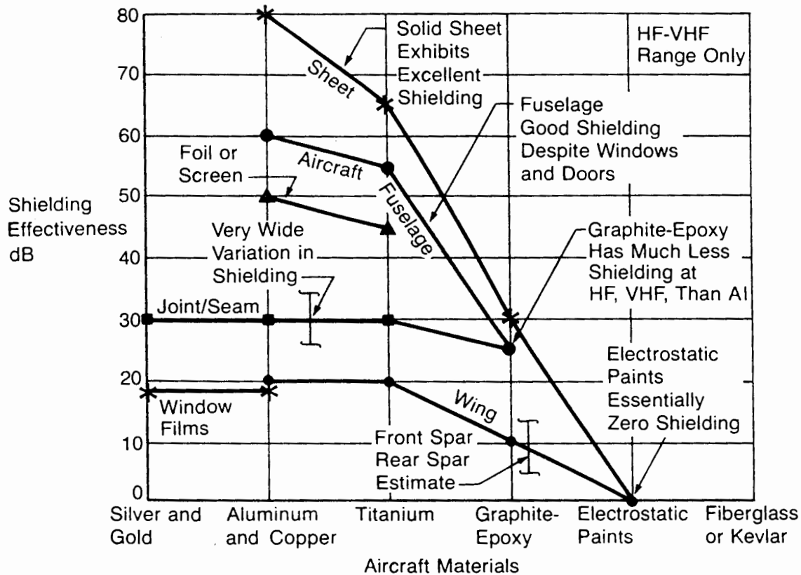
Figure 3.5-10 Material/Configuration SE Overview
