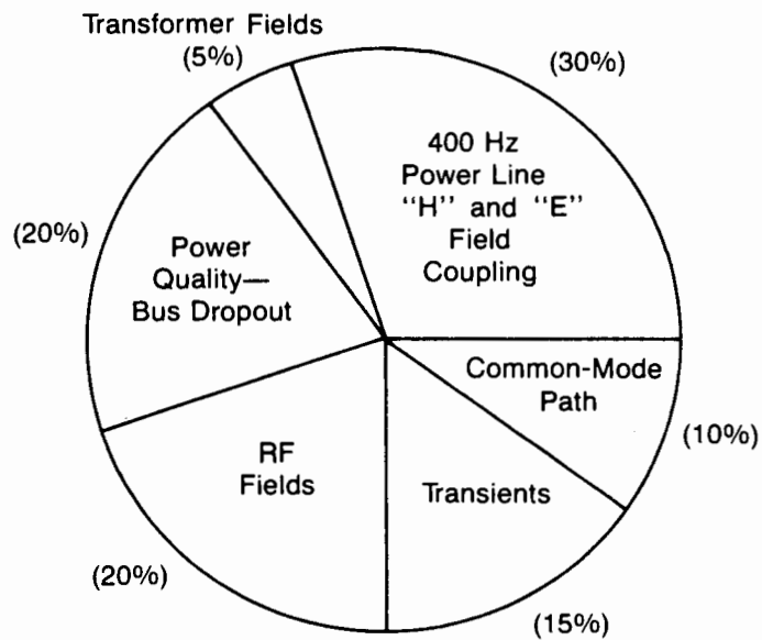
Figure 1.1-3 Percent Troubleshooting—A/C
