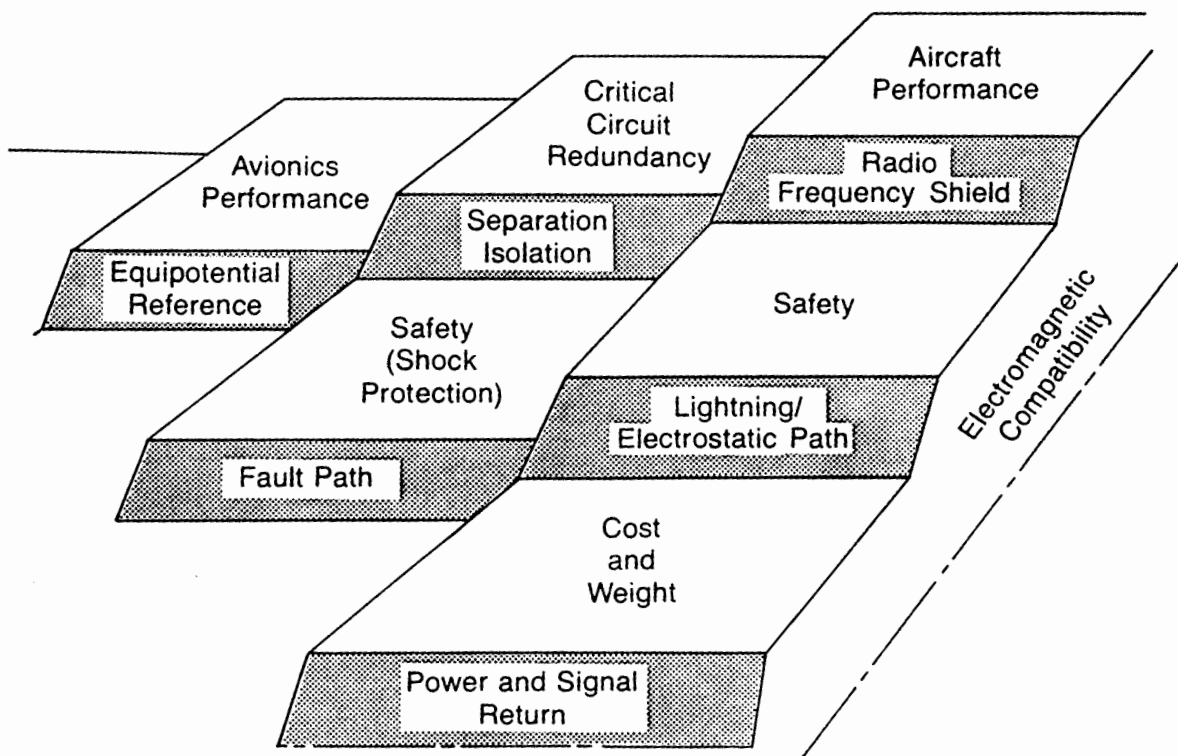
Figure 3.5-1 The Grounding Steps
