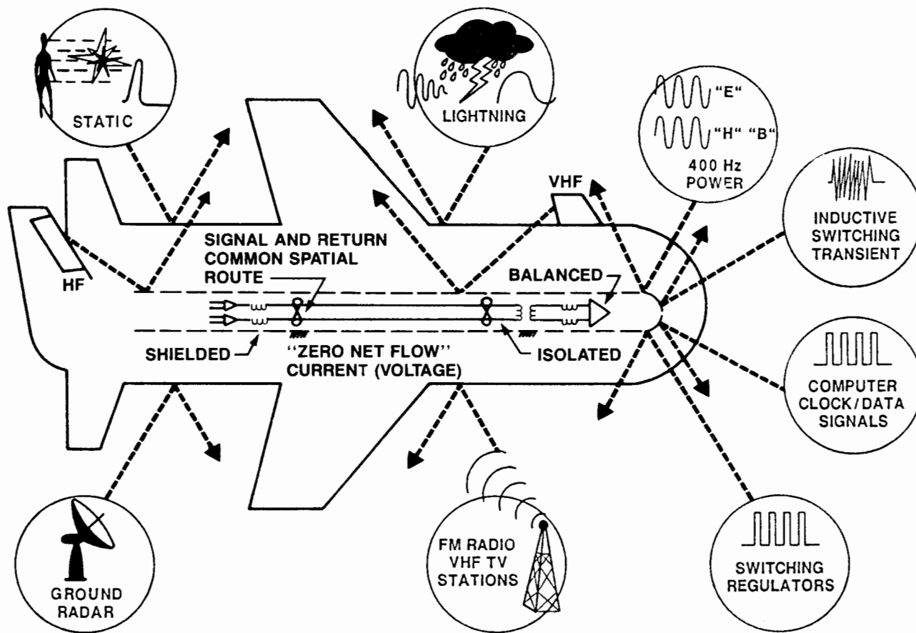
Figure 1.1-2 EMI Environment in Aircraft
