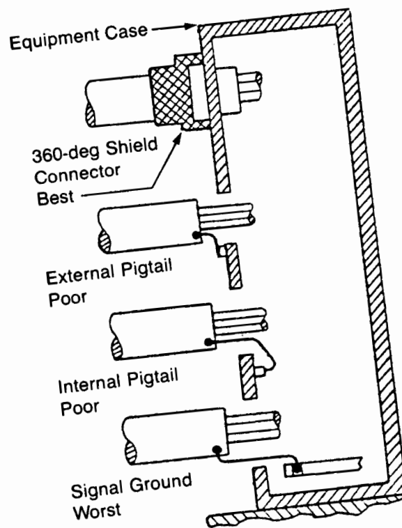
Figure 3.4-6 Shield Ties
