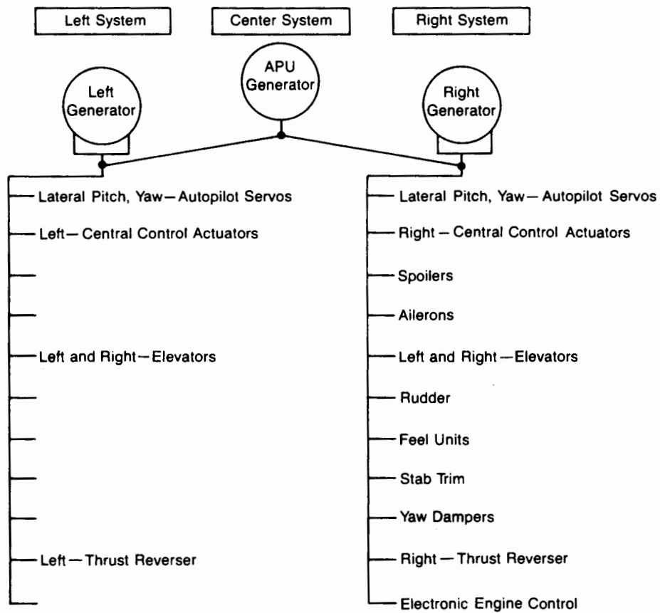
Figure 2.1-9 Separation Example
