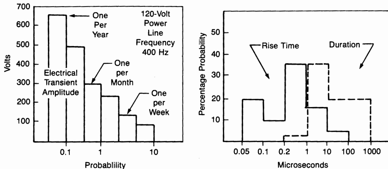
Figure 4.1-14 Electrical Transients
