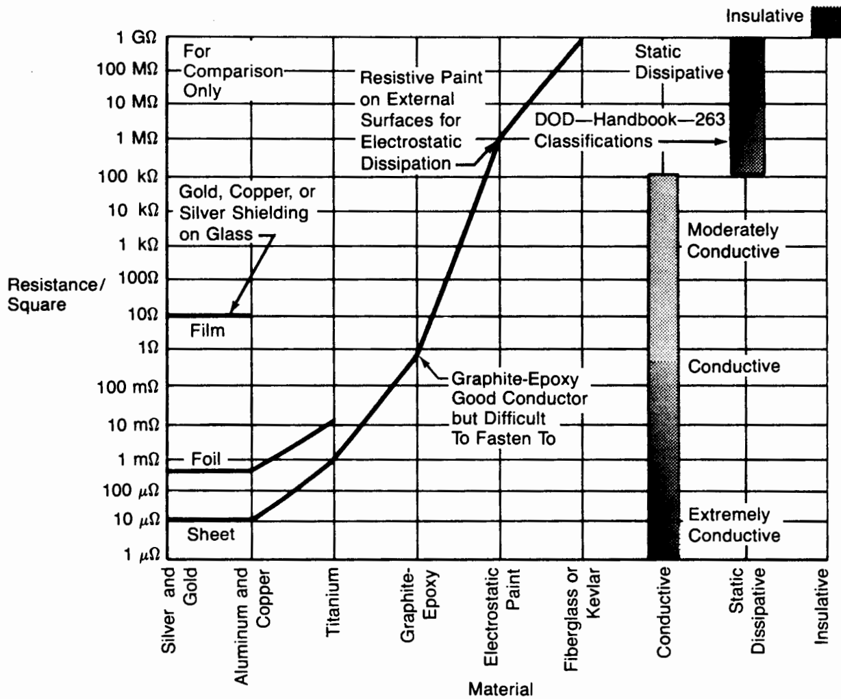
Figure 3.5-12 Material/Resistance Overview
