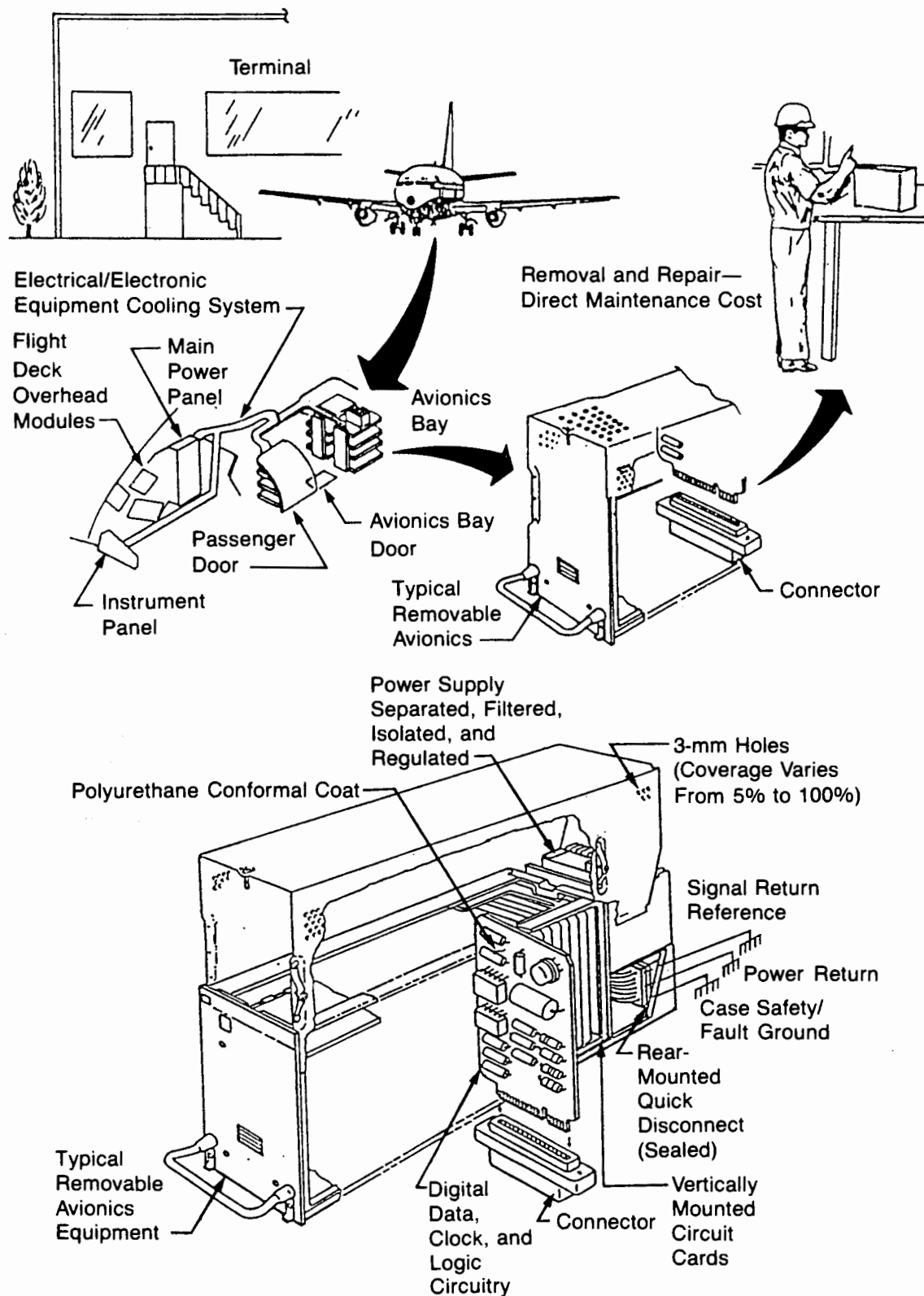
Figure 2.1-17 Line Replaceable Unit
