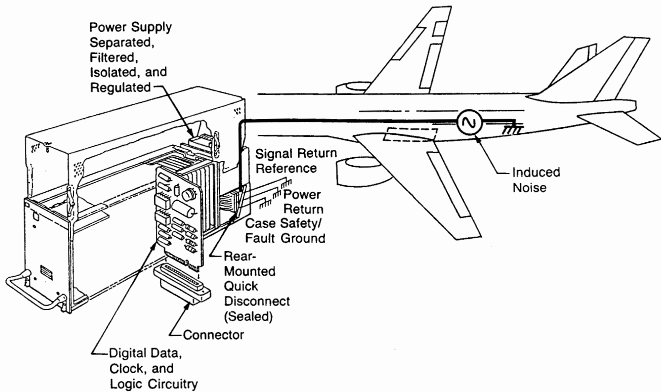
Figure 2.1-5 Structure Return
