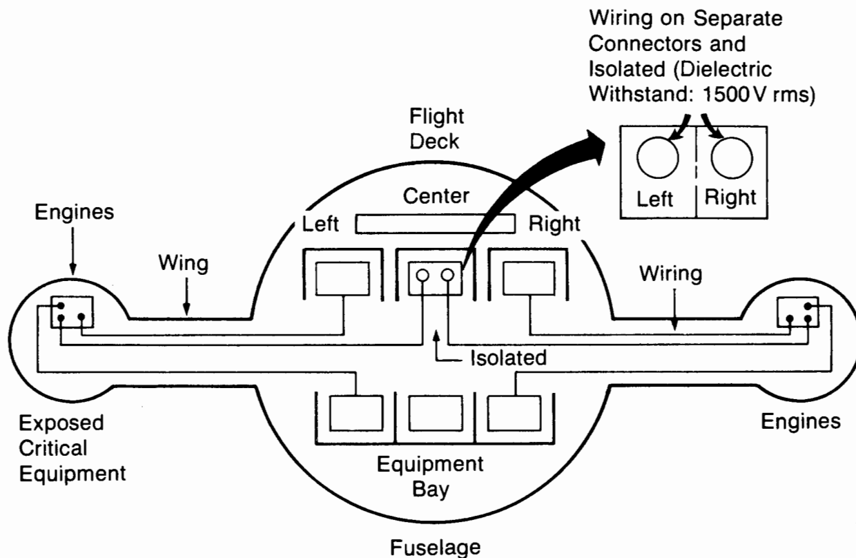
Figure 3.4-3 Critical Circuits Wire Separation
