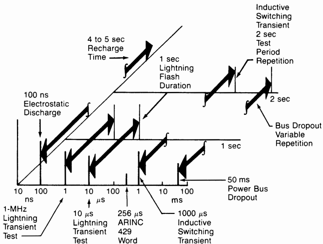
Figure 3.2-1. Transient Events
