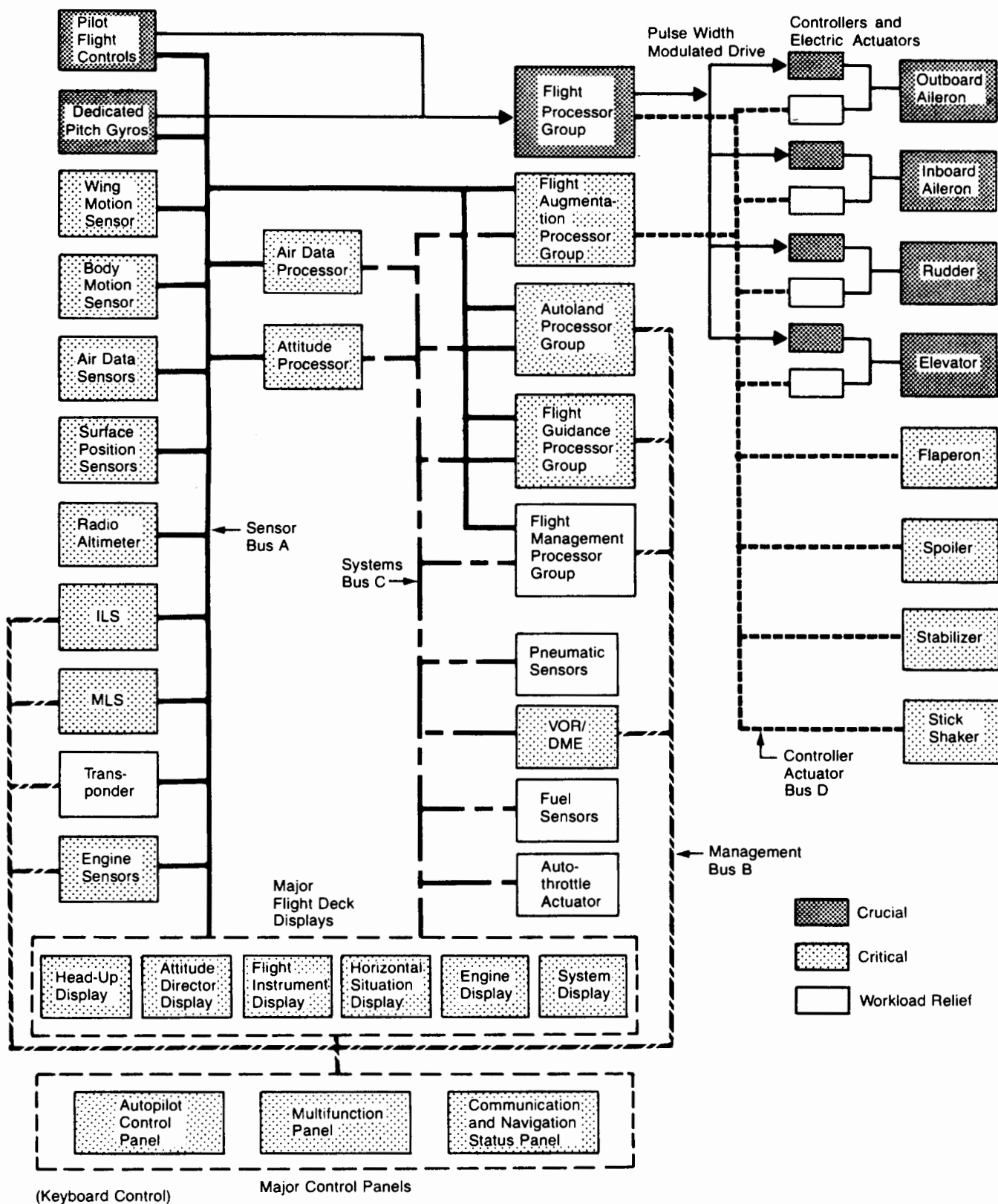
Figure 2.3-3 Projected Criticalities
