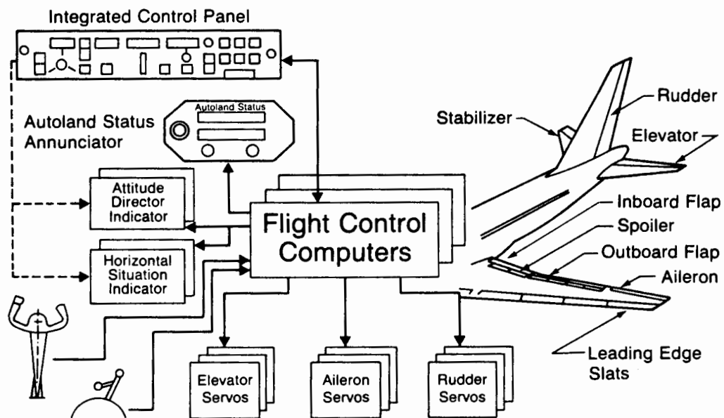
Figure 2.1-10 Flight Control Autopilot Redundancy
