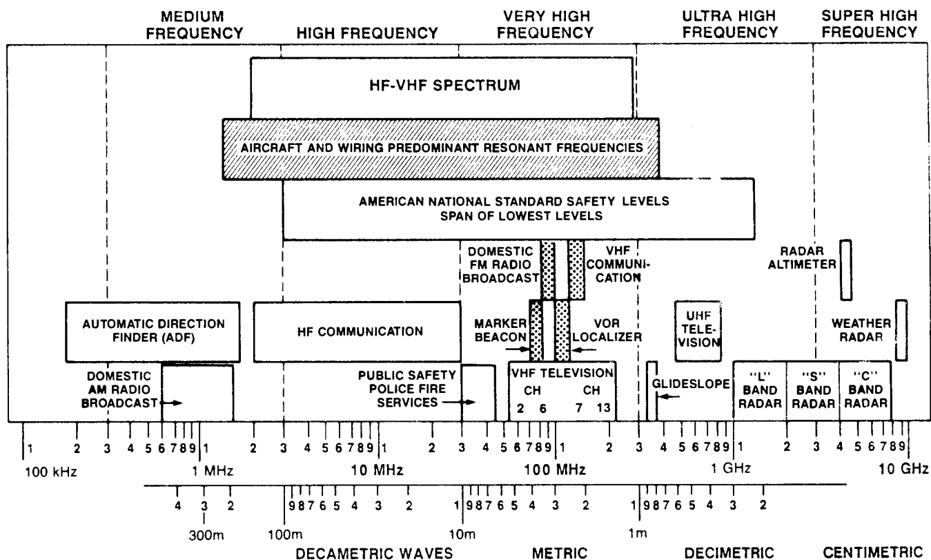
Figure 1.1-5 Radio Frequency Range
