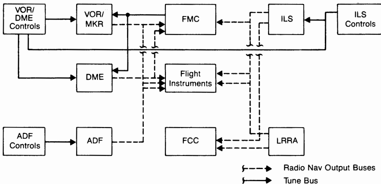
Figure 2.1-15 Navigation
