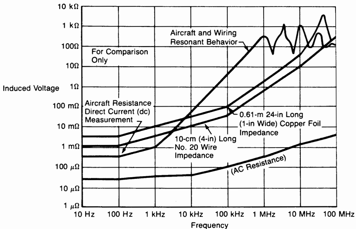
Figure 3.5-17 Aircraft and Strap Resonance
