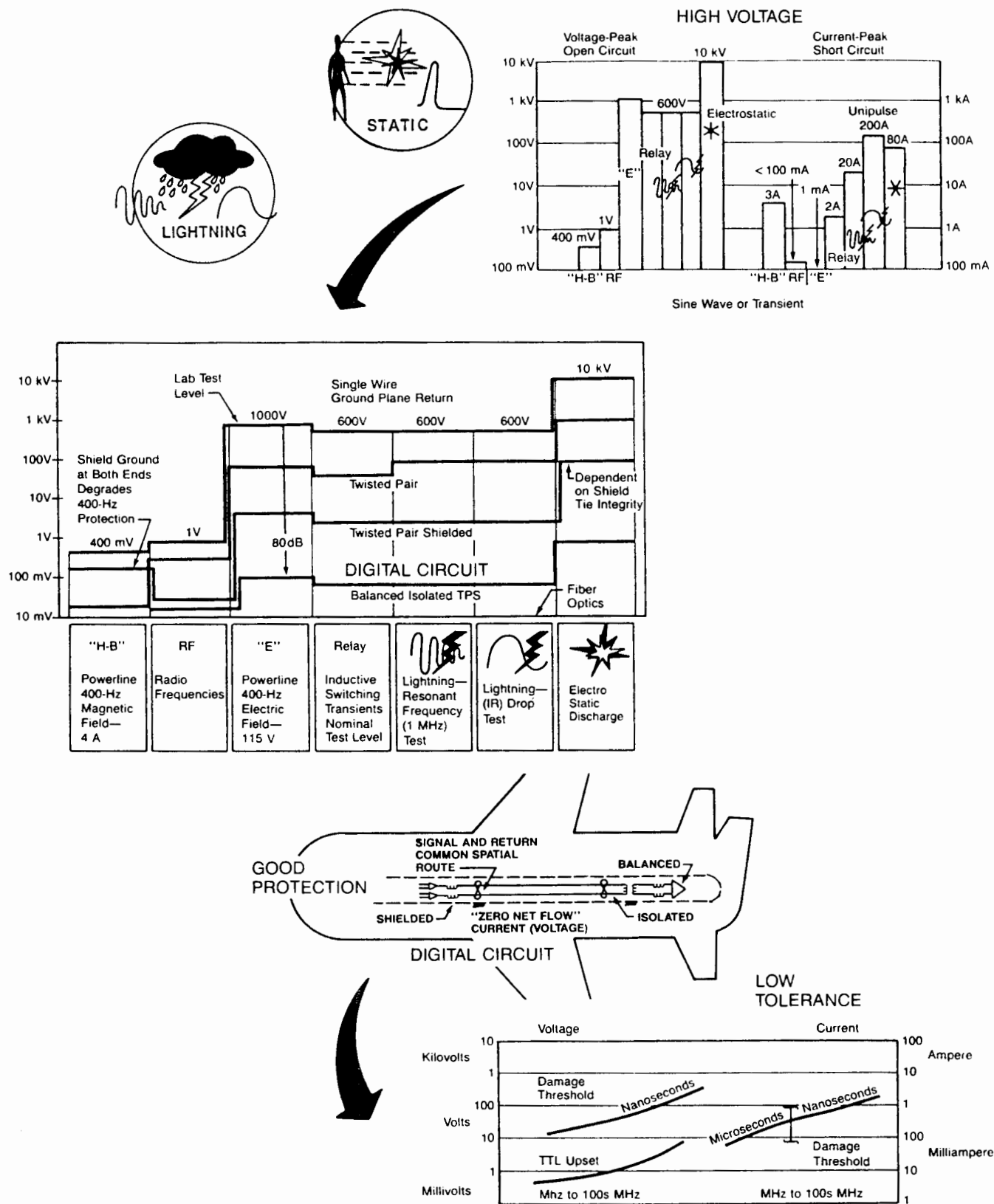
Figure 4.3-3 Trade—Digital Circuits
