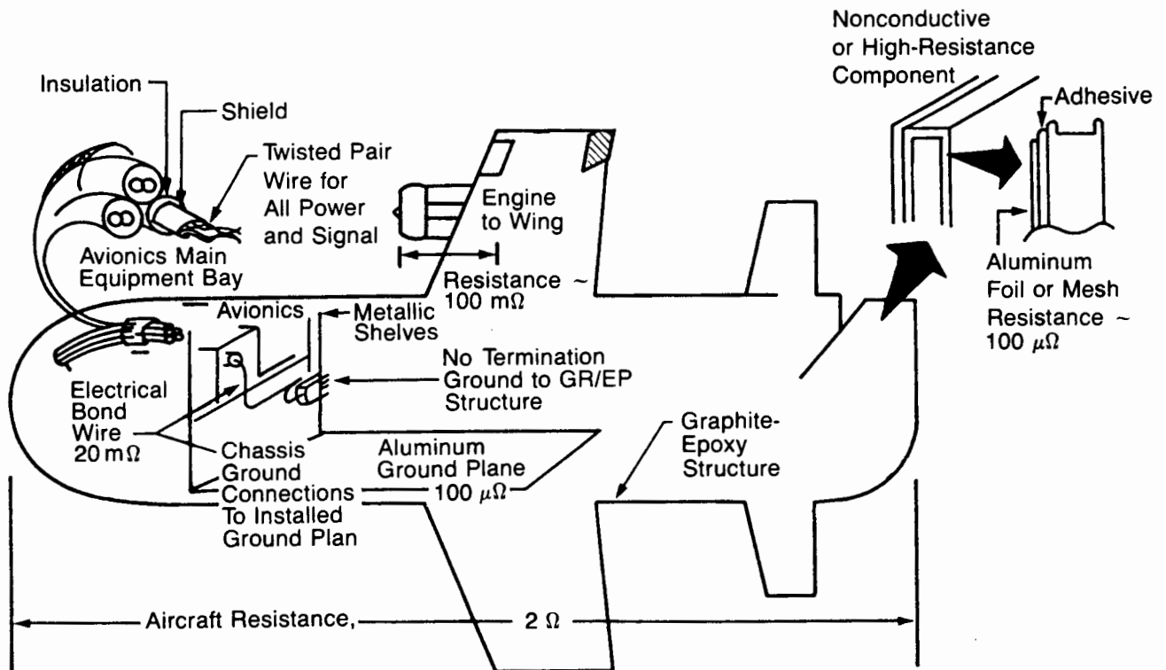
Figure 3.6-4 Graphite-Epoxy Details and Installation
