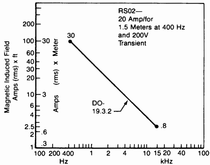
Figure B1. EMI Test Limits (Continued)
