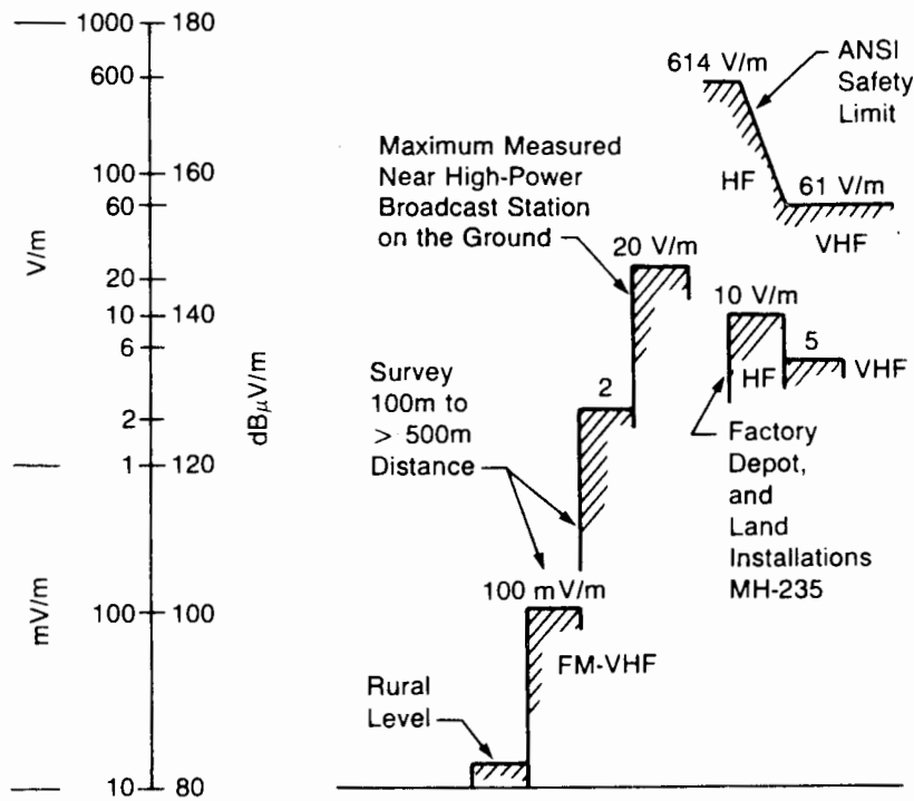
Figure 4.1-2 Selected RF Fields: HF-VHF Range
