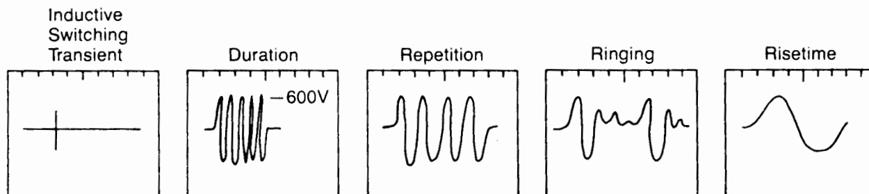
Figure 4.1-13 Transient Ringing
