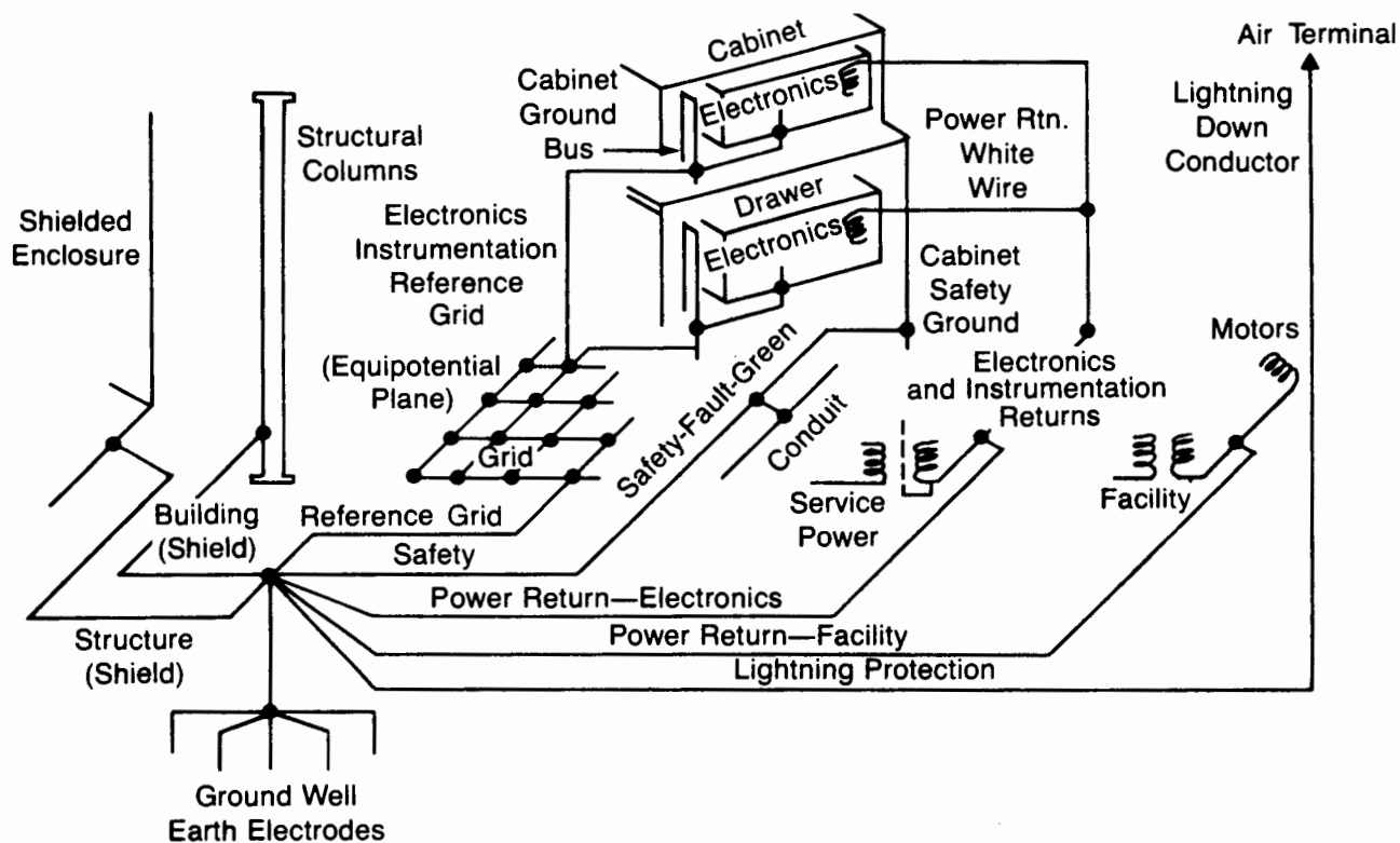
Figure 3.5-4 The Seven Earth Ground Connections
