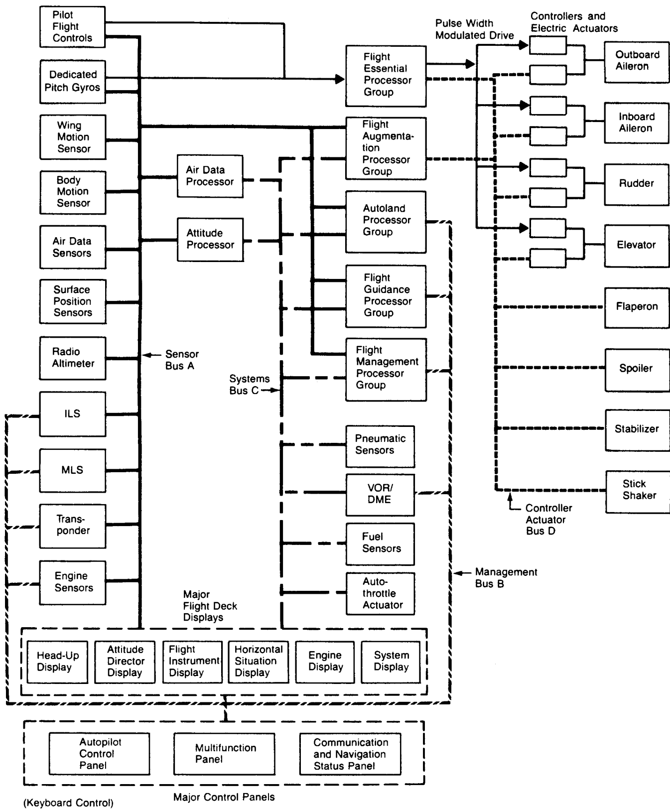
Figure 2.2-4 Hypothetical Architecture
