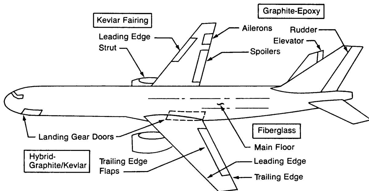
Figure 2.1-8 Nonmetallic Interfaces
