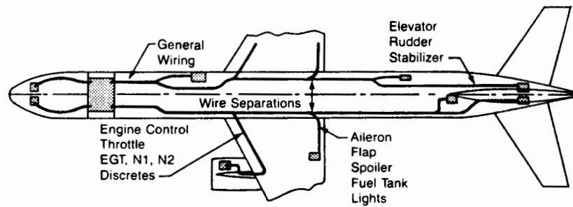
Figure 2.1-3 Wiring
