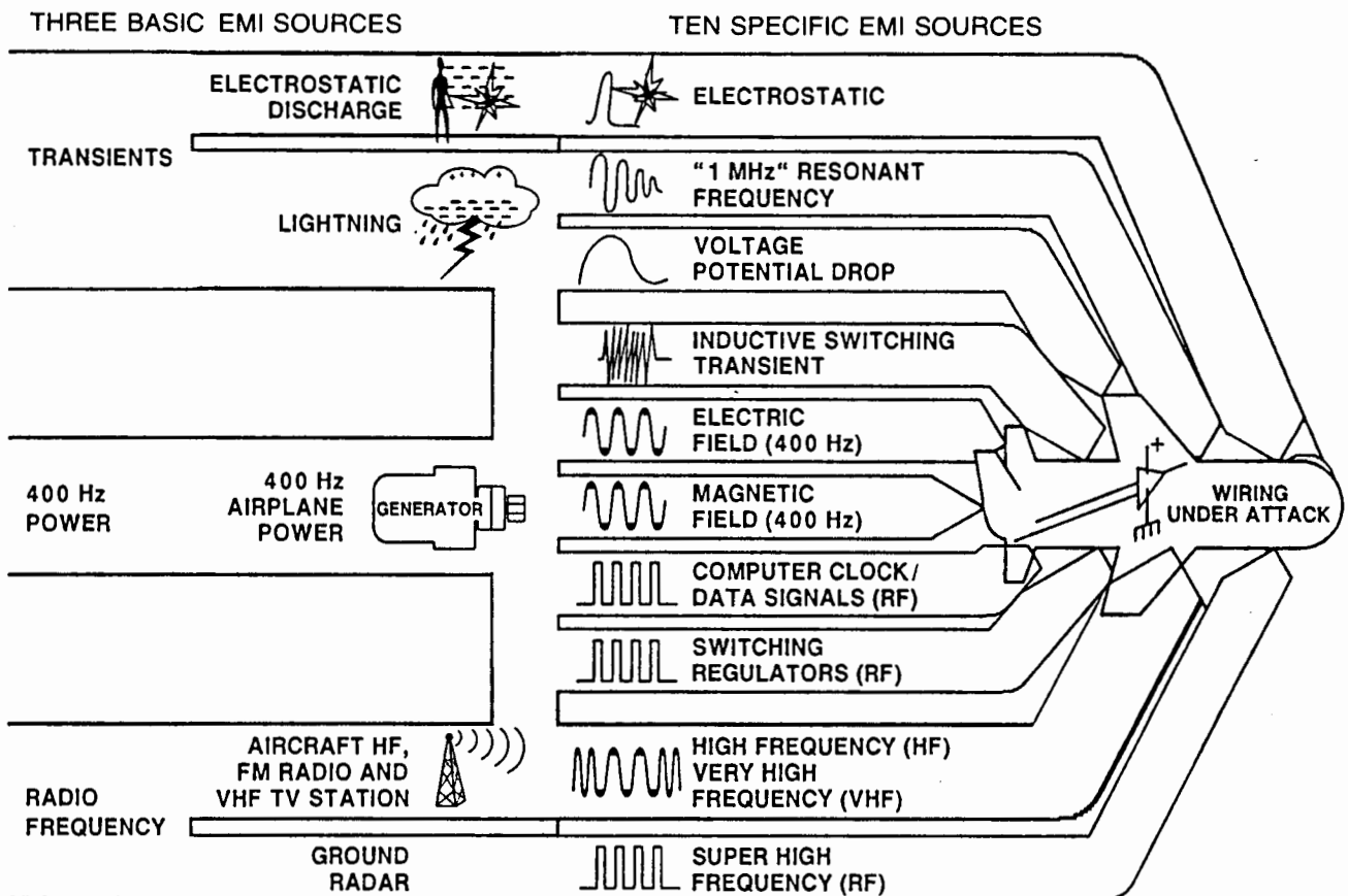
Figure 1.1-1 Representative EMI Sources
