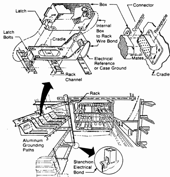
Figure 2.1-4 Main Bay Aluminum Structure
