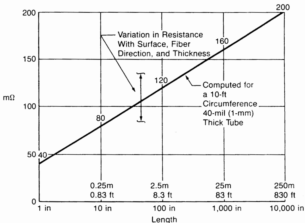
Figure 3.6-2 Graphite-Epoxy Resistance
