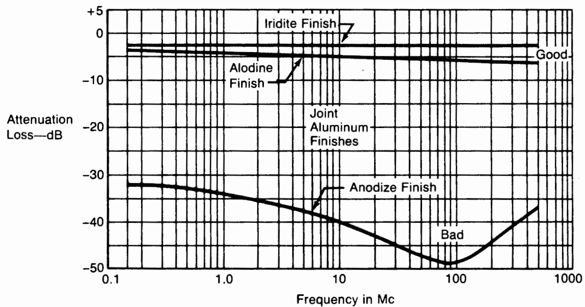
Figure 3.5-7 Loss of SE with Joint Finish
