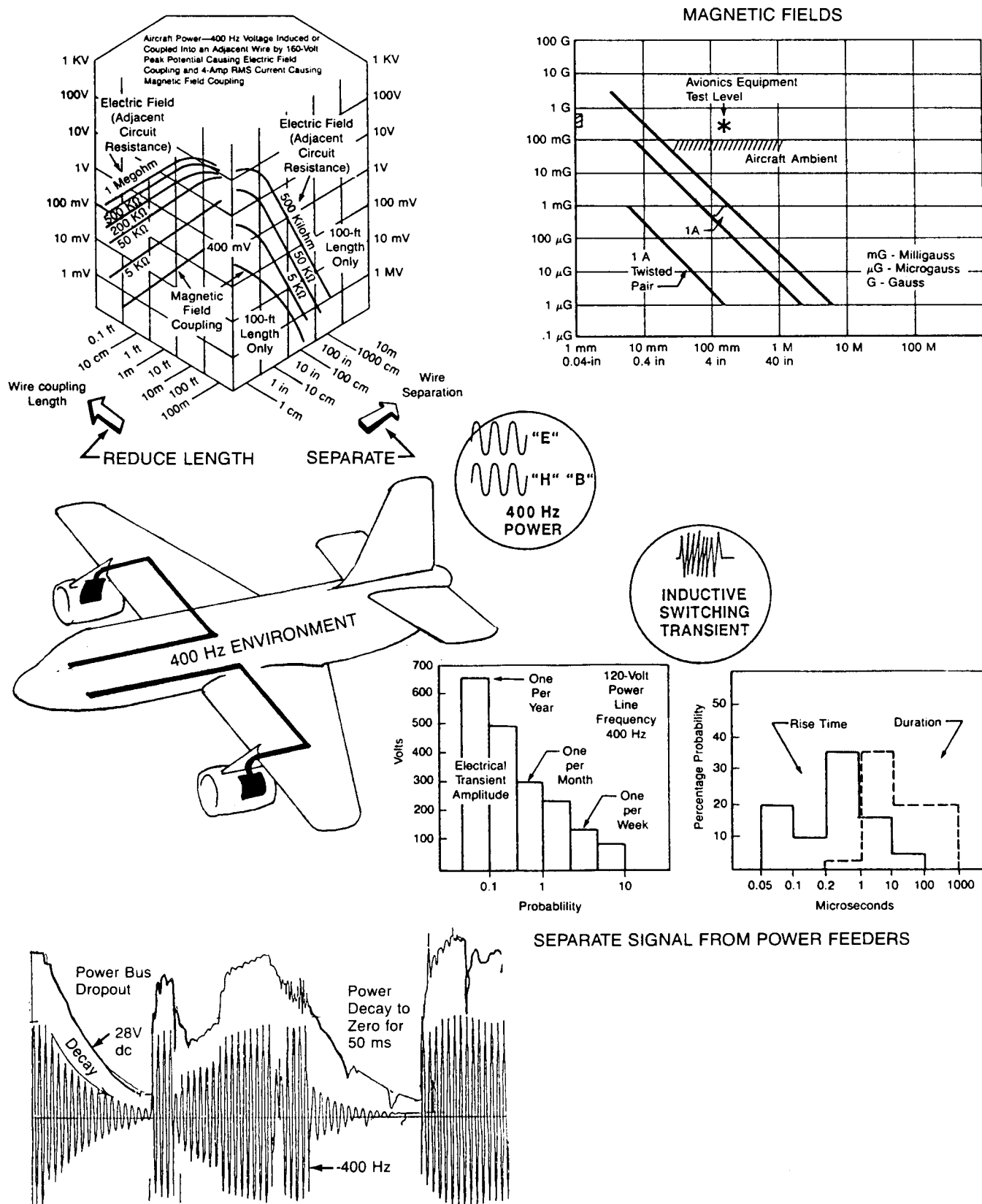
Figure 4.3-2 Trade—Wire Length/Separation
