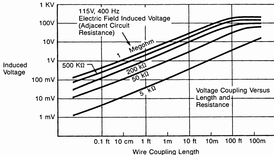
Figure 1.3-1 Representative "E" Field Coupling
