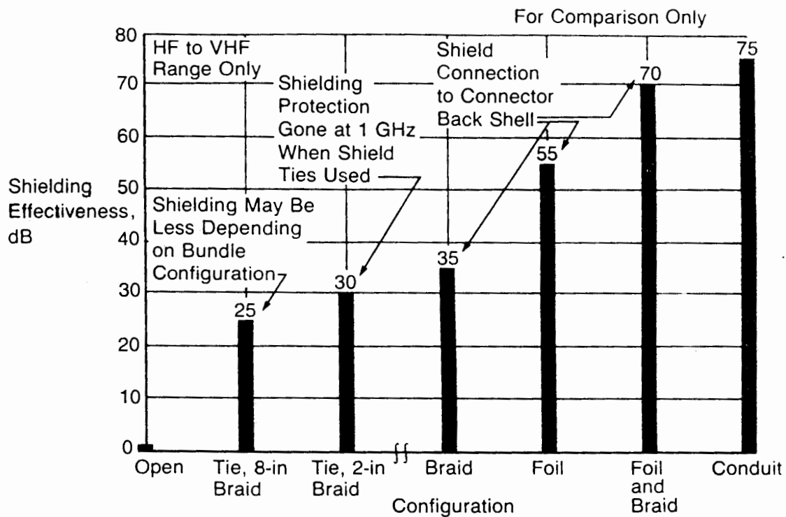
Figure 3.5-9 Wire SE Comparison at HF-VHF
