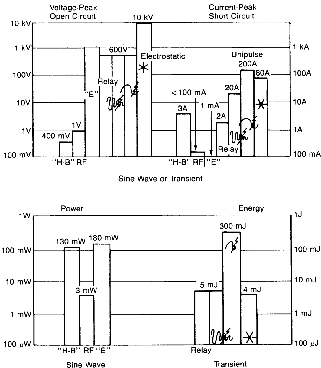
Figure 3.4-4 Selected EMI Levels
