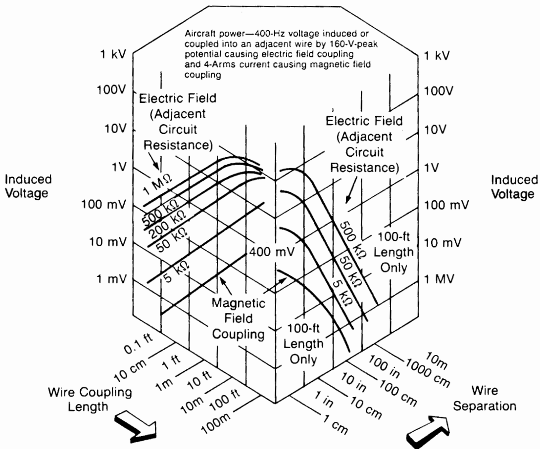
Figure 4.1-11 Coupling Versus Separation
