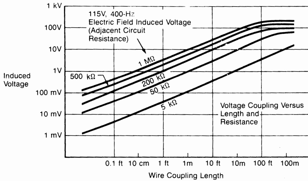
Figure 4.1-10 "E" Field Coupling
