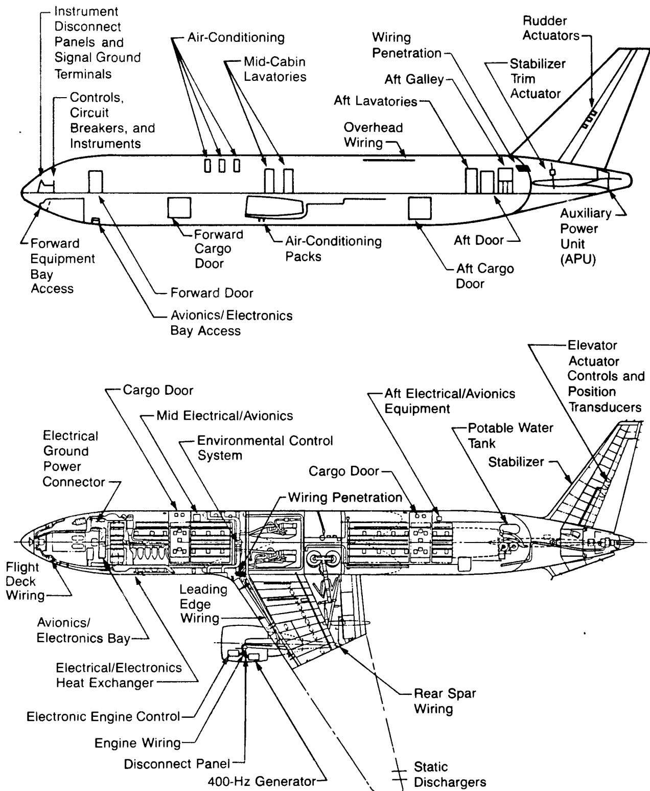
Figure 2.1-1 Present-Day Aircraft Systems
