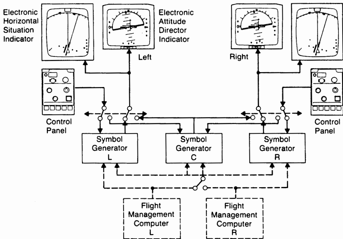
Figure 2.1-13 Flight Instrument System
