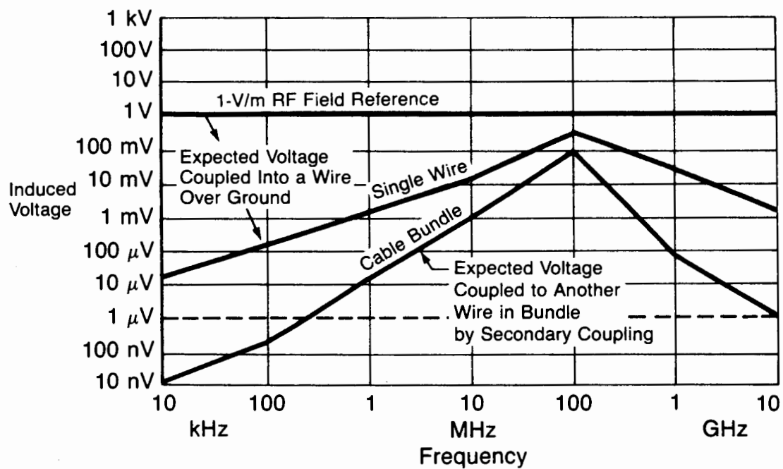
Figure 4.1-7 Representative Secondary Coupling
