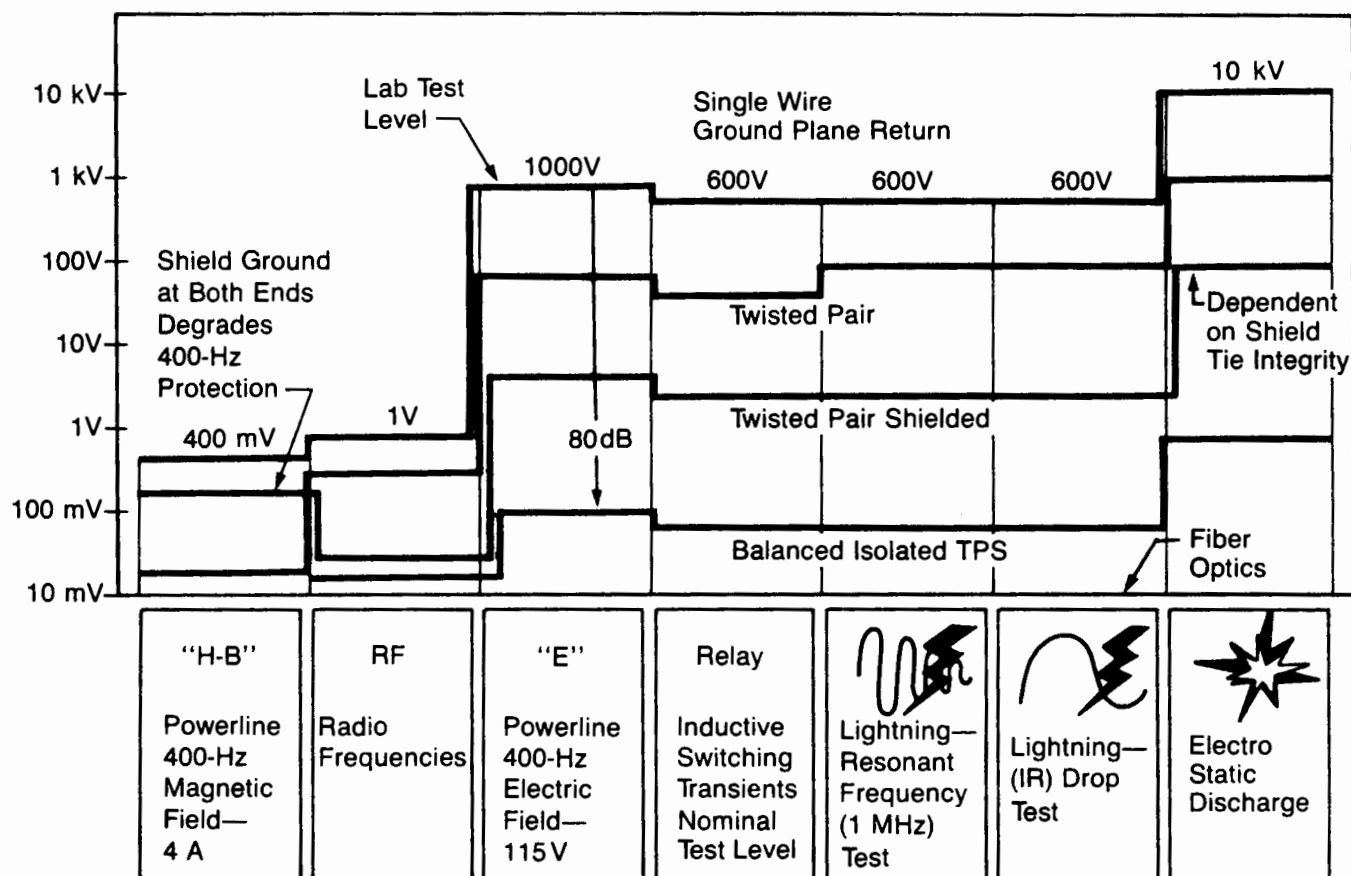
Figure 3.4-1 Circuit Response to EMI
