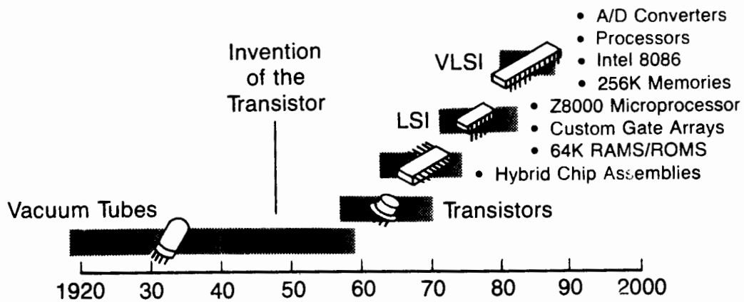
Figure 2.2-8 Microprocessor Evolution
