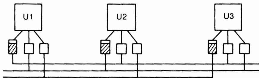
(a) ARINC 429
