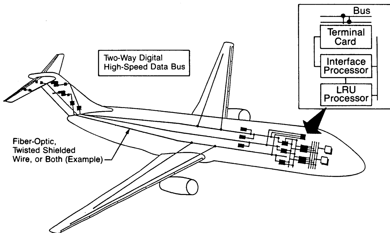
Figure 2.2-2 Data Bus Architecture
