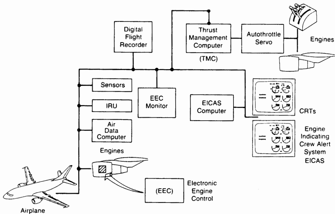
Figure 2.1-11 Electronic Engine Control
