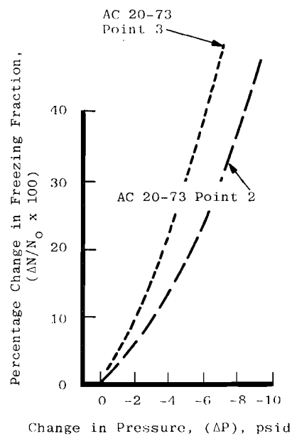
FIGURE 20. PERCENTAGE CHANGES IN THE SCALING PARAMETERS AS STATIC PRESSURE CHANGES FOR AN NACA 0012 AIRFOIL (6.0-IN. CHORD) AT 200 FT/SEC FLOW VELOCITY.
