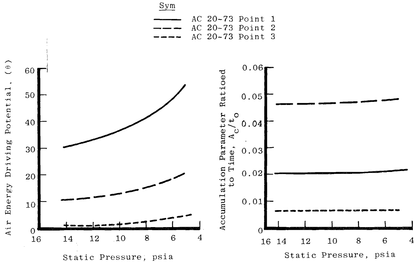
d. Effect on the accumulation parameter ratioed to time
