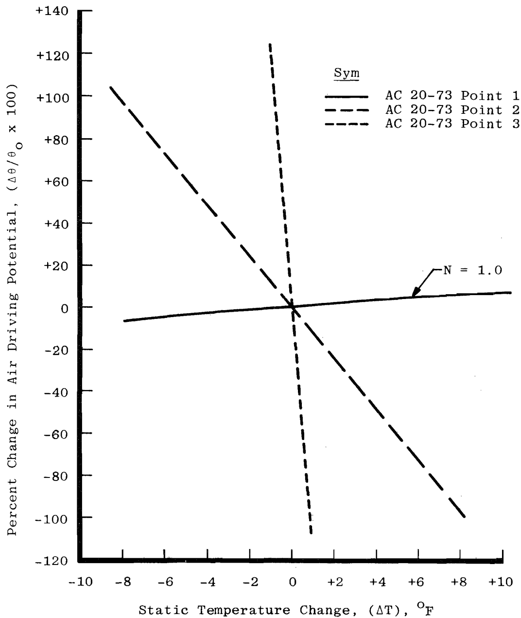
FIGURE 16. PERCENTAGE CHANGE IN AIR DRIVING POTENTIAL AS THE TEST CONDITIONS CHANGE FOR AN NACA 0012 AIRFOIL (6.0-IN. CHORD) AT 200 FT/SEC FLOW VELOCITY.
