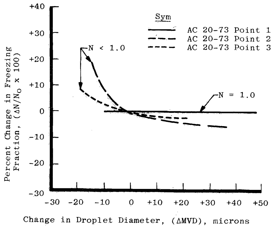
FIGURE 14. PERCENTAGE CHANGE IN FREEZING FRACTION AS TEST CONDITIONS CHANGE FOR AN NACA 0012 AIRFOIL (6.0-IN CHORD) AT 200 FT/SEC FLOW VELOCITY (CONCLUDED).
