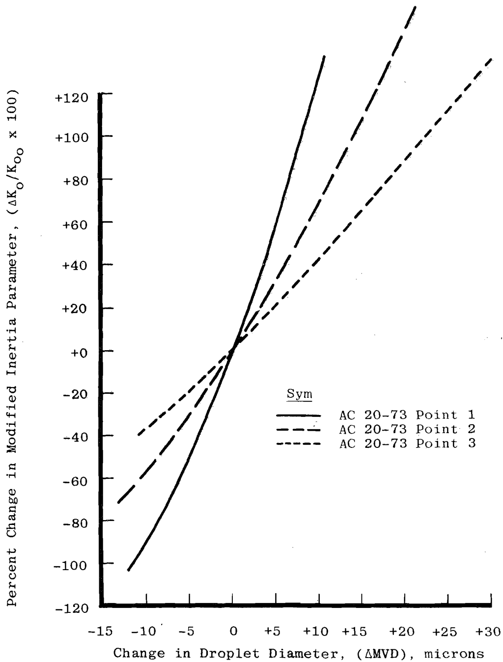
FIGURE 12. PERCENTAGE CHANGE IN MODIFIED INERTIA PARAMETER VERSUS CHANGE IN DROP SIZE FOR AN NACA 0012 AIRFOIL (6.0-IN. CHORD).
