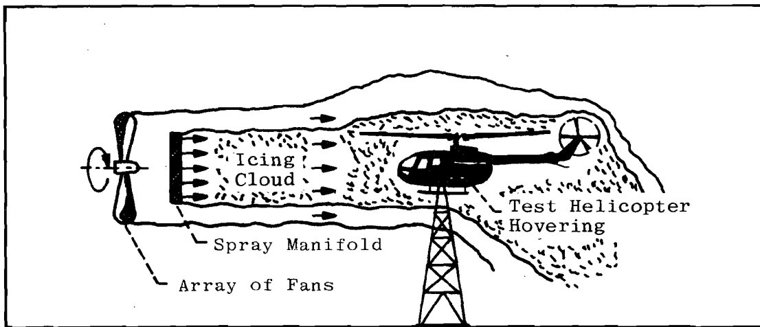
c. Fan blown spray in a large room or outdoors
