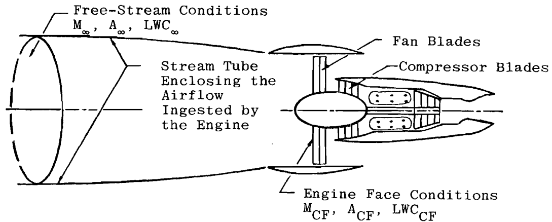
FIGURE 2. SCHEMATIC SHOWING POSSIBLE STREAM TUBE CONFIGURATION FOR TURBOFAN ICING CONDITIONS (TAKEN FROM AEDC-TR-73-144).
