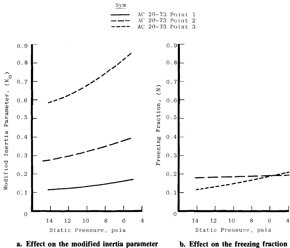
FIGURE 19. EFFECT OF STATIC PRESSURE ON THE SCALING PARAMETERS FOR AN NACA 0012 AIRFOIL (6.0-IN. CHORD) AT 200 FT/SEC FLOW VELOCITY.
