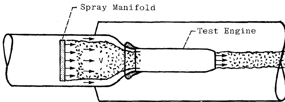
a. Direct connect
