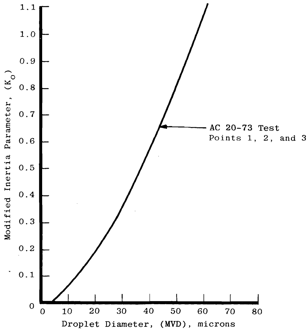
FIGURE 7. EFFECT OF DROP SIZE ON THE MODIFIED INERTIA PARAMETER FOR AN NACA 0012 AIRFOIL (6.0-IN. CHORD) AT 200 FT/SEC FLOW VELOCITY.
