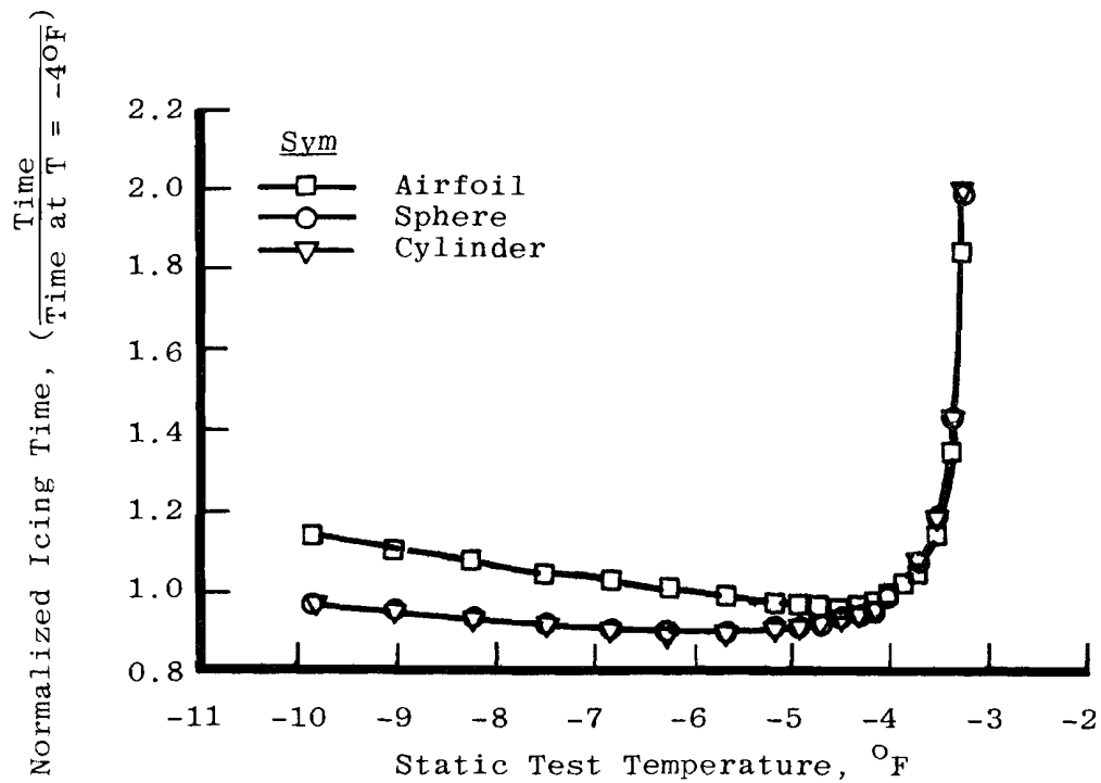
FIGURE 4. ICING CONDITION VARIABLE CHANGES REQUIRED FOR SIMILITUDE AT VARIOUS ICING TEMPERATURES FOR AC 20-73 POINT 1 (CONCLUDED).
