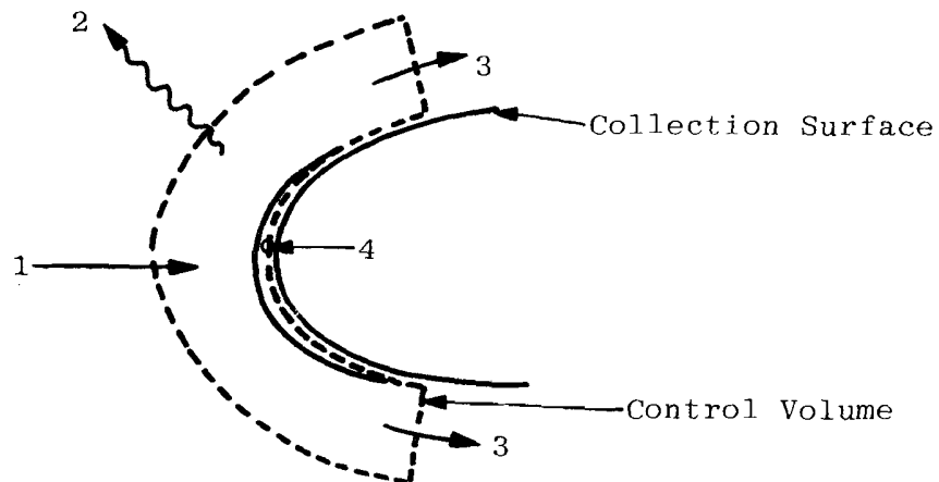
Mass Balance, Icing Surface
