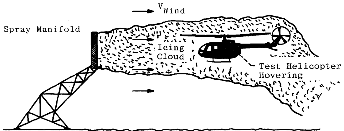
d. Windblown sprays in an outdoor facility
