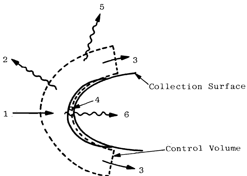
Energy Balance, Unheated Icing Surface
