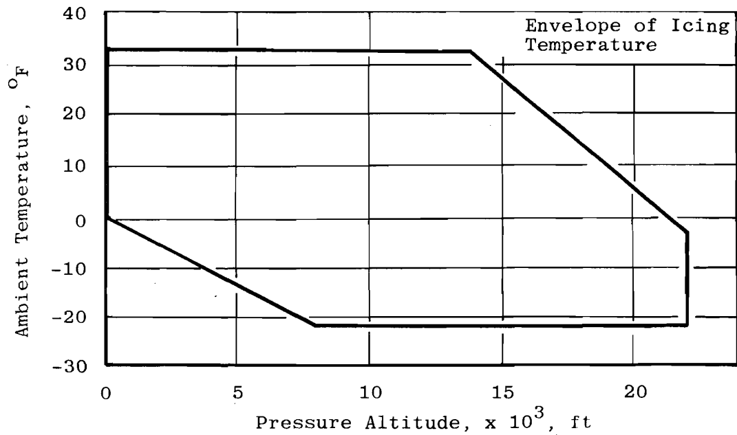
a. Continuous maximum (stratiform clouds) FIGURE 1. CLOUD ICING CONDITIONS.
