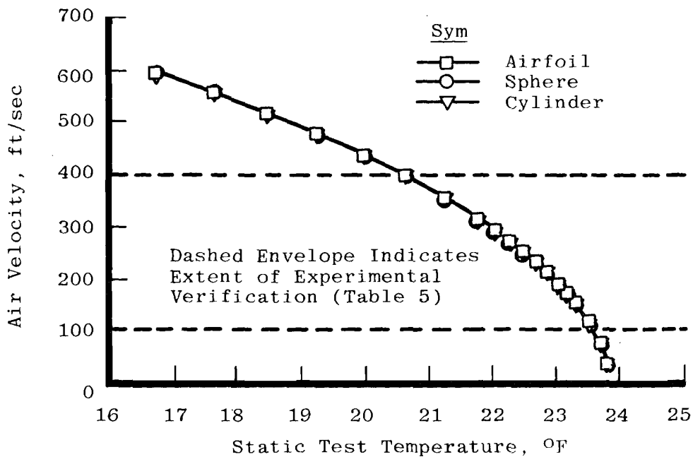
FIGURE 5. ICING CONDITION VARIABLE CHANGES REQUIRED FOR SIMILITUDE AT VARIOUS ICING TEMPERATURES FOR AC 20-73 POINT 2.
