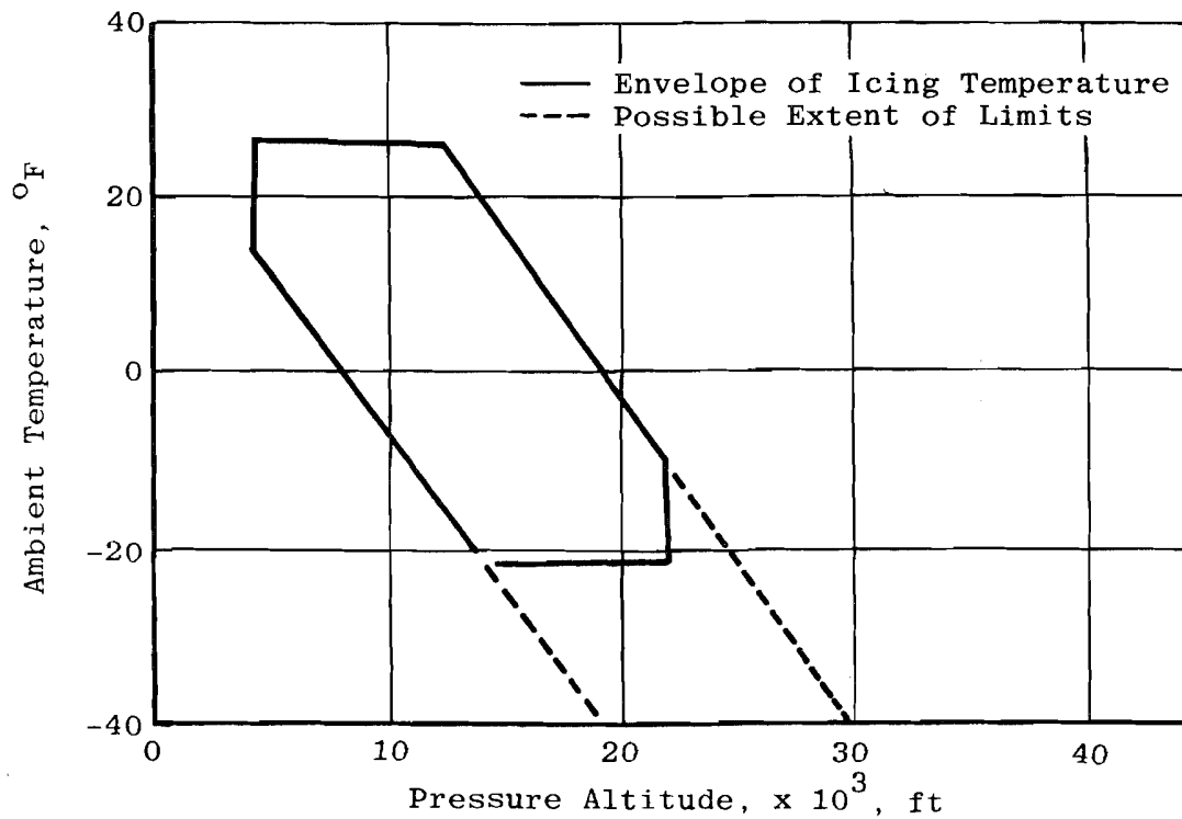
b. Intermittent maximum (cumuliform clouds) FIGURE 1. CLOUD ICING CONDITIONS (CONCLUDED).
