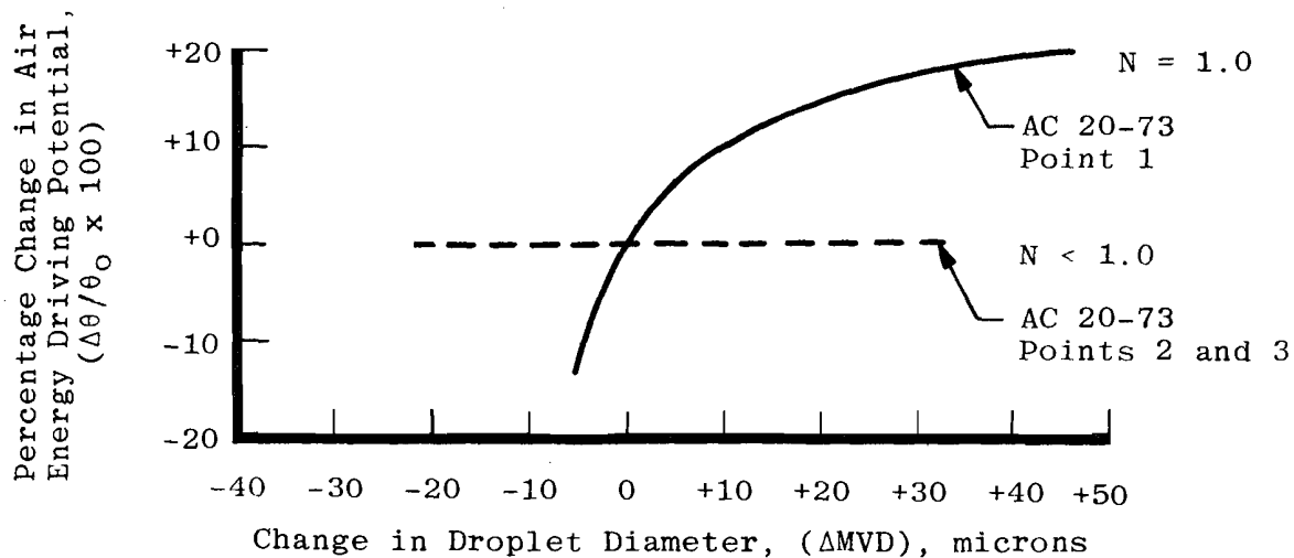
c. Effect of drop size
