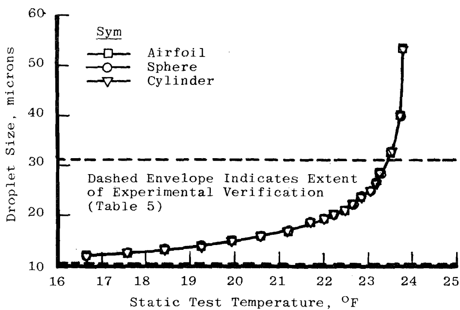
FIGURE 5. ICING CONDITION VARIABLE CHANGES REQUIRED FOR SIMILITUDE AT VARIOUS ICING TEMPERATURES FOR AC 20-73 POINT 2 (CONTINUED).
