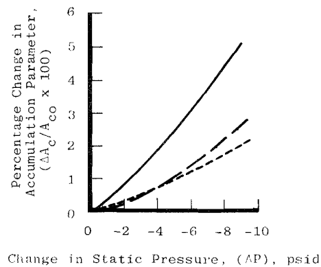
FIGURE 20. PERCENTAGE CHANGES IN THE SCALING PARAMETERS AS STATIC PRESSURE CHANGES FOR AN NACA 0012 AIRFOIL (6.0-IN. CHORD) AT 200 FT/SEC FLOW VELOCITY (CONCLUDED).
