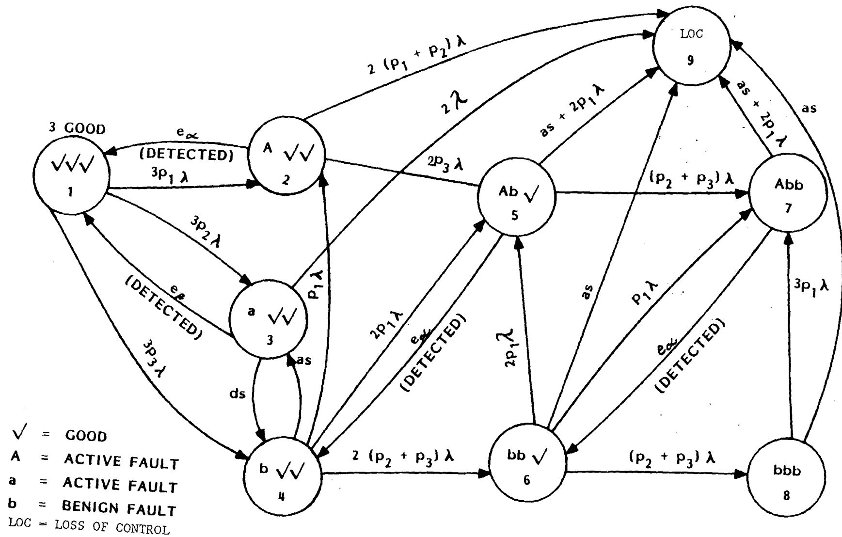
Figure 2. Multiple-Fault Model for a Multiprocessor System (with a single auxiliary software program)
