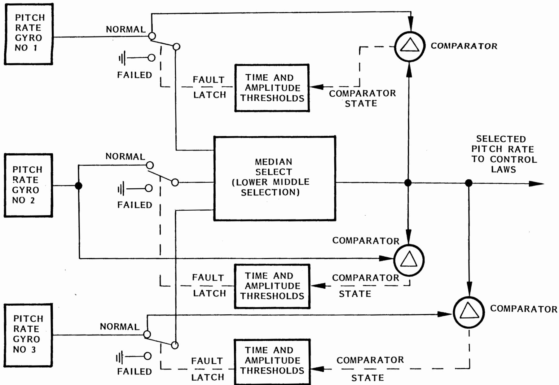
Figure 5. Triple Sensor Voter /Comparator
