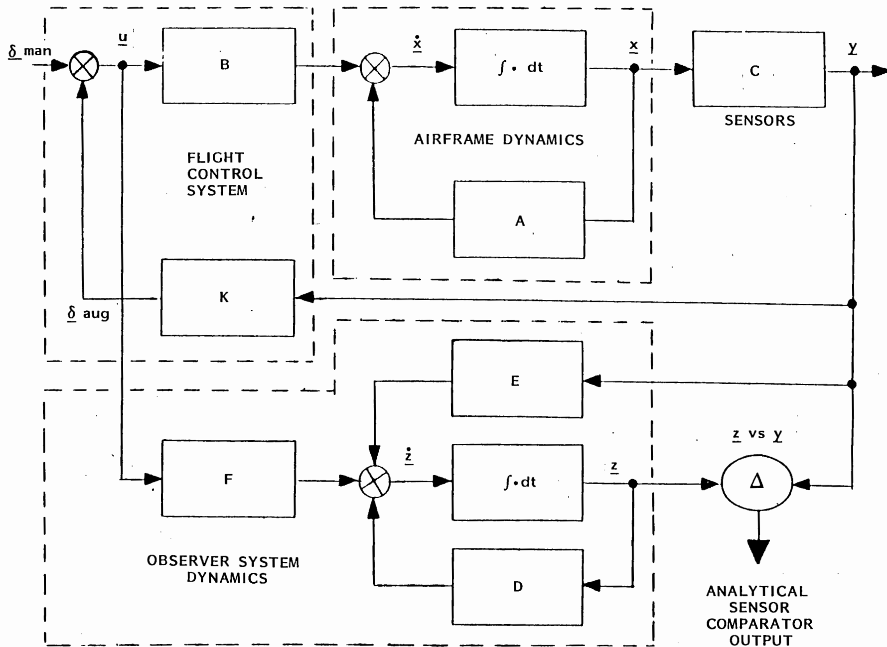
Figure 7. Observer System Sensor Fault Detection (Sheet 1 of 2)
