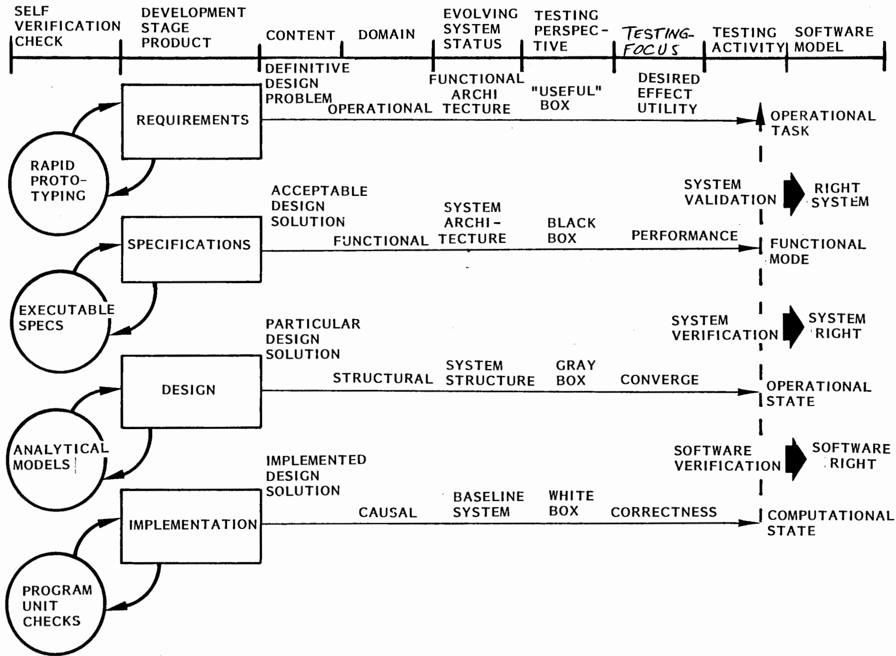
Figure 6. Multi-Level Testing Closure
