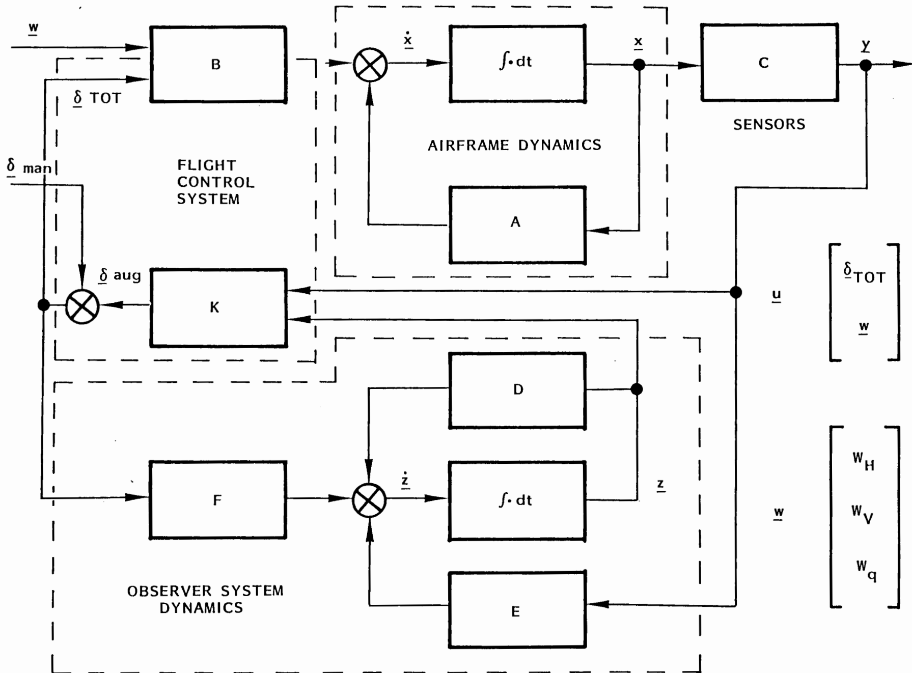
Figure 11. Observer Filtering Block Diagram
