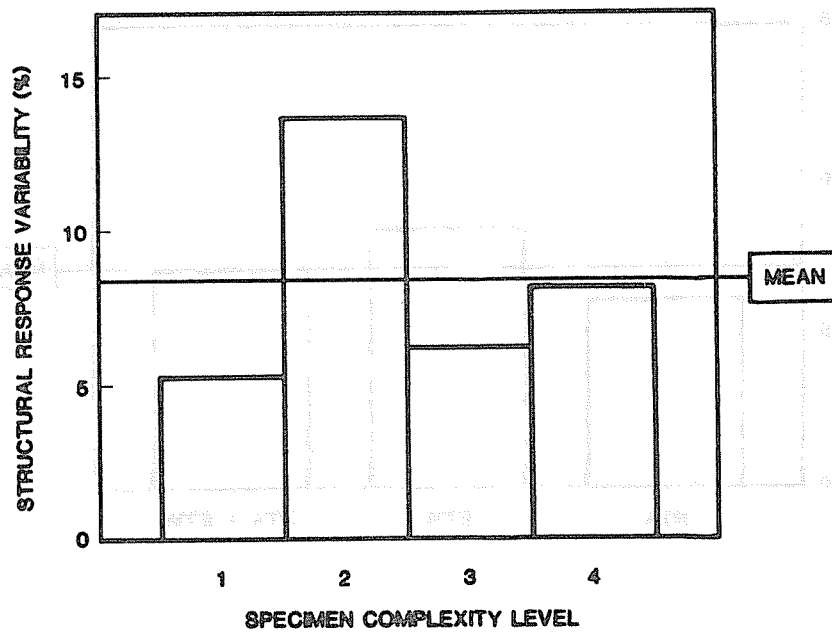
FIGURE 66. INFLUENCE OF SPECIMEN COMPLEXITY LEVEL ON ETW STRUCTURAL RESPONSE VARIABILITY.
