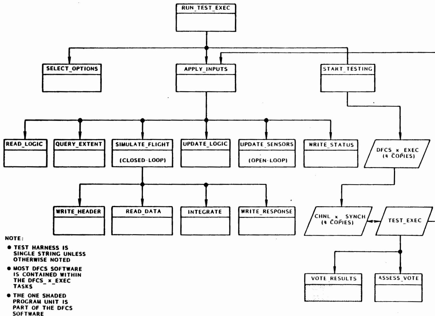
Figure 23 - Overall Test Program Call Graph
