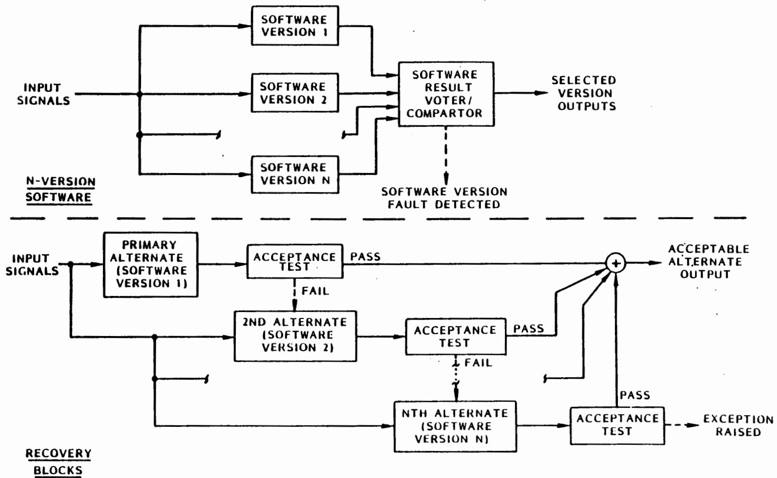
Figure 3 - Approaches to Software Fault Tolerance
