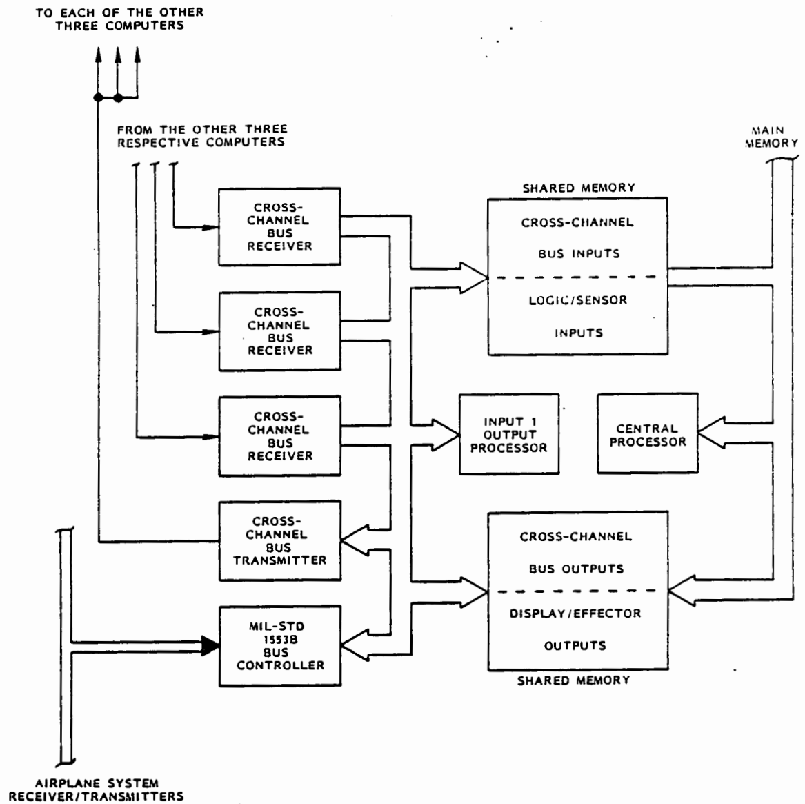
Figure 9 - Computer Input/Output Organization (Same for All Computers)
