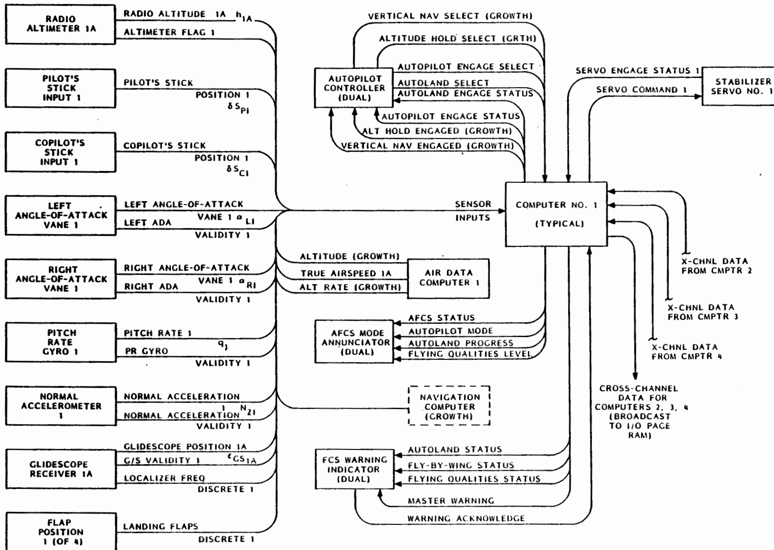
Figure 7 - System Signal Flow Diagram (Typical Channel)
