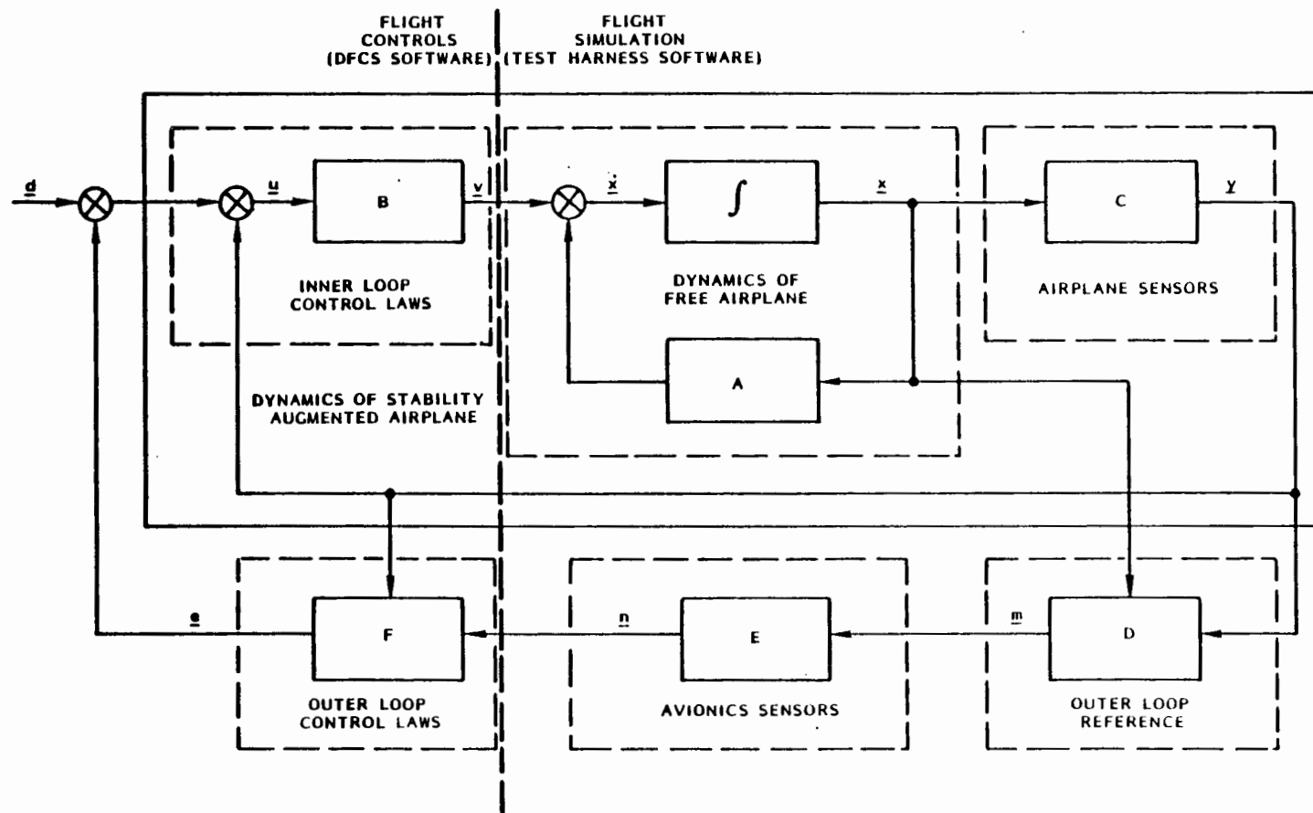
Figure 27 - Closed-Loop Simulation Block Diagram
