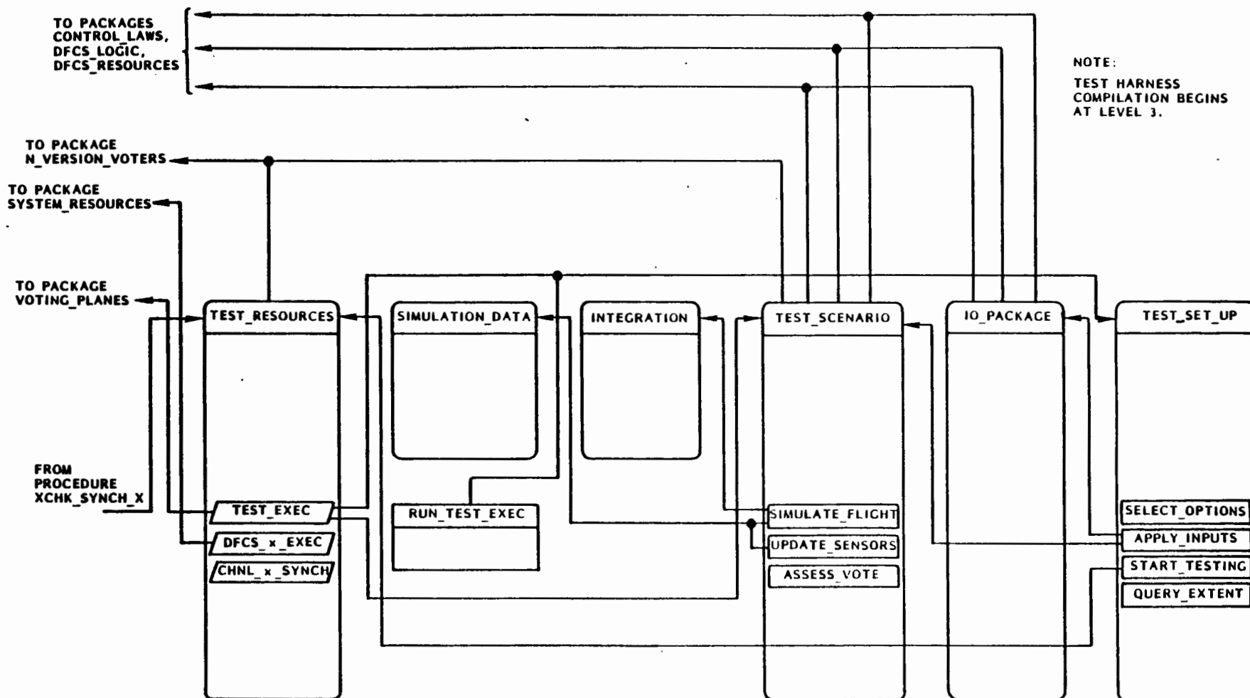
Figure 29 - Overall Compilation Dependencies (2 of 2)
