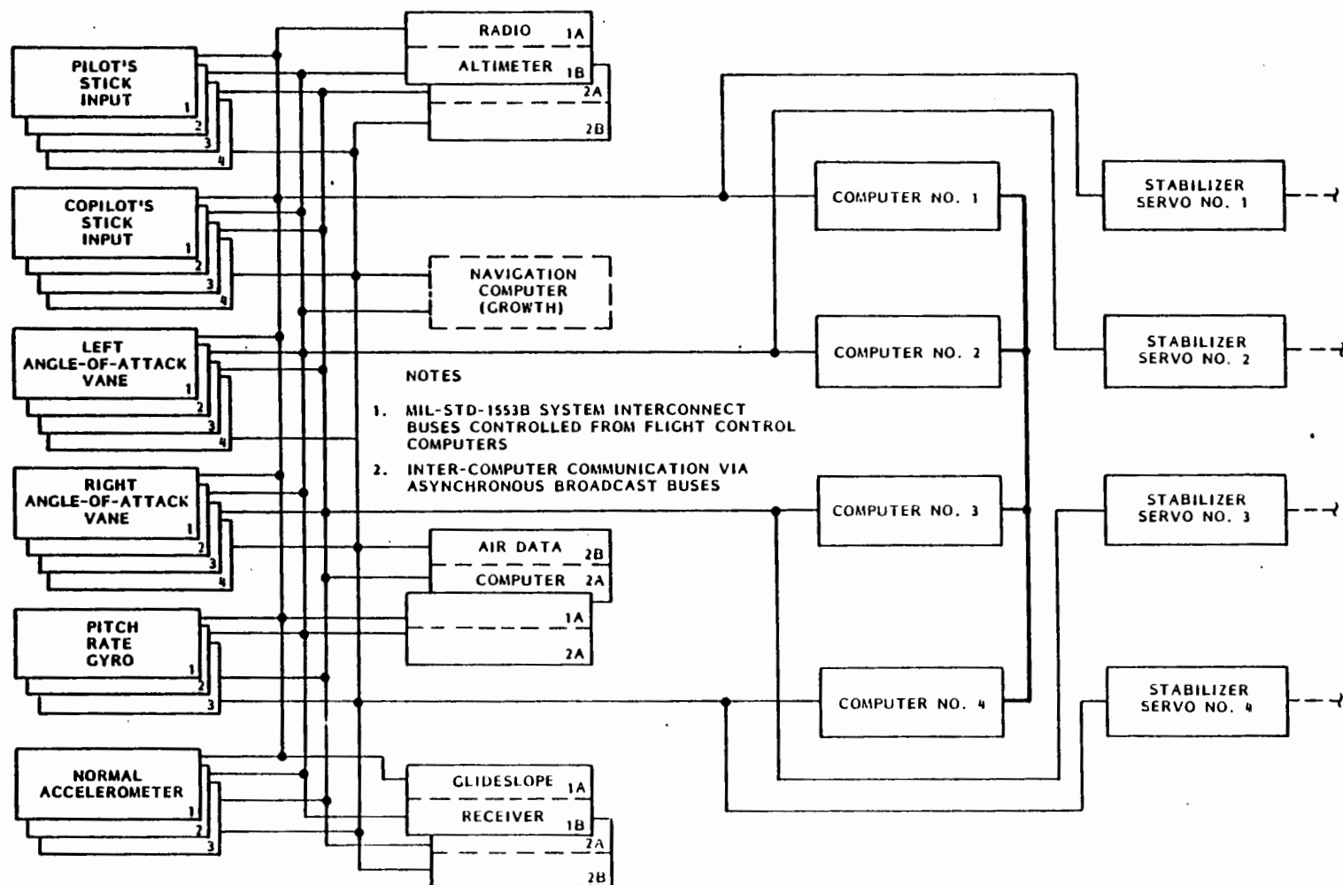
Figure 5 - System Block Diagram
