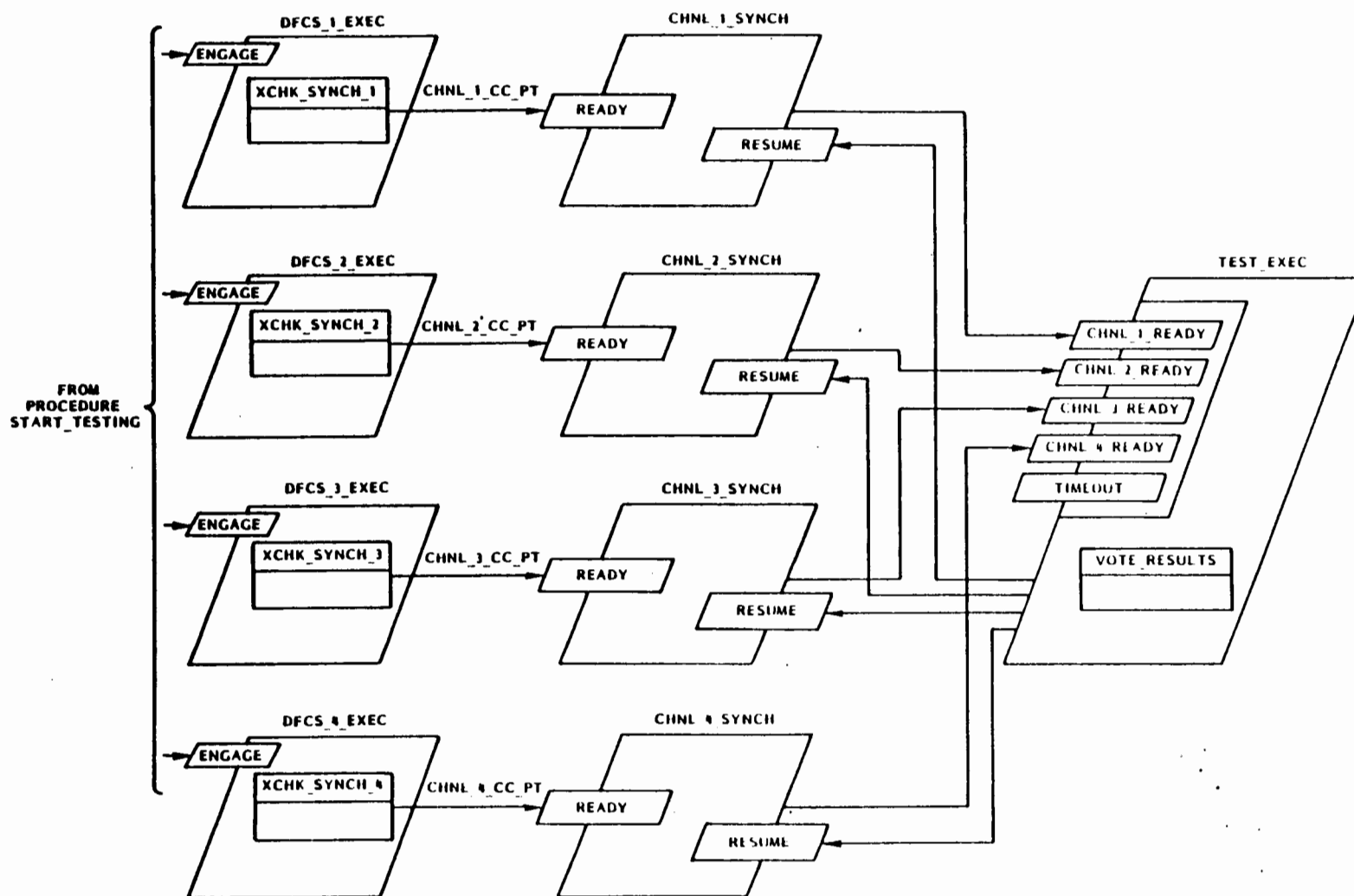
Figure 26 - Ada Multitasking Communication
