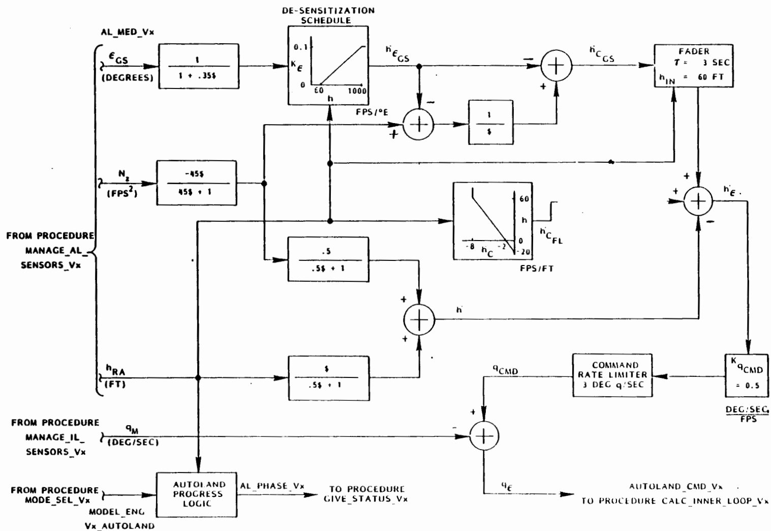
Figure 21 - Autoland Control Law Block Diagram
