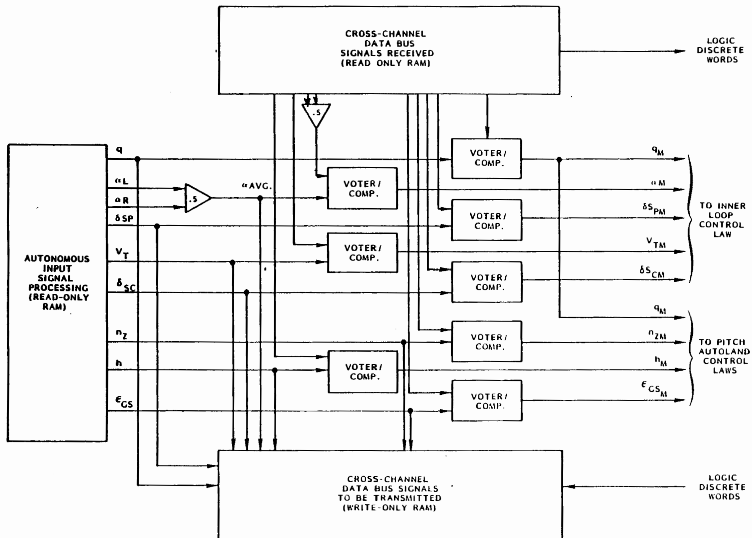
Figure 11 - Software Input Signal Flow
