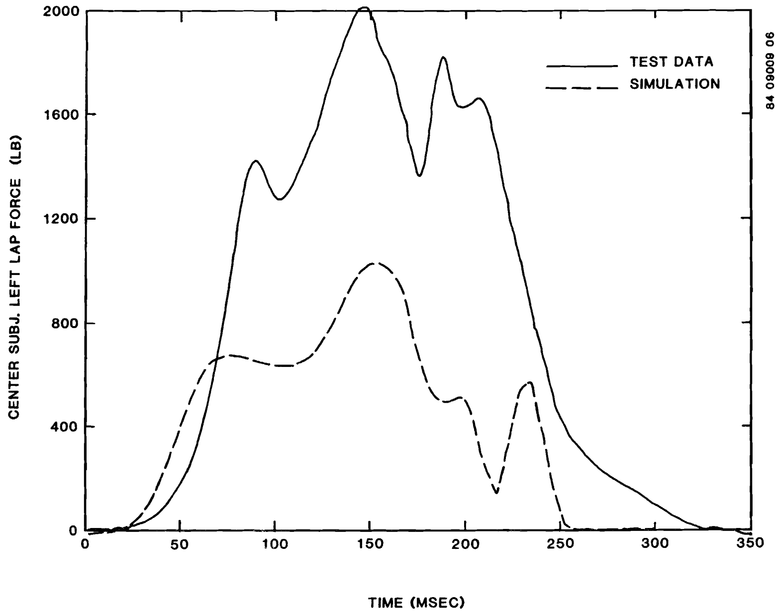
Figure 51. Modified transport aircraft seat, CAMI Test A83-085, center occupant left lap belt load.
