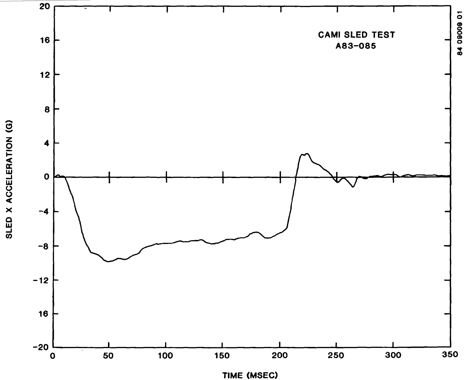
Figure 38. Sled deceleration, CAMI-modified transport aircraft seat Test A83-085.
