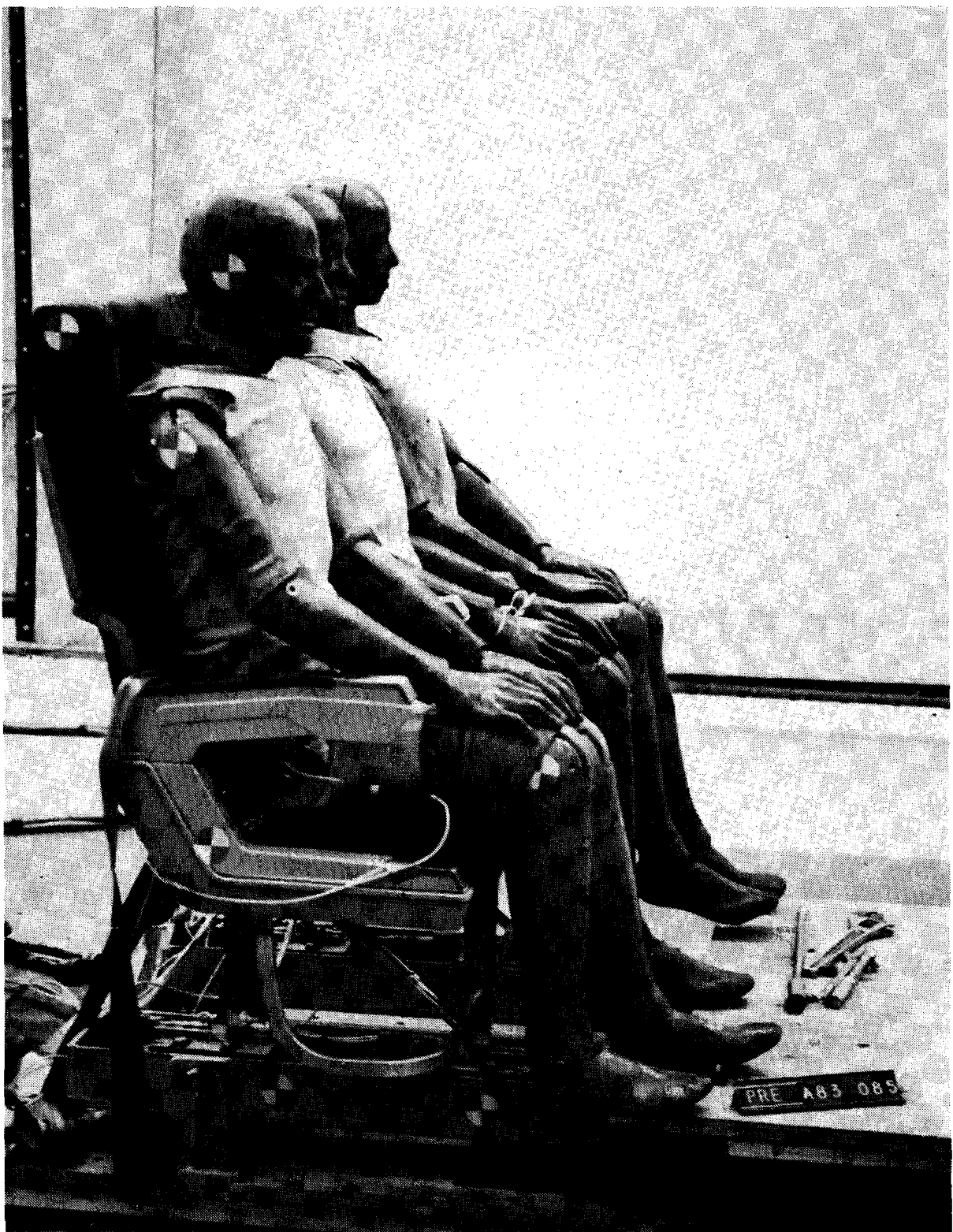
Figure 39. Modified transport aircraft seat and dummies prior to CAMI Test A83-085 (before floor warping).
