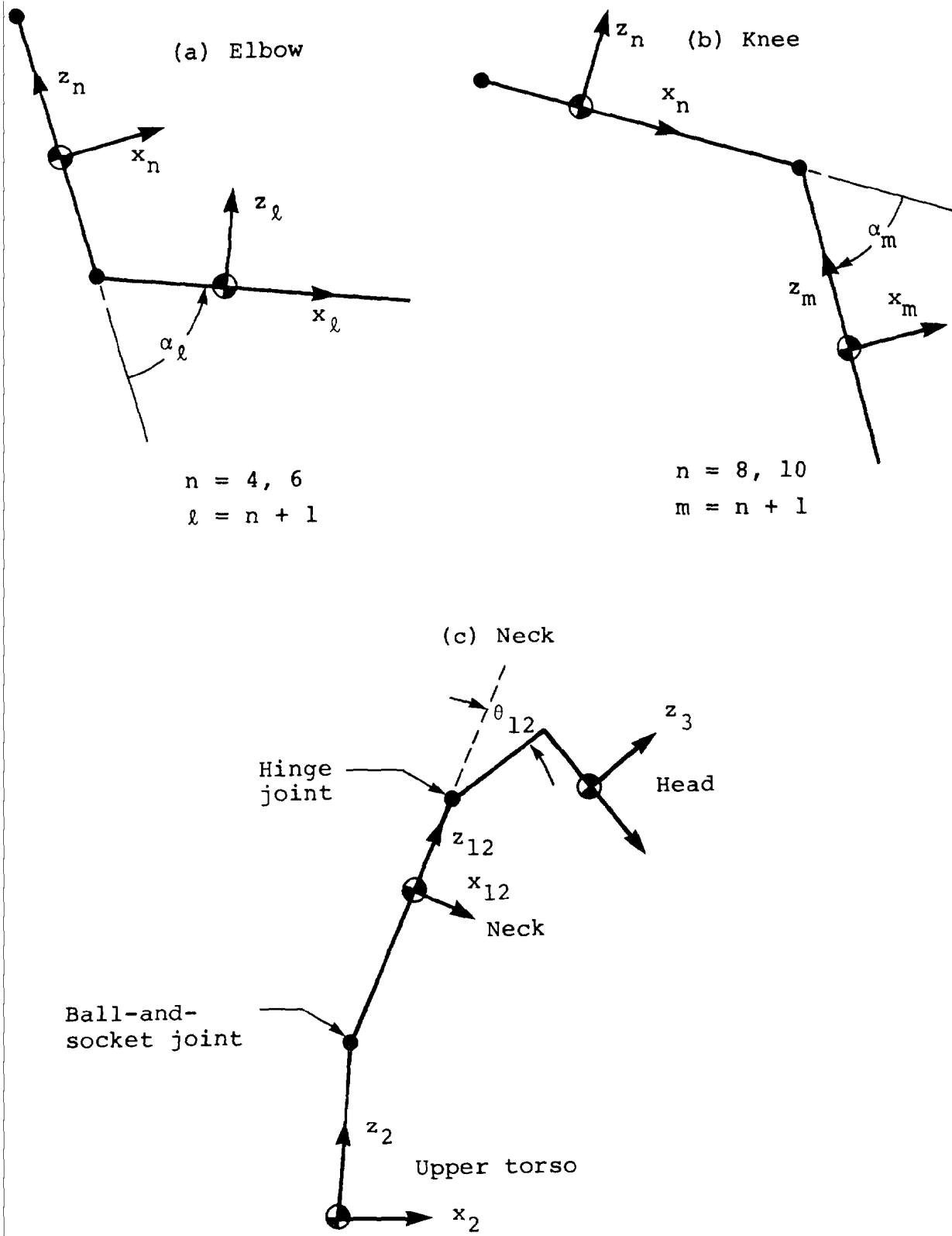
Figure 4. Definition of angular coordinates \alpha for elbows, knees, and neck.
