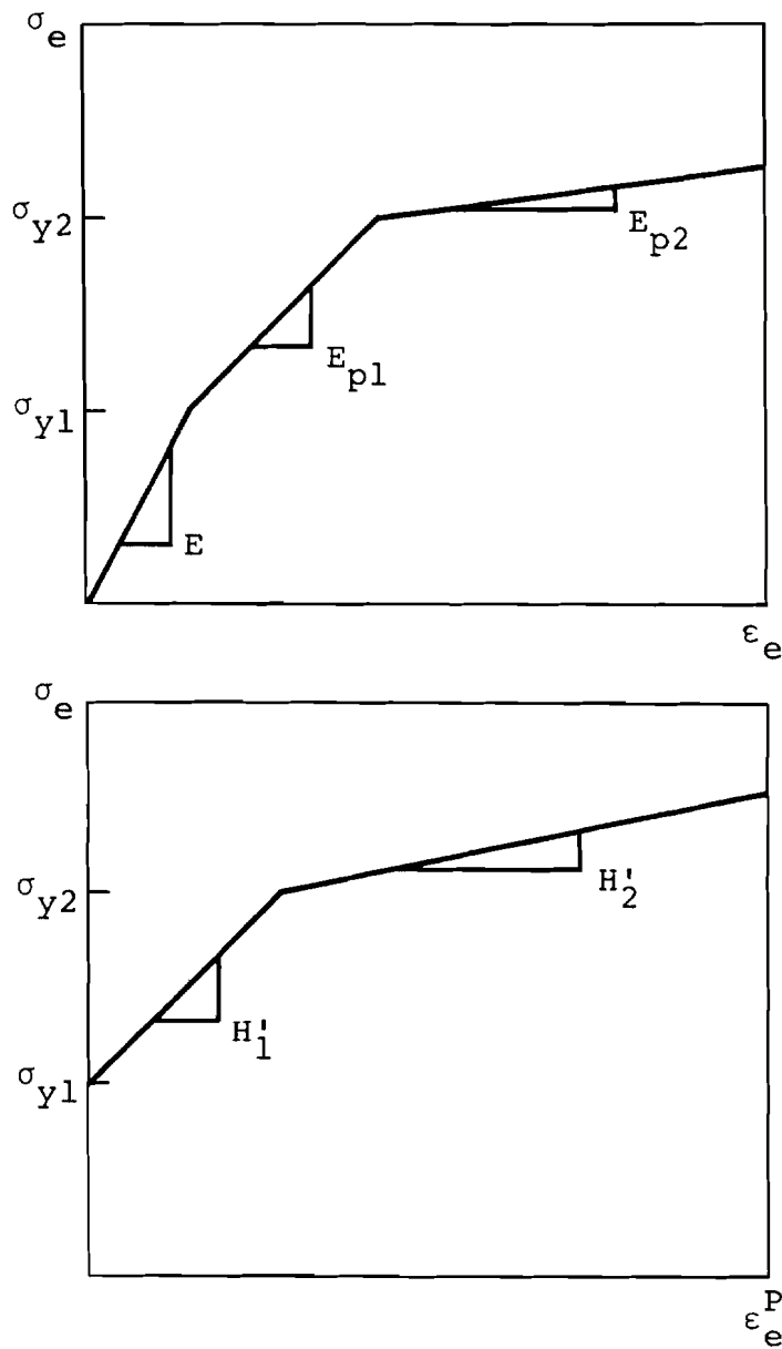
Figure 20. Trilinear stress-strain relation.
