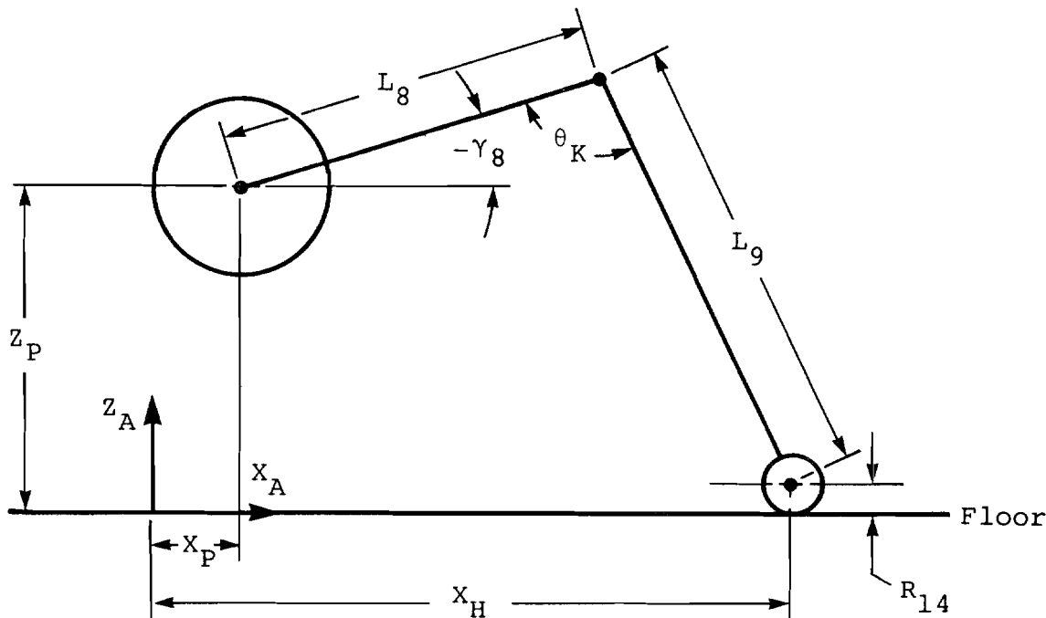
Figure 29. Leg position.
