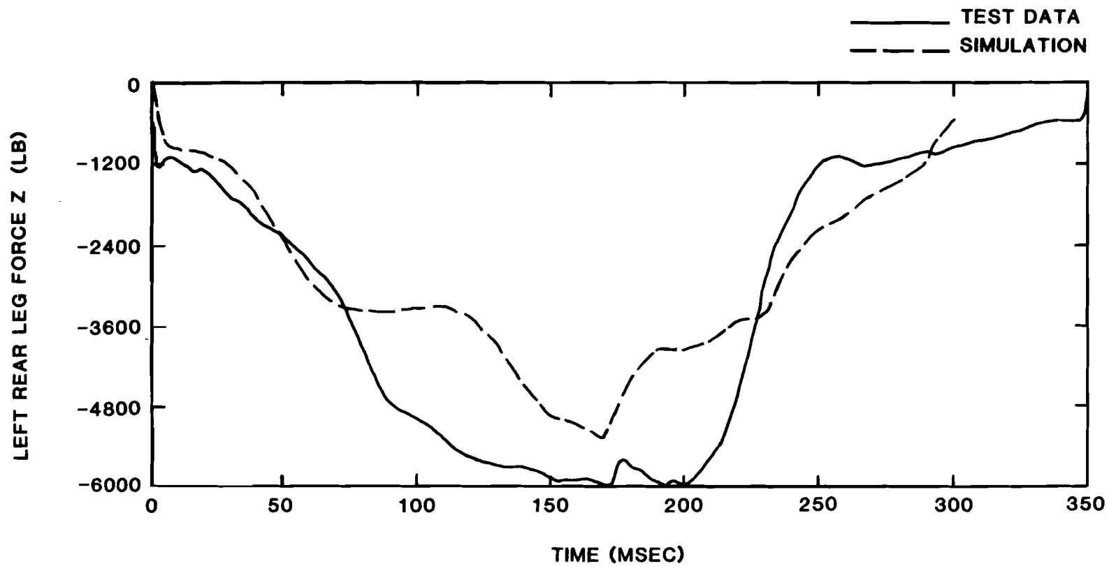
Figure 52. Modified transport aircraft seat, CAMI Test A83-085, left (underside) rear leg vertical reaction.
