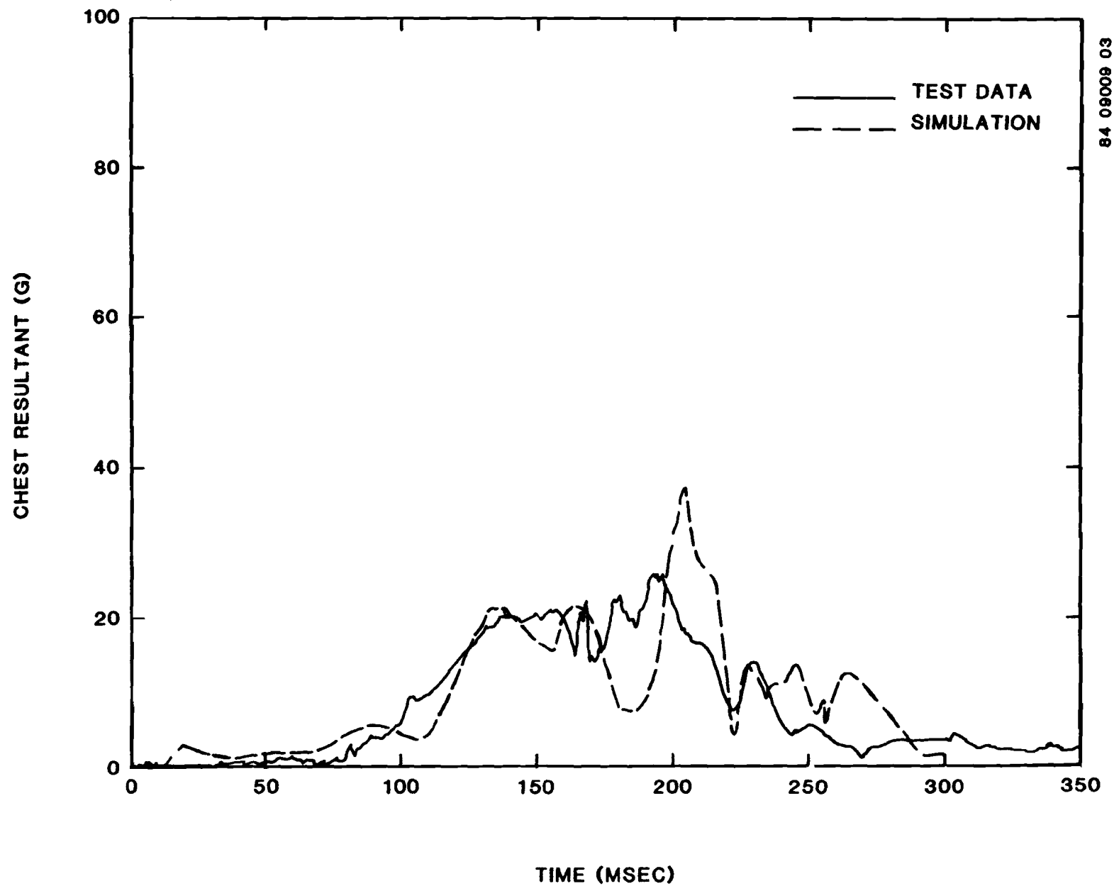
Figure 48. Modified transport aircraft seat, CAMI Test A83-085, chest (resultant) acceleration.
