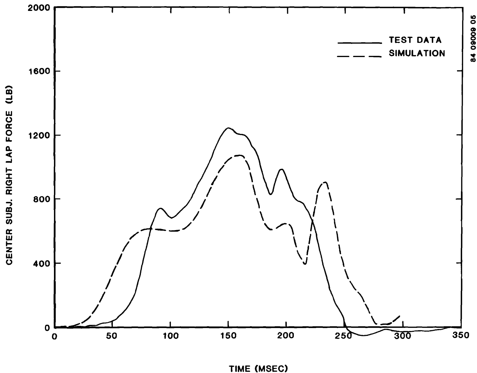
Figure 50. Modified transport aircraft seat, CAMI Test A83-085, center occupant right lap belt load.
