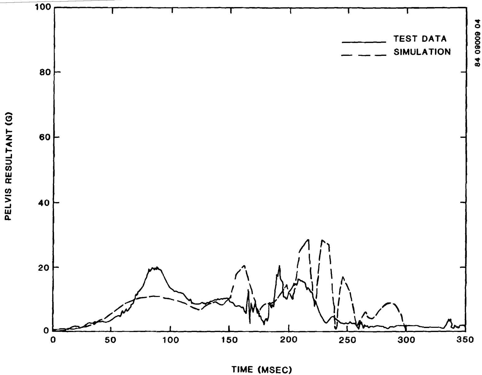
Figure 49. Modified transport aircraft seat, CAMI Test A83-085, pelvic (resultant) acceleration.
