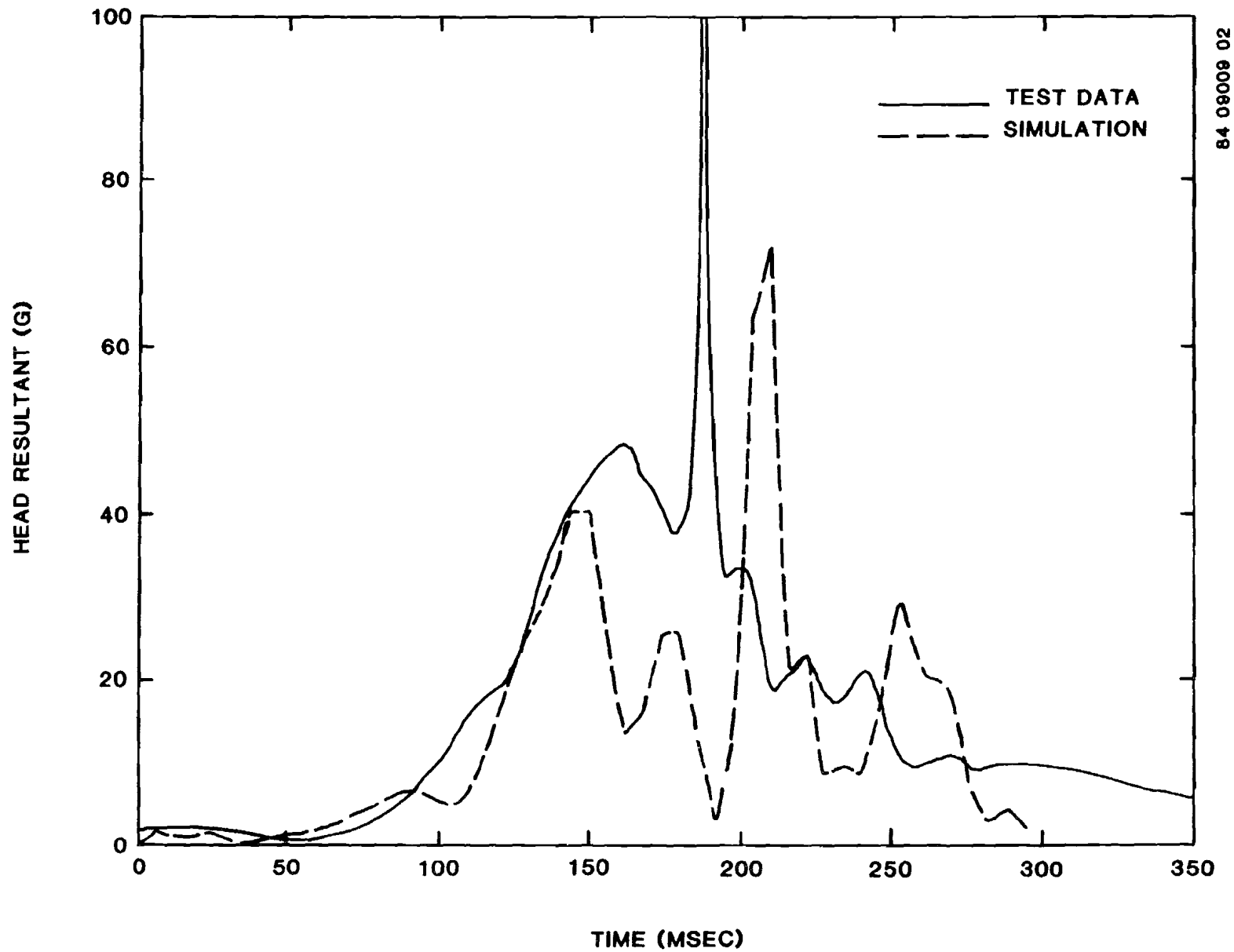
Figure 47. Modified transport aircraft seat, CAMI Test A83-085, head (resultant) acceleration.
