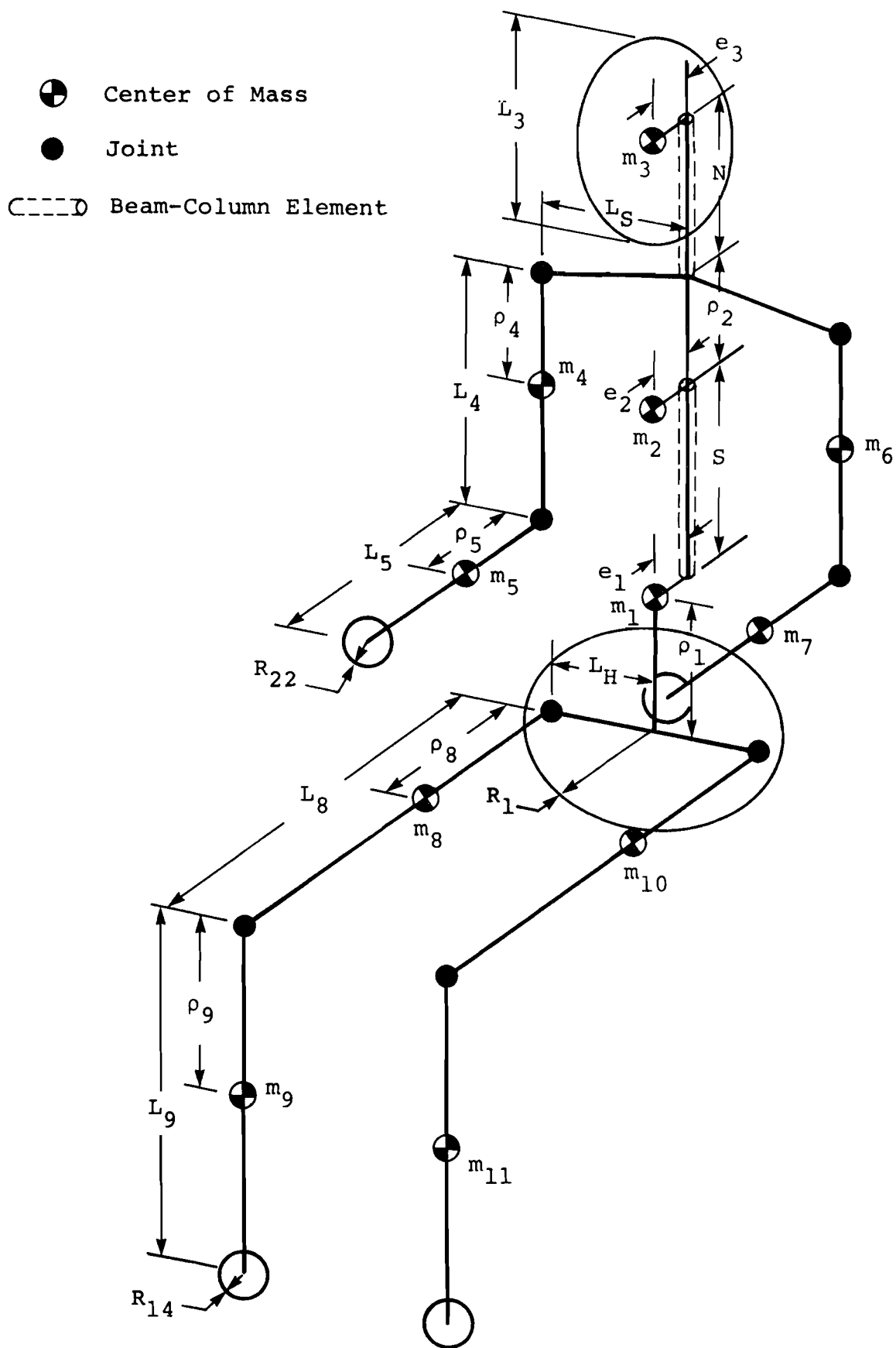
Figure 14. Program SOM-TA body segment dimensions.
