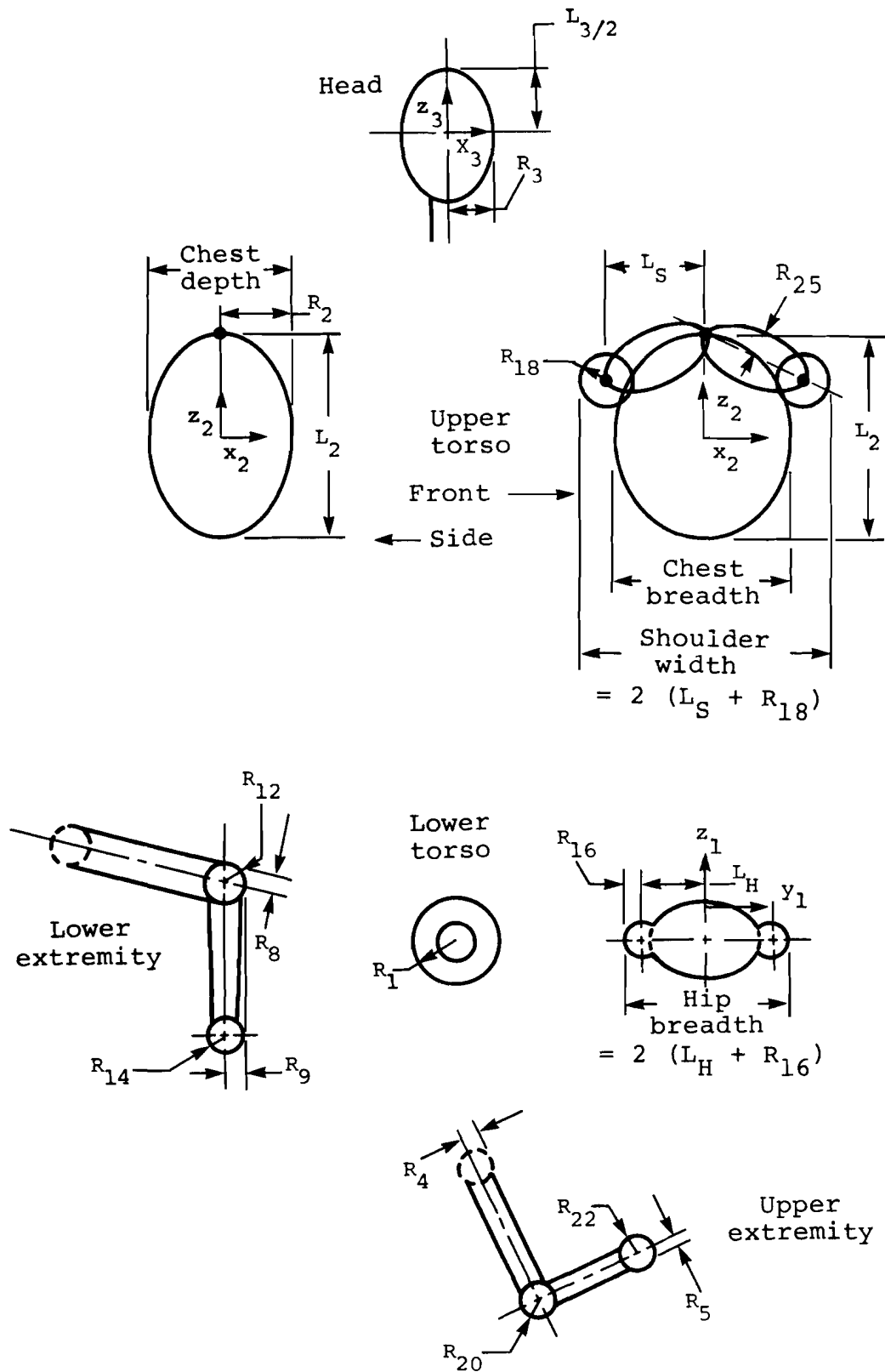
Figure 16. Body contact surface dimensions.
