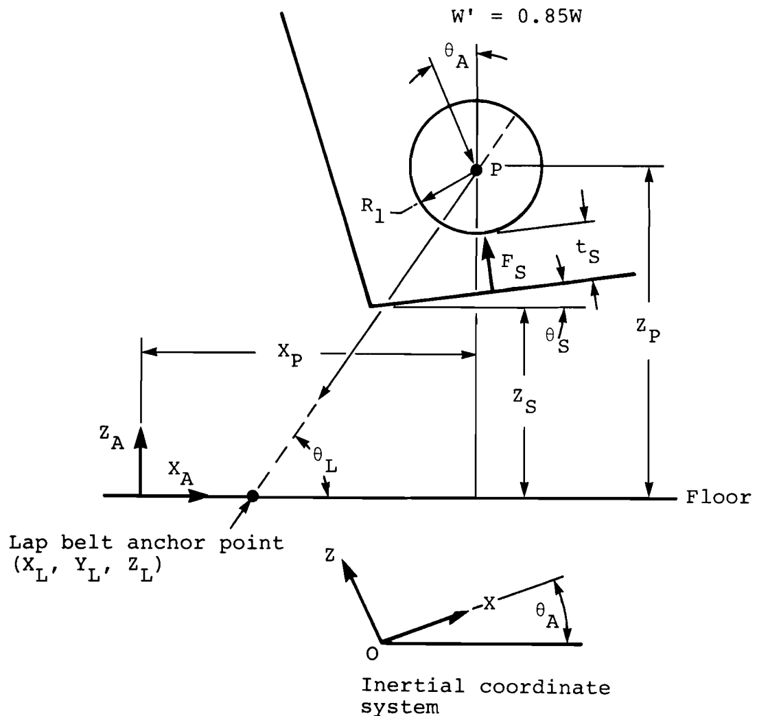
Figure 28. Forces acting on occupant torso (nose-down attitude).
