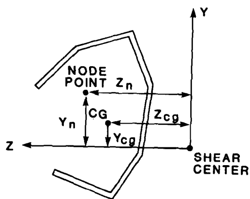
b) Cross-section geometry
