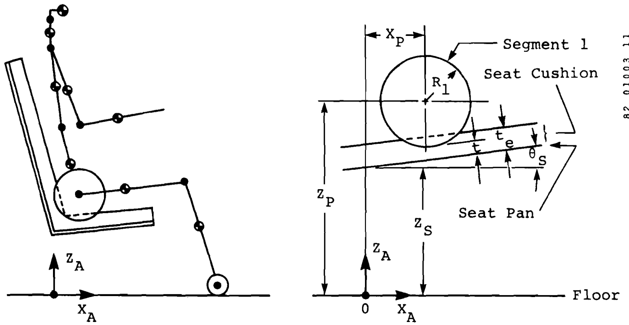
Figure 12. Seat cushion deflection.
