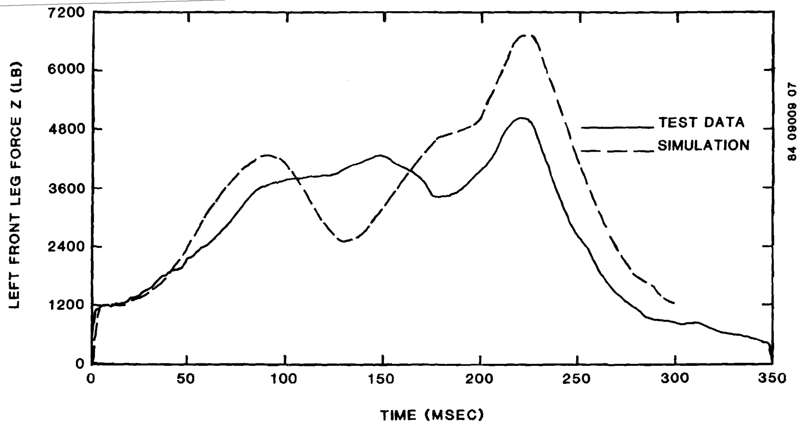
Figure 53. Modified transport aircraft seat, CAMI Test A83-085, left (underside) front leg vertical reaction.
