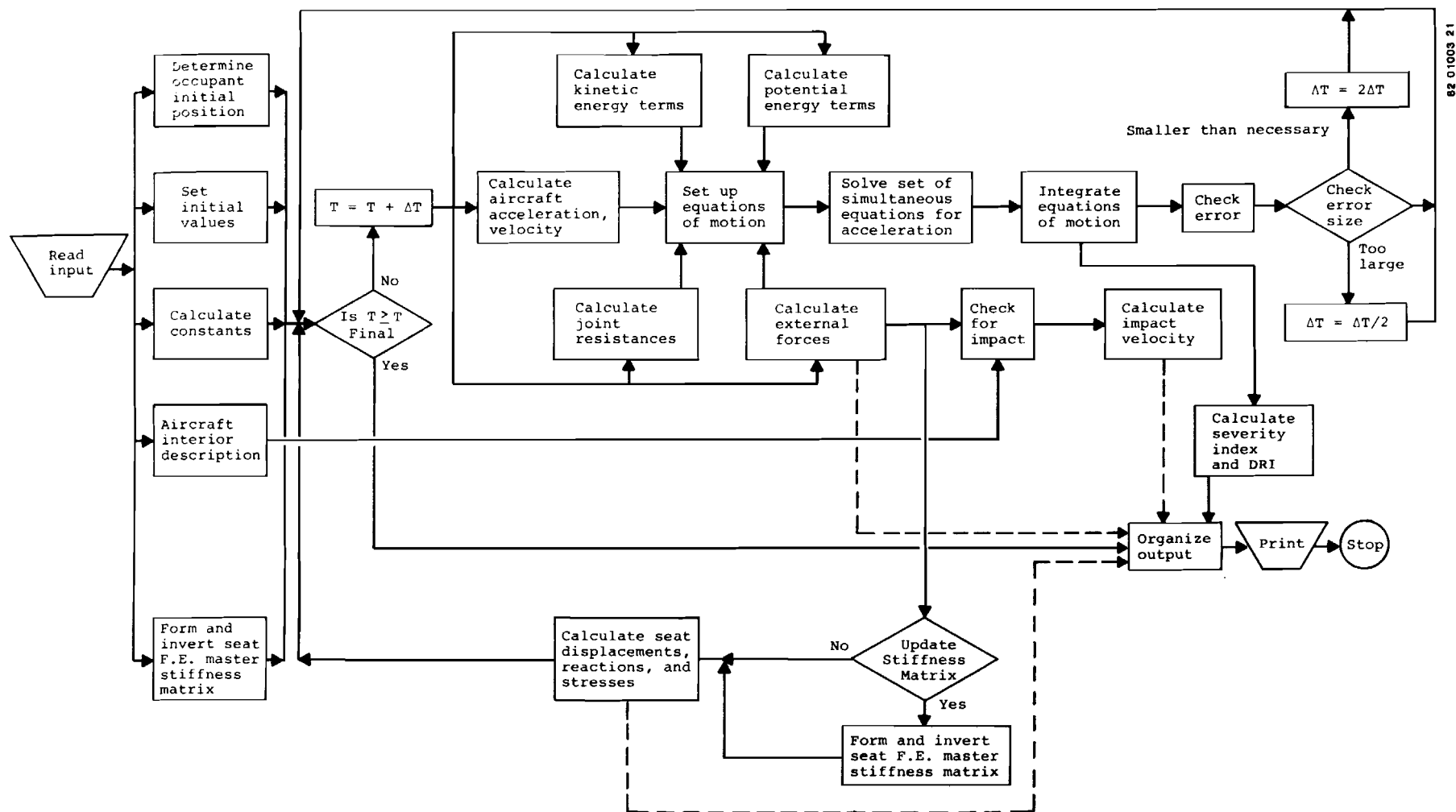
Figure 23. Program flow chart.
