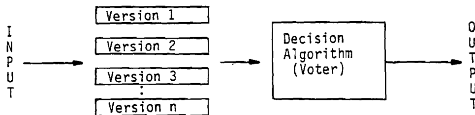
Figure 18. Basic N-Version Software
