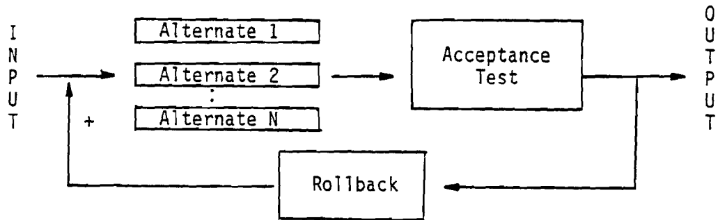
Figure 5. General Format of a Backward Recovery Block
