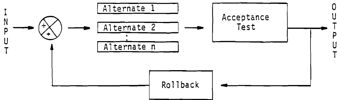
Figure 16. Basic Recovery Block
