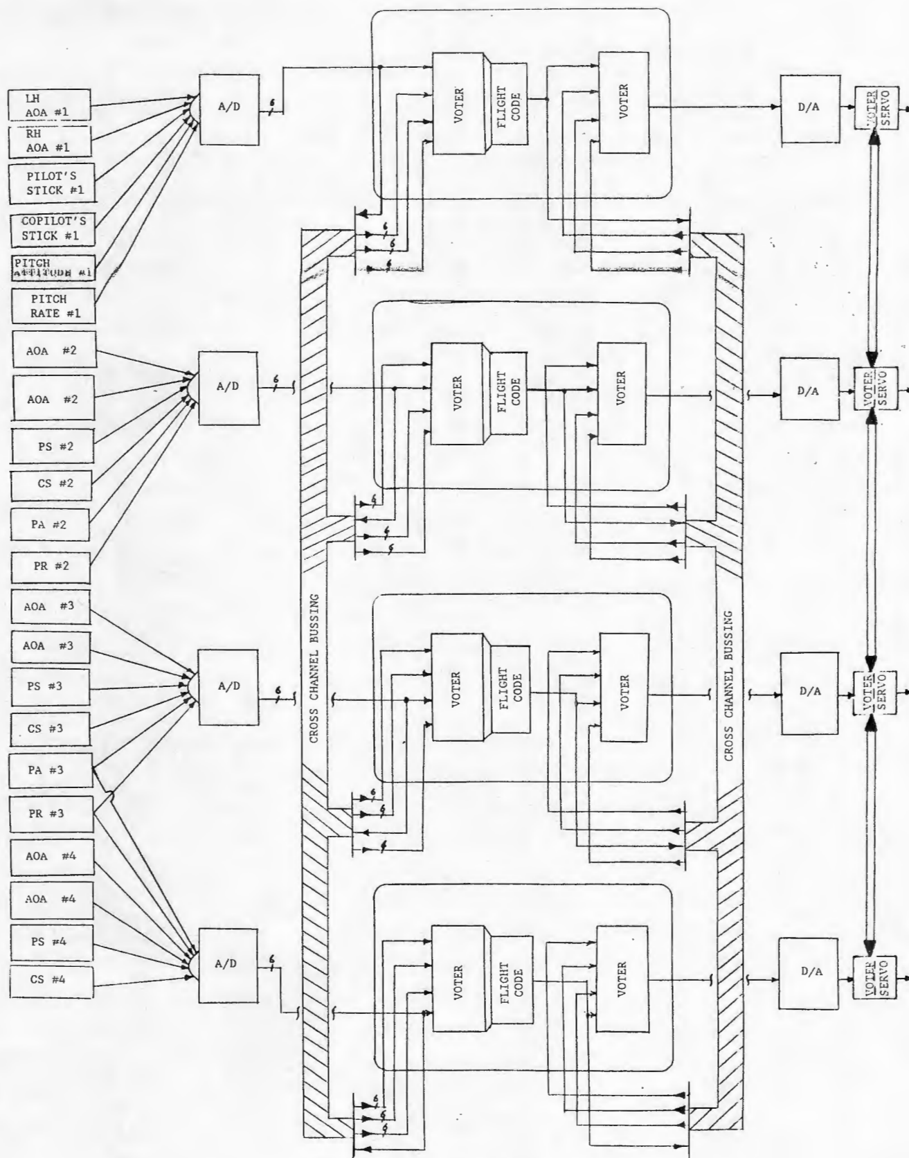
Figure 6. Baseline System Architecture
