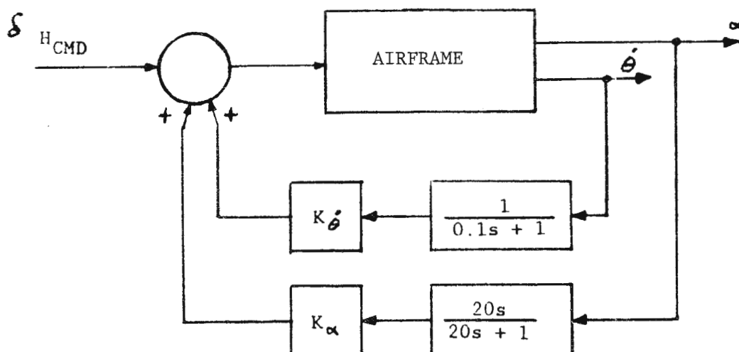
Figure 5. Augmented Fly-by-Wire Control Laws
