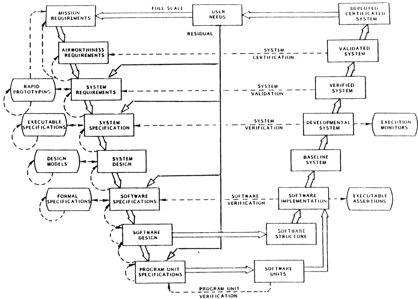
Figure 3. Digital Flight System Life Cycle
