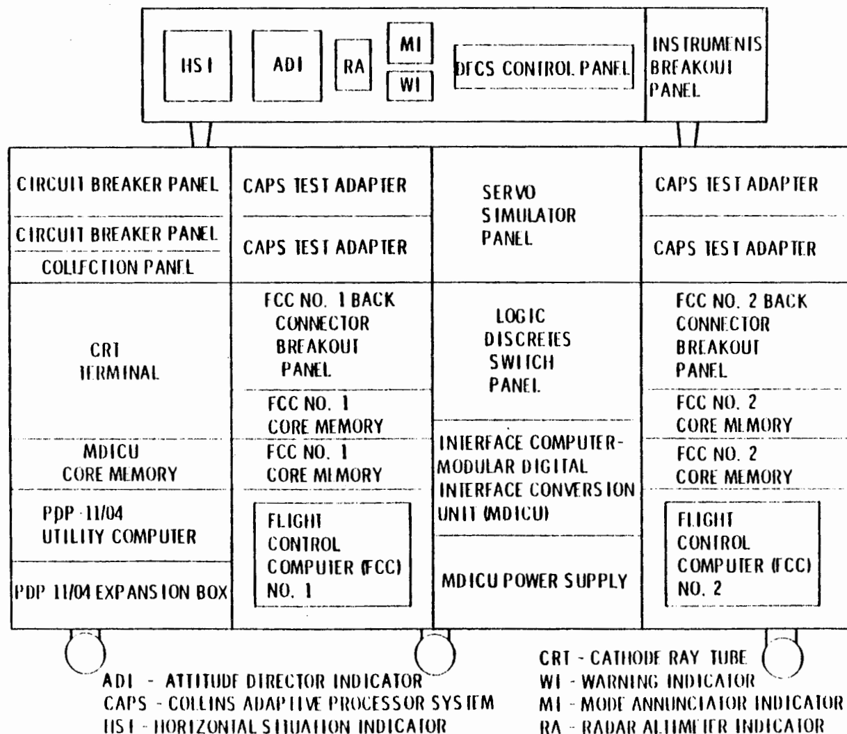
Figure 14. Palletized DFCS
