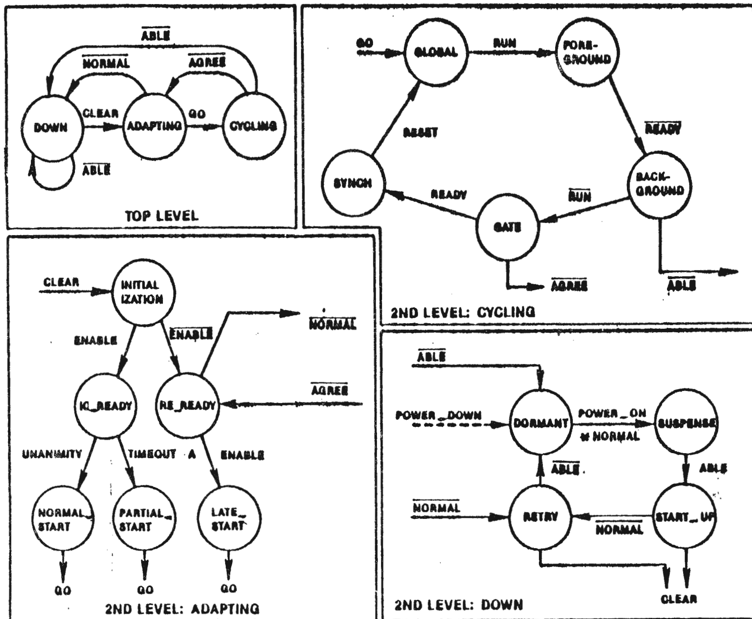
Figure 7. Channel Logic Transition Graphs
