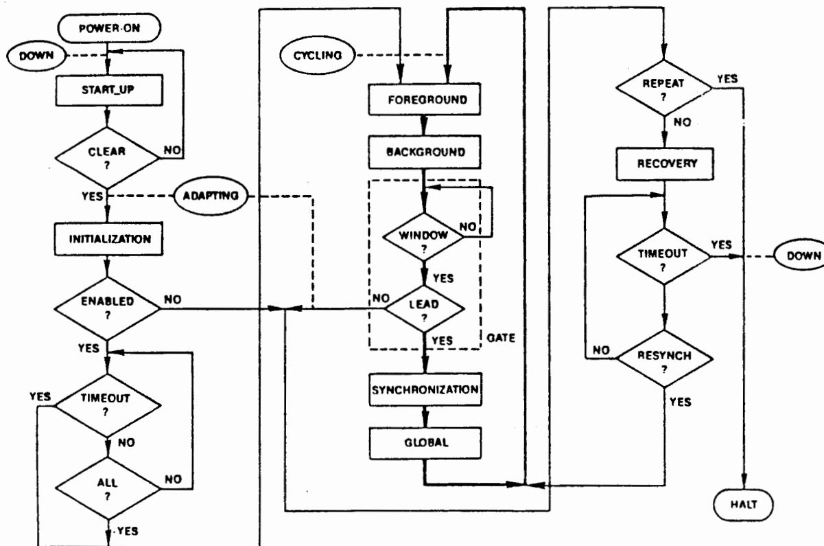
Figure 17. Software Control Flow Diagram
