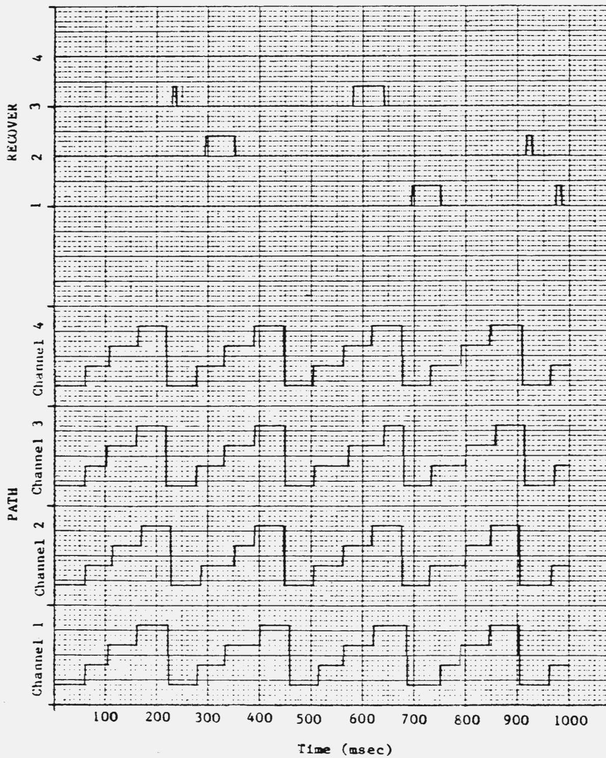
Figure 10. Predicate/Transition Network Simulation Output
