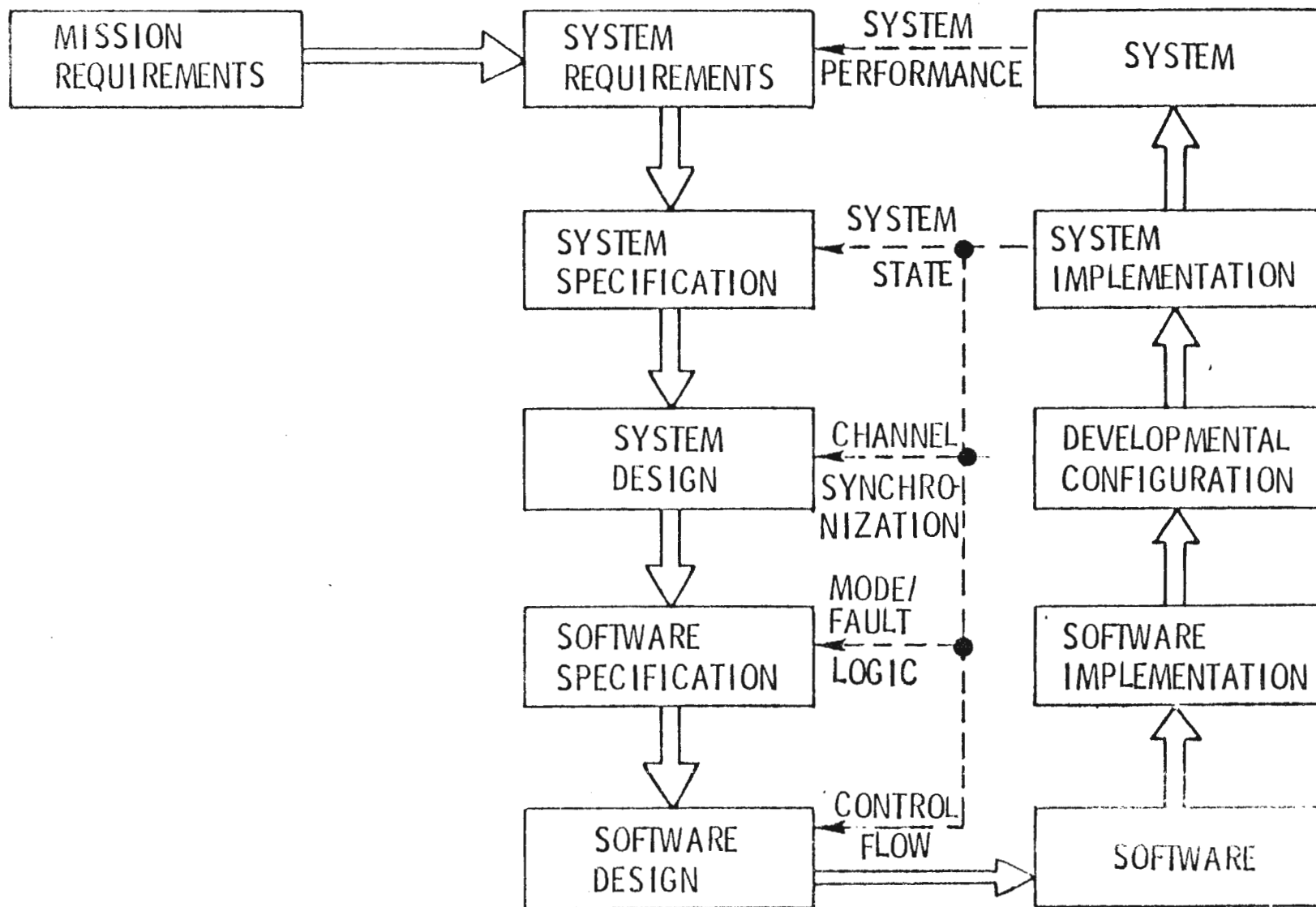
Figure 19. Multilevel Testing Closure
