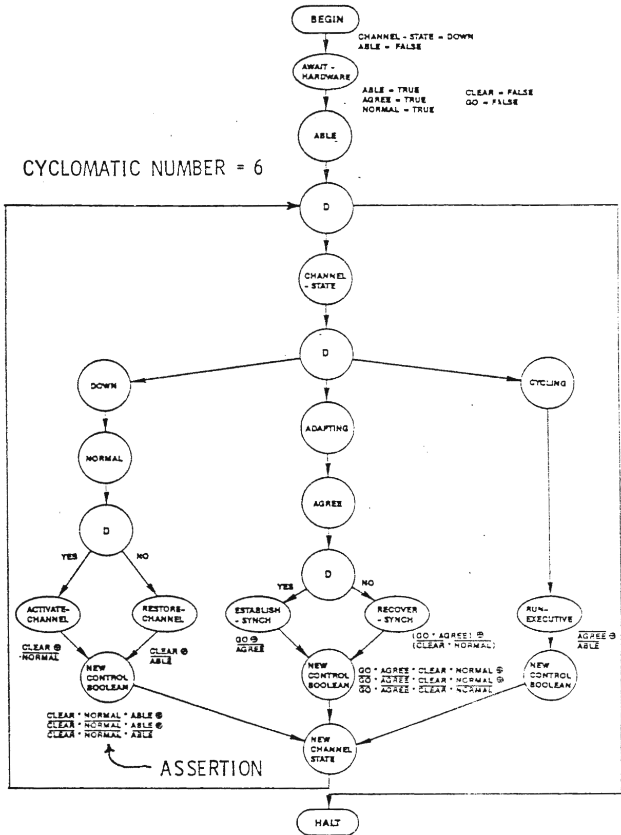
Figure 11. Top-Level Software Control Graph
