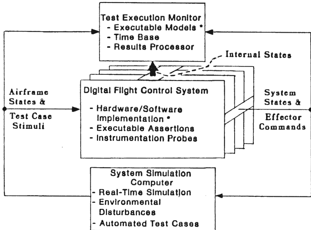
Figure 20. Automated Testing Scheme
