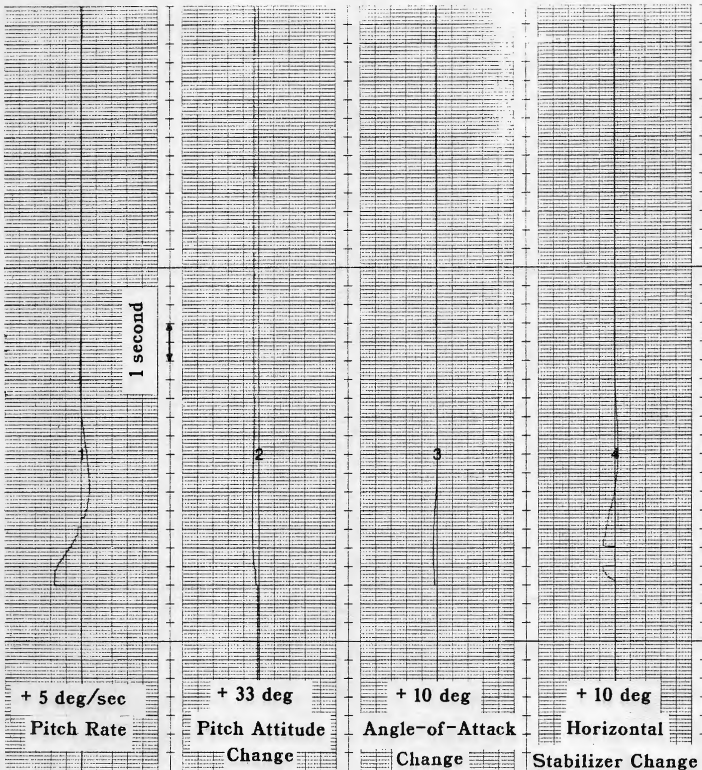
Figure 18. Augmented RSS Airplane Time History
