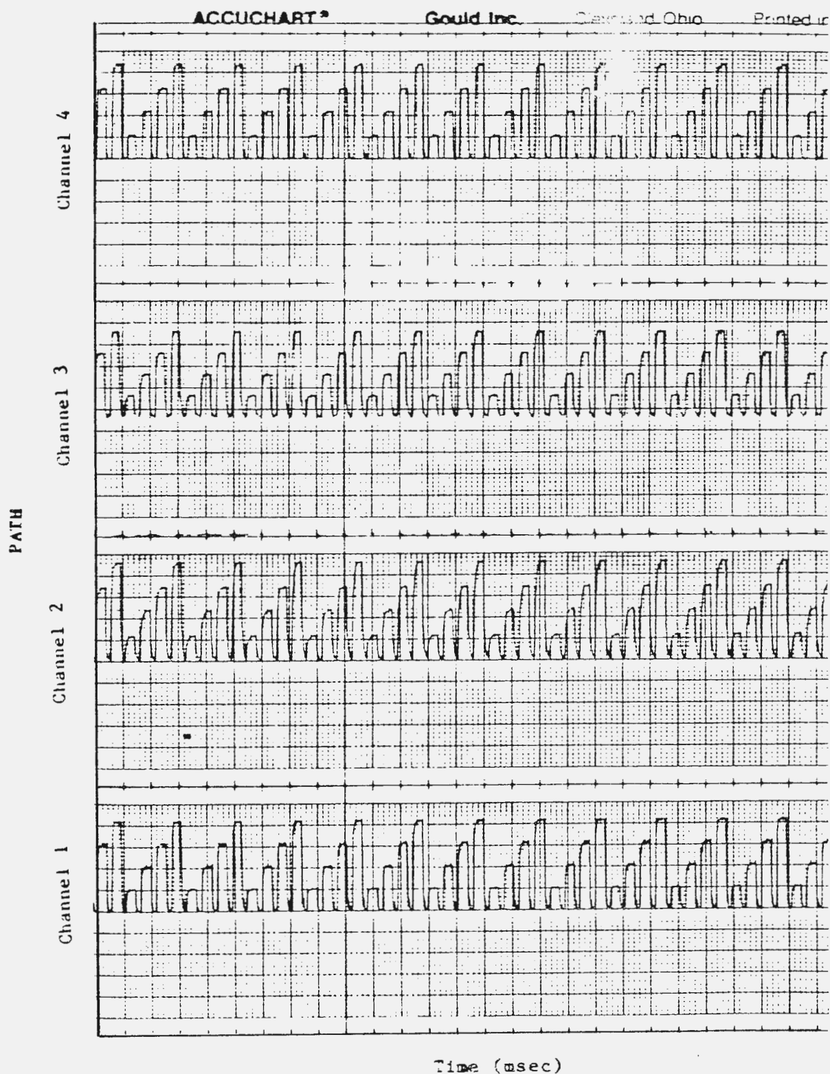
Figure 21. Normal Channel Synchronization Time History
