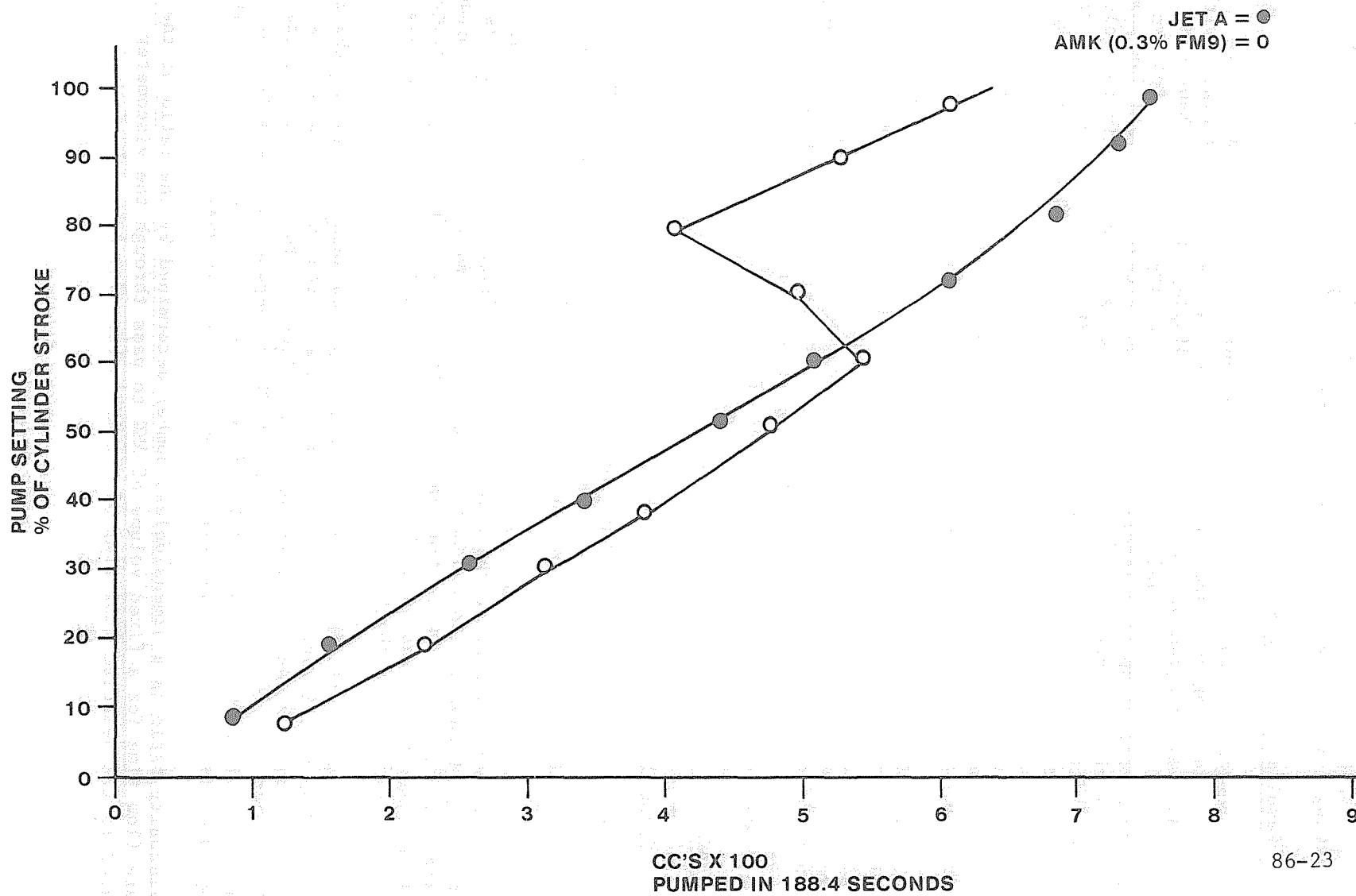
FIGURE 2.29 TEST DATA AND INERTIAL RHEOGRAM ON JET A AND AMK
