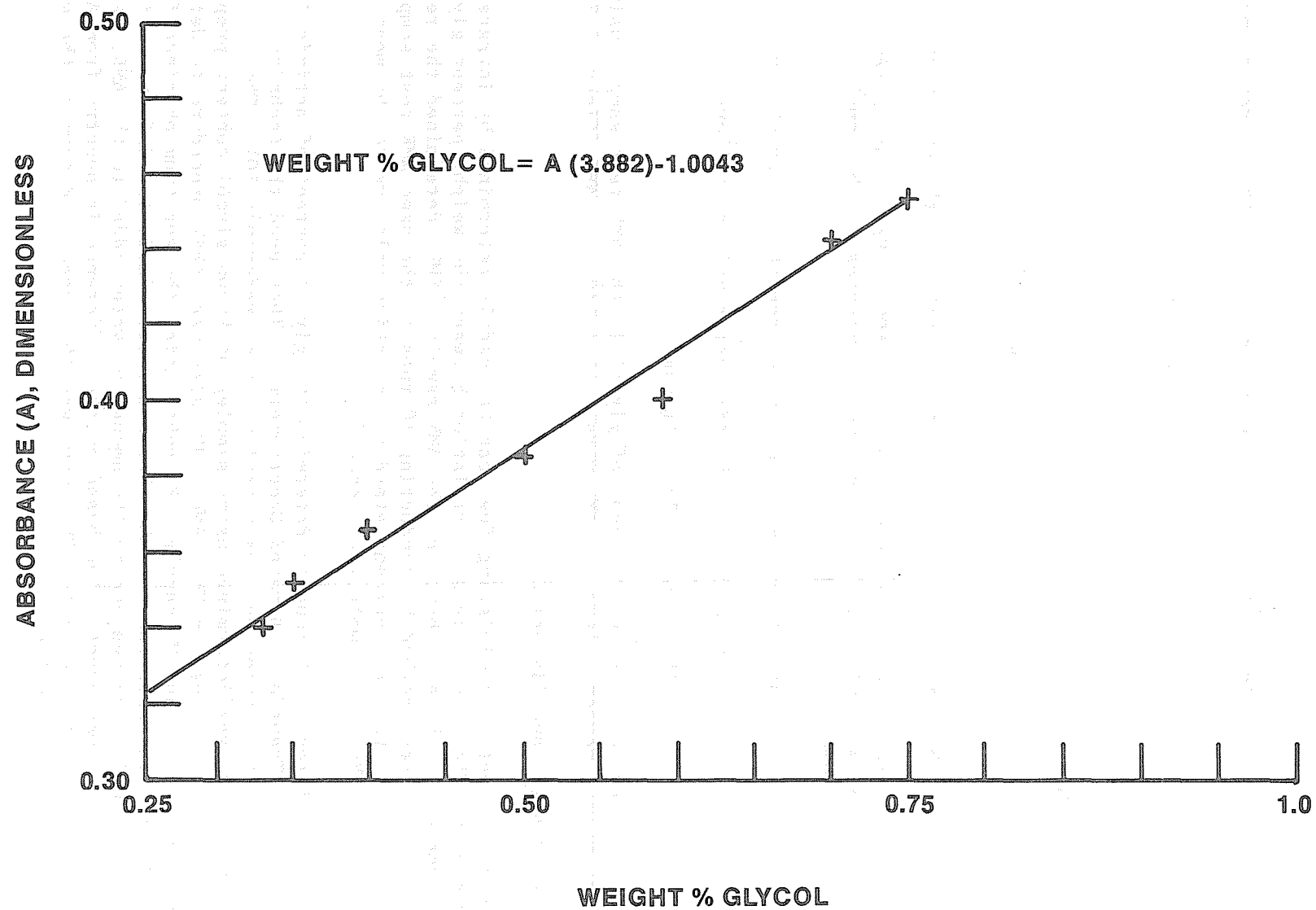
FIGURE 2.37 WEIGHT PERCENT GLYCOL IN AMK VERSUS INFRARED ABSORBANCE
