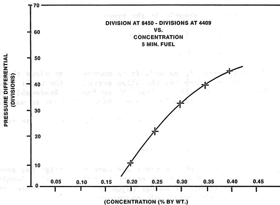
FIGURE 2.26 PRESSURE DIFFERENTIAL VERSUS CONCENTRATION
