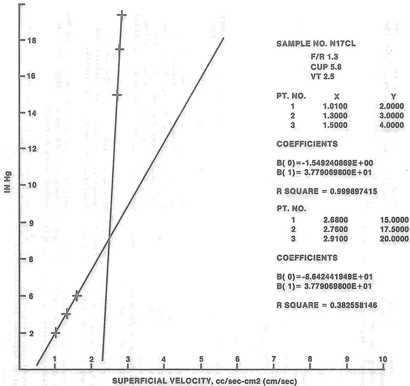
FIGURE 2.13 SAMPLE TRANSITION VELOCITY PLOT
