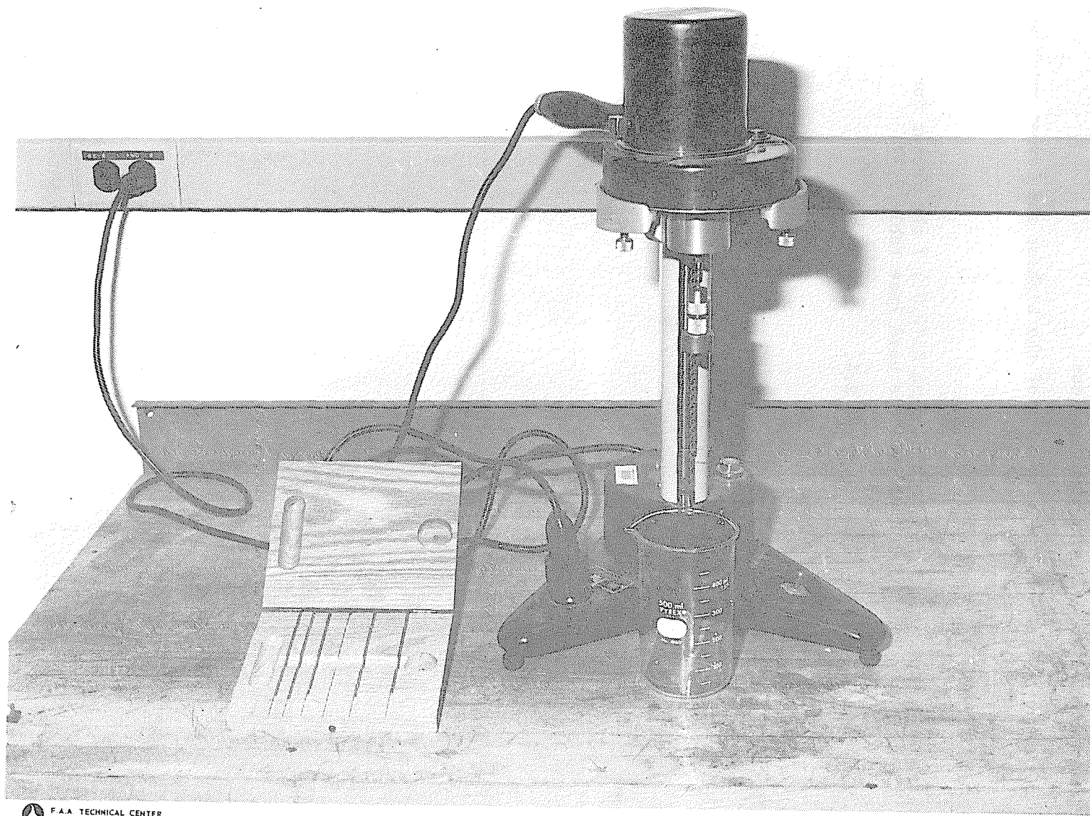
FIGURE 2.41 BROOKFIELD VISCOMETER
