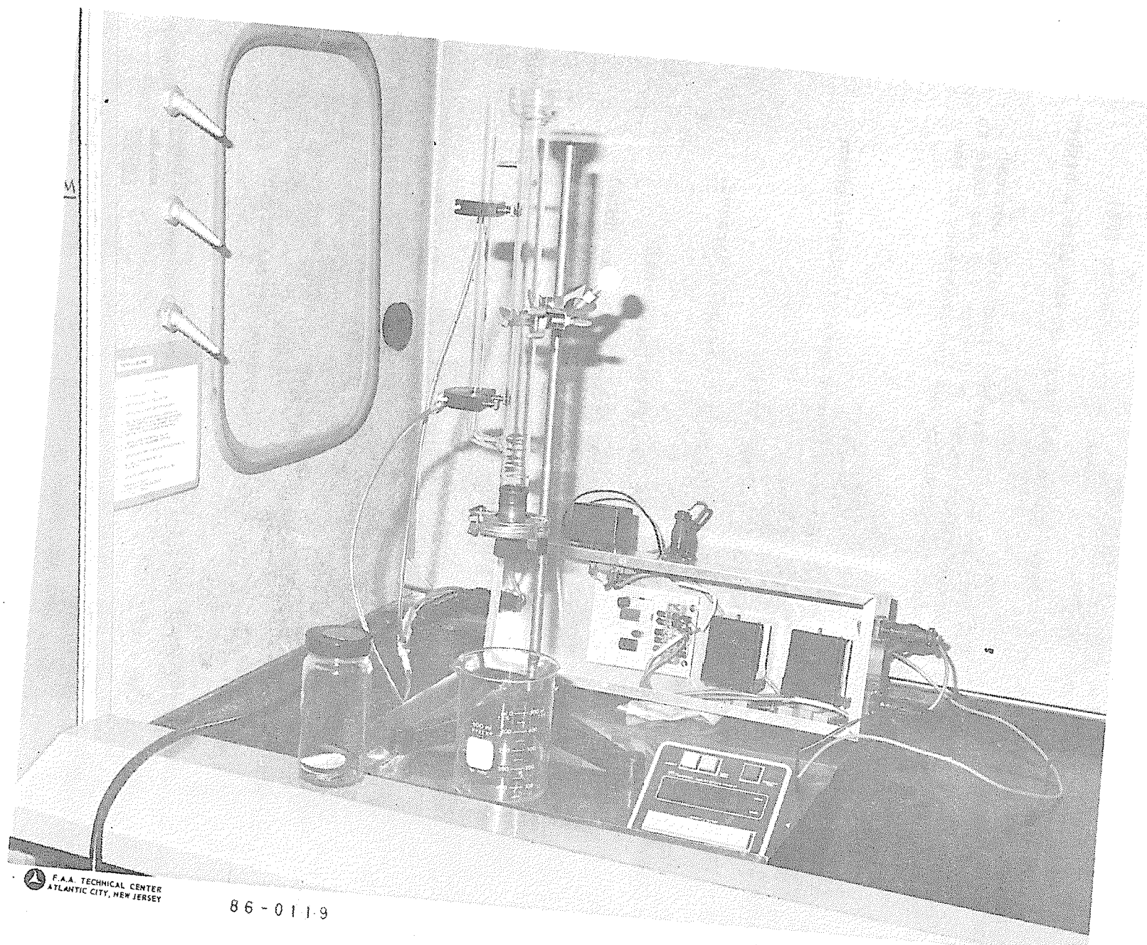
FIGURE 2.1 FILTER RATIO APPARATUS
