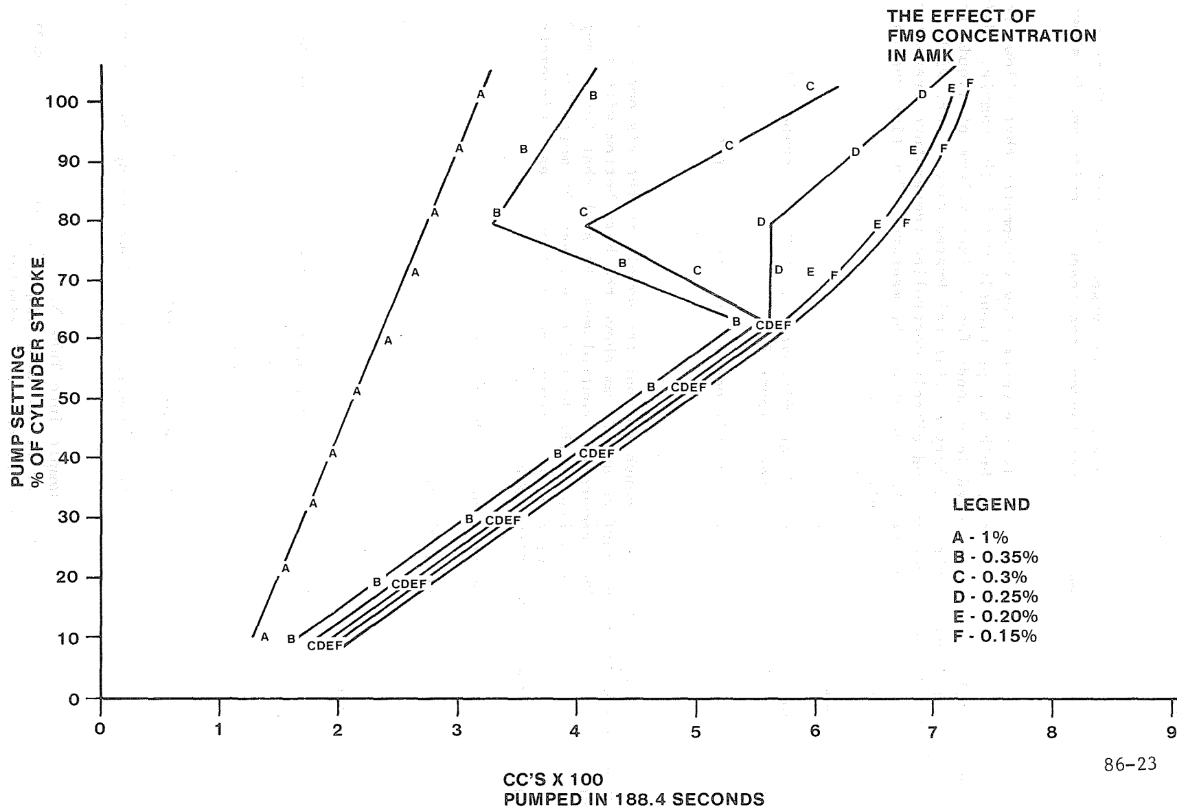
FIGURE 2.30 INERTIAL RHEOGRAMS ON THE EFFECT OF FM-9 CONCENTRATION IN AMK
