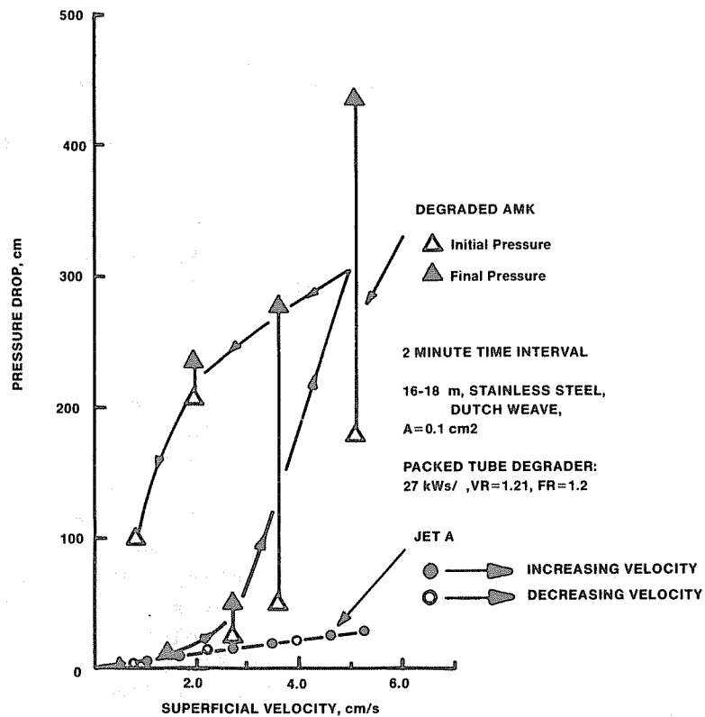
FIGURE 2.17 EFFECT OF SUPERFICIAL VELOCITY ON PRESSURE DROP ACROSS A FILTER WITH JET A AND DEGRADED AMK
