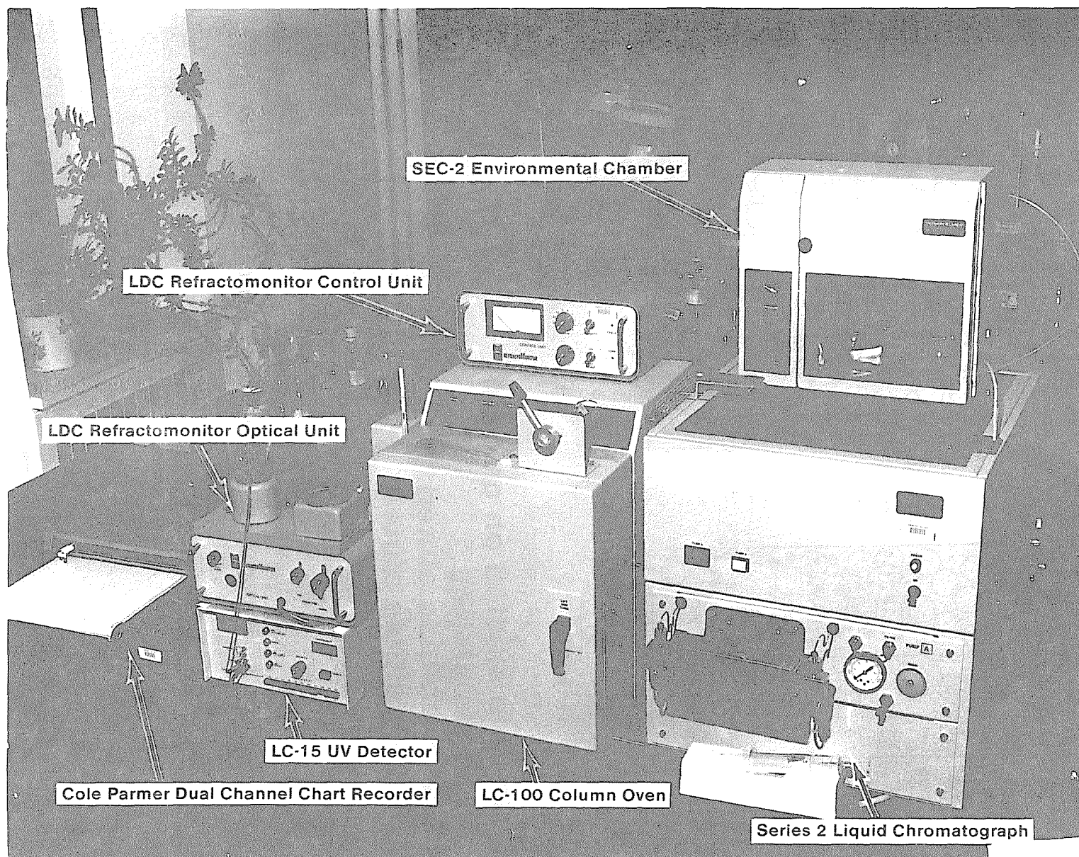
FIGURE 2.19 GEL PERMEATION CHROMATOGRAPH
