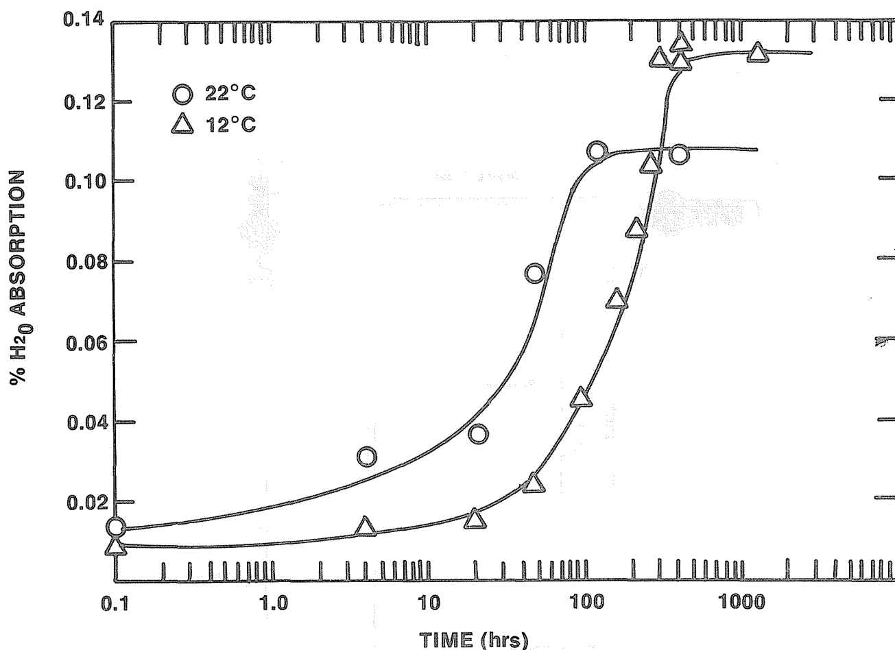
FIGURE 2.34 UPTAKE OF WATER BY FM-9 AMK
