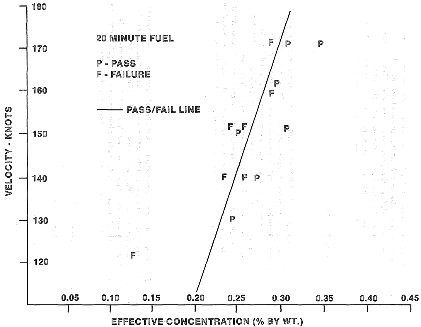
FIGURE 2.27 WING SPILLAGE TEST RESULTS VERSUS EFFECTIVE CONCENTRATION
