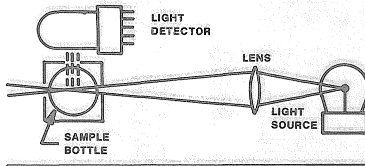
FIGURE 2.6 SCHEMATIC OF NEPHELOMETER OPERATION
