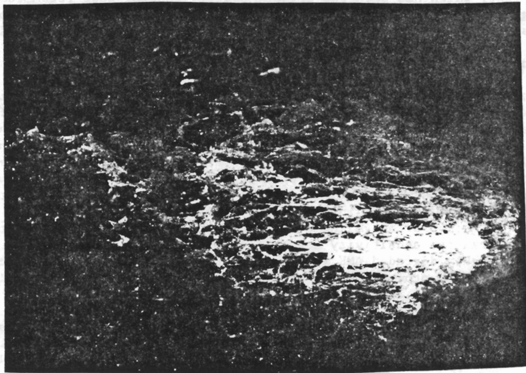
FIGURE 1. BREAKUP OF JET A AND AMK BY HIGH VELOCITY AIR High velocity air breaks up stream of Jet A into fine mist (top) but produces only a sheeting action on AMK stream (bottom) which hangs together as ligaments and large droplets in tests at JPL.
