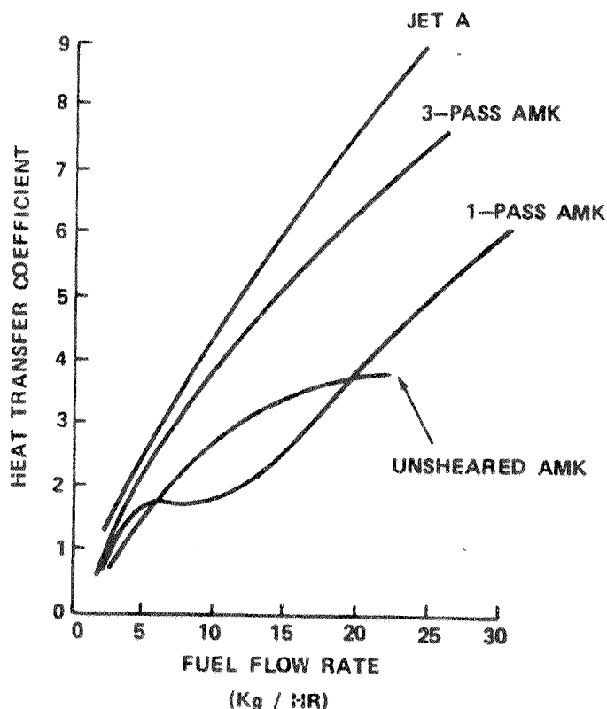
FIGURE 4. AMK HEAT TRANSFER GRAPH
