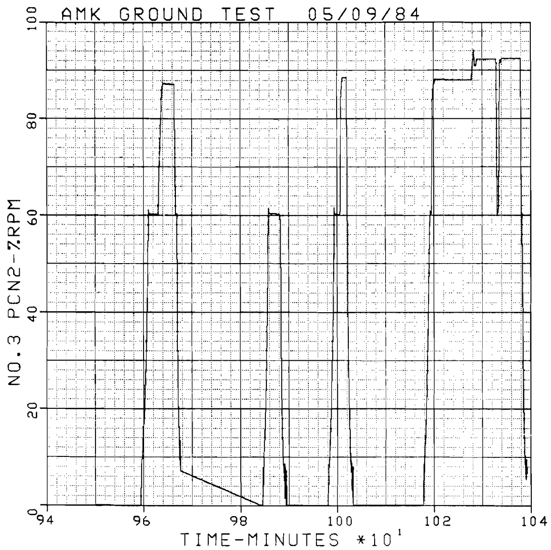
FIGURE 83. NUMBER 3 ENGINE SPEED
