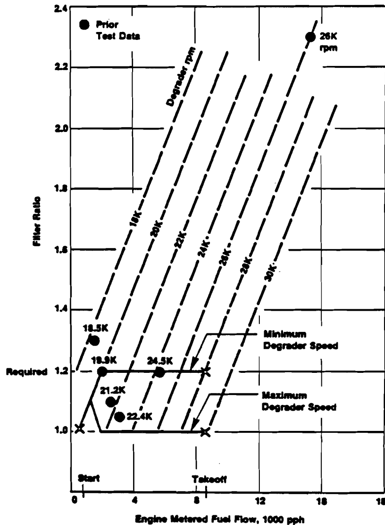
FIGURE 5. DEGRADER SPEED SCHEDULE RELATIONSHIP TO FLOW AND FILTER RATIO
