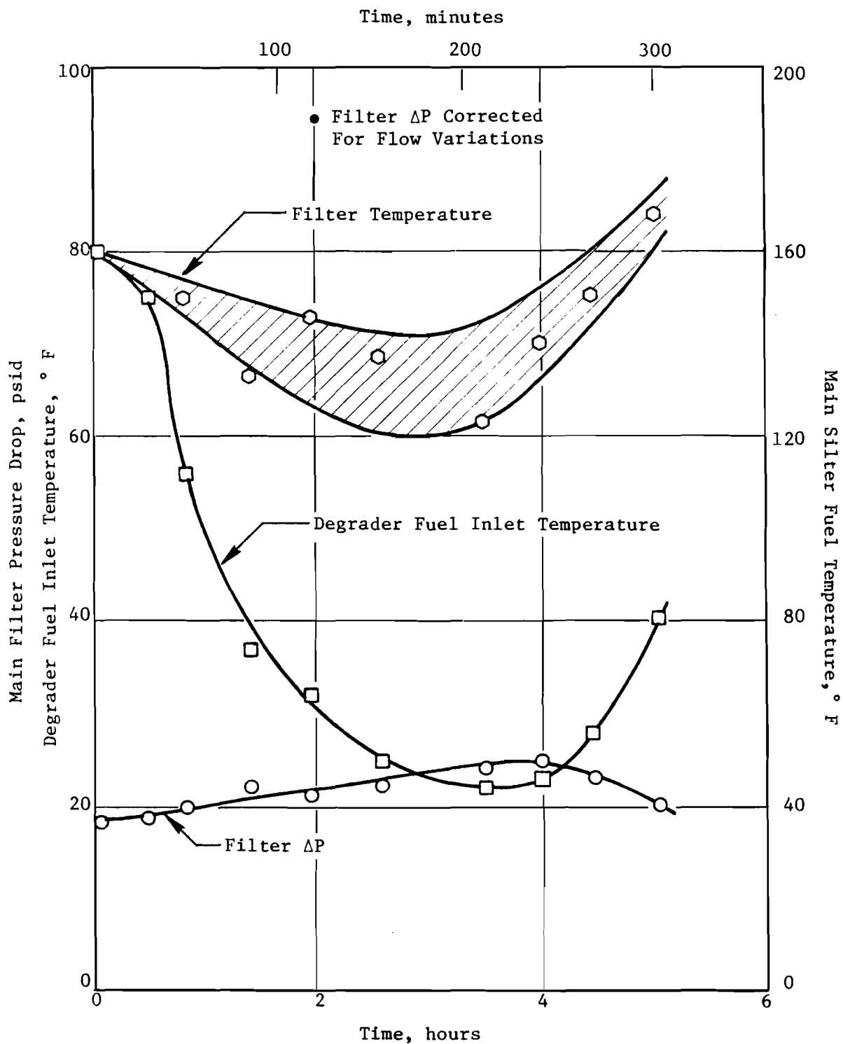
FIGURE 116. GENERAL INFLUENCE OF AMK FUEL TEMPERATURE ON NUMBER 3 ENGINE MAIN FUEL FILTER \Delta P (8-30-84 FLIGHT)
