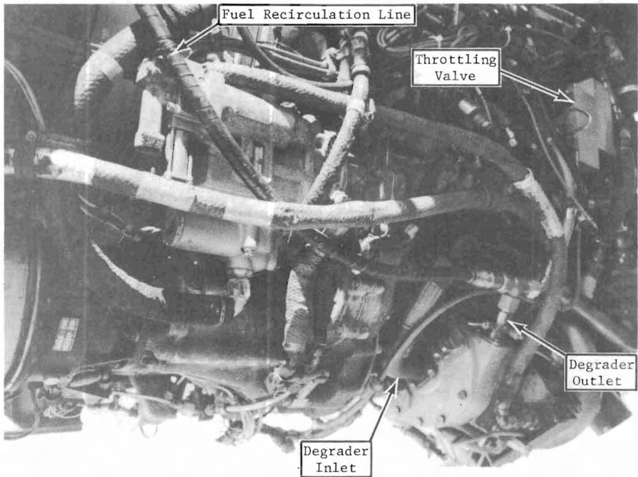
FIGURE 28. DEGRADER INLET AND OUTLET
