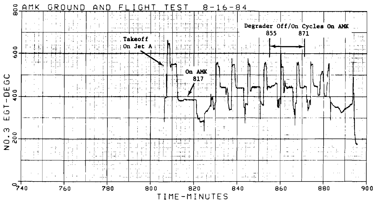
FIGURE 93. NUMBER 3 ENGINE EGT
