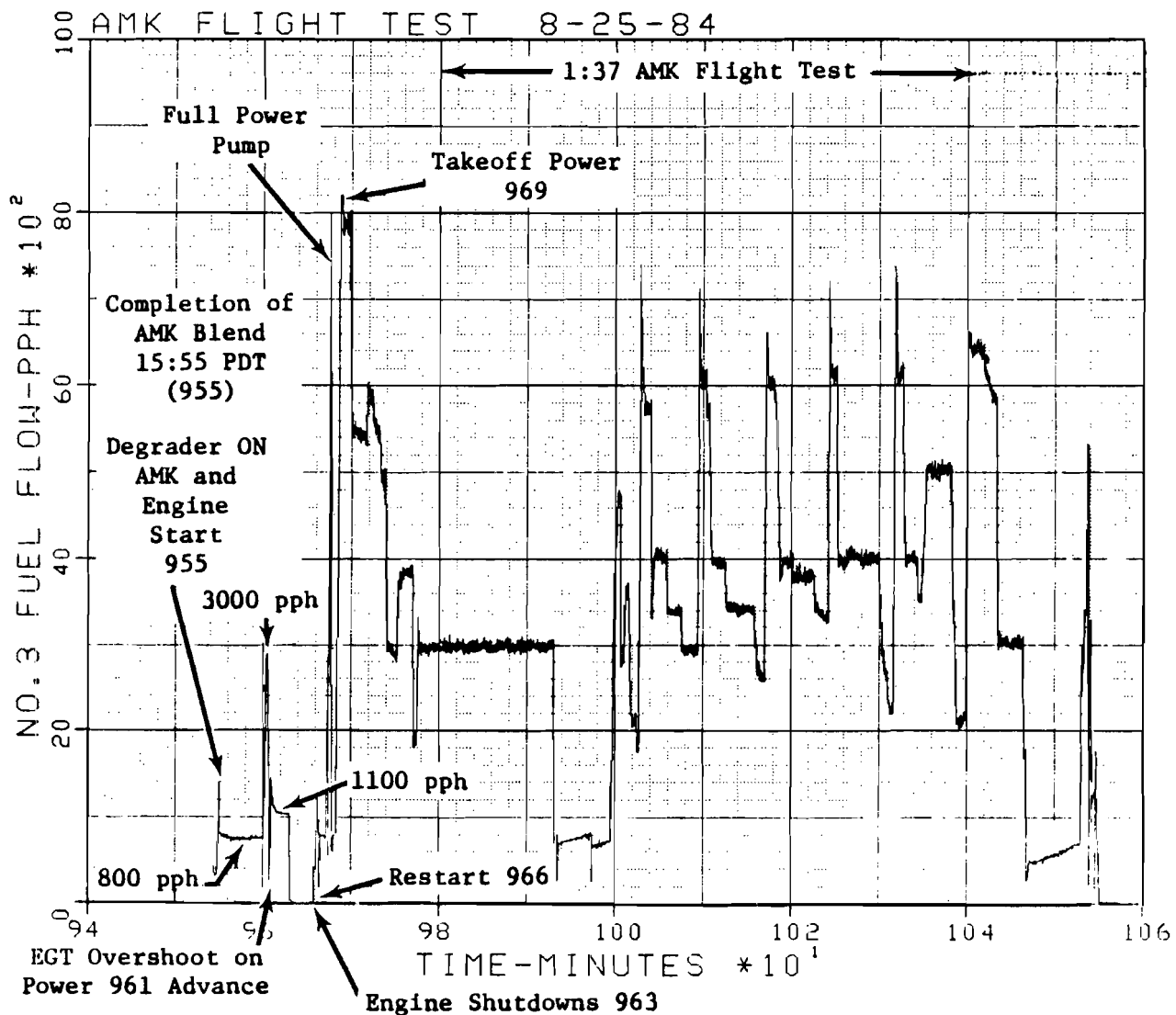
FIGURE 103. NUMBER 3 ENGINE FUEL FLOW
