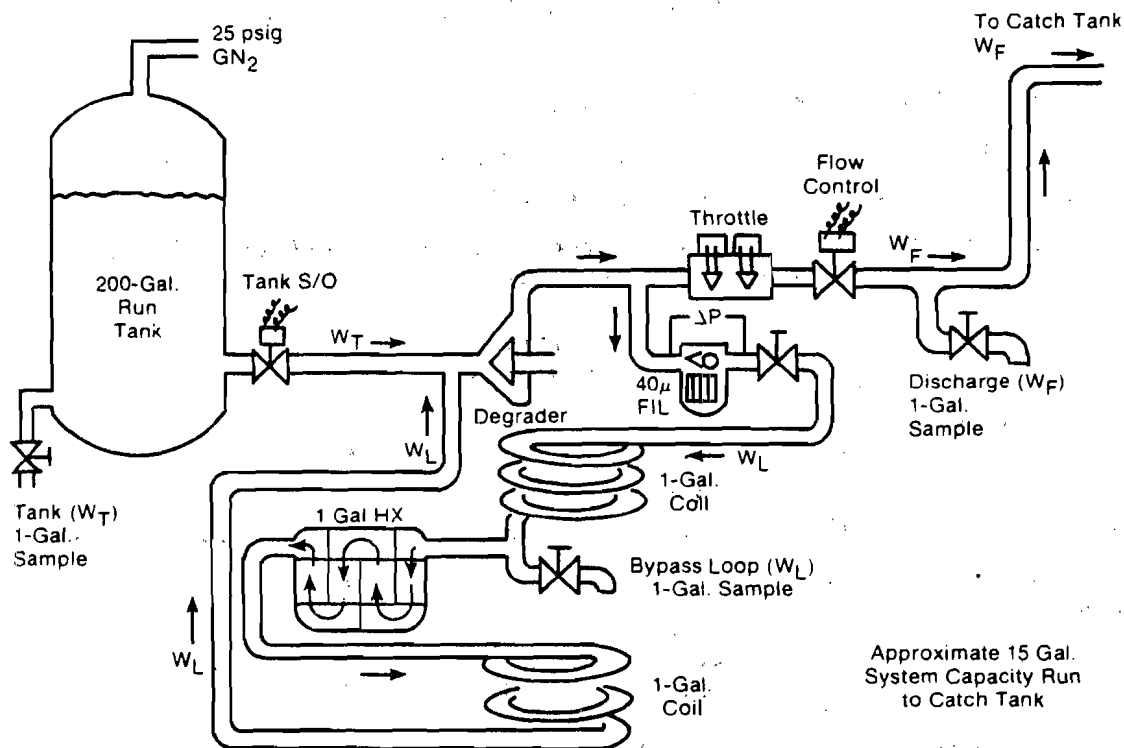
FIGURE 49. SIMPLIFIED AMK TEST SCHEMATIC
