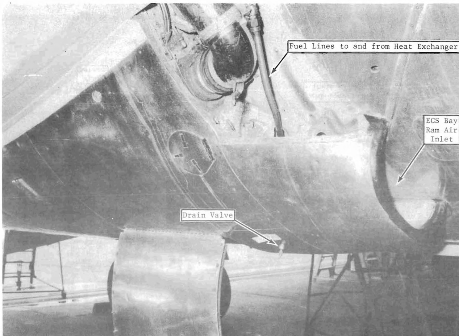
FIGURE 31. OUTSIDE VIEW OF ECS BAY
