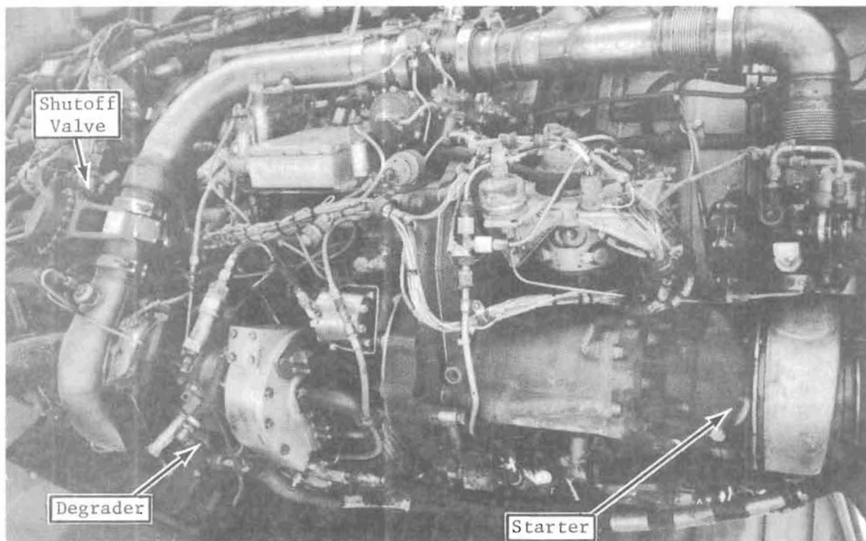
FIGURE 35. BOTTOM VIEW OF NUMBER 3 ENGINE
