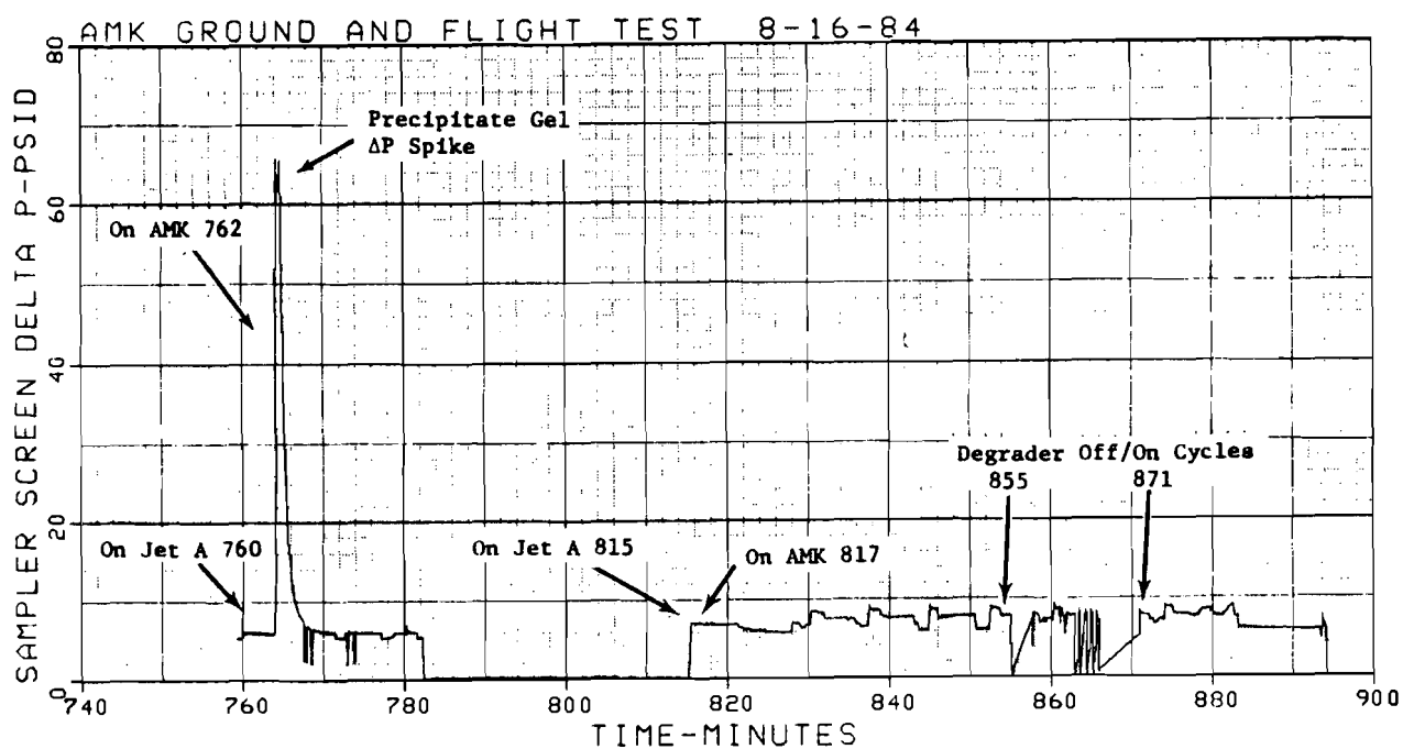
FIGURE 91. SAMPLER FILTER ΔP
