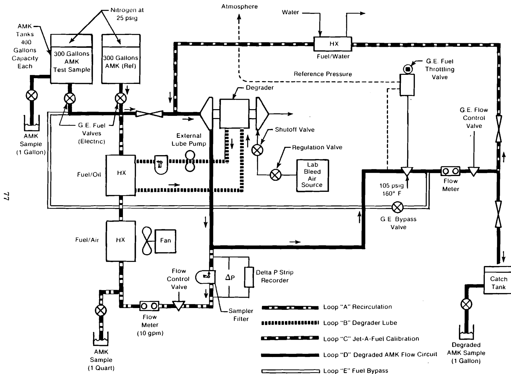
FIGURE 42. AMK FUEL DEGRADER SYSTEM TEST SCHEMATIC
