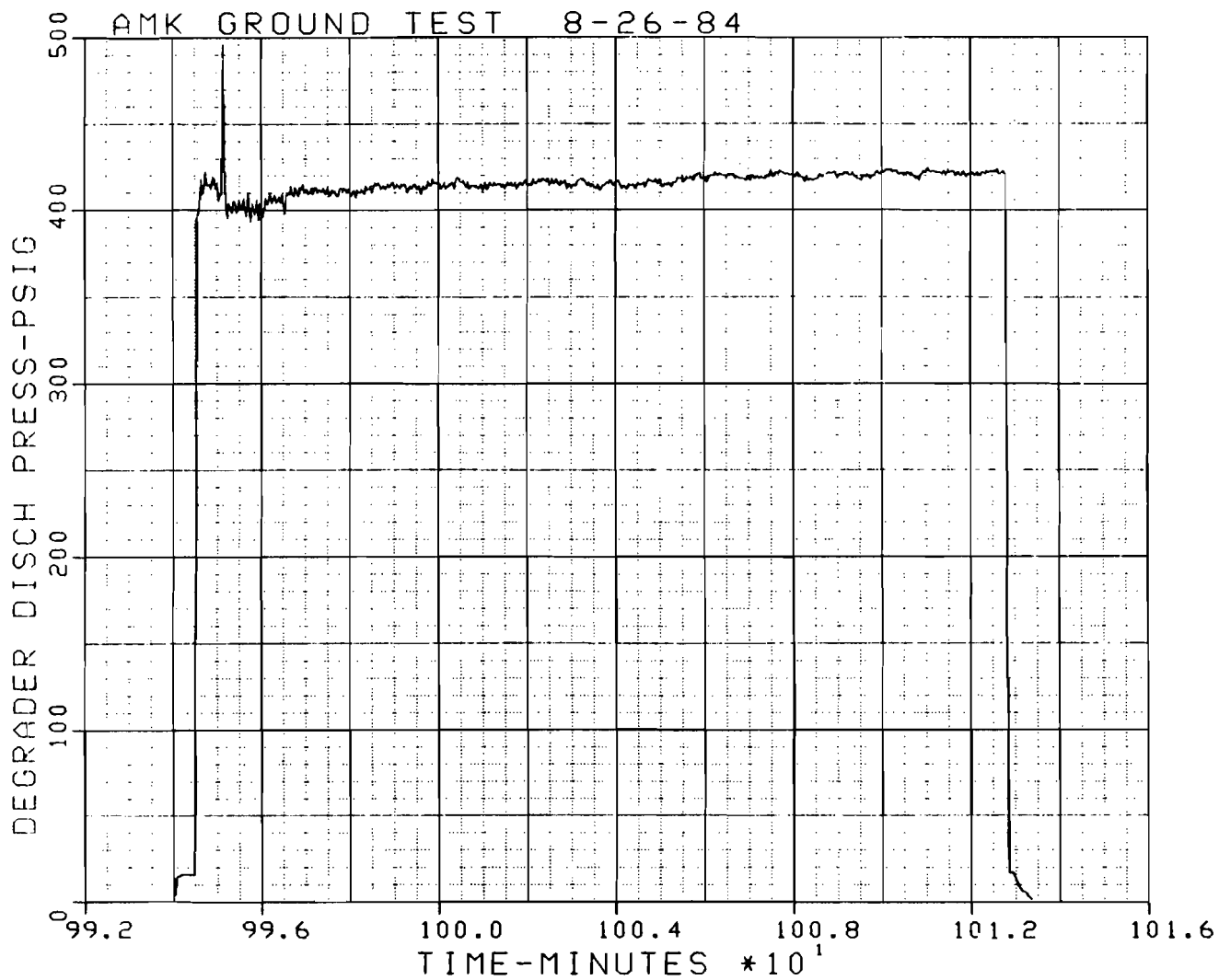
FIGURE 105. DEGRADER FUEL DISCHARGE PRESSURE
