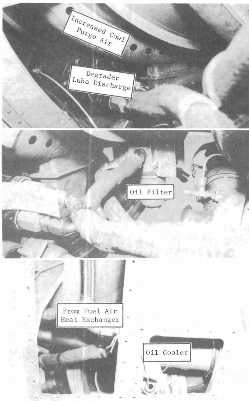
FIGURE 26. LUBE SYSTEM COMPONENTS
