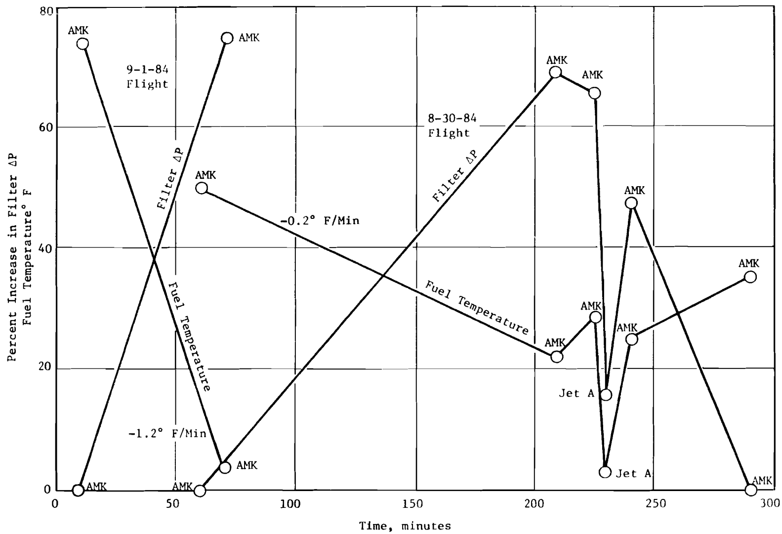
FIGURE 117. TREND OF SAMPLER FILTER \Delta P AS A FUNCTION OF DEGRADER FUEL INLET TEMPERATURE
