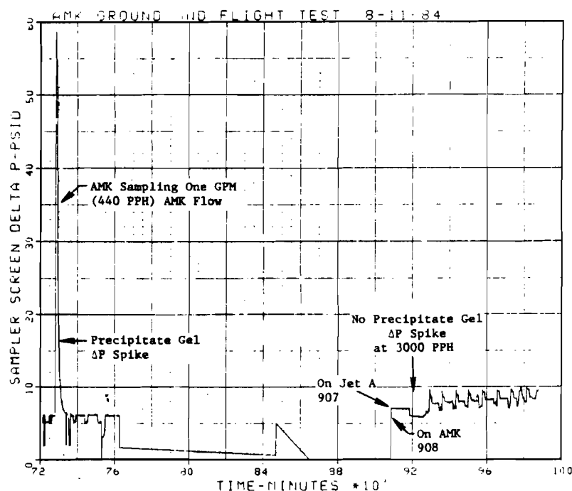
FIGURE 86. SAMPLER FILTER \Delta P
