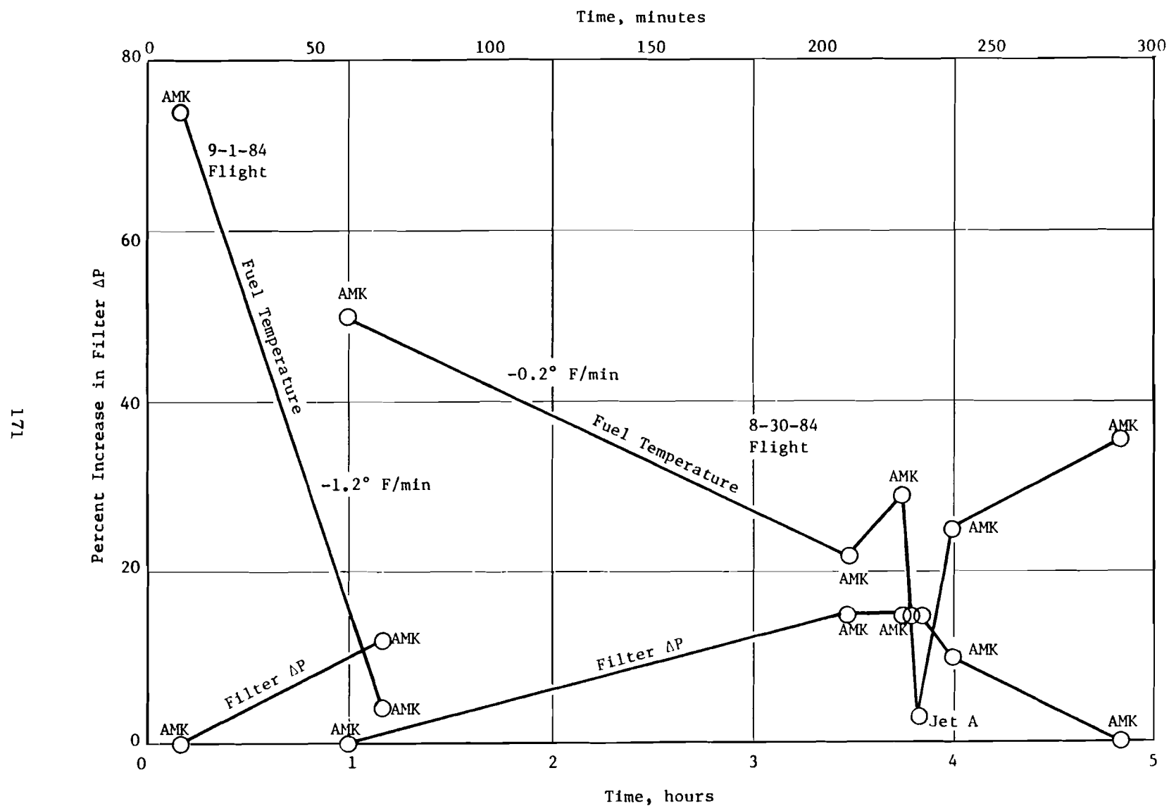
FIGURE 118. TREND OF MAIN FILTER \Delta P AS A FUNCTION OF DEGRADER FUEL INLET TEMPERATURE
