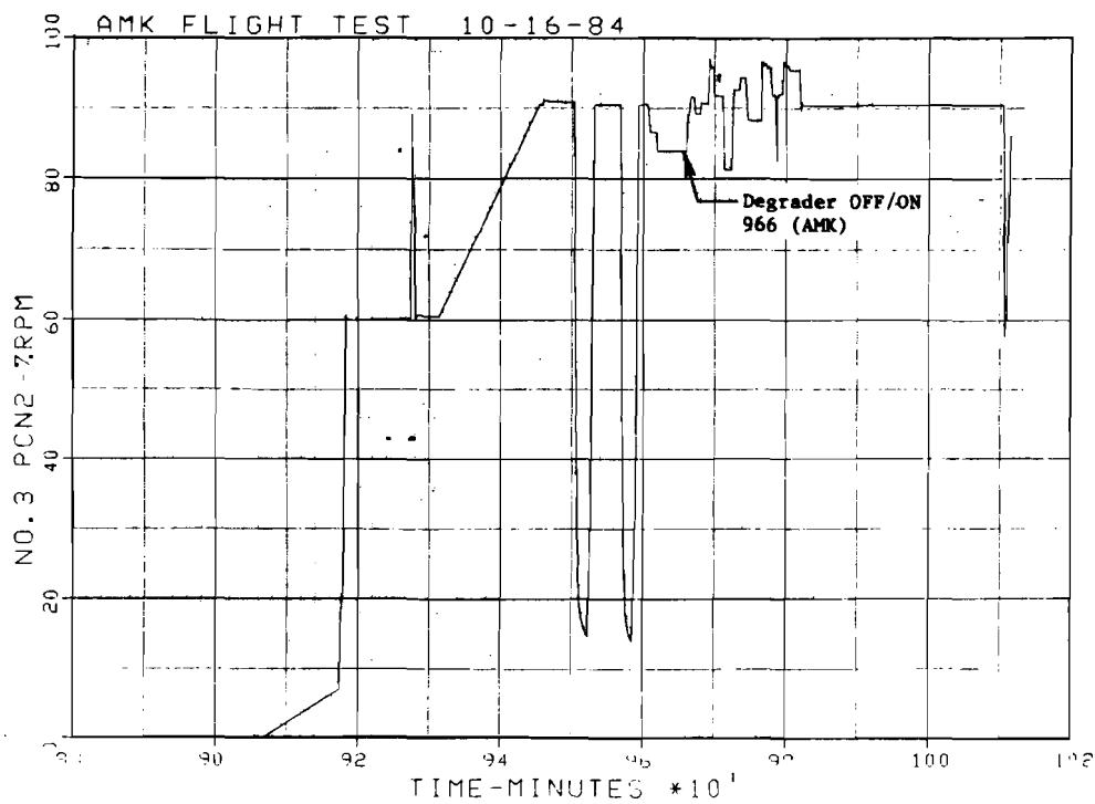
FIGURE 130. NUMBER 3 ENGINE SPEED
