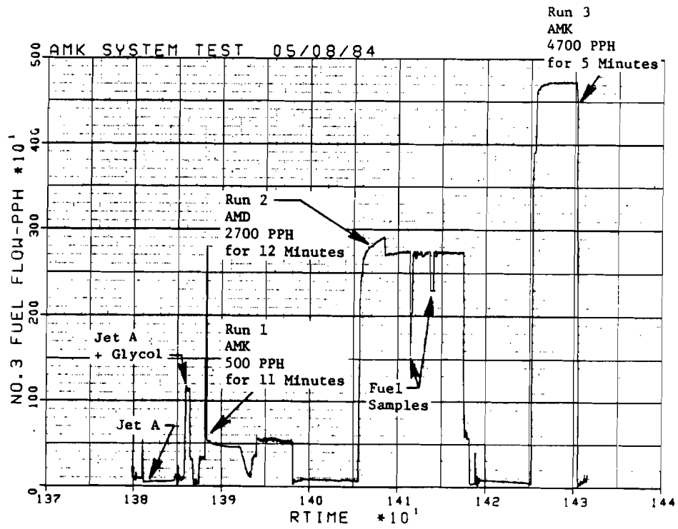
FIGURE 57. SYSTEM TEST FUEL FLOW AND TEST EVENTS
