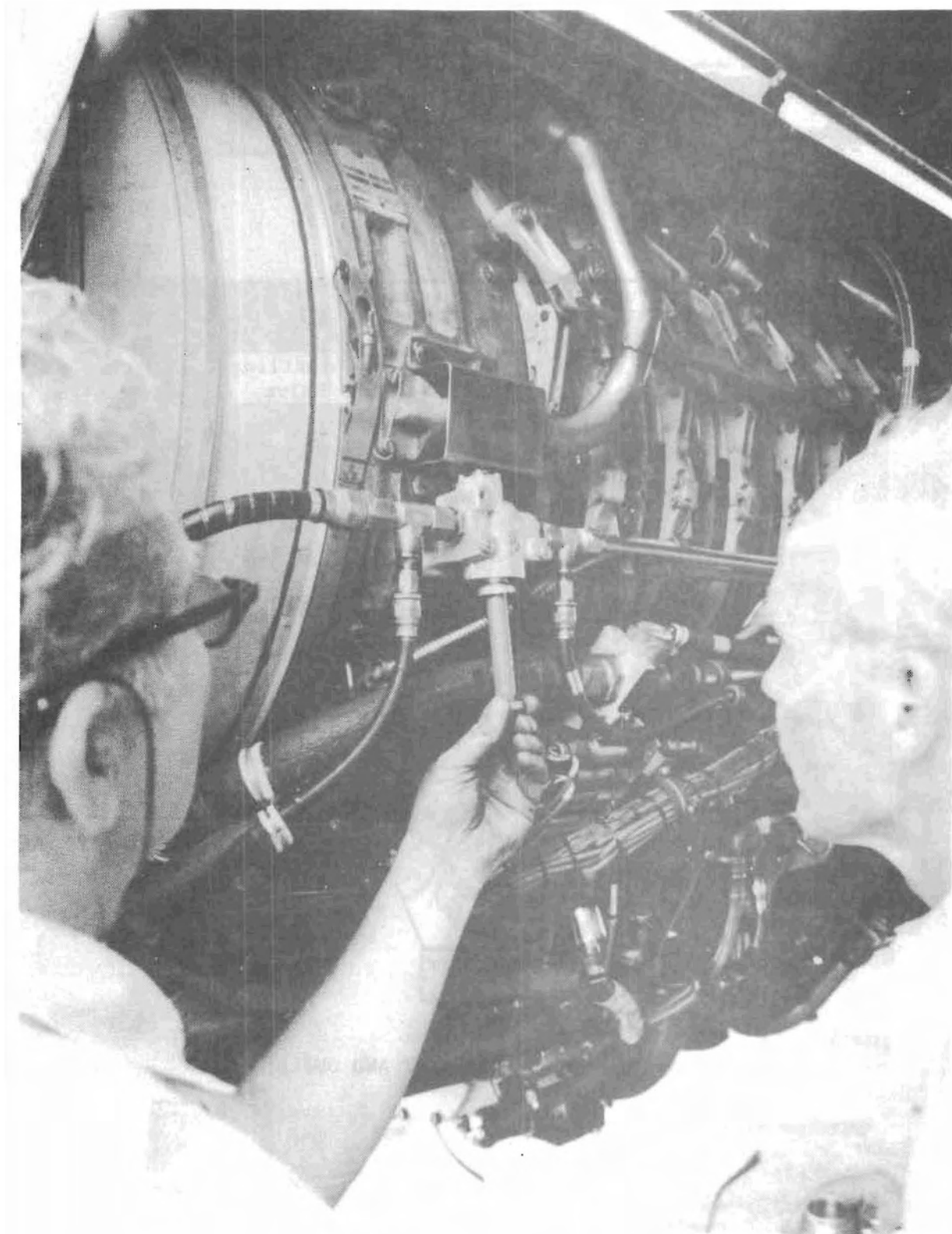
FIGURE 29. SAMPLER FILTER
