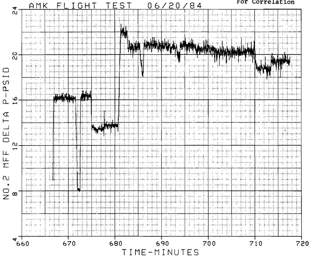
FIGURE 79. NUMBER 2 ENGINE MAIN FUEL FILTER \Delta P
