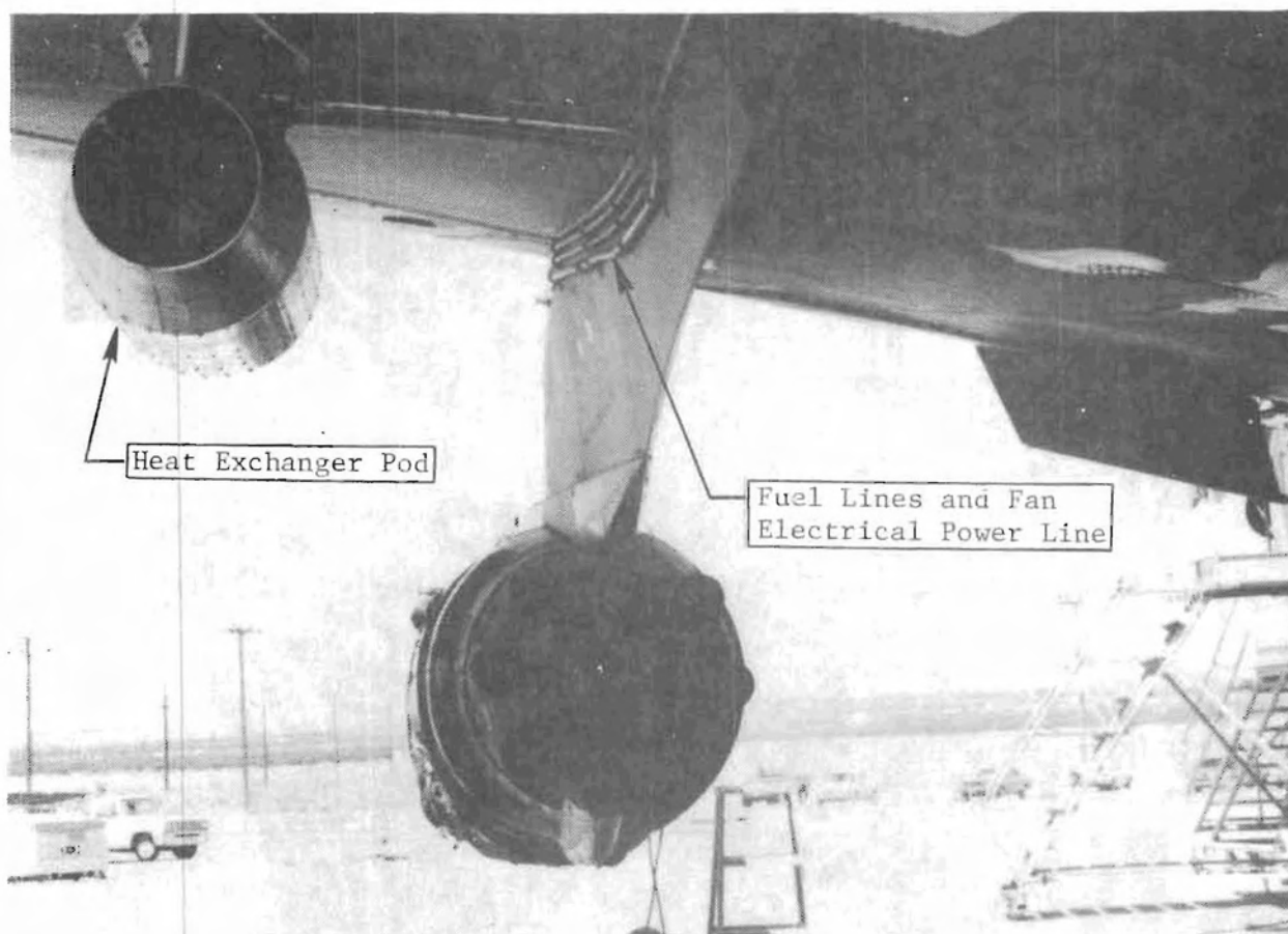
FIGURE 135. B720 HEAT EXCHANGER POD
