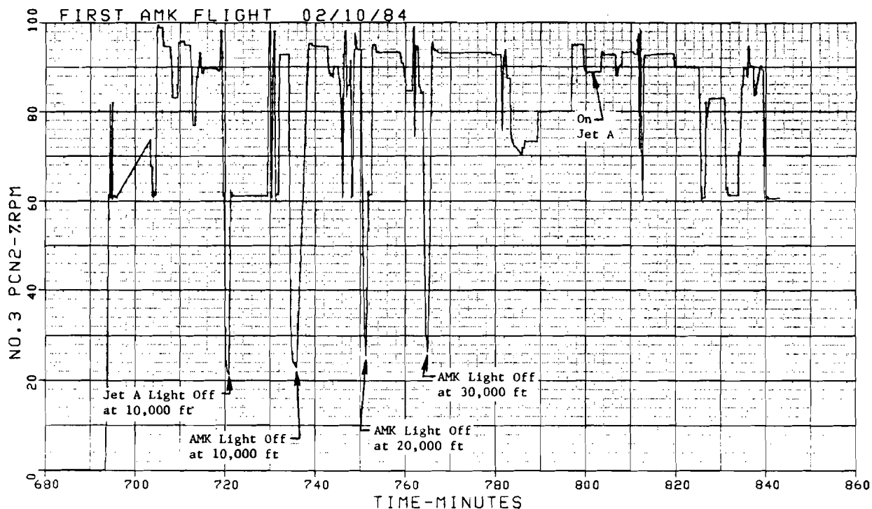
FIGURE 85. ENGINE SPEED (N 2 )
