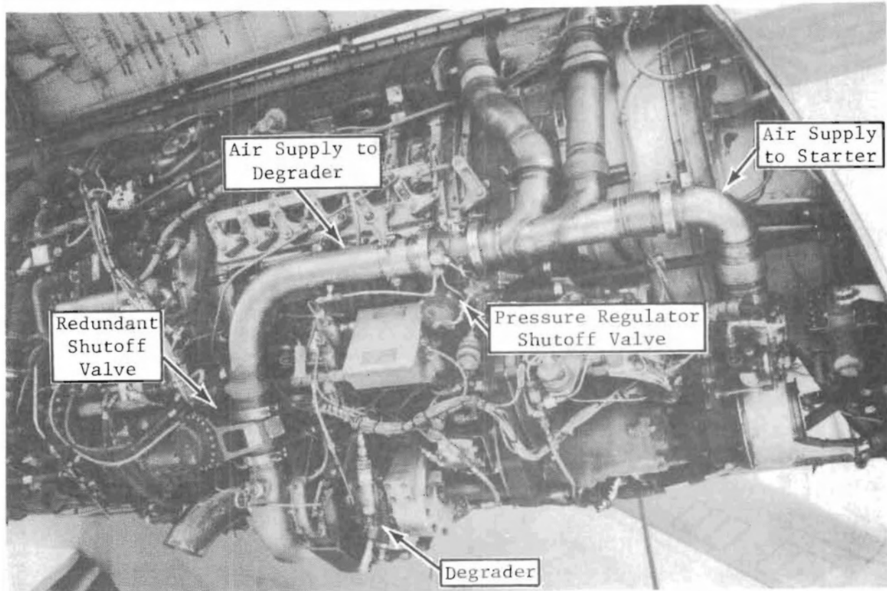
FIGURE 33. VIEW OF RIGHT SIDE OF NUMBER 3 ENGINE
