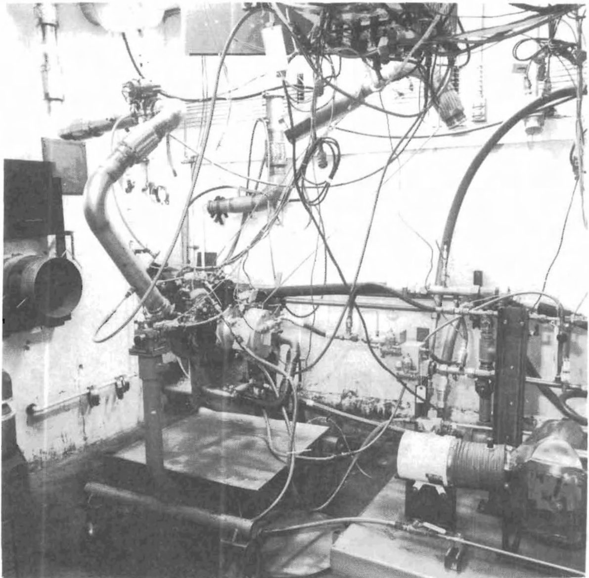
FIGURE 44. ATMP80-1 PUMP/DEGRADER TEST MODULE
