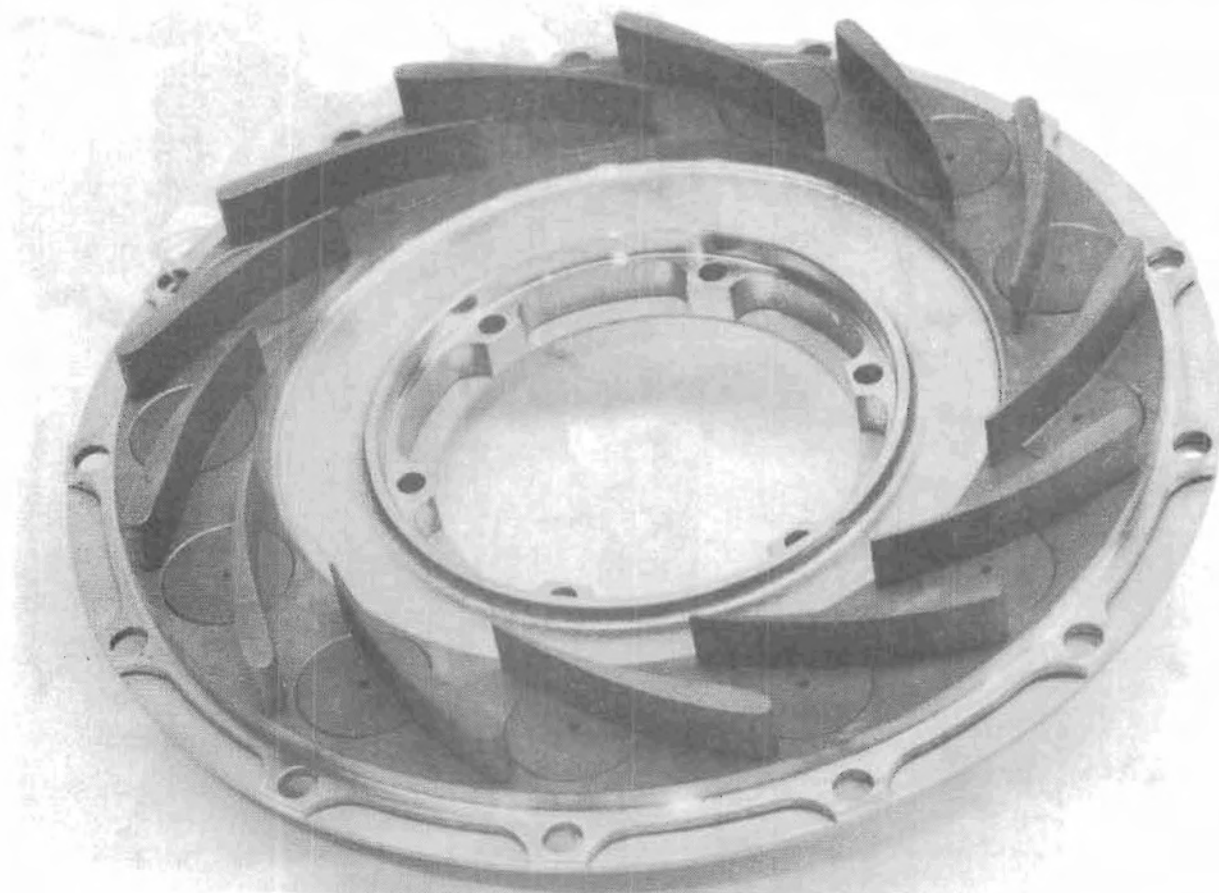
FIGURE 17. VARIABLE-AREA NOZZLE
