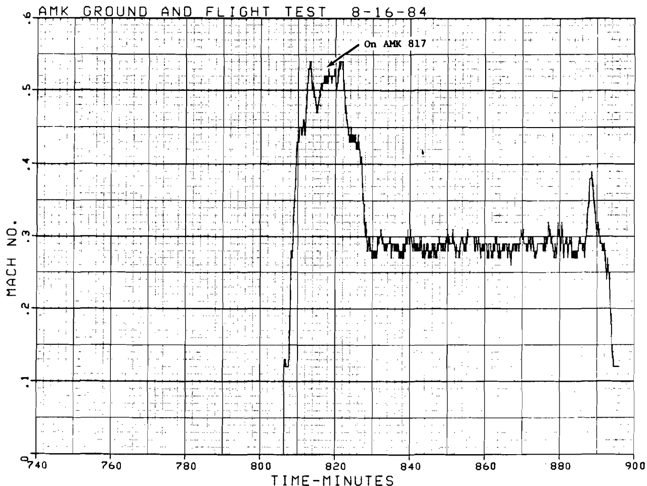
FIGURE 89. MACH NUMBER
