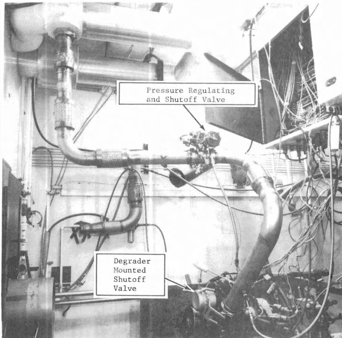
FIGURE 43. PNEUMATIC SUPPLY AND REGULATION/SHUTOFF VALVES
