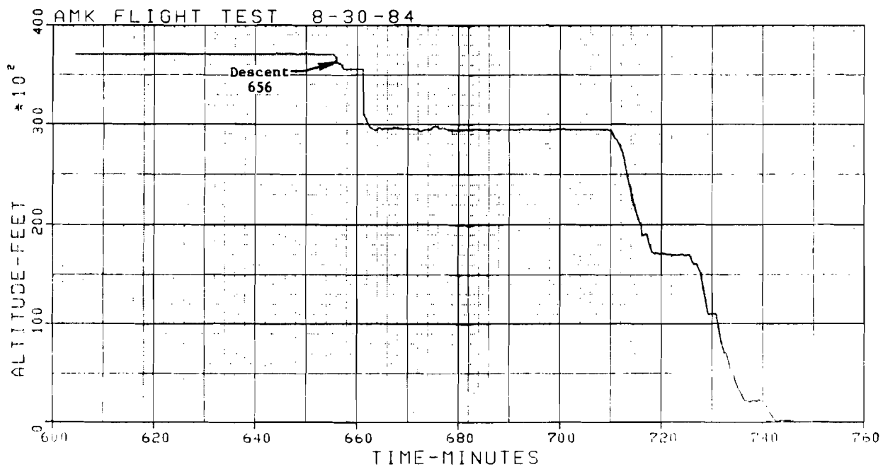
FIGURE 108. PRESSURE ALTITUDE
