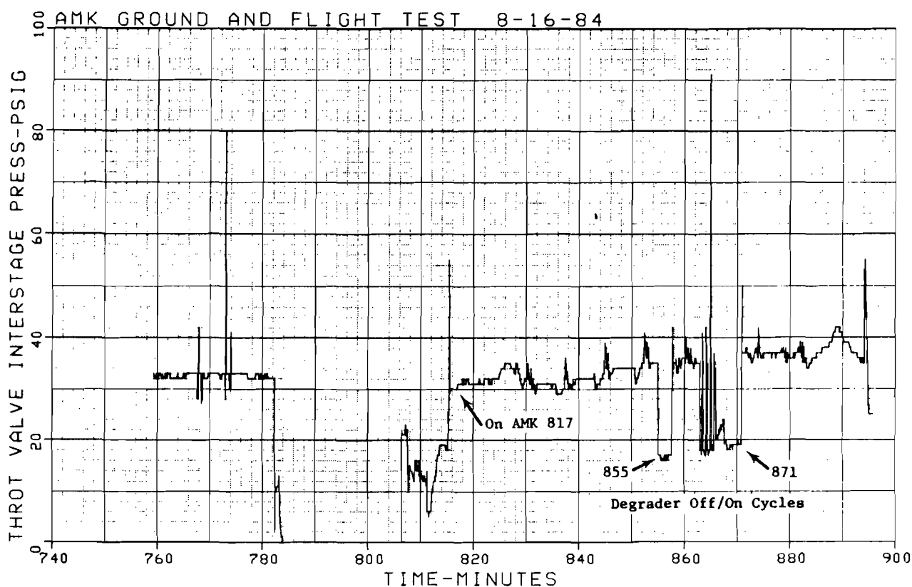
FIGURE 95. THROTTLING VALVE INTERSTAGE PRESSURE
