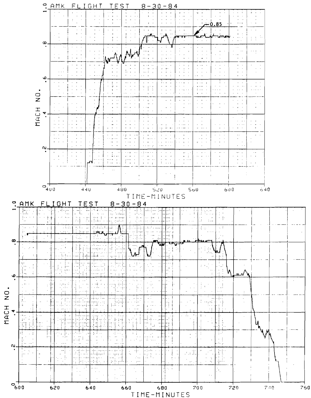
FIGURE 109. MACH NUMBER
