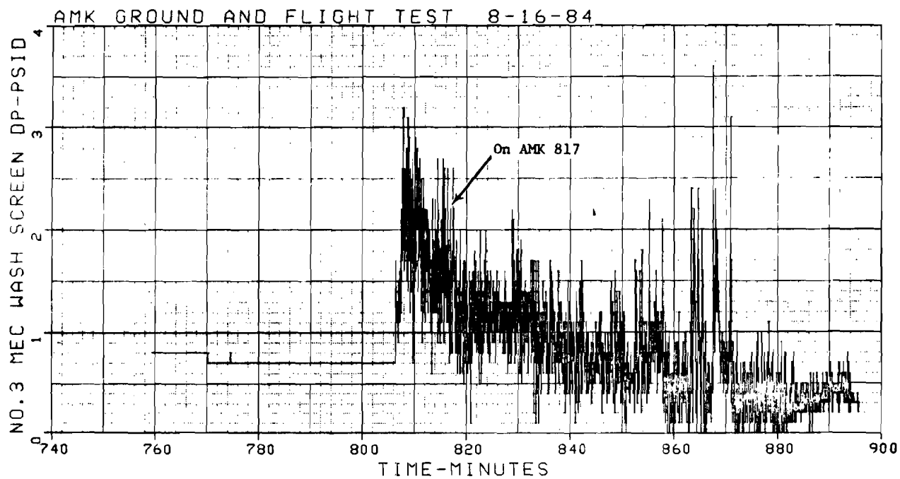
FIGURE 97. NUMBER 3 SERVO WASH SCREEN \Delta P
