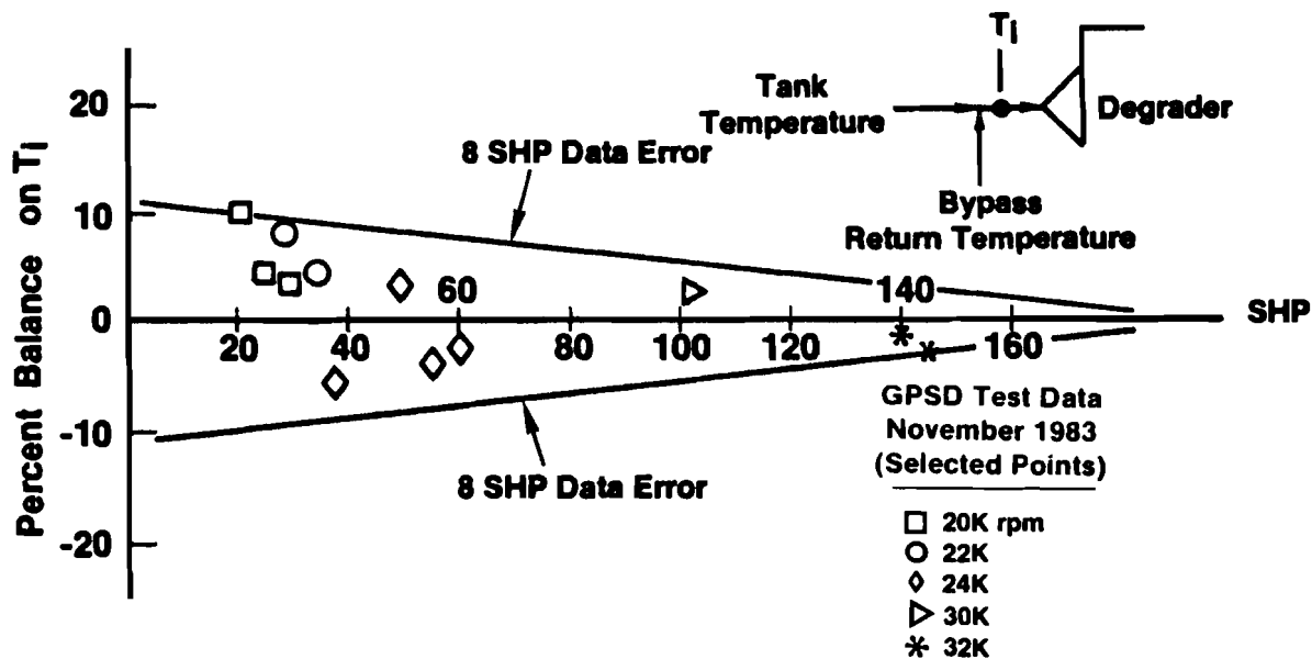
FIGURE 52. DEGRADER SHAFT HORSEPOWER CHECK
