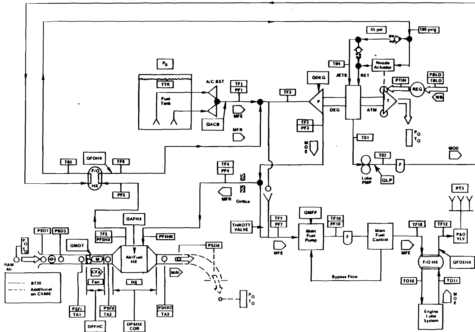
FIGURE 8. AMK DEGRADER/ENGINE COMPUTER MODEL
