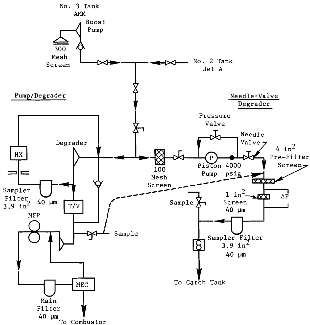
FIGURE 99. TEST SETUP FOR COMPARISON OF DEGRADERS
