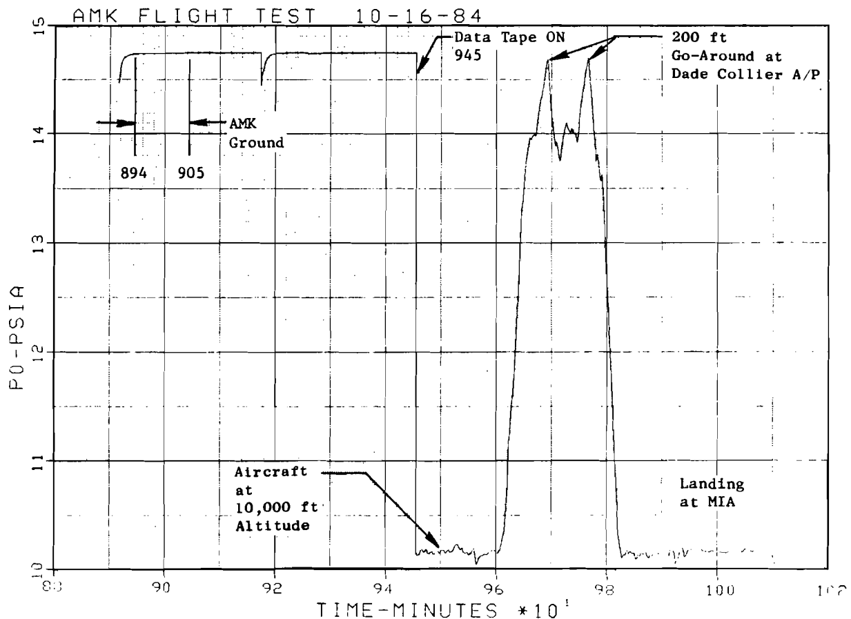
FIGURE 126. ALTITUDE PRESSURE
