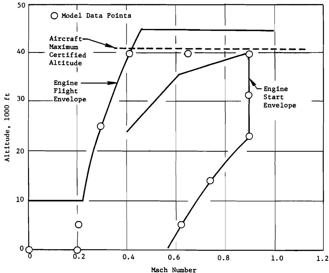
FIGURE 9. ENGINE FLIGHT ENVELOPE DATA POINTS FOR COMPUTER MODEL
