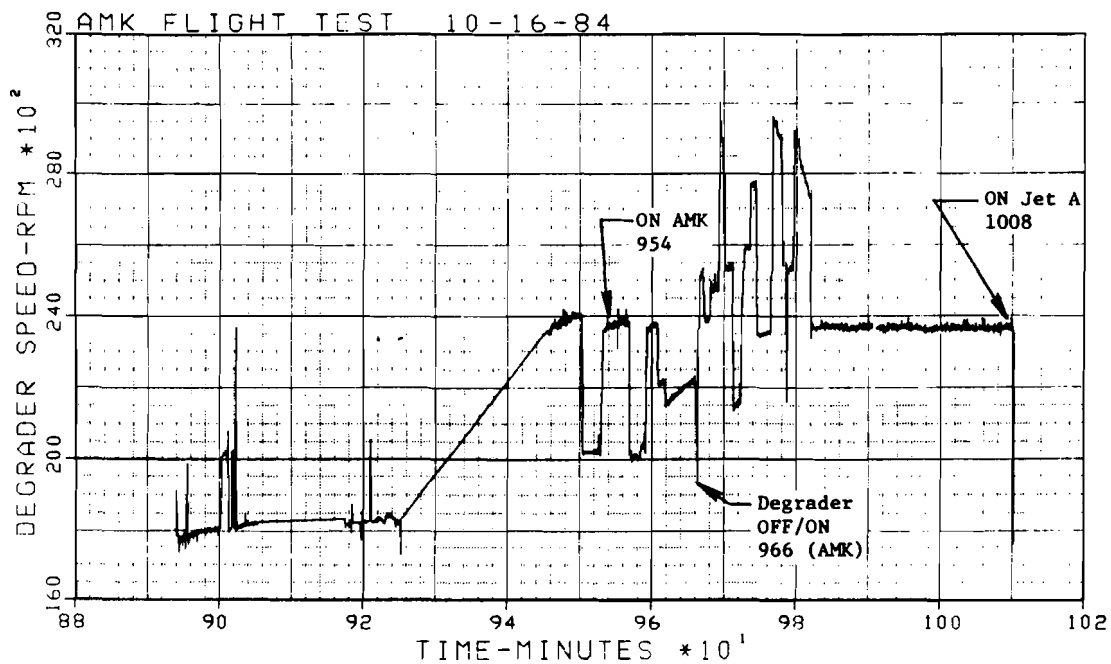
FIGURE 128. DEGRADER SPEED
