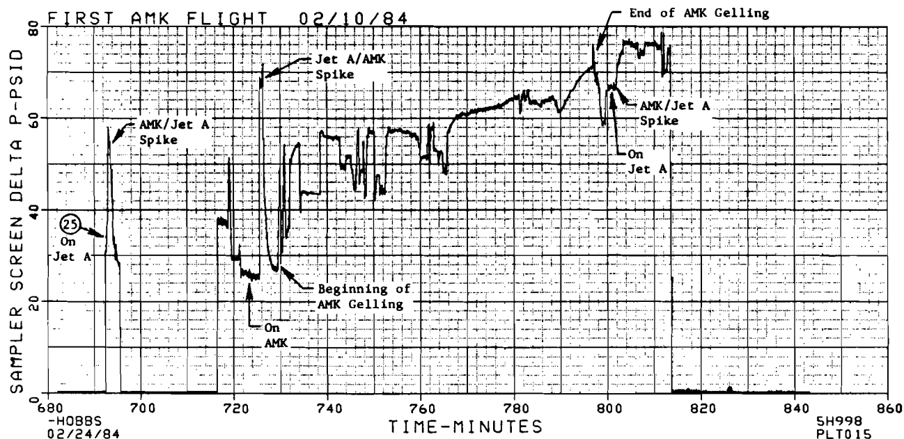
FIGURE 55. DEGRADER RECIRCULATION SAMPLER FILTER \Delta P - FUNCTION OF DEGRADER PRESSURE
