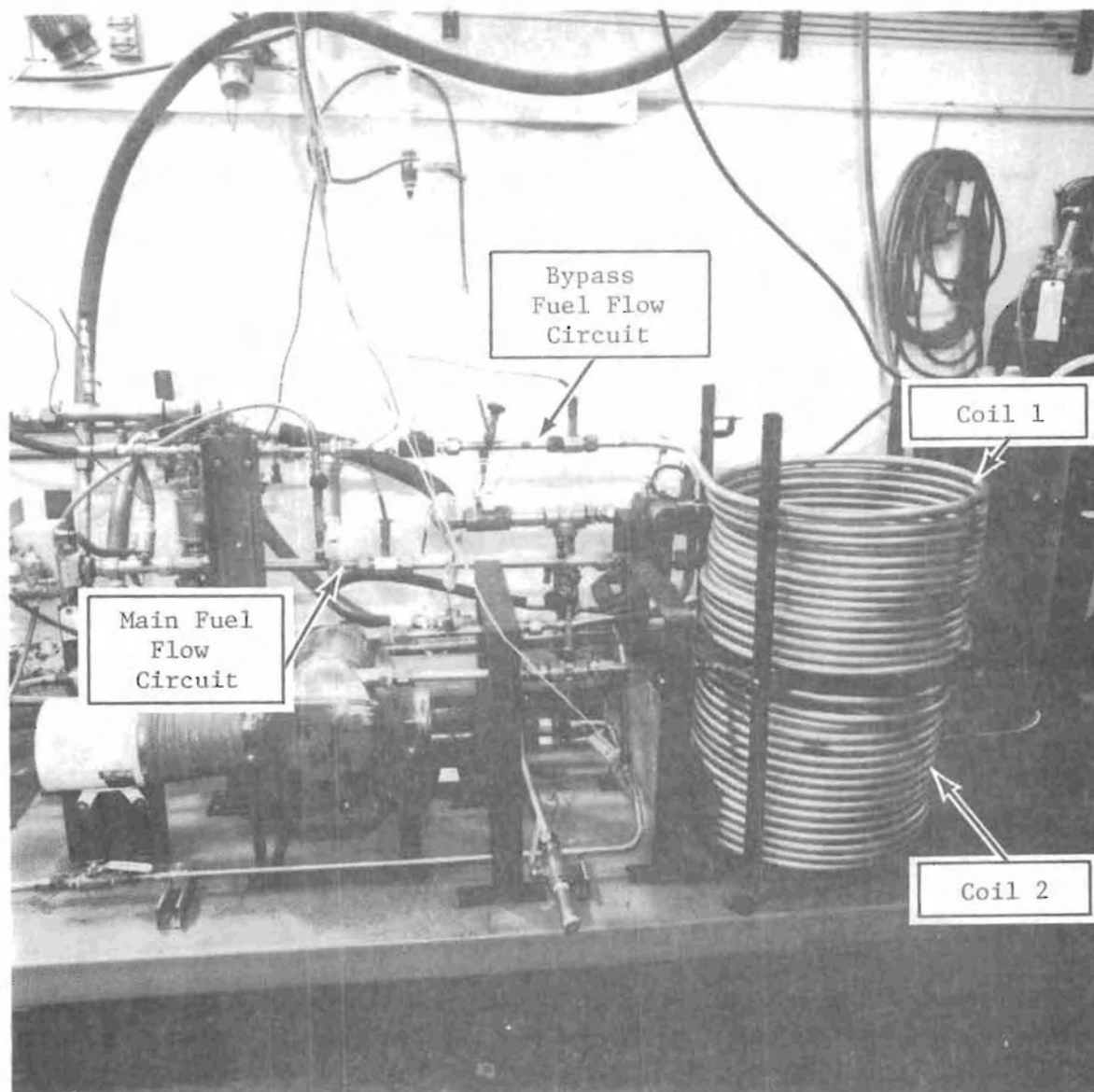
FIGURE 45. FUEL FLOW CIRCUITS
