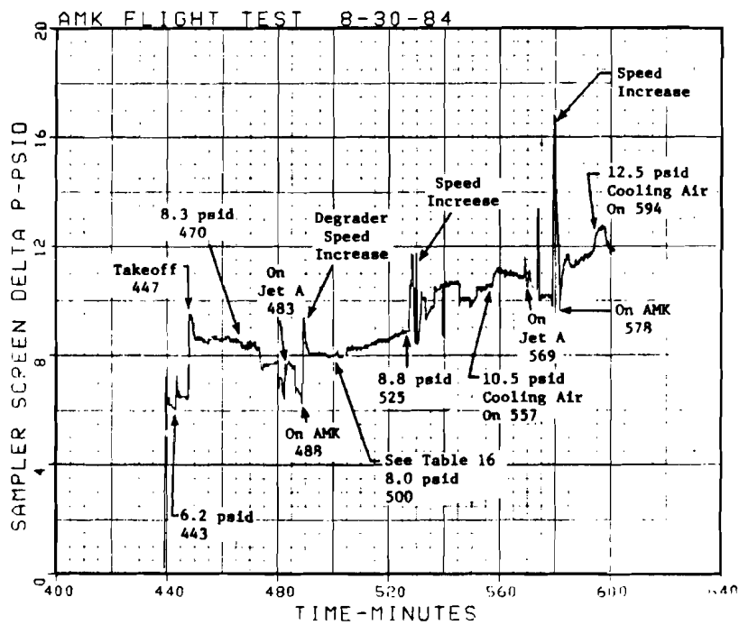
FIGURE 114. SAMPLER FILTER \Delta P
