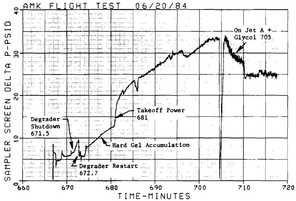
FIGURE 75. SAMPLER FILTER \Delta P
