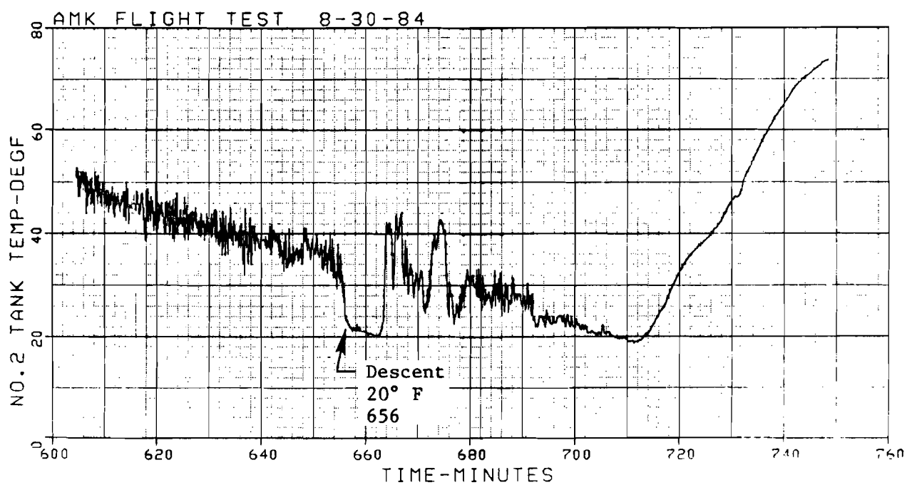
FIGURE 111. NUMBER 2 TANK TEMPERATURE
