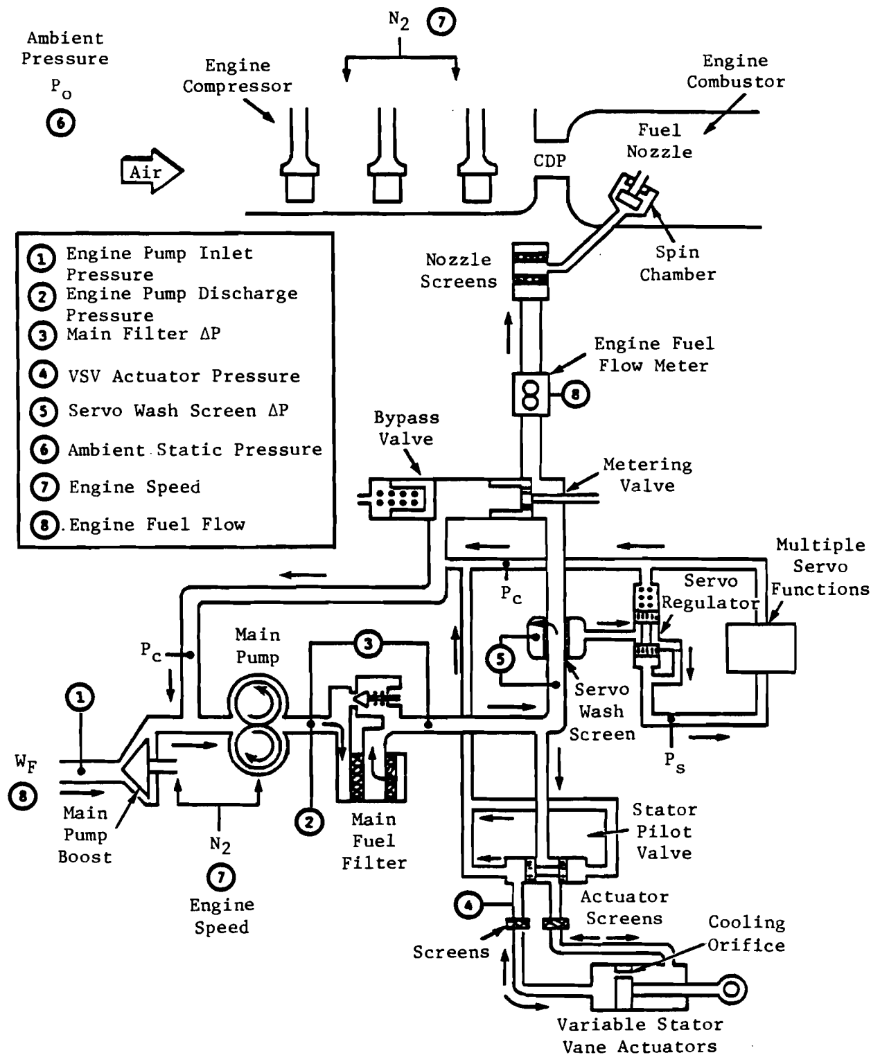
FIGURE 69. ENGINE FUEL SYSTEM SCHEMATIC
