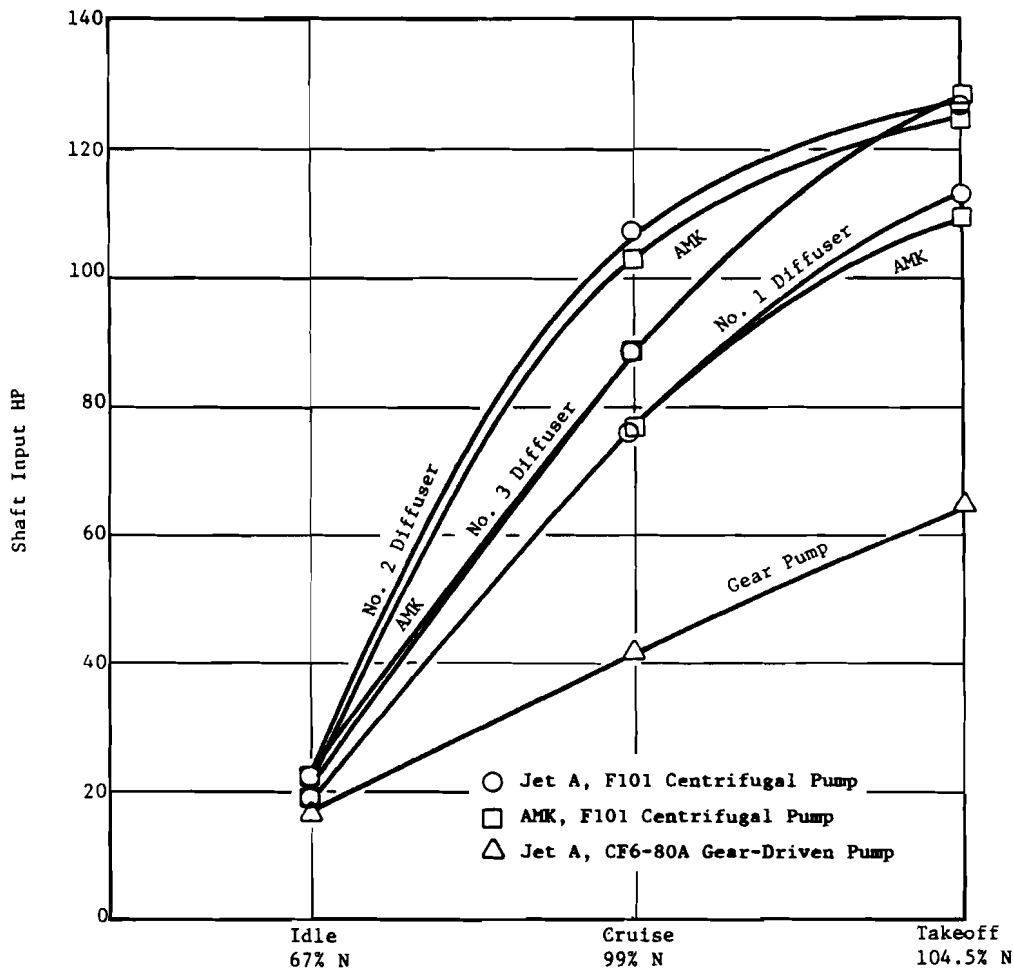
FIGURE 4. DEGRADER/PUMP POWER REQUIREMENTS
