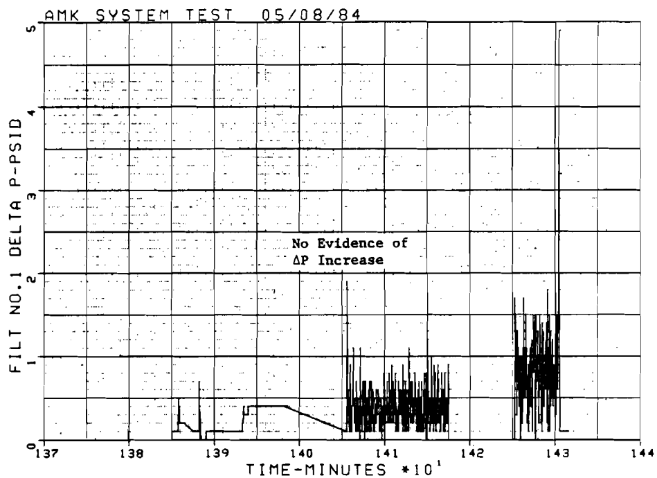
FIGURE 58. NUMBER 1 (MAIN) FILTER ΔP
