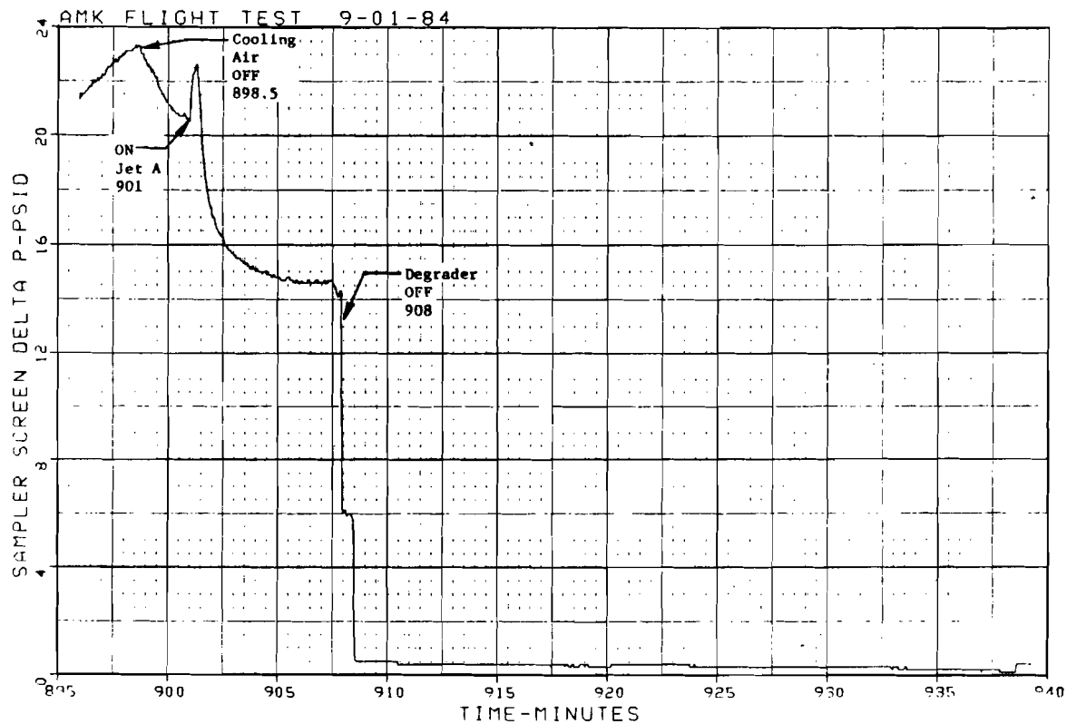
FIGURE 119. SAMPLER FILTER \Delta P
