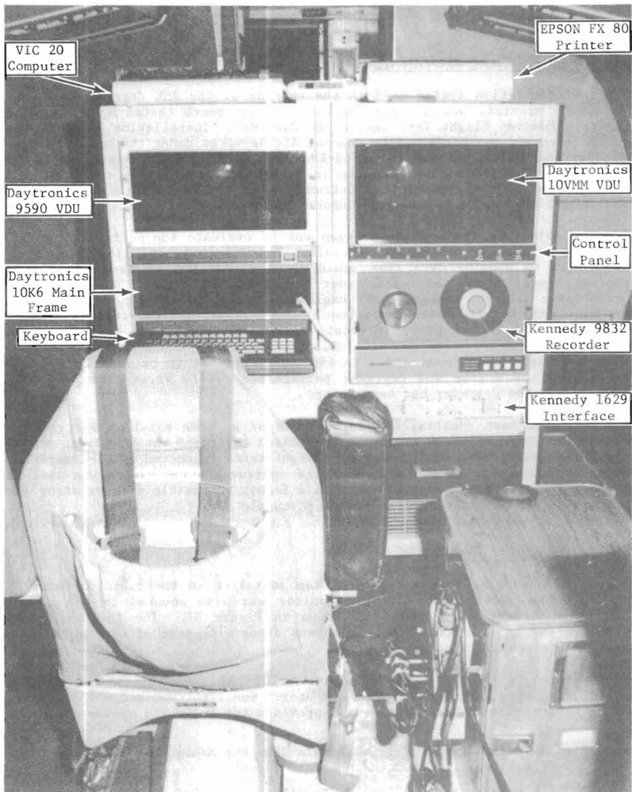
FIGURE 36. ONBOARD INSTRUMENTATION DATA SYSTEM
