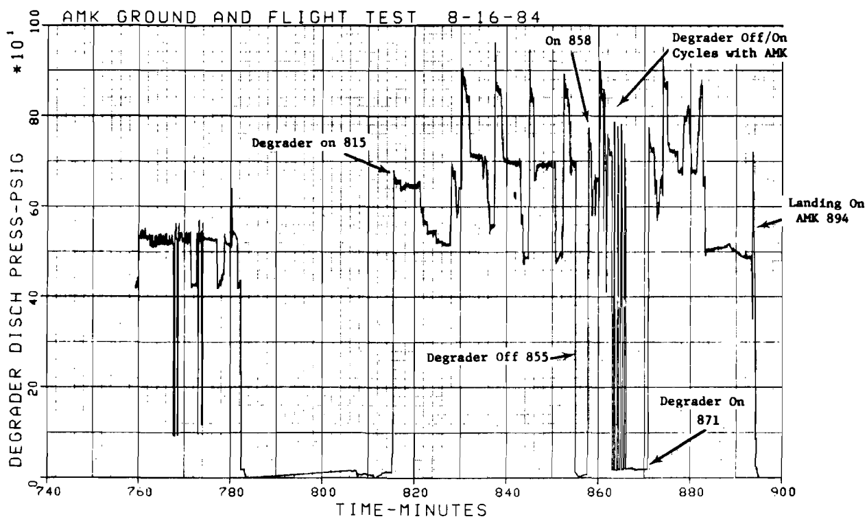
FIGURE 94. DEGRADER FUEL DISCHARGE PRESSURE
