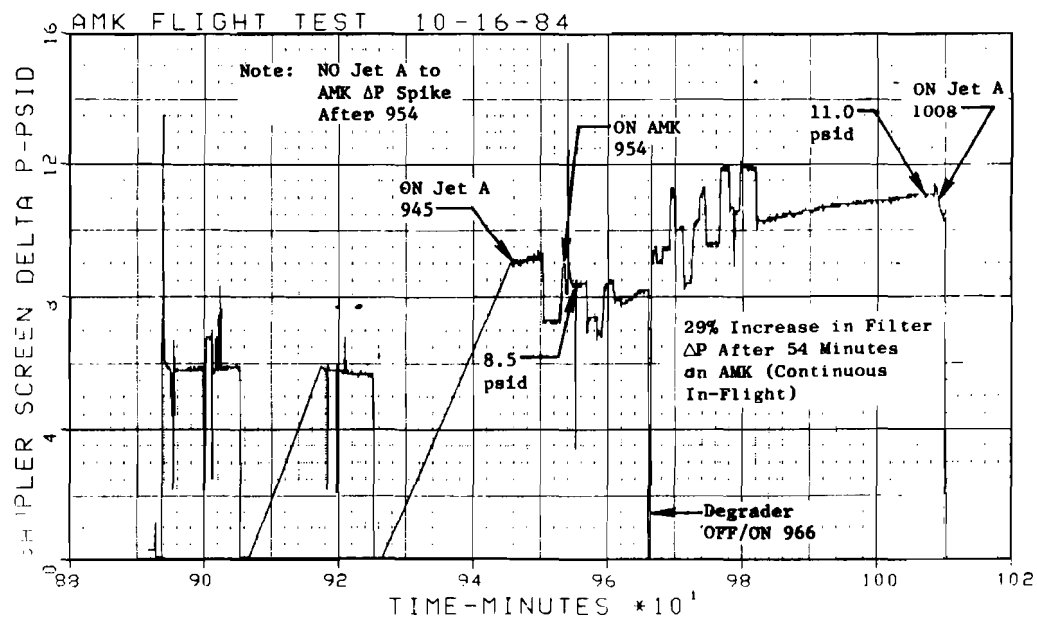
FIGURE 129. SAMPLER FILTER \Delta P
