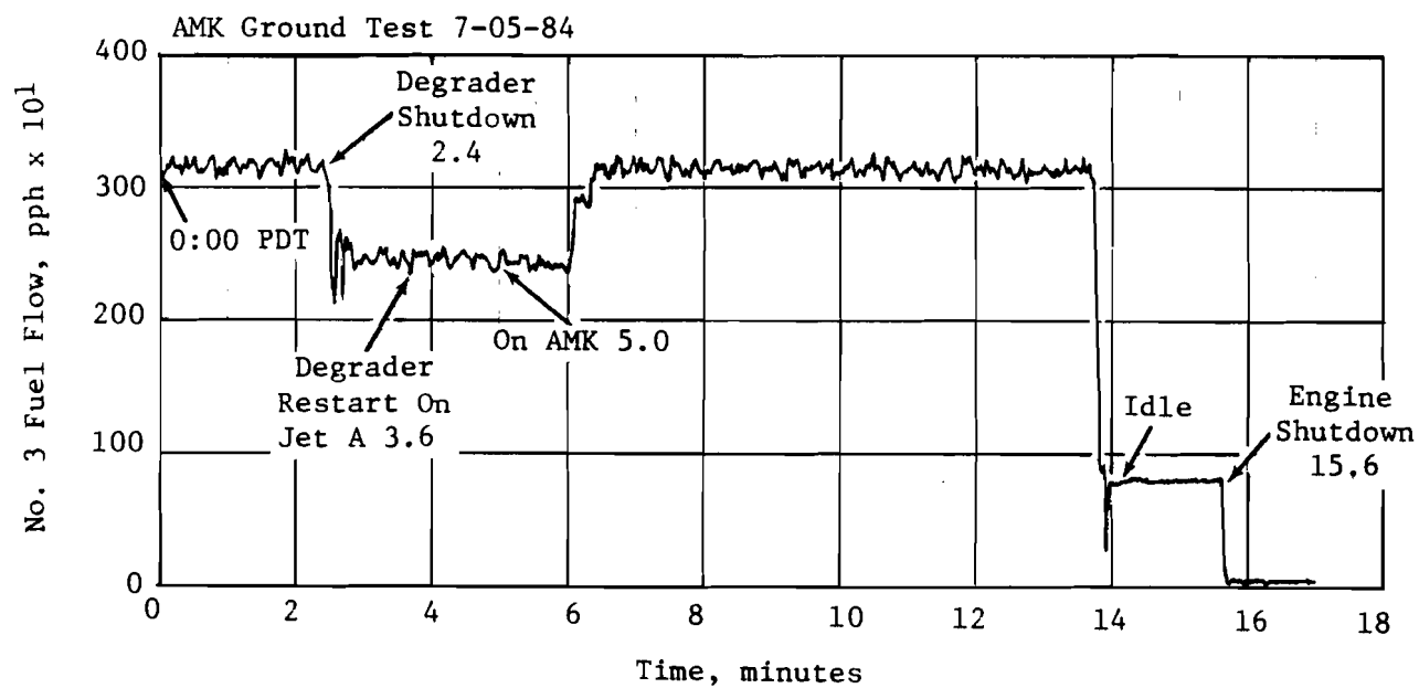
FIGURE 100. FUEL FLOW
