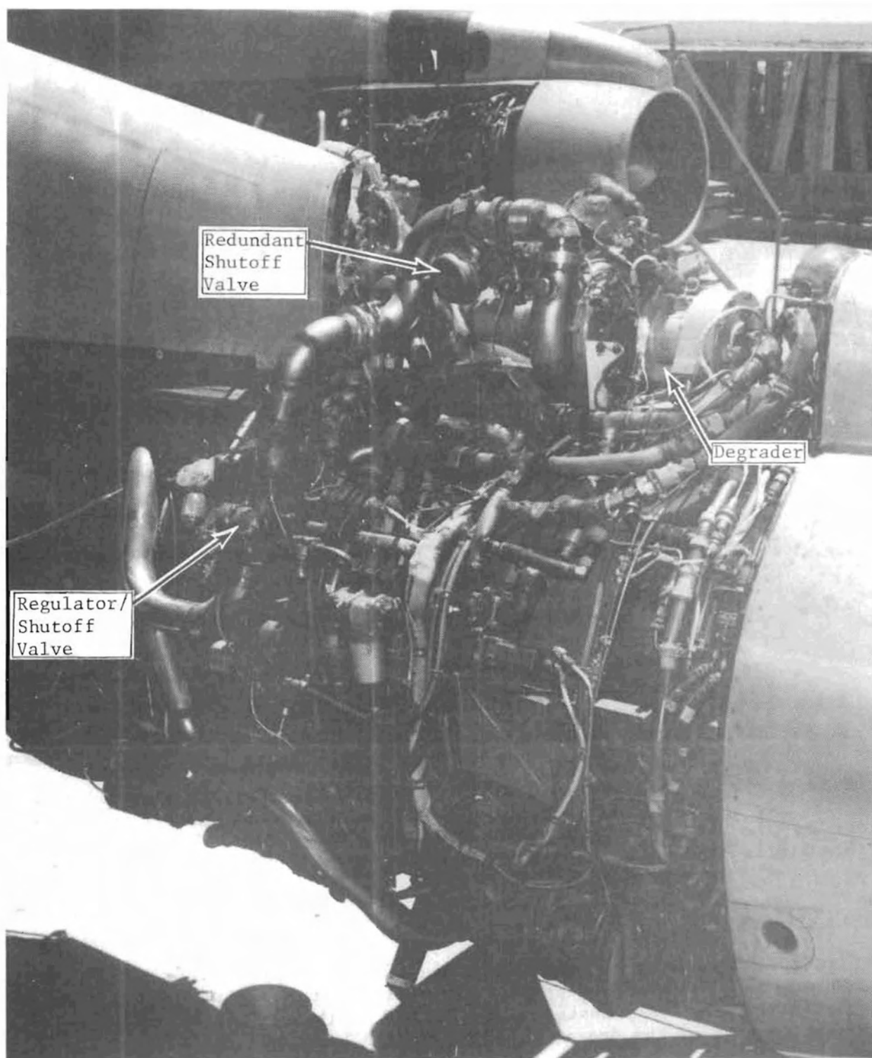
FIGURE 134. B720 PUMP/DEGRADER INSTALLATION
