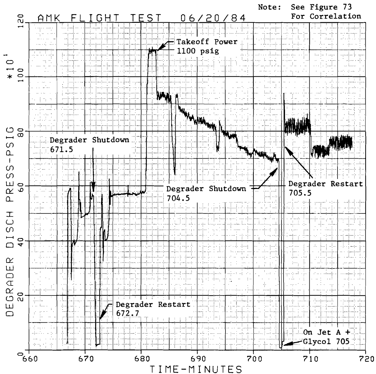
FIGURE 74. DEGRADER FUEL DISCHARGE PRESSURE
