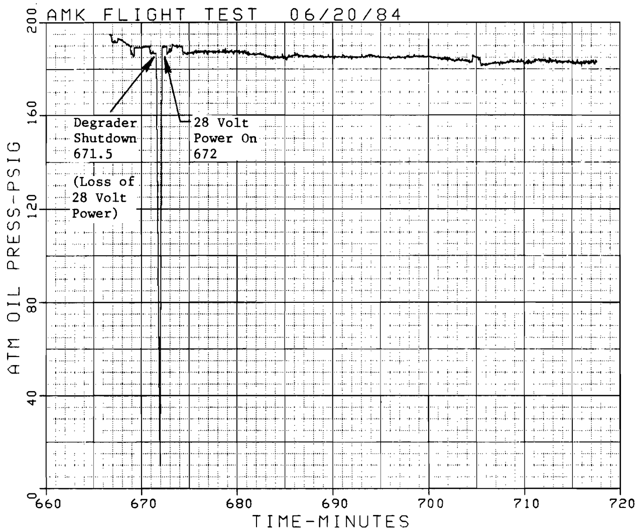
FIGURE 81. DEGRADER OIL PRESSURE
