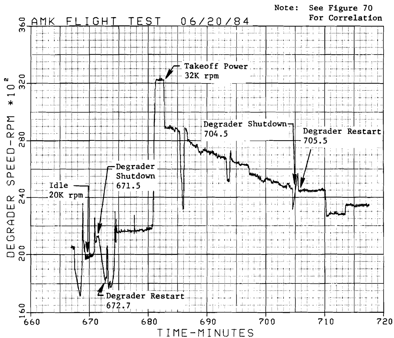
FIGURE 73. DEGRADER SPEED
