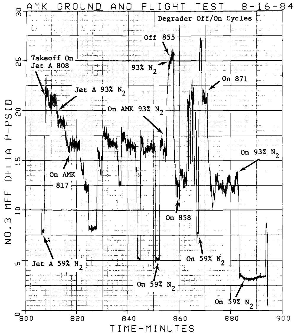
FIGURE 98. NUMBER 3 ENGINE MAIN FUEL FILTER \Delta P
