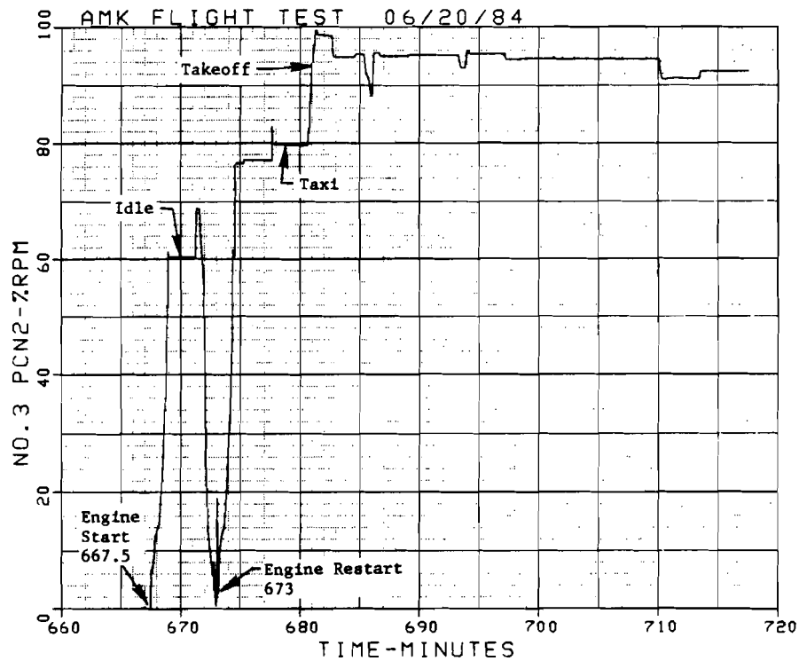
FIGURE 76. NUMBER 3 ENGINE SPEED
