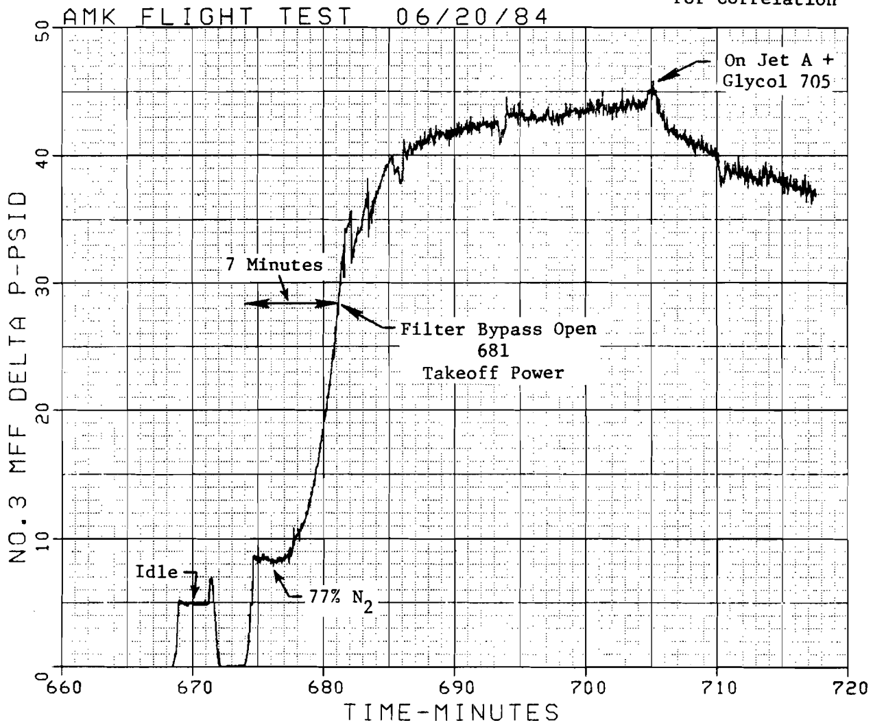
FIGURE 77. NUMBER 3 ENGINE MAIN FILTER \Delta P
