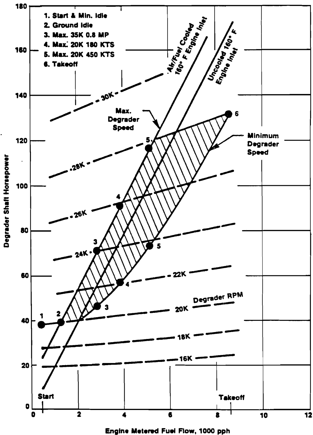
FIGURE 12. CJ805 DEGRADER SPEED SCHEDULE RELATIONSHIP TO FLOW AND POWER
