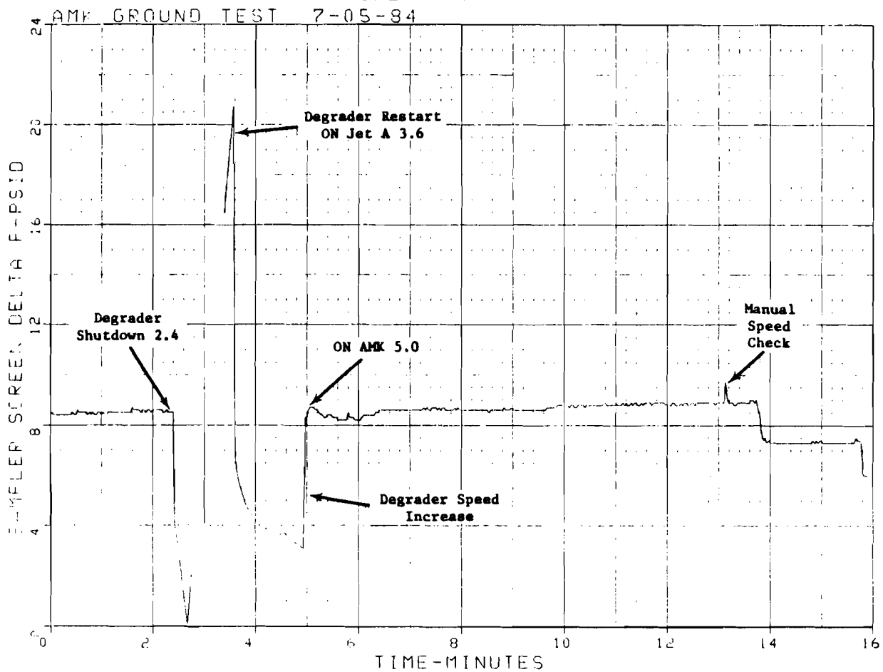
FIGURE 101. SAMPLER FILTER \Delta P
