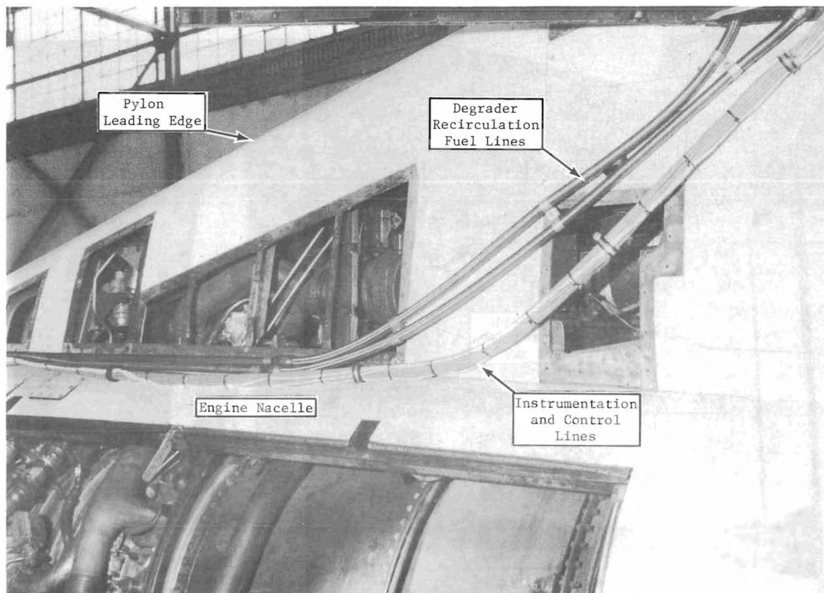
FIGURE 24. INSTALLATION OF CONTROL AND FUEL LINES, NO. 3 PYLON
