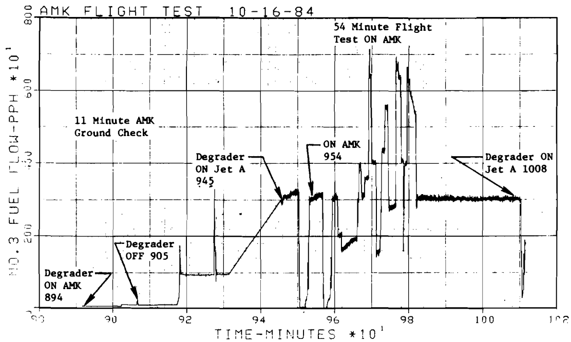
FIGURE 127. NUMBER 3 ENGINE FUEL FLOW
