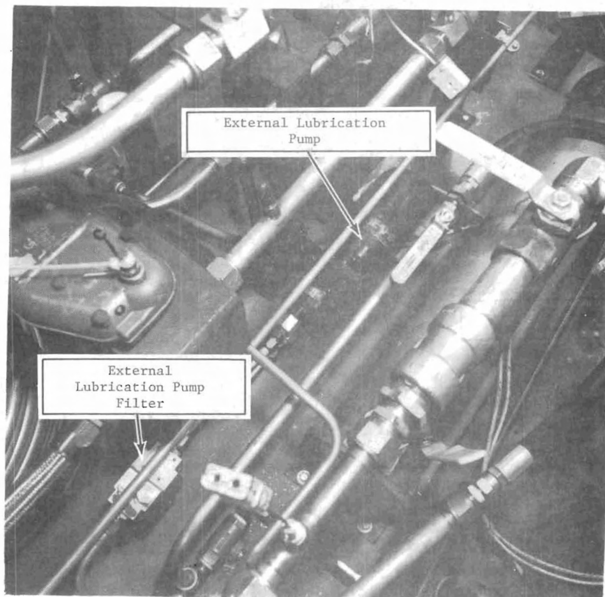
FIGURE 47. LUBE PUMP AND FILTER
