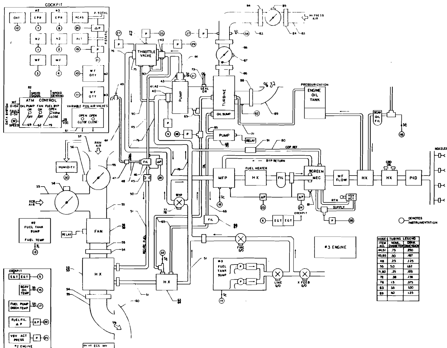
FIGURE 25. CV880 AMK INSTALLATION SCHEMATIC
