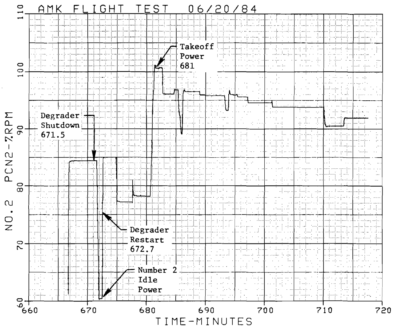
FIGURE 78. NUMBER 2 ENGINE SPEED
