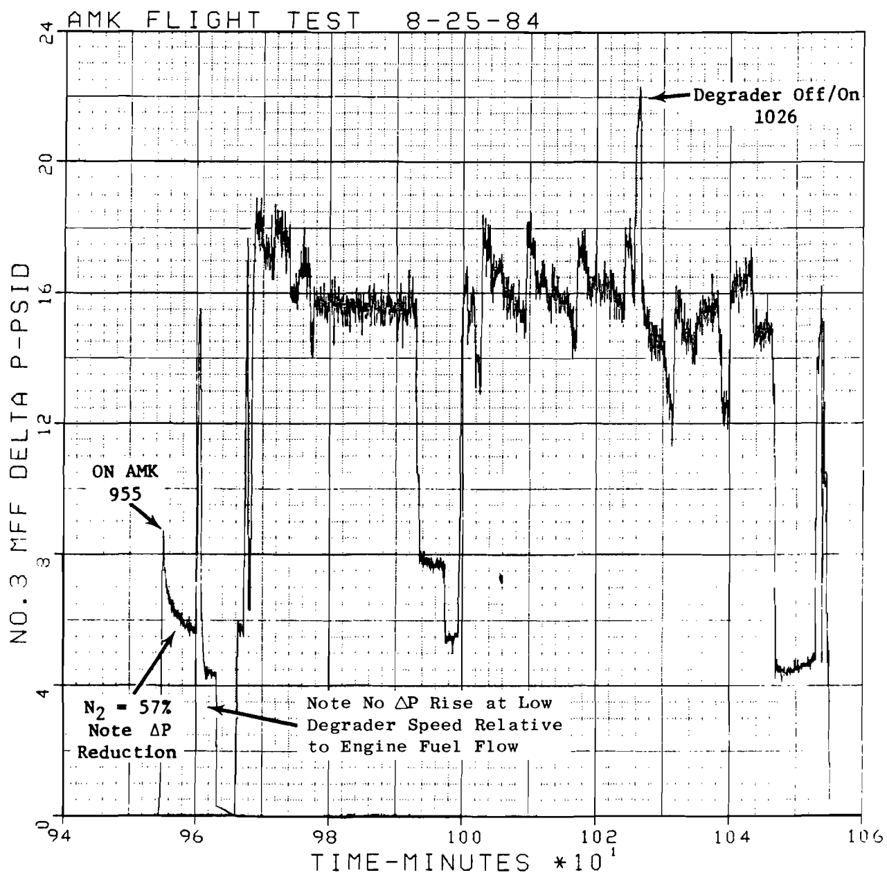
FIGURE 102. NUMBER 3 ENGINE MAIN FUEL FILTER \Delta P
