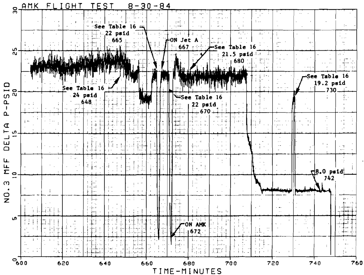
FIGURE 113. NUMBER 3 ENGINE MAIN FUEL FILTER \Delta P
