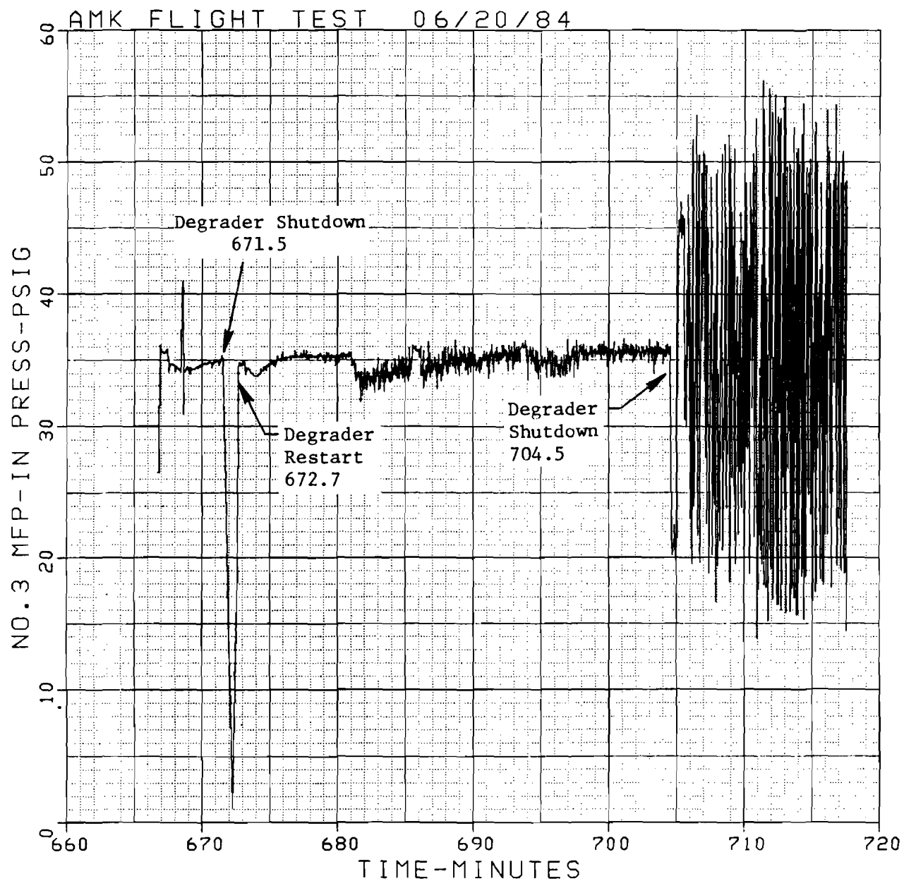
FIGURE 82. NUMBER 3 ENGINE FUEL PUMP INLET PRESSURE
