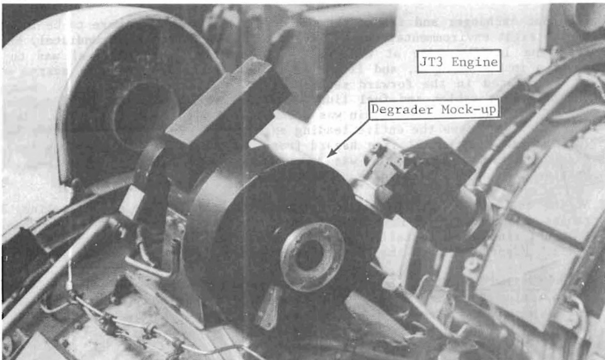
FIGURE 22. INSTALLATION OF DEGRADER MOCK-UPS
