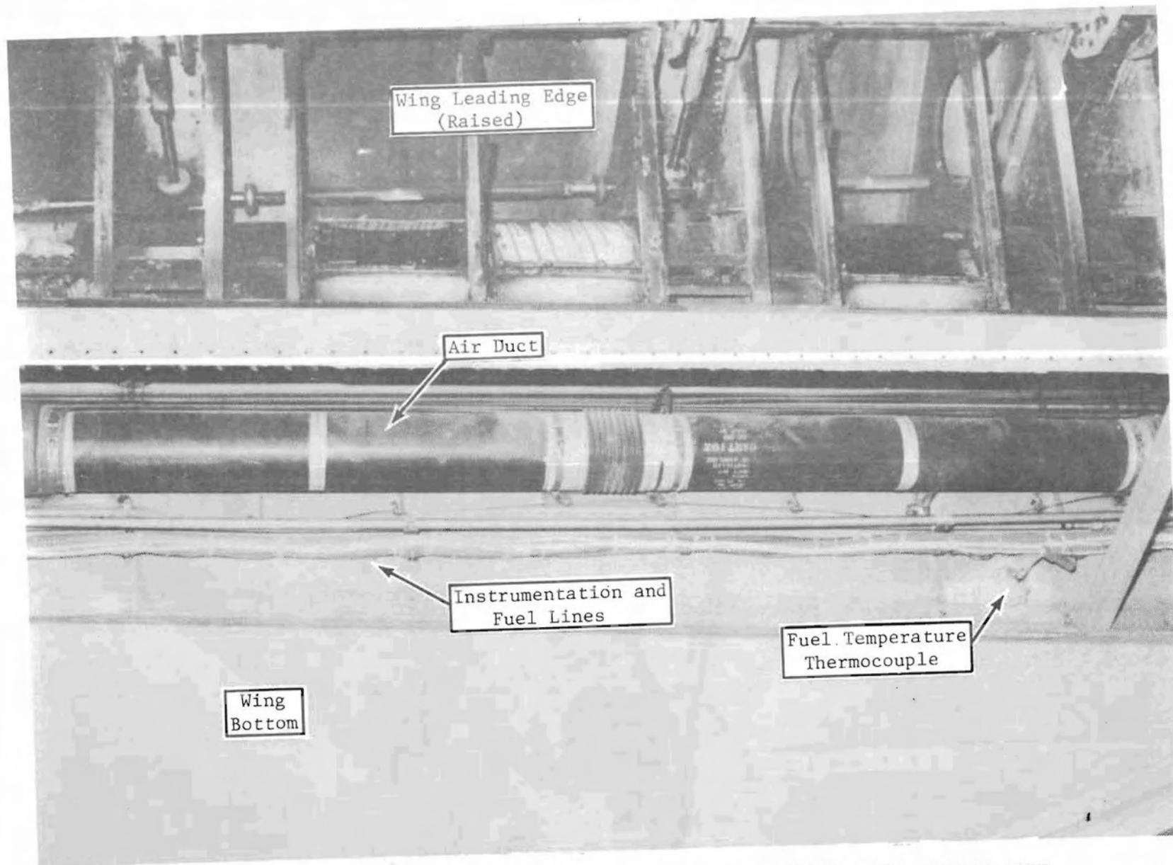
FIGURE 30. ROUTING OF INSTRUMENTATION AND FUEL LINES WITHIN WING LEADING EDGE
