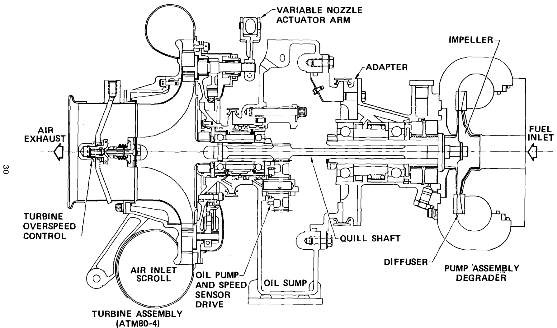
FIGURE 15. CROSS SECTION OF DEGRADER ASSEMBLY ATMP80-1
