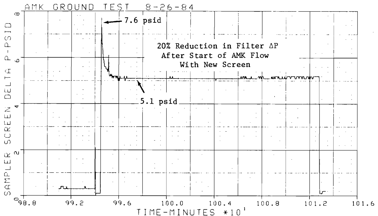
FIGURE 106. SAMPLER FILTER \Delta P
