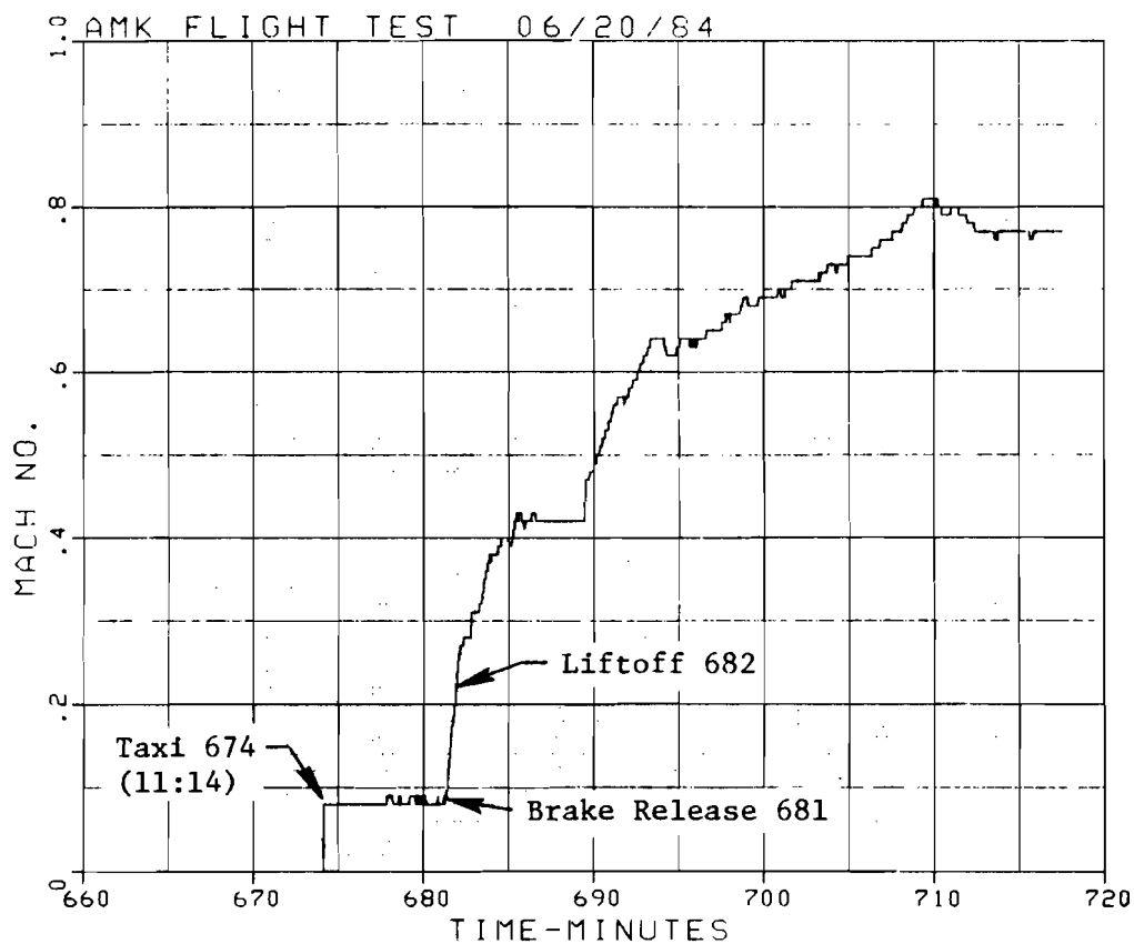
FIGURE 72. MACH NUMBER
