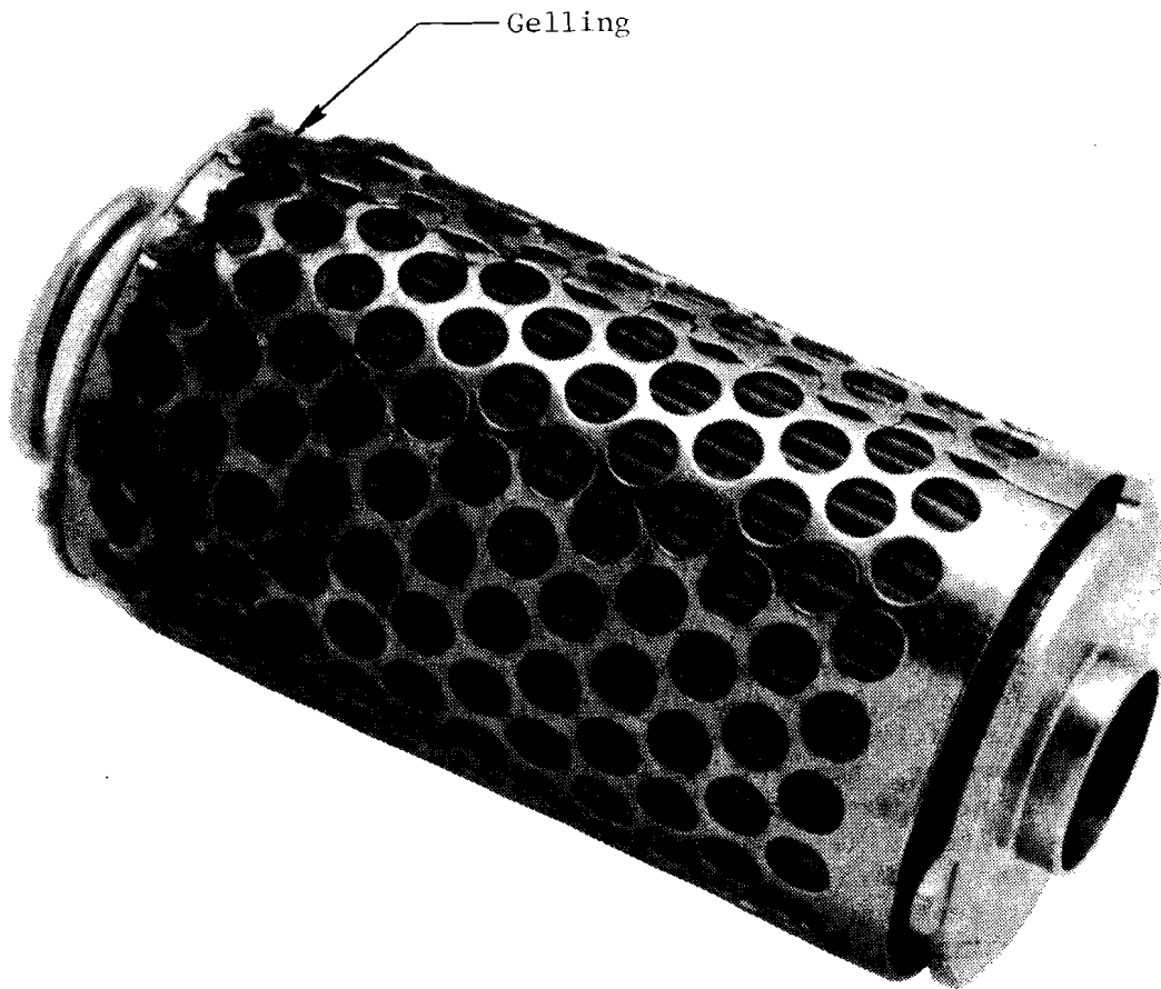
FIGURE 50. FUEL BYPASS FILTER SHOWING EVIDENCE OF AMK PRECIPITATE GEL
