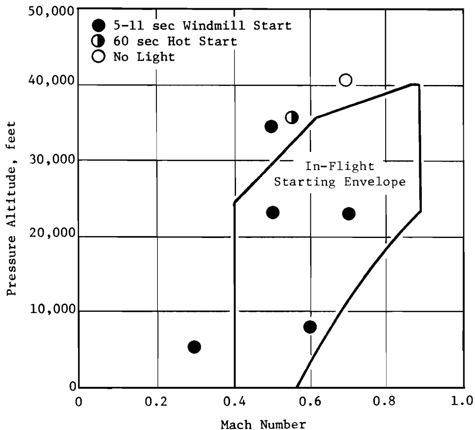
FIGURE 41. CV880 ENGINE IN-FLIGHT STARTING ENVELOPE
