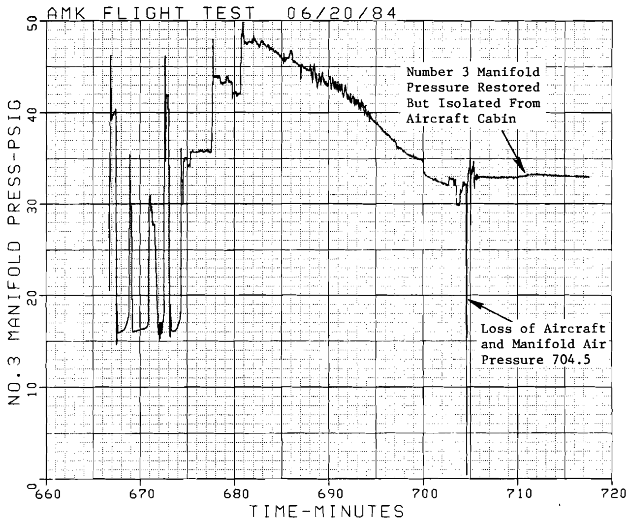
FIGURE 80. AIR MANIFOLD PRESSURE
