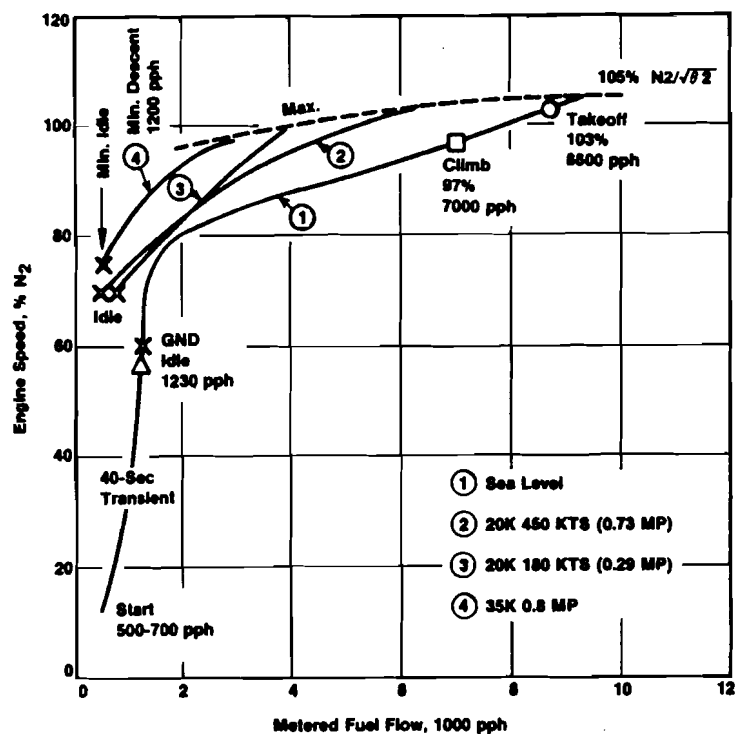
FIGURE 13. CJ805 ENGINE UNCORRECTED SPEED VERSUS FUEL FLOW - STANDARD DAY
