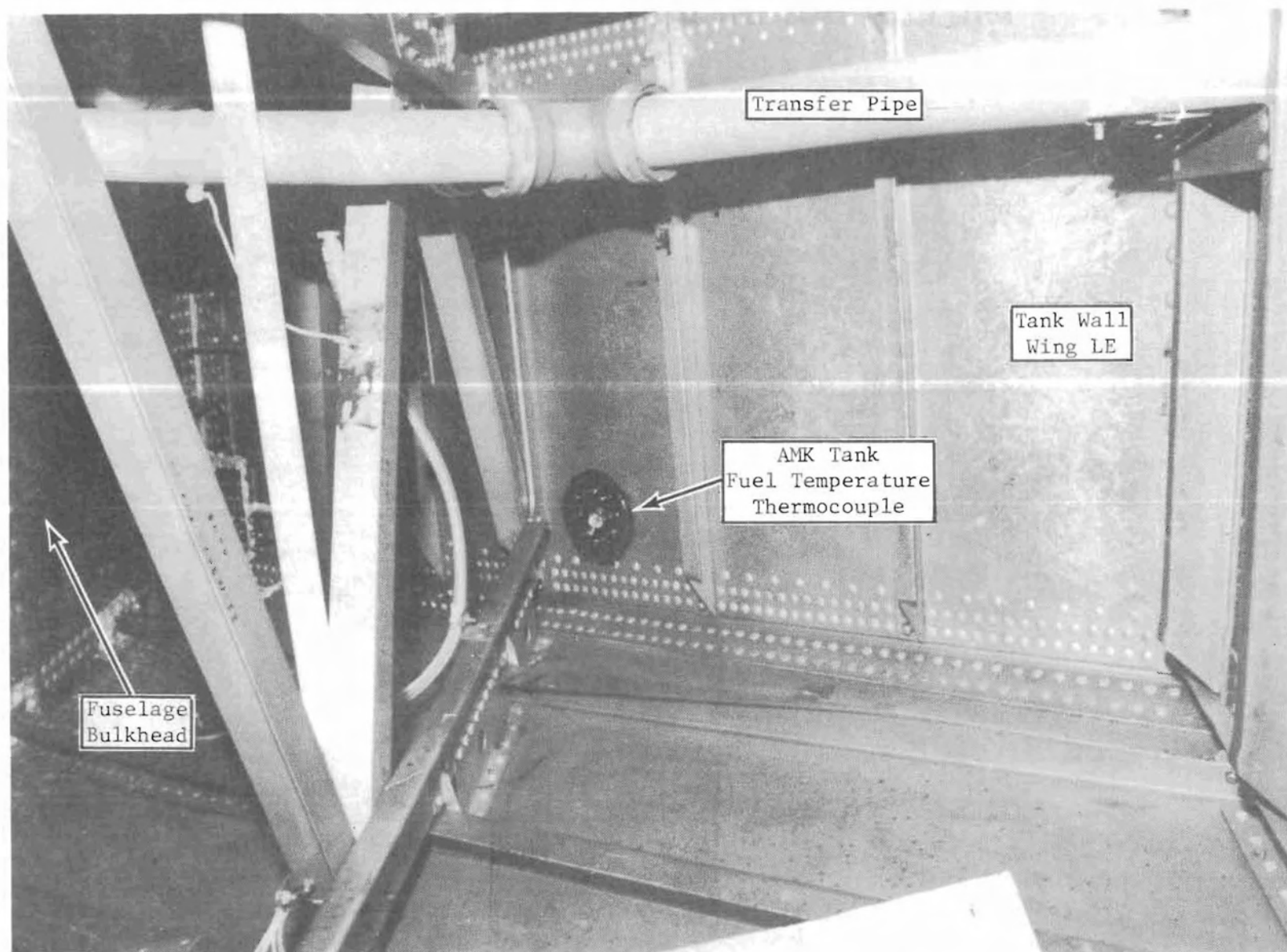
FIGURE 23. INTERIOR OF NUMBER 3 WING TANK
