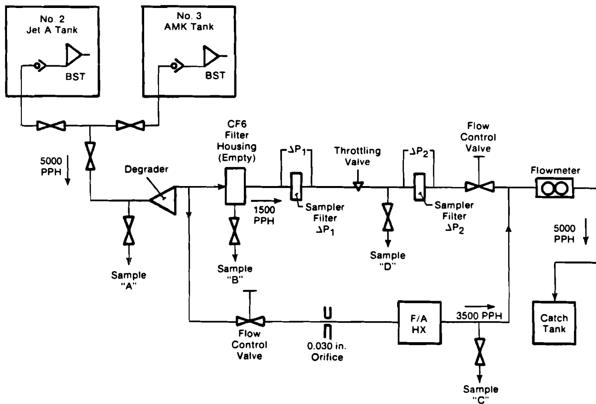
FIGURE 61. CONFIGURATION FOR MARCH 3, 1984 SYSTEM TEST
