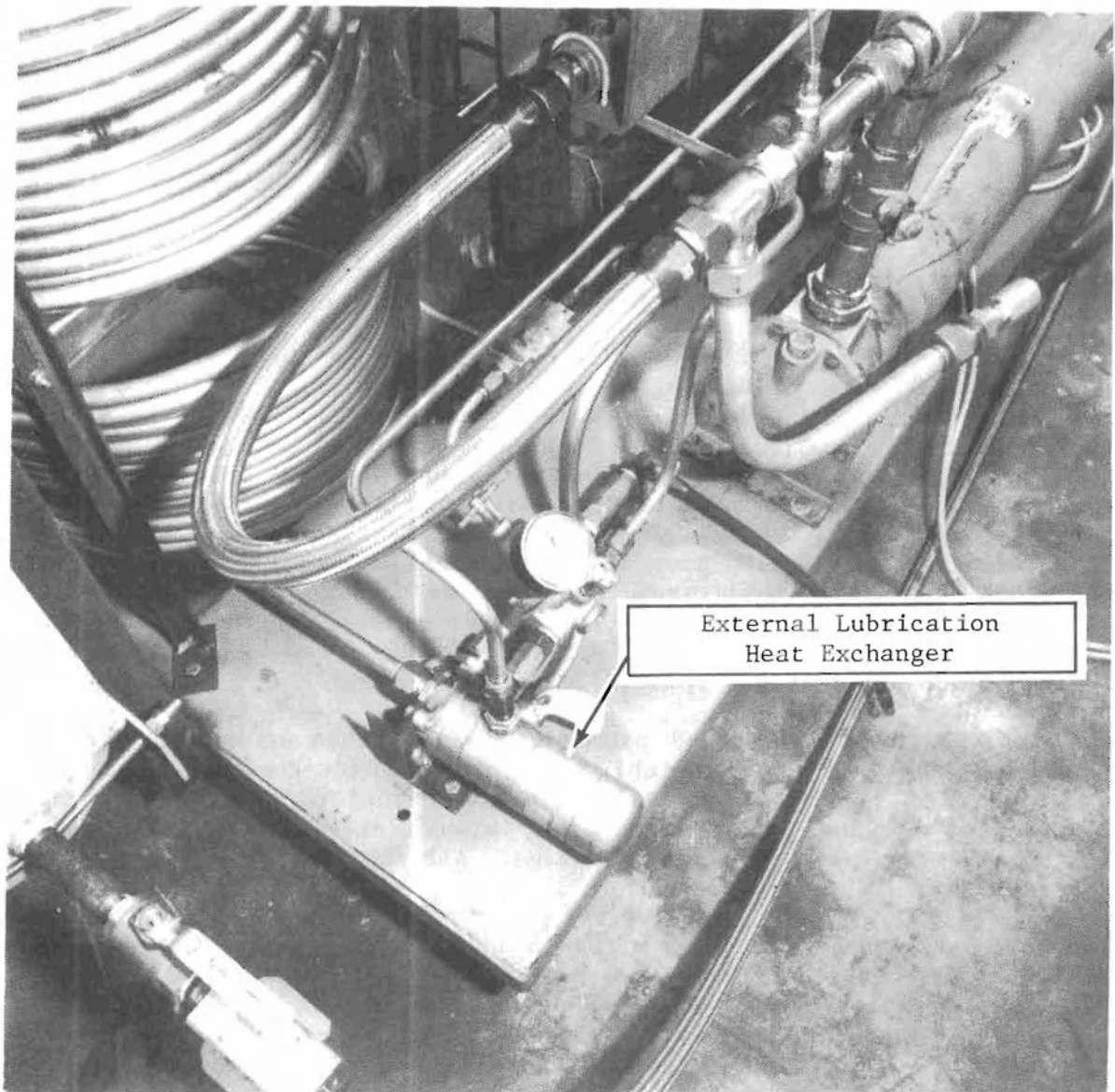
FIGURE 48. LUBE SYSTEM OIL/FUEL HEAT EXCHANGER
