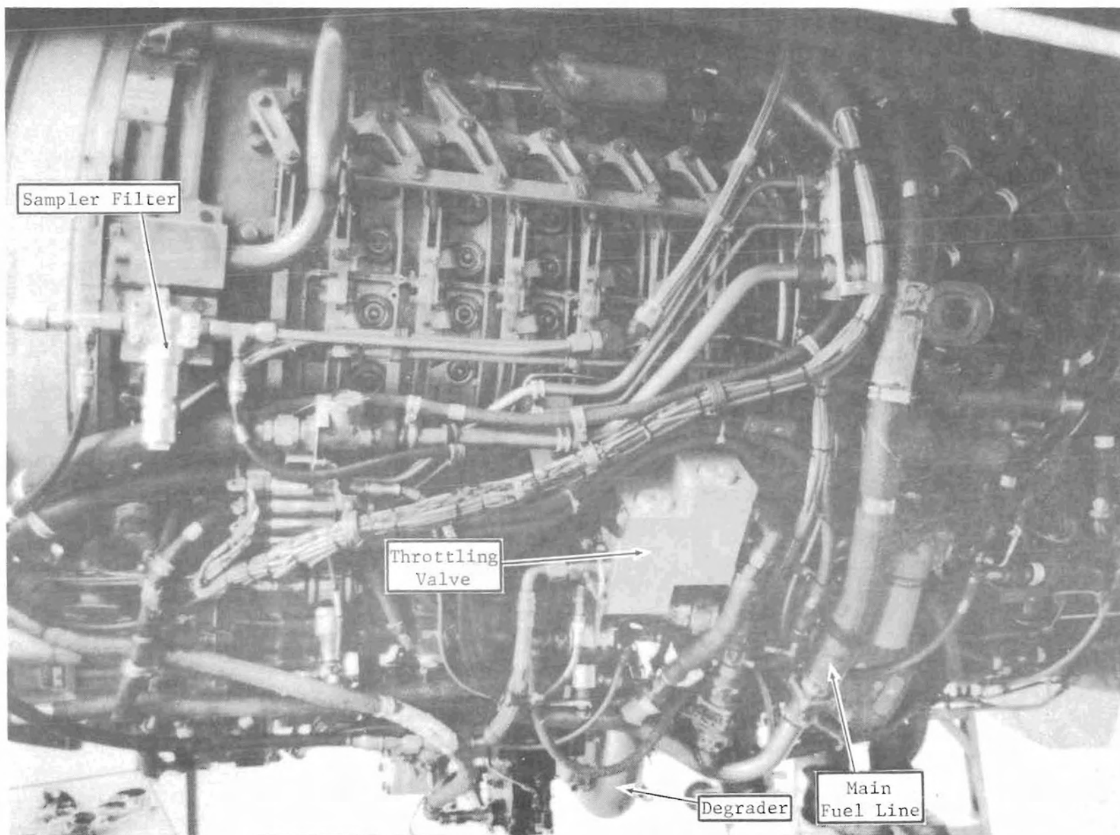
FIGURE 27. OVERALL VIEW LEFT SIDE OF NUMBER 3 ENGINE
