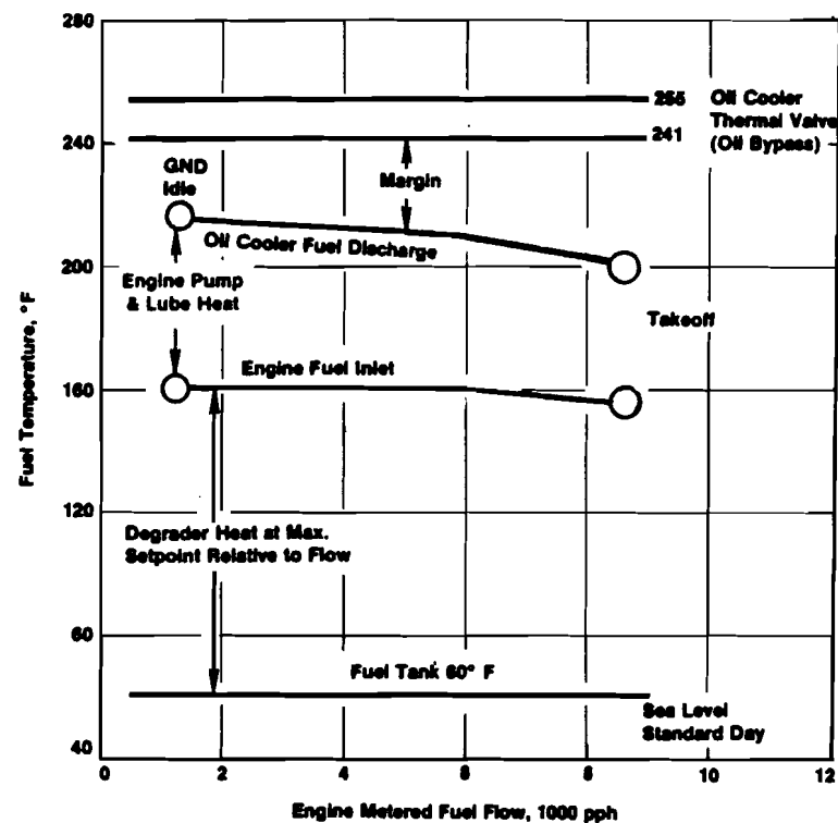
FIGURE 14. FUEL TEMPERATURE LIMITS
