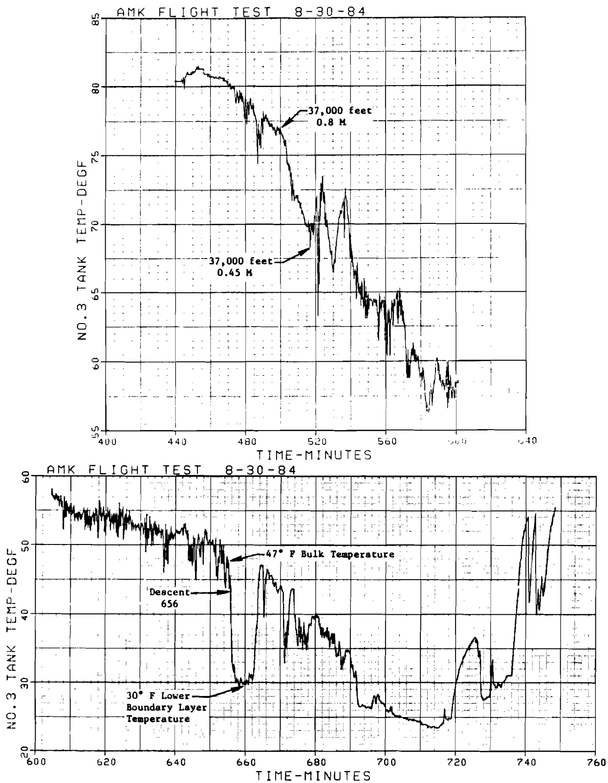
FIGURE 110. NUMBER 3 TANK TEMPERATURE
