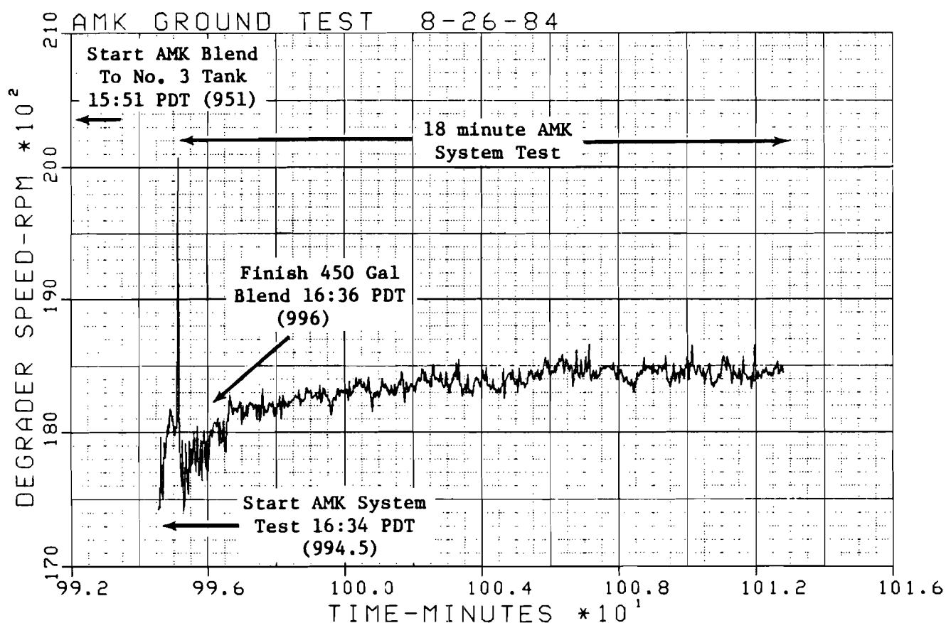
FIGURE 104. DEGRADER SPEED
