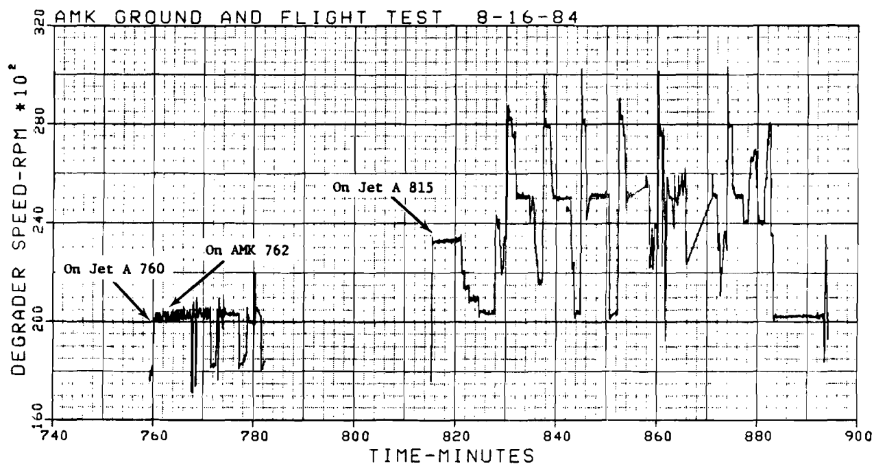
FIGURE 90. DEGRADER SPEED
