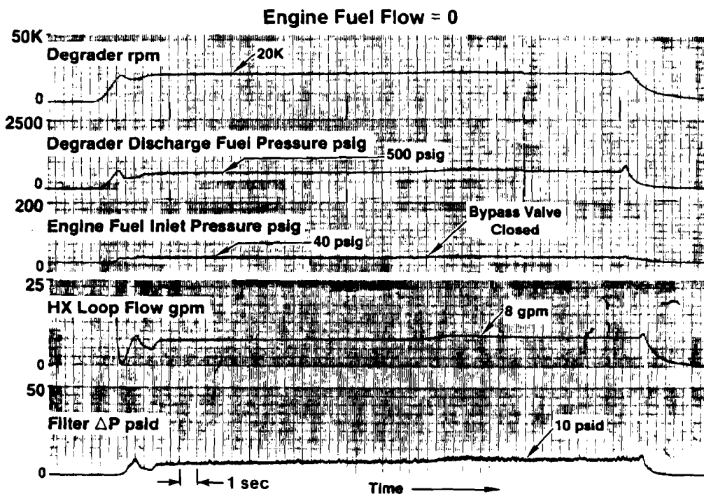
FIGURE 53. FILTER \Delta P RESULTS DURING START-UP
