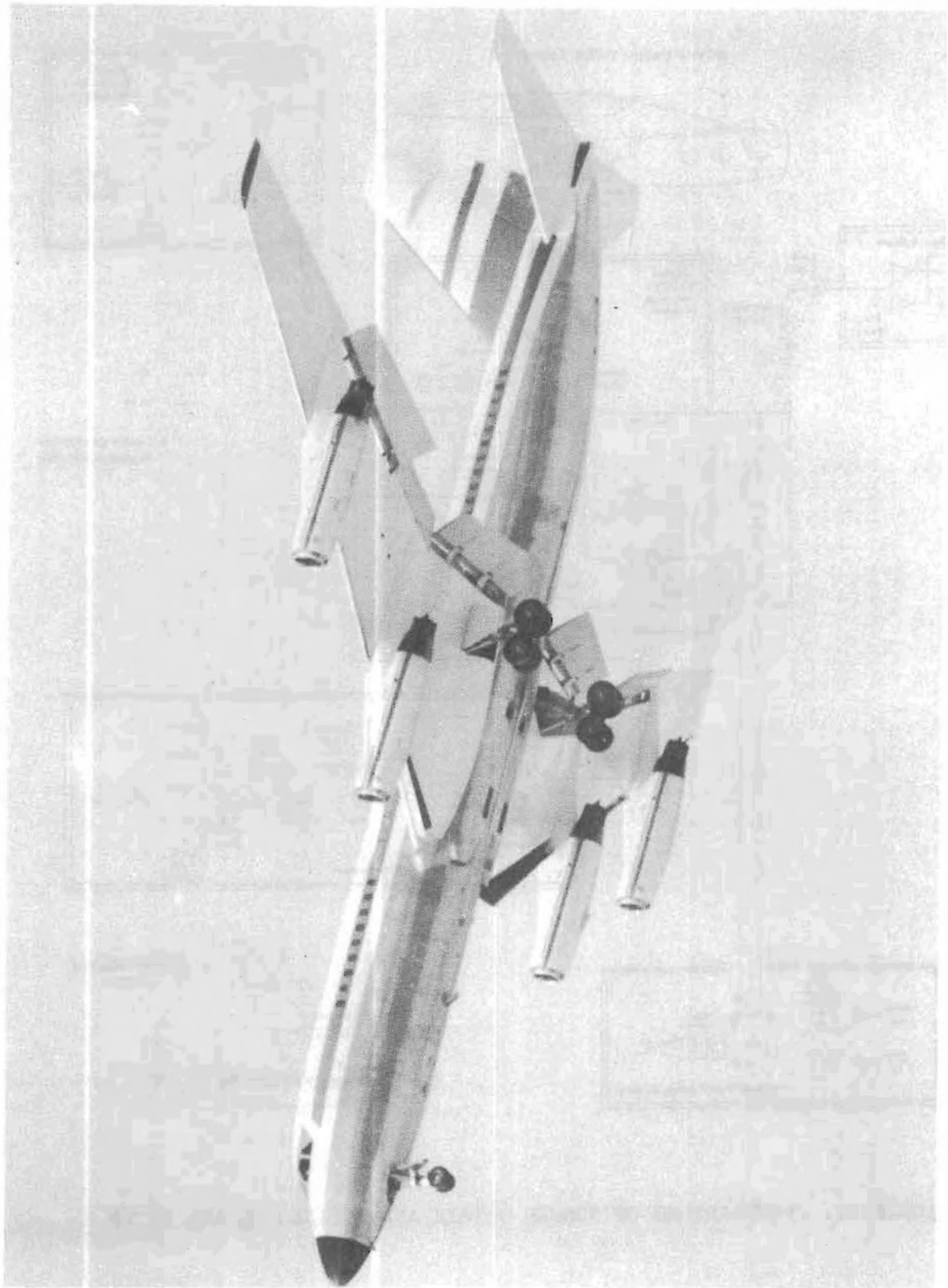
FIGURE 20. CV880 DEGRADER FLIGHT TEST VEHICLE
