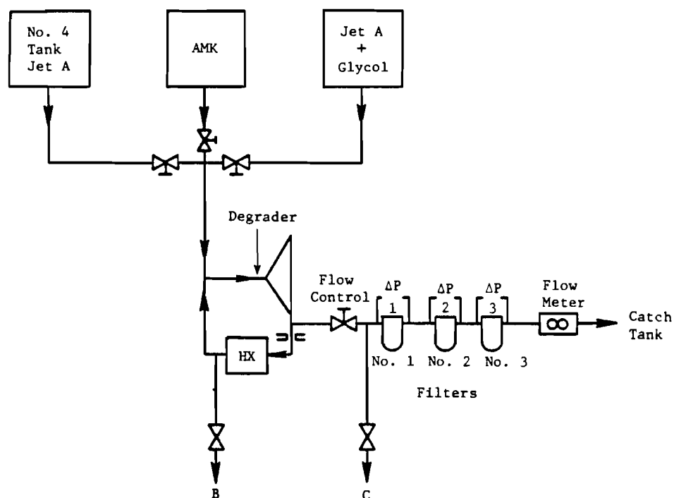
FIGURE 56. SYSTEM TEST SETUP
