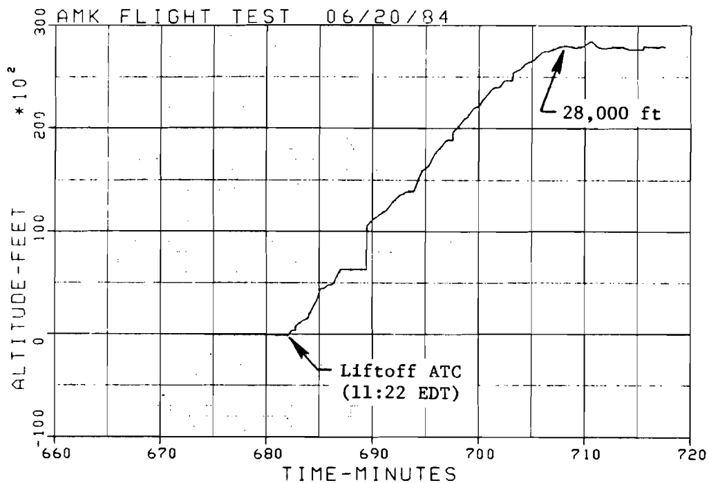
FIGURE 71. PRESSURE ALTITUDE
