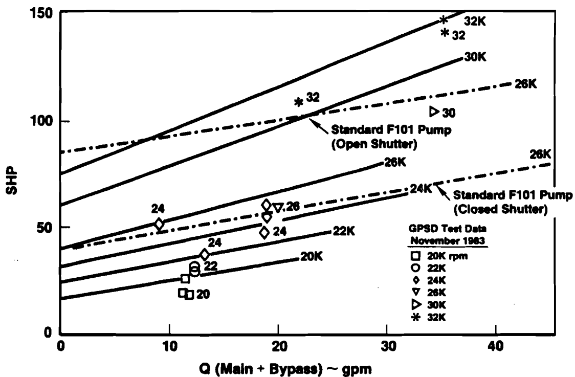
FIGURE 51. DEGRADER SHAFT HORSEPOWER
