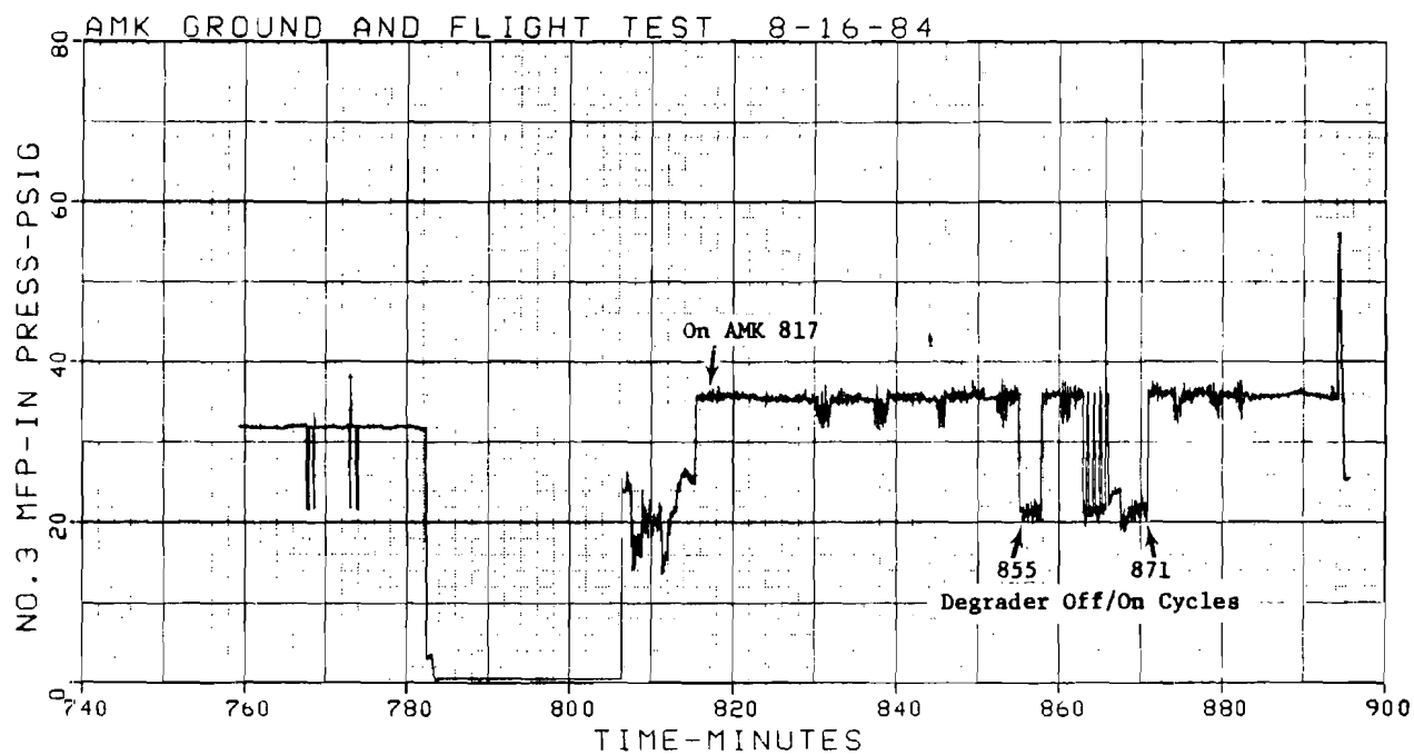
FIGURE 96. NUMBER 3 ENGINE MAIN FUEL FILTER INLET PRESSURE
