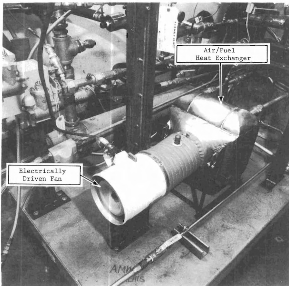
FIGURE 46. FUEL COOLING HEAT EXCHANGER AND FAN
