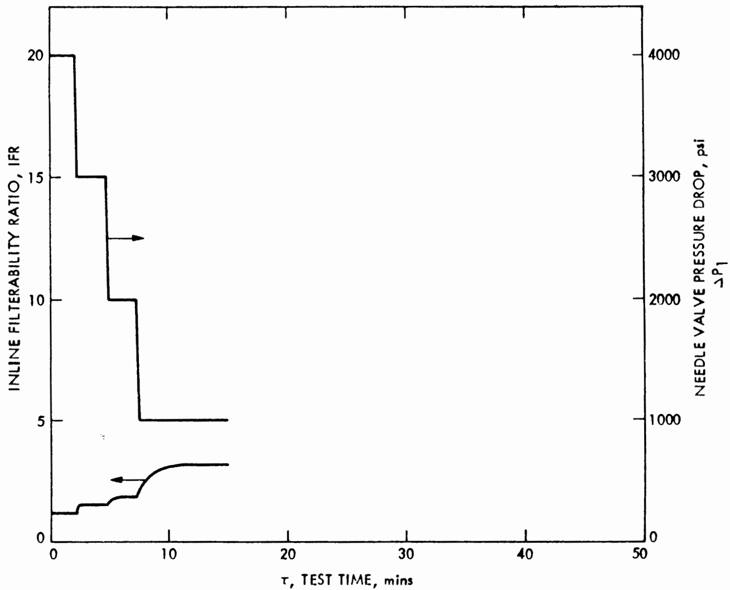
Figure 9 FILTRATION CHARACTERISTICS, TEST NO. 6 (SEE TABLE 5)
