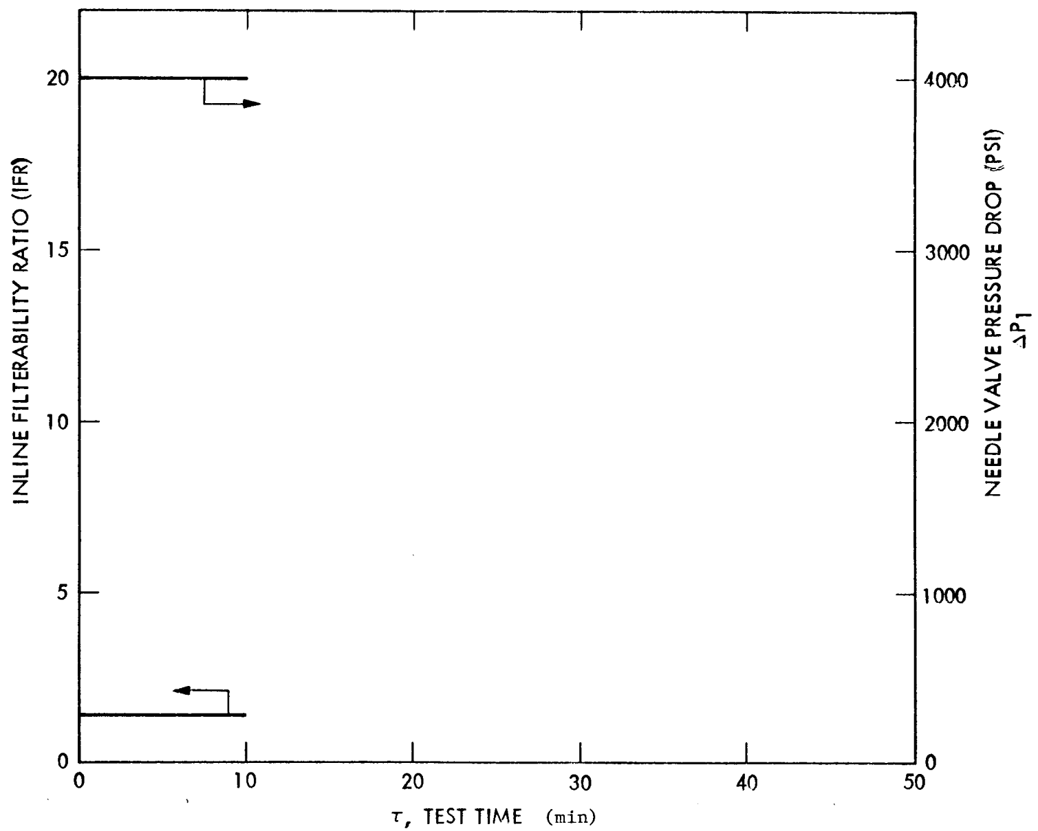
Figure 12 FILTRATION CHARACTERISTICS, TEST NO. 9 (SEE TABLE 5)
