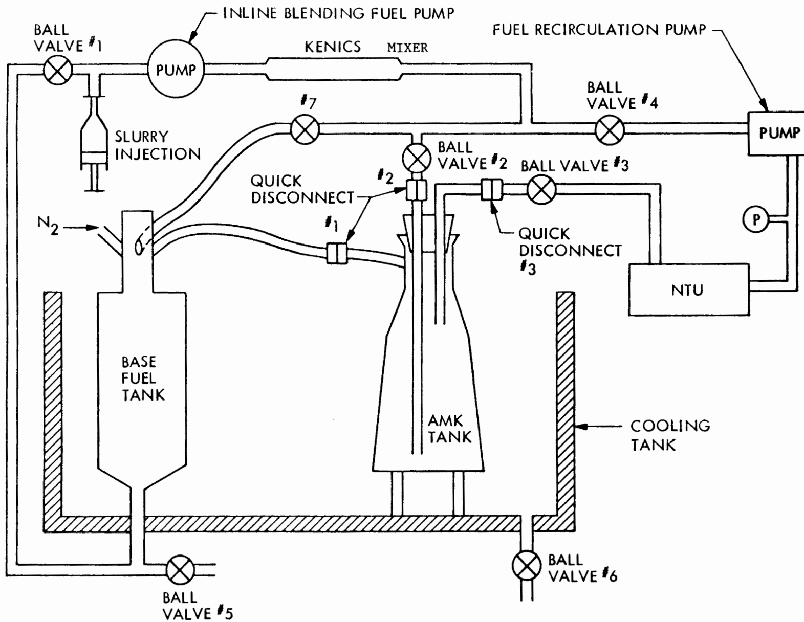
Figure 6 LOW TEMPERATURE INLINE BLENDING APPARATUS
