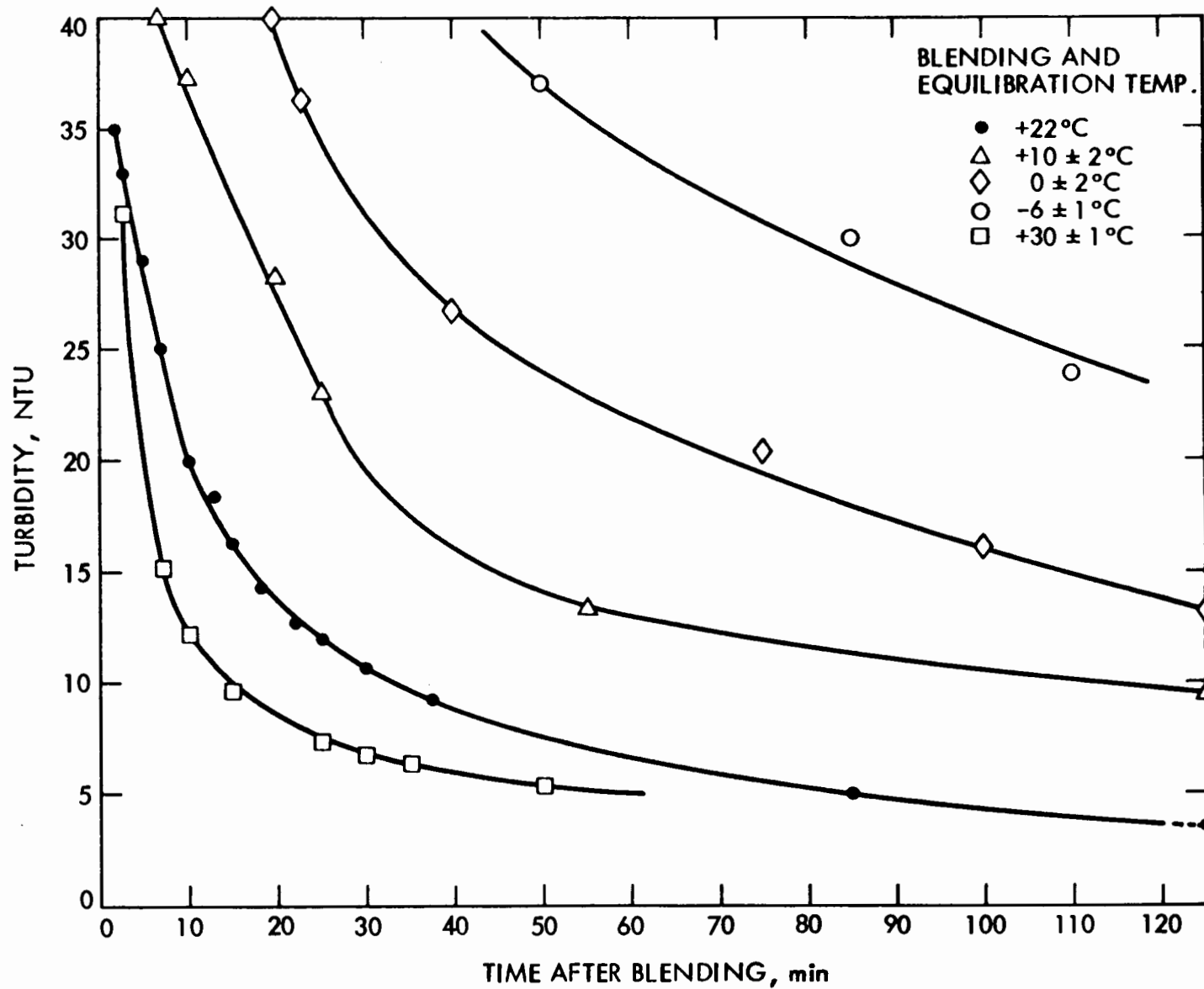
Figure 13 INFLUENCE OF BLENDING TEMPERATURE ON POLYMER DISSOLUTION RATE
