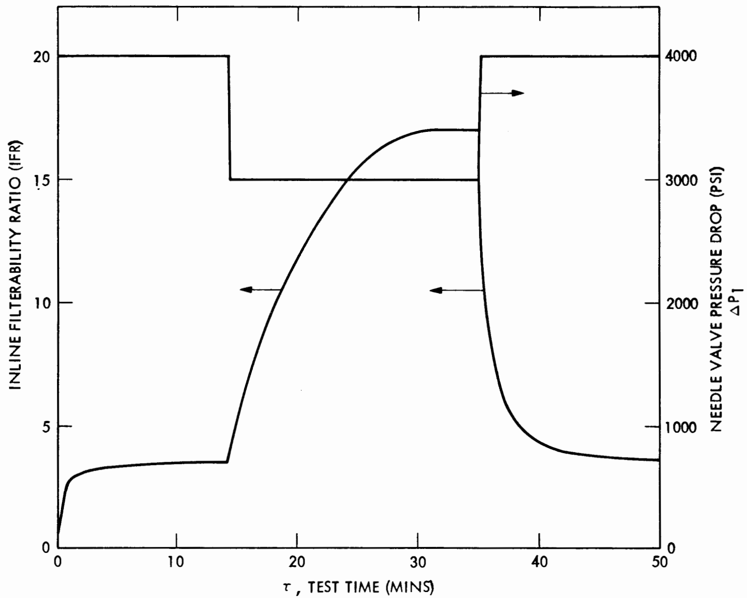
Figure 10 FILTRATION CHARACTERISTICS, TEST NO. 7 (see TABLE 5)
