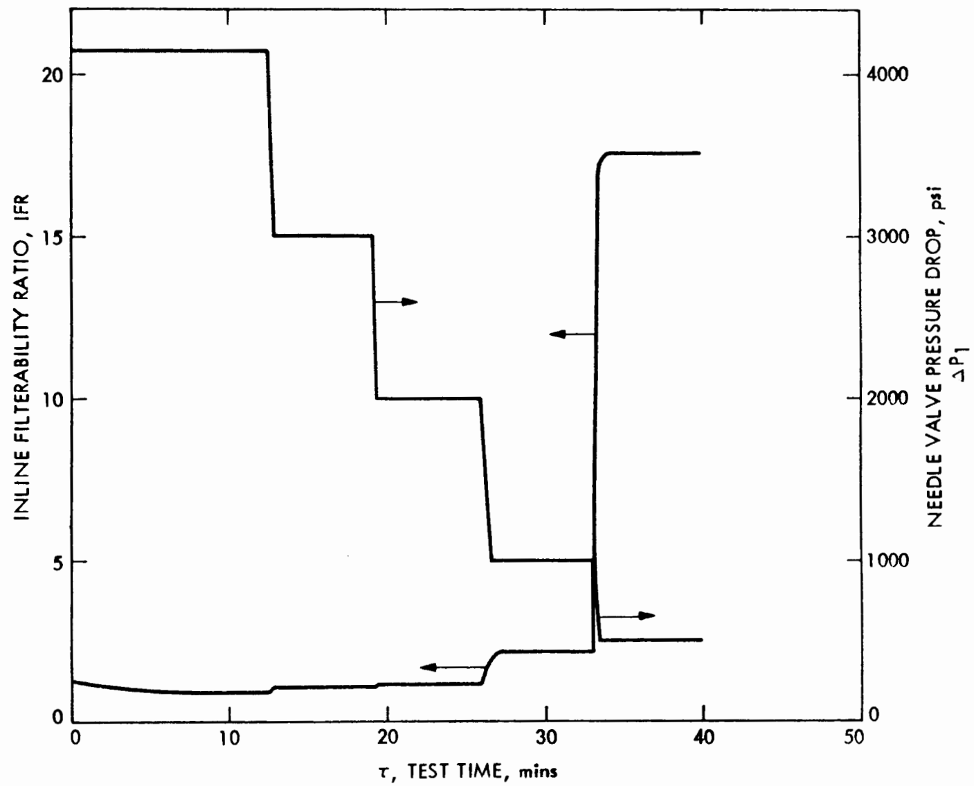
Figure 8 FILTRATION CHARACTERISTICS, TEST NO. 5 (SEE TABLE 5)
