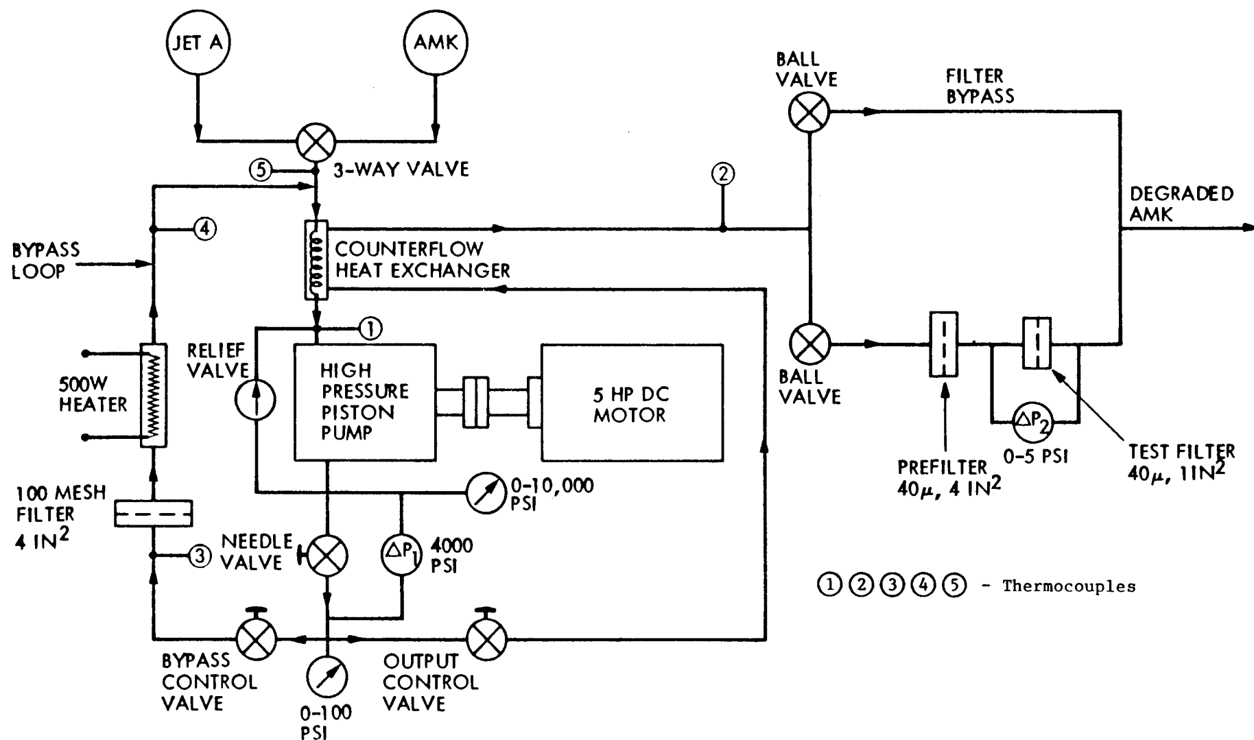
Figure 4 SCHEMATIC OF MARK II DEGRADER/FILTERABILITY APPARATUS
