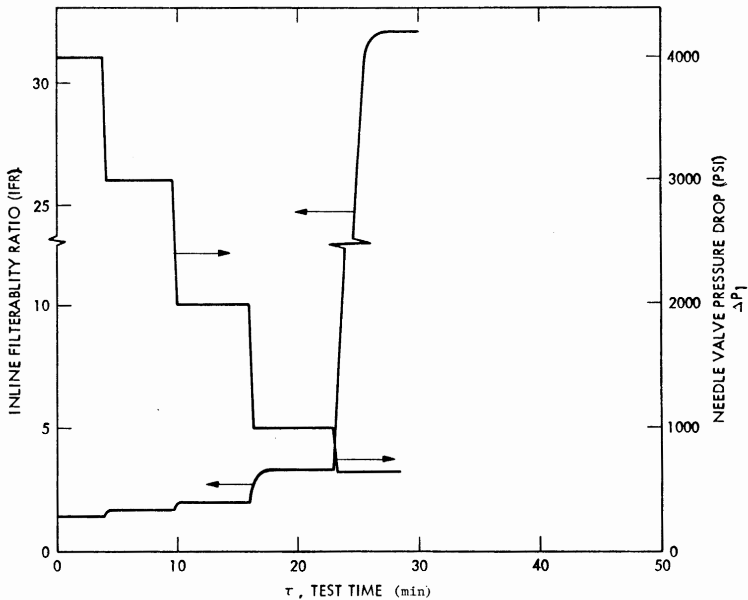
Figure 11 FILTRATION CHARACTERISTICS, TEST NO. 8 (SEE TABLE 5)
