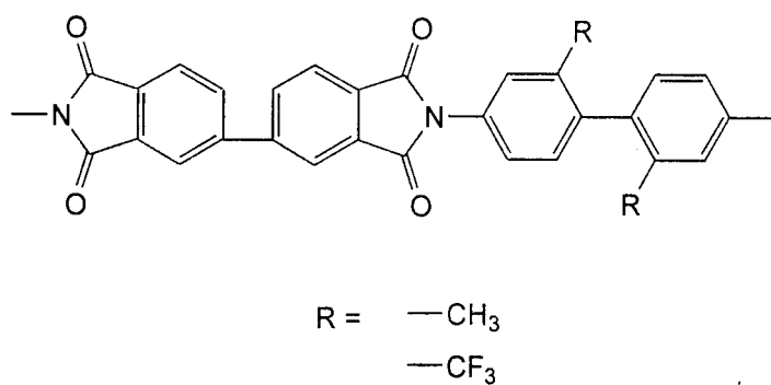
Figure 1.7 Gel-spinnable polyimides.
