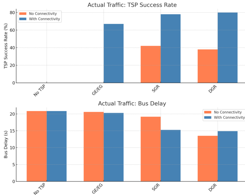
Figure 3: Comparison of TSP Success Rate and Bus Delay Under Actual Traffic Flow Conditions
