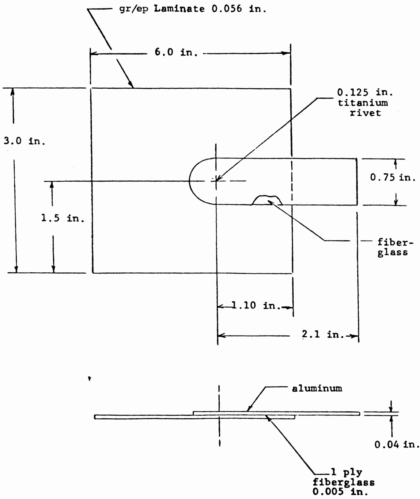
FIGURE 20. RIVET IN GR/EP LAMINATE TEST SPECIMEN
