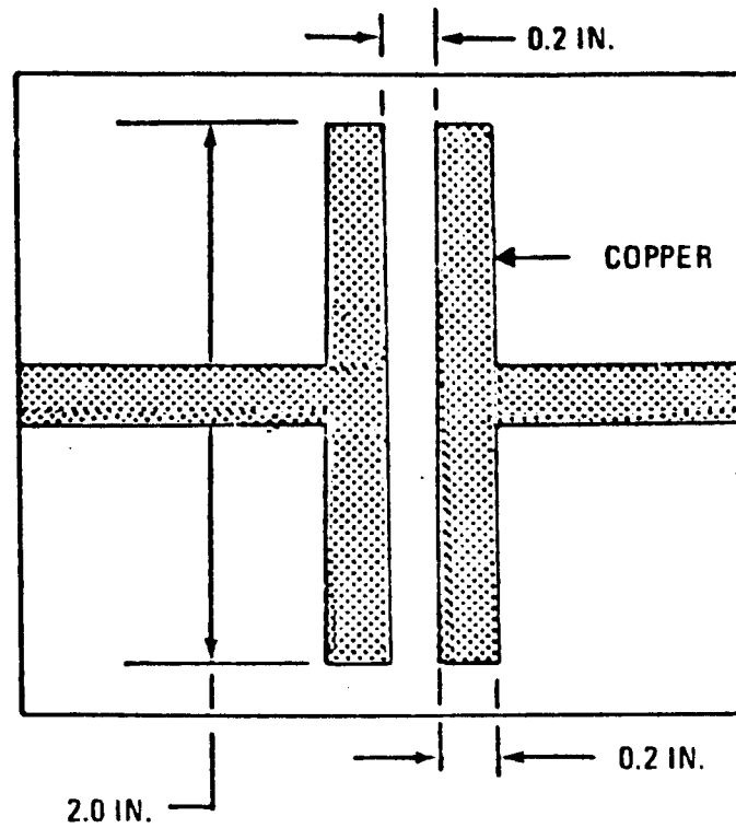
a. SURFACE PROBE DIMENSIONS
