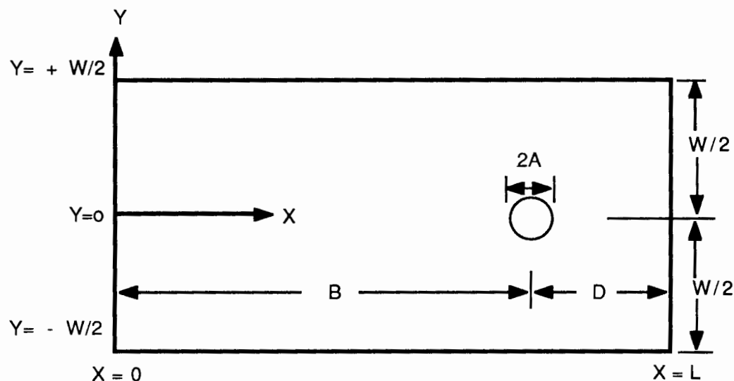
FIGURE B-1. GEOMETRY OF FASTENER IN PANEL
