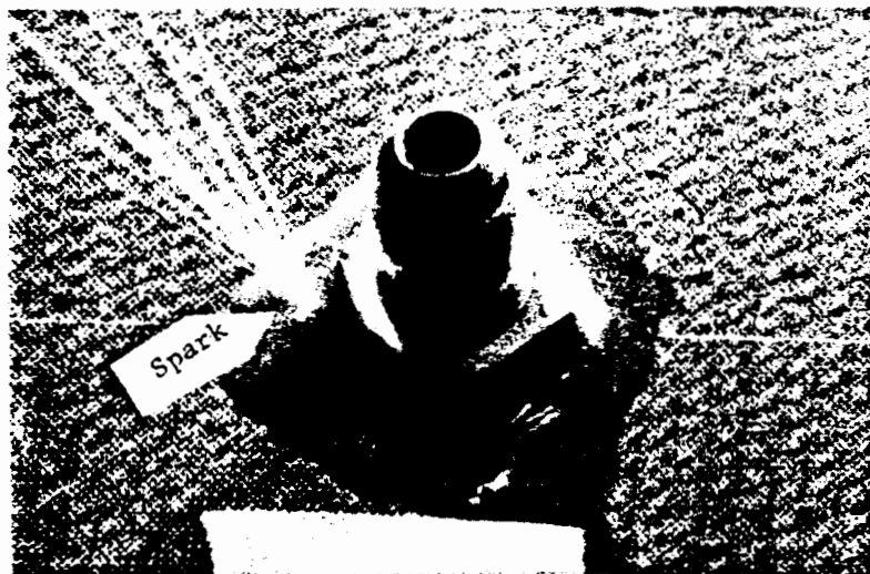
FIGURE 23. SPARK AT WASHER TO GR/EP INTERFACE RESULTING FROM A 15 kA CURRENT STRIKE TO THE FUEL FEED-THROUGH ELBOW. WET SIDE VIEW SHOWN.
