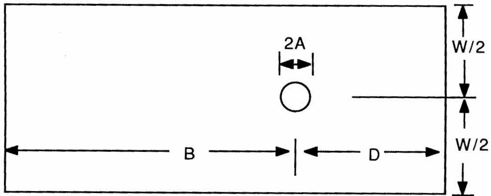
FIGURE 19. SAMPLE GEOMETRY WITH FASTENER
