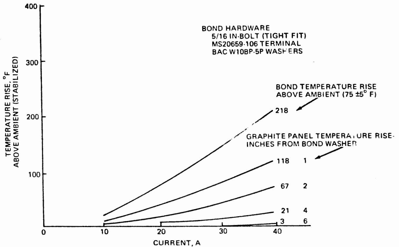
a. ELECTRICAL BOND GRAPHITE PANEL TEMPERATURE/CURRENT CURVES
