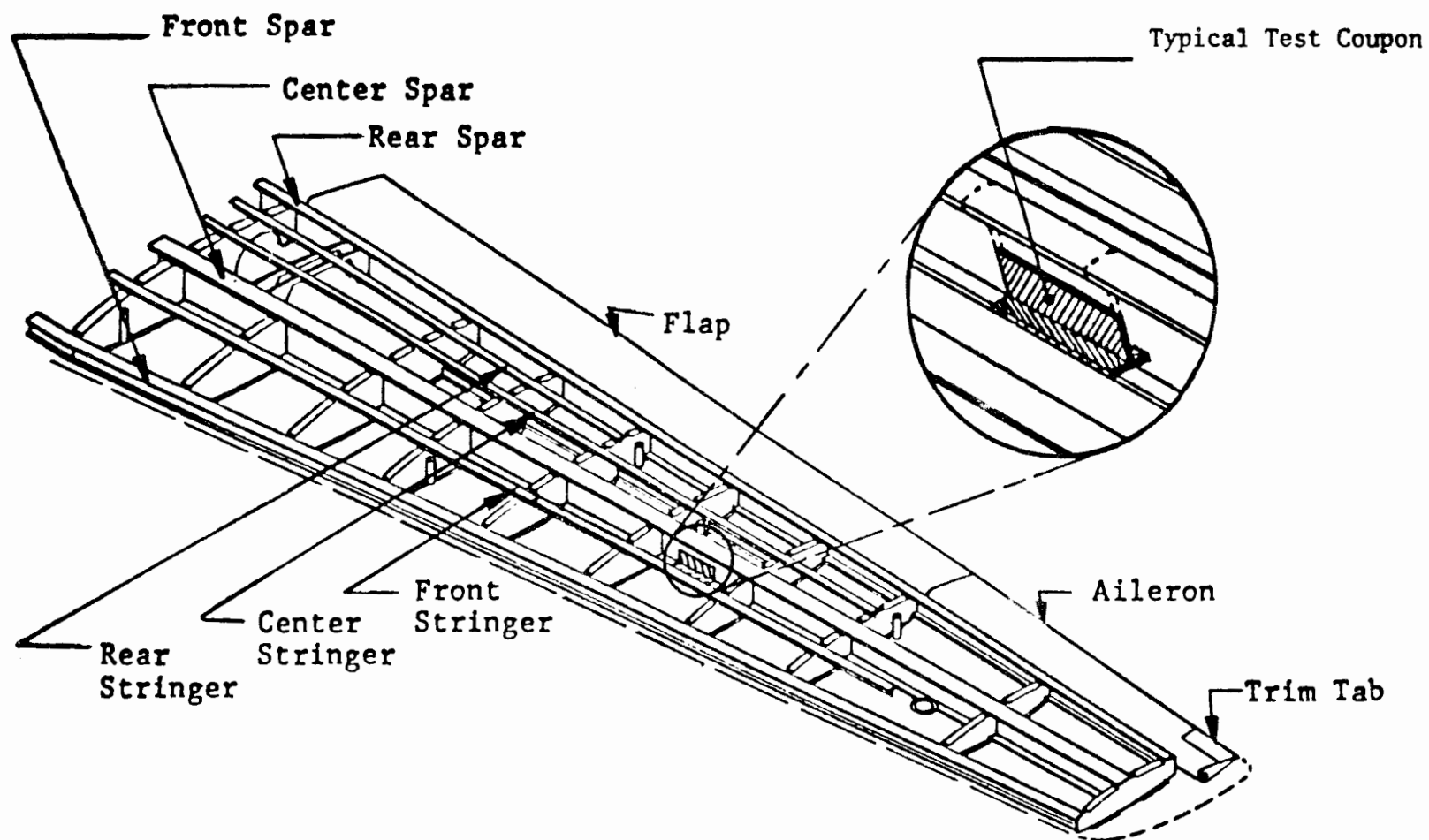
FIGURE 6. GR/EP WING INTERIOR VIEW
