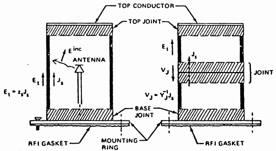
b. CYLINDRICAL SECTIONS
