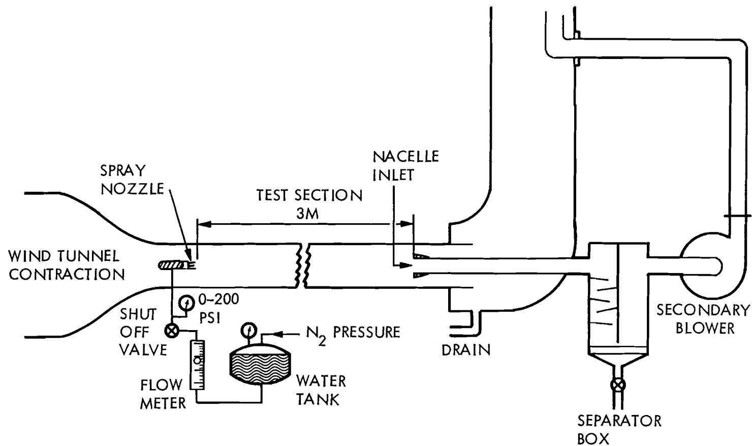
Figure 5. Schematic Diagram of Engine Water Ingestion Simulation Facility
