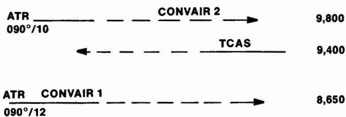
PROFILE 25: MULTIPLE AIRCRAFT
