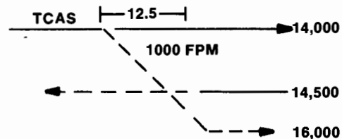
PROFILE 9: MANEUVERING INTERUDER, ALTITUDE CROSSING
