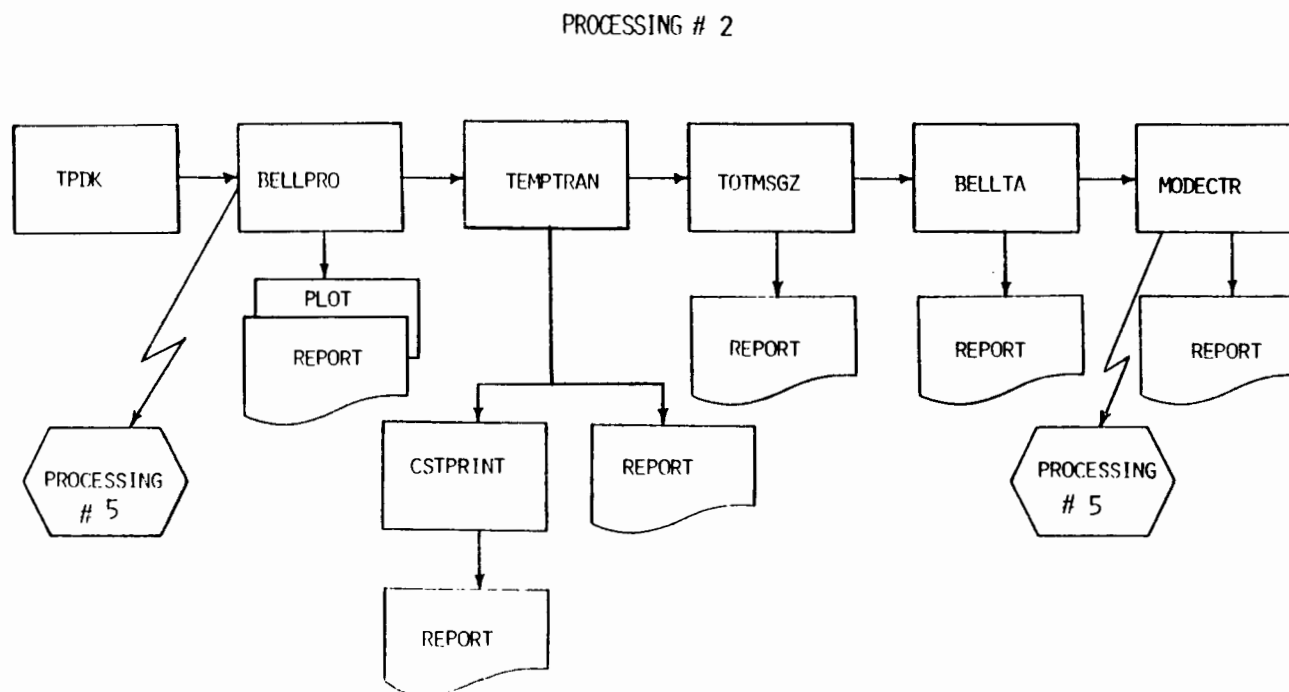
FIGURE 5. FLIGHT DATA REDUCTION FLOW CHART (SHEET 1 OF 2)
