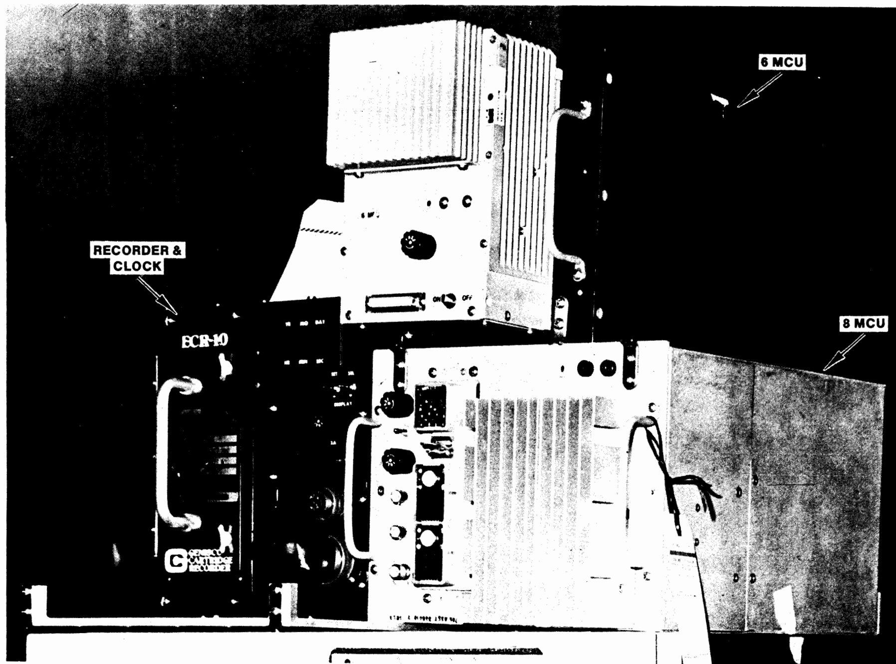
FIGURE 2. TCAS AVIONICS AND RECORDER/CLOCK
