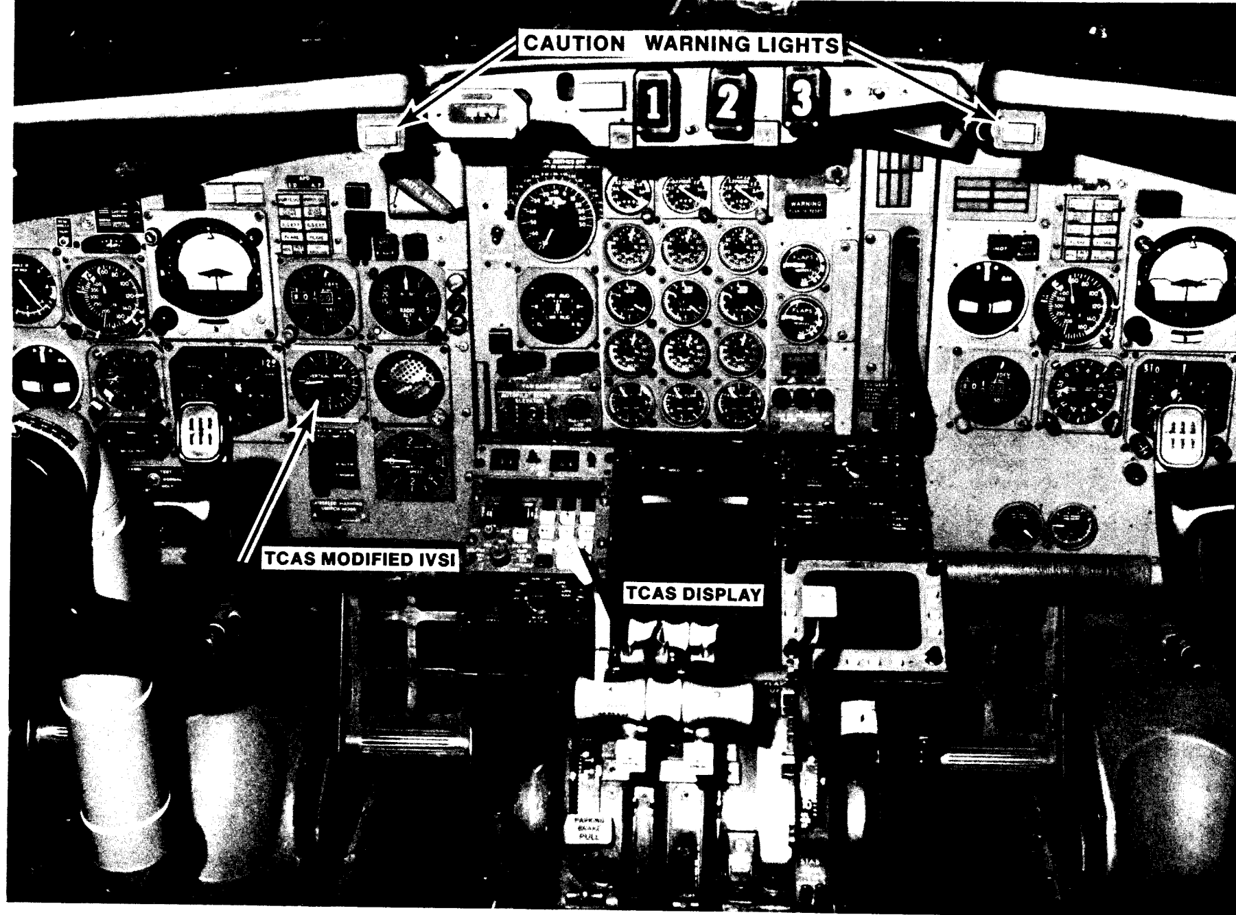
FIGURE 3. COCKPIT INSTALLATION - TCAS DISPLAYS
