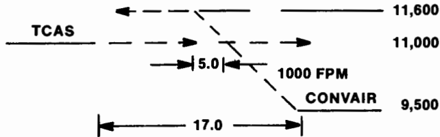
PROFILE 21: MANEUVERING INTRUDER; ALTITUDE CROSSING
