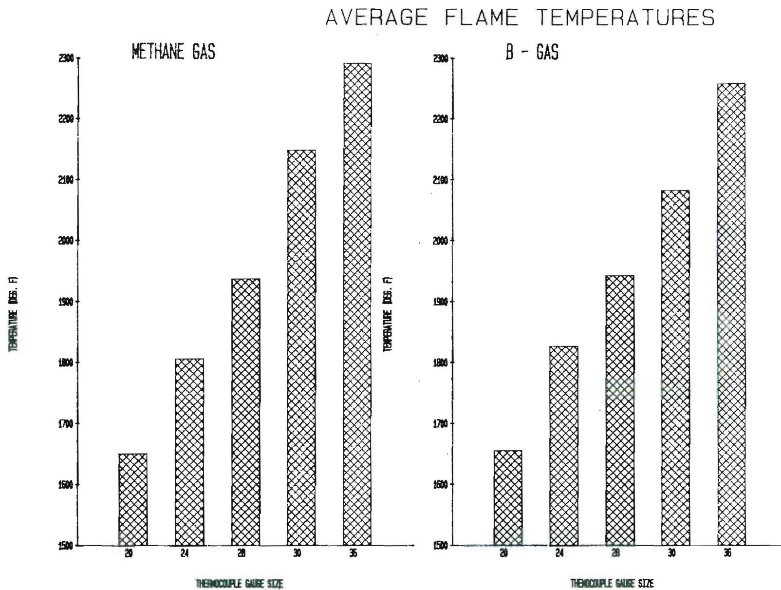
FIGURE 3. AVERAGE FLAME TEMPERATURES
