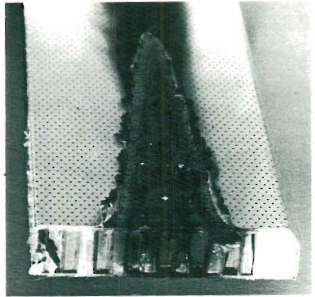
MIDPOINT-LOWER EDGE-FRONT FACE FLAME PLACEMENT
