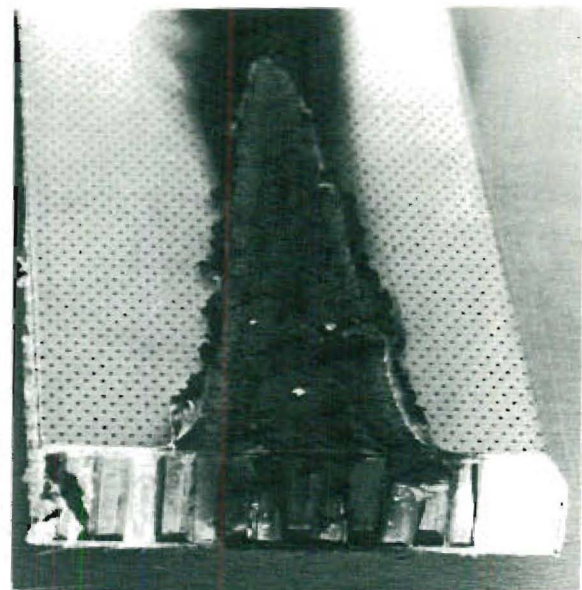
MIDPOINT-LOWER EDGE- FRONT FACE FLAME PLACEMENT
