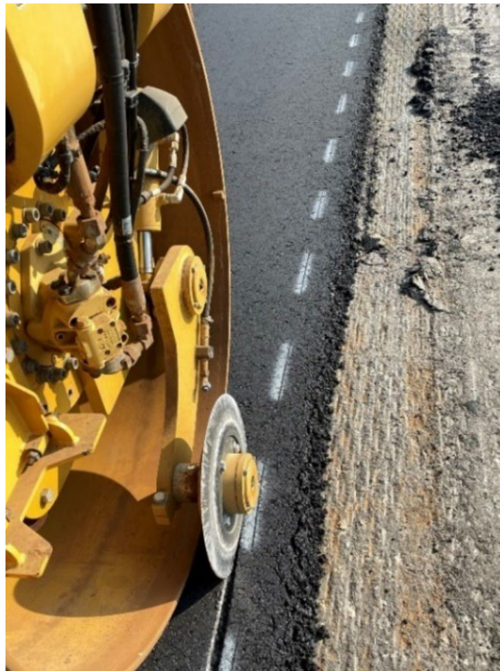
Figure 137. Cutting Wheel Mounted on a Roller
