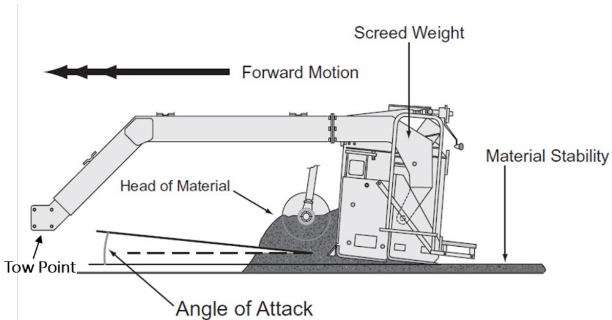
Figure 95. Elements That Impact Screed Forces
