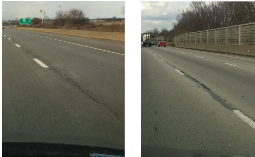
Figure 124. Premature Deterioration of Longitudinal Joints
