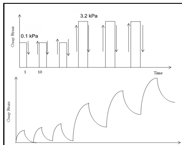
Figure 4. MSCR Stress and Strain Responses
