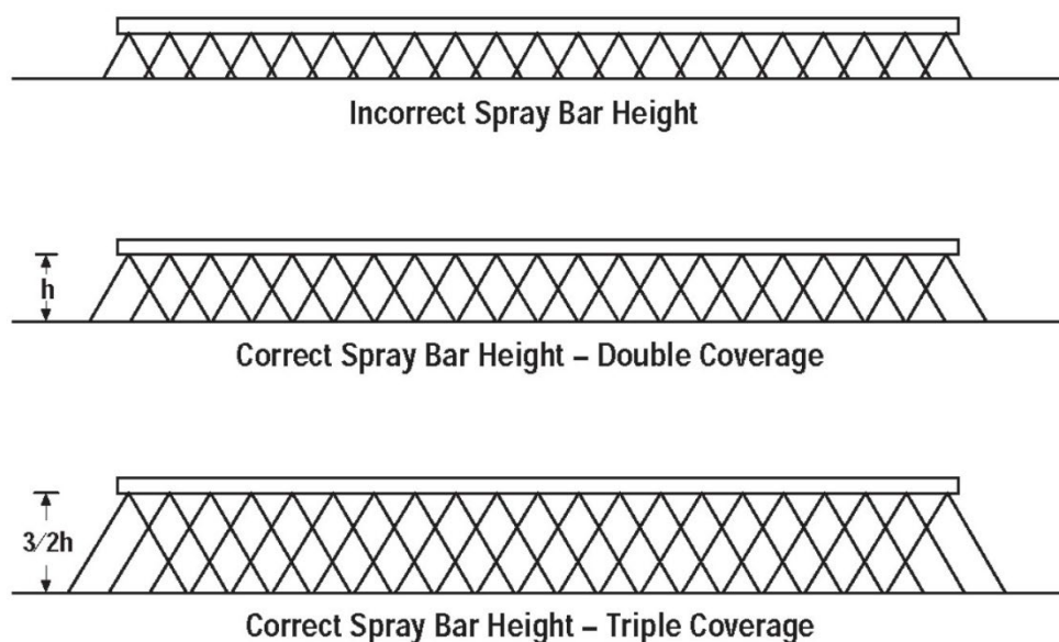
Figure 72. Spray Fan Overlap
