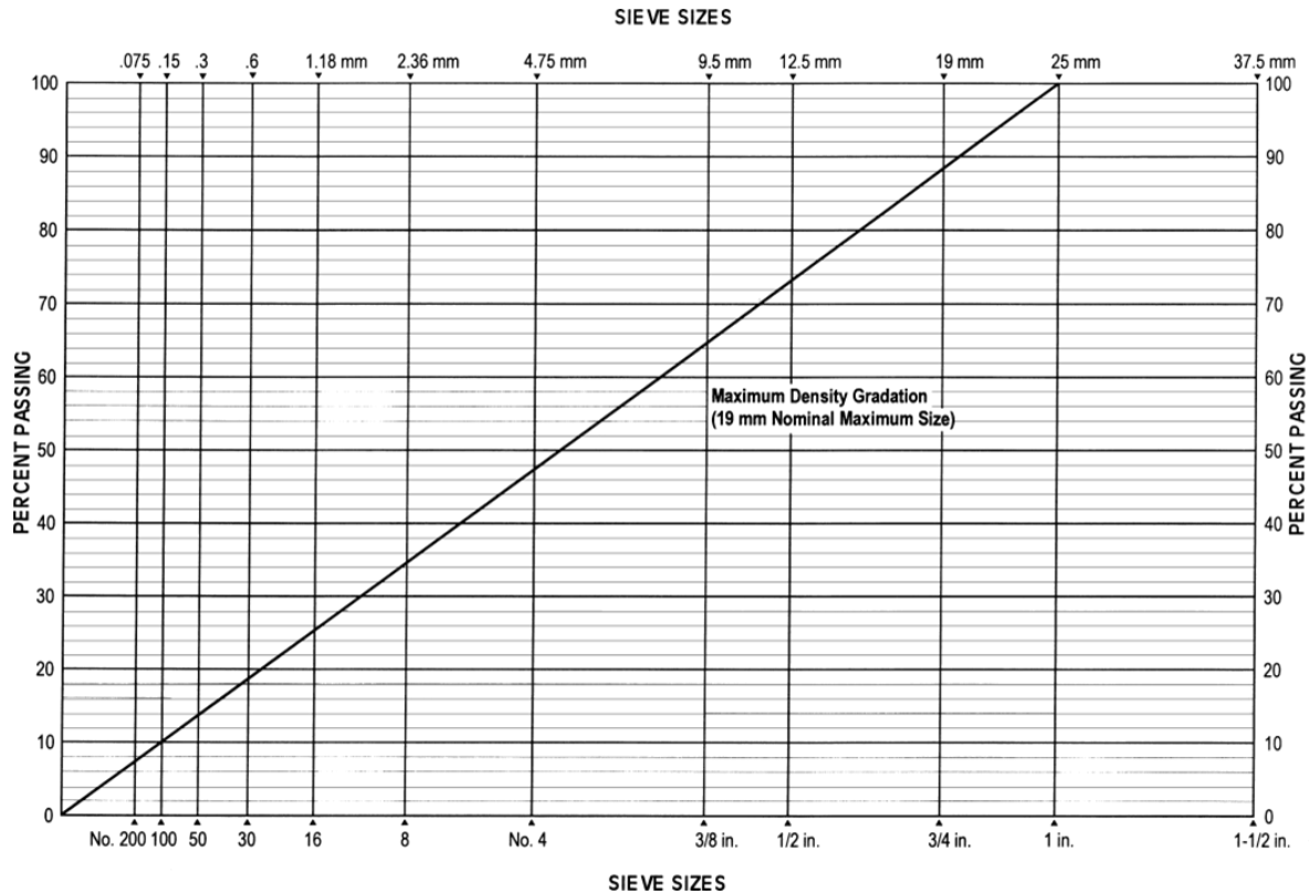
Figure 8. Gradation Chart, Exponential Scale (0.45)
