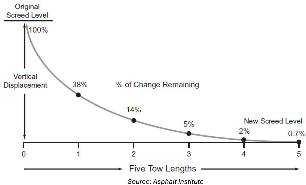
Figure 97. Distance Required for the Screed to Reach Equilibrium
