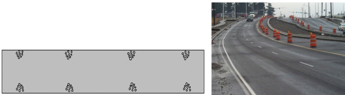
Figure 151. Examples of Truck-End Segregation
