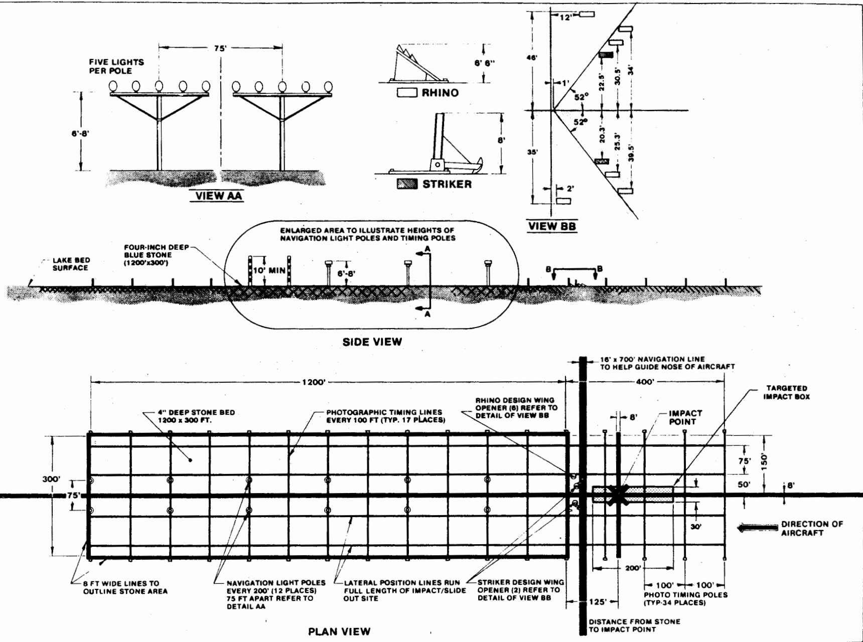
FIGURE 8. CID IMPACT SITE SCHEMATIC
