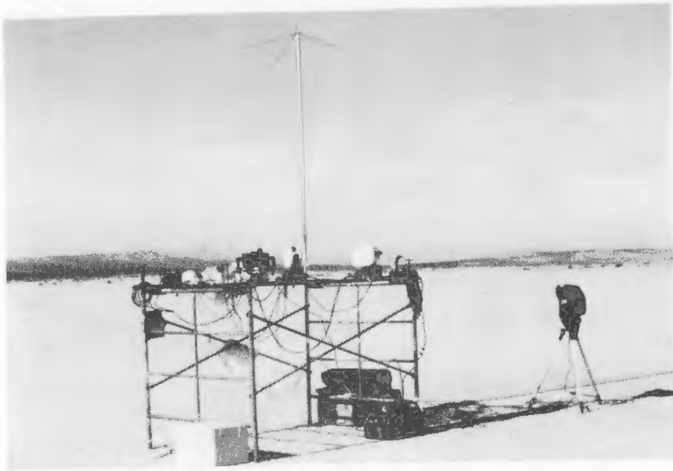
FIGURE 13. REMOTE CAMERA STATION #5 INCLUDING PAO CAMERAS
