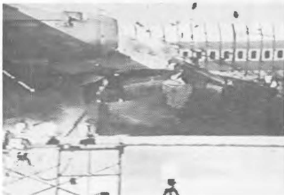
FIGURE 20. CID ENGINE #3 IGNITION AS PHOTOGRAPHED BY REMOTE TRACKER
