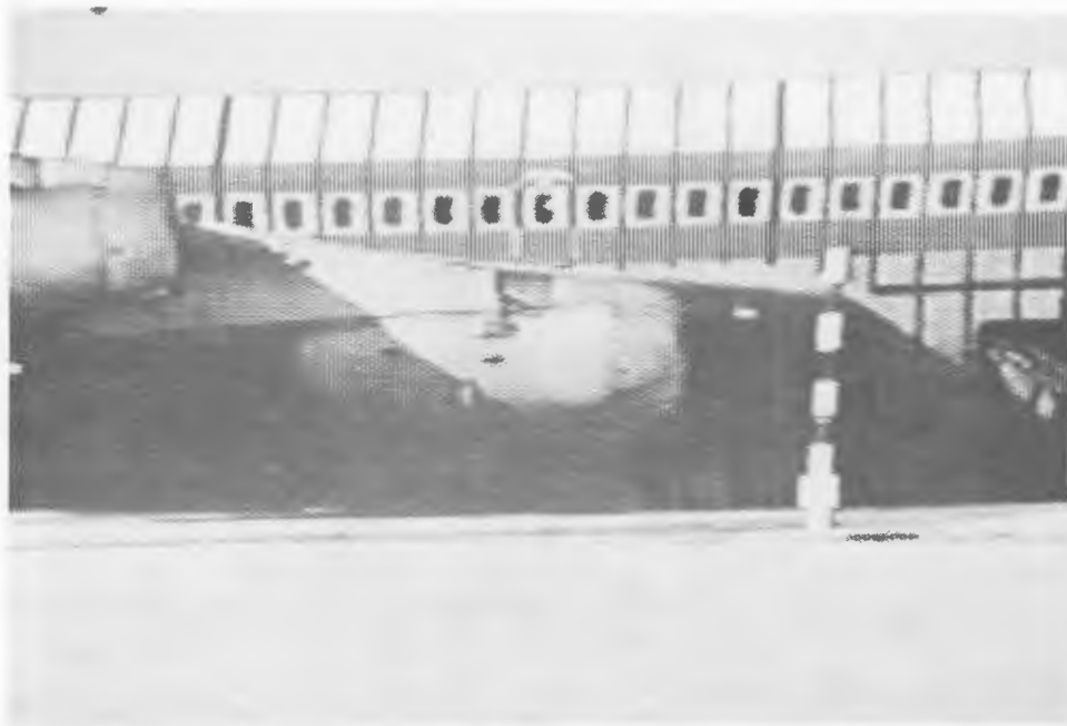
FIGURE 21. VIEW FROM REMOTE TRACKER SHOWING ENGINE #3 AND CALIBRATION POST
