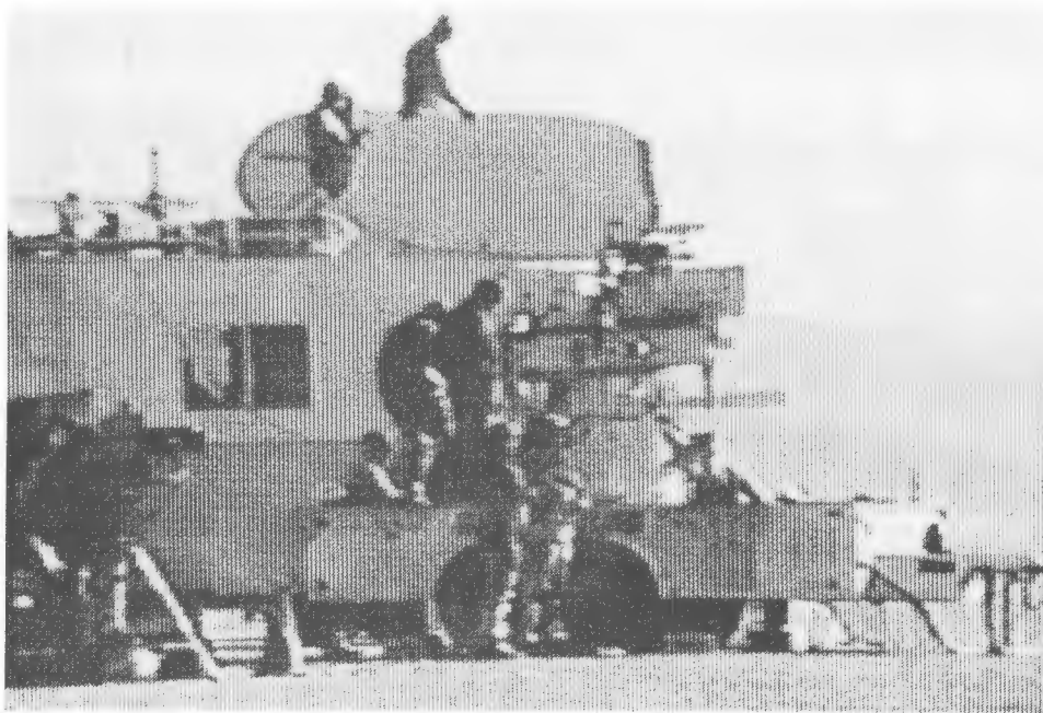
FIGURE 23. SITE 17/22 MANNED CINE-SEXTANT TRACKING CREW
