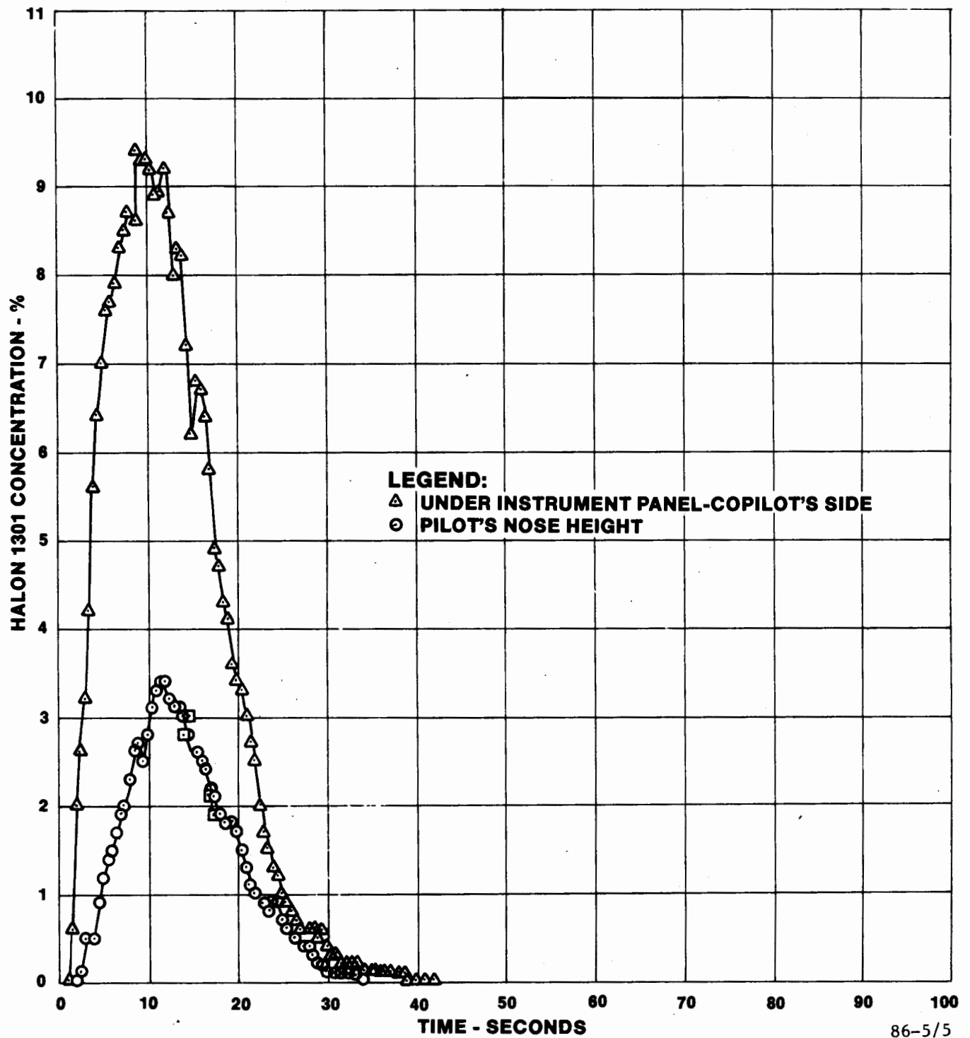
FIGURE 5. HALON 1301 CONCENTRATIONS - 3-POUND EXTINGUISHER DIRECTED UNDER INSTRUMENT PANEL - COPILOT'S SIDE - OVERHEAD VENTS OPEN
