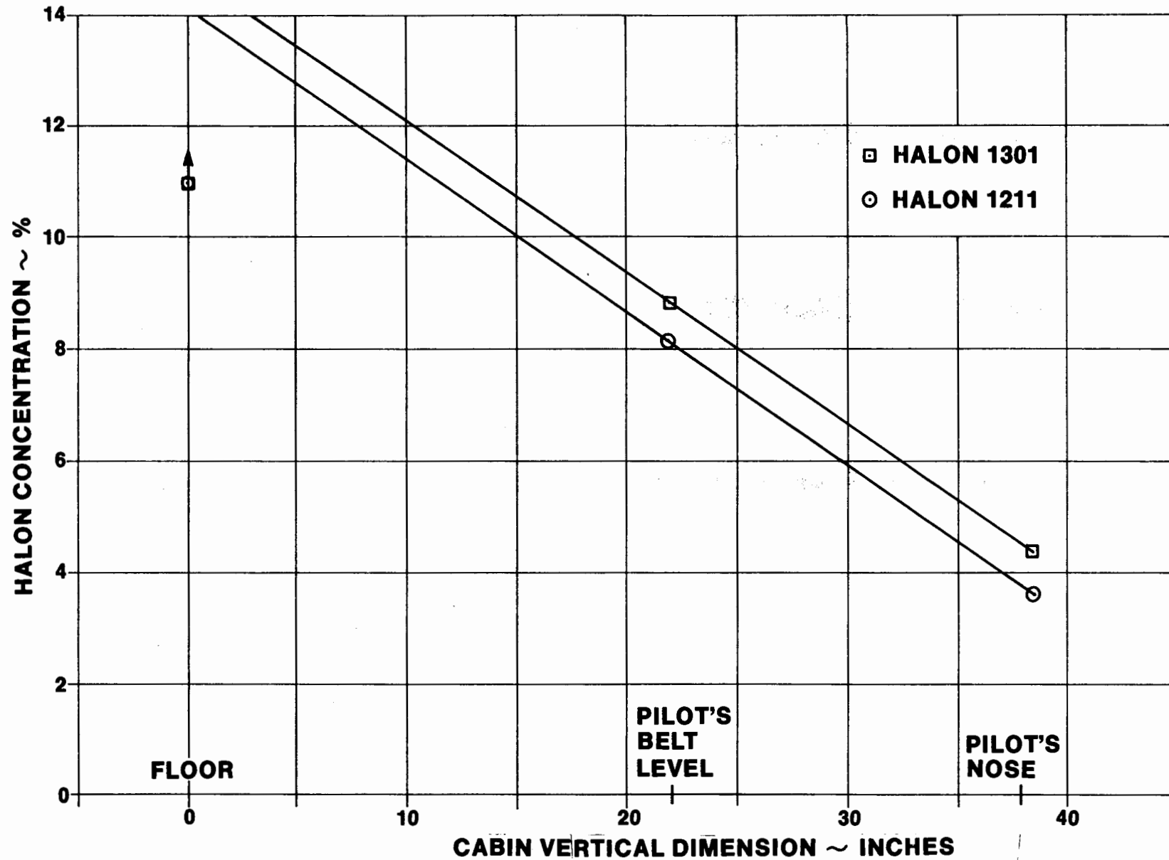
FIGURE 35. STRATIFICATION OF HALON EXTINGUISHING AGENTS
