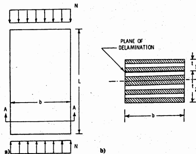
FIGURE 13. GEOMETRY AND LOADING OF RECTANGULAR PLATE DELAMINATION. EXAMPLE: a) GEOMETRY AND LOADING; b) VIEW A-A SHOWING LAMINATE CROSS-SECTION
