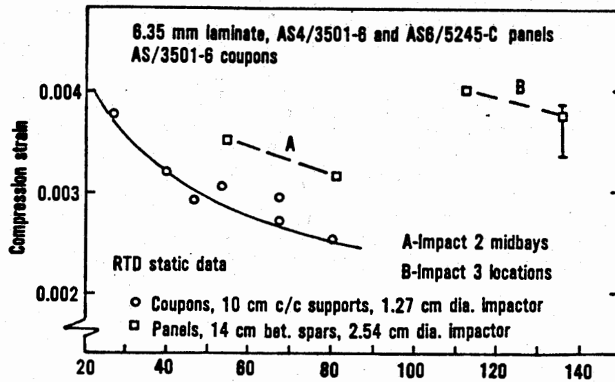
FIGURE 10. THREE-SPAR PANELS - SPECIMEN COMPLEXITY EFFECT
