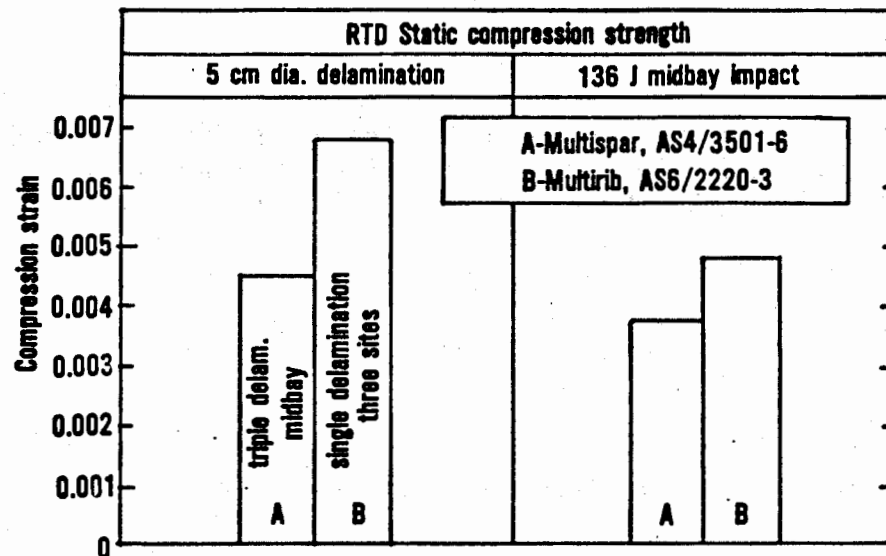
FIGURE 11. PANEL DESIGN COMPARISON - STATIC STRENGTH
