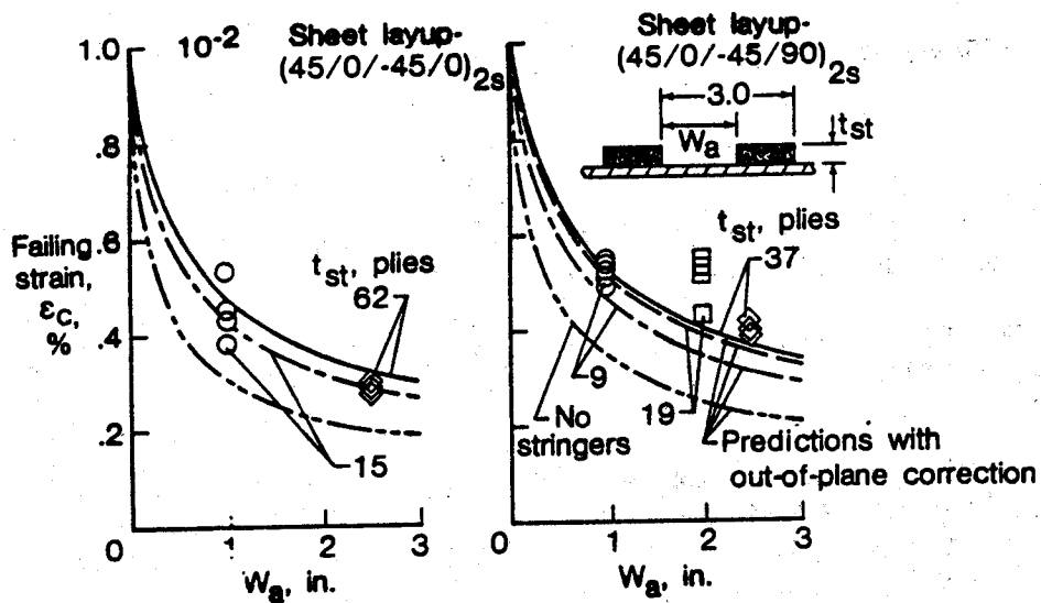
FIGURE 23. FAILING STRAIN VERSUS STRINGER SPACING
