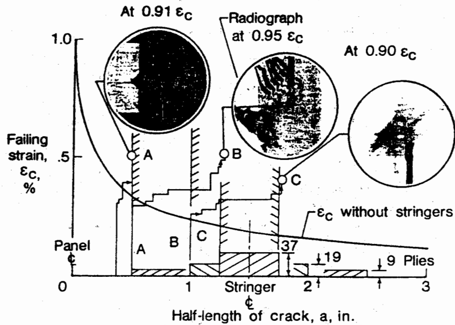
FIGURE 18. FAILING STRAIN VERSUS CRACK-TIP POSITION
