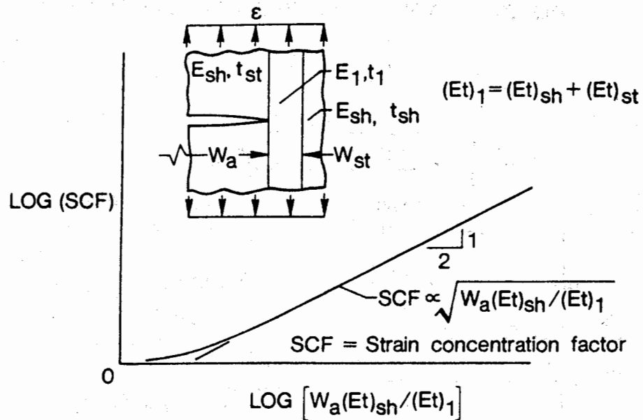
FIGURE 19. RESULTS FROM SHEAR LAG ANALYSIS
