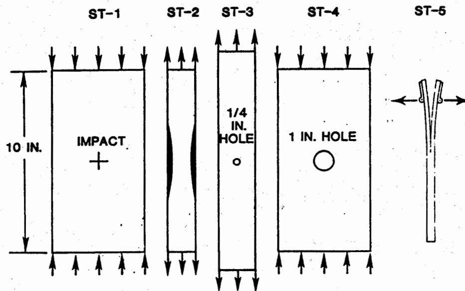
FIGURE 12. STANDARD TESTS FOR TOUGHENED COMPOSITES
