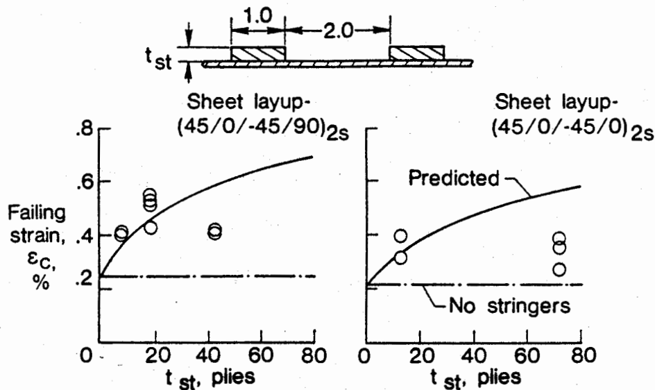
FIGURE 21. FAILING STRAIN VERSUS STRINGER THICKNESS
