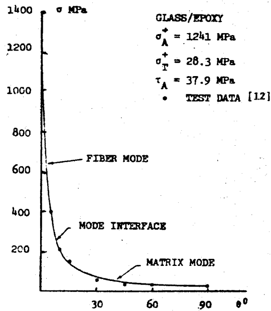
FIGURE 3. STATIC OFF-AXIS SPECIMEN DATA THEORY AND EXPERIMENT
