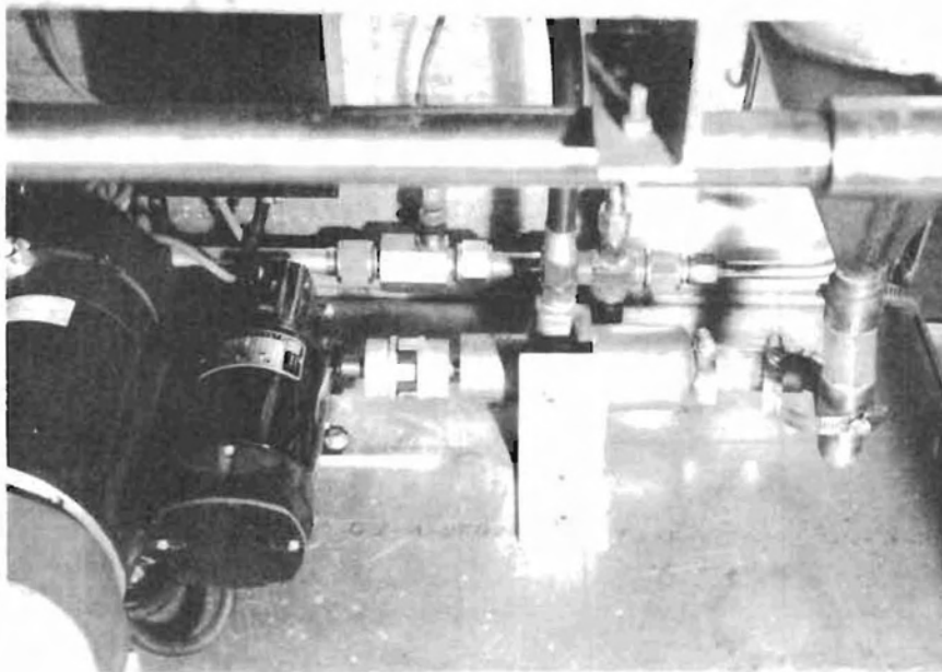
Figure 2 Photograph of slurry pump and speed controlled DC motor drive.
