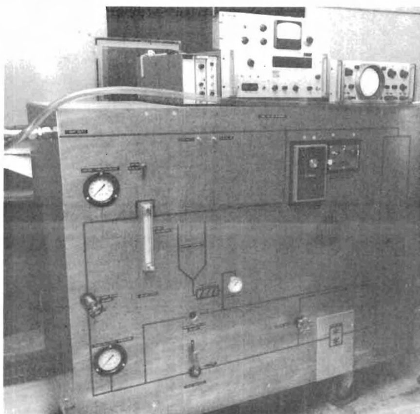
Figure 6 Photograph of JPL Inline Blender No. 1
