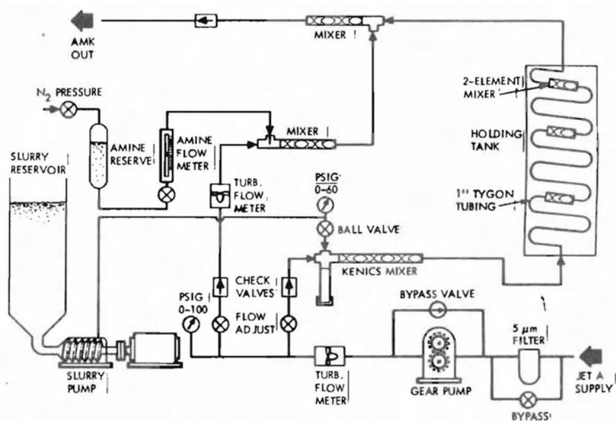
Figure 5 Schematic of the Inline Blender System
