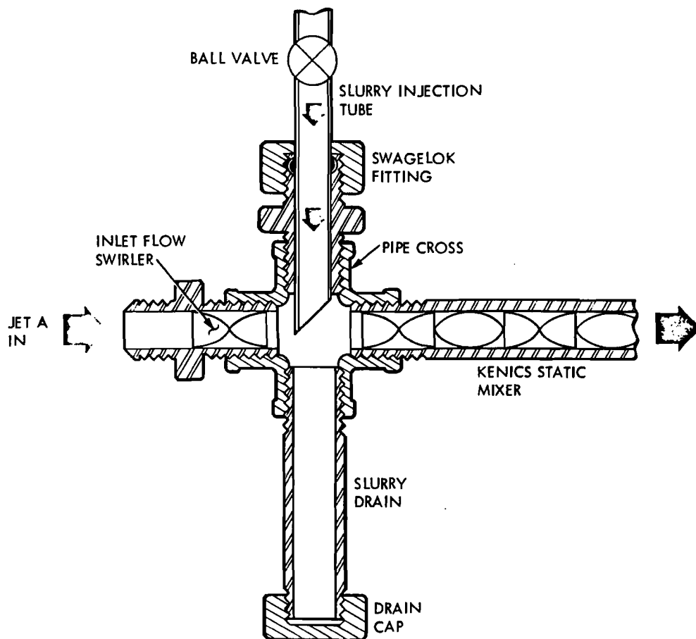
Figure 4 Details of slurry injection and dispersion scheme
