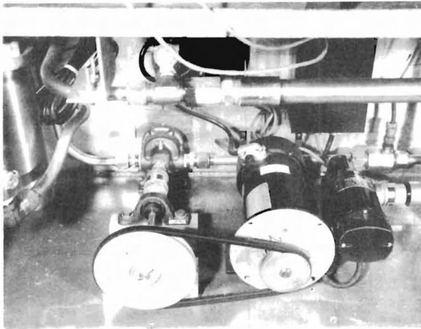
Figure 1 Photograph of gear pump and speed controlled DC motor drive
