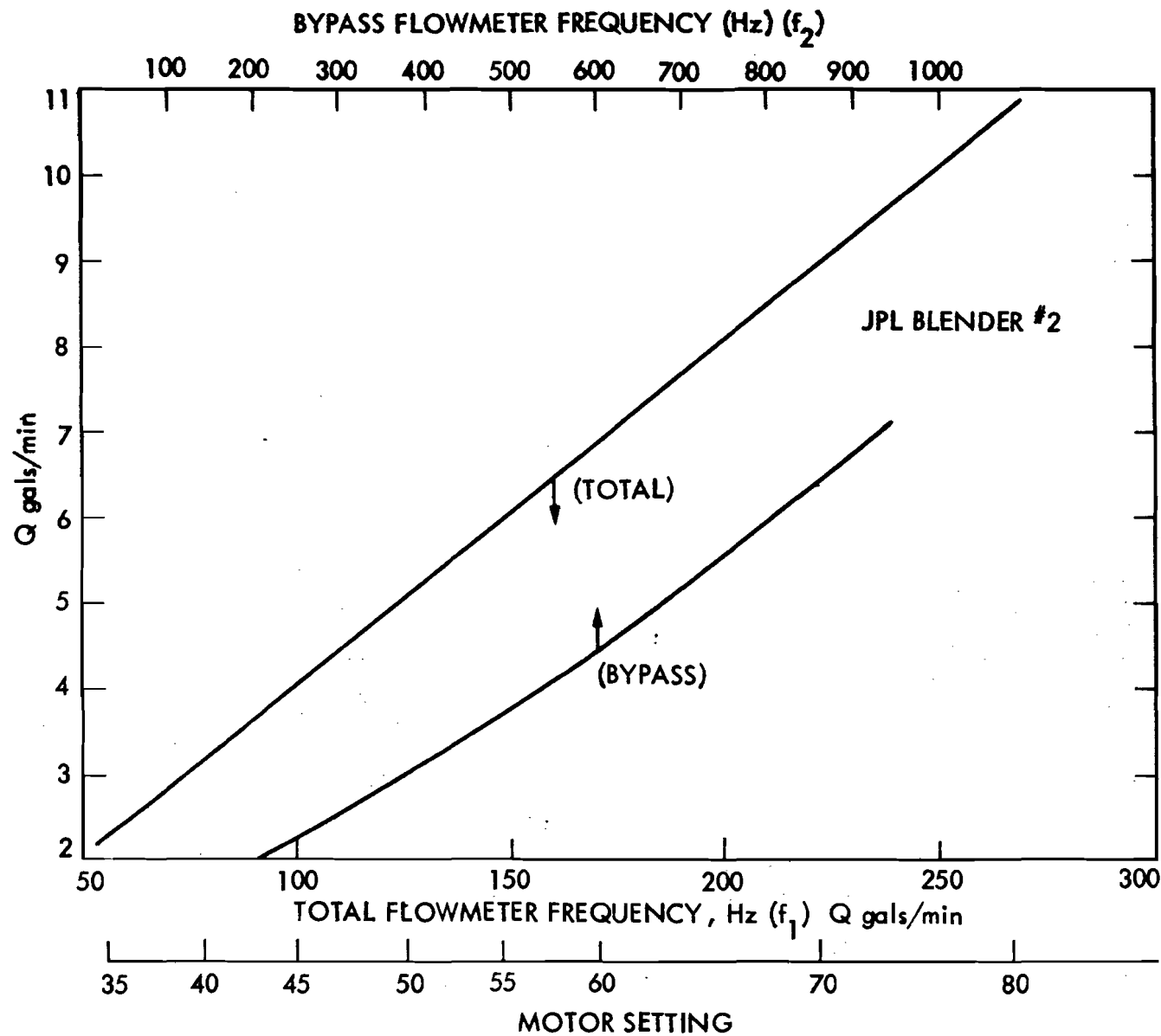
Figure 8 Turbine flow meter calibrations for JPL continuous Inline Blender No.2
