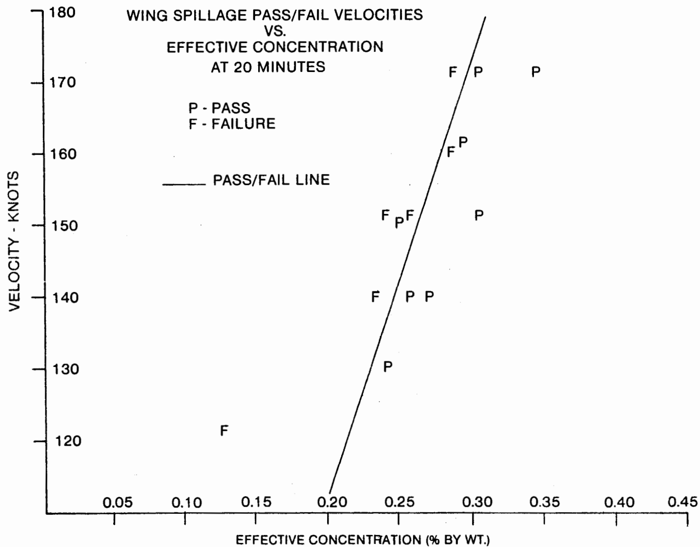
FIGURE 8. WING SPILLAGE TEST RESULTS VERSUS EFFECTIVE CONCENTRATION PASS/FAIL BOUNDARY INDICATED
