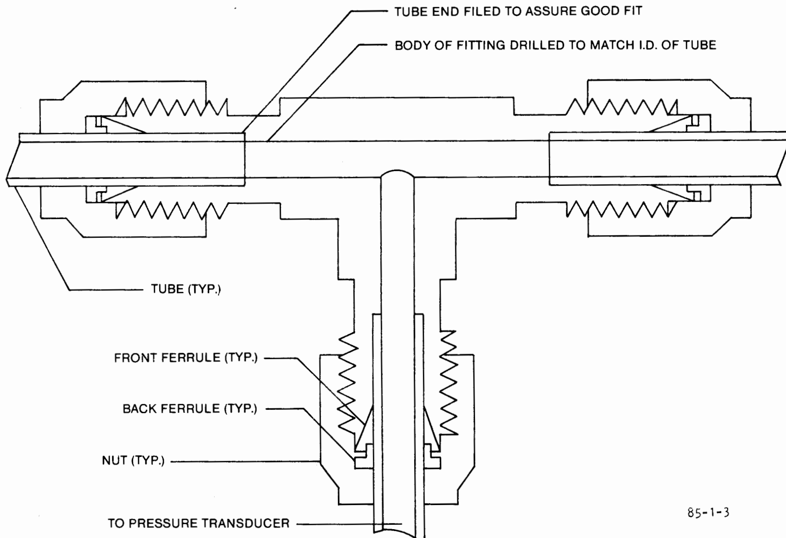
FIGURE 3. CROSS SECTION OF T-TUBE FITTING USED IN DIE SWELL AND CAPILLARY TUBE EXPERIMENTS
