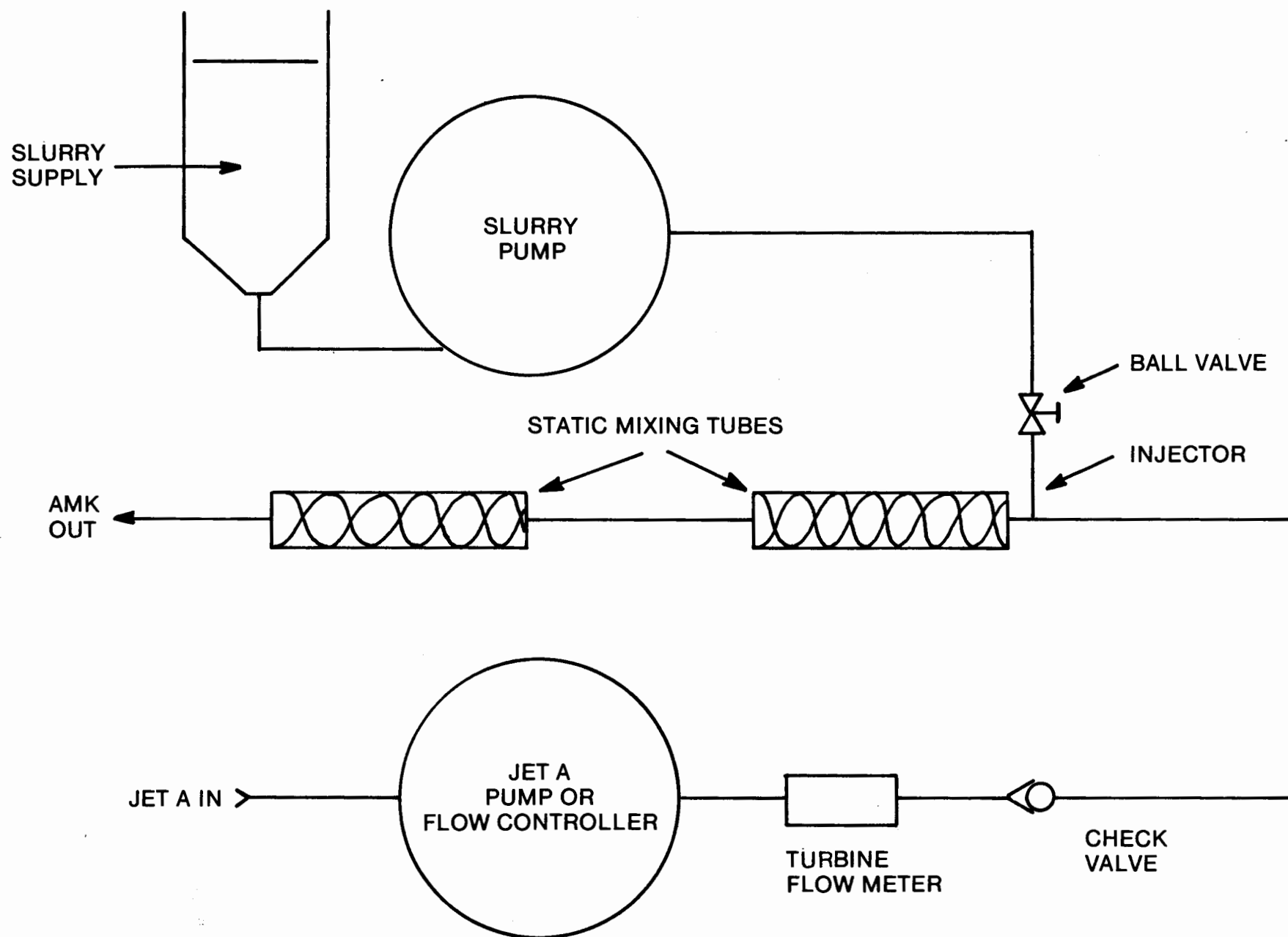
FIGURE C-1. SCHEMATIC OF LARGE SCALE BLENDER
