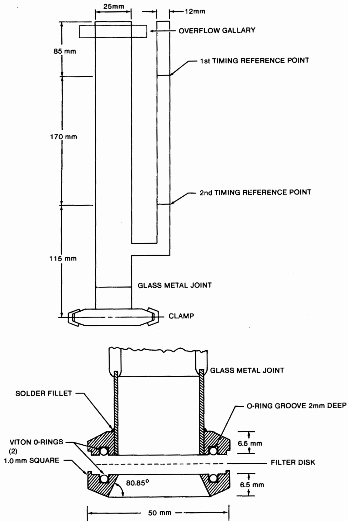
FIGURE F-1. DESCRIPTION OF FILTER RATIO APPARATUS
