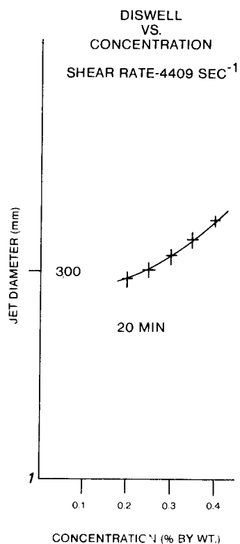
FIGURE 6. THE DIE SWELL VERSUS CONCENTRATION CURVE FOR 20-MINUTE OLD FUEL
