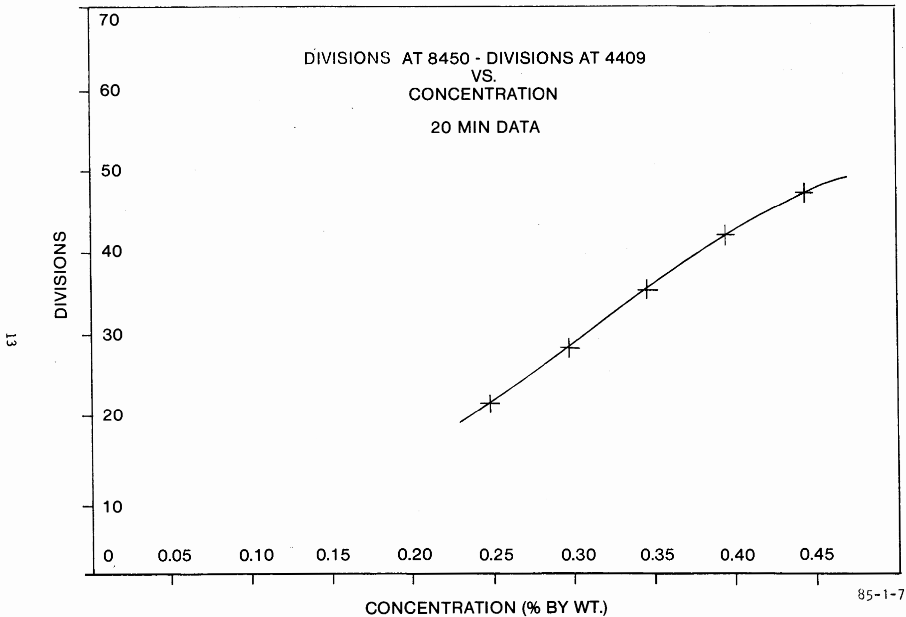
FIGURE 7. THE DELTA DIVISIONS VERSUS CONCENTRATION CURVE FOR 20-MINUTE OLD FUEL
