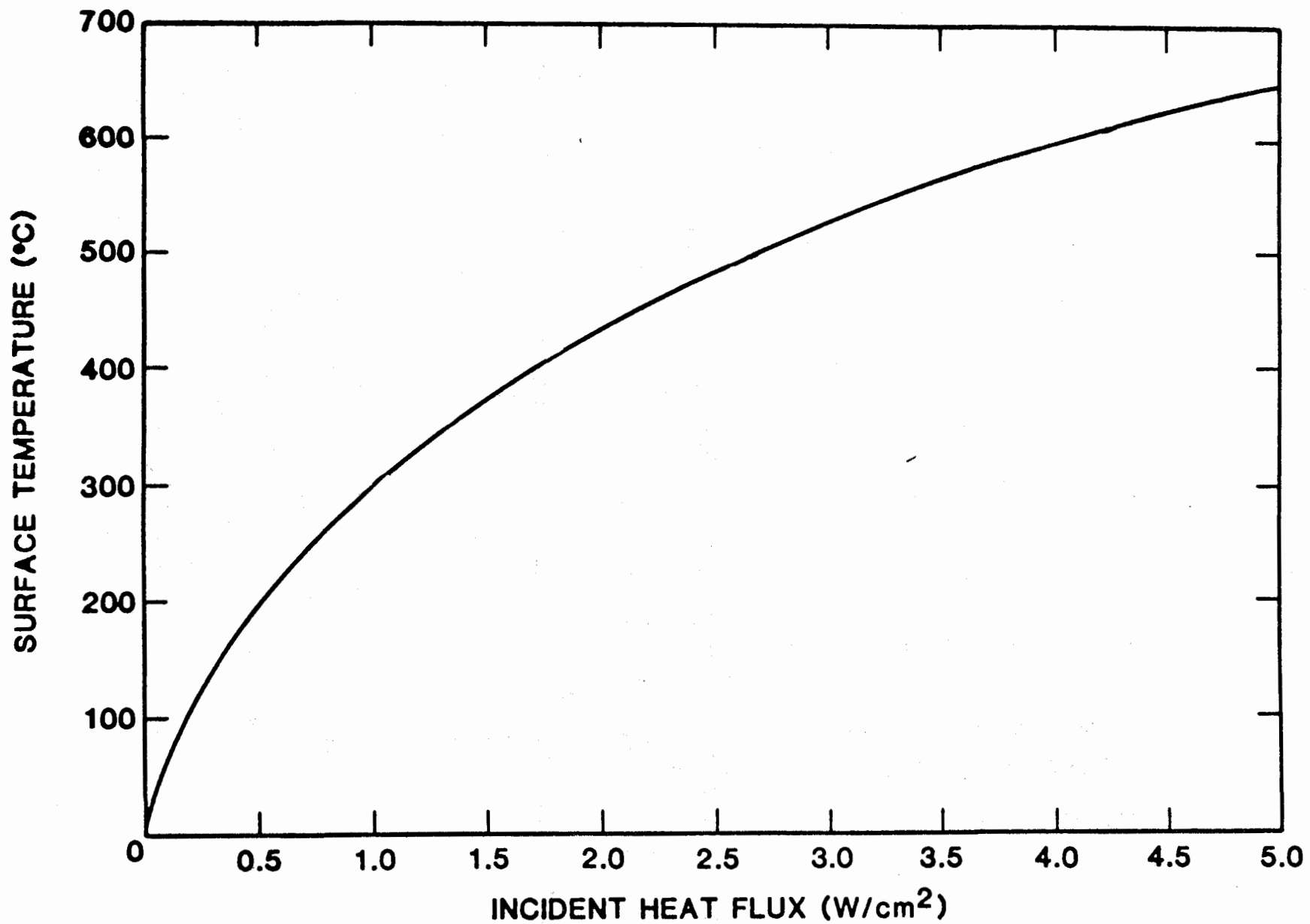
FIGURE 3.8. EQUILIBRIUM SURFACE TEMPERATURE AS A FUNCTION OF EXTERNAL RADIANT HEATING IN A TEST APPARATUS.
