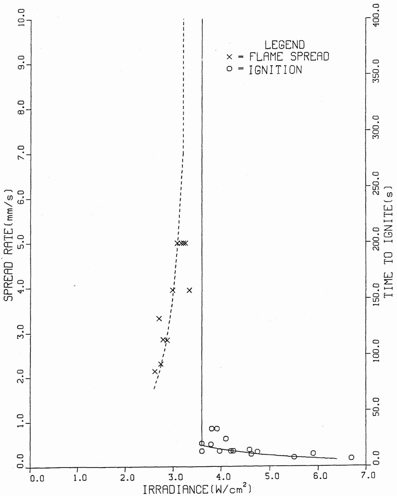
FIGURE 3.4. SPREAD AND IGNITION RESULTS FOR AIRCRAFT PANEL #2, PHENOLIC FIBERGLASS.
