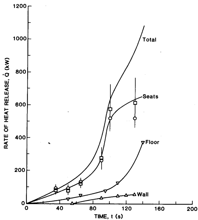
FIGURE 1.8. ESTIMATES OF HEAT RELEASE RATES DURING TEST 35 (REGULAR SEATS). SYMBOLS: ○, ▽, ▲ - BASED ON AREA-OF-INVOLVEMENT AND CALORIMETER HEAT RELEASE DATA; □ - BASED ON FLAME HEIGHT DATA.
