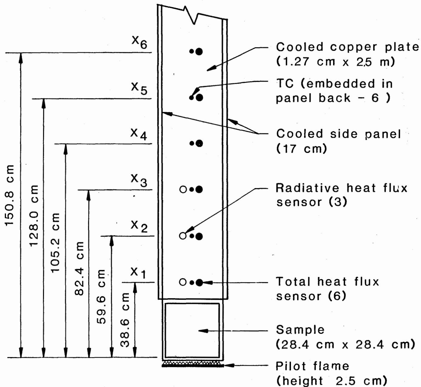
FIGURE 3.9. SCHEMATIC OF FLAME HEIGHT AND HEAT TRANSFER APPARATUS.
