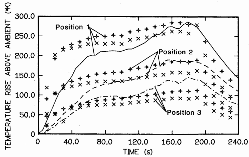
FIGURE 2.11. COMPUTED TEST 111, LOWER CEILING SURFACE TEMPERATURE (+: \beta=0. ; x: \beta=3.0\text{m}^2 ) AND CORRESPONDING MEASURED NEAR-CEILING TEMPERATURES AT POSITIONS 1, 2, and 3.
