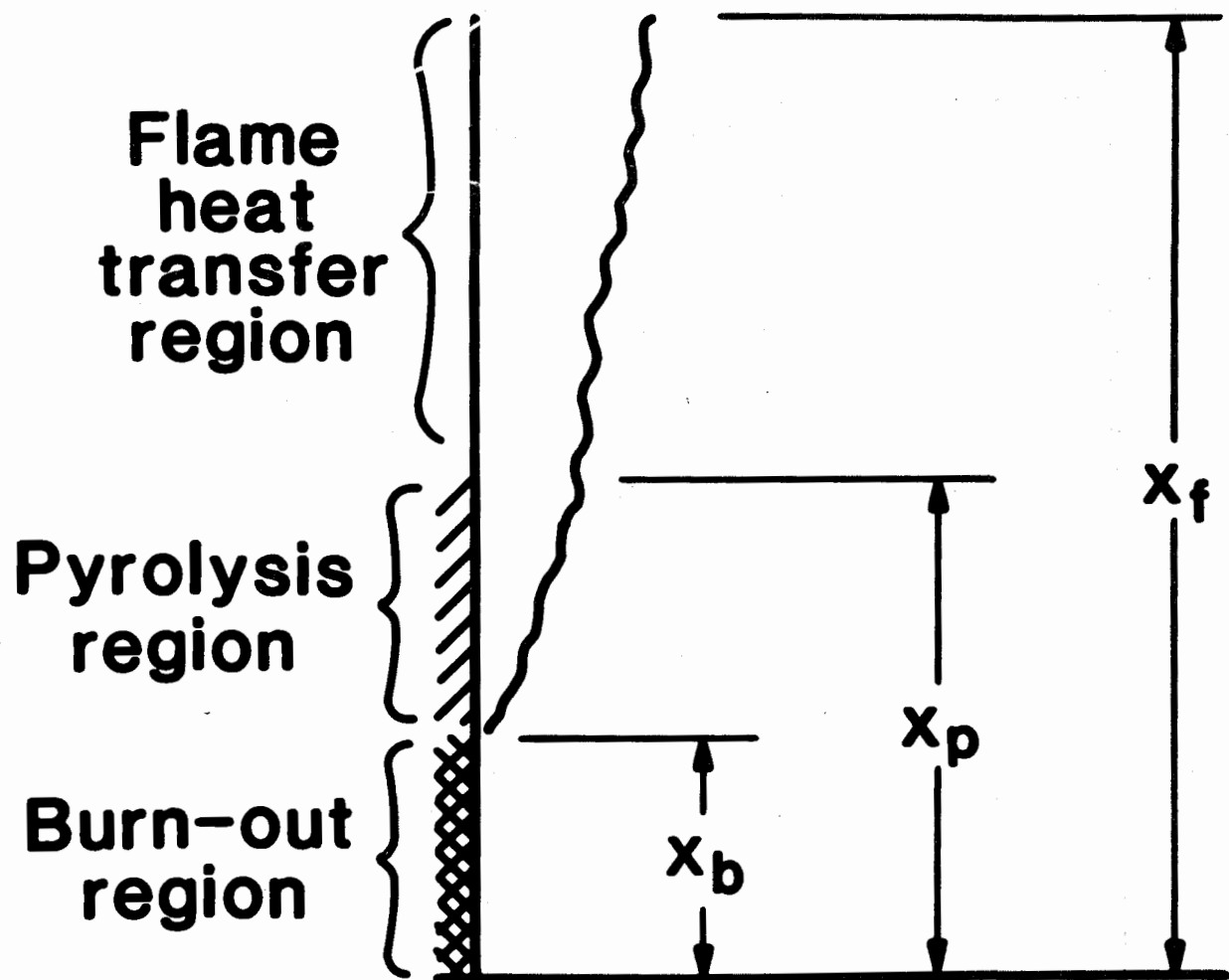
FIGURE 3.10. SCHEMATIC OF FLAME SPREAD PROBLEM.
