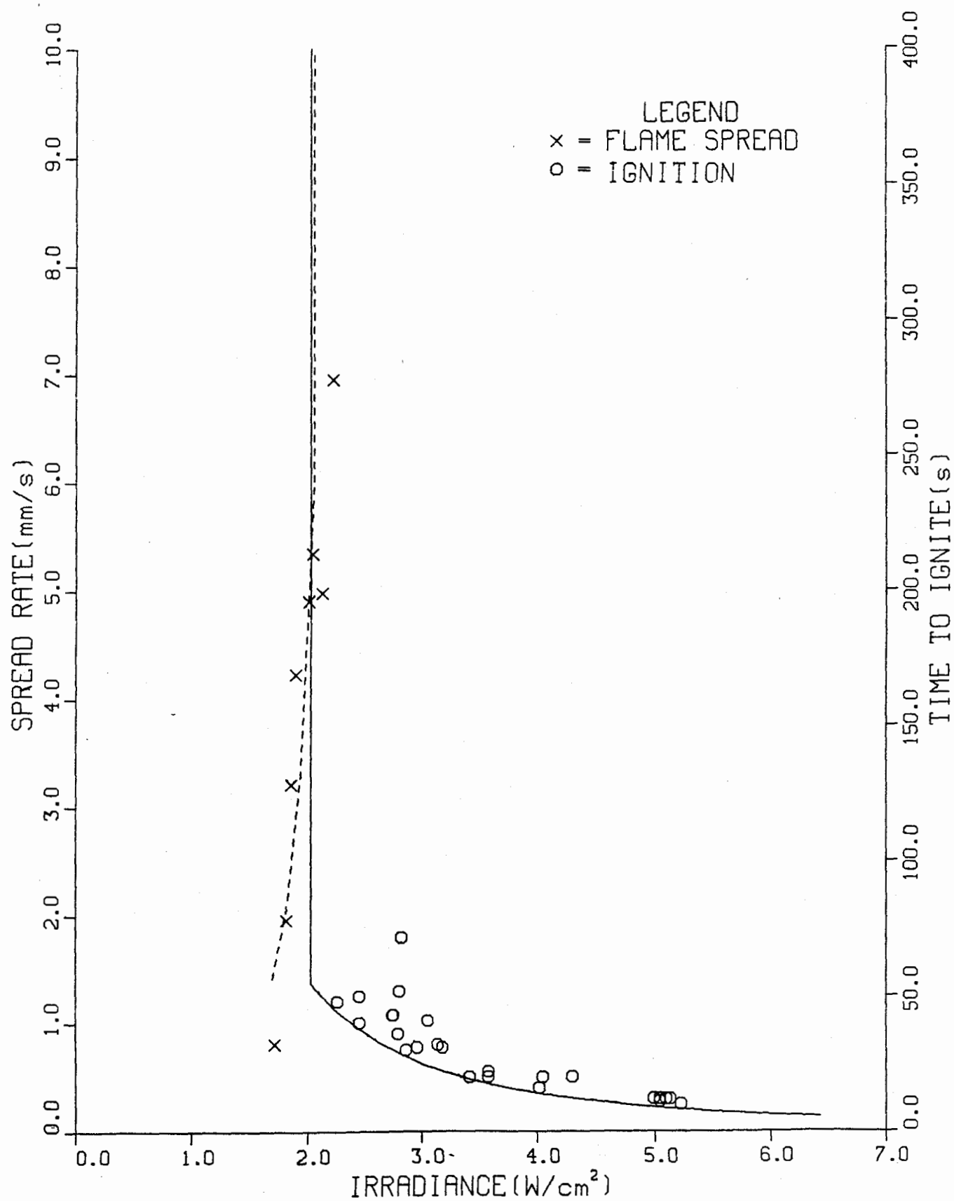
FIGURE 3.5. SPREAD AND IGNITION RESULTS FOR AIRCRAFT PANEL #3, EPOXY KEVLAR.
