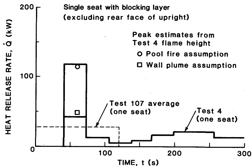
FIGURE 1.7. HEAT RELEASE RATE FROM SINGLE VONAR-3 SEAT (EXCLUDING REAR FACE OF UPRIGHT) BASED ON: —, CALORIMETER DATA AND AREA-OF-INVOLVEMENT DATA FROM TEST 4; ○, □, FLAME HEIGHT DATA FROM TEST 4; ----, MASS LOSS DATA FROM TEST 107.
