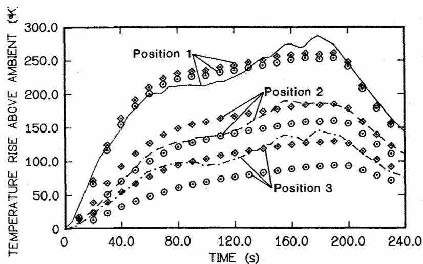
FIGURE 2.13 PREDICTED AND MEASURED TEST 111 THERMOCOUPLE TEMPERATURES (\beta = 2.0 \text{ m}^2) . \diamond : PREDICTED T_w , CONFIGURATION 1 \circ : PREDICTED T_w , CONFIGURATION 2 —, — — —, — — — — —: MEASURED T_w
