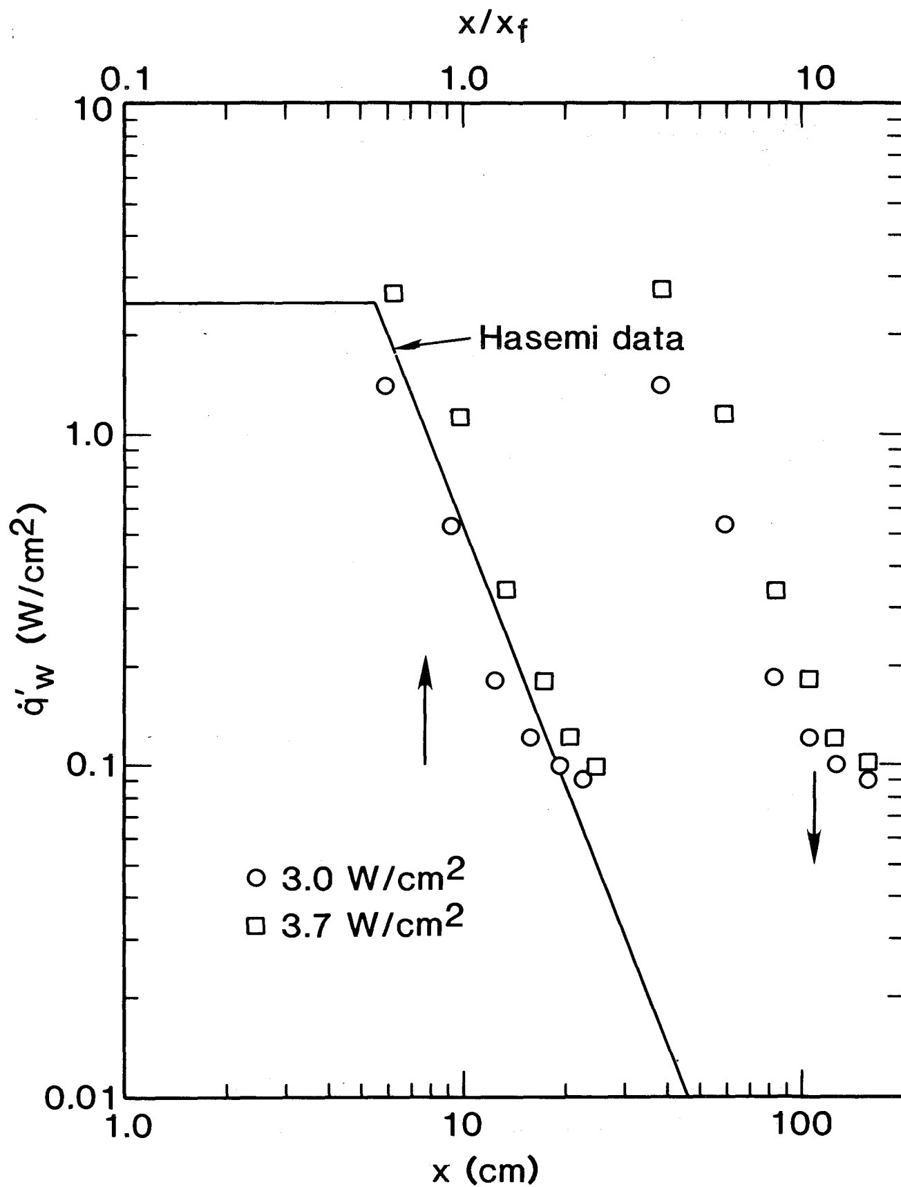
FIGURE 3.14. WALL HEAT FLUX DISTRIBUTION FOR AIRCRAFT PANEL #4, PHENOLIC KEVLAR.
