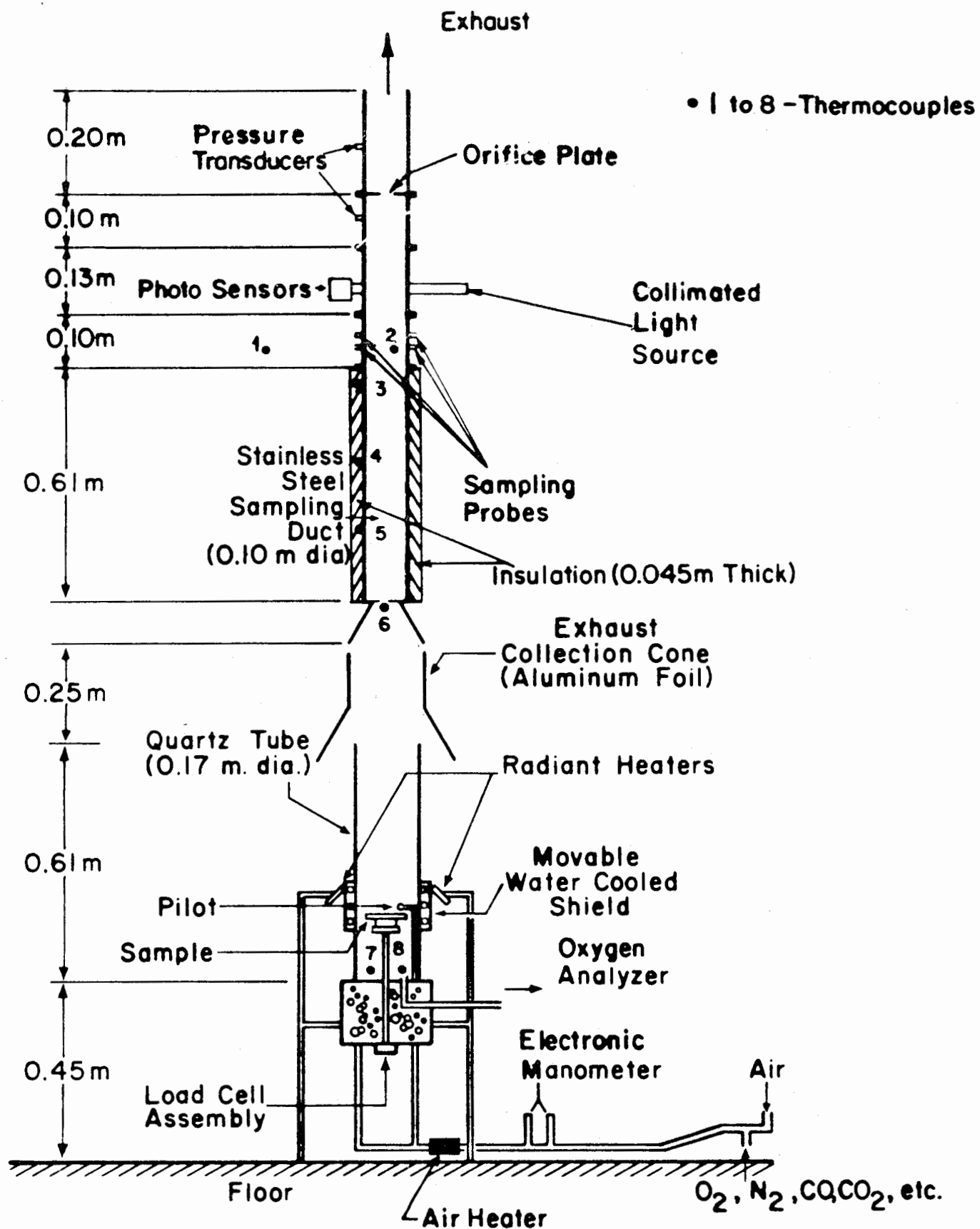
FIGURE 5.1. EXPERIMENTAL APPARATUS
