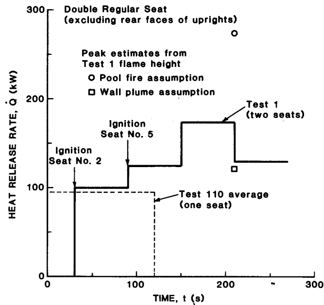
FIGURE 1.5. HEAT RELEASE RATE FROM DOUBLE REGULAR SEAT (EXCLUDING REAR FACES OF UPRIGHTS) BASED ON: —, CALORIMETER DATA AND AREA-OF-INVOLVEMENT DATA FROM TEST 1: ○ - □, FLAME HEIGHT DATA FROM TEST 1; ----, MASS LOSS DATA FROM TEST 110.
