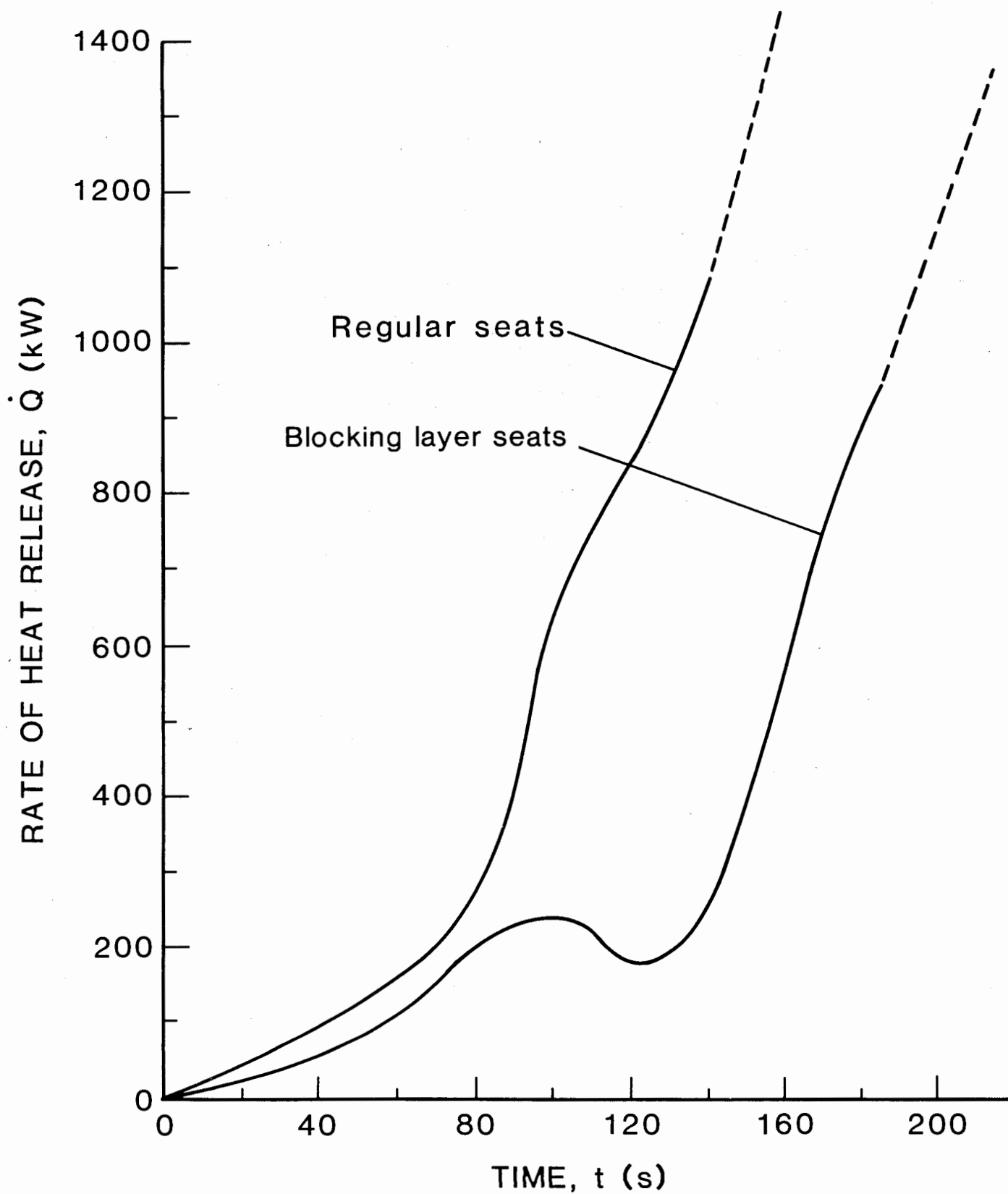
FIGURE 2.16. ESTIMATE FOR \dot{Q}_{seat} FOR ARRAYS OF POLYURETHANE SEATS WITH AND WITHOUT BLOCKING LAYERS [13] ( — — — EXTRAPOLATED FROM CURVES OF [13]).
