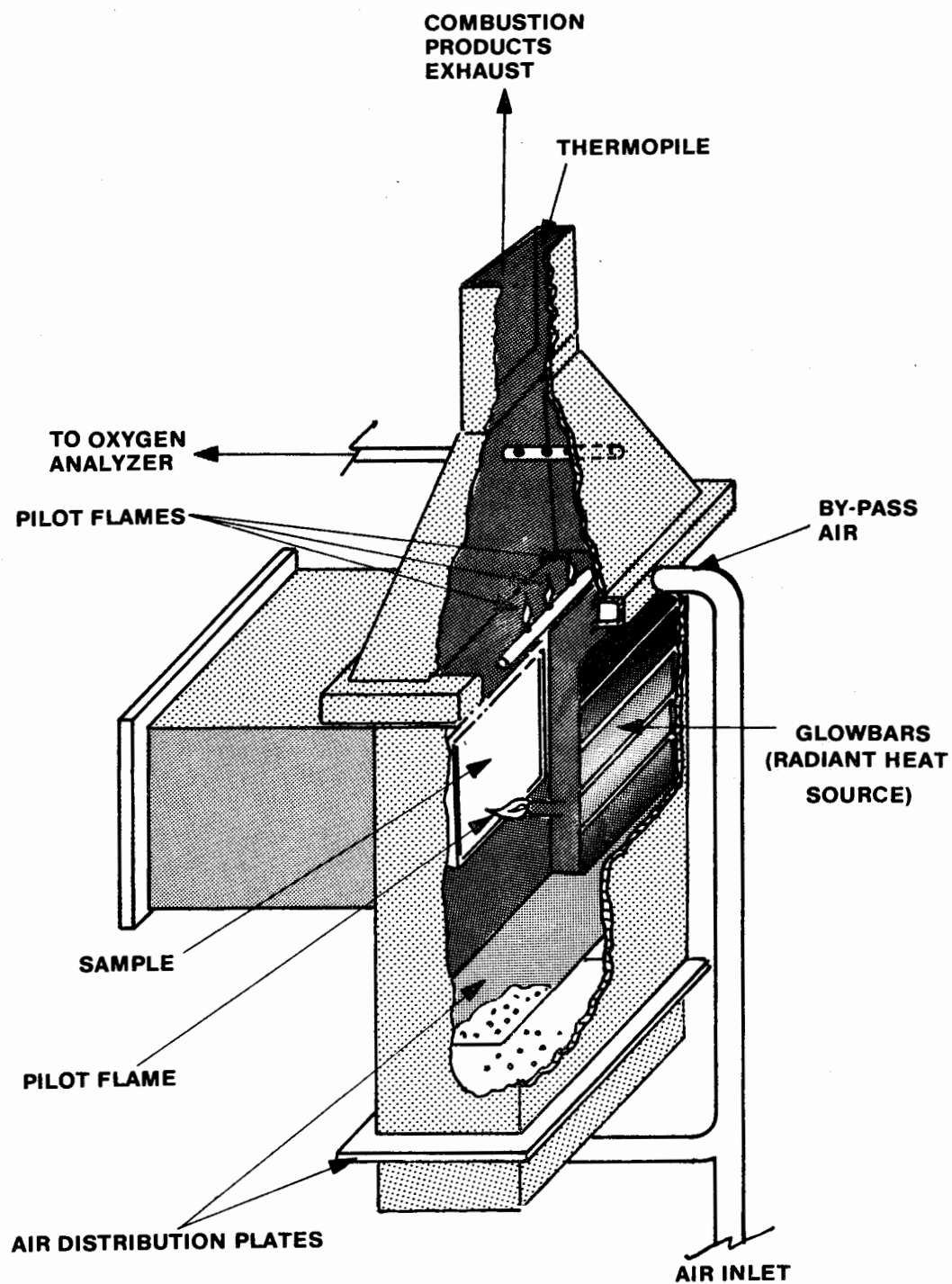
FIGURE 5. FAA OHIO STATE HEAT RELEASE APPARATUS
