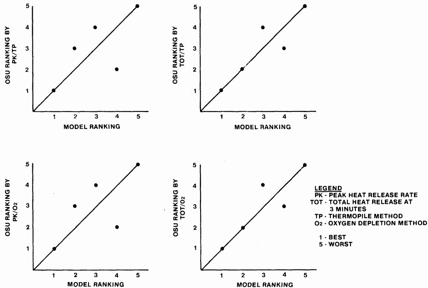
FIGURE 15. COMPARISON OF MATERIALS RANKING BETWEEN MODEL AND OSU APPARATUS AT 2.5 \text{ W/CM}^2 , PILOTTED
