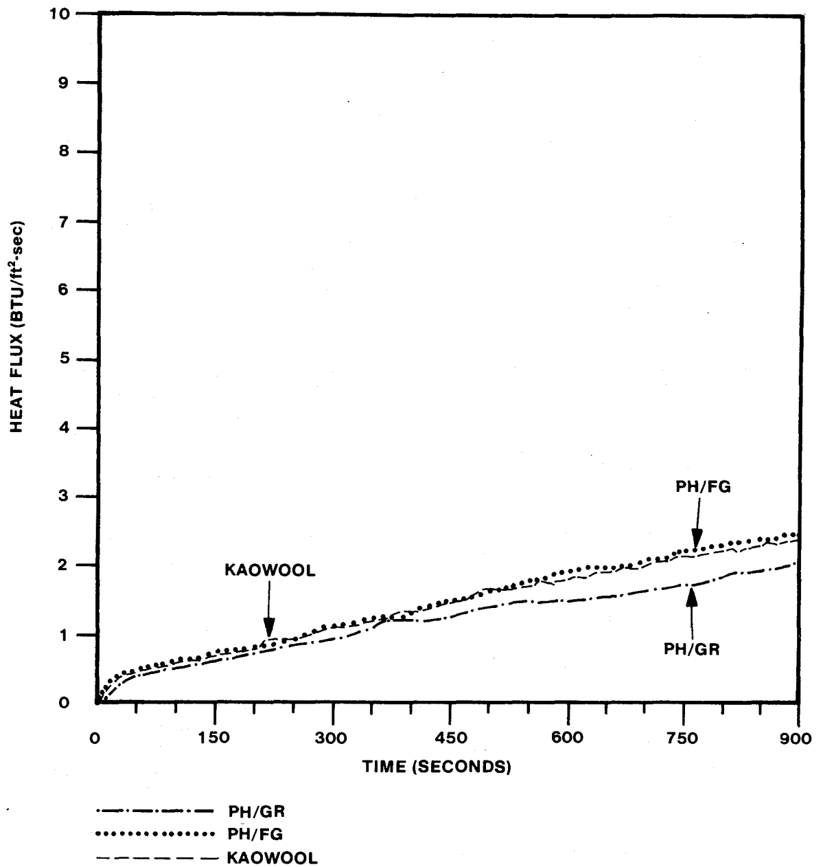
FIGURE 9. HEAT FLUX PROFILE FOR FIRE RESISTANT PANELS
