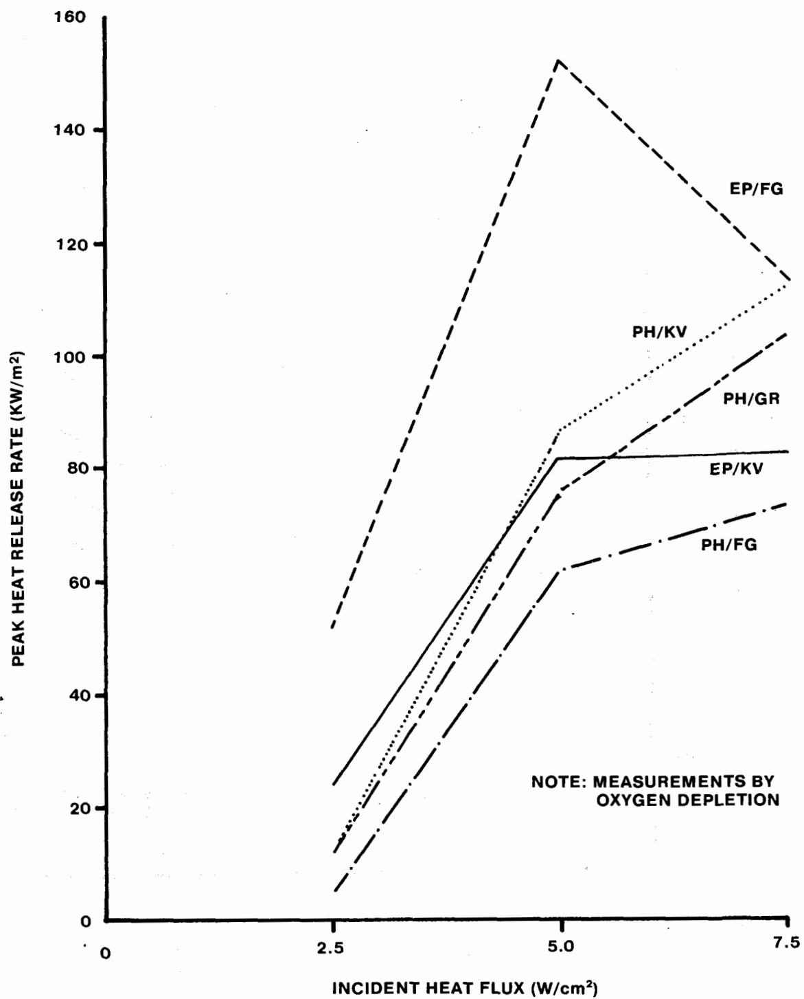
FIGURE 10. PEAK HEAT RELEASE RATE DATA (O 2 DEPLETION) FOR AIRCRAFT PANELS BY OSU APPARATUS
