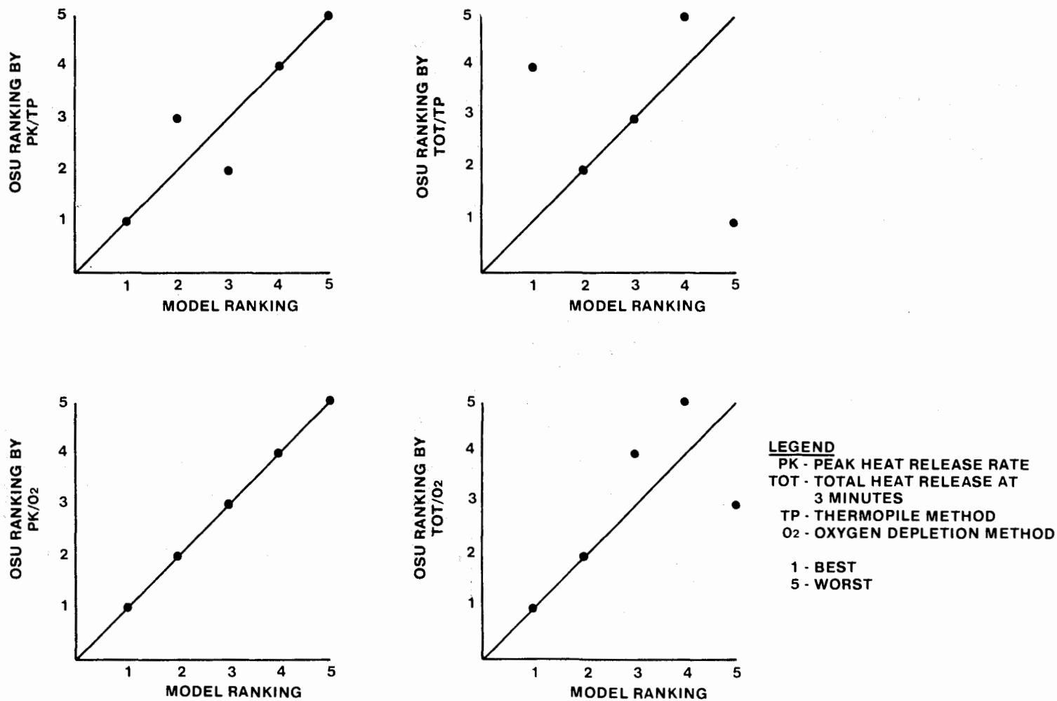
FIGURE 16. COMPARISON OF MATERIALS RANKING BETWEEN MODEL AND OSU AT 5.0 W/CM 2 , PILOTTED
