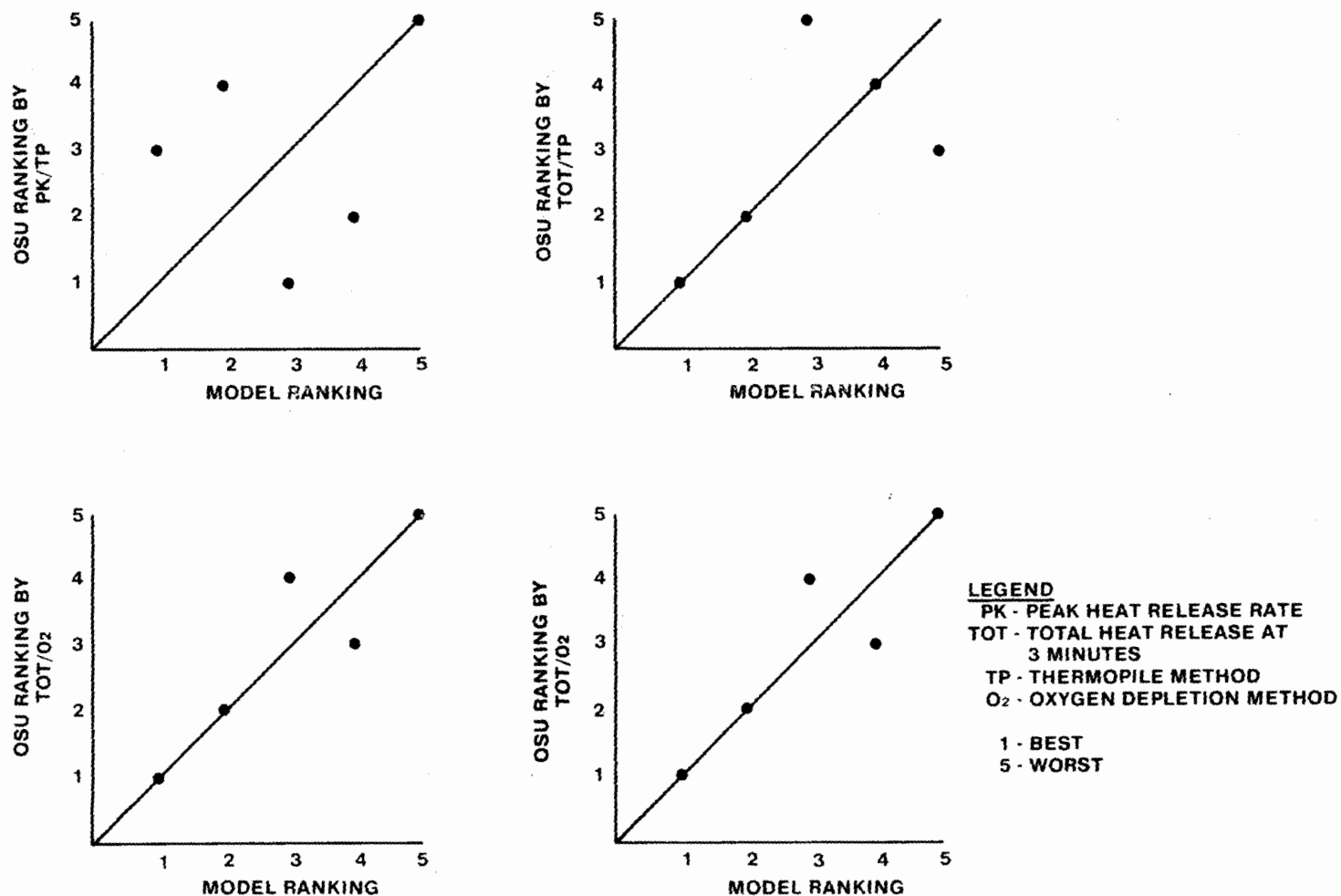
FIGURE 17. COMPARISON OF MATERIALS RANKING BETWEEN MODEL AND OSU APPARATUS AT 5 W/CM 2 , NON-PILOTED
