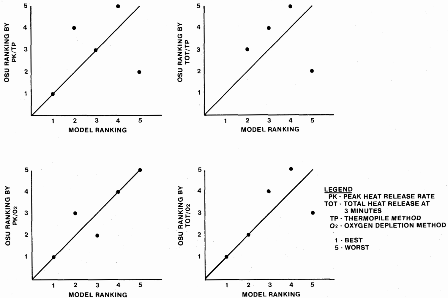
FIGURE 18. COMPARISON OF MATERIALS RANKING BETWEEN MODEL AND OSU APPARATUS AT 7.5 \text{ W/CM}^2 , PILOTTED
