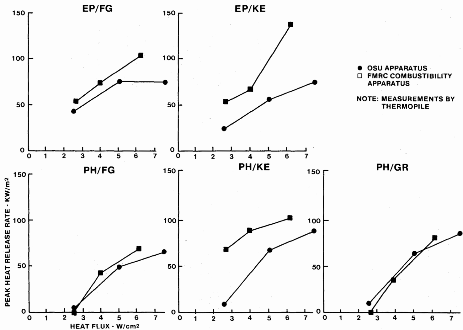
FIGURE 21. COMPARISON OF PEAK HEAT RELEASE RATE BY THERMOPILE MEASUREMENT IN THE OSU AND COMBUSTIBILITY APPARATUSES
