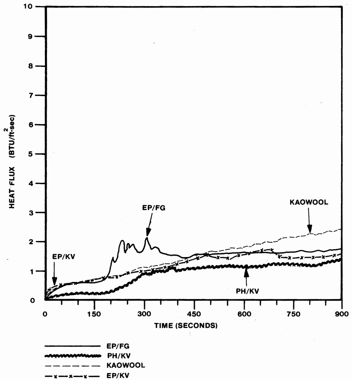
FIGURE 8. HEAT FLUX PROFILE FOR FLAMMABLE PANELS
