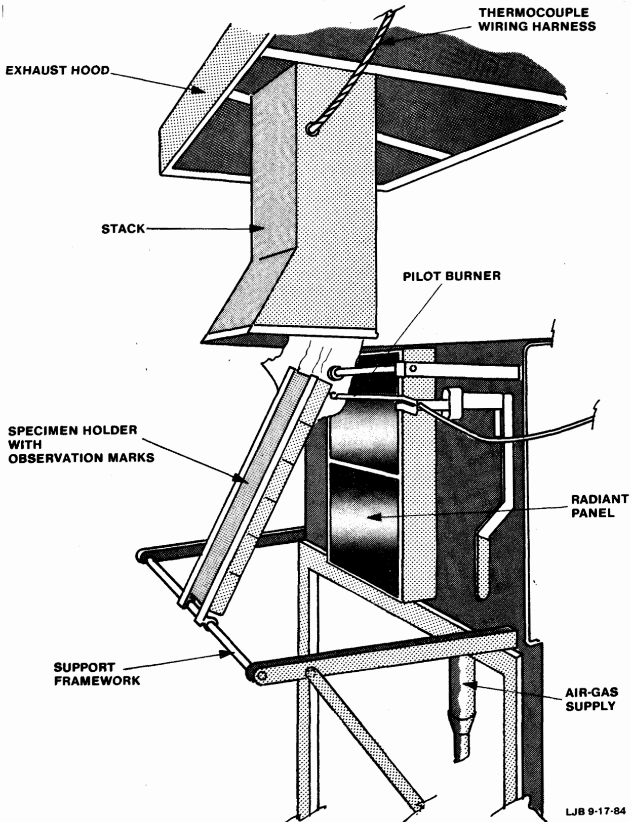
FIGURE 4. RADIANT PANEL TEST METHOD
