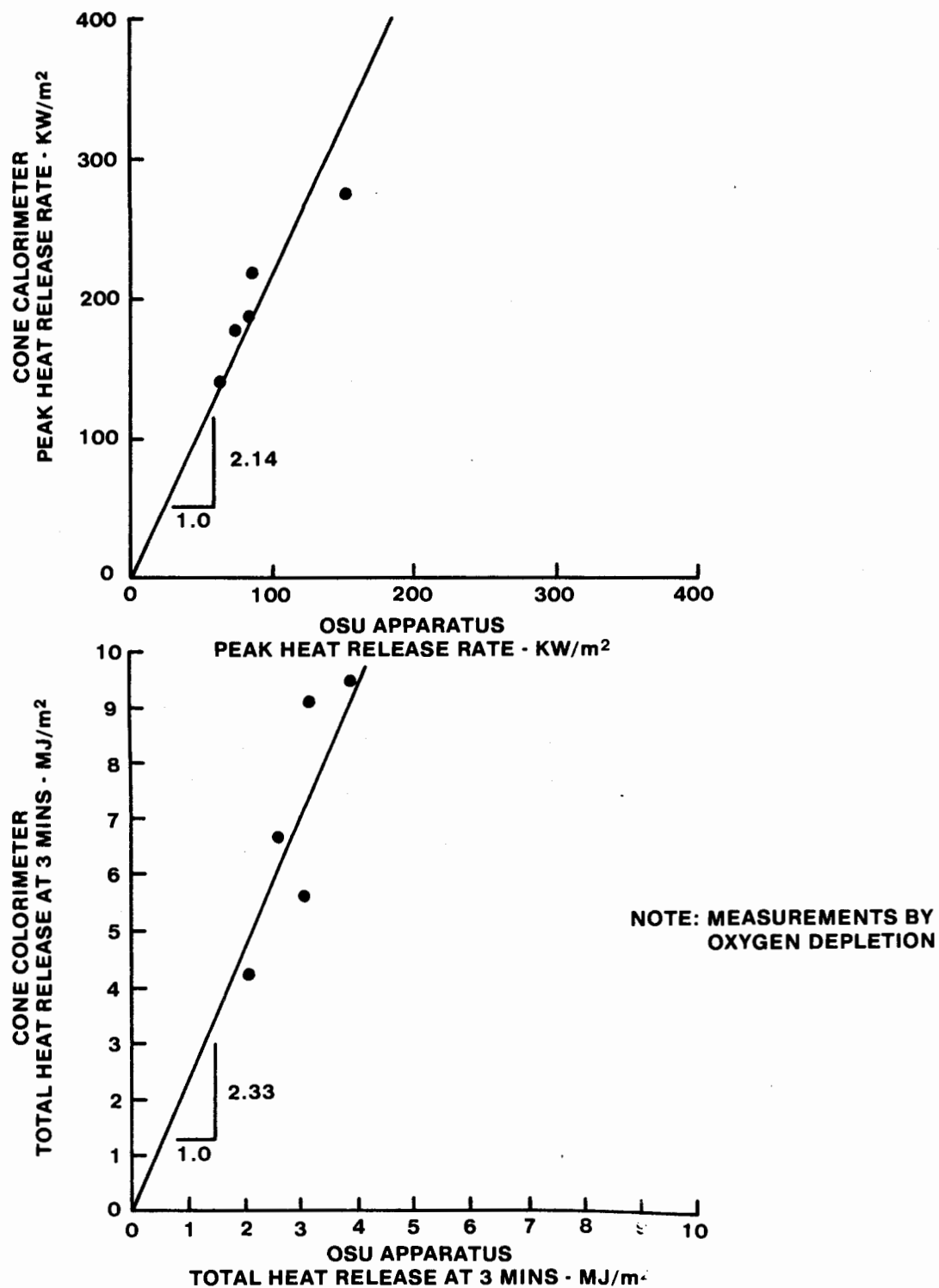
FIGURE 20. COMPARISON OF HEAT RELEASE DATA BETWEEN CONE CALORIMETER AND OSU APPARATUS
