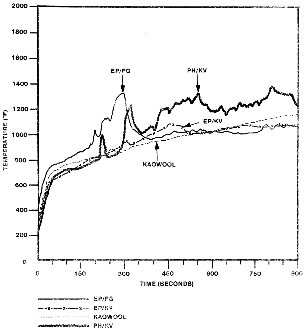
FIGURE 6. MODEL CEILING TEMPERATURE PROFILE FOR FLAMMABLE PANELS
