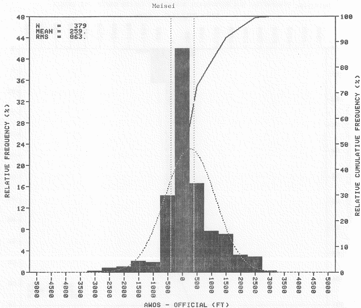
FIGURE 12. CLOUD HEIGHT DIFFERENCE HISTOGRAMS FOR CEILOMETERS WHEN OFFICIAL CEILING IS GREATER THAN 1,500 FEET (SHEET 2 OF 2)
