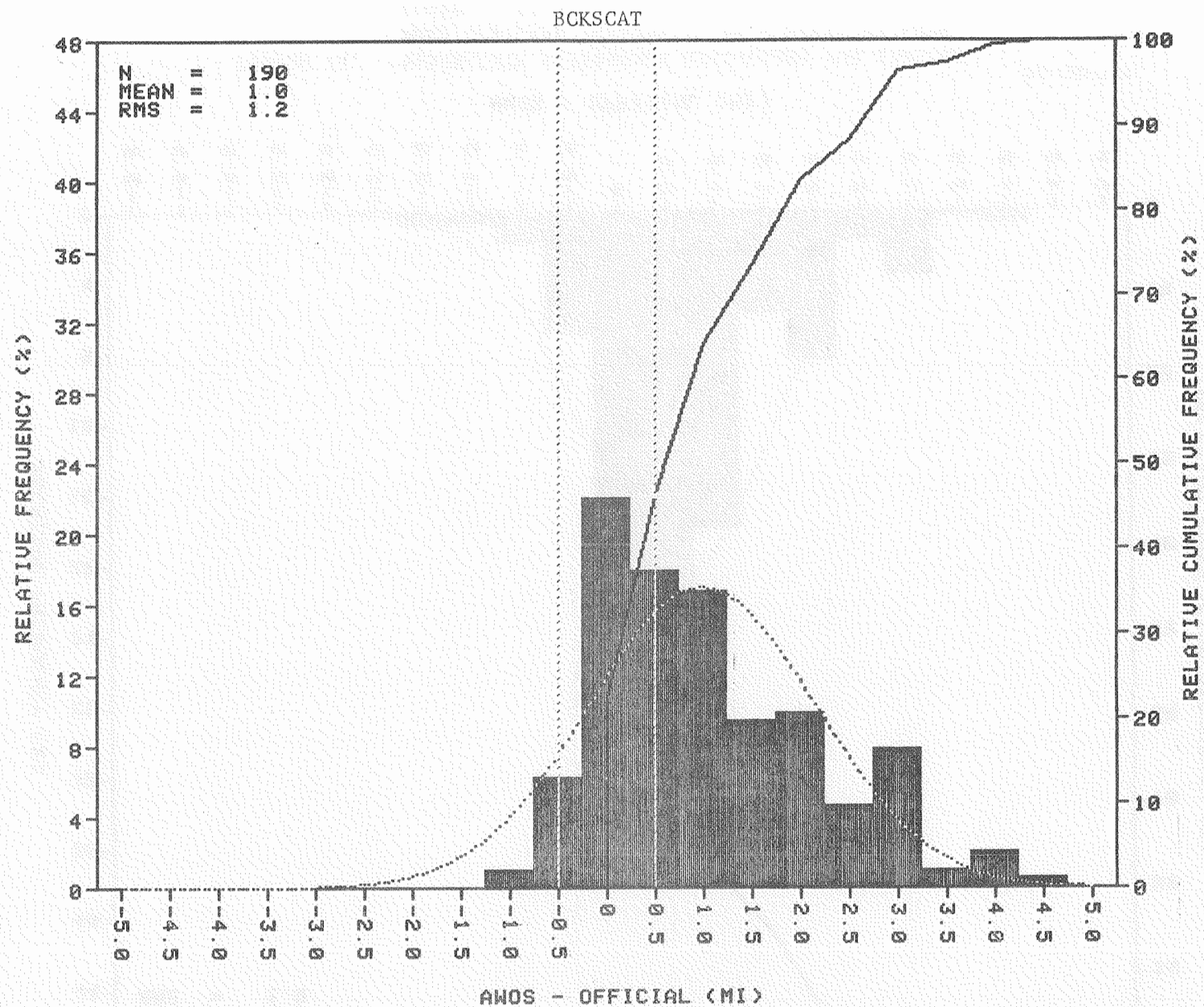
FIGURE 18. VISIBILITY DIFFERENCE HISTOGRAMS FOR SENSORS WHEN OFFICIAL VISIBILITY IS 2 MILES OR LESS (SHEET 1 OF 2)
