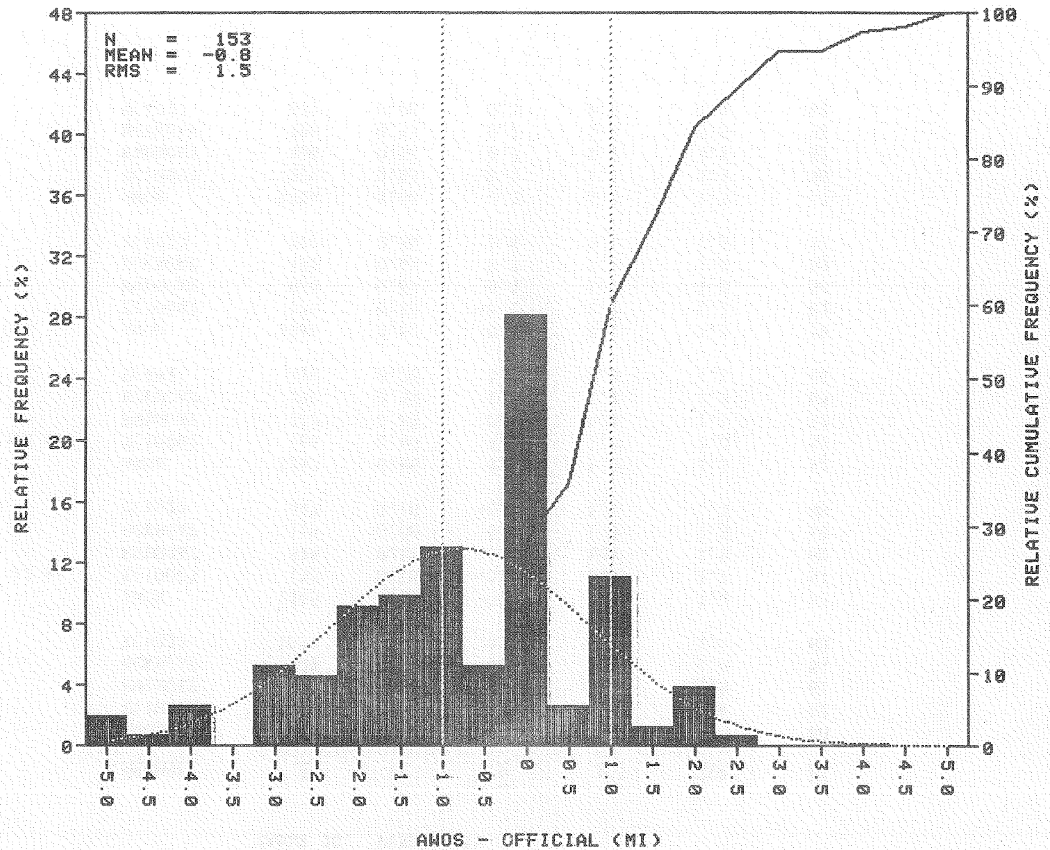
FIGURE 15. VISIBILITY DIFFERENCE HISTOGRAMS FOR SENSORS WHEN OFFICIAL VISIBILITY IS GREATER THAN 2 MILES (SHEET 1 OF 2)
