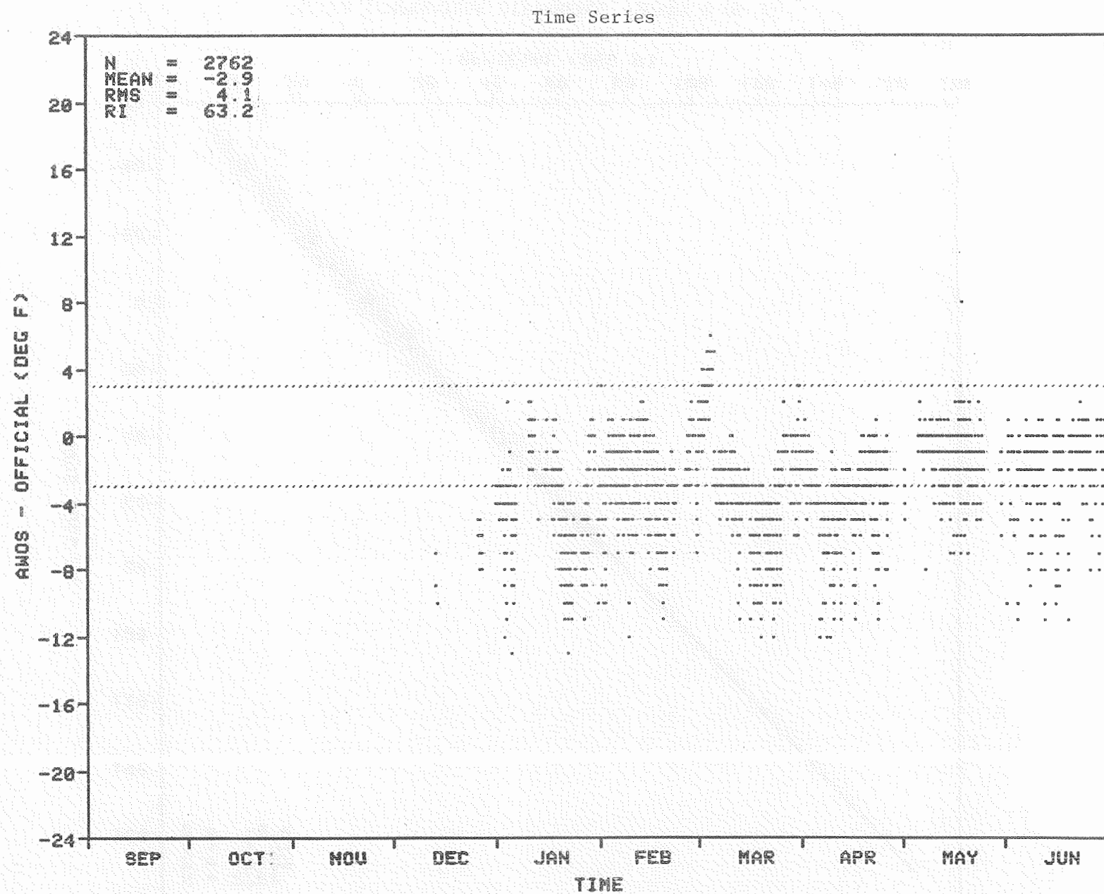
FIGURE 19. GALENA TEMPERATURE DIFFERENCE (SHEET 1 OF 2)
