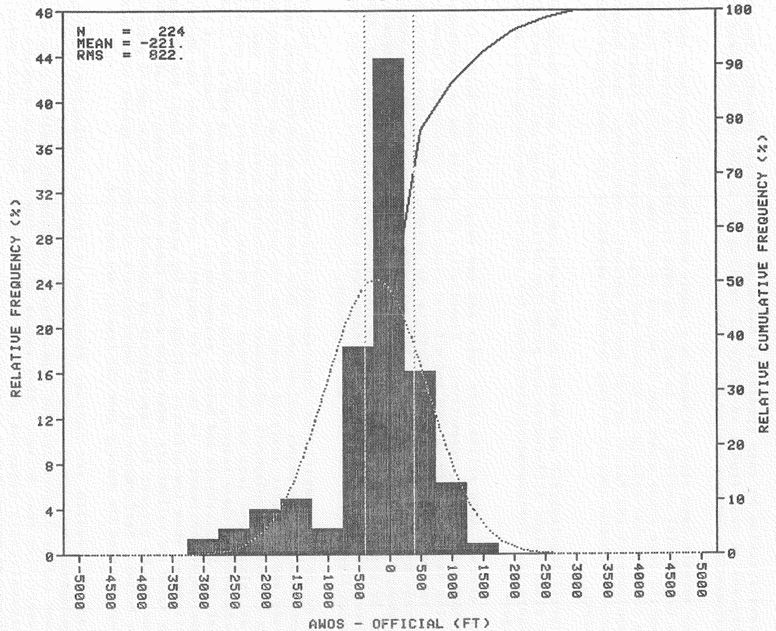
FIGURE 12. CLOUD HEIGHT DIFFERENCE HISTOGRAMS FOR CEILOMETERS WHEN OFFICIAL CEILING IS GREATER THAN 1,500 FEET (SHEET 1 OF 2)
