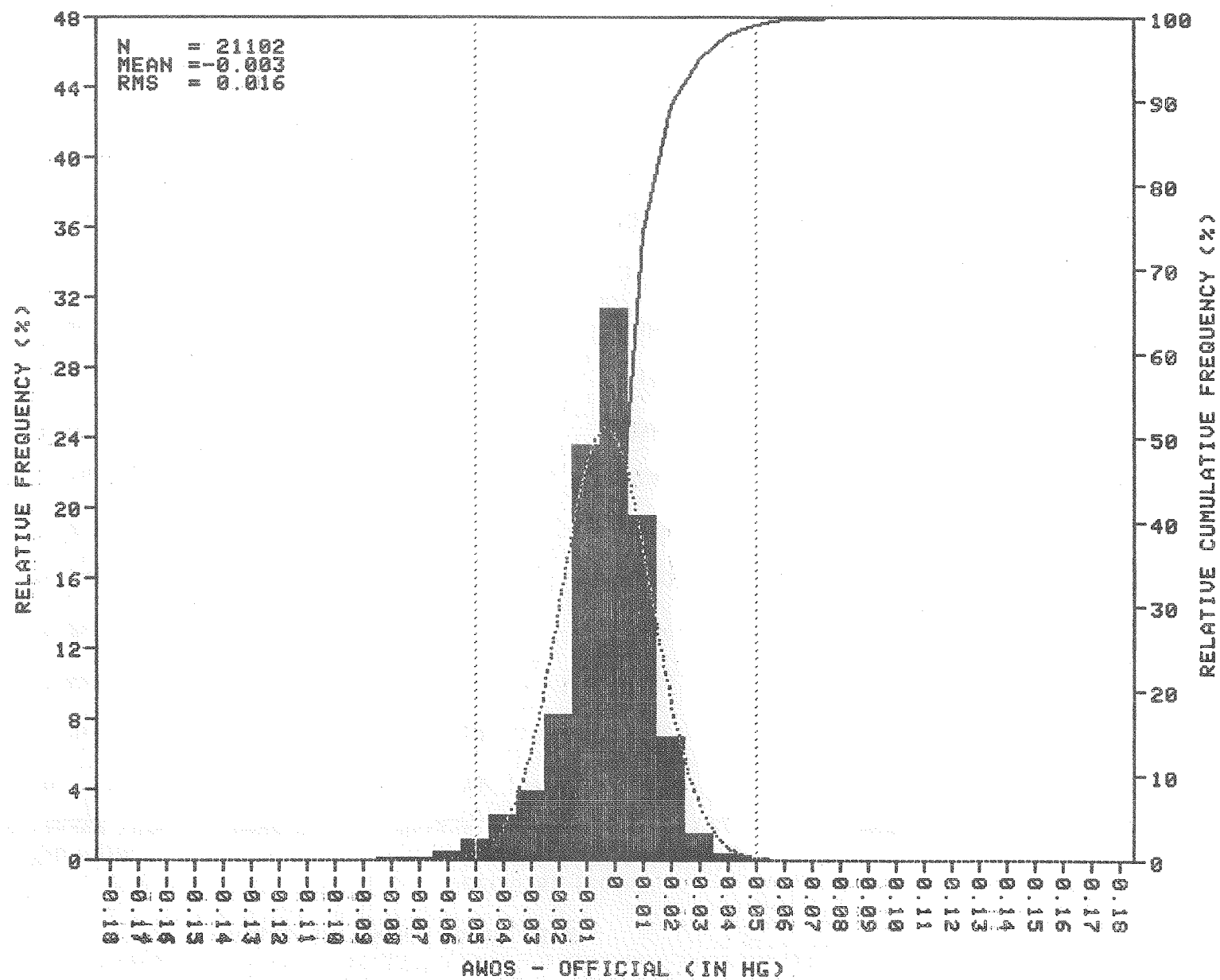
FIGURE 23. OVERALL AWOS ALTIMETER SETTING DIFFERENCE HISTOGRAM
