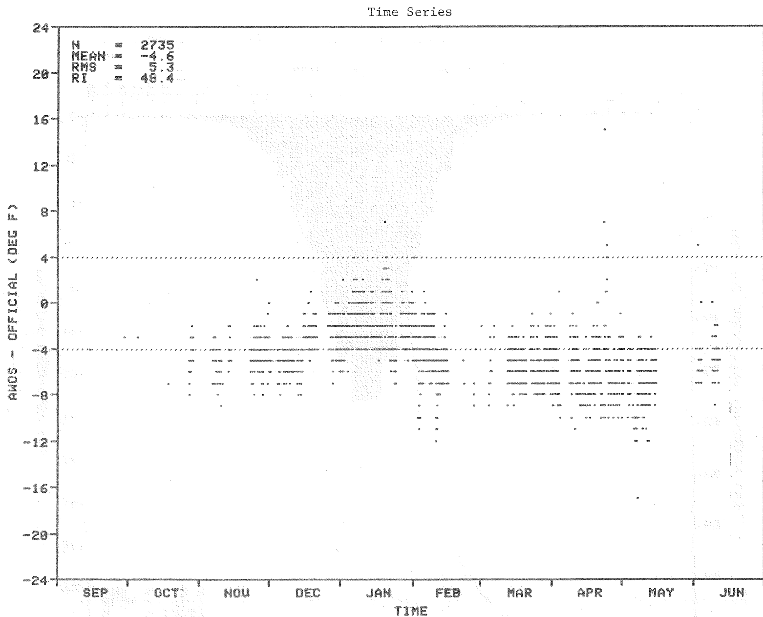
FIGURE 22. WASHINGTON, D.C., DEW POINT TEMPERATURE DIFFERENCE (SHEET 1 OF 2)
