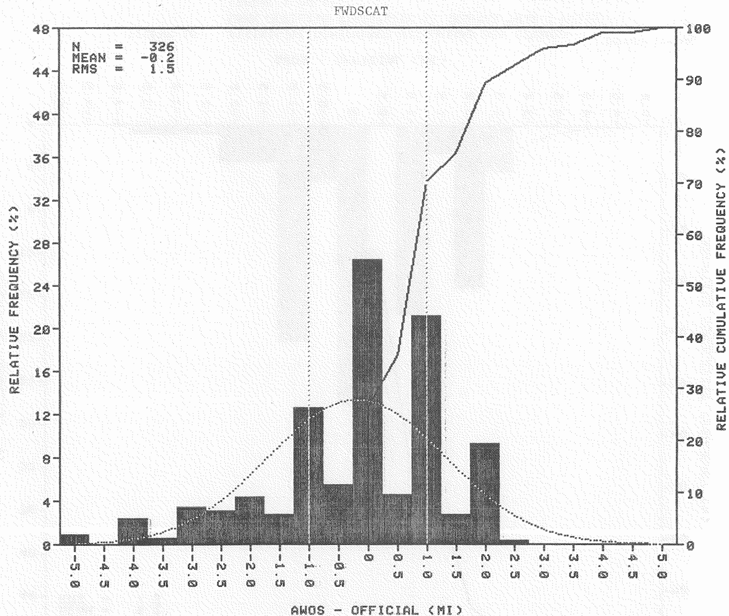
FIGURE 15. VISIBILITY DIFFERENCE HISTOGRAMS FOR SENSORS WHEN OFFICIAL VISIBILITY IS GREATER THAN 2 MILES (SHEET 2 OF 2)
