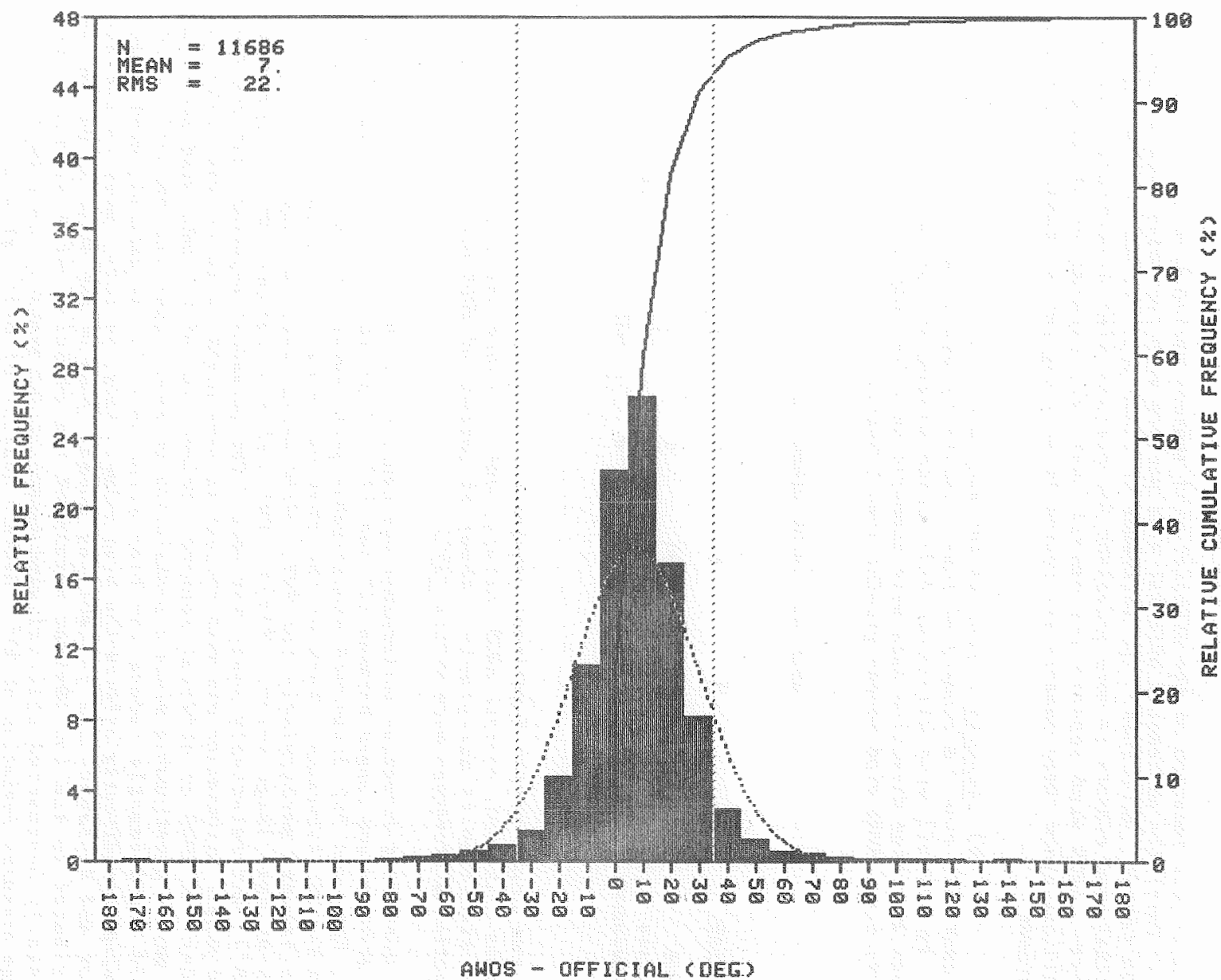
FIGURE 24. OVERALL AWOS WIND DIRECTION DIFFERENCE HISTOGRAM
