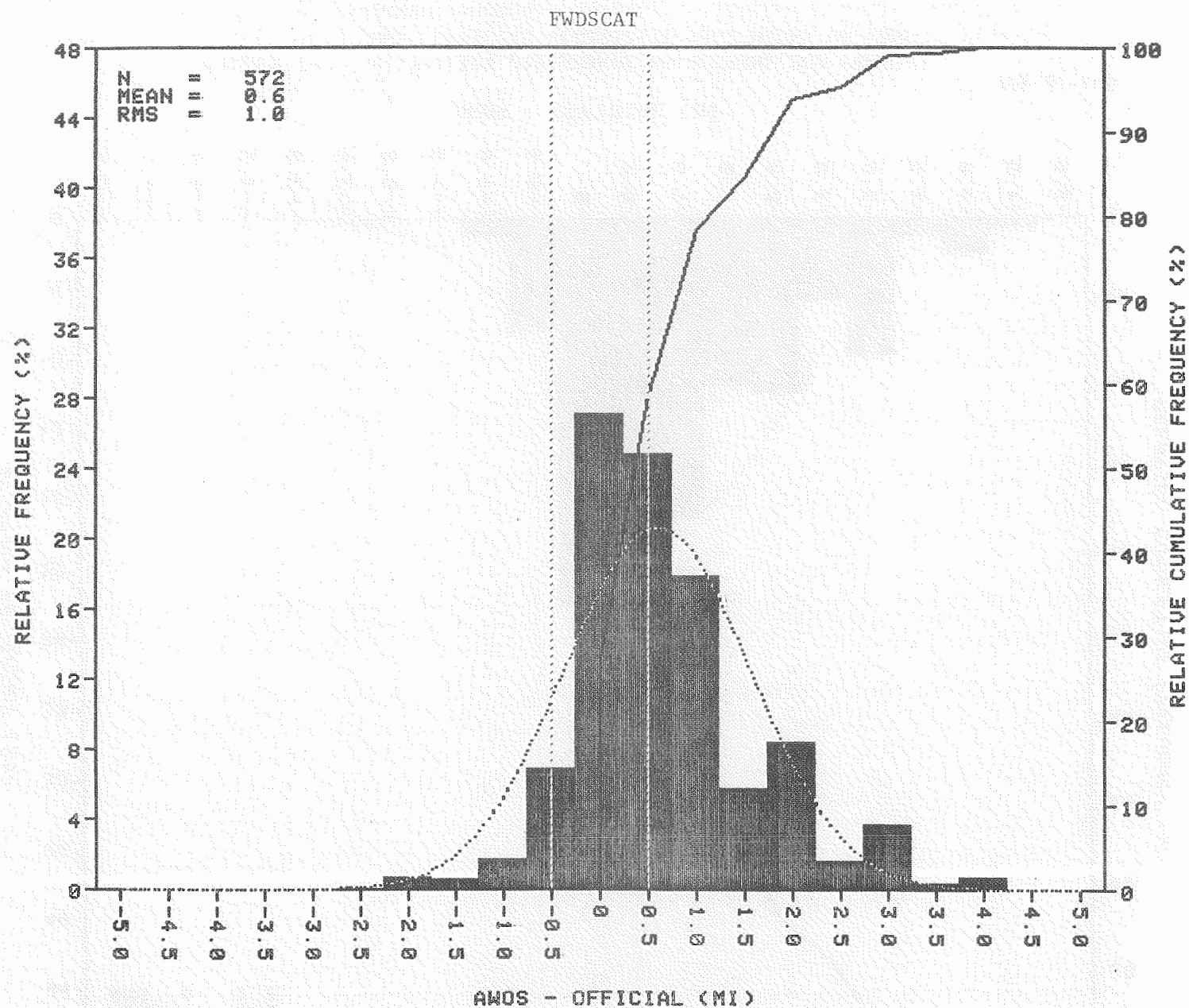
FIGURE 17. VISIBILITY DIFFERENCE HISTOGRAMS FOR SENSORS WHEN OFFICIAL VISIBILITY IS 2 MILES OR LESS (SHEET 2 OF 2)
