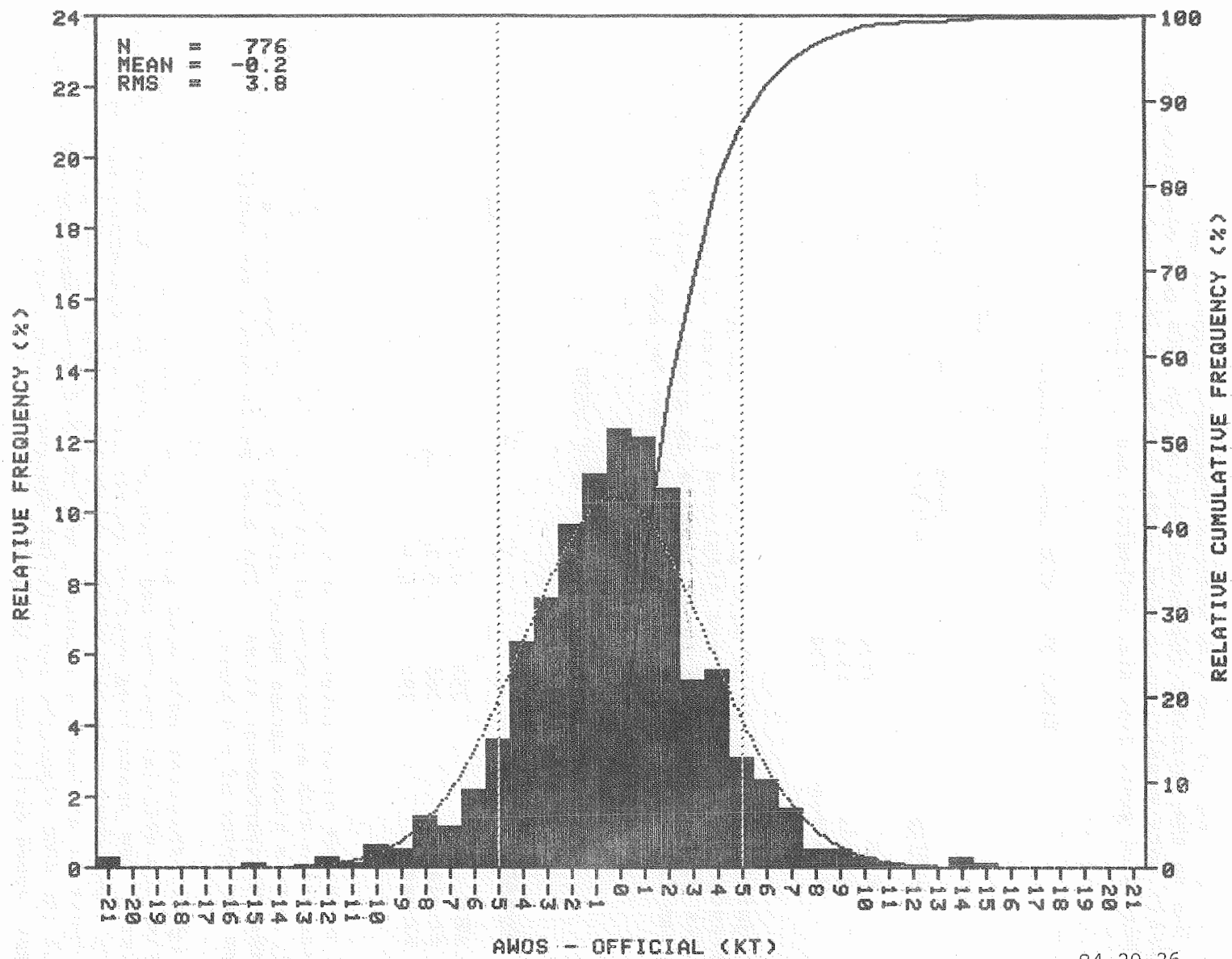
FIGURE 26. OVERALL AWOS WIND GUST SPEED DIFFERENCE HISTOGRAM
