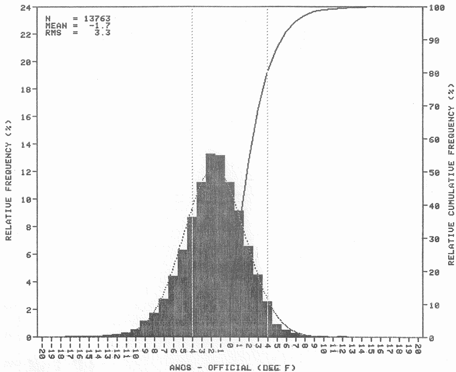
FIGURE 21. OVERALL AWOS DEW POINT TEMPERATURE DIFFERENCE HISTOGRAM
