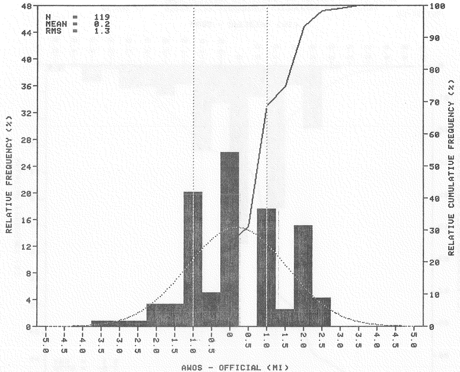
FIGURE 16. VISIBILITY DIFFERENCE HISTOGRAMS FOR SENSORS WHEN OFFICIAL VISIBILITY IS GREATER THAN 2 MILES (SHEET 1 OF 2)
