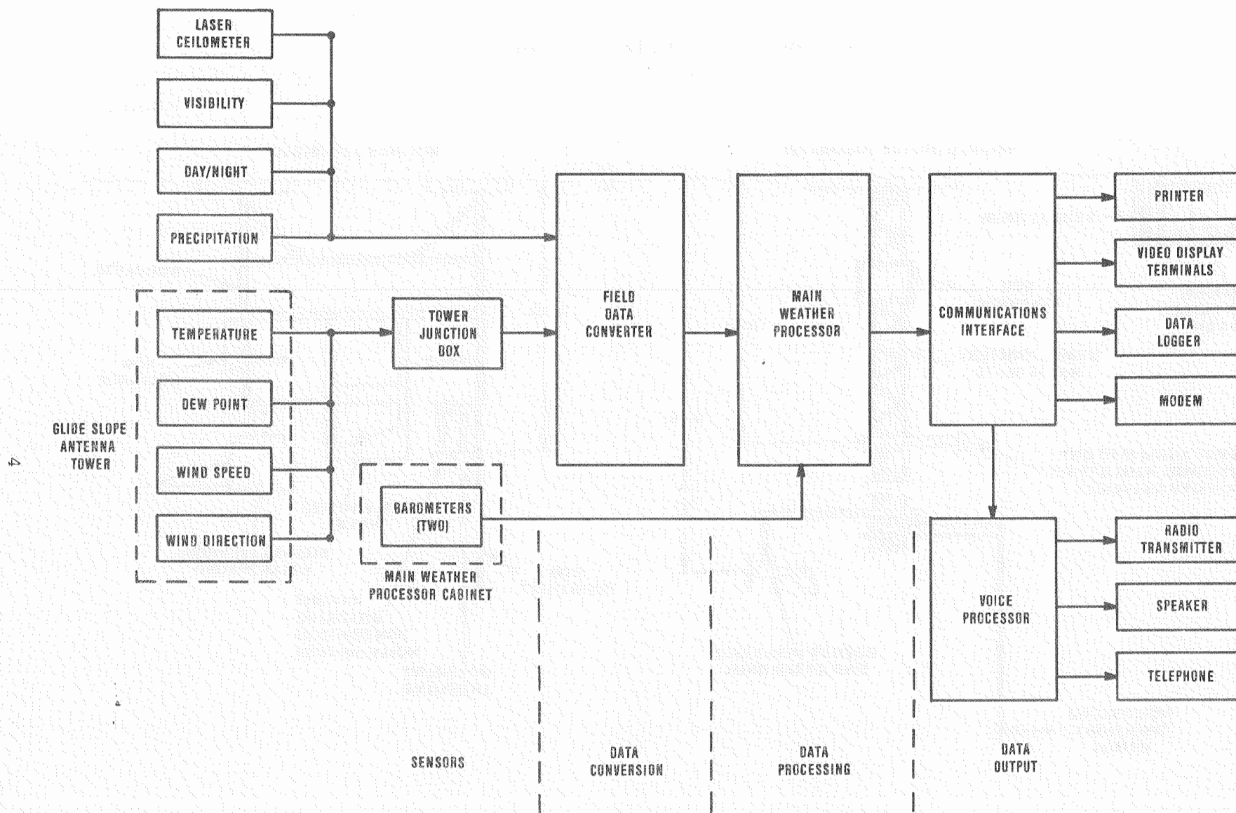
FIGURE 2. AWOS SYSTEM BLOCK DIAGRAM
