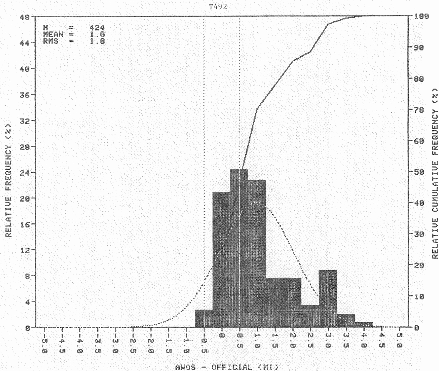
FIGURE 18. VISIBILITY DIFFERENCE HISTOGRAMS FOR SENSORS WHEN OFFICIAL VISIBILITY IS 2 MILES OR LESS (SHEET 2 of 2)
