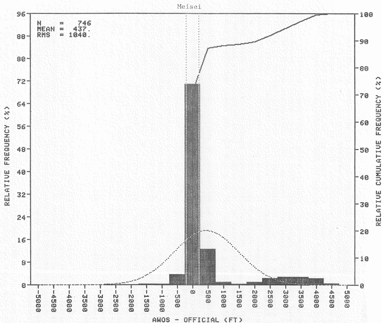
FIGURE 13. CLOUD HEIGHT DIFFERENCE HISTOGRAMS FOR CEILOMETERS WHEN OFFICIAL CEILING IS 1,500 FEET OR LESS (SHEET 2 OF 2)
