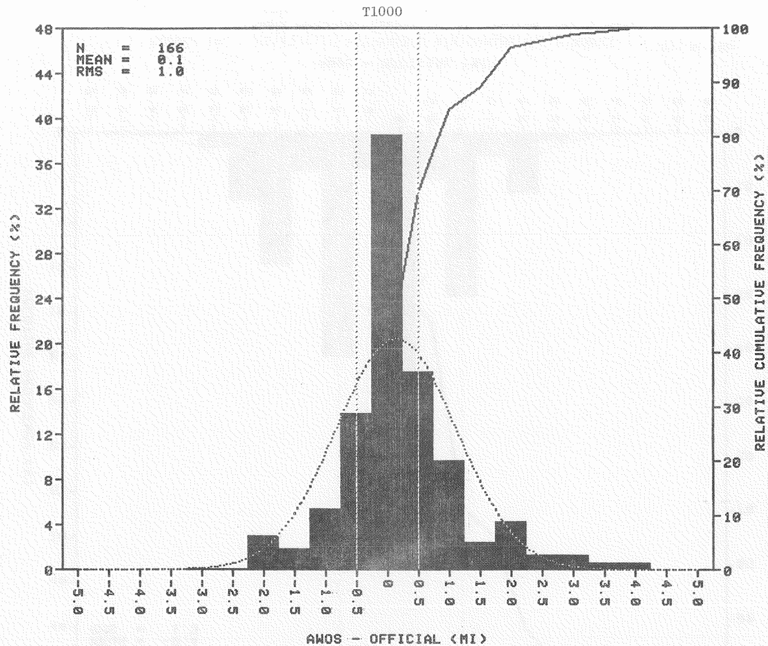
FIGURE 17. VISIBILITY DIFFERENCE HISTOGRAMS FOR SENSORS WHEN OFFICIAL VISIBILITY IS 2 MILES OR LESS (SHEET 1 OF 2)
