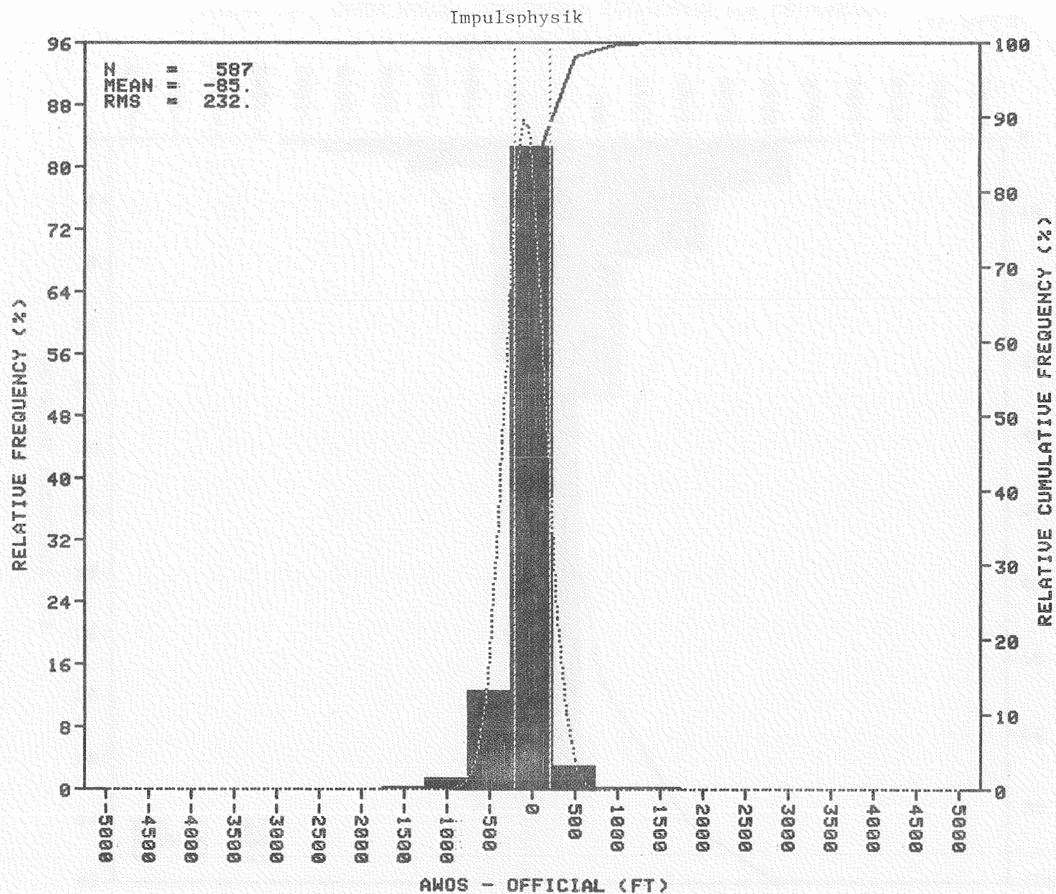
FIGURE 13. CLOUD HEIGHT DIFFERENCE HISTOGRAMS FOR CEILOMETERS 84-20-13a WHEN OFFICIAL CEILING IS 1,500 FEET OR LESS (SHEET 1 OF 2)
