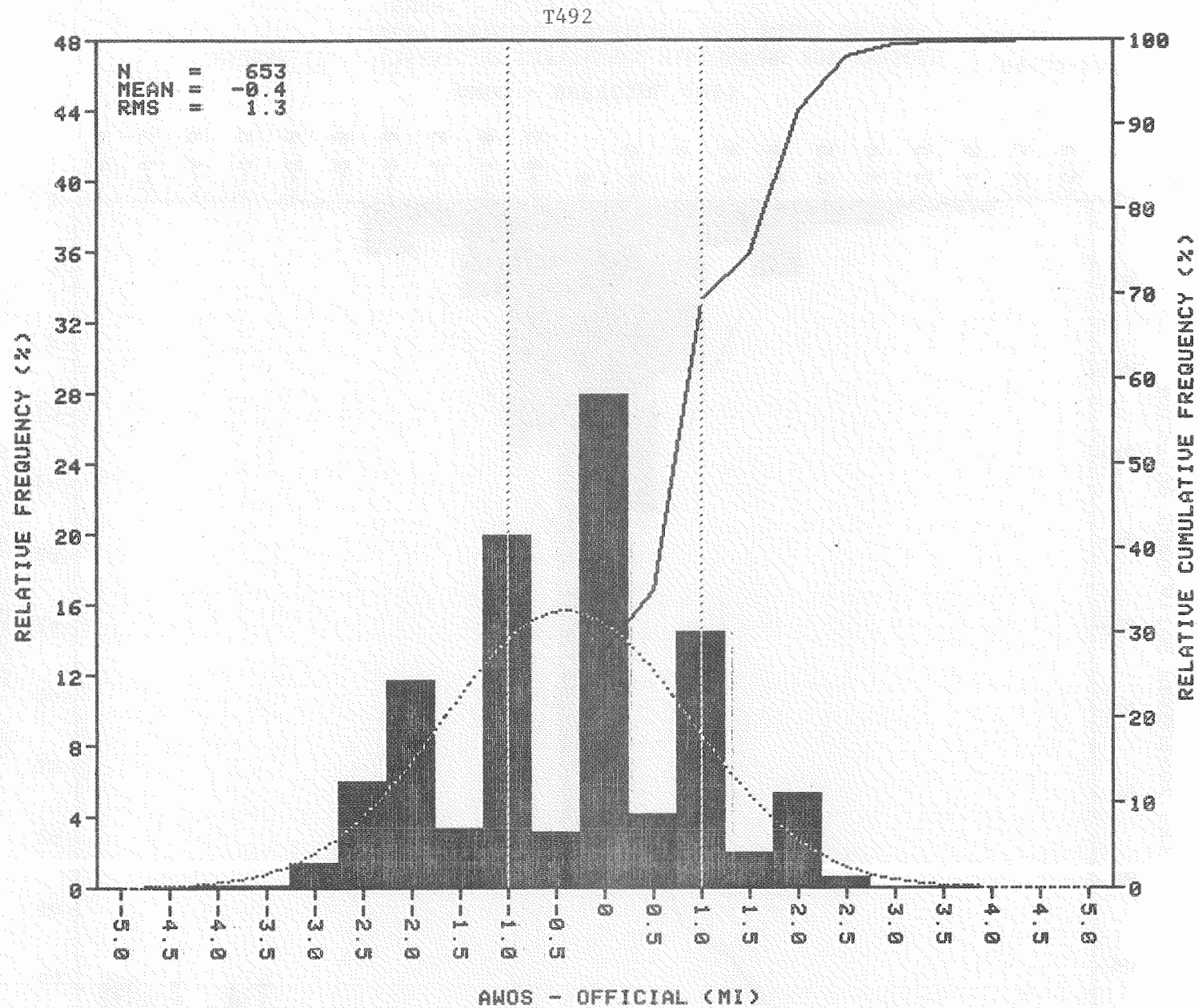
FIGURE 16. VISIBILITY DIFFERENCE HISTOGRAMS FOR SENSORS WHEN OFFICIAL VISIBILITY IS GREATER THAN 2 MILES (SHEET 2 OF 2)
