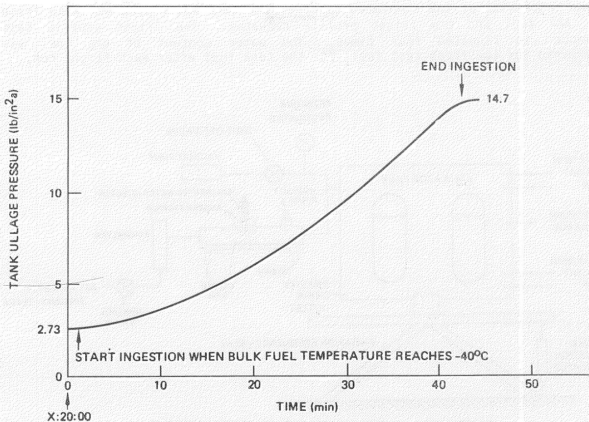
FIGURE 18. WATER VAPOR INGESTION PRESSURE SCHEDULE
