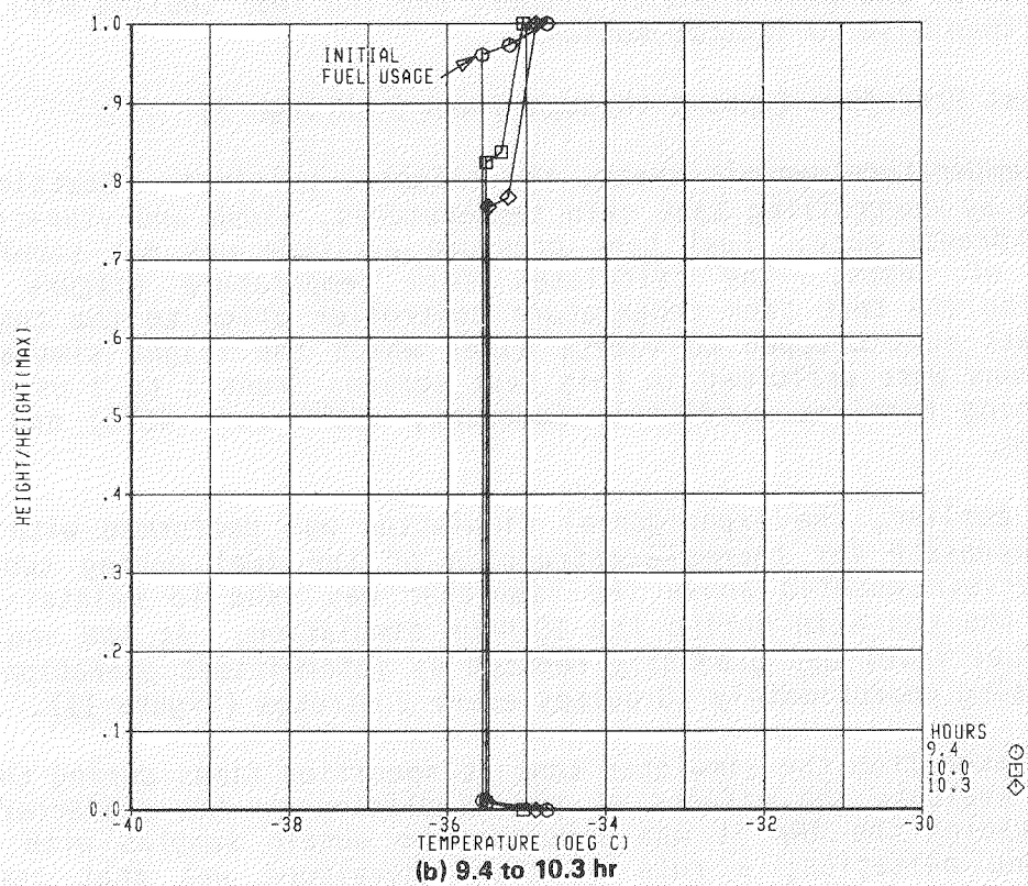
FIGURE 8. CALCULATED FUEL TEMPERATURES-HELSINKI TO SEATTLE
