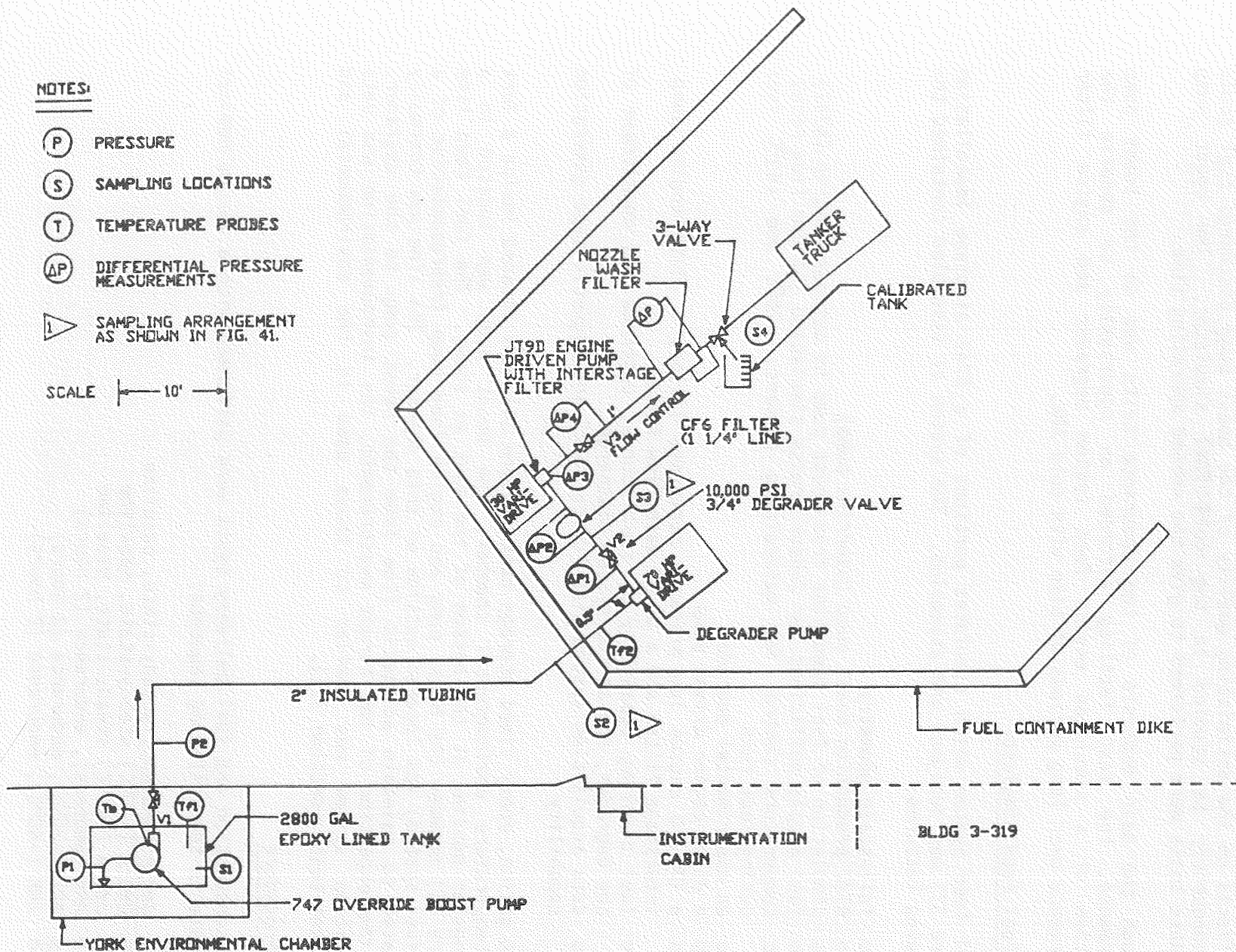
FIGURE 33. BOOST PUMP ENDURANCE TEST SETUP
