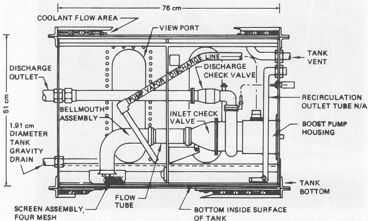
FIGURE 2. INTERIOR OF COLD FUEL SIMULATOR TANK
