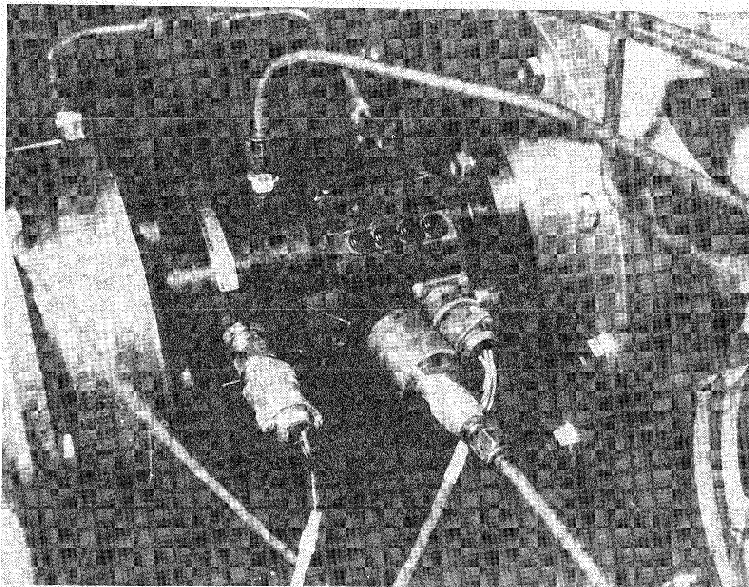
FIGURE 40. TYPICAL TORQUE METER INSTALLATION FOR DEGRADER PUMP AND ENGINE DRIVEN PUMP
