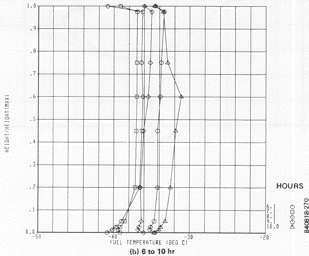
FIGURE 14. MEASURED TEMPERATURE PROFILES, JET A
