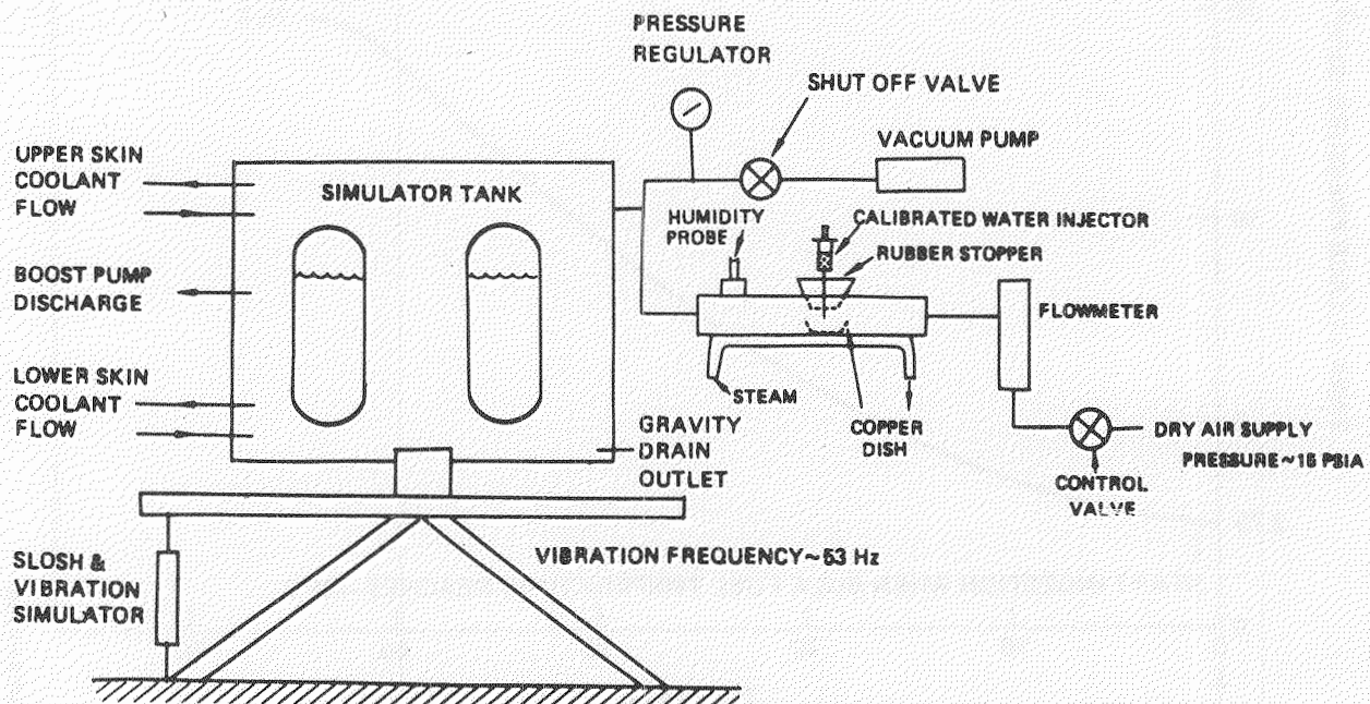
FIGURE 20. WATER VAPOR INGESTION TEST SETUP
