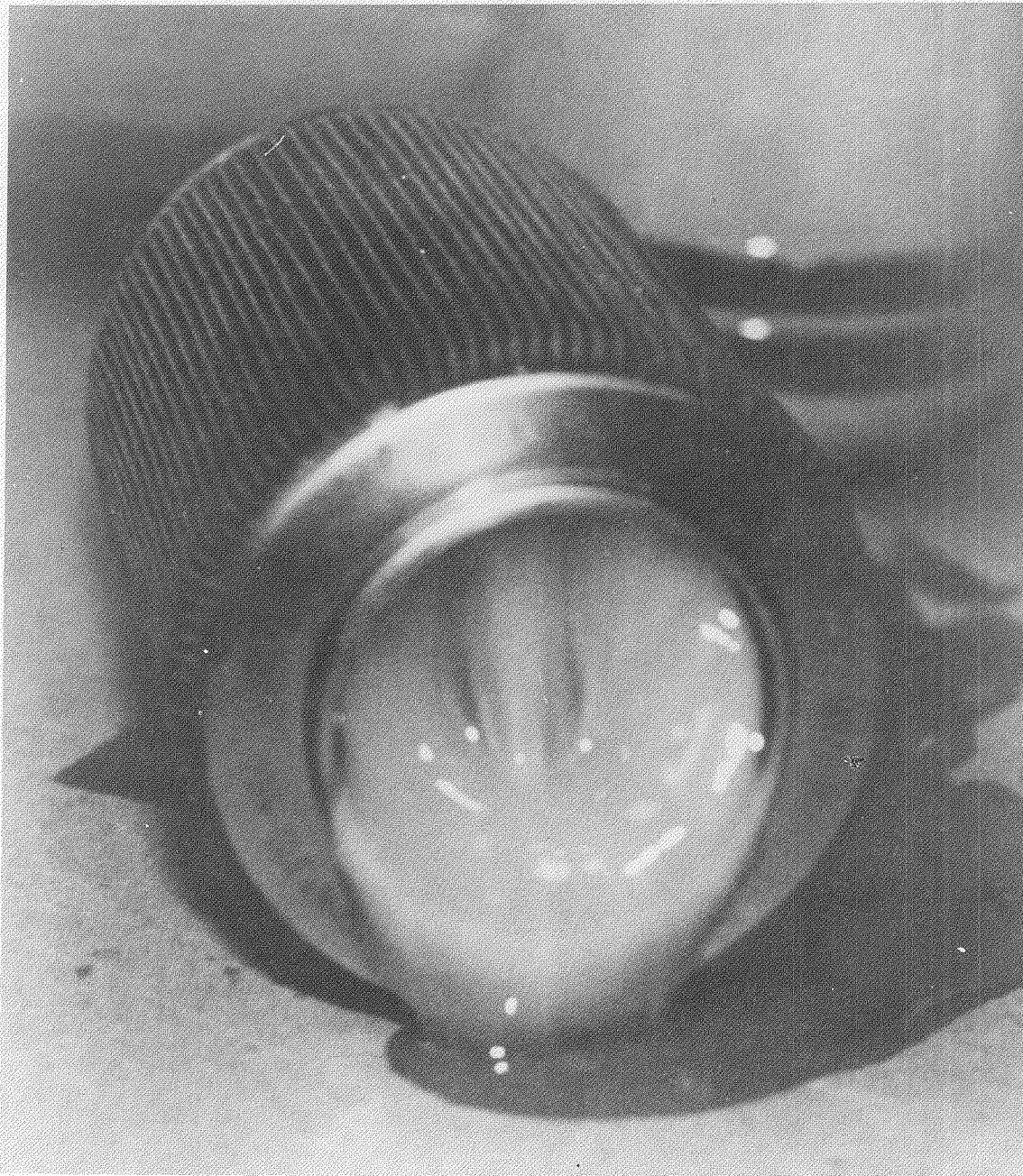
FIGURE 44. JT9D ENGINE DRIVEN PUMP, INTERSTAGE FILTER FOLLOWING -40°C AMK ENDURANCE TEST
