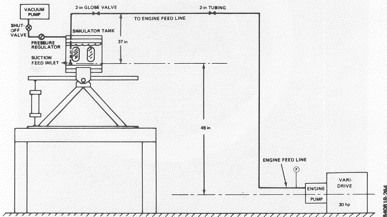
FIGURE 26. TEST CONFIGURATION FOR SUCTION FEED PERFORMANCE
