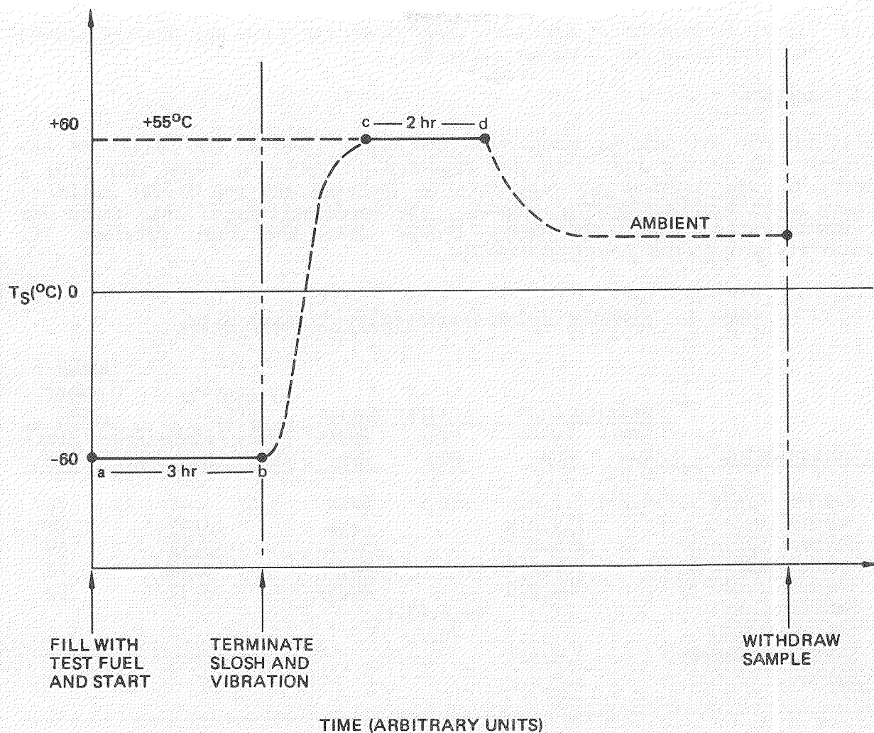
FIGURE 17. THERMAL CYCLE PROFILE USED IN ENVIRONMENTAL TESTS
