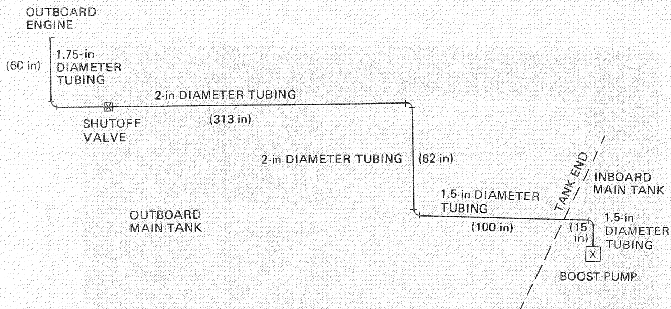
FIGURE 35. SIMULATED 747 BOOST PUMP LINE TO ENGINE
