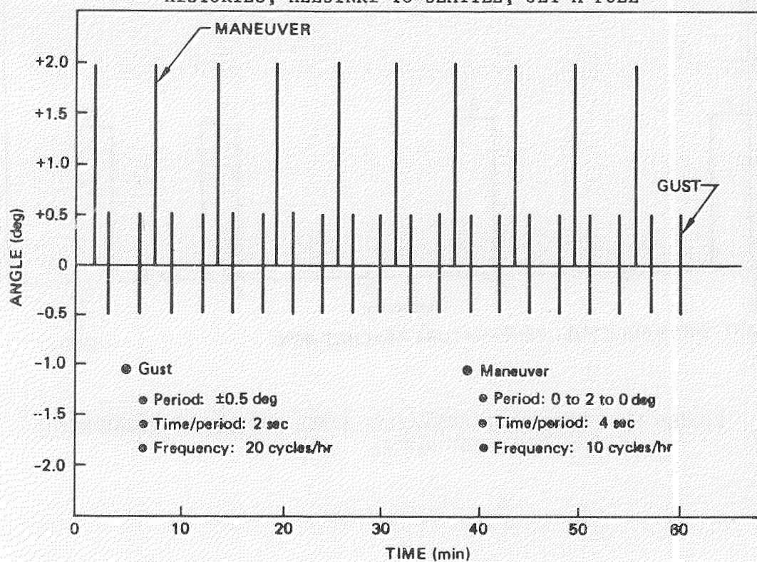
FIGURE 10. SIMULATED GUST AND MANEUVER CYCLES
