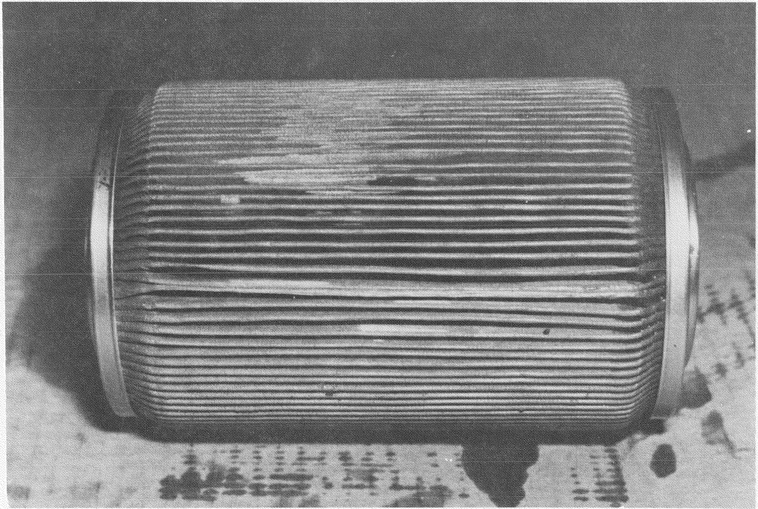
FIGURE 41. CF6 -50 LOW PRESSURE CARTRIDGE FILTER
