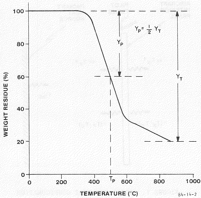
FIGURE 2. TYPICAL THERMOGRAM
