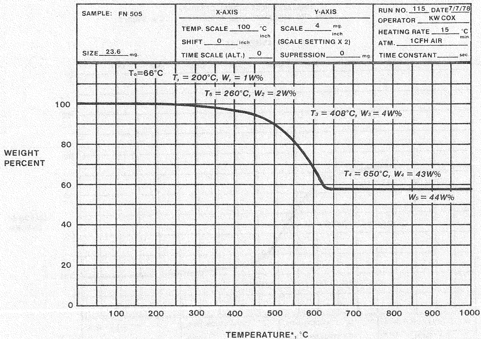
FIGURE B-4. THERMOGRAM F505 (NARMCO 8250) PHENOLIC (TAKEN FROM REFERENCE 11)
