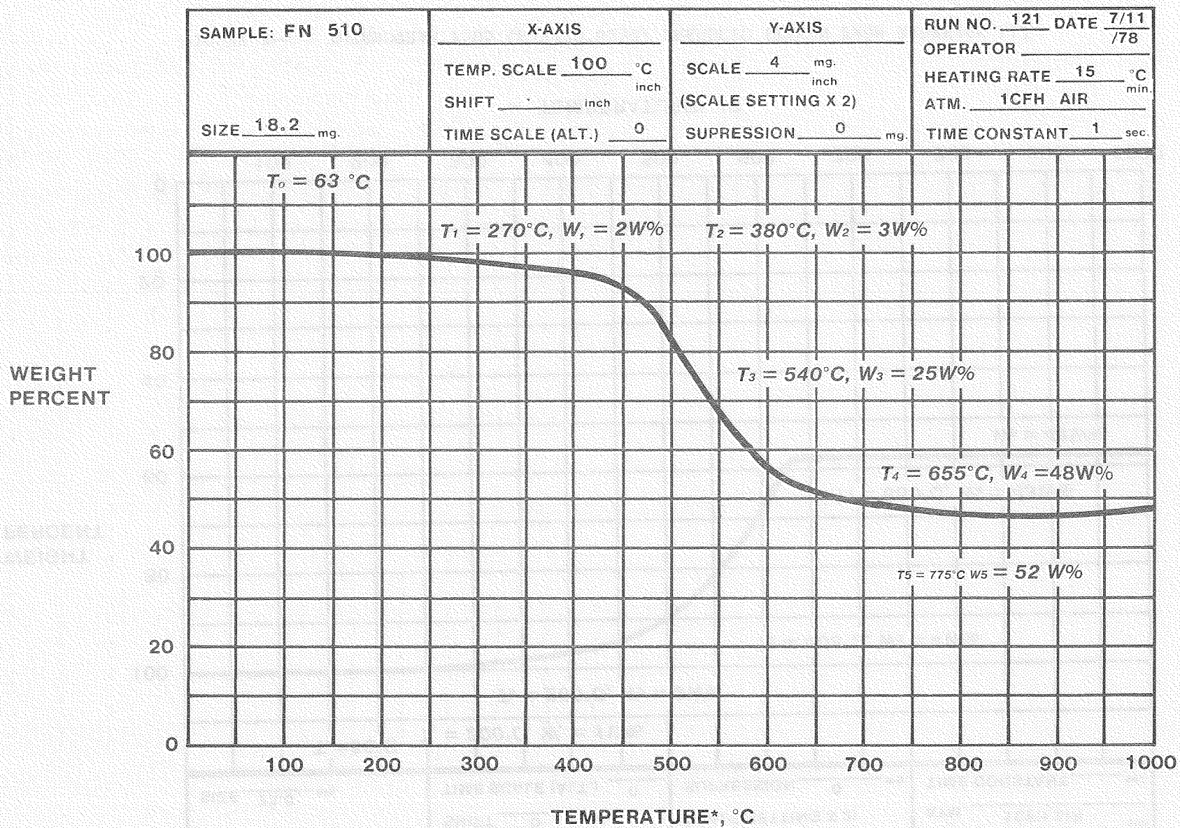
FIGURE B-5. THERMOGRAM F510 (FIBERITE MXT 6032) PHENOLIC (TAKEN FROM REFERENCE 11)
