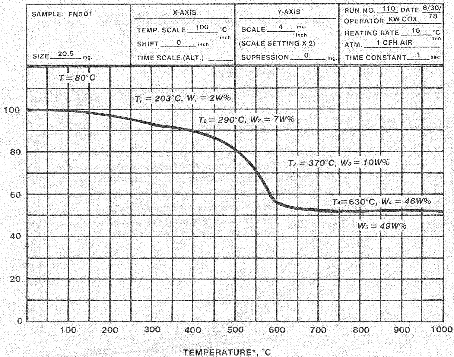
FIGURE B-3. THERMOGRAM F501 (CIBA GEIGY FIBERDUX 917) PHENOLIC (TAKEN FROM REFERENCE 11)
