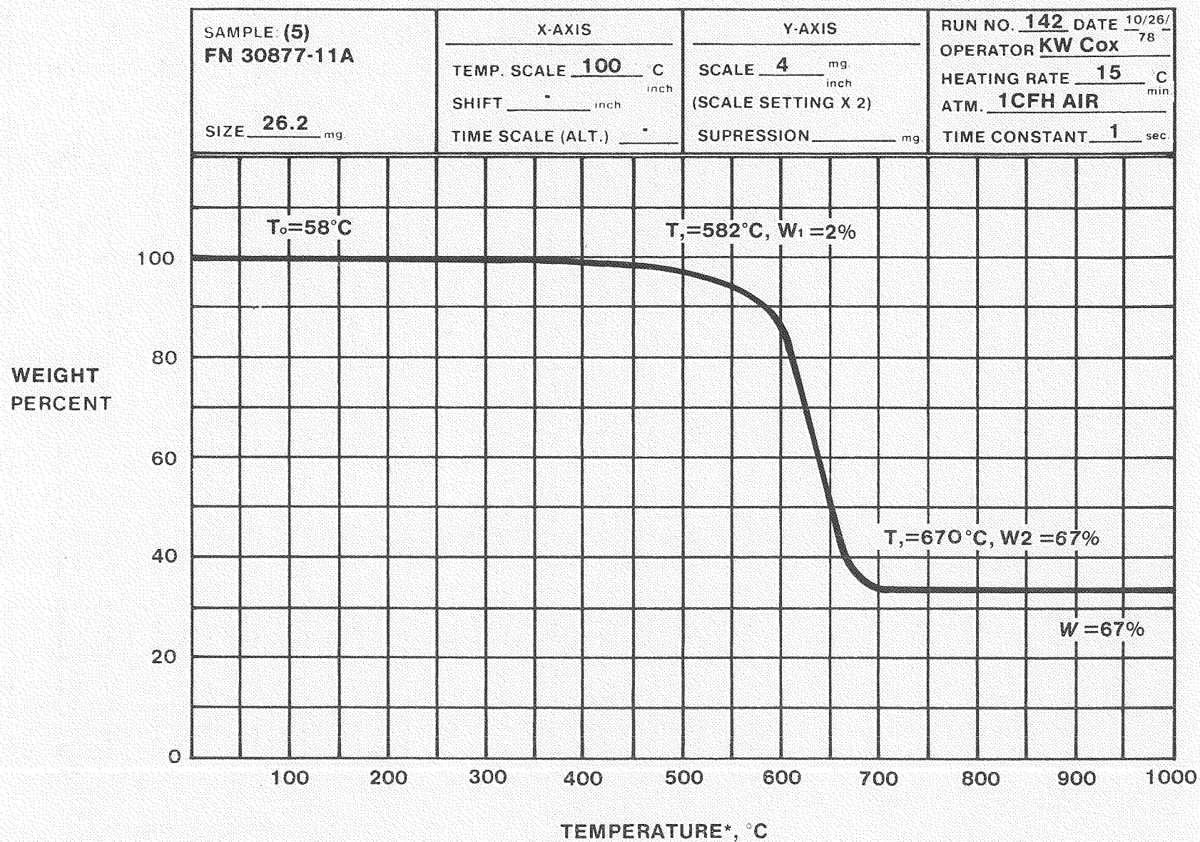
FIGURE B-6. THERMOGRAM FN308/7-11A (POLYIMIDE/GLASS) (TAKEN FROM REFERENCE 11)
