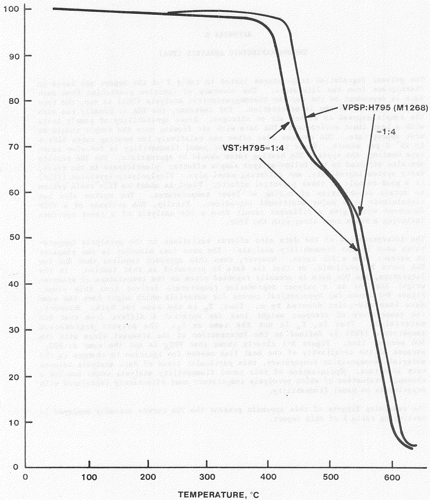
FIGURE B-1. TYPICAL THERMOGRAVIMETRIC ANALYSIS OF VINYLSTYRILPYRIDINE MODIFIED BISMALEIMIDE IN AIR (10°C/min) (TAKEN FROM REFERENCE 12)
