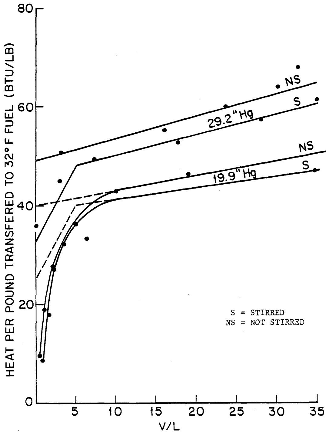
FIGURE 23. HEAT ADDED PER POUND OF FUEL VS VAPOR TO LIQUID RATIO FOR WET 100LL.
