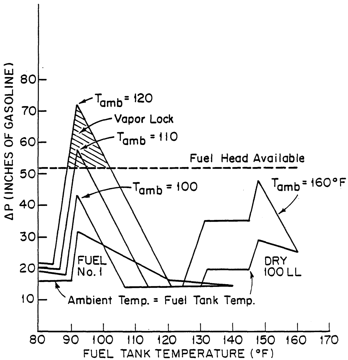
FIGURE 47. EFFECT OF AGITATION OF FUEL IN TANK.
