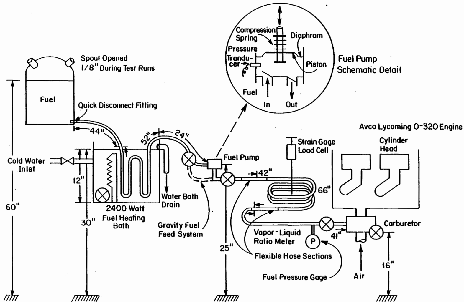
FIGURE 7. SCHEMATIC DIAGRAM OF TWO FUEL DELIVERY SYSTEMS.
