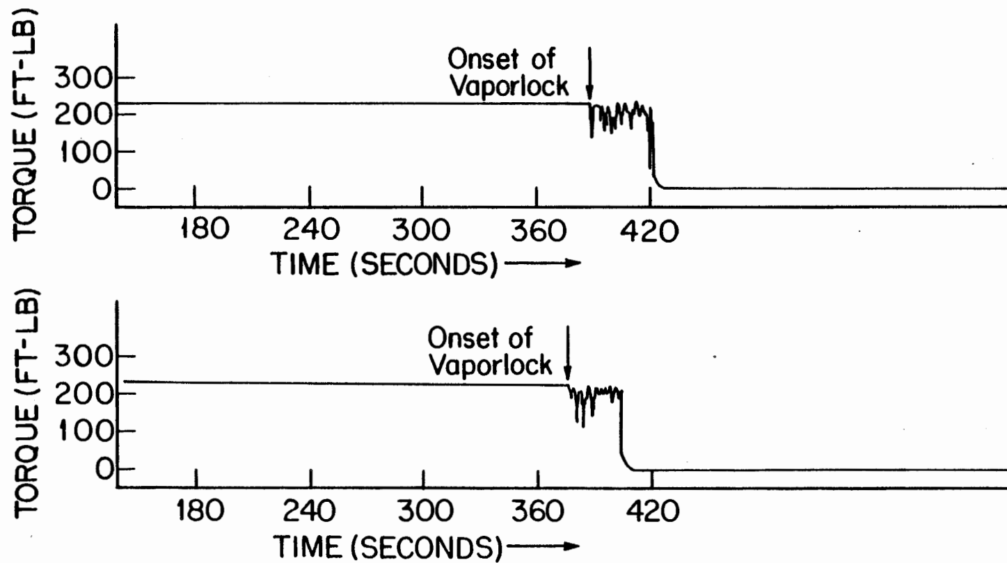
FIGURE 15. TORQUE VARIATION AS VAPOR LOCK DEVELOPS.
