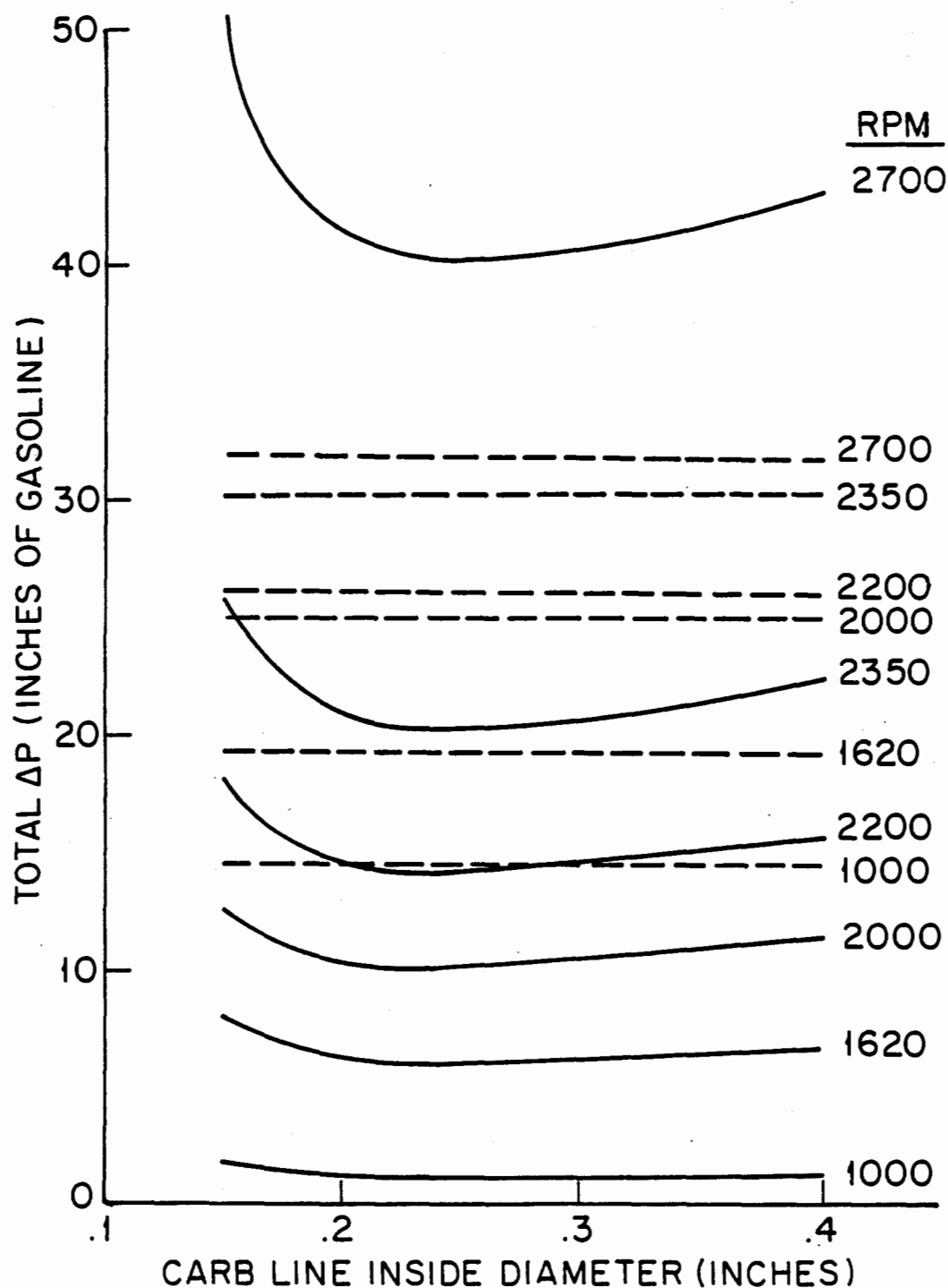
FIGURE 37. EFFECT OF CARBURETOR LINE INSIDE DIAMETER ON TOTAL SYSTEM PRESSURE DROP AND TOTAL PRESSURE HEAD AVAILABLE WITH INSULTATED STRAINER.
