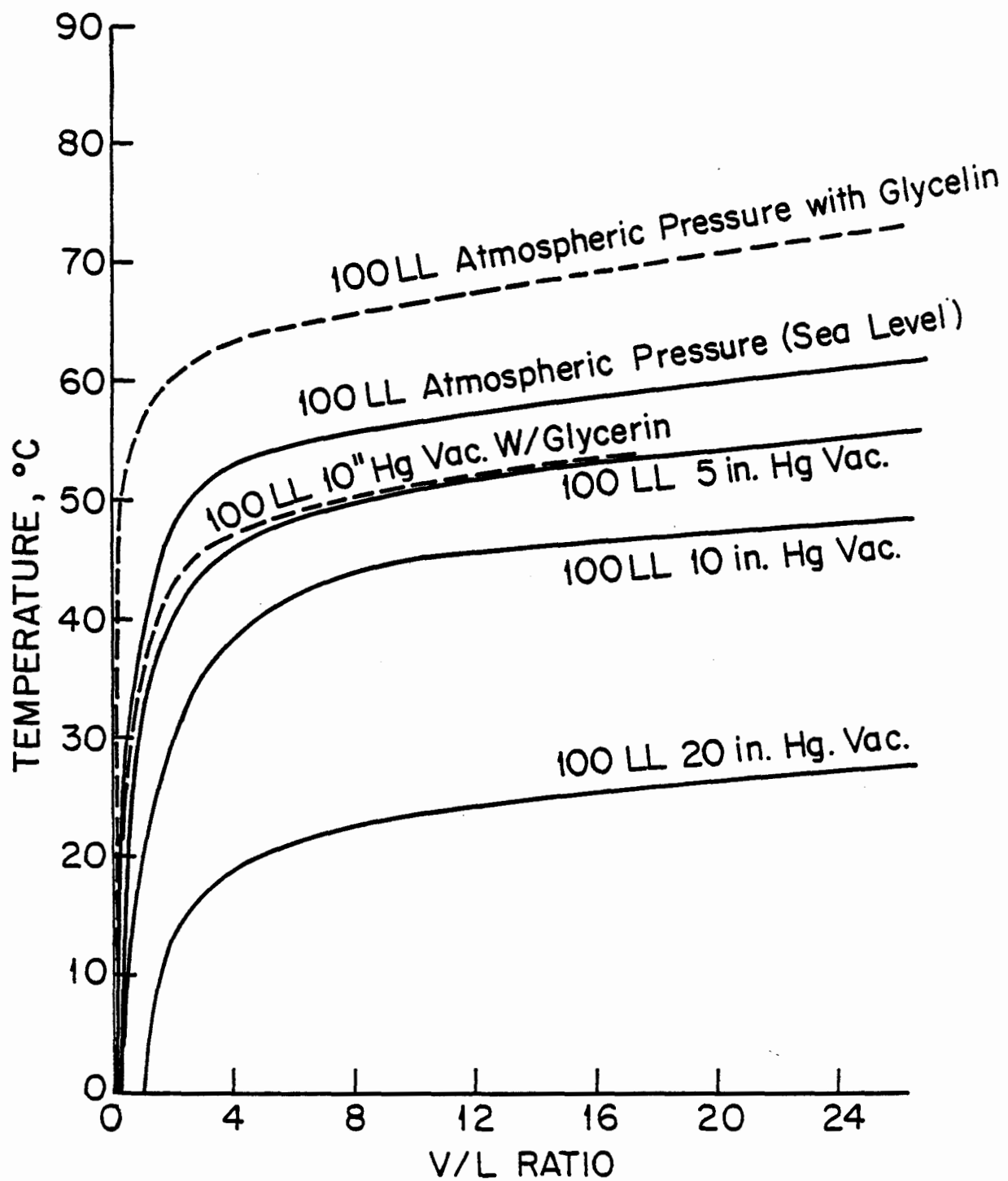
FIGURE 6. VAPOR-LIQUID RATIO AT ALTITUDE FOR 100LL FUEL WITH WATER
