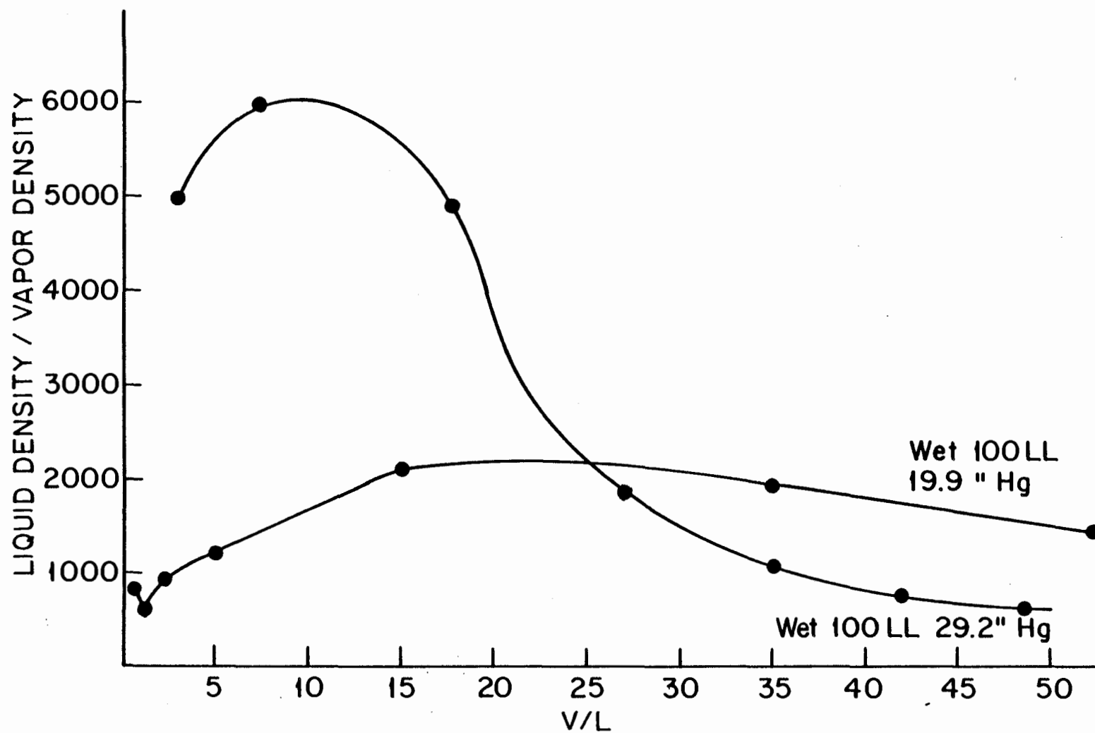
FIGURE 30. DENSITY RATIO BETWEEN LIQUID AND TOTAL VAPOR EVOLVED UP TO DIFFERENT VAPOR TO LIQUID RATIOS - wet 100LL
