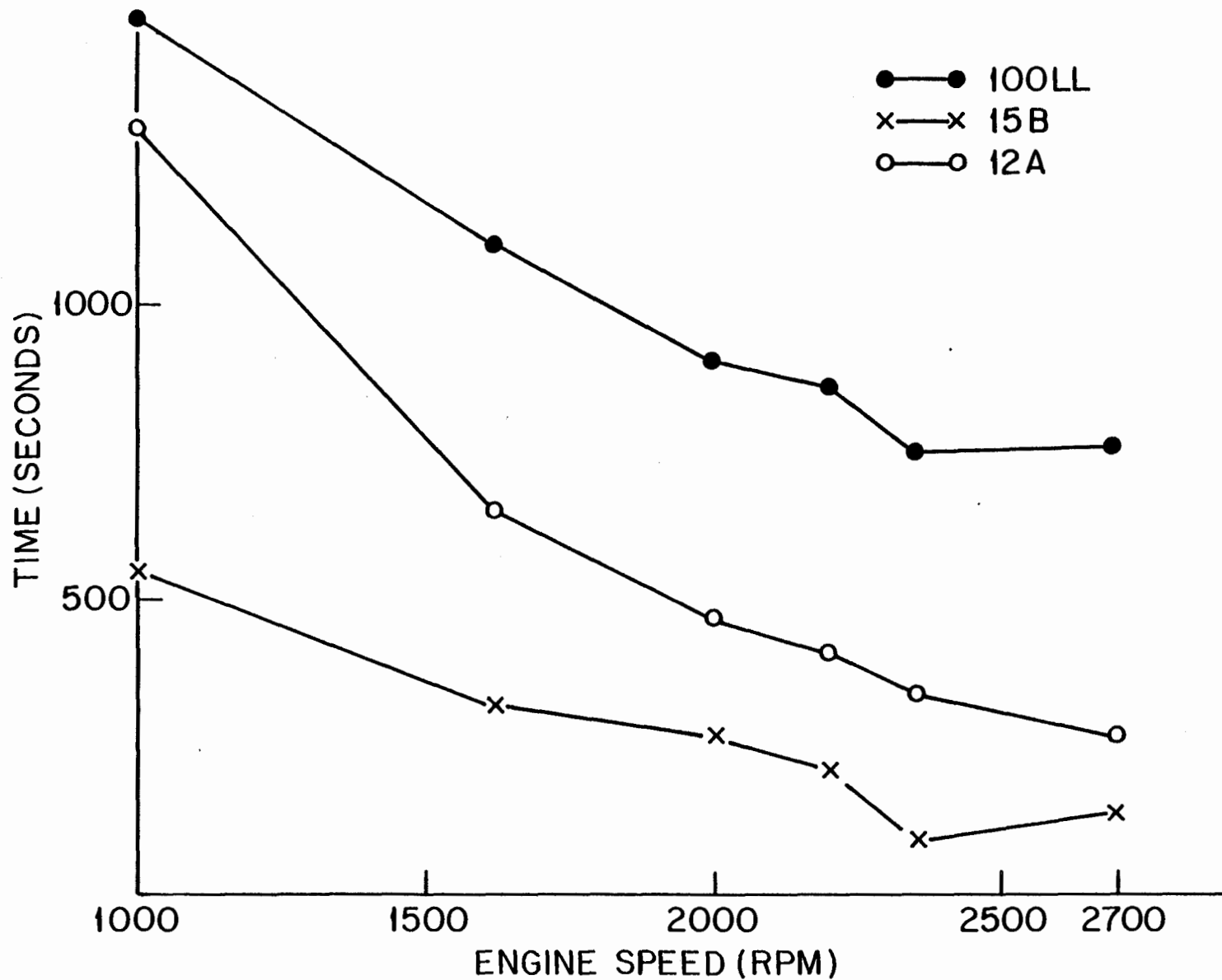
FIGURE 18. TIME FOR VAPOR LOCK (WITH FUEL PUMP)
