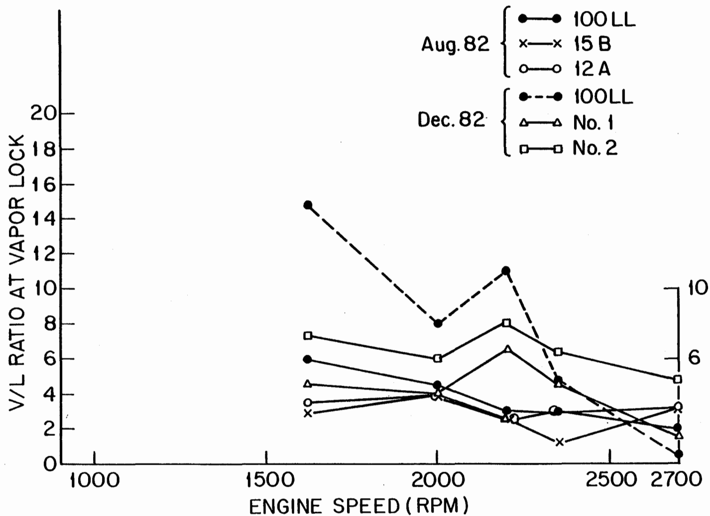
FIGURE 17. VAPOR TO LIQUID RATIO WHEN VAPOR LOCK OCCURS (GRAVITY FEED SYSTEM, NO PUMP).
