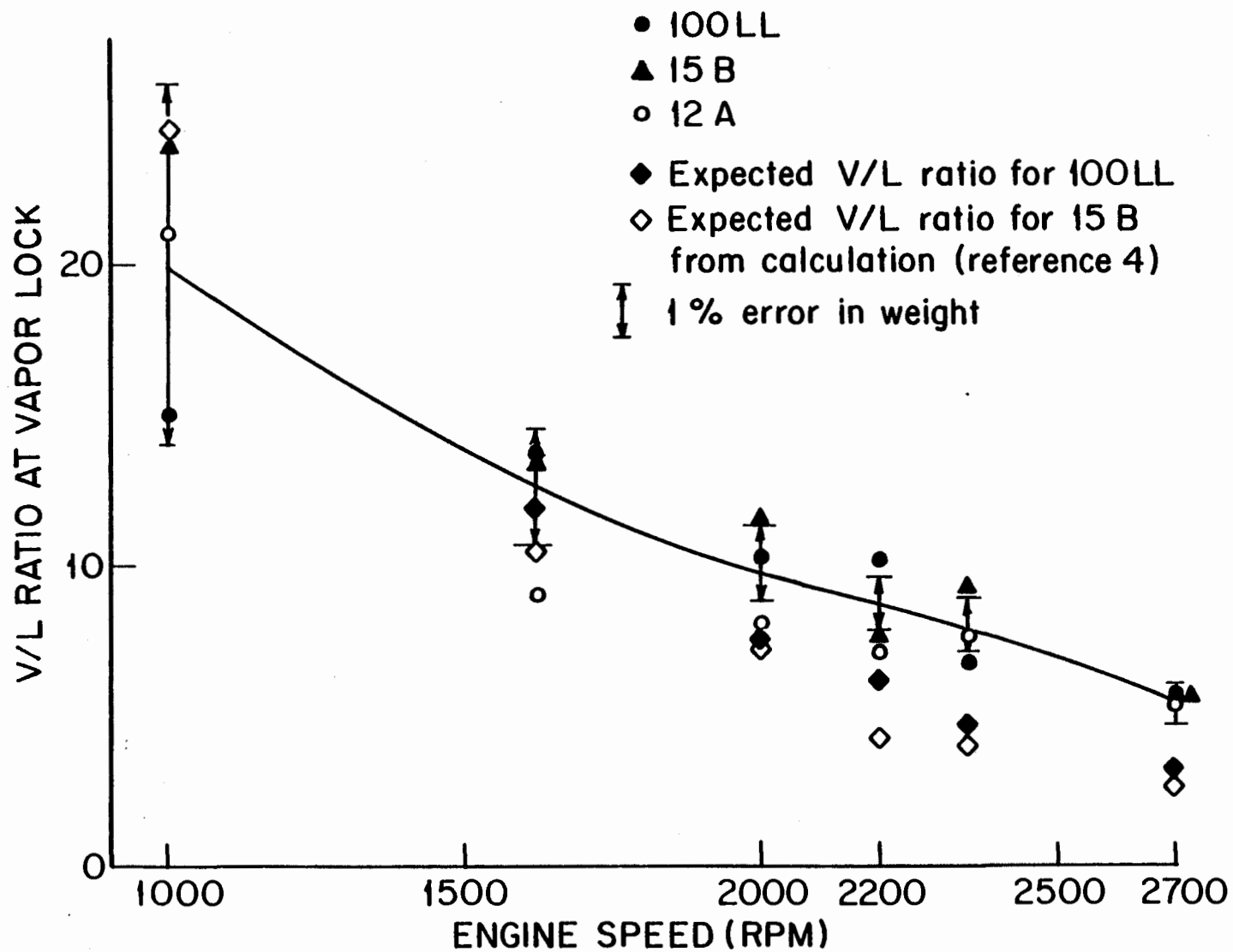
FIGURE 16. VAPOR TO LIQUID RATIO WHEN VAPOR LOCK OCCURS (WITH FUEL PUMP)
