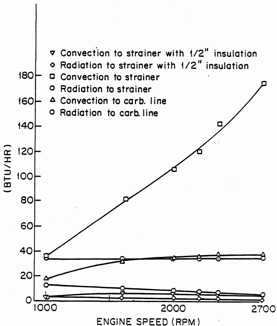
FIGURE 33. CALCULATED RADIANT AND CONVECTIVE HEAT TRANSFER TO STRAINER (BASELINE AND INSULATED) AND CARBURETOR LINE. Baseline strainer (2-1/4 x 3-1/4 uninsulated), .25 inch inside diameter carburetor line with .15 inch polymeric wall.
