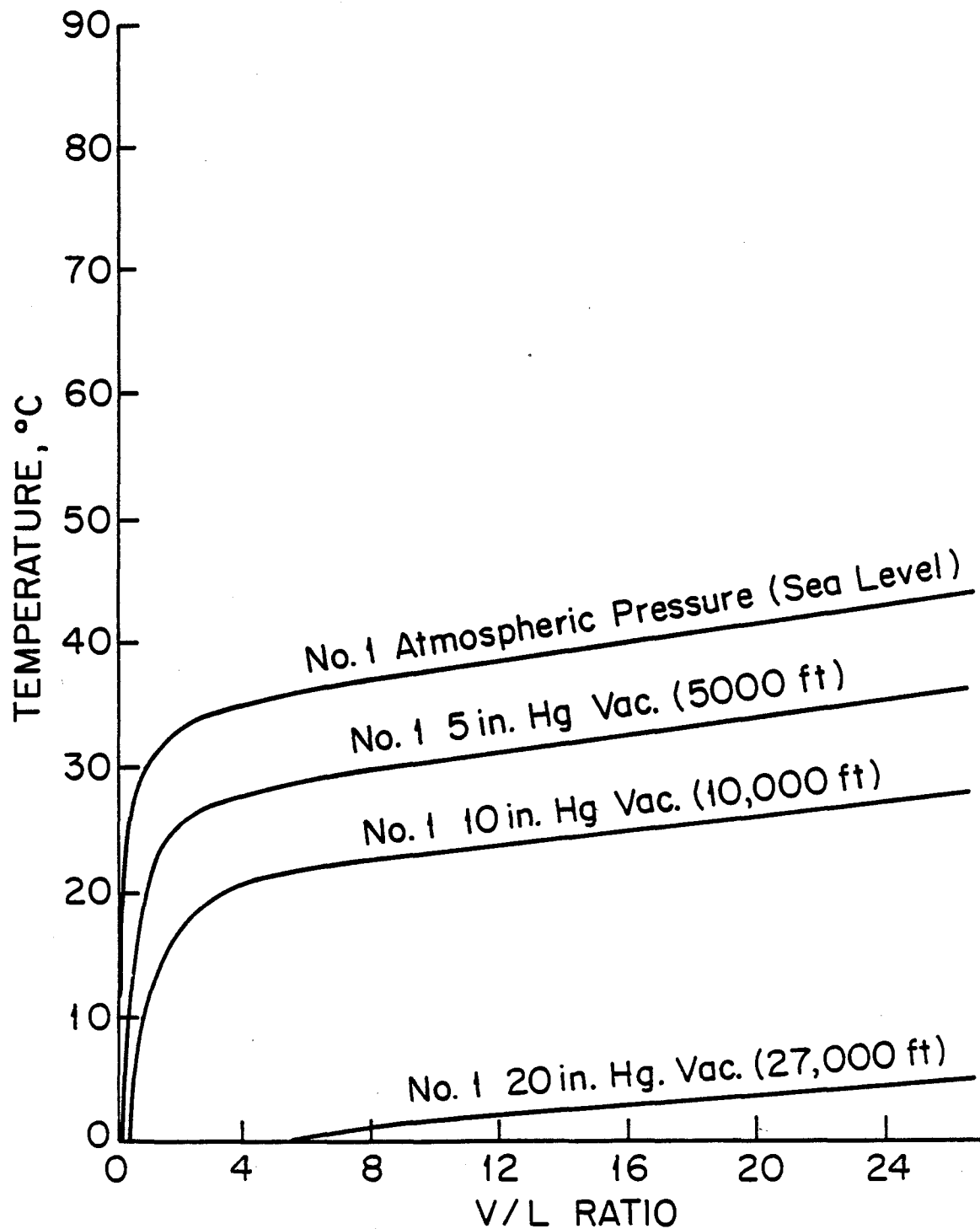
FIGURE 5. VAPOR-LIQUID RATIO AT ALTITUDE FOR NO. 1 FUEL.
