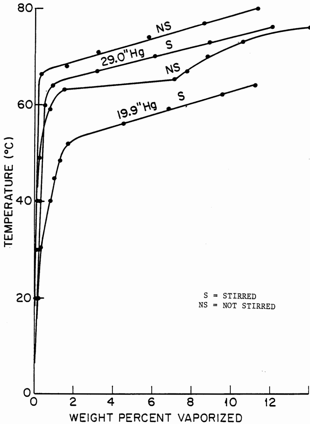
FIGURE 27. WEIGHT PERCENT VAPORIZED VS TEMPERATURE FOR DRY 100 LL.
