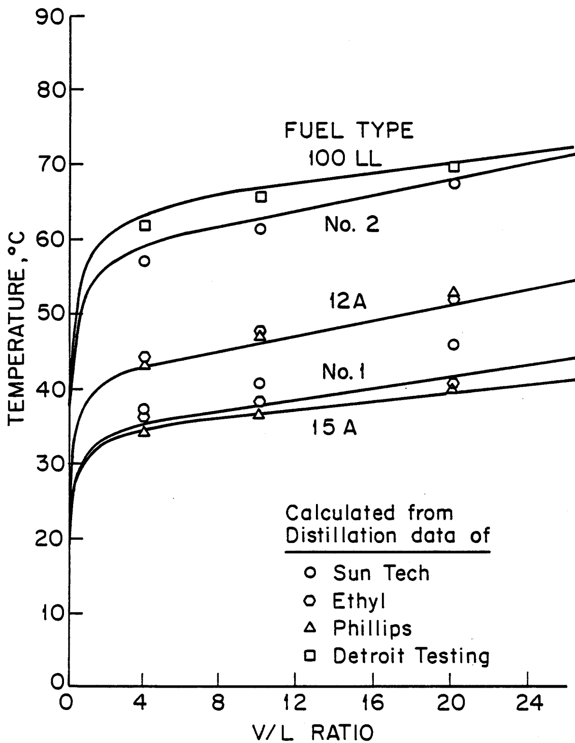
FIGURE 3. VAPOR-LIQUID RATIOS AT DIFFERENT TEMPERATURES. SOLID LINES ARE EXPERIMENTAL. POINTS ARE CALCULATED.
