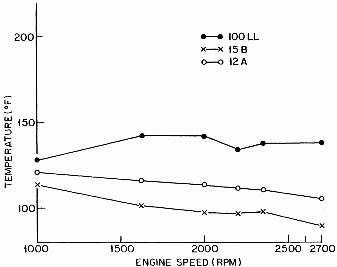
FIGURE 20. FUEL TEMPERATURE (BEFORE CARBURETOR INLET) WHEN VAPOR LOCK OCCURS WITH FUEL PUMP.
