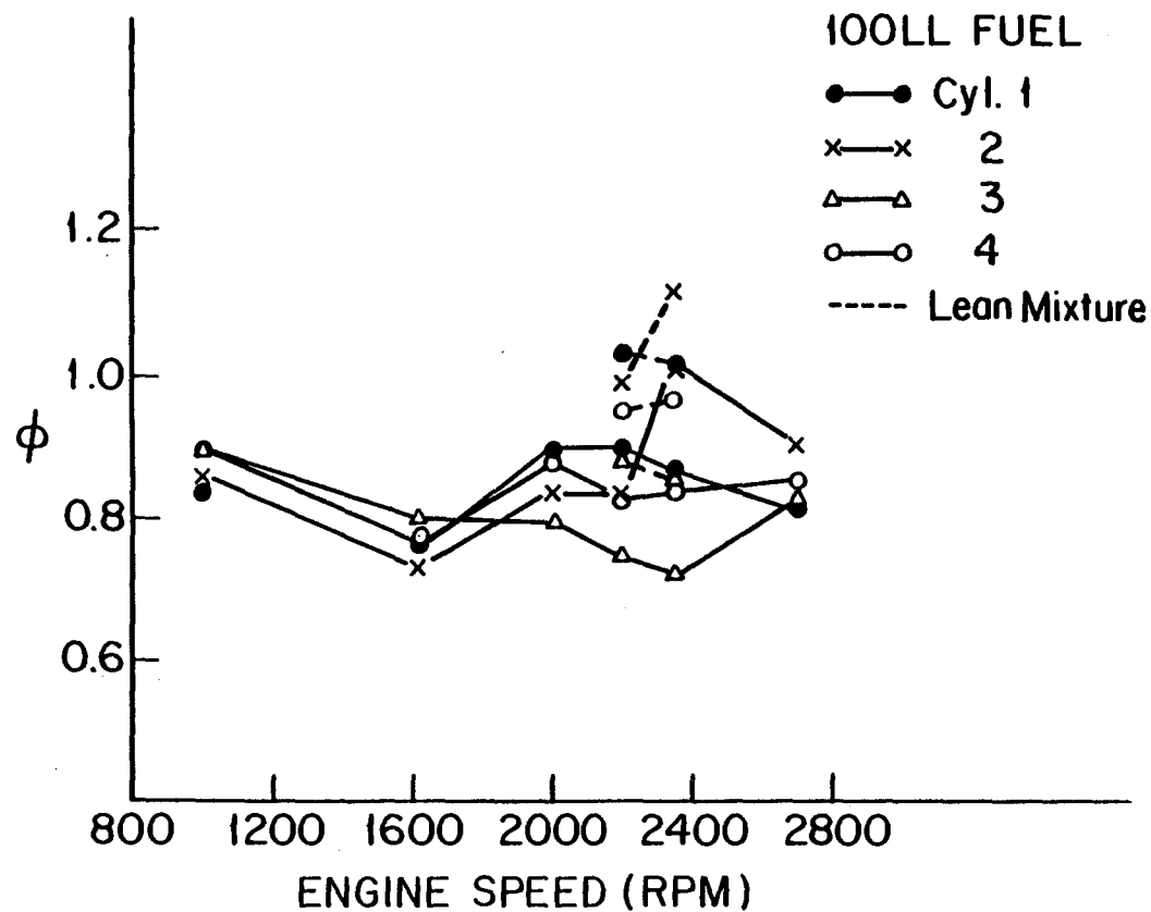
FIGURE 11. EQUIVALENCE RATIO DISTRIBUTION WITH 100 LL FUEL.
