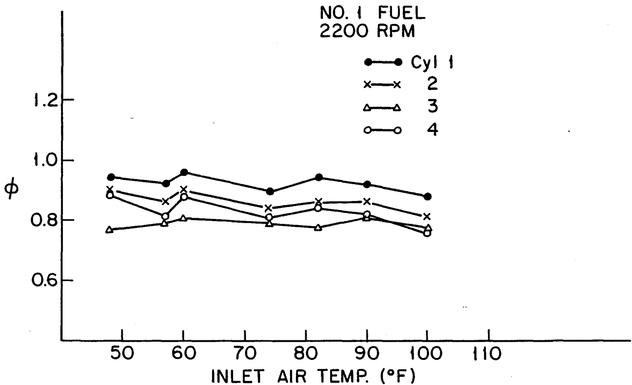
FIGURE 13. INLET AIR TEMPERATURE EFFECT ON MIXTURE DISTRIBUTION.
