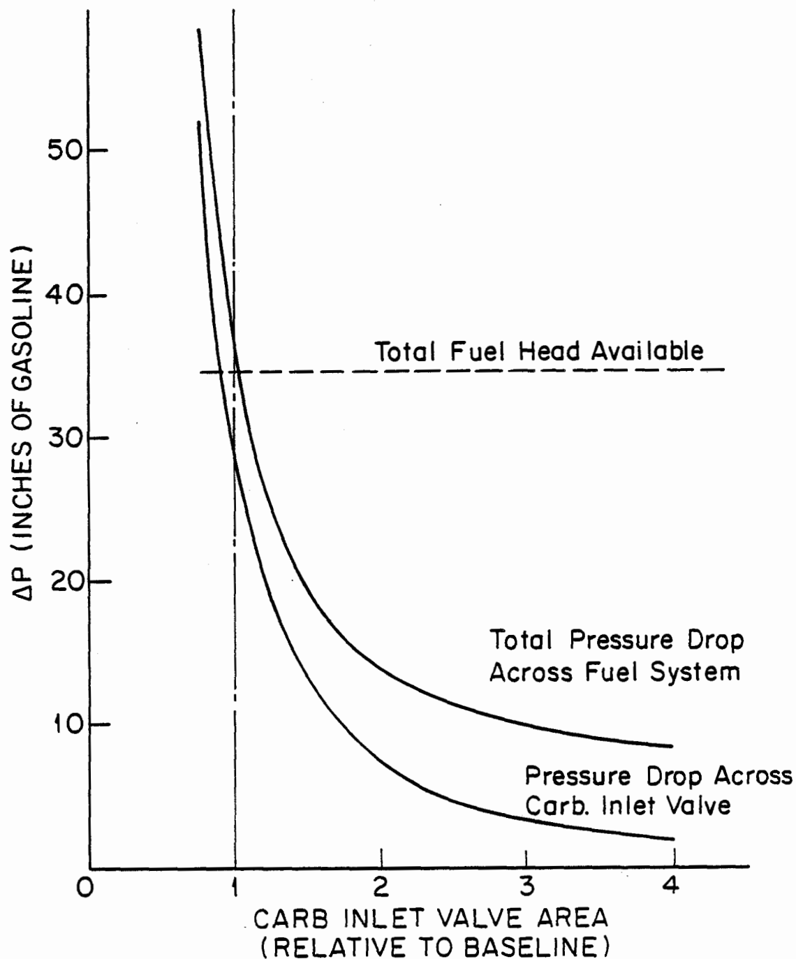
FIGURE 43. EFFECT OF CARBURETOR INLET VALVE AREA ON PRESSURE DROP. Uninsulated strainer, baseline conditions, fuel no. 1, no agitation, fuel temperature = ambient temperature = 85°F (2700 rpm at critical fuel temperature).
