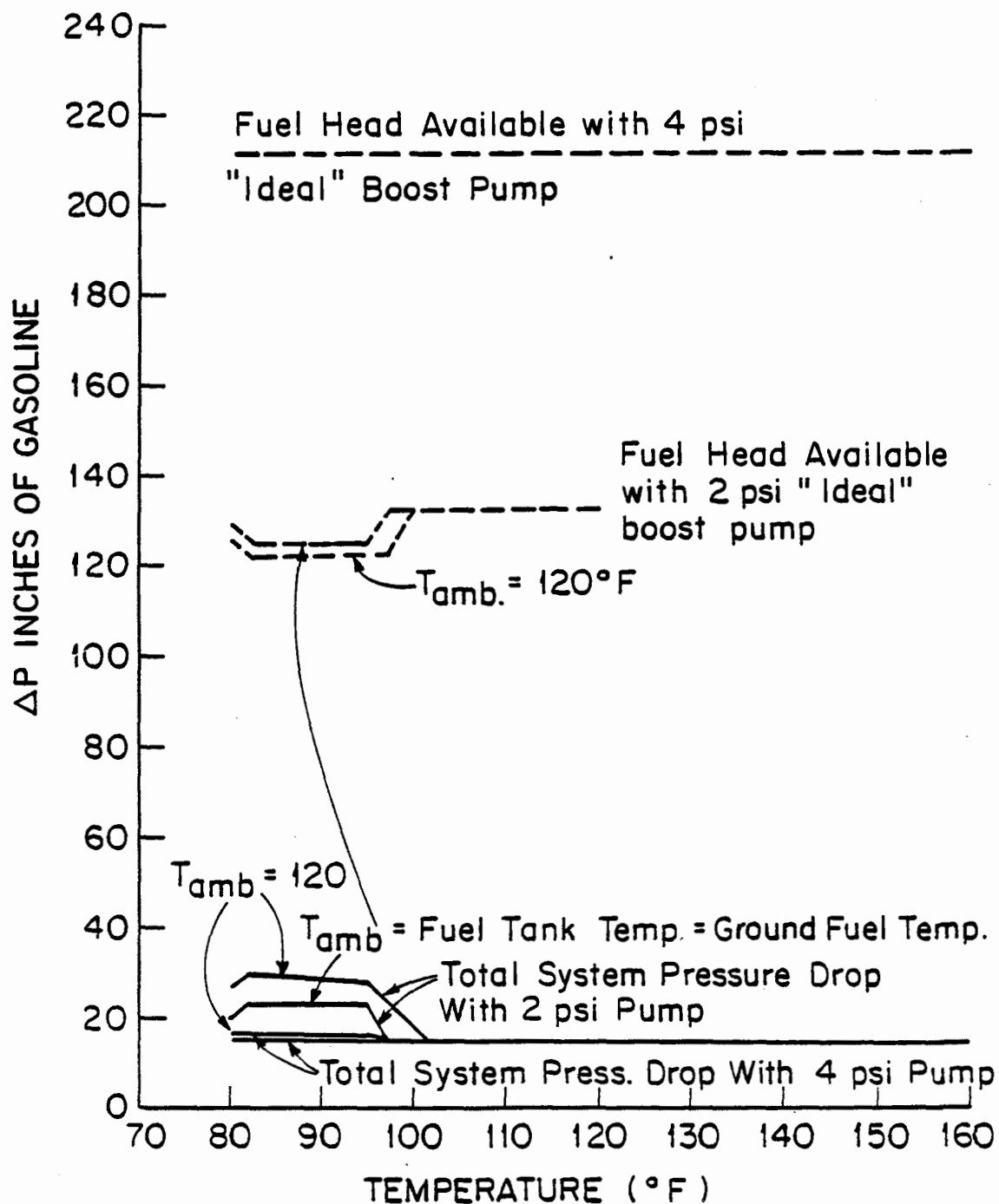
FIGURE 49. EFFECTIVENESS OF "IDEAL" BOOST PUMP.
