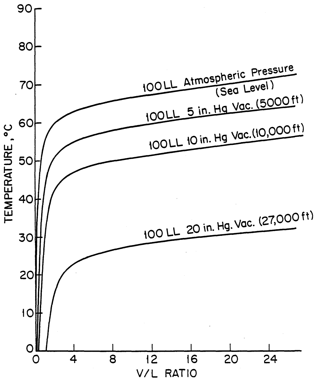
FIGURE 4. VAPOR-LIQUID RATIOS AT ALTITUDE FOR 100LL FUEL
