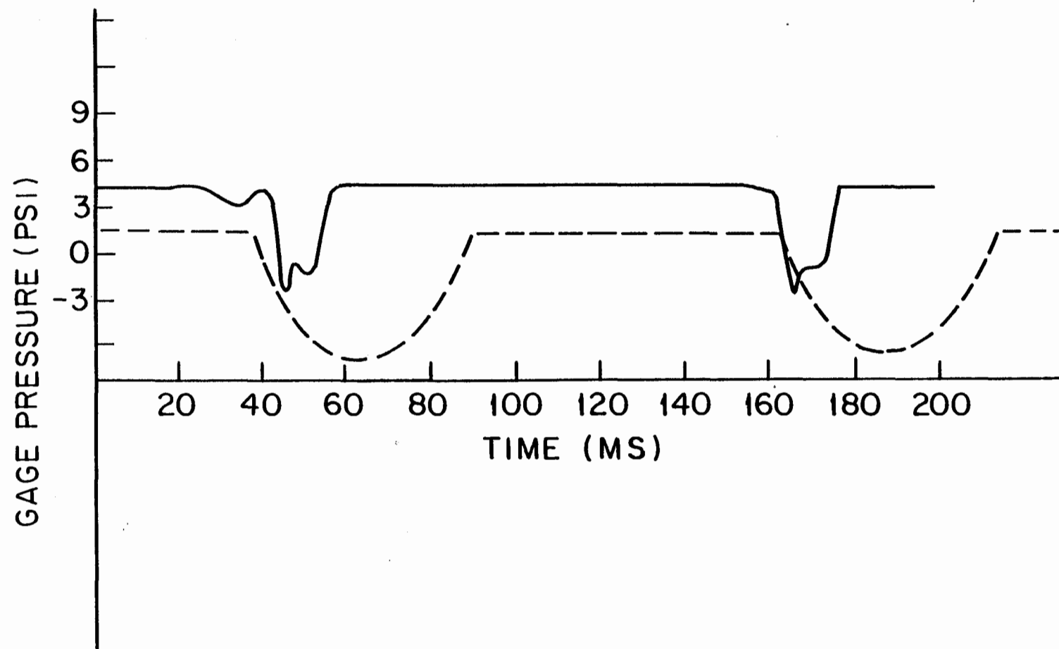
FIGURE 9. PRESSURE VARIATION INSIDE FUEL PUMP.
