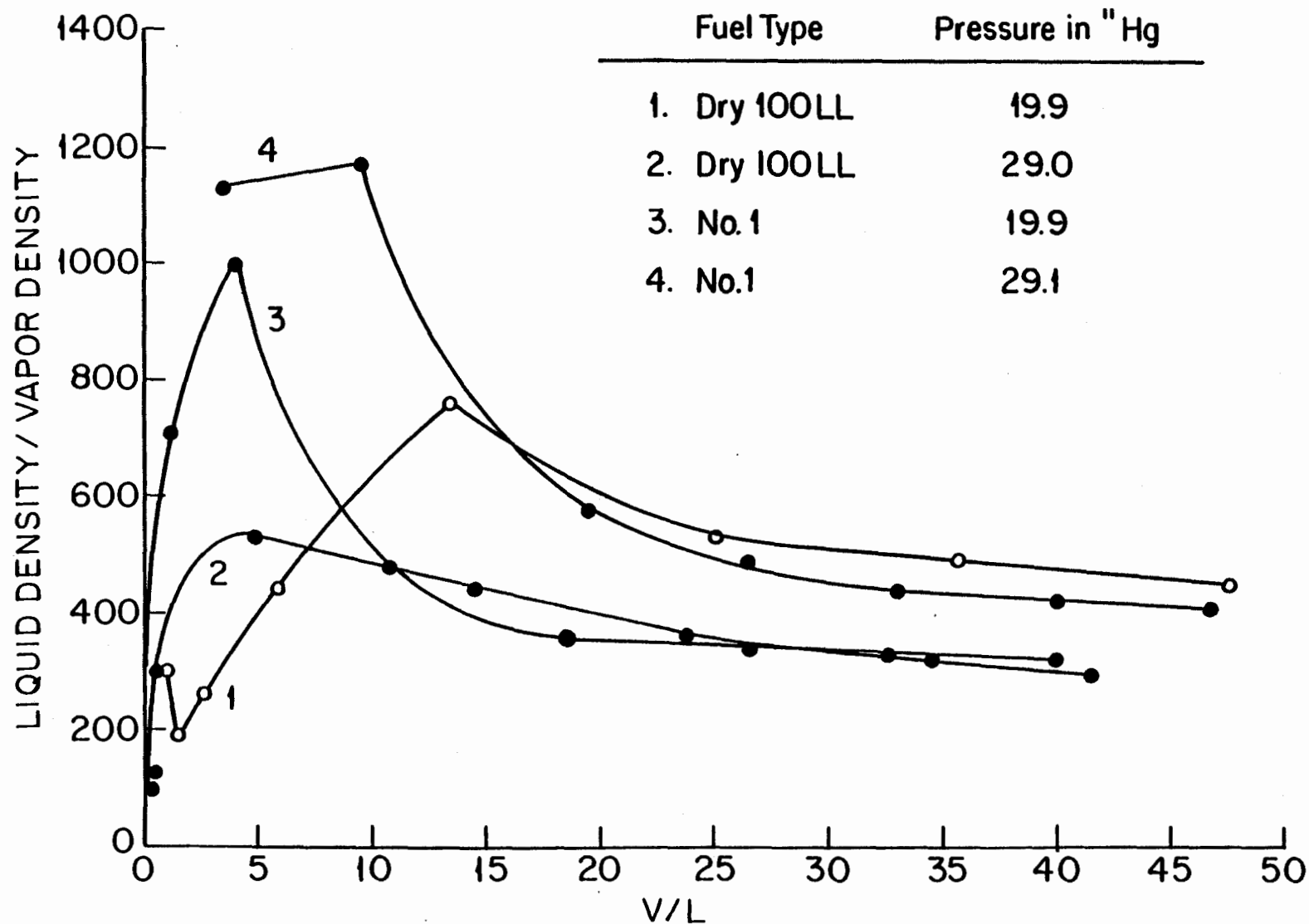
FIGURE 29. DENSITY RATIO BETWEEN LIQUID AND TOTAL VAPOR EVOLVED UP TO DIFFERENT VAPOR TO LIQUID RATIOS - No. 1 fuel and dry 100LL.
