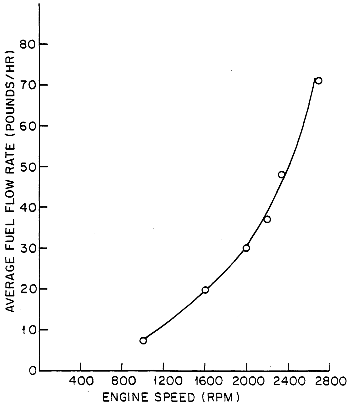
FIGURE 50. MEASURED FUEL CONSUMPTION RATE VS ENGINE SPEED
