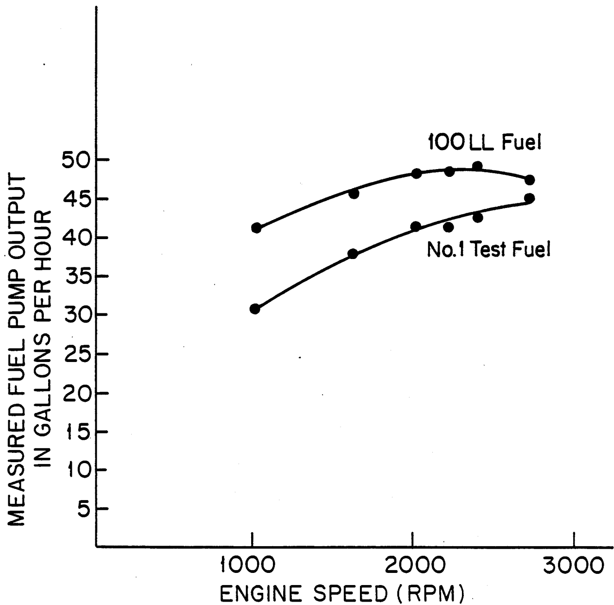
FIGURE 8. FUEL PUMP FLOW AT VARIOUS ENGINE SPEEDS.
