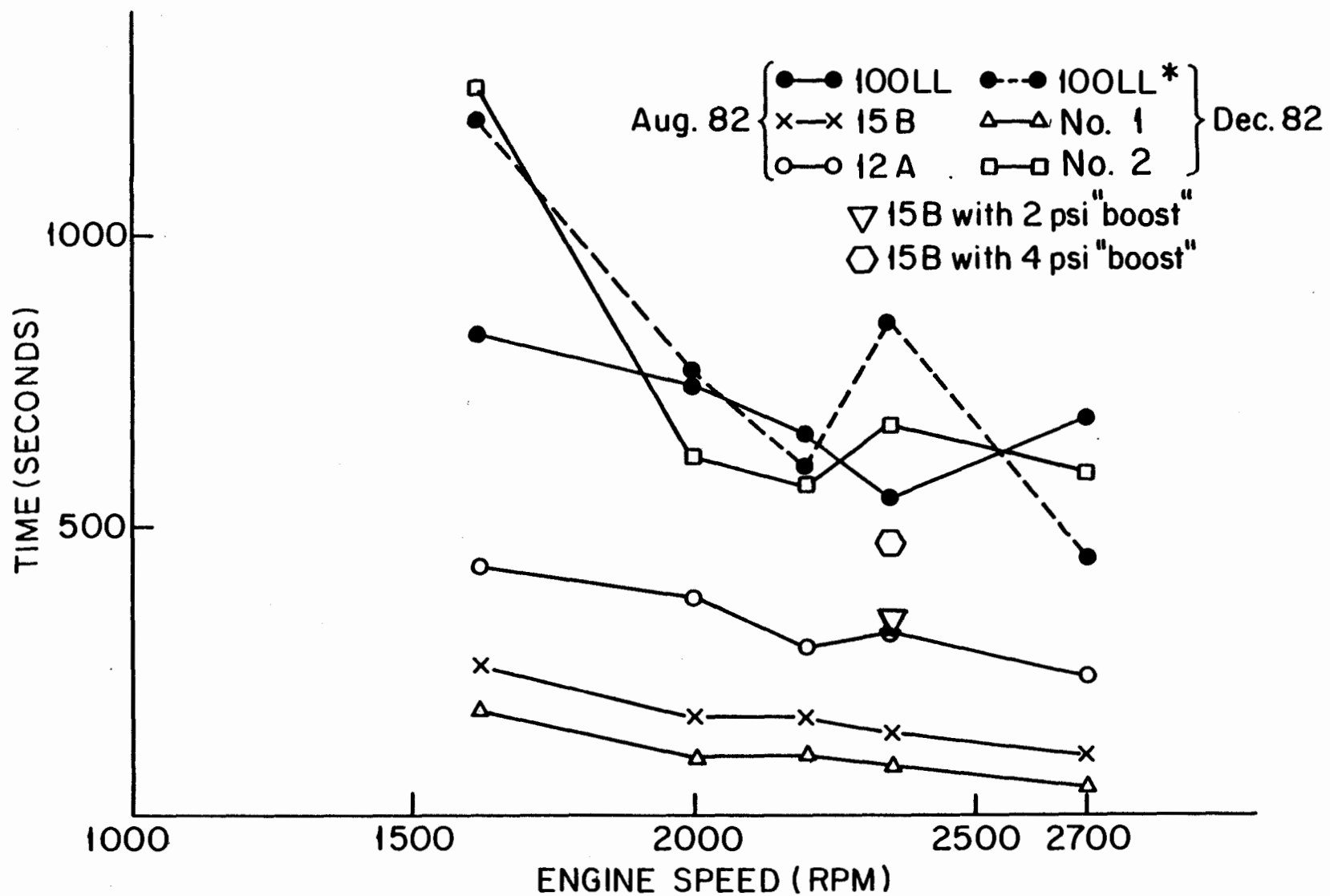
FIGURE 19. TIME FOR VAPOR LOCK (GRAVITY FEED SYSTEM, NO PUMP)
