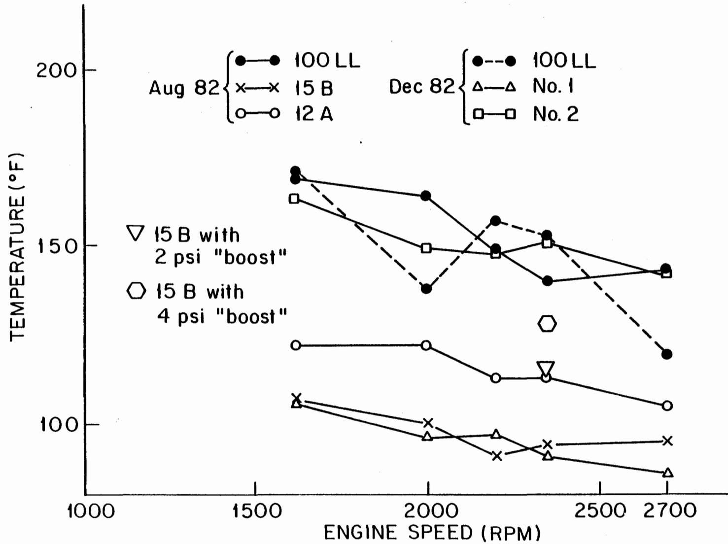
FIGURE 21. FUEL TEMPERATURE (BEFORE CARBURETOR INLET) WHEN VAPOR LOCK OCCURS, GRAVITY FEED SYSTEM, NO PUMP.
