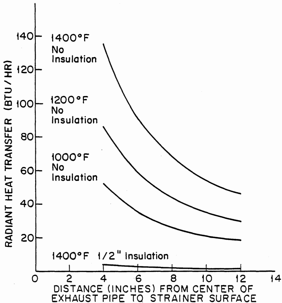
FIGURE 34. CALCULATED RADIANT HEAT TRANSFER TO STRAINER (BASELINE AND INSULATED) VERSUS DISTANCE FROM EXHAUST PIPE FOR VARIOUS SURFACE TEMPERATURES.
