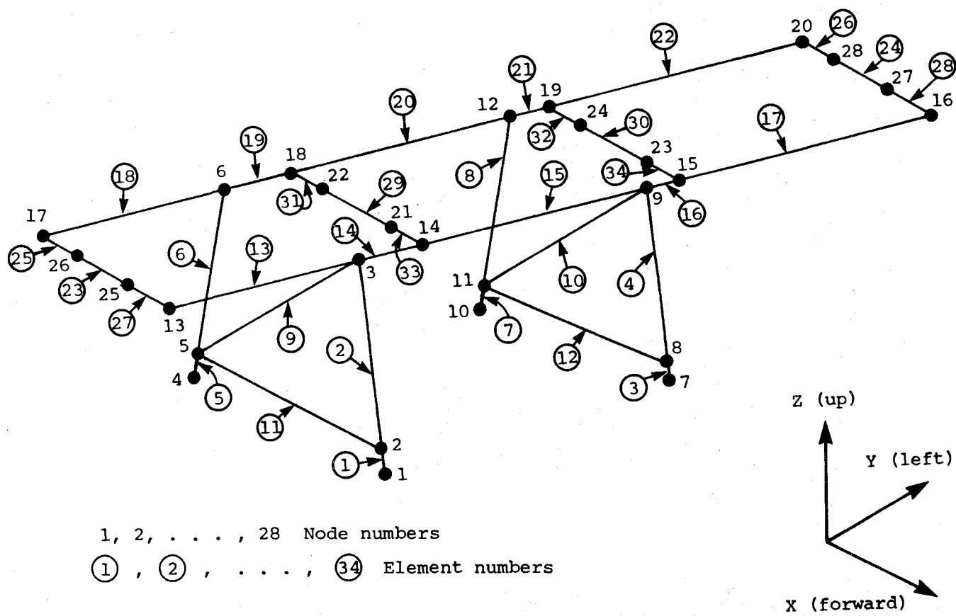
Figure B-1. Standard Weber seat NASTRAN model.
