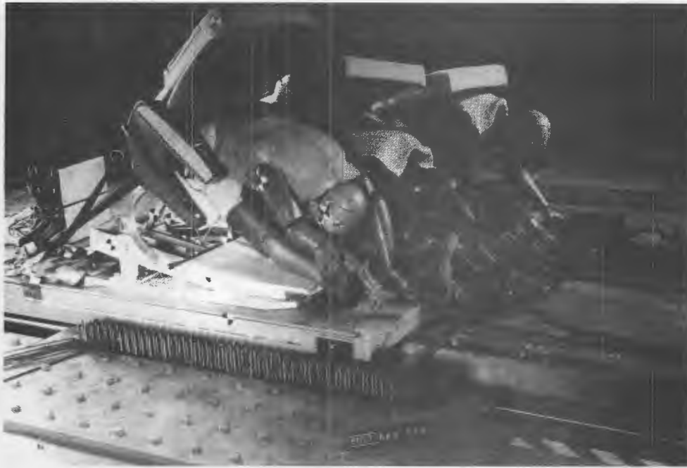
Figure 136. Posttest standard Weberlite seat (Dynamic Test).
