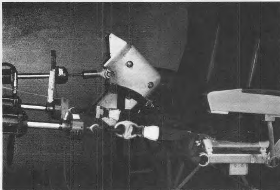
Figure 63. Weber MOD I seat aisle-side body block after stroking.
