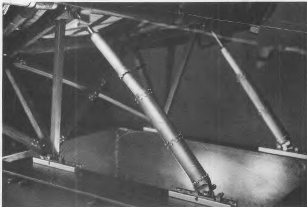
Figure 79. Location of energy absorber failure on the Weber MOD II seat (Forward Static Test).
