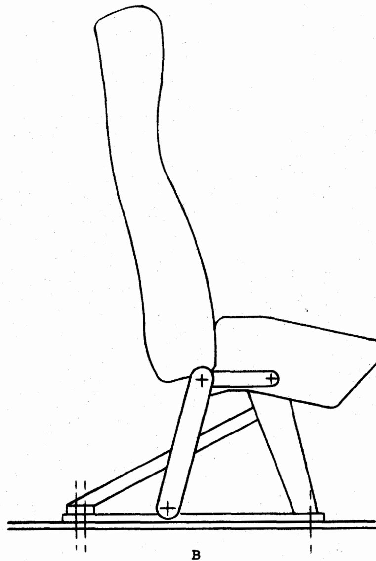
Figure 36. Telescoping seat pan arrangement.
