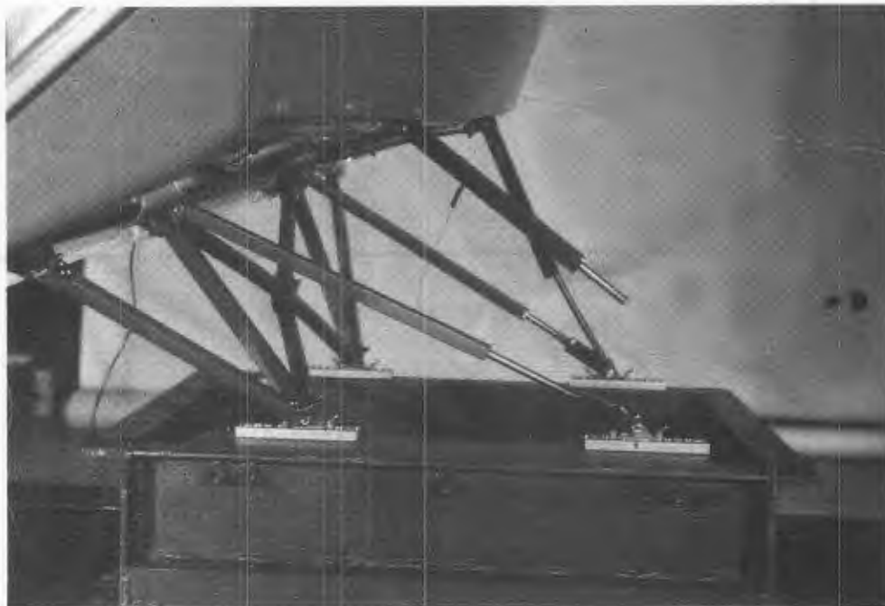
Figure 148. Posttest failed window-side leg energy absorber of Weberlite MOD seat (Forward Static Test).
