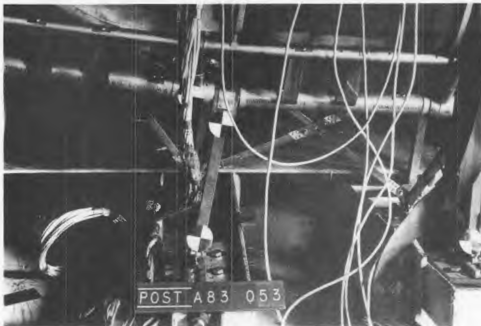
Figure 68. Posttest rear window-side leg and rear tube of Weber MOD I seat (Dynamic Test).
