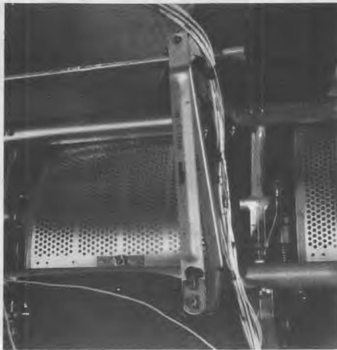
Figure 96. Failed window-side leg track fittings of standard UOP seat (Dynamic Test).
