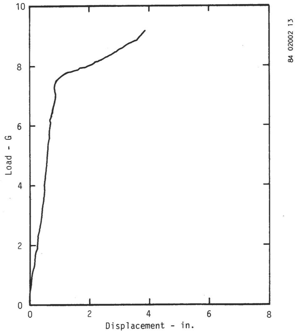
Figure 166. Load versus forward displacement of Weber aft-facing MOD seat.
