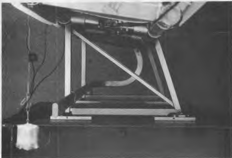
Figure 131. Standard Weberlite seat leg structure.
