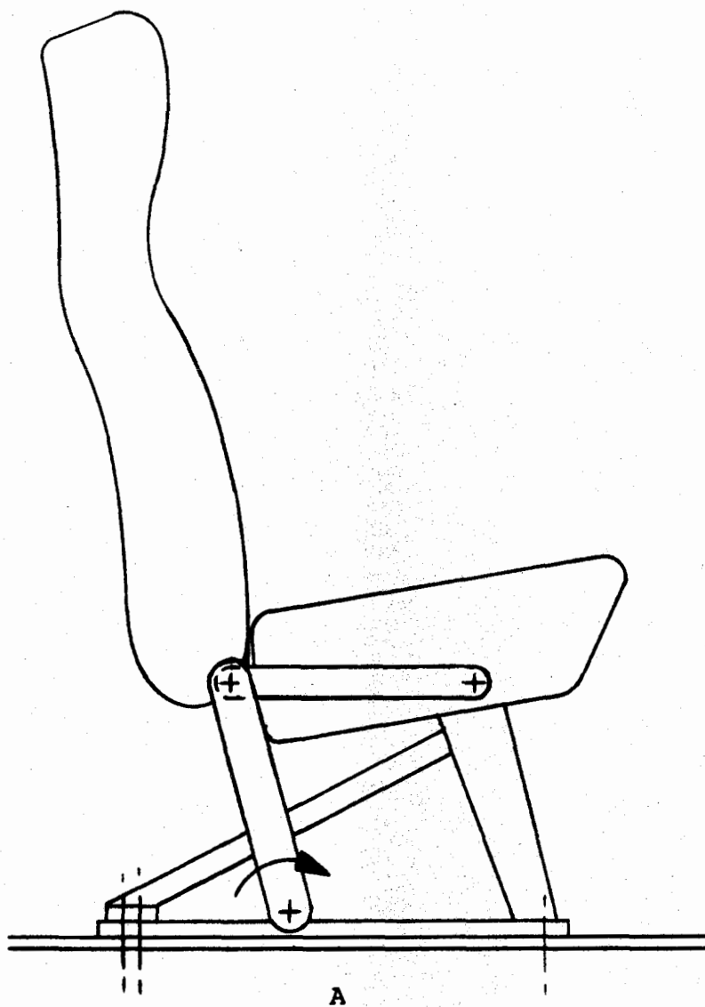
Figure 36. Telescoping seat pan arrangement.
