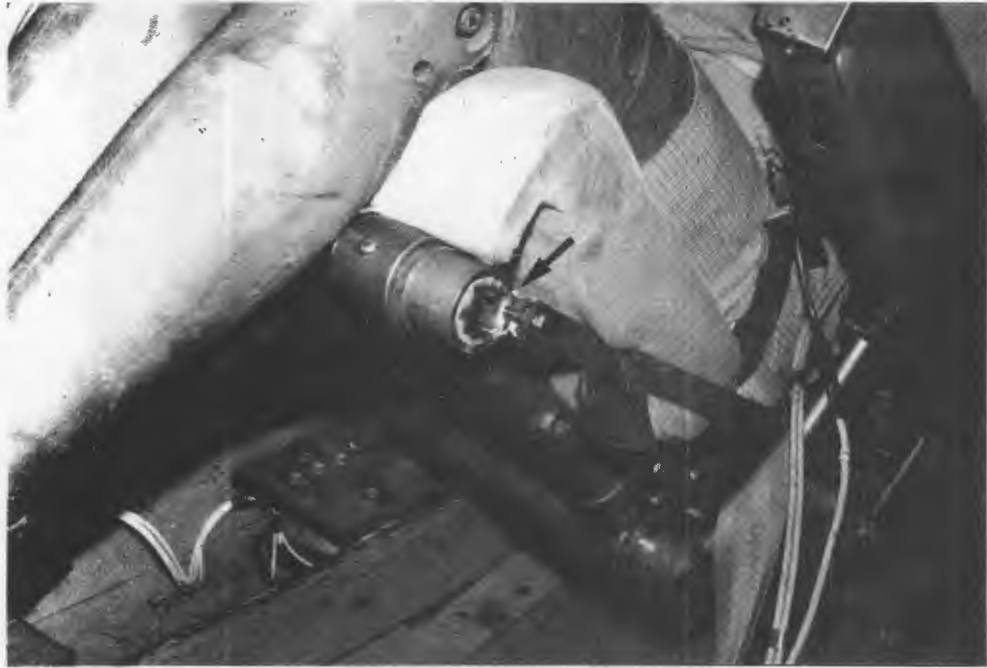
Figure 175. Attachment point of aisle-side strap to rear tube of Weber aft-facing MOD seat.
