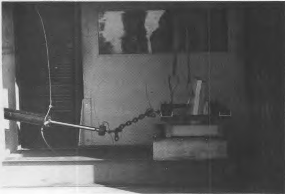
Figure 180. Downward test setup for the flight attendant seat.
