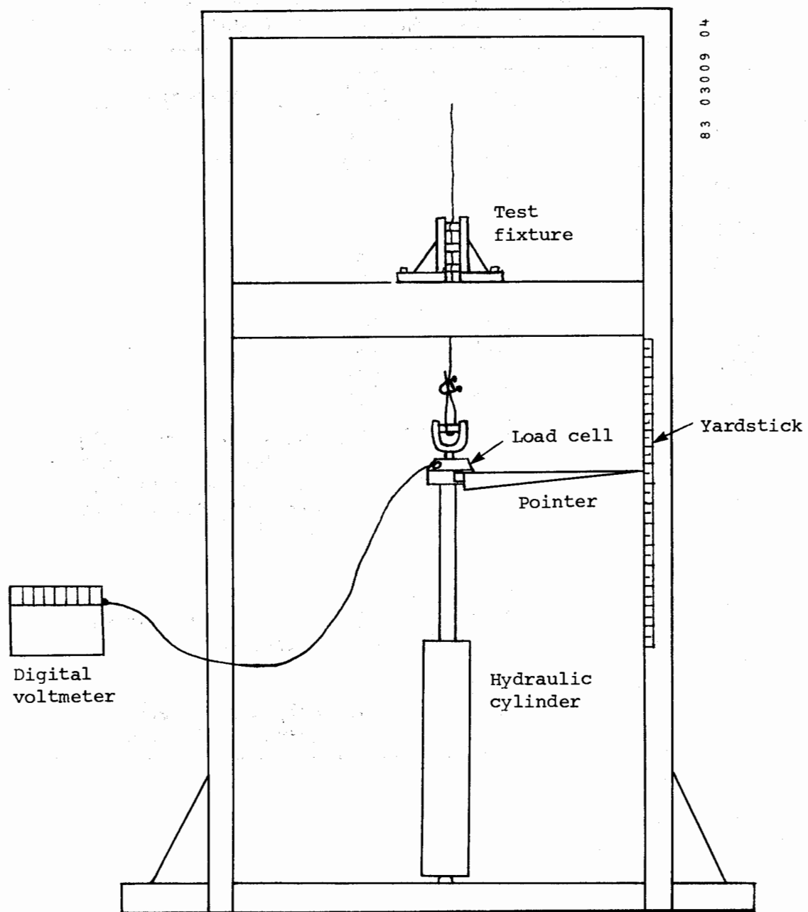
Figure G-2. Wire-pulling test apparatus.
