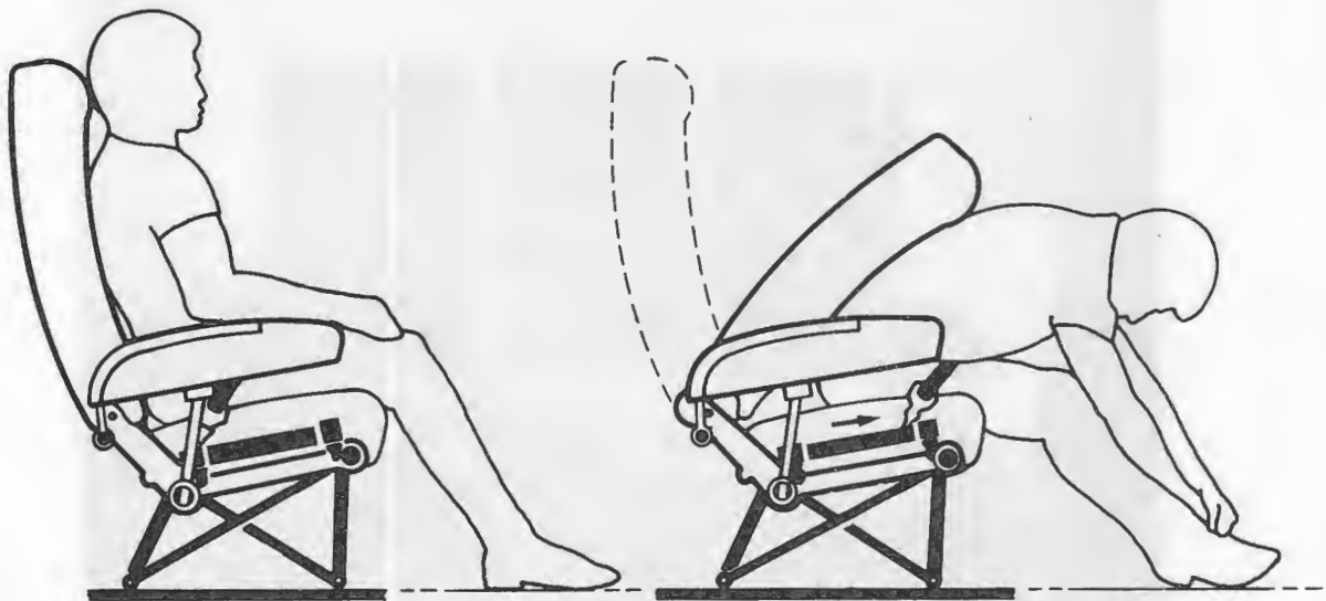
Figure 55. Weber MOD I seat before and after stroking.
