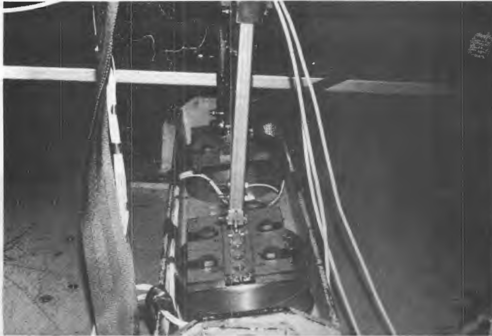
Figure 112. Pretest window-side rear leg of UOP MOD I seat after 10-degree track roll (Dynamic Test).
