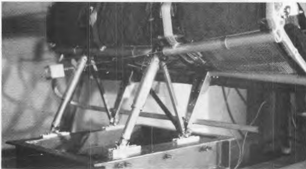
Figure 123. Posttest stroked rear leg energy absorbers of UOP MOD II seat (Forward Static Test).
