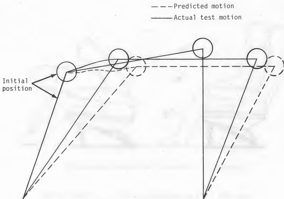
Figure 139. Leg structure kinematics of Weberlite MOD seat.
