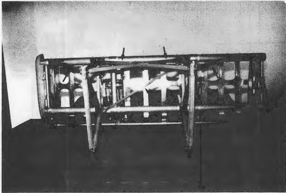
Figure 75. Weber MOD II seat lateral bracing - bottom view.
