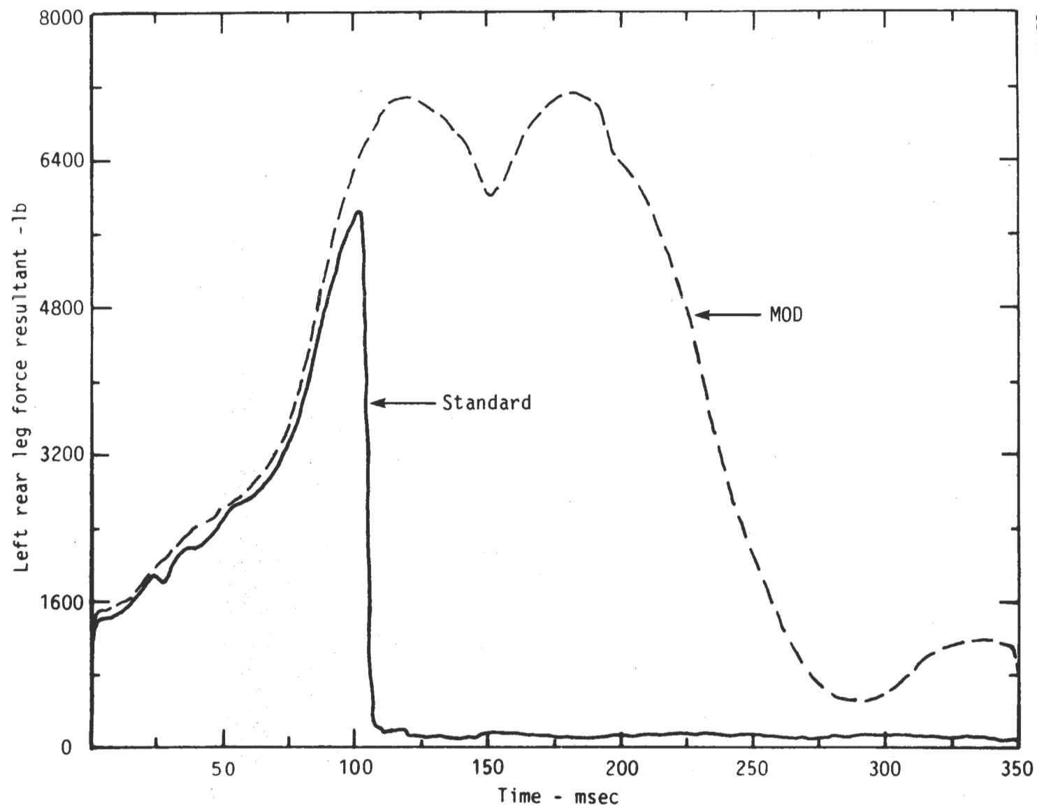
Figure 71. Rear window-side leg force resultants of standard and Weber MOD I seats.
