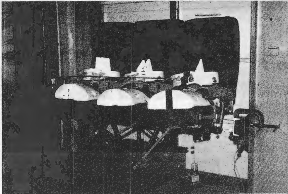
Figure 14. Lateral static test arrangement.
