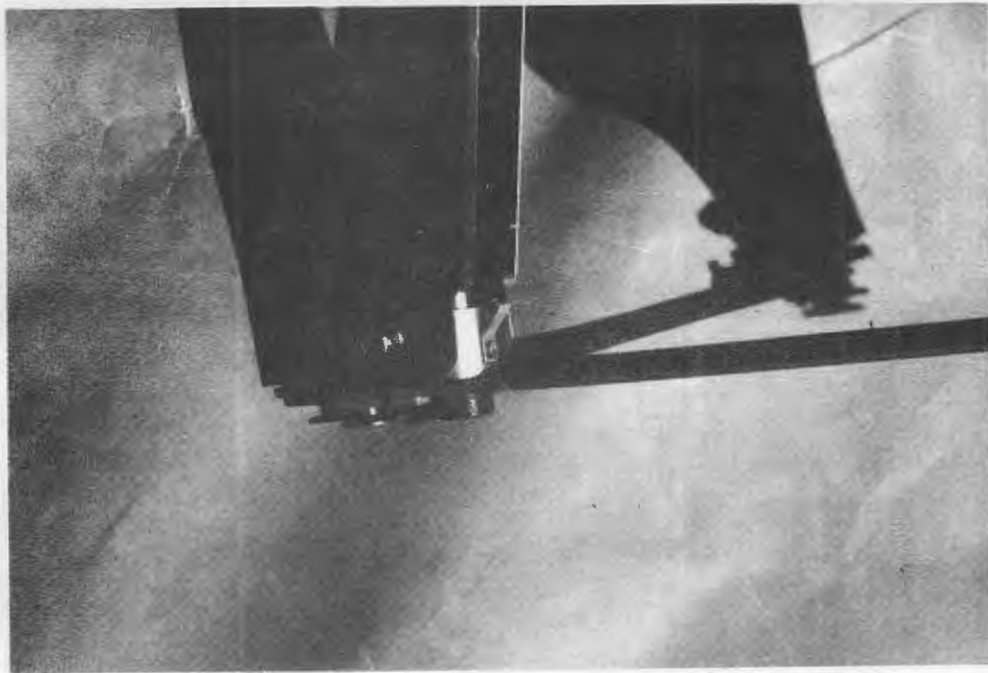
Figure 91. Rear track fitting of standard UOP seat.
