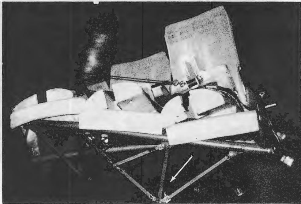
Figure 149. Posttest front view of Weberlite MOD seat (Lateral Test).
