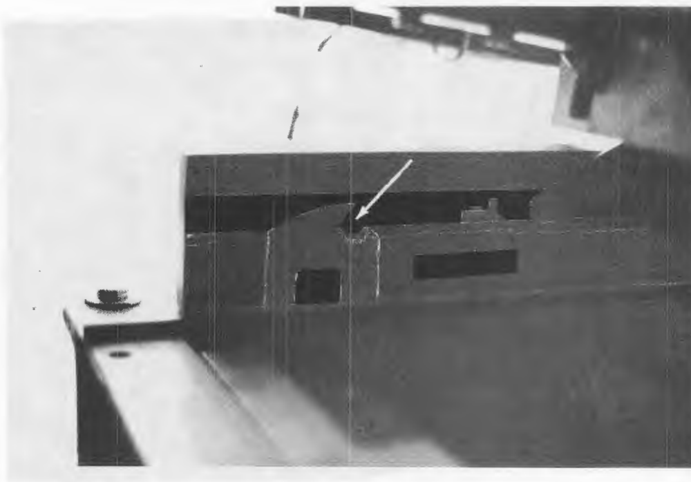
Figure 182. Posttest pivot bolt bracket failure of Trans-Aero flight attendant seat (Downward Test).
