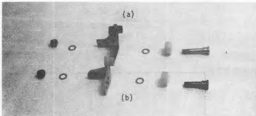
Figure 189. Comparison of modified (a) and standard (b) seat pan roller bracket assemblies.
