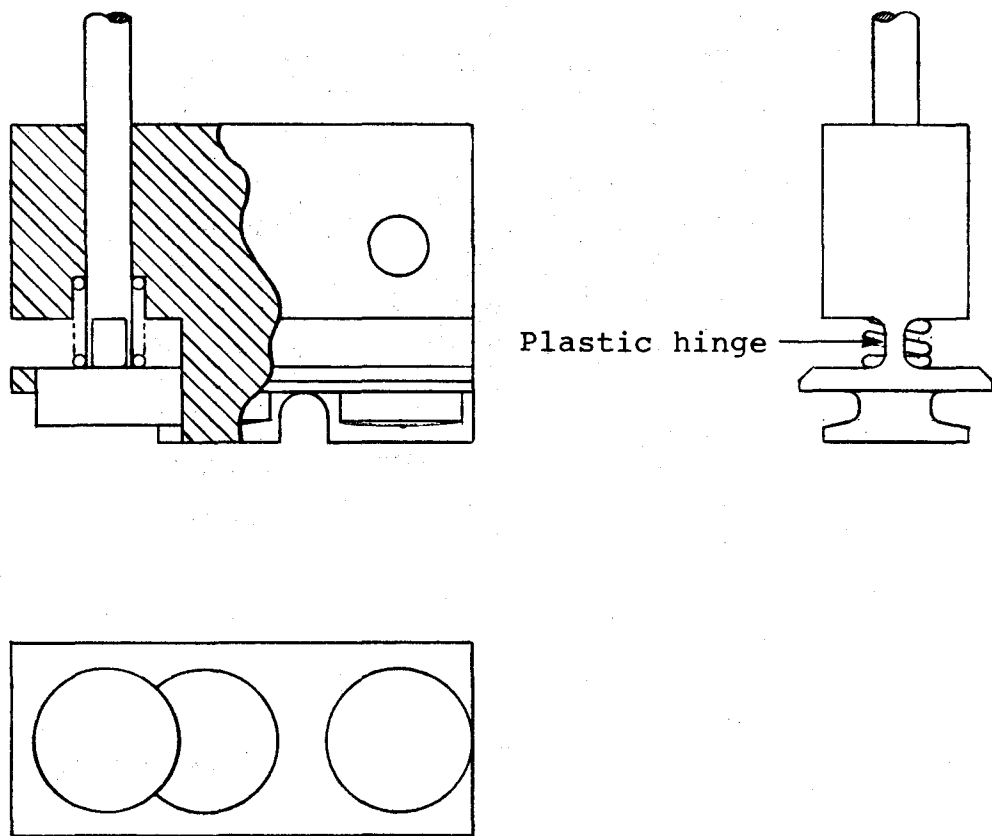
Figure 22. Track fitting concept with plastic hinge at track level.
