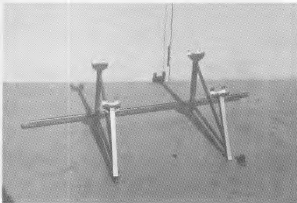
Figure 47. Leg assembly of standard Weber seat.
