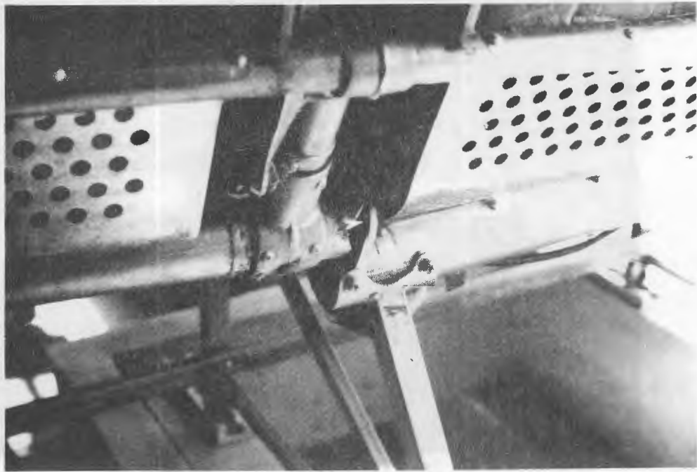
Figure 50. Posttest ruptured rear tube of standard Weber seat (Forward Static Test).
