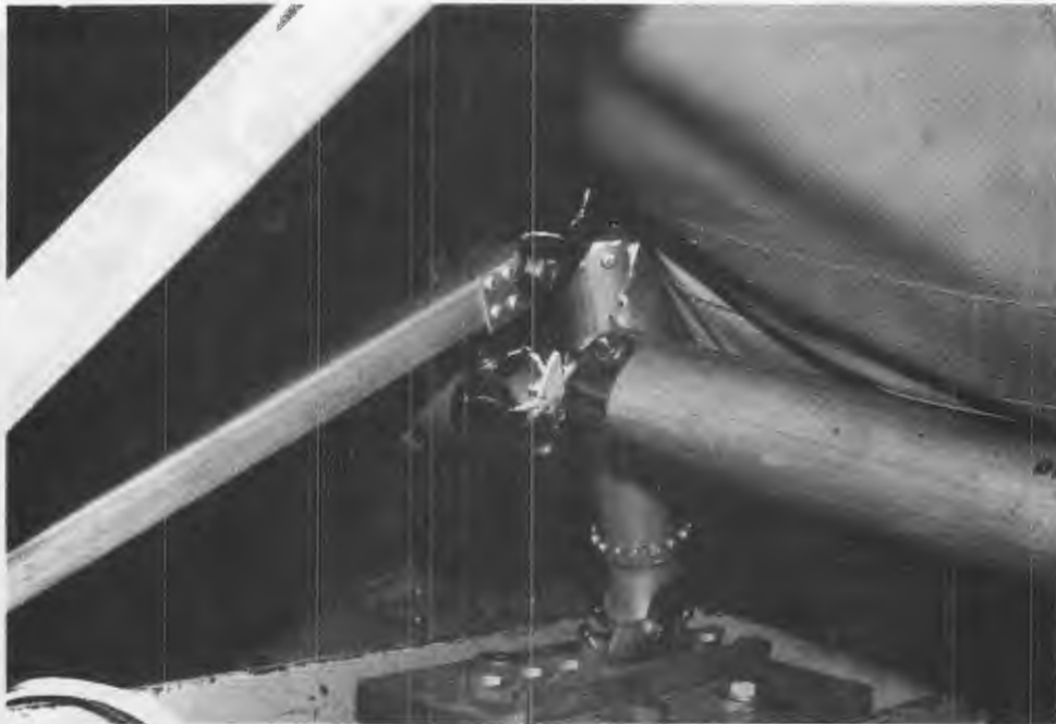
Figure 173. Posttest aisle-side energy absorber of Weber aft-facing MOD seat (Dynamic Test).
