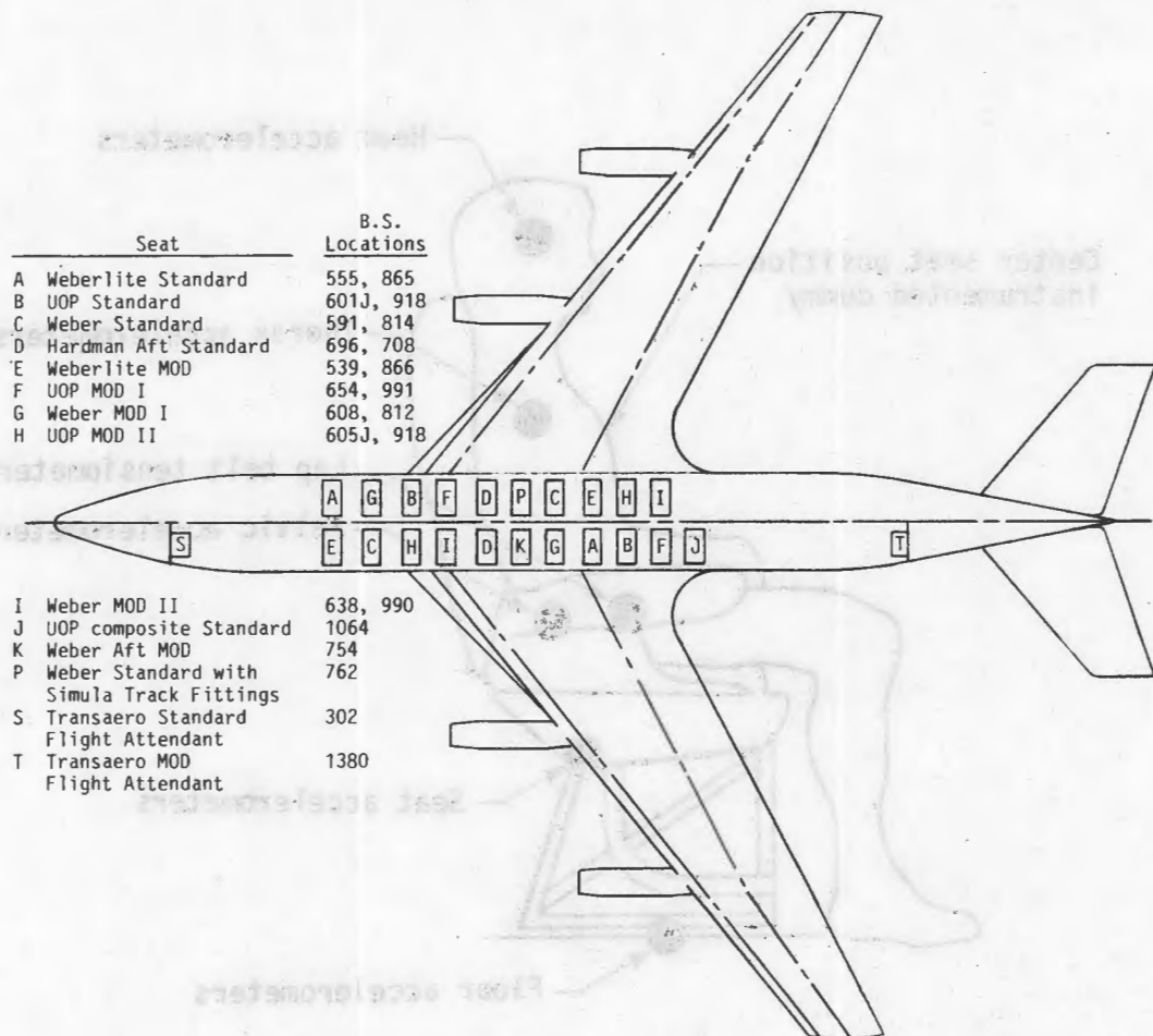
Figure 192. Position of seat experiments aboard aircraft.
