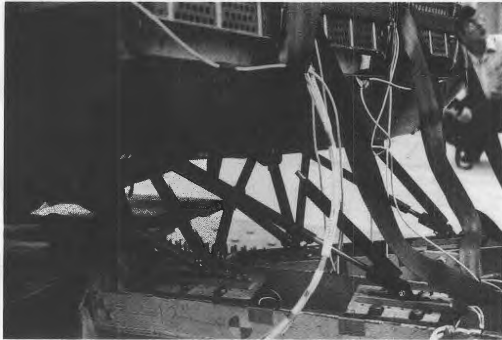
Figure 153. Posttest failed rear leg and diagonal energy absorber of Weberlite MOD seat (Dynamic Test).
