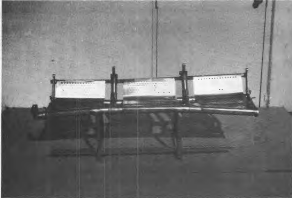
Figure 52. Posttest bent front tube of standard Weber seat (Forward Static Test).
