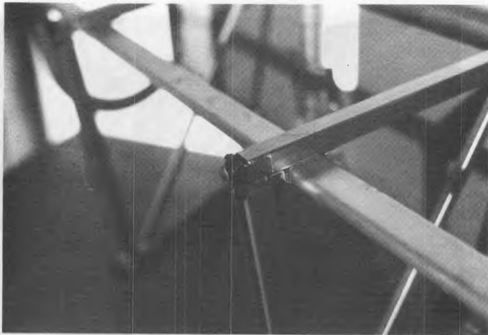
Figure 133. Standard Weberlite seat front track fitting.
