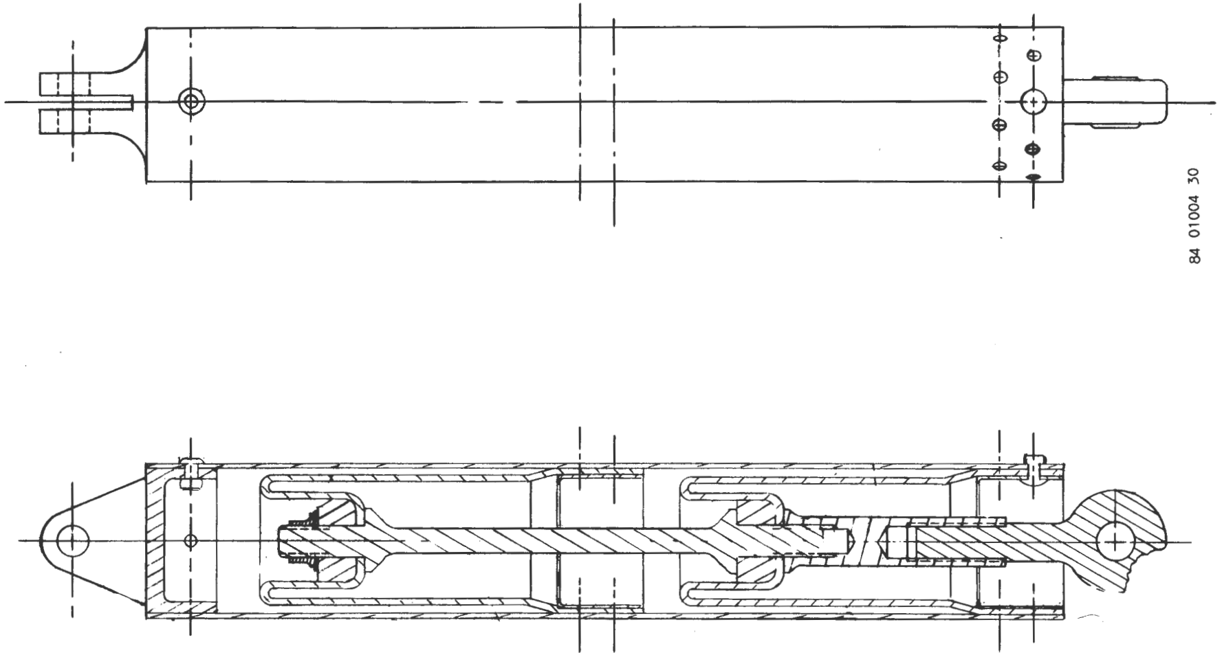
Figure 77. Weber MOD II seat energy absorber.
