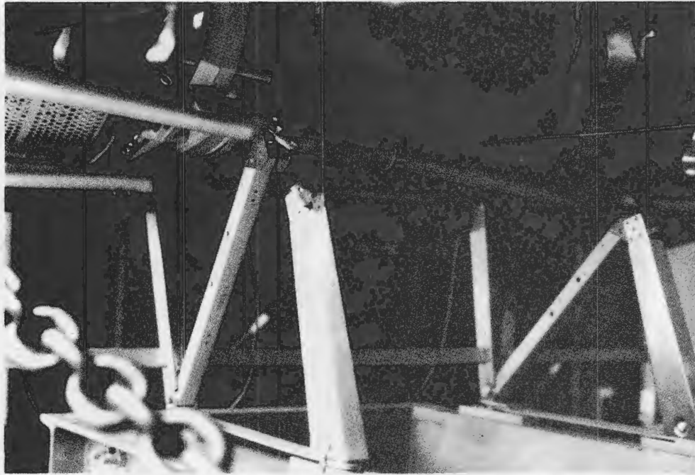
Figure 93. Posttest failed leg fitting on standard UOP seat (Forward Static Test).
