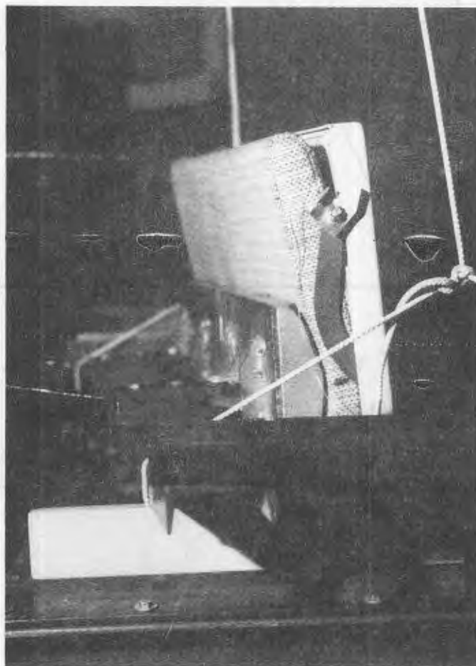
Figure 190. Posttest Trans-Aero flight attendant seat MOD pivot arm bracket failure (Downward Test).
