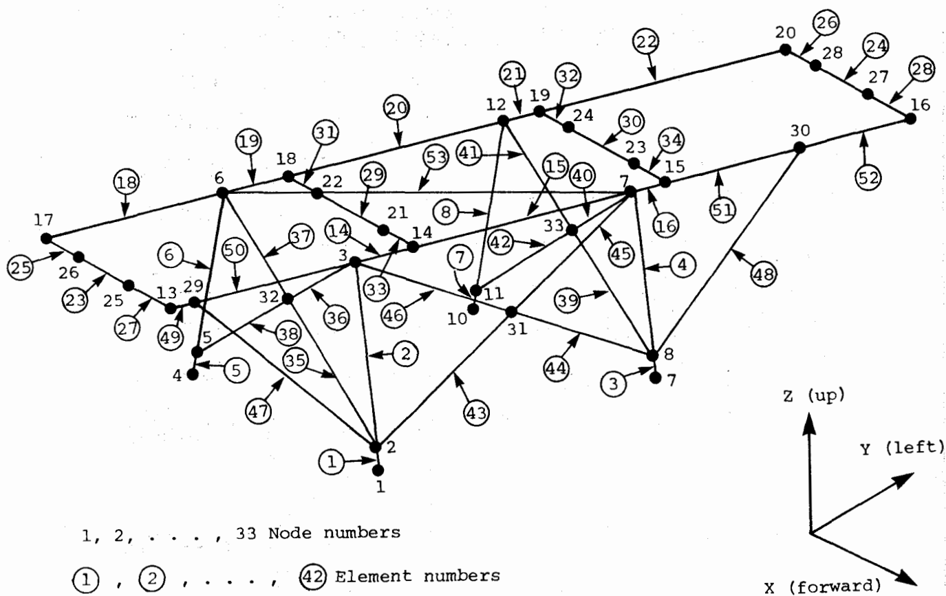
Figure B-2. Weber MOD I seat NASTRAN model.
