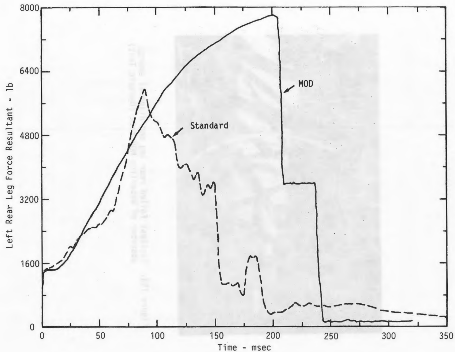
Figure 154. Rear window-side leg force resultants of standard and Weberlite MOD seats.
