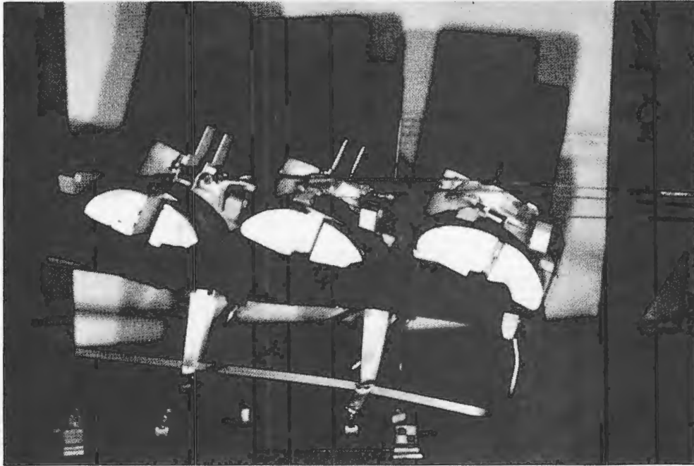
Figure 125. Posttest UOP MOD II seat (Lateral Test).
