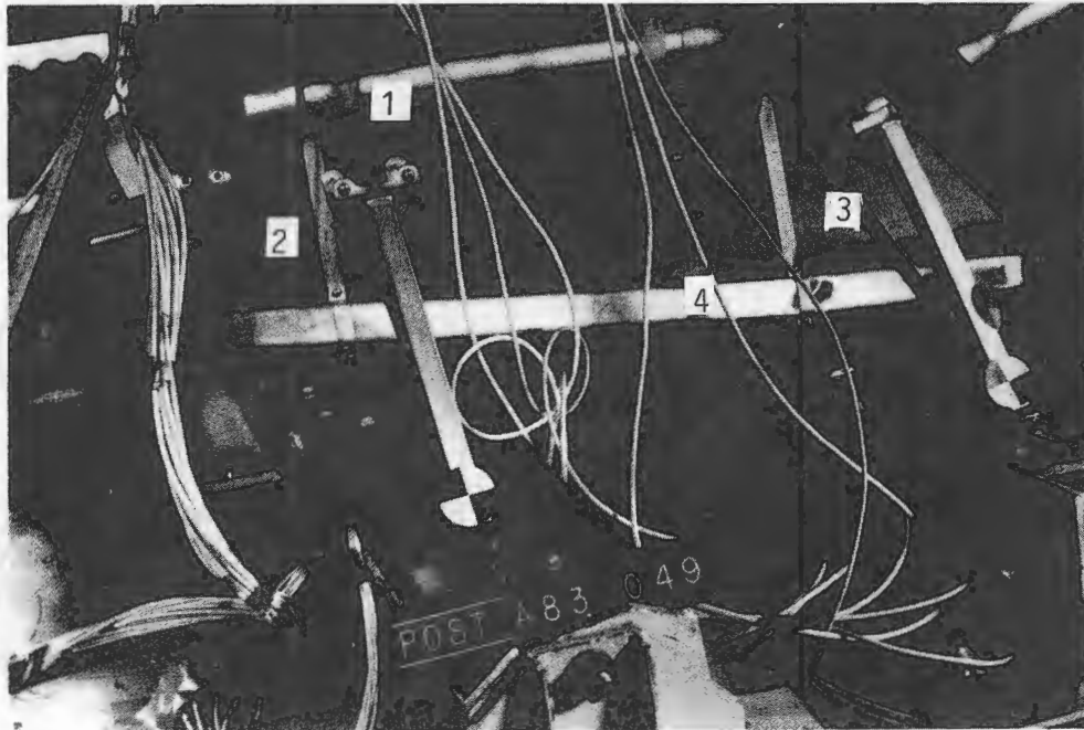
Figure 138. Failure points of standard Weberlite seat (Dynamic Test).
