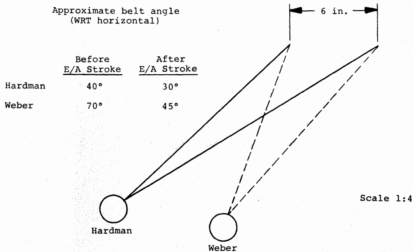
Figure E-4. Position of rear seat tubes and lap belts.
