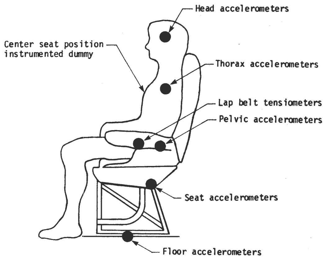
Figure 193. Typical complete instrumentation setup for test aircraft seats.
