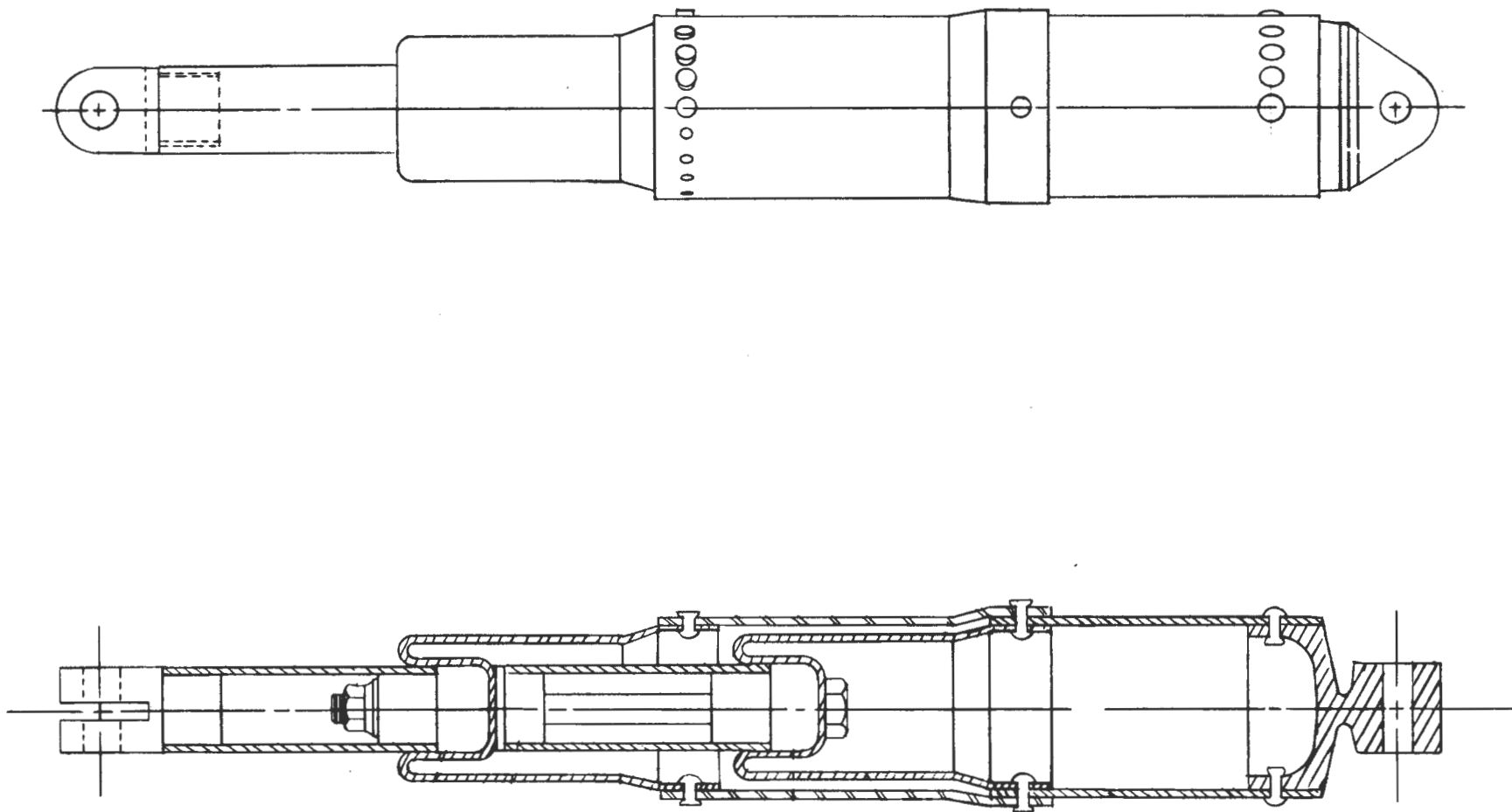
Figure 163. Weber aft-facing MOD seat energy absorber.
