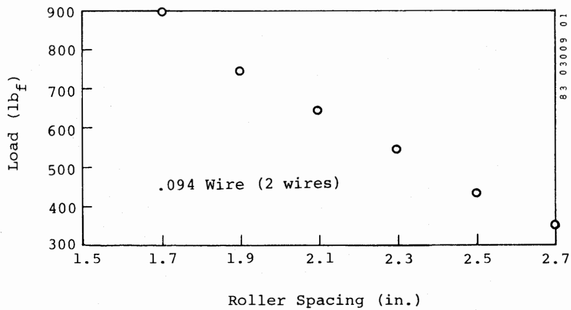
Figure G-3. Wire-pull results for .094 wire.
