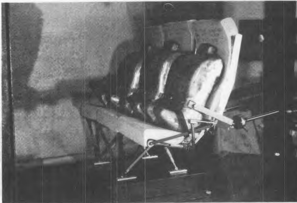
Figure 164. Arrangement of Weber aft-facing MOD seat (Forward Static Test).
