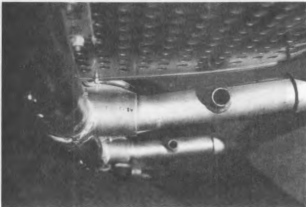
Figure 51. Posttest buckled spreader tube of standard Weber seat (Forward Static Test).
