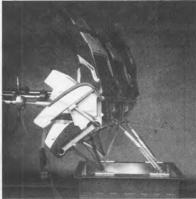
Figure 78. Posttest Weber MOD II seat (Forward Static Test).
