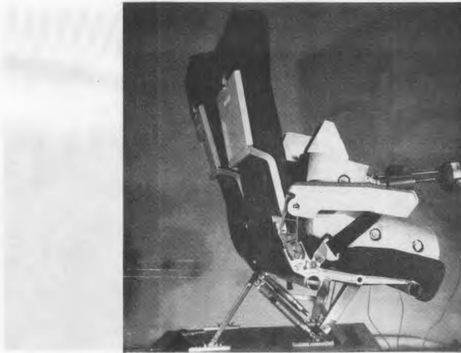
Figure 105. Posttest UOP MOD I seat (Forward Static Test).
