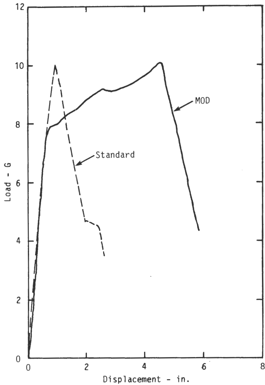
Figure 110. Load versus forward displacement of standard and UOP MOD I seats.
