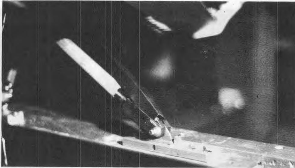
Figure 151. Stroked aisle-side diagonal of Weberlite MOD seat (Lateral Test).
