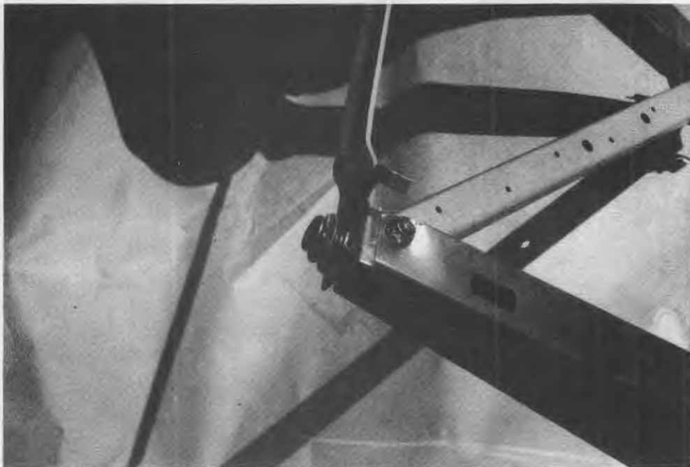
Figure 92. Anti-rattle mechanism on front leg of UOP seat.
