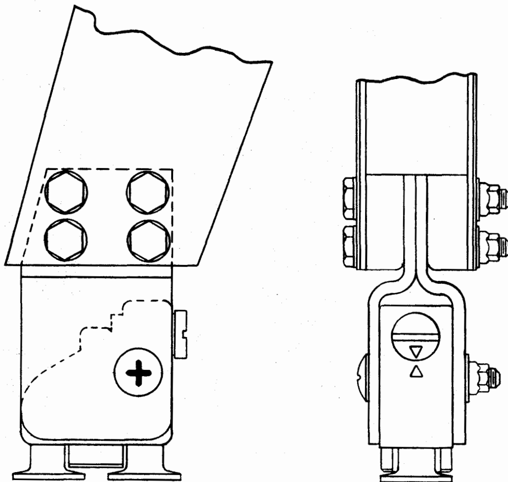
Figure 20. Plastic hinge adapted to Brownline track fitting.
