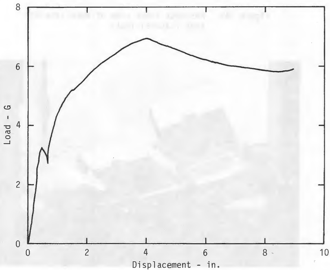
Figure 151. Stroked aisle-side diagonal of Weberlite MOD seat (Lateral Test).
