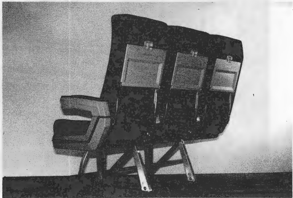
Figure 88. Standard UOP seat - rear view.
