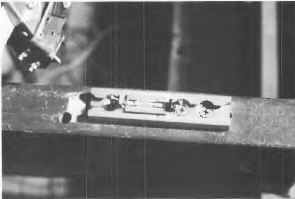
Figure 126. Posttest top view of front window-side leg and failed track fitting of UOP MOD II seat (Lateral Test).
