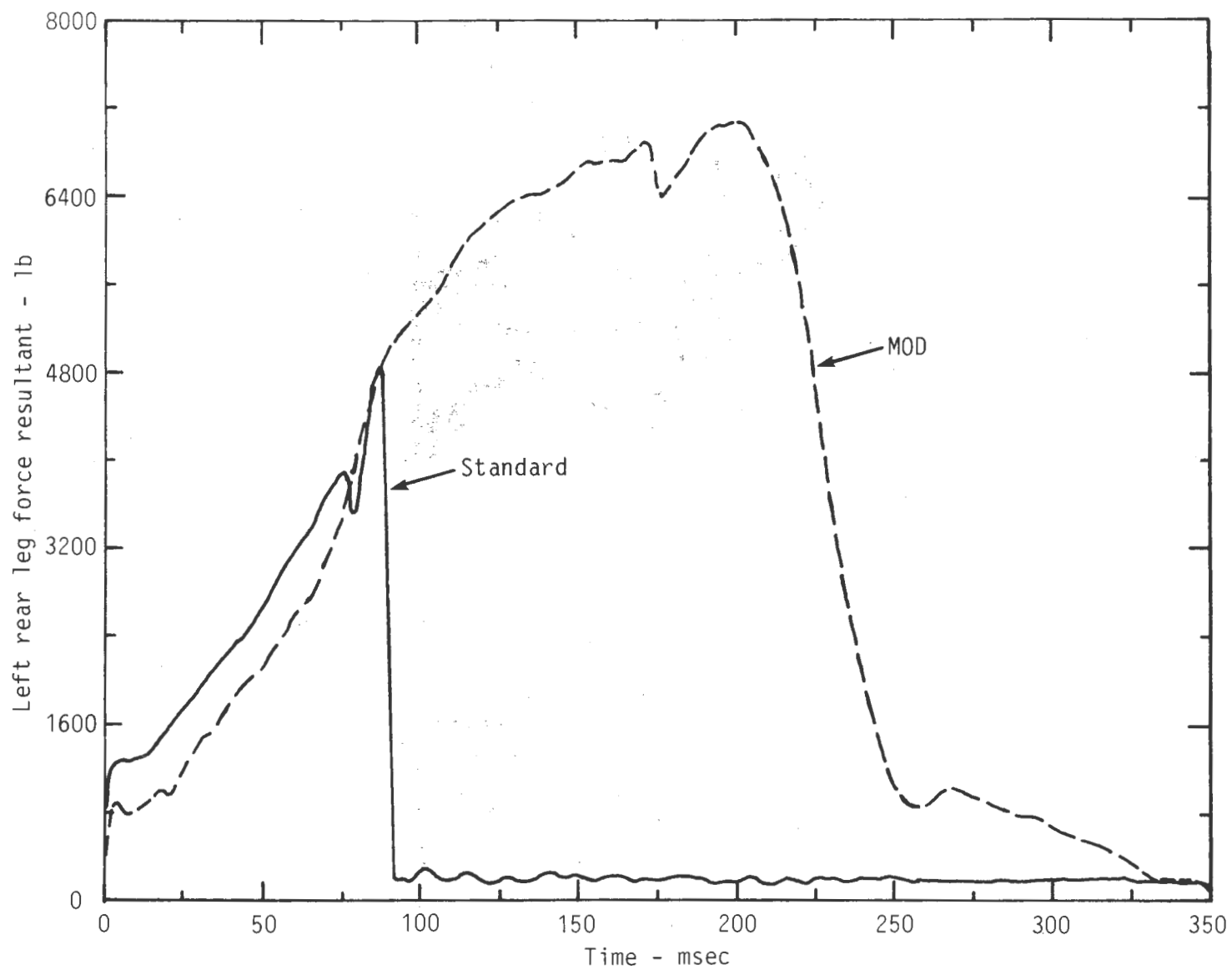
Figure 114. Rear window-side leg force resultants of standard and UOP MOD I seats.
