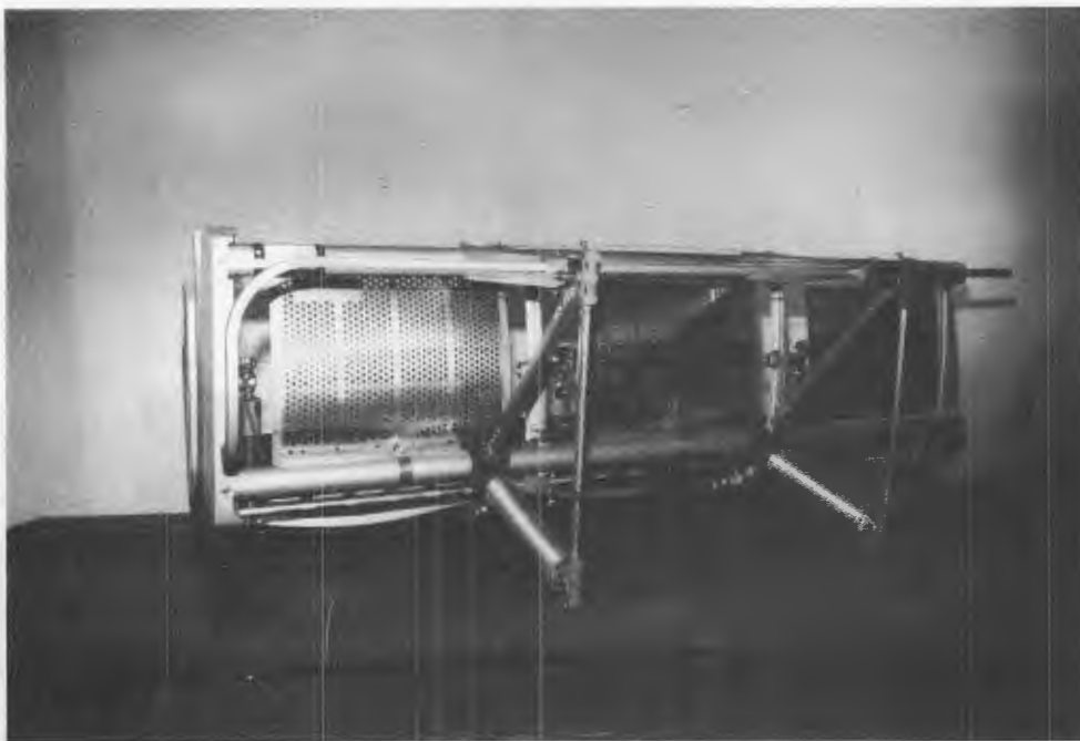
Figure 119. Leg structure and energy absorbers of UOP MOD II seat.
