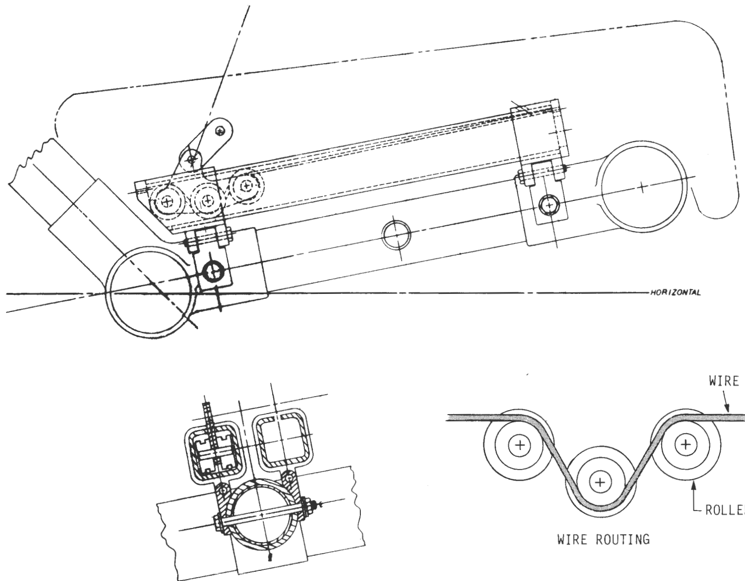
Figure 60. Weber MOD I seat lap belt energy absorber.
