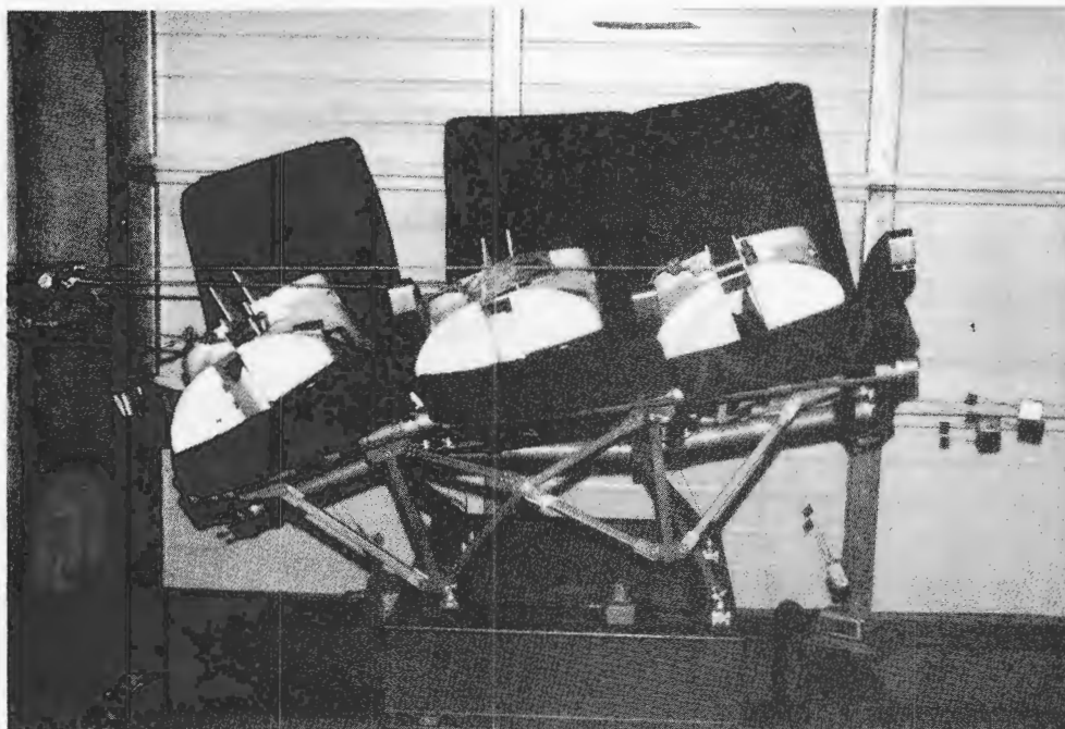
Figure 65. Posttest Weber MOD I seat (Lateral Test).
