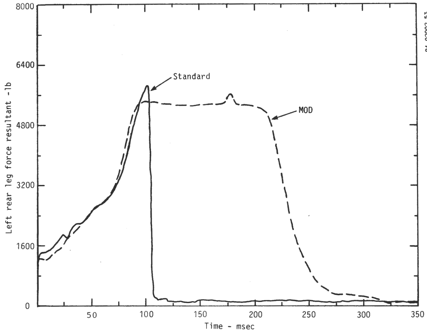
Figure 86. Rear window-side leg force resultants of standard and Weber MOD II seats.
