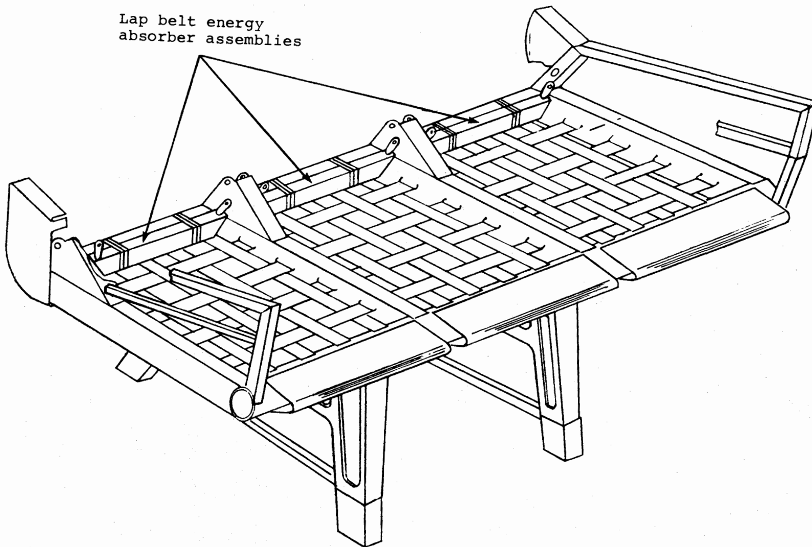
Figure 5. Installation of Hardman lap belt energy absorber.
