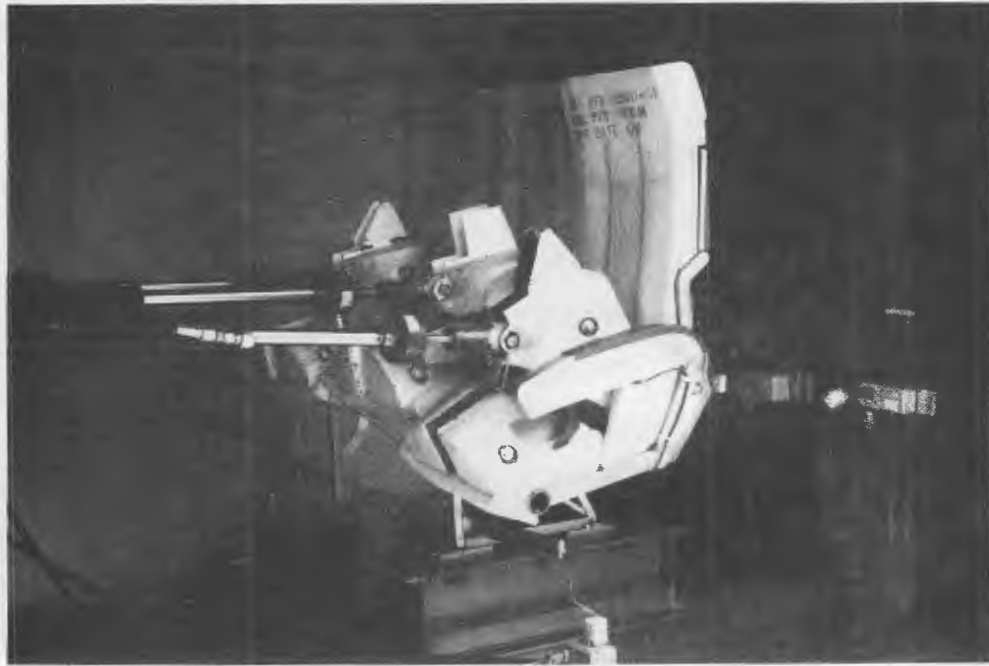
Figure 134. Posttest standard Weberlite seat (Forward Static Test).
