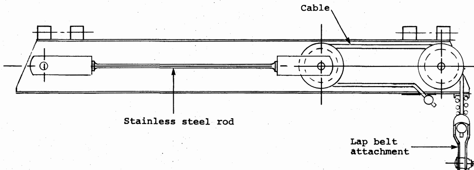
Figure 4. Hardman lap belt energy absorber.
