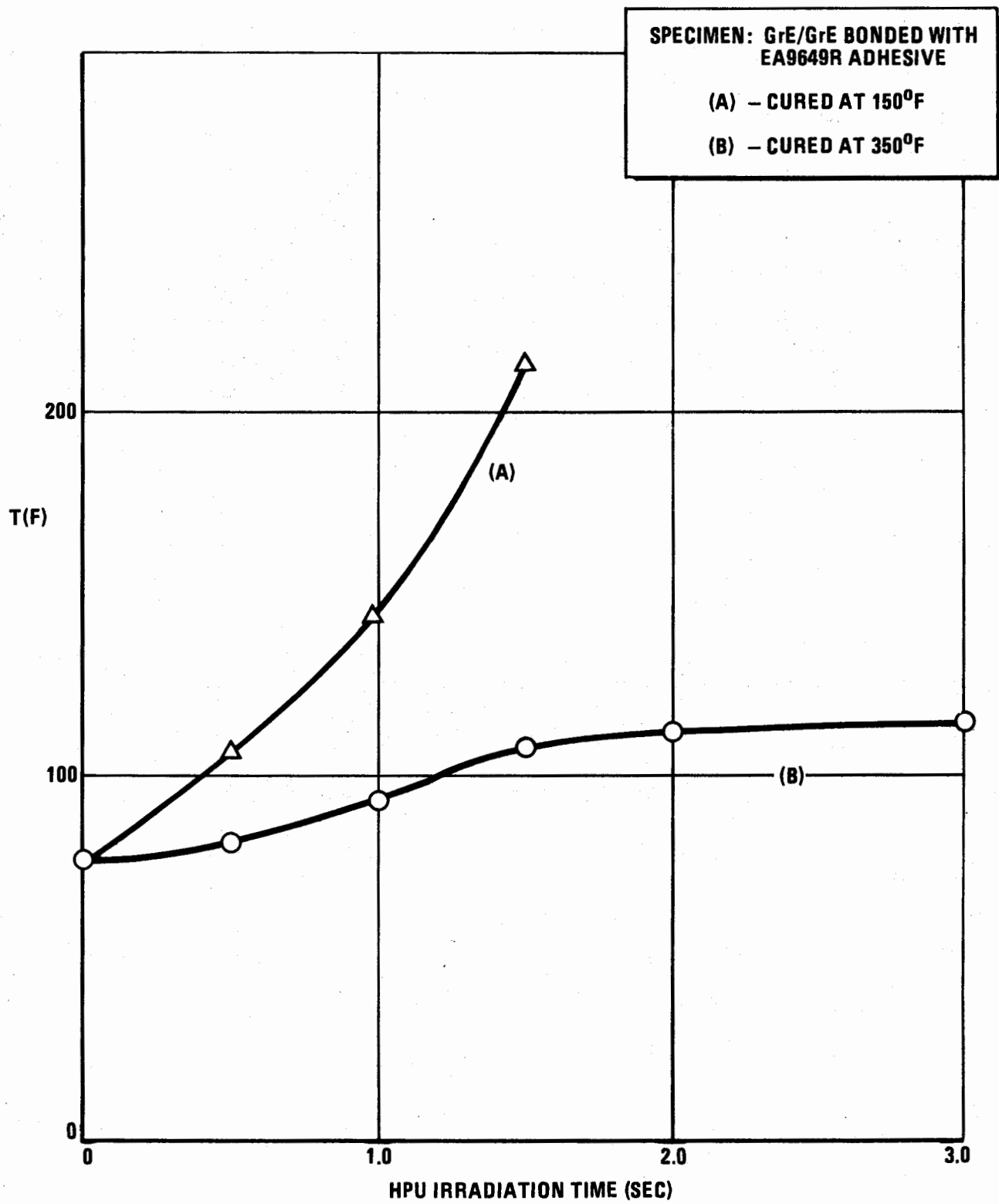
FIGURE 19 BONDLINE TEMPERATURE DURING HPU IRRADIATION
