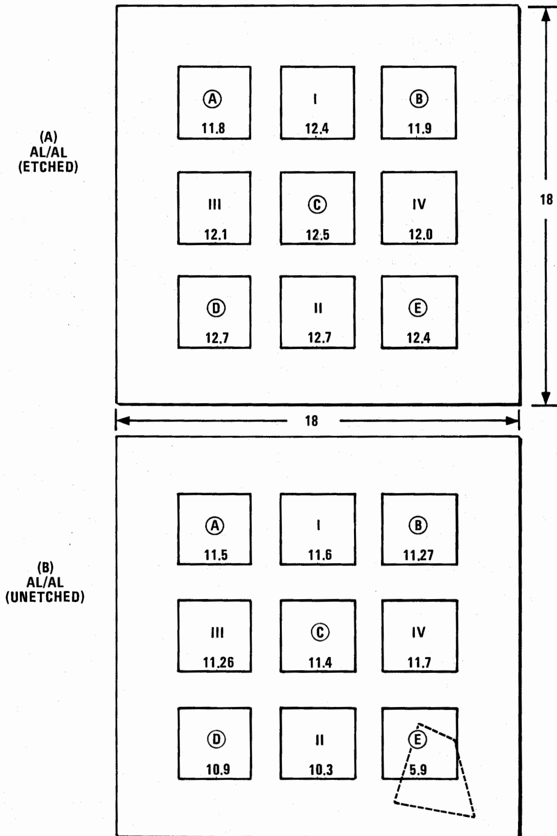
FIGURE 7 HPU TEST ON AL/AL PLATES: (A) ETCHED AND (B) UNETCHED
