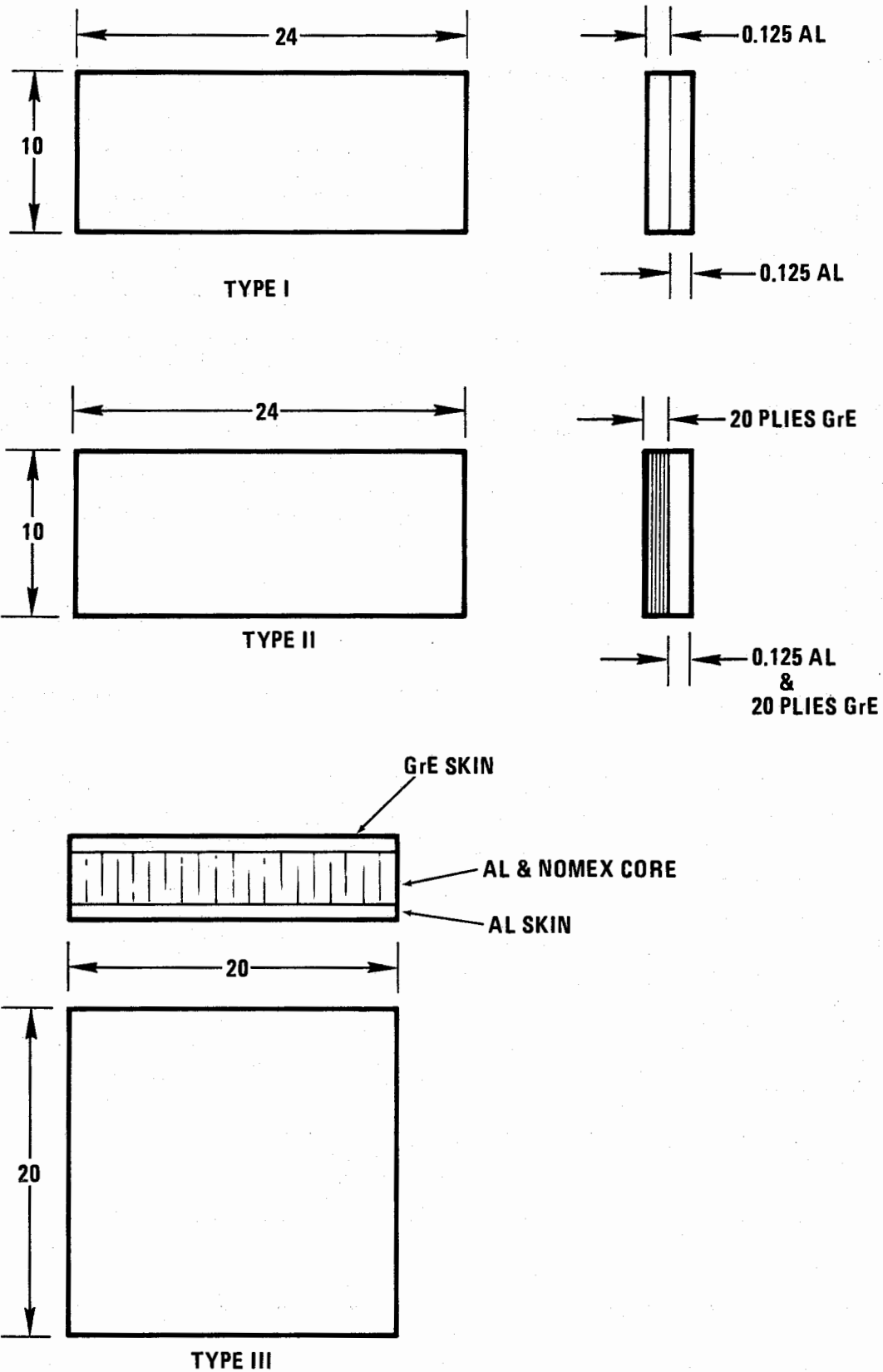
FIGURE 1 SPECIMEN CONFIGURATION
