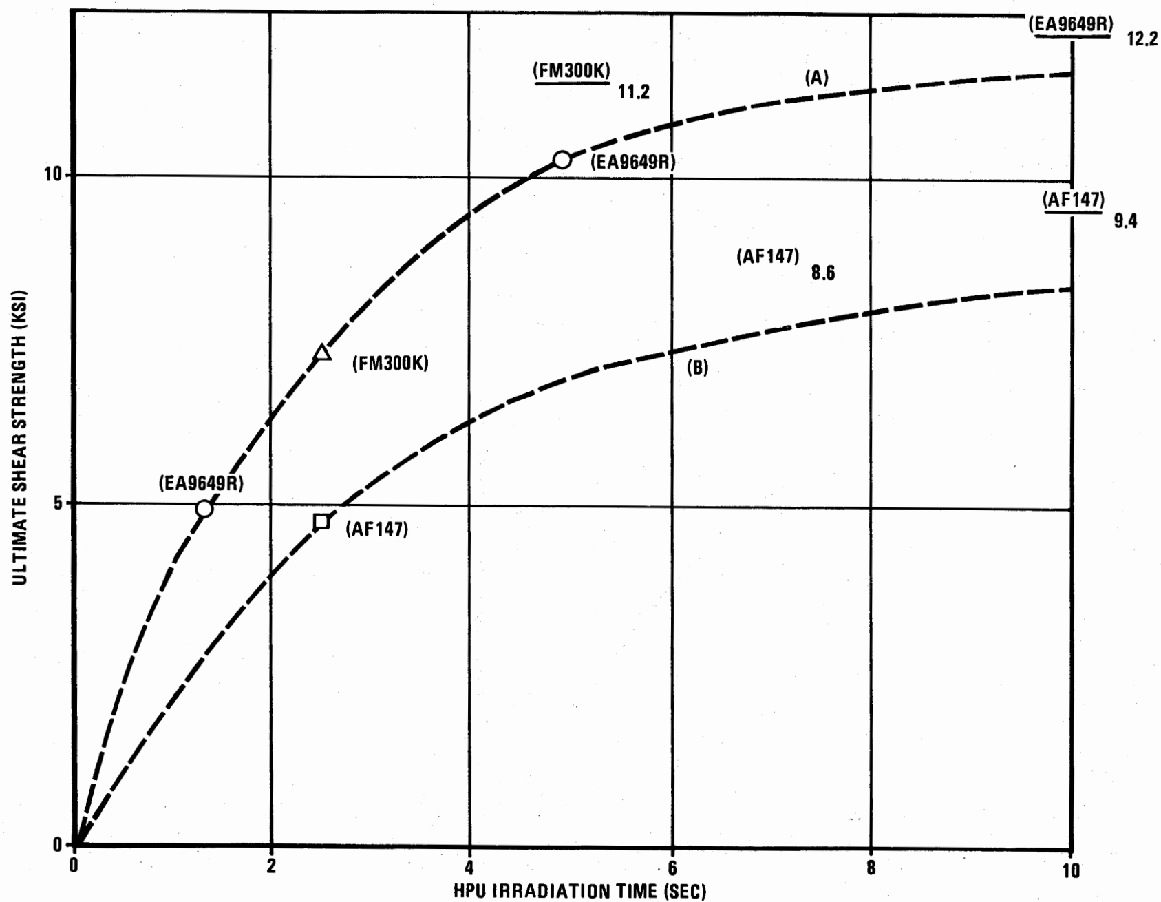
FIGURE 6 ULTIMATE SHEAR STRENGTH VS HPU IRRADIATION TIME FOR AL/AL SPECIMENS
