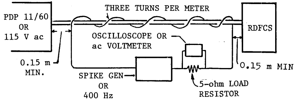
Figure 18.- RS02 cable test setup.
