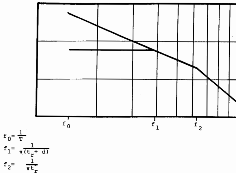
Figure 1.- Typical digital signal waveform.
