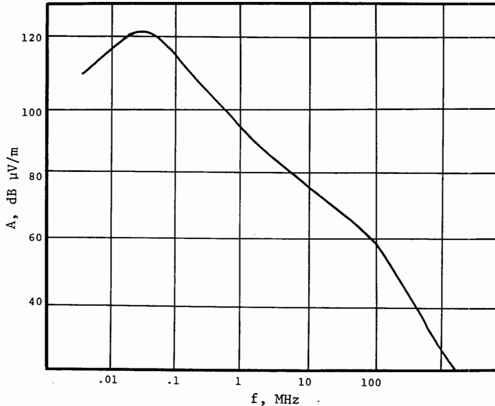
Figure 3.- Spectrum of total lightning flash. (Normalized to a bandwidth of 1 kHz and at a distance of 10 km. Uman and Krider, IEEE Transactions on EMC, EMC-24(2), 1982.)
