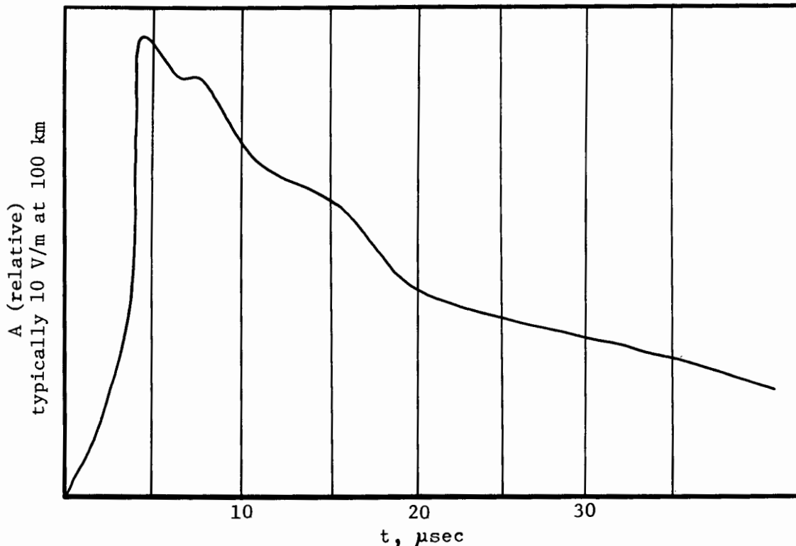
Figure 2.- Typical lightning flash waveform (cloud to ground).
