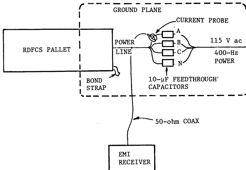
Figure 12.- CE03 test setup.
