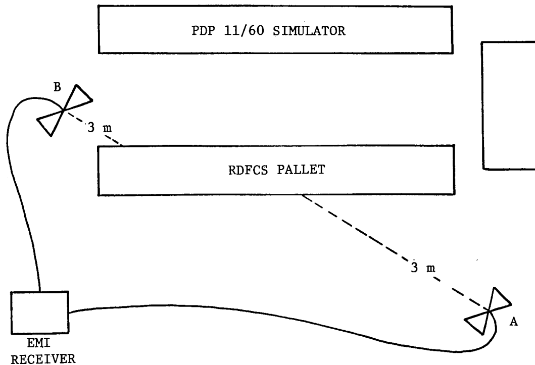
Figure 13.- RE02 (modified) test setup.
