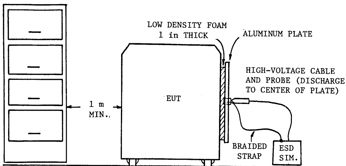
Figure 22.- ESD direct discharge test setup.
