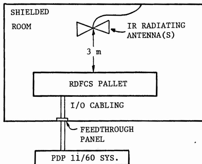
Figure 20.- RS02 (modified) ESD susceptibility test setup.
