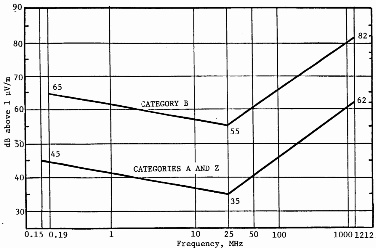
Figure 6.- Maximum level of radiated CW interference from any one piece of equipment.
