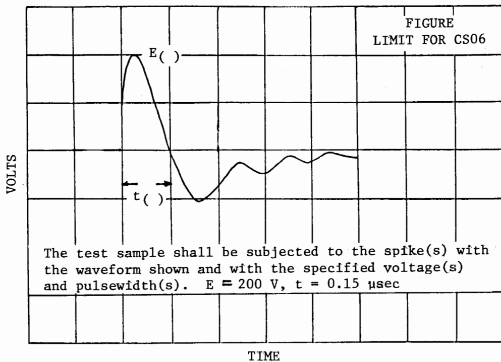
Figure 14.- Limit for CS06.
