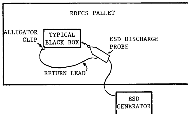
Figure 22.- ESD direct discharge test setup.
