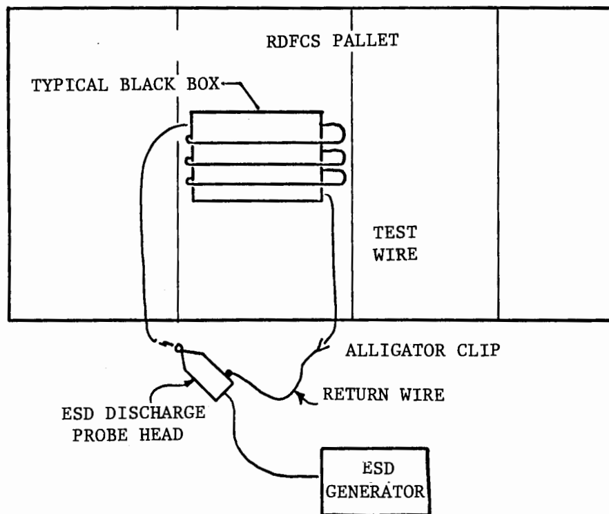
Figure 20.- RS02 (modified) ESD susceptibility test setup.
