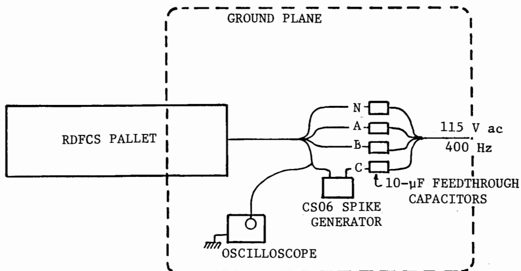
Figure 15.- CS06 test setup.
