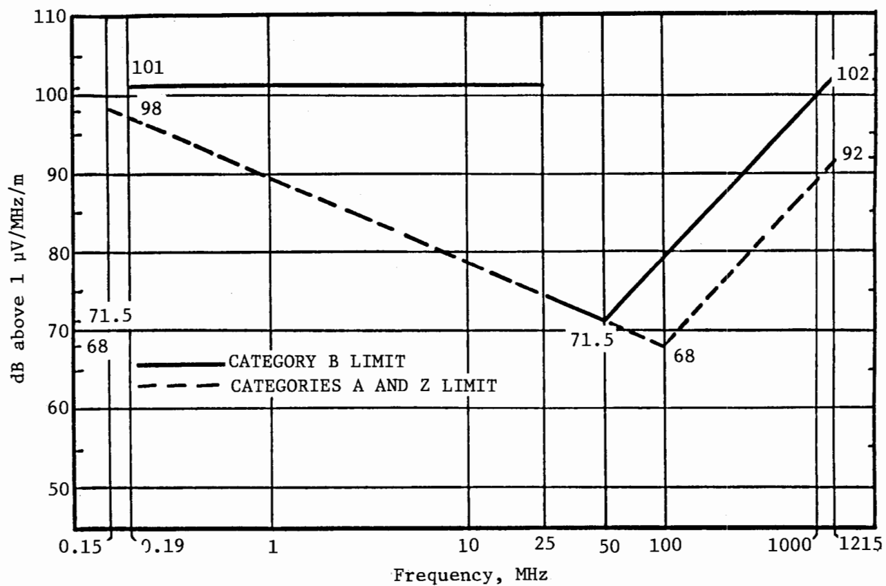
Figure 7.- Maximum level of radiated broadband and pulsed CW from any one piece of equipment.
