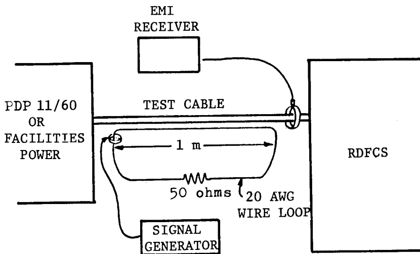
Figure 17.- RF-induced cable susceptibility test setup.
