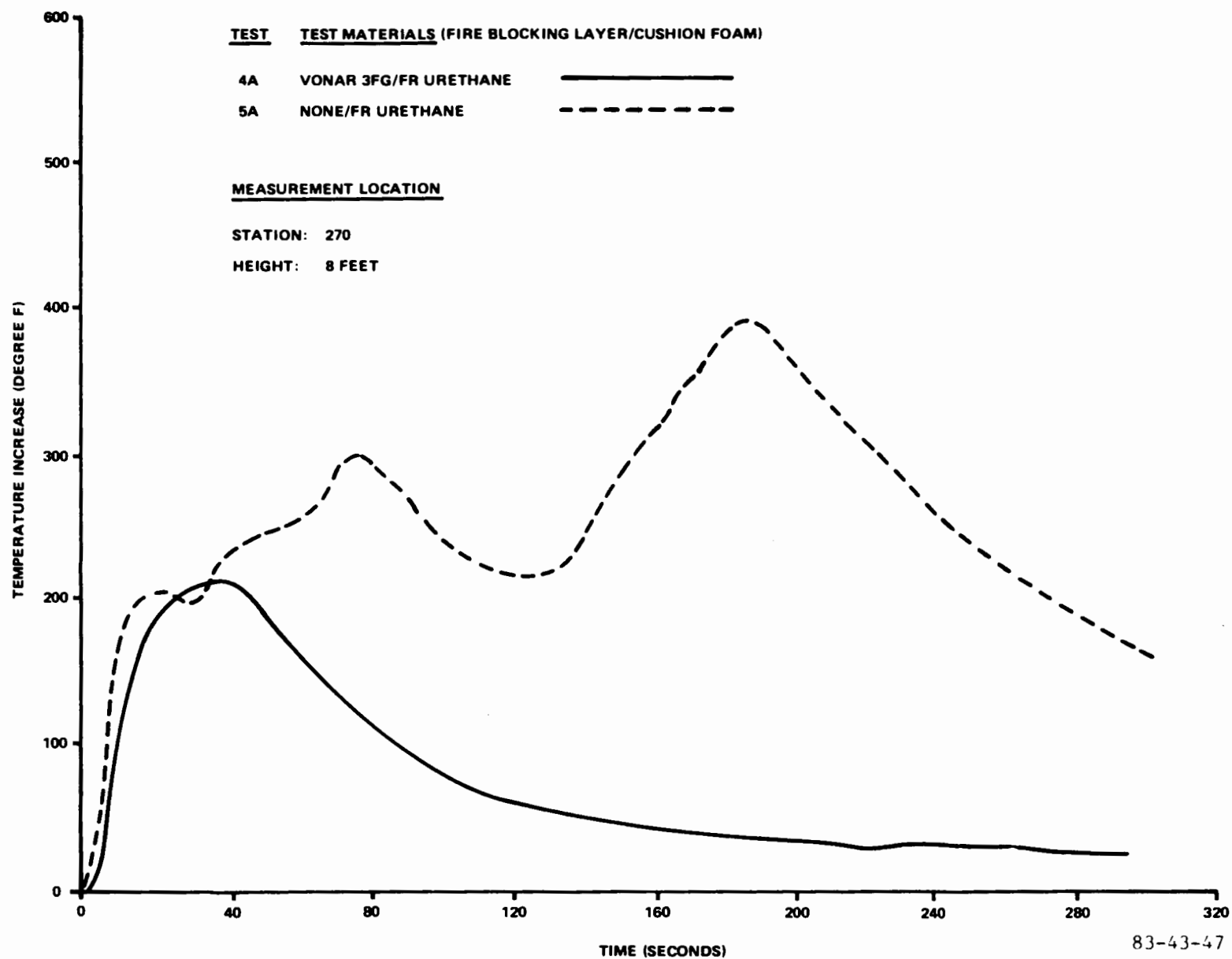
FIGURE 47. IN-FLIGHT GASOLINE TEST TEMPERATURE COMPARISON
