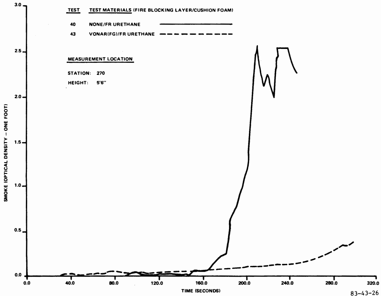
FIGURE 26. POST-CRASH SERIES FIVE SMOKE COMPARISON
