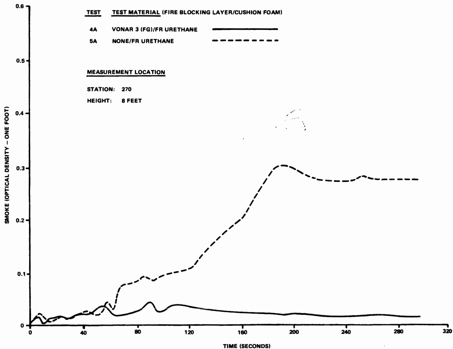
FIGURE 48. IN-FLIGHT GASOLINE TEST SMOKE COMPARISON
