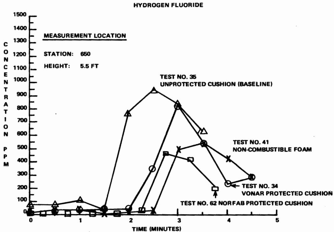
FIGURE B-6. EFFECT OF CUSHIONING PROTECTION AND MATERIALS ON HF AND HCl LEVES IN POST-CRASH FIRES
