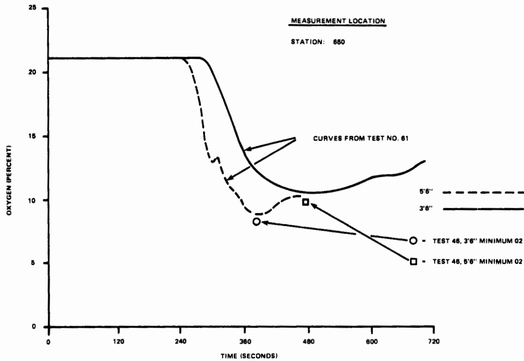
FIGURE 56. FULL-SCALE IN-FLIGHT OXYGEN COMPARISONS
