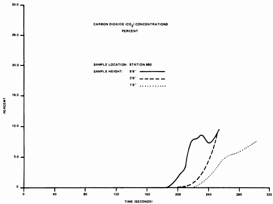
FIGURE C-5. CO 2 PROFILE STATION 650 (1 of 2 Sheets)
