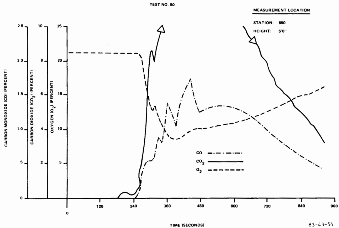
FIGURE 55. FULL-SCALE IN-FLIGHT SMOKE MEASUREMENTS
