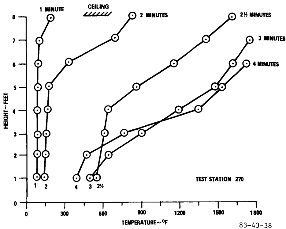
FIGURE 38. HEAT STRATIFICATION IN FORWARD CABIN
