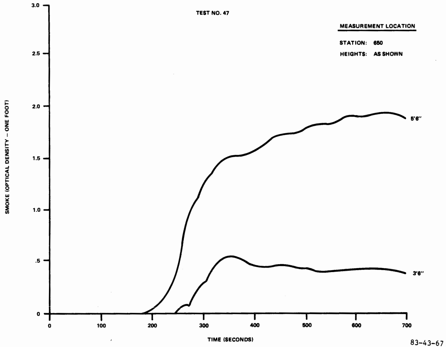
FIGURE 67. RAMP FIRE SMOKE PROFILE
