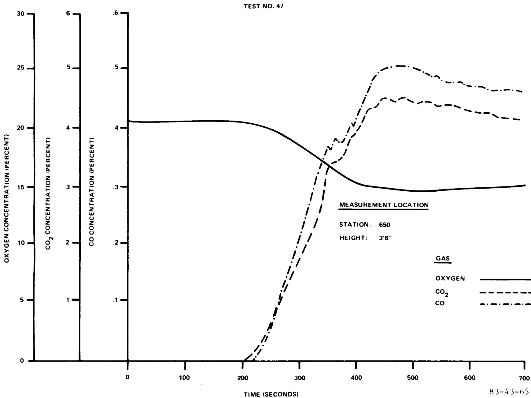
FIGURE 65. RAMP FIRE GAS CONCENTRATIONS
