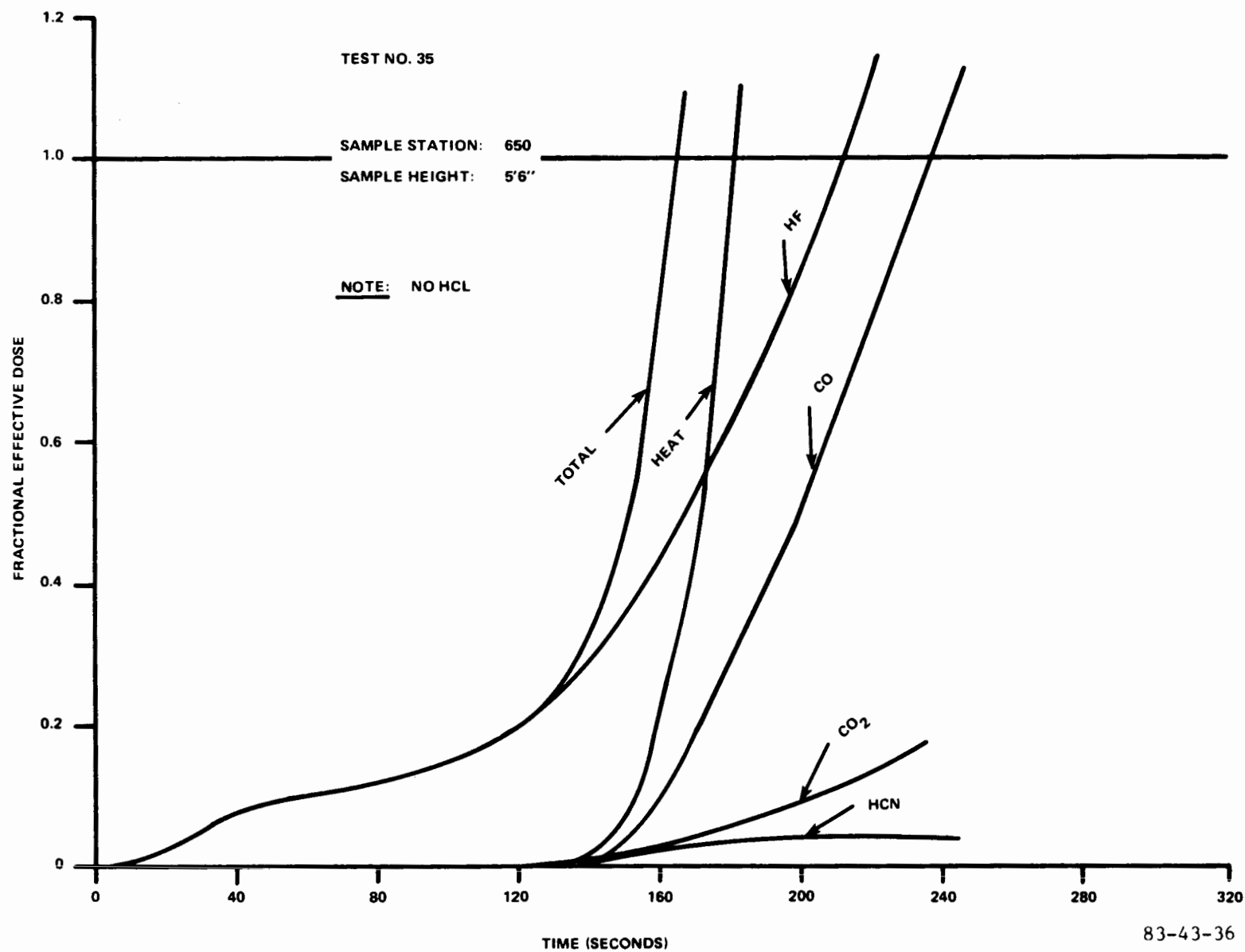
FIGURE 36. FRACTIONAL EFFECTIVE DOSE PLOT FOR TEST NUMBER 35 (NO HCL)
