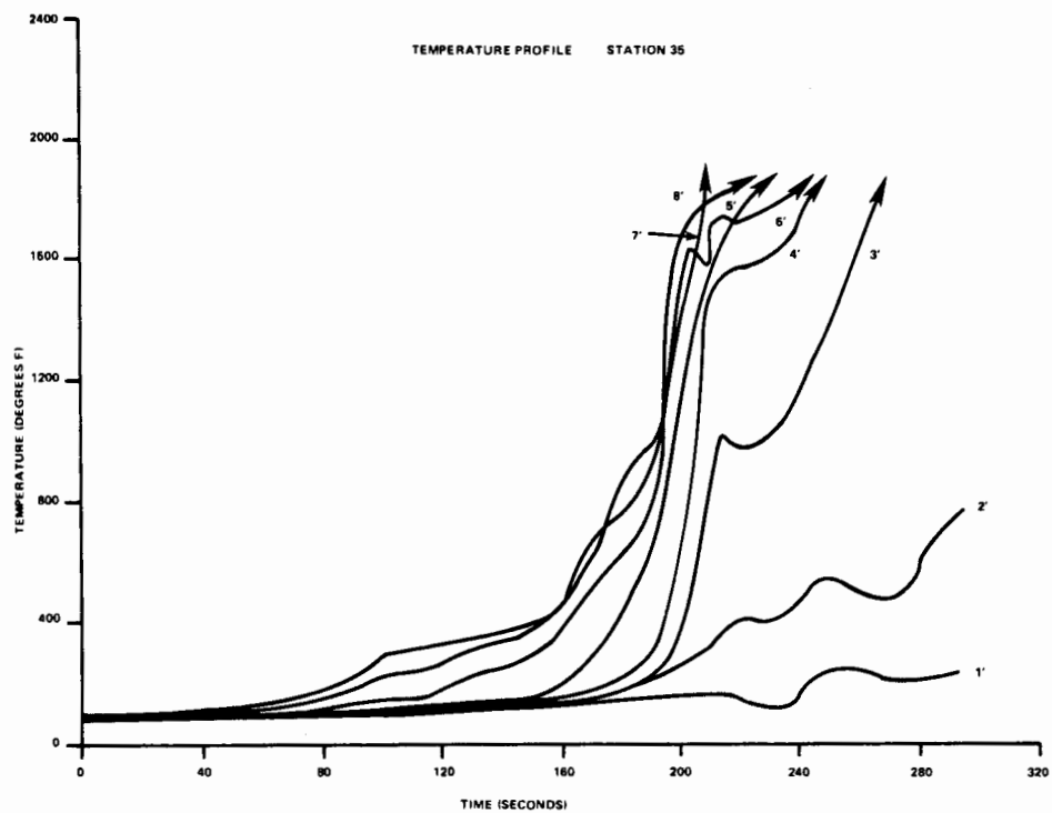
FIGURE C-1. TEMPERATURE PROFILE STATION 35 (1 of 2 Sheets)
