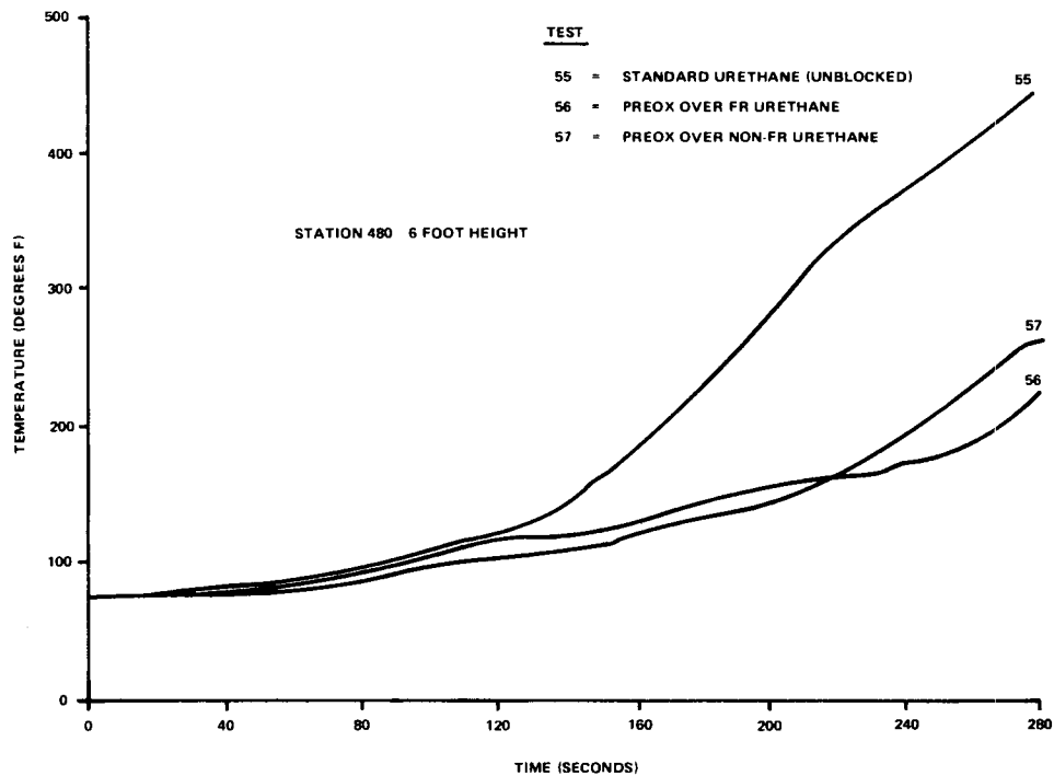
COMPARISON OF FR URETHANE AND NON-FR URETHANE FOAM UNDER A BLOCKING LAYER
