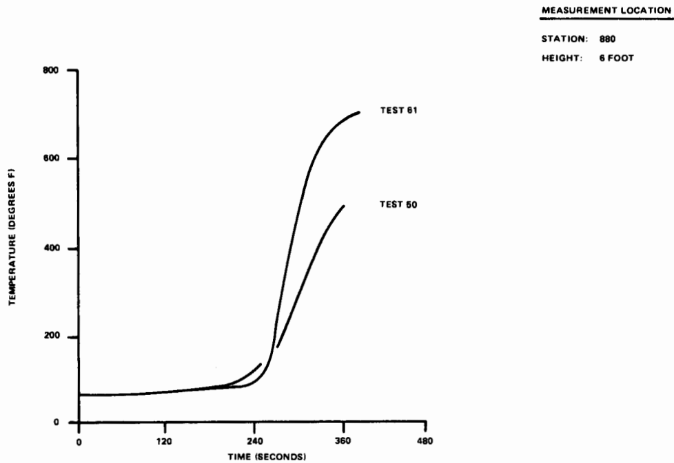
FIGURE 58. FULL-SCALE IN-FLIGHT TEMPERATURE COMPARISONS, STATION 880
