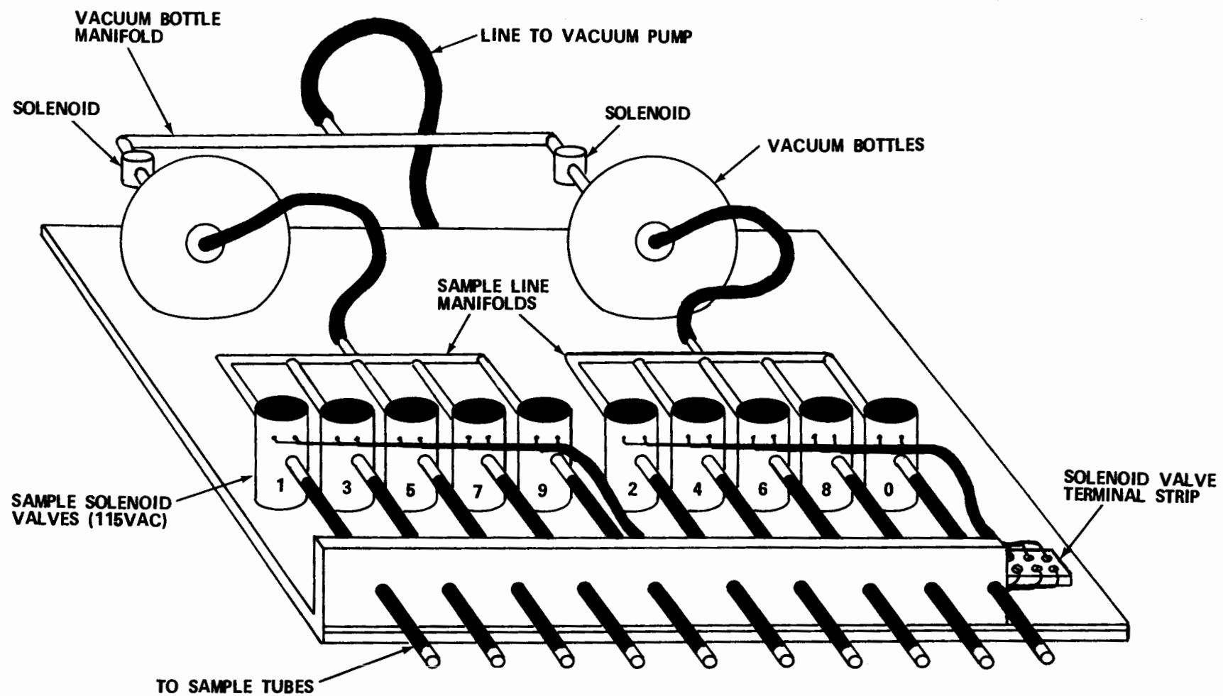
FIGURE B-2. SOLENOID VALVE ASSEMBLY
