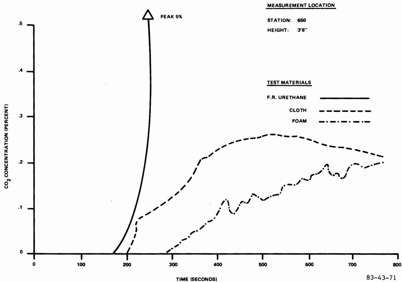
FIGURE 71. RAMP FIRE BLOCKING LAYER CO 2 COMPARISON
