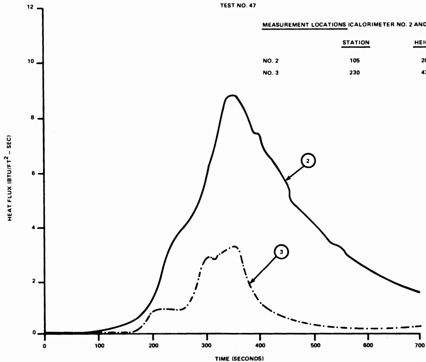
FIGURE 66. RAMP FIRE HEAT FLUX MEASUREMENTS
