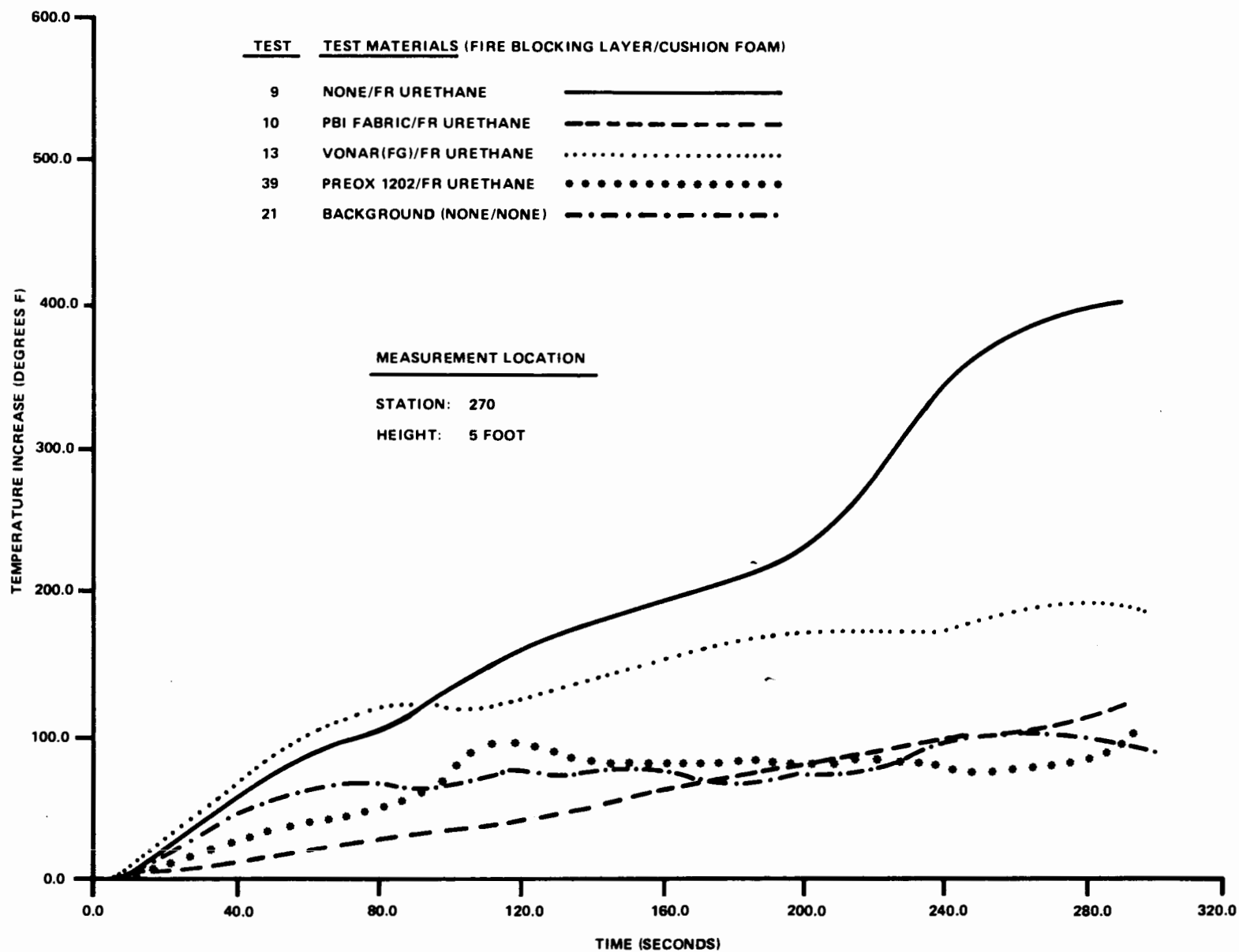
FIGURE 17. POST-CRASH SERIES THREE TEMPERATURE COMPARISON
