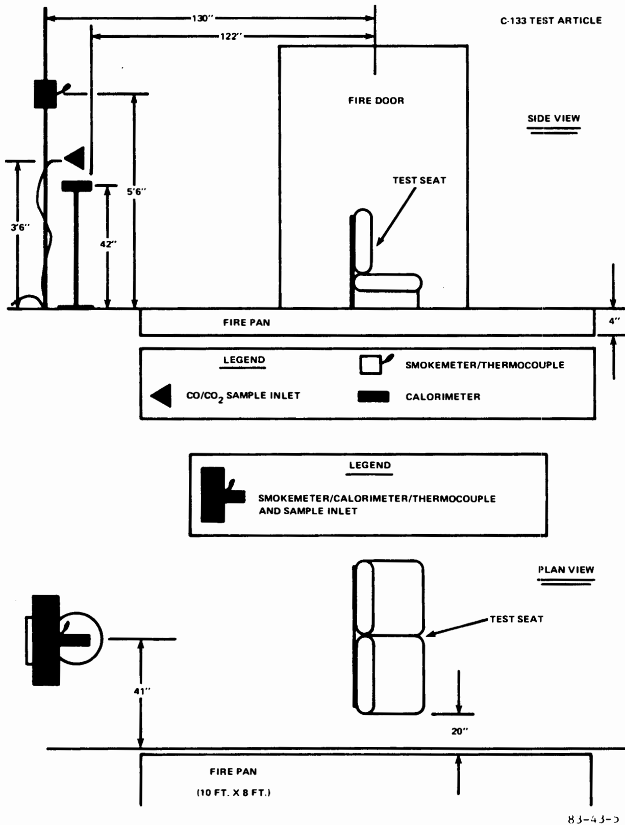
FIGURE 5. POST-CRASH SERIES ONE CONFIGURATION
