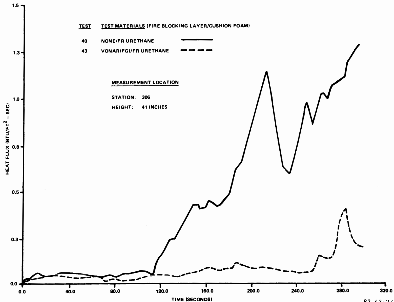
FIGURE 27. POST-CRASH SERIES FIVE HEAT FLUX COMPARISON
