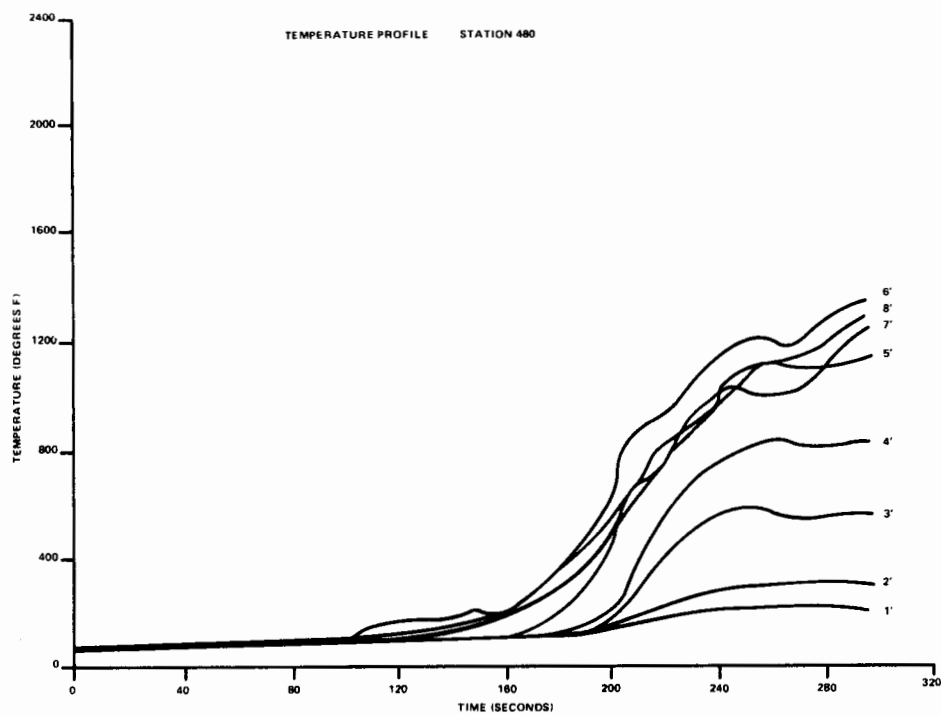
FIGURE C-2. TEMPERATURE PROFILE STATION 480 (1 of 2 Sheets)
