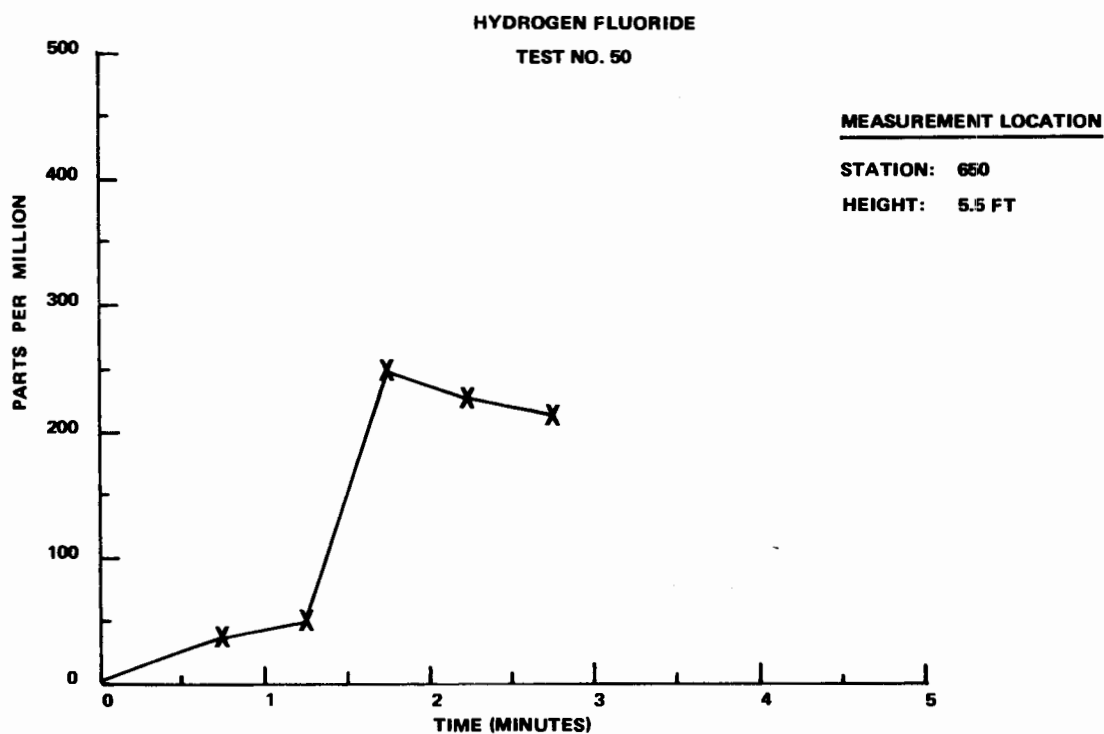
FIGURE 53. FULL-SCALE IN-FLIGHT ACID GAS MEASUREMENTS
