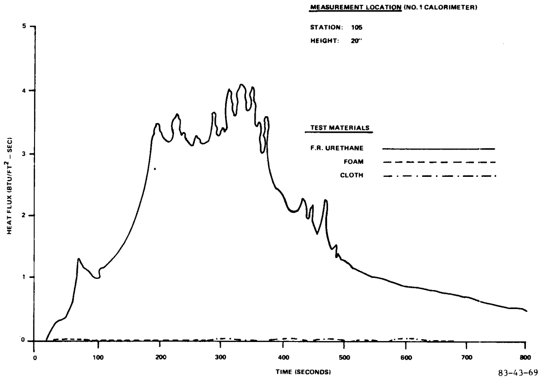
FIGURE 69. RAMP FIRE BLOCKING LAYER HEAT FLUX COMPARISON
