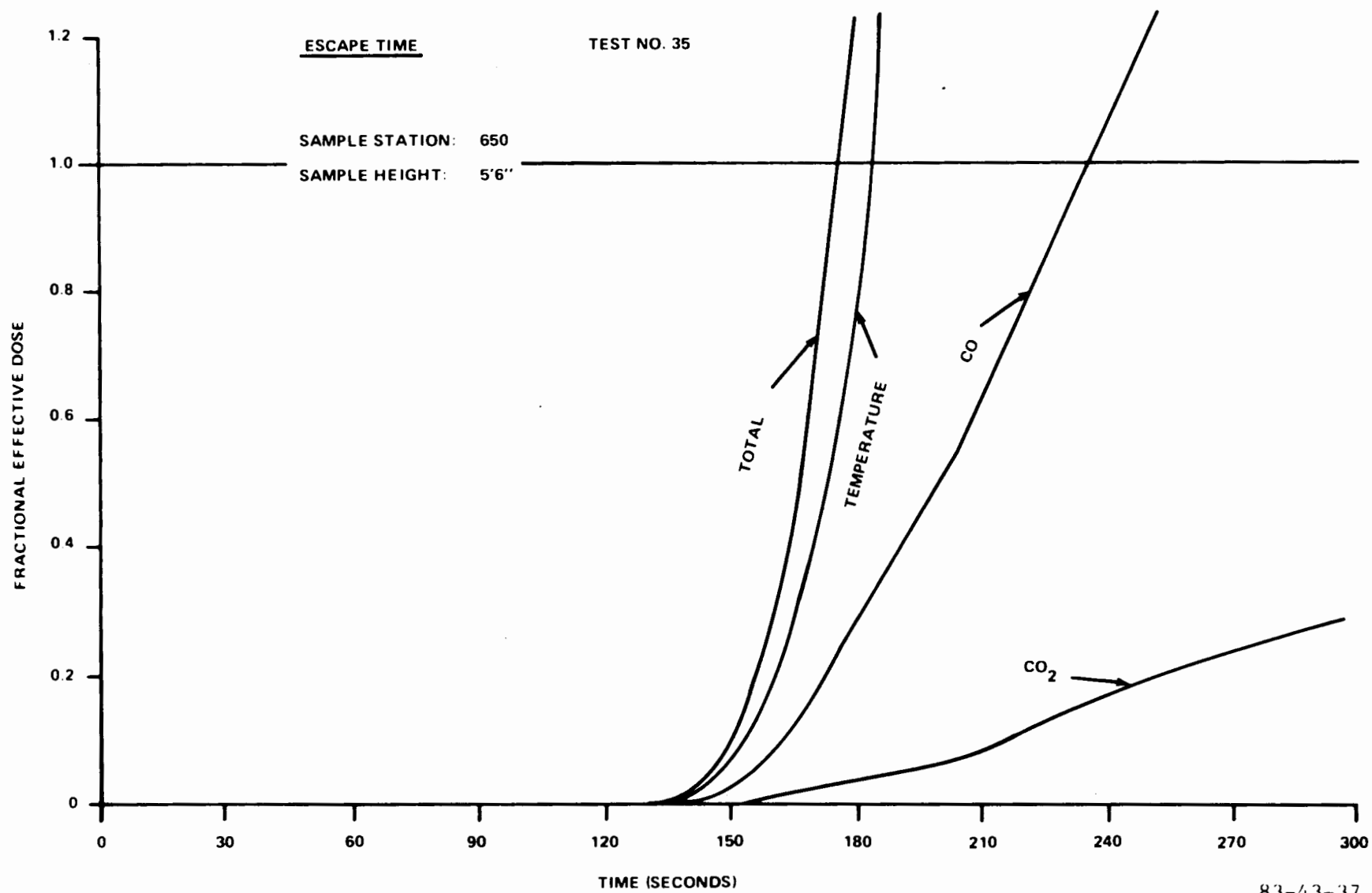
FIGURE 37. FRACTIONAL EFFECTIVE DOSE PLOT FOR TEST NUMBER 35 ( NO HCl, HF, HCN)
