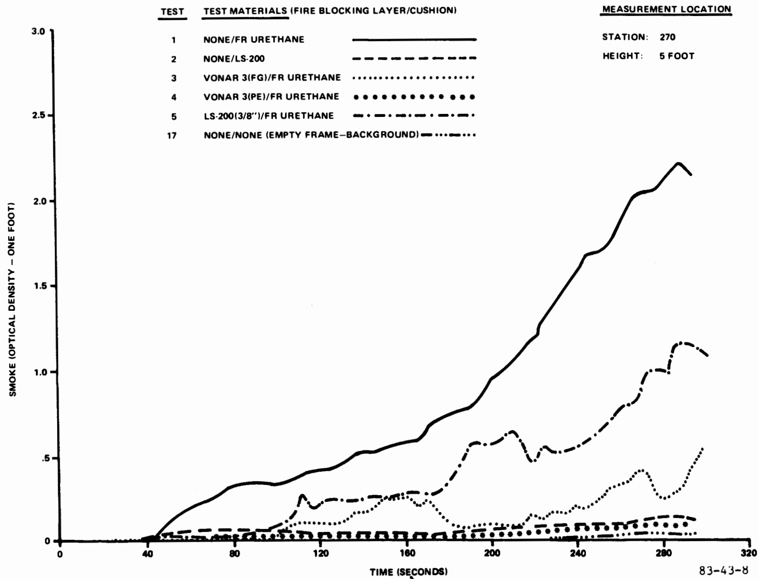
FIGURE 8. POST-CRASH SERIES ONE SMOKE COMPARISON
