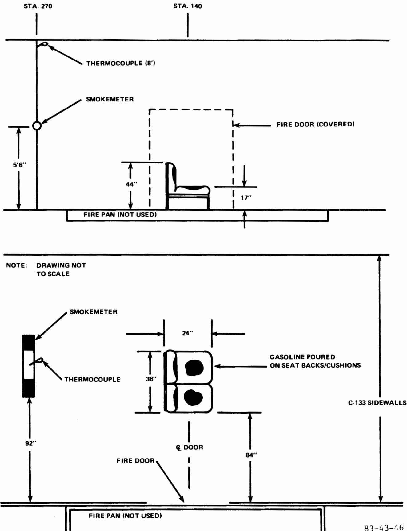
FIGURE 46. IN-FLIGHT GASOLINE TEST CONFIGURATIONS
