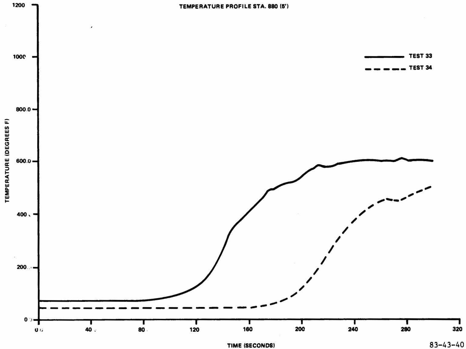
FIGURE 40. TEMPERATURE COMPARISON OF FULL-SCALE TESTS WITH AND WITHOUT WIND
