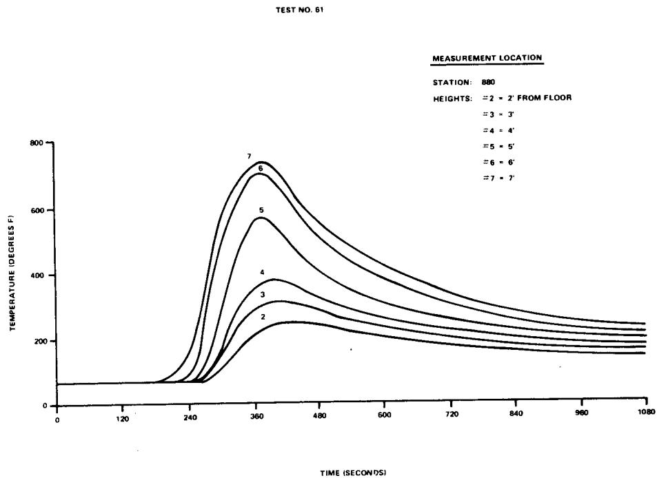
FIGURE 52. FULL-SCALE IN-FLIGHT TEMPERATURE PROFILE
