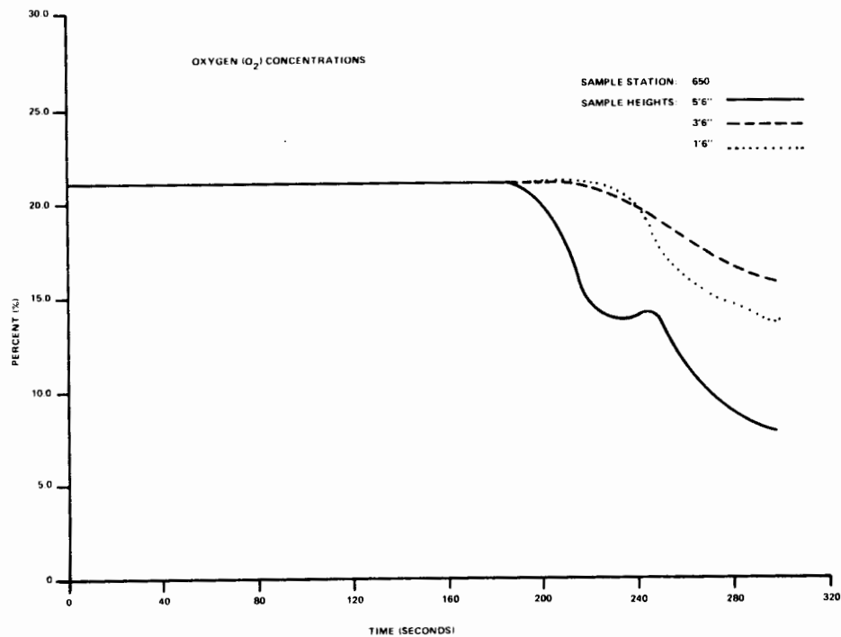
FIGURE C-9. O_2 PROFILE STATION 650 (1 of 2 Sheets)
