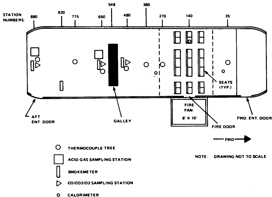
FIGURE 29. INSTALLATION OF WIDE-BODY MATERIALS INSIDE C-133 TEST ARTICLE
