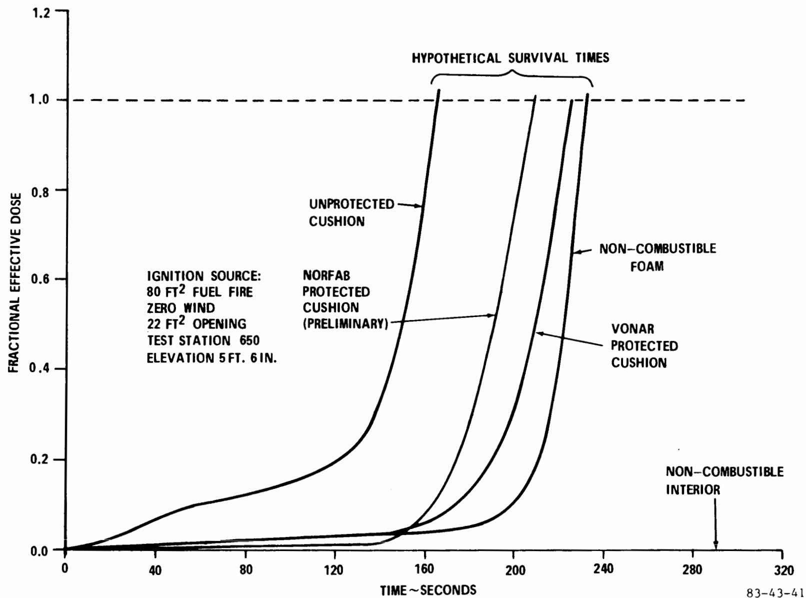
FIGURE 41. EFFECT OF CUSHIONING PROTECTION ON CALCULATED SURVIVAL TIME UNDER FULL-SCALE POST-CRASH FIRE CONDITIONS
