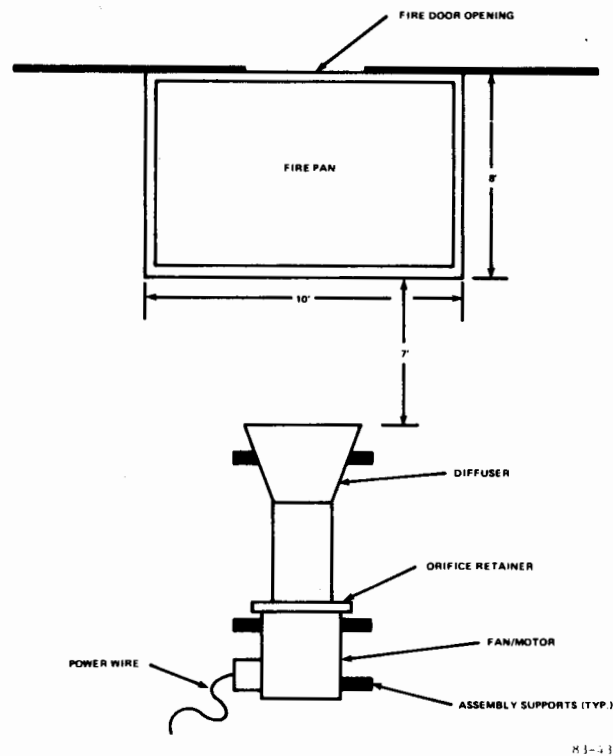
FIGURE 2. SIMULATED WIND CONFIGURATION
