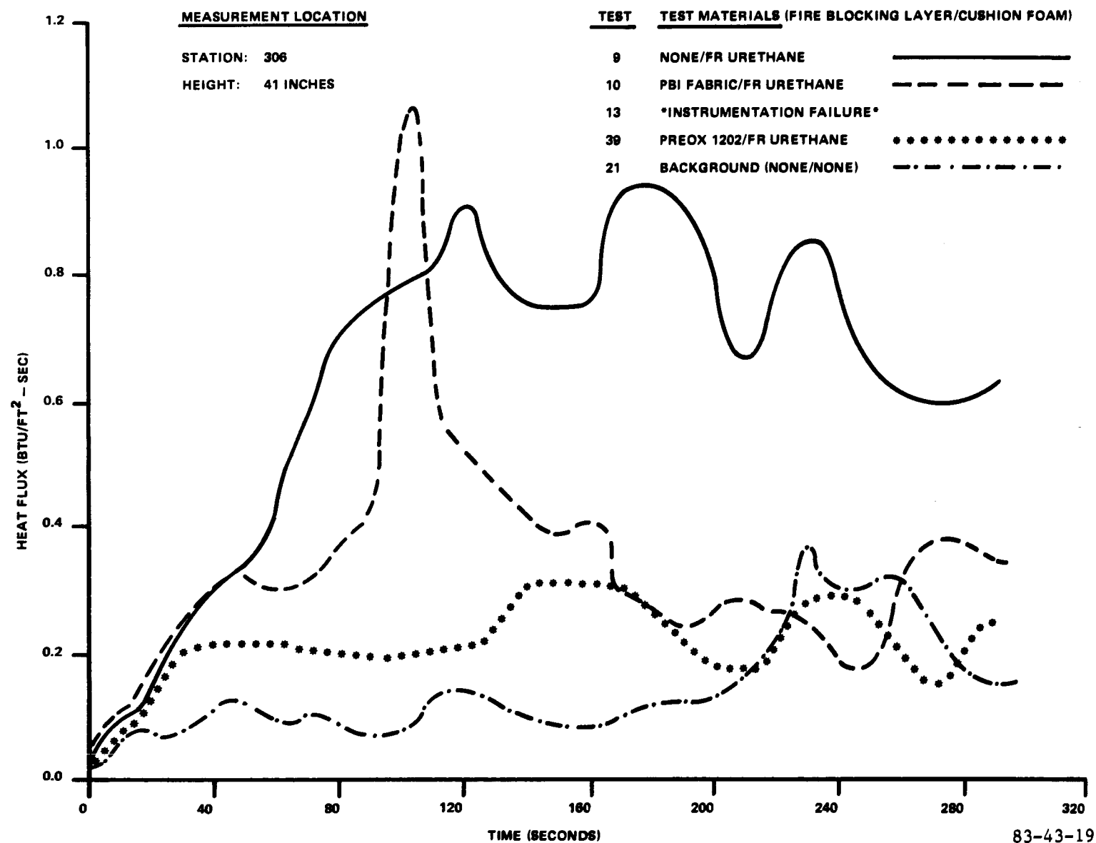
FIGURE 19. POST-CRASH SERIES THREE HEAT FLUX COMPARISON
