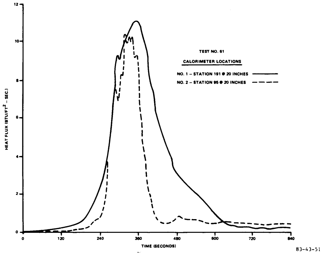
FIGURE 51. FULL-SCALE IN-FLIGHT HEAT FLUX
