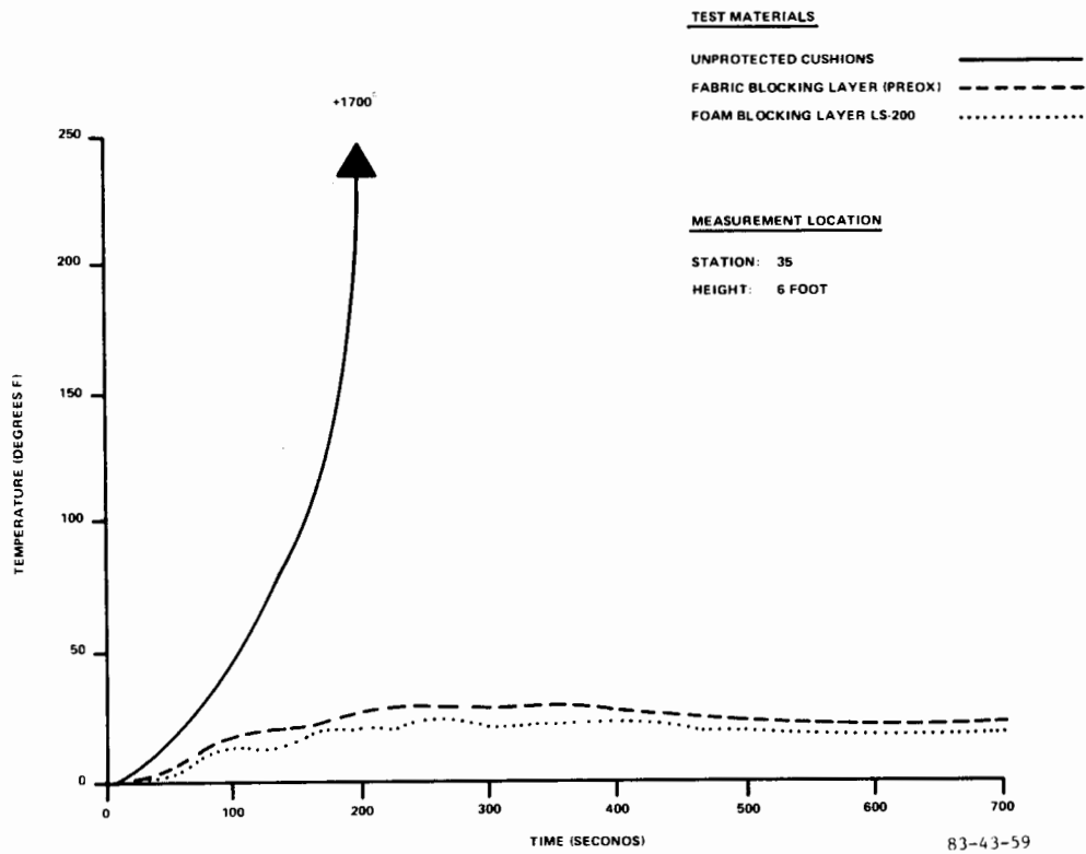
FIGURE 59. FULL-SCALE IN-FLIGHT BLOCKING LAYER COMPARISON TEMPERATURE
