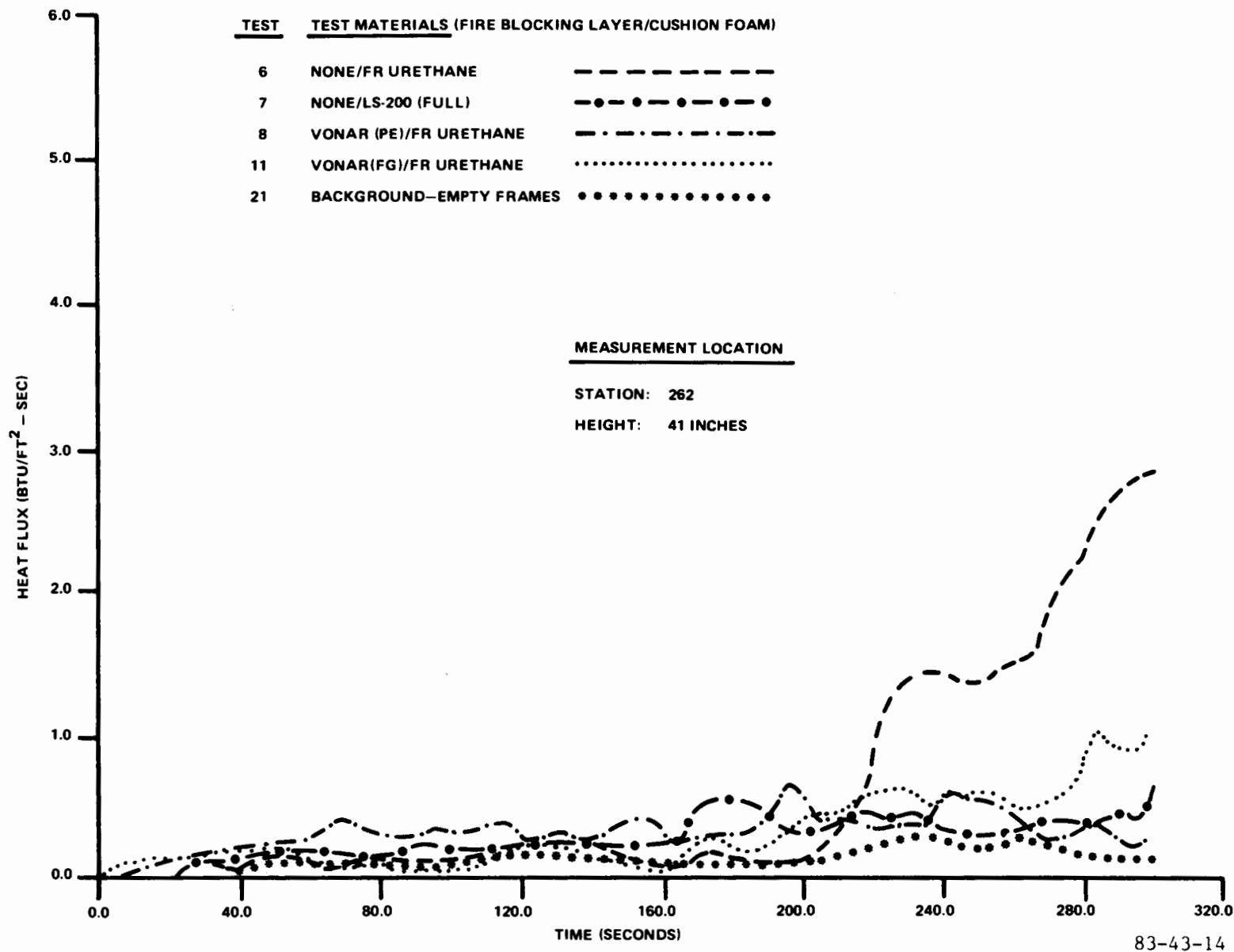
FIGURE 14. POST-CRASH SERIES TWO HEAT FLUX COMPARISON
