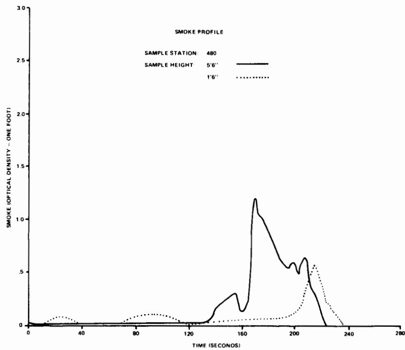
FIGURE C-4. SMOKE PROFILE STATION 480 (2 of 2 Sheets)
