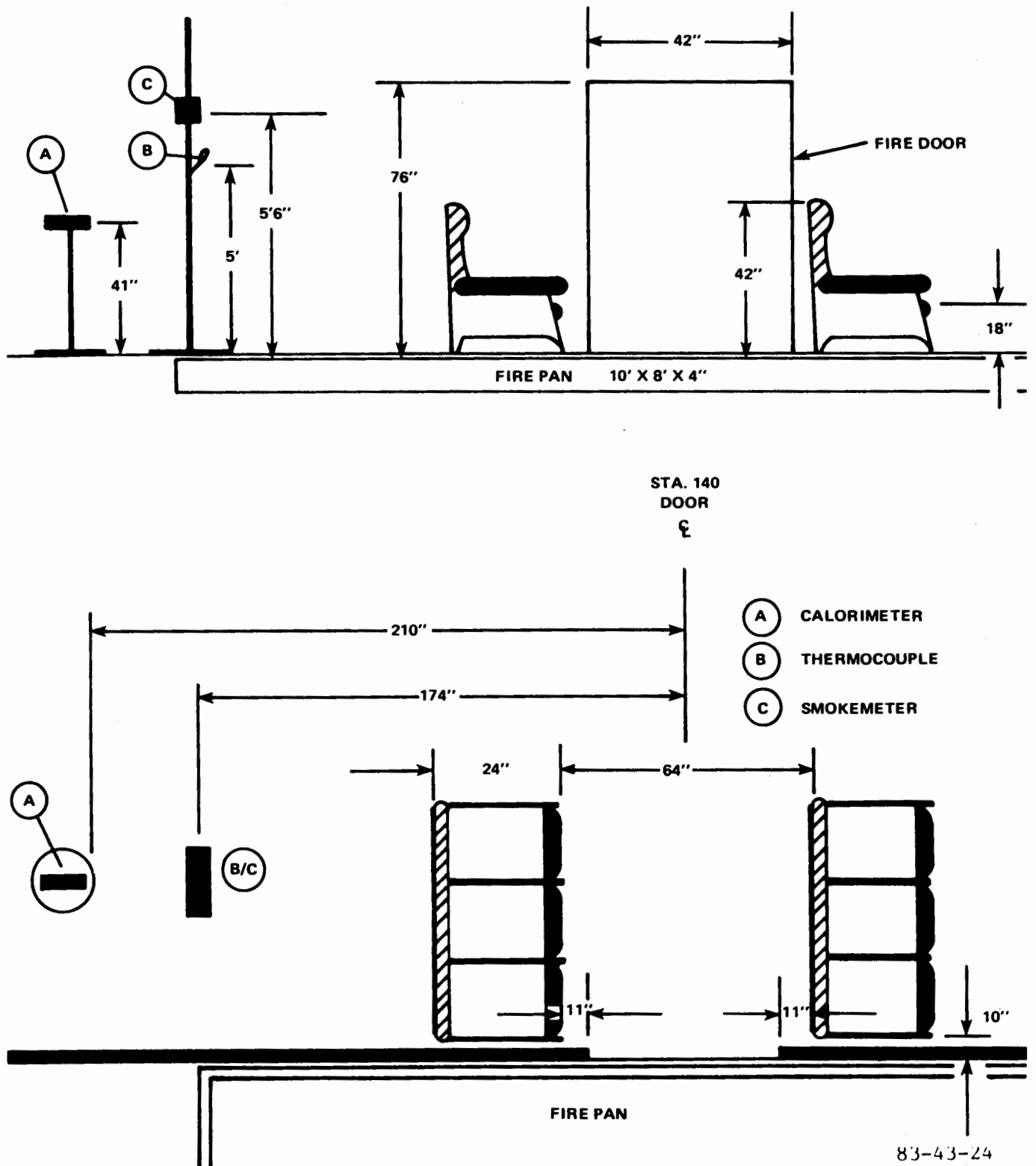
FIGURE 24. POST-CRASH SERIES FIVE CONFIGURATION
