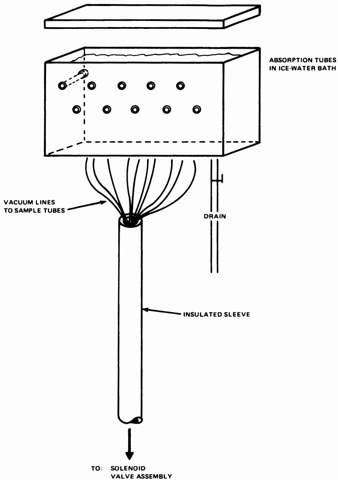
FIGURE B-1. C133 ACID GAS SAMPLING STATION
