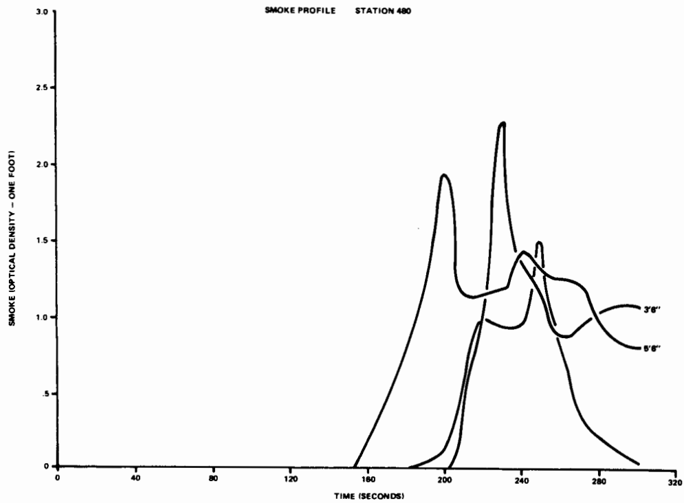
FIGURE C-4. SMOKE PROFILE STATION 480 (1 of 2 Sheets)
