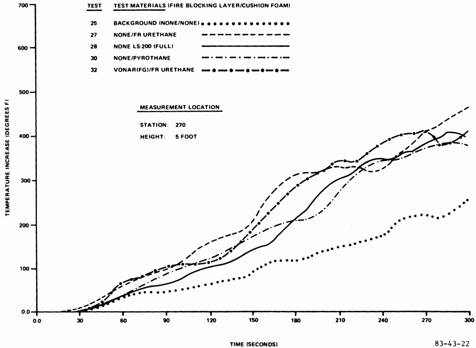
FIGURE 22. POST-CRASH SERIES FOUR TEMPERATURE COMPARISON
