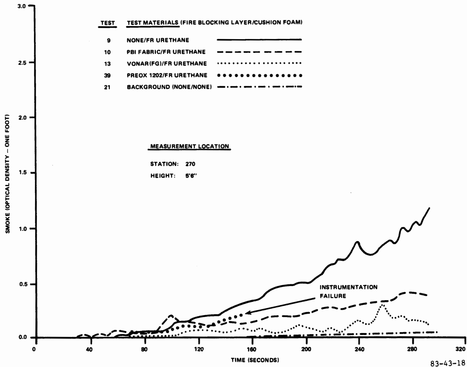
FIGURE 18. POST-CRASH SERIES THREE SMOKE COMPARISON
