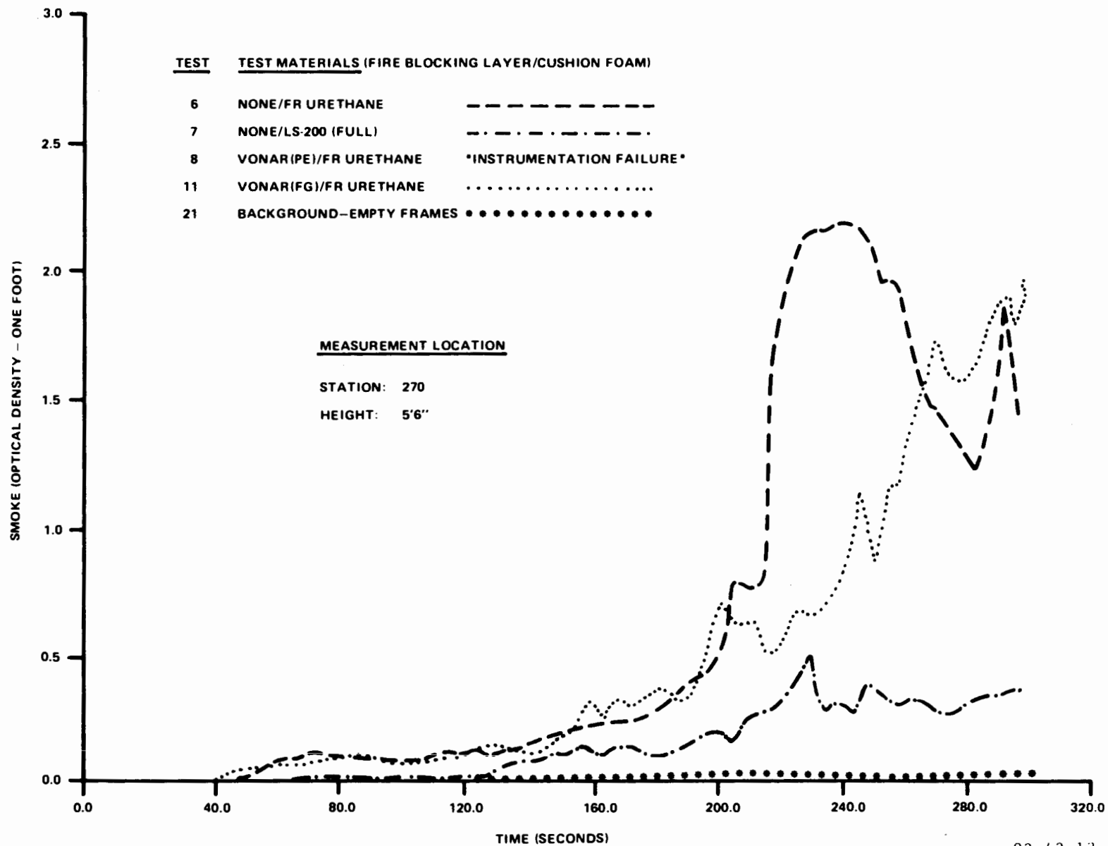
FIGURE 13. POST-CRASH SERIES TWO SMOKE COMPARISON
