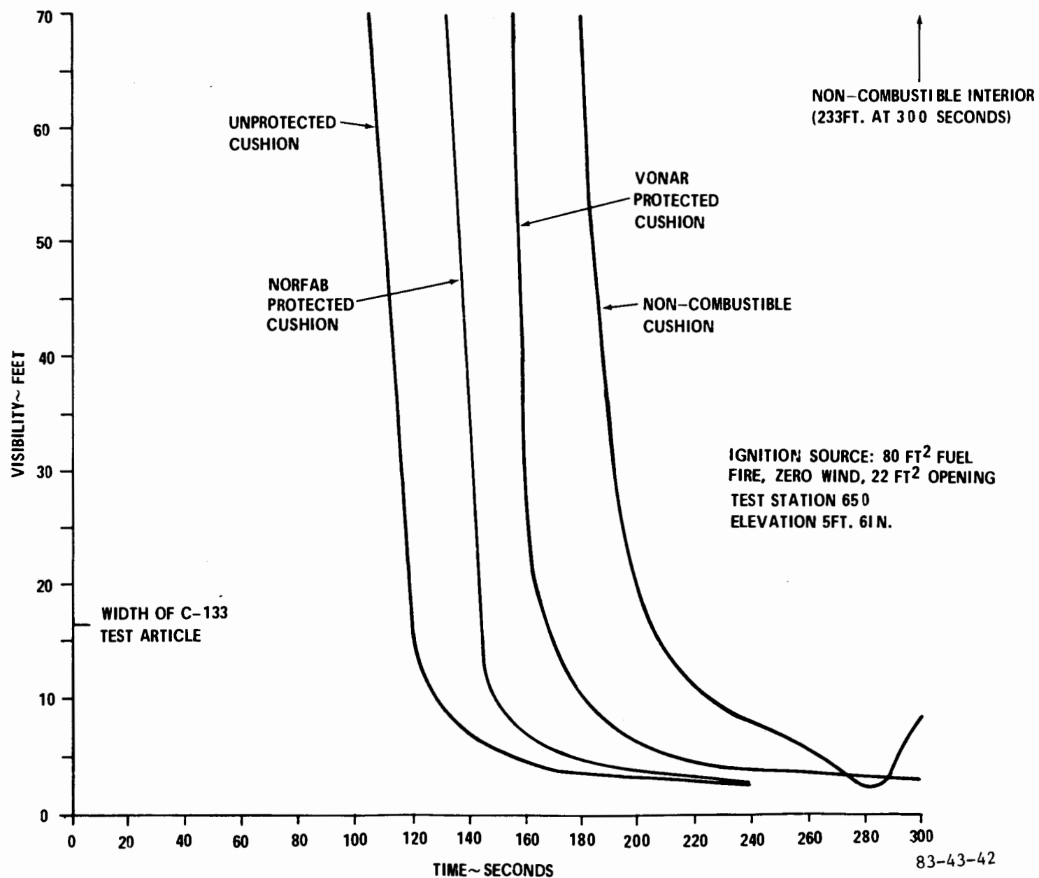
FIGURE 42. EFFECT OF CUSHIONING PROTECTION ON CALCULATED VISIBILITY THROUGH SMOKE UNDER FULL-SCALE POST-CRASH FIRE CONDITIONS
