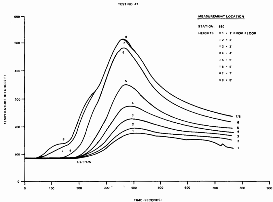
FIGURE 64. RAMP FIRE TEMPERATURE PROFILES (2 of 2 Sheets)
