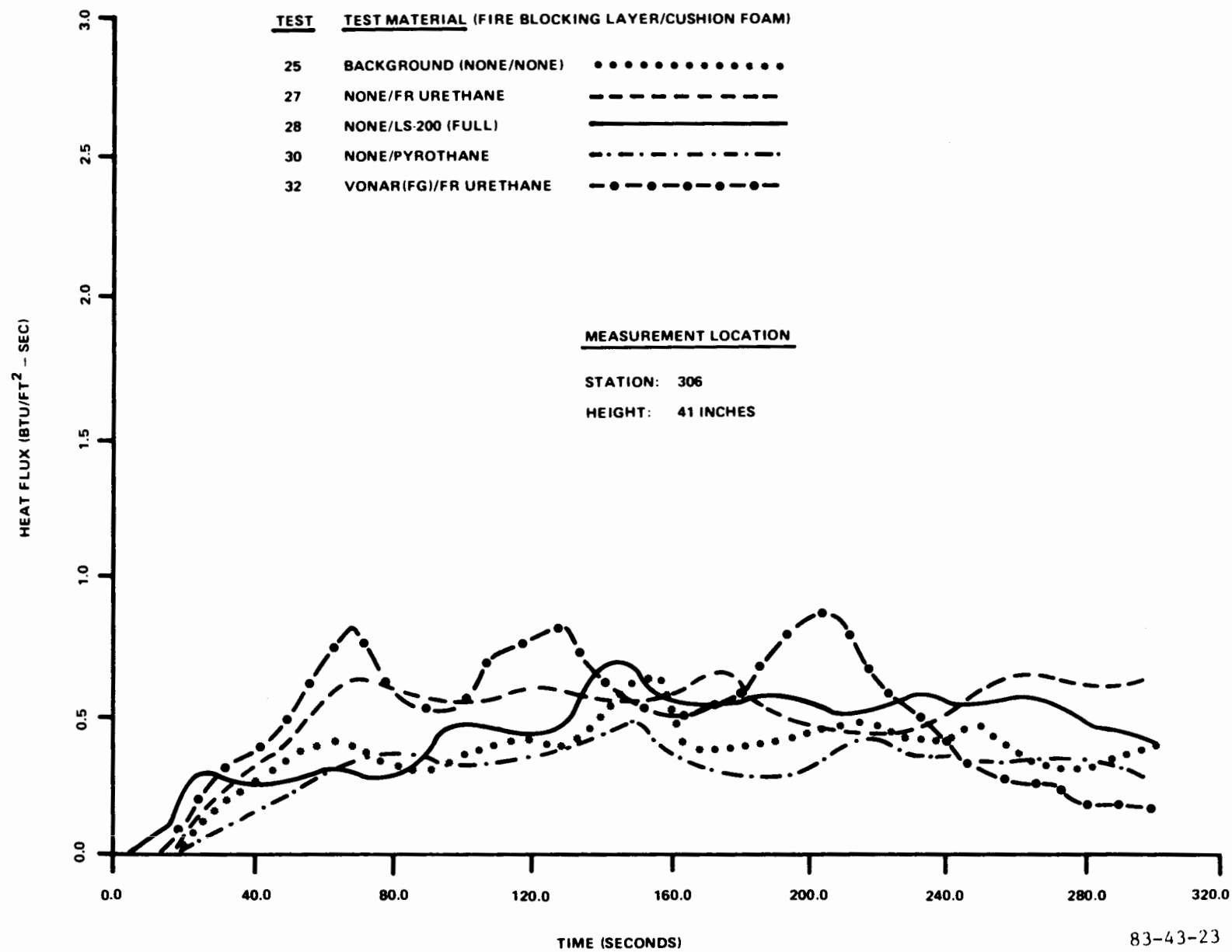
FIGURE 23. POST-CRASH SERIES FOUR HEAT FLUX COMPARISON
