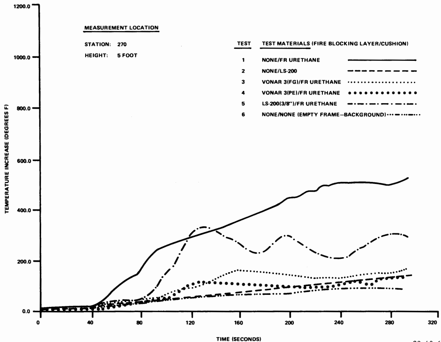
FIGURE 6. POST-CRASH SERIES ONE TEMPERATURE COMPARISON
