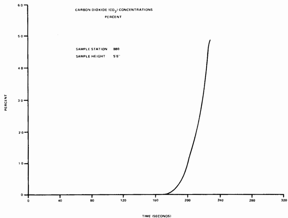
FIGURE C-6. CO 2 PROFILE STATION 880 (1 of 2 Sheets)
