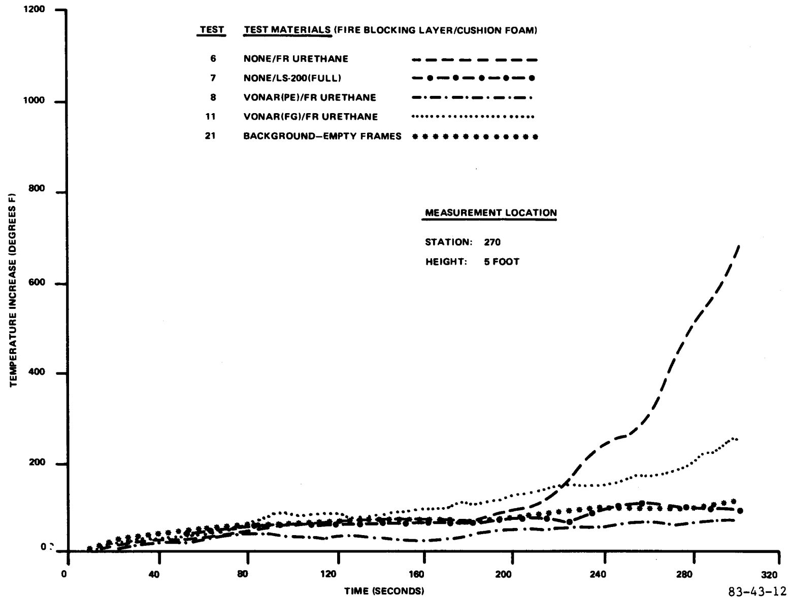
FIGURE 12. POST-CRASH SERIES TWO TEMPERATURE COMPARISON
