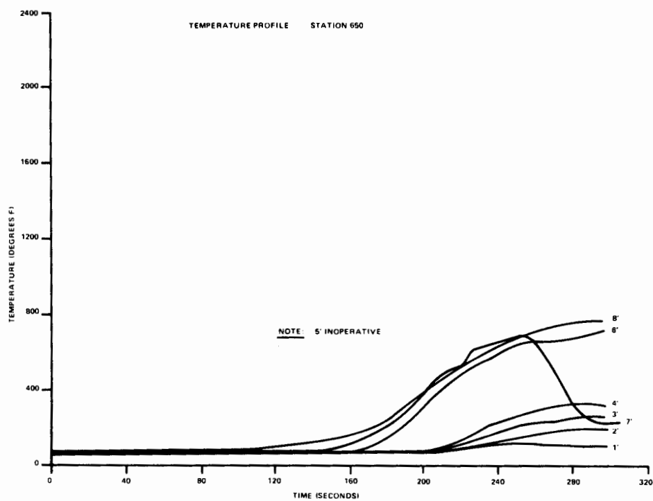
FIGURE C-3. TEMPERATURE PROFILE STATION 650 (1 of 2 Sheets)
