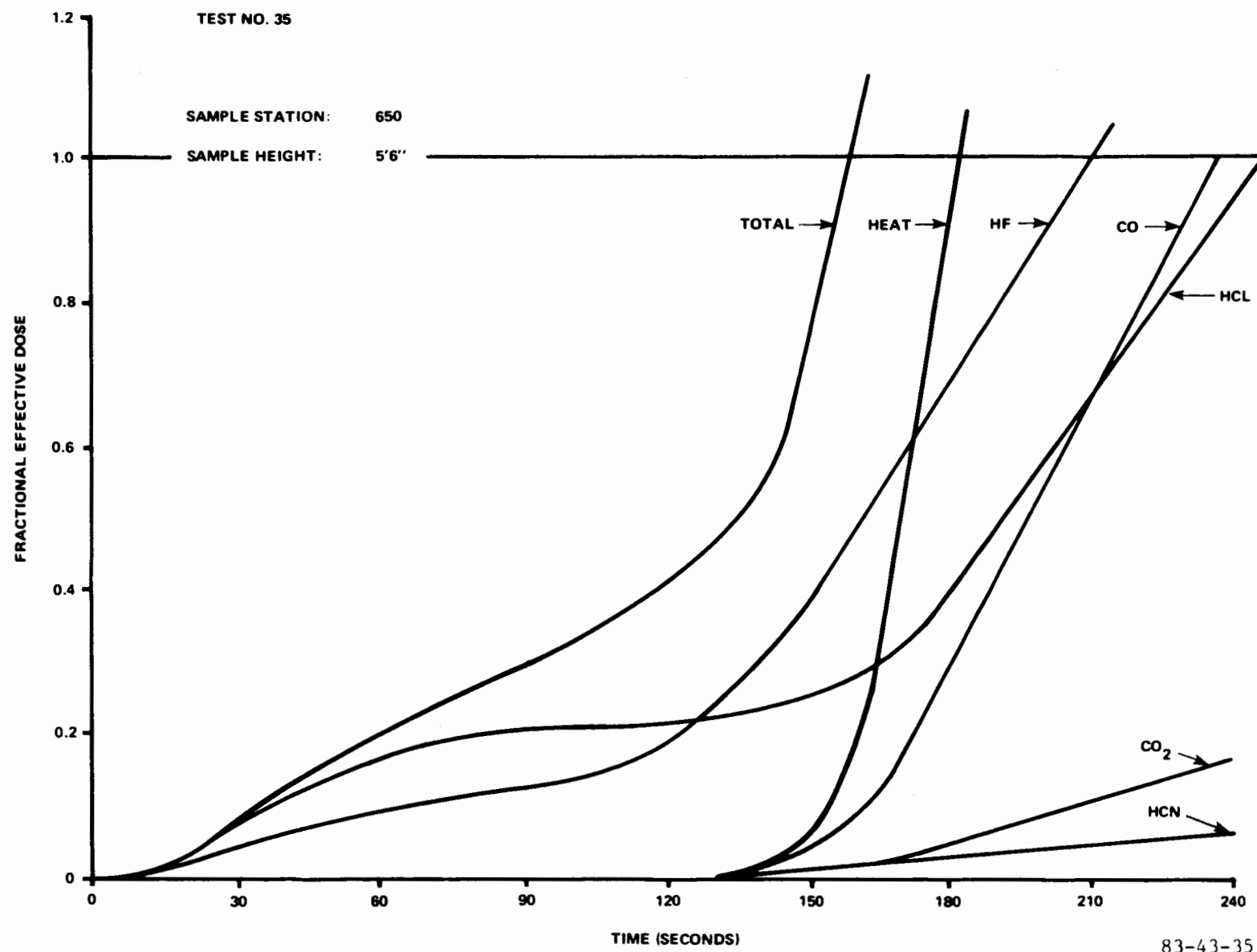
FIGURE 35. FRACTIONAL EFFECTIVE DOSE PLOT FOR TEST NUMBER 35 (ALL HAZARDS)
