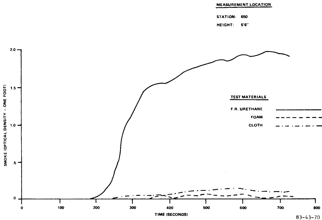
FIGURE 70. RAMP FIRE BLOCKING LAYER SMOKE COMPARISON
