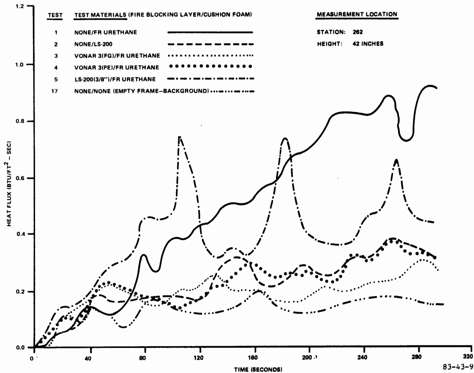
FIGURE 9. POST-CRASH SERIES ONE HEAT FLUX COMPARISON
