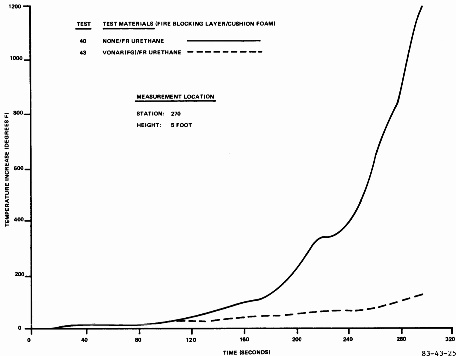
FIGURE 25. POST-CRASH SERIES FIVE TEMPERATURE COMPARISON
