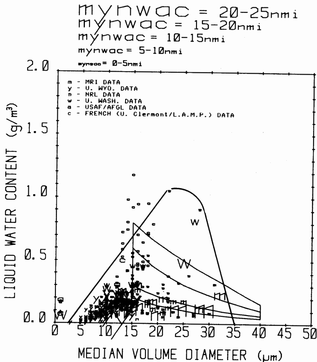
FIGURE 24. SCATTERPLOT OF OBSERVED LWC, MVD COMBINATIONS IN THE MODERN DATA FOR LAYER CLOUDS UP TO 10,000 FT AGL AND FOR CLOUD TEMPERATURES FROM -10^{\circ}C to 0^{\circ}C . The various plotting symbols represent different data sources as indicated in the key. The size of each plotted symbol is proportional to its statistical weight (i.e., the observed horizontal extent of the associated icing event) as shown by the scale above the graph. The center of each plotted symbol corresponds to the average (and approximately constant) value of LWC and MVD observed during the icing event. Values of LWC for which no MVD measurements are available are plotted arbitrarily at 1 \mu m MVD. A total of 1320 data miles is represented in this graph. The Continuous Maximum envelope from FIG. 1 of FAR-25, App. C, is superimposed for comparison. The other smooth curve is the observed, apparent limit to the CONUS data for this temperature interval.
