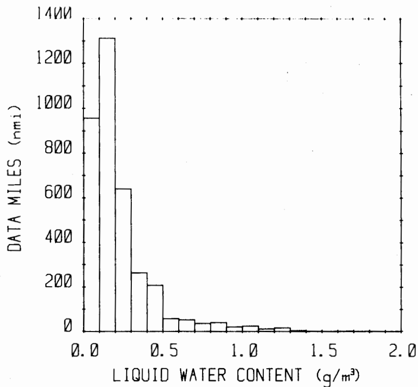
FIGURE 18. FREQUENCY DISTRIBUTION OF LWC IN ALL SUPERCOOLED CLOUD TYPES BELOW 10,000 FT AGL AS OBSERVED IN THE MODERN DATA. A total of 3645 data miles is represented in this Figure.
