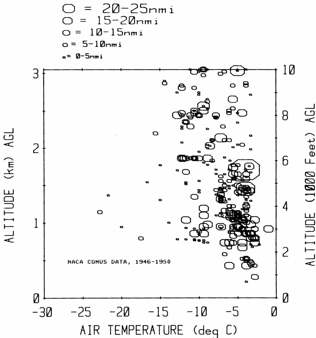
FIGURE 30. SCATTERPLOT OF ICING EVENT TEMPERATURES VS. ALTITUDE FOR NACA DATA FROM SUPERCOOLED LAYER CLOUDS (St, Sc, Ns, As, Ac) UP TO 10,000 FT AGL. The size of each symbol is proportional to its statistical weight (i.e., the observed horizontal extent of the associated icing event) as shown by the scale above the graph. The center of each symbol corresponds to the average (and approximately constant) value of altitude and OAT observed during the icing event. A total of 2610 data miles is represented in this graph.
