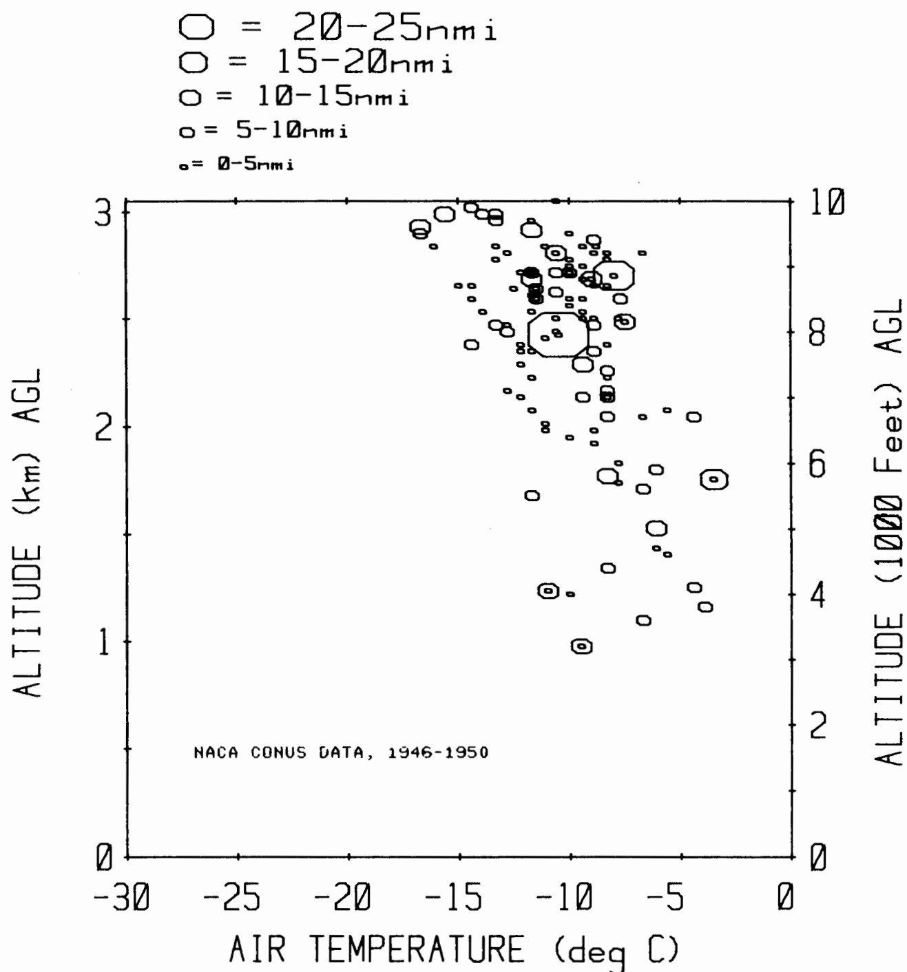
FIGURE 32. SCATTERPLOT OF ICING EVENT TEMPERATURES VS. ALTITUDE FOR NACA DATA FROM SUPERCOOLED CONVECTIVE CLOUDS (Cu, Cb) UP TO 10,000 FT AGL. The size of each symbol is proportional to its statistical weight (i.e., the observed horizontal extent of the associated icing event) as shown by the scale above the graph. The center of each symbol corresponds to the average (and approximately constant) value of altitude and OAT observed during the icing event. A total of 620 data miles is represented in this graph.
