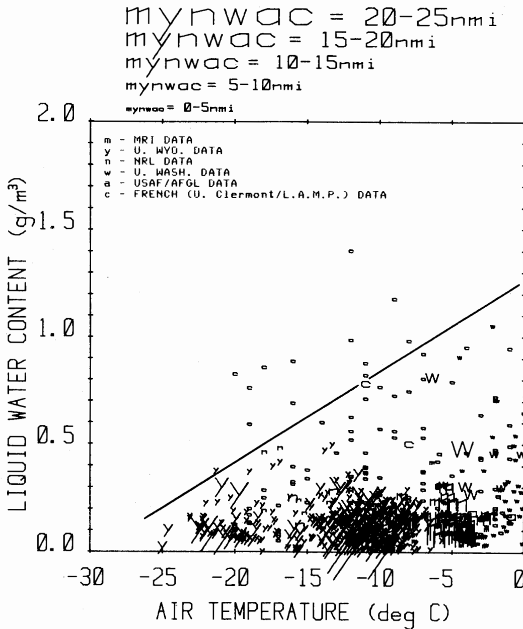
FIGURE 33. SCATTERPLOT OF LWC VS. OAT FOR MODERN DATA FROM SUPERCOOLED LAYER CLOUDS (St, Sc, Ns, As, Ac) UP TO 10,000 FT AGL. The various plotting symbols represent different data sources as indicated in the key. The size of each symbol is proportional to its statistical weight (i.e., the observed horizontal extent of the associated icing event) as shown by the scale above the graph. The center of each symbol corresponds to the average (and approximately constant) value of LWC and OAT observed during the icing event. The solid line represents the apparent upper limit to LWC as a function of temperature for CONUS supercooled layer clouds below 10,000 ft AGL. The position of the line is based on the maximum LWC values in the combined NACA and modern CONUS data sets. A total of 2660 data miles is represented in this graph.
