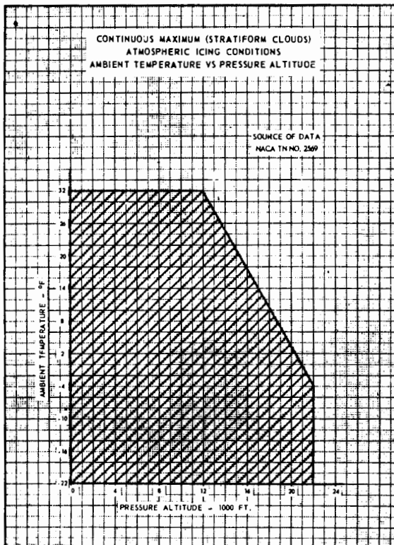
FIGURE 2. CONTINUOUS MAXIMUM ENVELOPE OF TEMPERATURE VS. ALTITUDE (FROM FAR-25, APP. C.)
