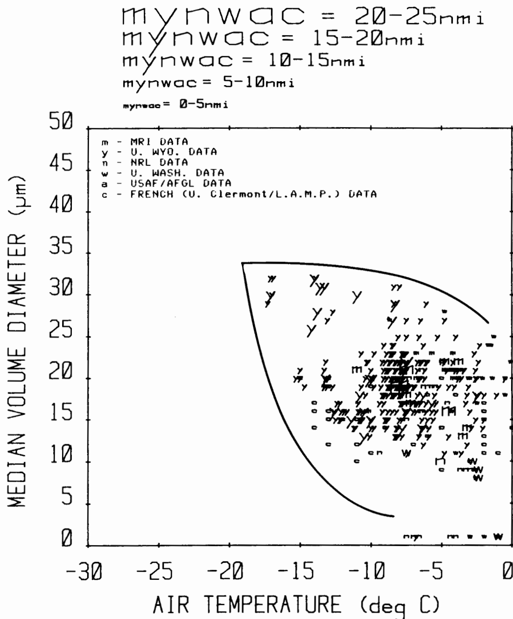
FIGURE 40. SCATTERPLOT OF MVD VS. OAT FOR MODERN DATA FROM SUPERCOOLED CONVECTIVE CLOUDS (Cu, Cb) UP TO 10,000 FT AGL. The various plotting symbols represent different data sources as indicated in the key. The size of each symbol is proportional to its statistical weight (i.e., the observed horizontal extent of the associated icing event) as shown by the scale above the graph. The center of each symbol corresponds to the average (and approximately constant) value of MVD and OAT observed during the icing event. The solid line bounding the data points represents the apparent upper and lower limit to MVD as a function of temperature for supercooled convective clouds below 10,000 ft AGL. The position of the line is based on extreme MVD values in both the NACA and modern data sets. The data points plotted at 1 \mu m MVD are those for which the MVD values are actually unknown. A total of 980 data miles is represented in this graph.
