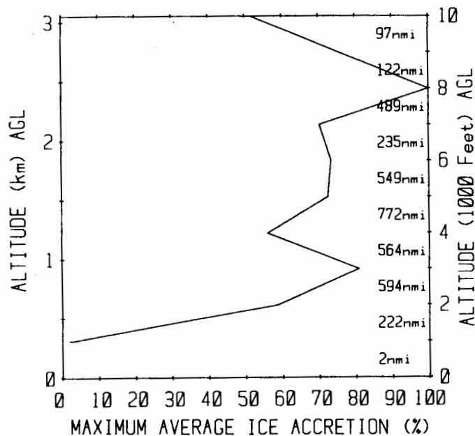
FIGURE 15. ALTITUDE VARIATION OF AVERAGE ICE ACCRETION PER EXTENDED ICING ENCOUNTER AS DETERMINED FROM THE MODERN DATA. Ice accretion amounts represented by the product \bar{W}H are computed for all extended icing encounters occurring in each 1000 ft altitude interval. The average value of \bar{W}H for each altitude interval is expressed as a percentage of the largest of these interval-wide averages. At each 1000 ft level the plotted line indicates this percentage value for the 1000 ft altitude interval immediately below. An extended encounter is a series of consecutive icing events added together sequentially until a gap of some specified duration (3 nmi for this case) is reached. \bar{W} is the LWC averaged over the extended encounter (gaps not included) and H is the horizontal extent of the extended encounter (gaps not included). The right-hand column of numbers gives the number of data miles contributing within each 1000 ft interval. A total of 3645 data miles is represented in this Figure.
