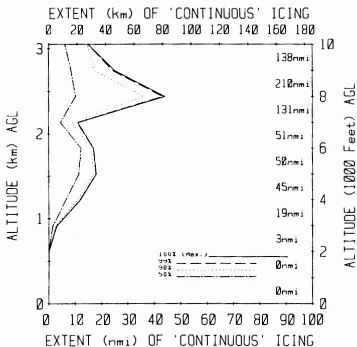
FIGURE 12. ALTITUDE VARIATION OF HORIZONTAL EXTENTS OF EXTENDED ICING ENCOUNTERS IN CONVECTIVE CLOUDS (Cu, Cb) AS OBSERVED IN THE NACA DATA (1946-1950). An extended encounter is a series of consecutive icing events added together sequentially until a gap of some specified duration (3 nmi for this case) is reached. At each 1000 ft level the n th percentile curves indicate the horizontal extent which was unexceeded in n\% of the extended encounters within the 1000 ft altitude interval immediately below. The right-hand column of numbers gives the number of data miles contributing within each 1000 ft interval. A total of 650 data miles is represented in this Figure.
