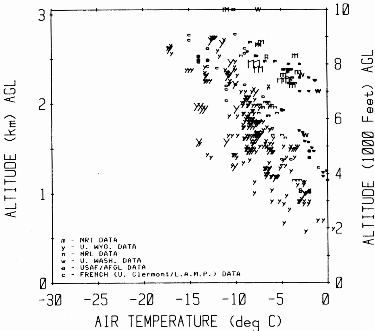
FIGURE 31. SCATTERPLOT OF ICING EVENT TEMPERATURES VS. ALTITUDE FOR MODERN DATA FROM SUPERCOOLED CONVECTIVE CLOUDS (Cu, Cb) UP TO 10,000 FT AGL. The various plotting symbols represent different data sources as indicated in the key. The size of each symbol is proportional to its statistical weight (i.e., the observed horizontal extent of the associated icing event) as shown by the scale above the graph. The center of each symbol corresponds to the average (and approximately constant) value of altitude and OAT observed during the icing event. A total of 980 data miles is represented in this graph.
