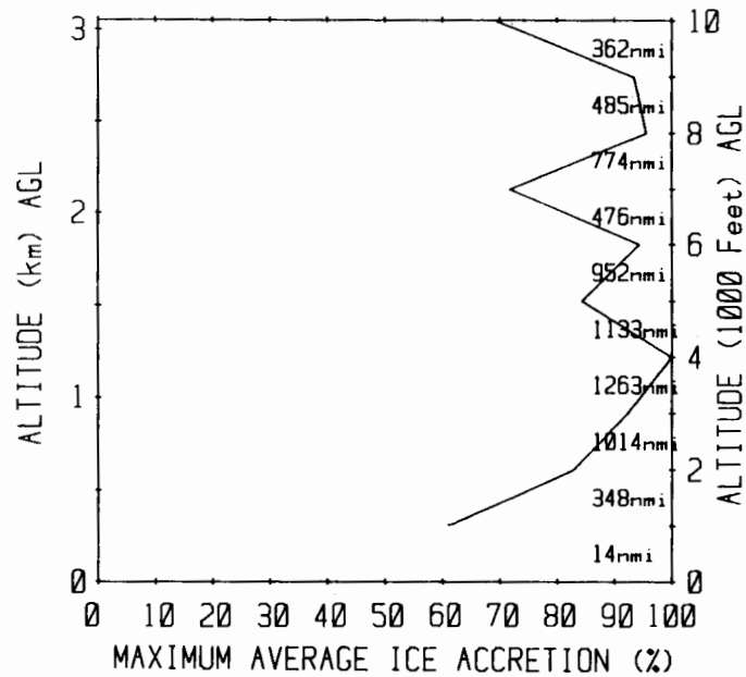
FIGURE 16. ALTITUDE VARIATION OF AVERAGE ICE ACCRETION PER EXTENDED ICING ENCOUNTER AS DETERMINED FROM THE COMBINED NACA AND MODERN DATA. Ice accretion amounts represented by the product WH are computed for all extended icing encounters occurring in each 1000 ft altitude interval. The average value of WH for each altitude interval is expressed as a percentage of the largest of these interval-wide averages. At each 1000 ft level the plotted line indicates this percentage value for the 1000 ft altitude interval immediately below. An extended encounter is a series of consecutive icing events added together sequentially until a gap of some specified duration (3 nmi for this case) is reached. W is the LWC averaged over the extended encounter (gaps not included) and H is the horizontal extent of the extended encounter (gaps not included). The right-hand column of numbers gives the number of data miles contributing within each 1000 ft interval. A total of 6820 data miles is represented in this Figure.
