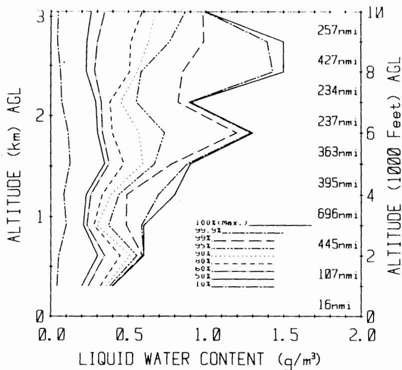
FIGURE 7. ALTITUDE VARIATION OF SUPERCOOLED LWC FOR ALL CLOUD TYPES AS OBSERVED IN THE NACA DATA (1946-1950). At each 1000 ft level the n th percentile curves indicate the value of LWC that was unexceeded in n\% of the data miles recorded in supercooled clouds within the 1000 ft altitude interval immediately below. The right-hand column of numbers gives the number of data miles accumulated within each 1000 ft interval. A total of 3170 data miles is represented in this Figure.
