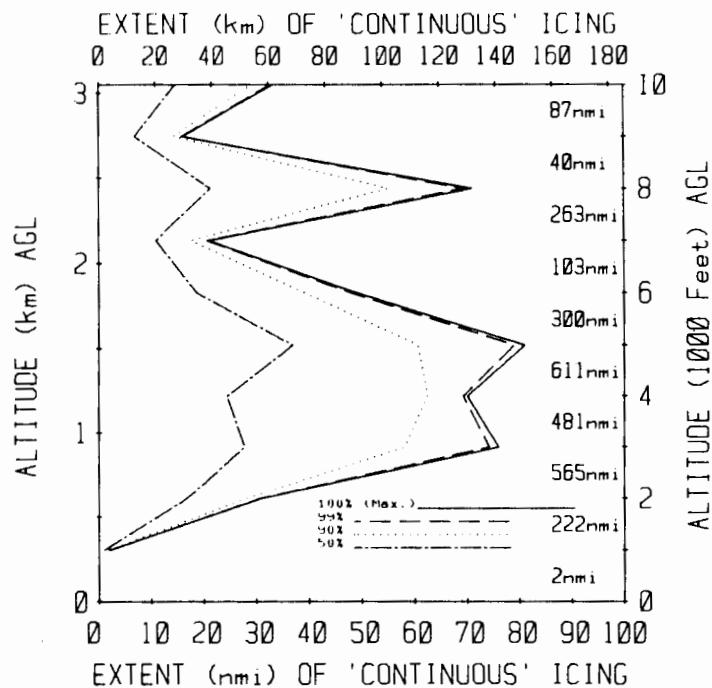
FIGURE 11. ALTITUDE VARIATION OF HORIZONTAL EXTENTS OF EXTENDED ICING ENCOUNTERS IN LAYER CLOUDS (St, Sc, Ns, As, Ac) AS OBSERVED IN THE MODERN DATA. An extended encounter is a series of consecutive icing events added together sequentially until a gap of some specified duration (3 nmi for this case) is reached. At each 1000 ft level the n th percentile curves indicate the horizontal extent which was unexceeded in n\% of the extended encounters within the 1000 ft altitude interval immediately below. The right-hand column of numbers give the number of data miles contributing within each 1000 ft interval. A total of 2675 data miles is represented in this Figure.
