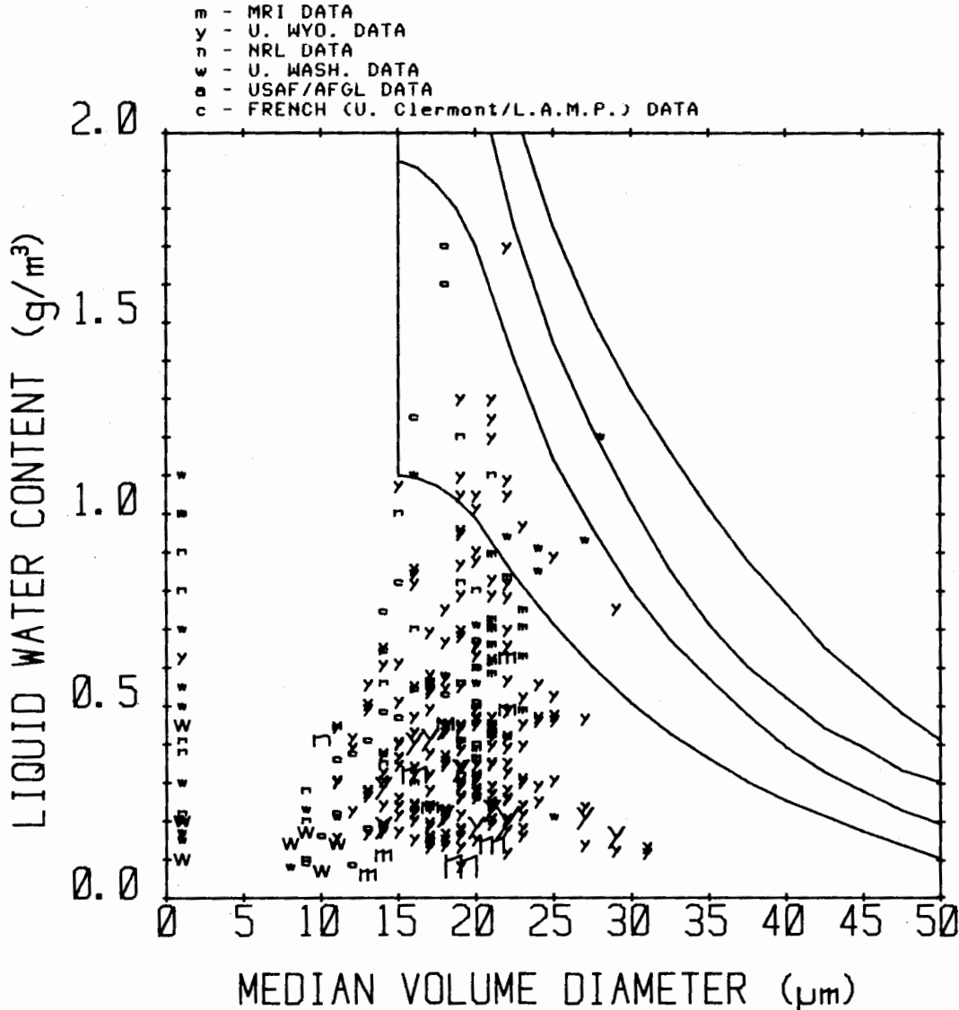
FIGURE 27. SCATTERPLOT OF OBSERVED LWC, MVD COMBINATIONS IN THE MODERN DATA FOR CONVECTIVE CLOUDS UP TO 10,000 FT AGL AND FOR CLOUD TEMPERATURES FROM -10^{\circ}\text{C} to 0^{\circ}\text{C} . The various plotting symbols represent different data sources as indicated by the key. The size of each plotted symbol is proportional to its statistical weight (i.e., the observed horizontal extent of the associated icing event) as shown by the scale above the graph. The center of each plotted symbol corresponds to the average (and approximately constant) value of LWC and MVD observed during the icing event. Values of LWC for which no MVD measurements are available are plotted arbitrarily at 1\text{ }\mu\text{m} MVD. A total of 734 data miles is represented in this graph. The Intermittent Maximum envelope from FIG. 4 of FAR-25, App. C, is superimposed for comparison.
