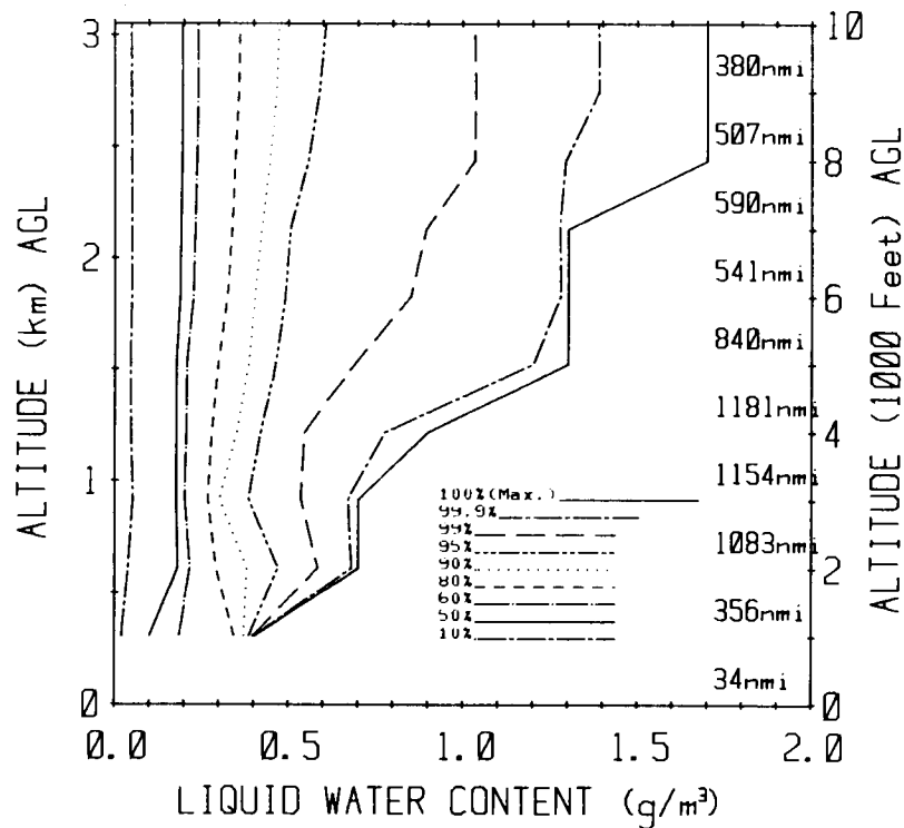
FIGURE 9. CUMULATIVE VARIATION WITH ALTITUDE FOR SUPERCOOLED LWC FROM ALL CLOUD TYPES AS RECORDED IN THE ENTIRE CONUS DATA BASE. At each 1000 ft level the nth percentile curves indicate the value of LWC that was unexceeded in n% of the data miles accumulated at all altitudes below the specified level. The right-hand column of numbers gives the number of data miles recorded within each 1000 ft interval. A total of 6660 data miles is represented in this Figure.
