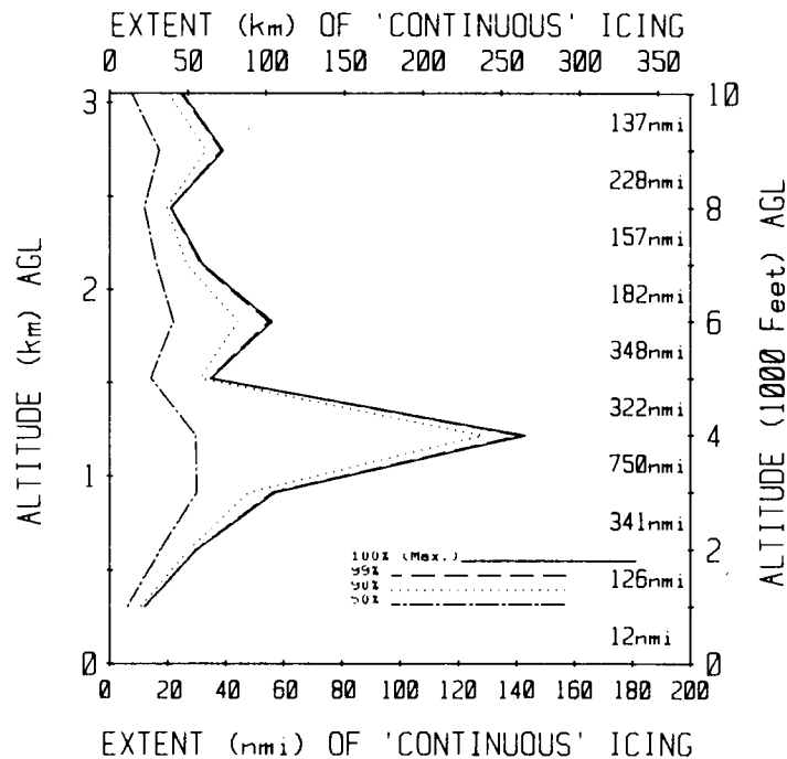
FIGURE 10. ALTITUDE VARIATION OF HORIZONTAL EXTENS OF EXTENDED ICING ENCOUNTERS IN LAYER CLOUDS (St, Sc, Ns, As, Ac) AS OBSERVED IN THE NACA DATA (1946-1950). An extended encounter is a series of consecutive icing events added together sequentially until a gap of some specified duration (3 nmi for this case) is reached. At each 1000 ft level the nth percentile curves indicate the horizontal extent which was unexceeded in n% of the extended encounters within the 1000 ft altitude interval immediately below. The right-hand column of numbers gives the number of data miles contributing within each 1000 ft interval. A total of 2600 data miles is represented in this Figure.
