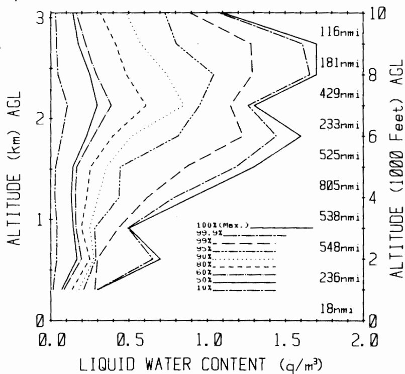
FIGURE 8. ALTITUDE VARIATION OF SUPERCOOLED LWC FOR ALL CLOUD TYPES AS OBSERVED IN THE MODERN DATA. At each 1000 ft level the n th percentile curves indicate the value of LWC that was unexceeded in n\% of the data miles recorded in supercooled clouds within the 1000 ft altitude interval immediately below. The right-hand column of numbers gives the number of data miles accumulated within each 1000 ft interval. A total of 3630 data miles is represented in this Figure.
