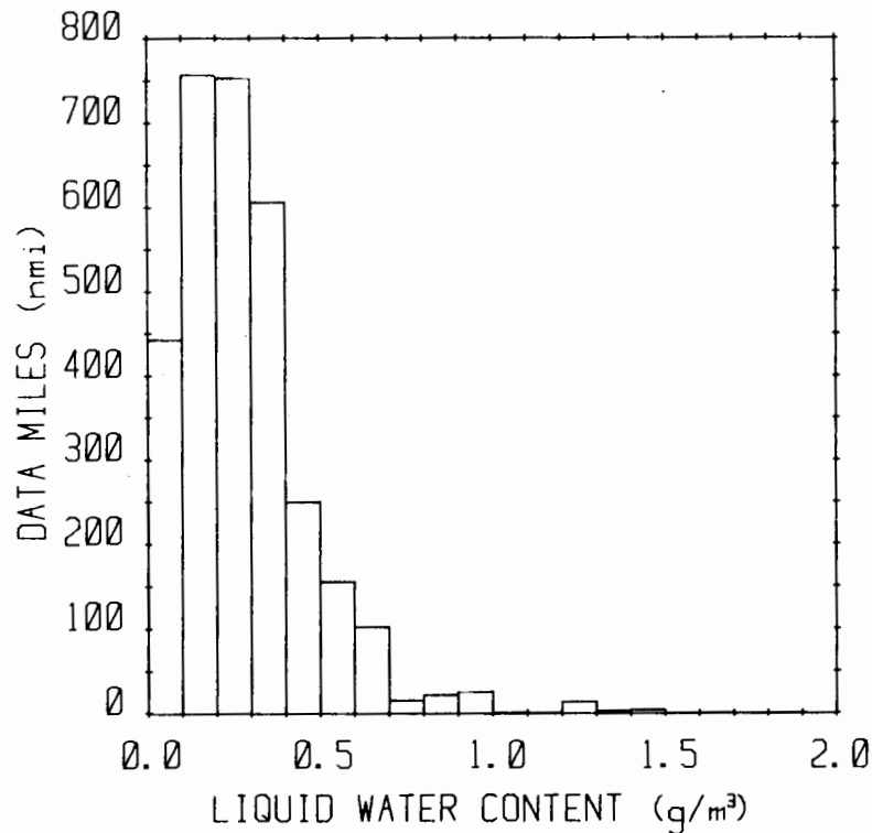
FIGURE 17. FREQUENCY DISTRIBUTION OF LWC IN ALL SUPERCOOLED CLOUD TYPES BELOW 10,000 FT AGL AS OBSERVED IN THE NACA DATA (1946-1950). A total of 3200 data miles is represented in this Figure.
