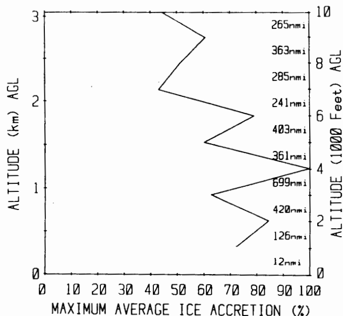
FIGURE 14. ALTITUDE VARIATION OF AVERAGE ICE ACCRETION PER EXTENDED ICING ENCOUNTER AS DETERMINED FROM THE NACA DATA (1946-1950). Ice accretion amounts represented by the product \bar{W}H are computed for all extended icing encounters occurring in each 1000 ft altitude interval. The average value of \bar{W}H for each altitude interval is expressed as a percentage of the largest of these interval-wide averages. At each 1000 ft level the plotted line indicates this percentage value for the 1000 ft altitude interval immediately below. An extended encounter is a series of consecutive icing events added together sequentially until a gap of some specified duration (3 nmi for this case) is reached. \bar{W} is the LWC averaged over the extended encounter (gaps not included) and H is the horizontal extent of the extended encounter (gaps not included). The right-hand column of numbers gives the number of data miles contributing within each 1000 ft interval. A total of 3170 data miles is represented in this Figure.
