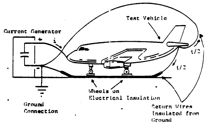
Figure 4-7. Typical setups for complete vehicle tests.
