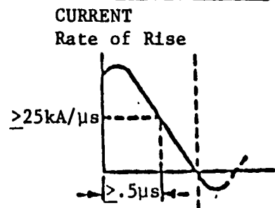
FIGURE 9. CURRENT WAVEFORMS
