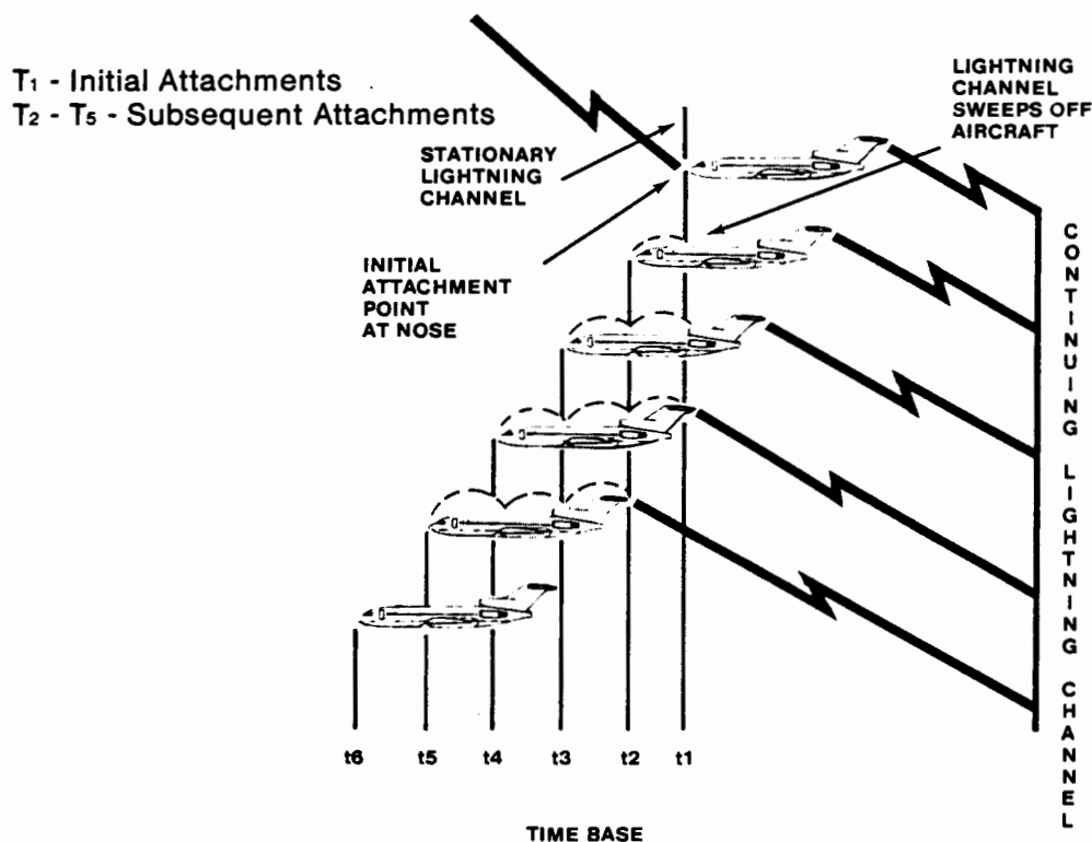
FIGURE 6. SWEPT-STROKE PHENOMENON (LIGHTNING CHANNEL POSITION SHOWN RELATIVE TO AIRCRAFT)
