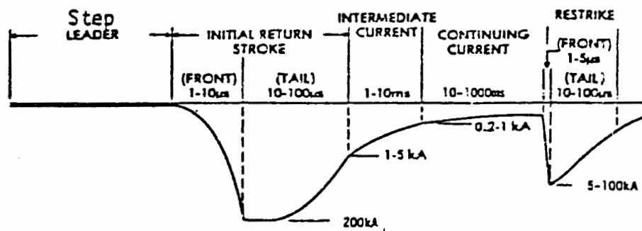
(A) Generalized waveshape of current in negative cloud-to-ground lightning.
