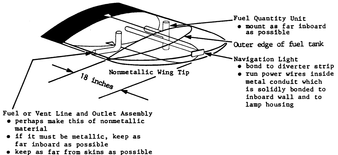
FIGURE 16. LOCATION OF METALLIC PARTS WITHIN NONCONDUCTING FUEL TANKS
