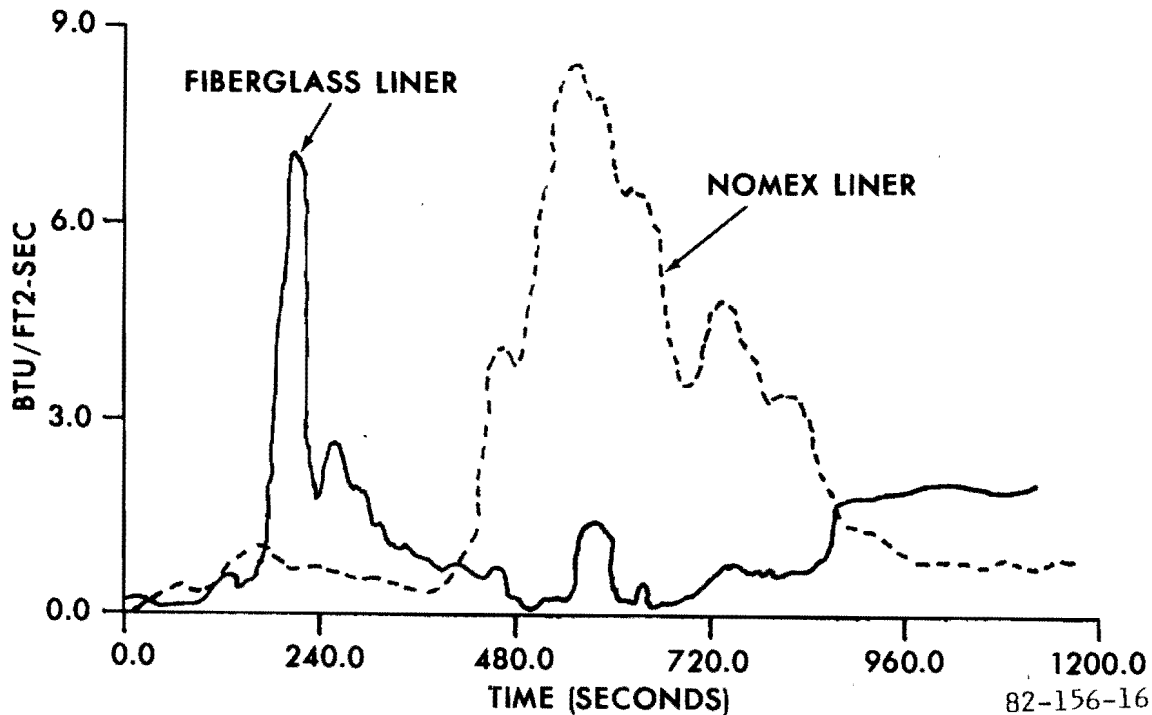
FIGURE 15. HEAT FLUX ON CEILING LINERS
