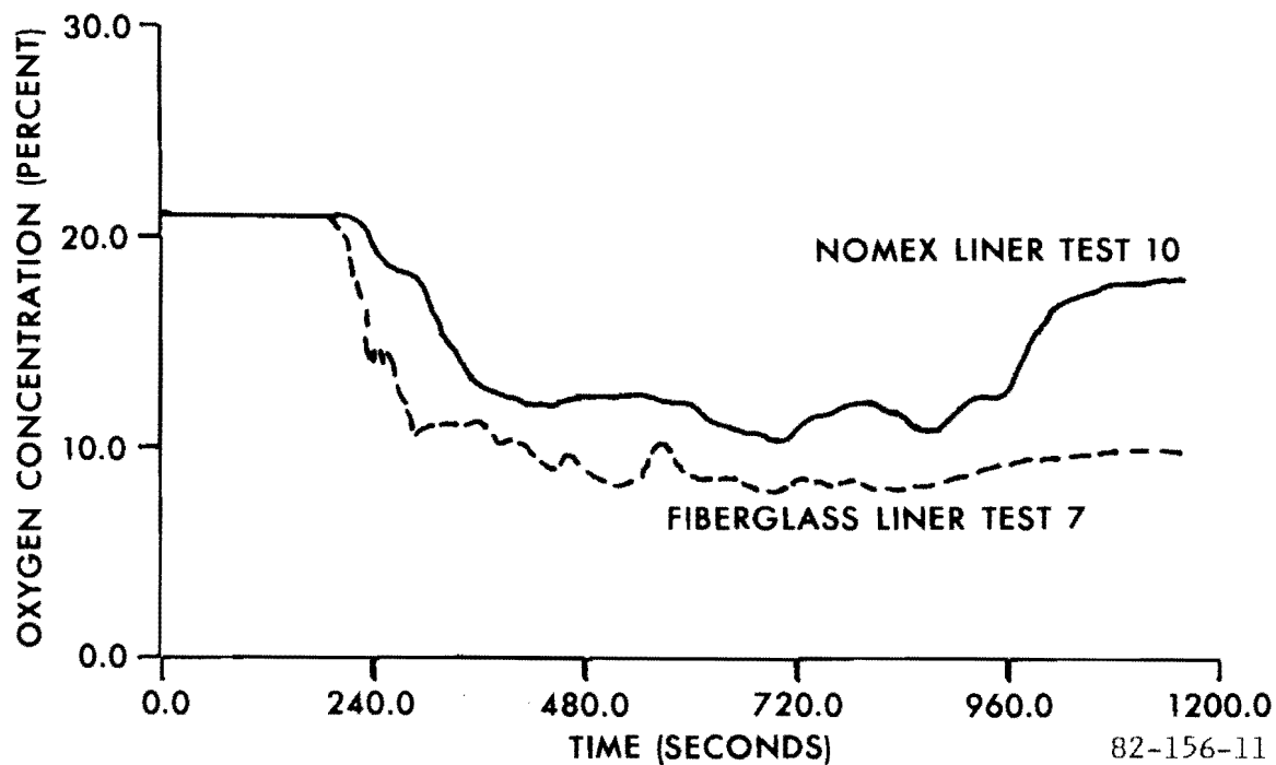
FIGURE 10. OXYGEN CONCENTRATION WITH NOMEX™ AND FIBERGLASS LINERS
