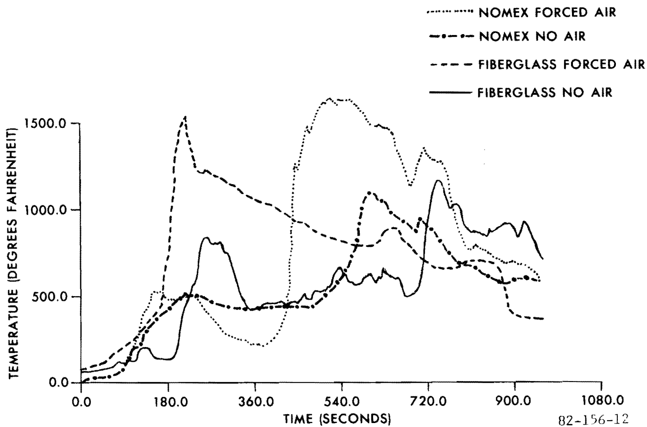
FIGURE 11. BELOW CEILING TEMPERATURES
