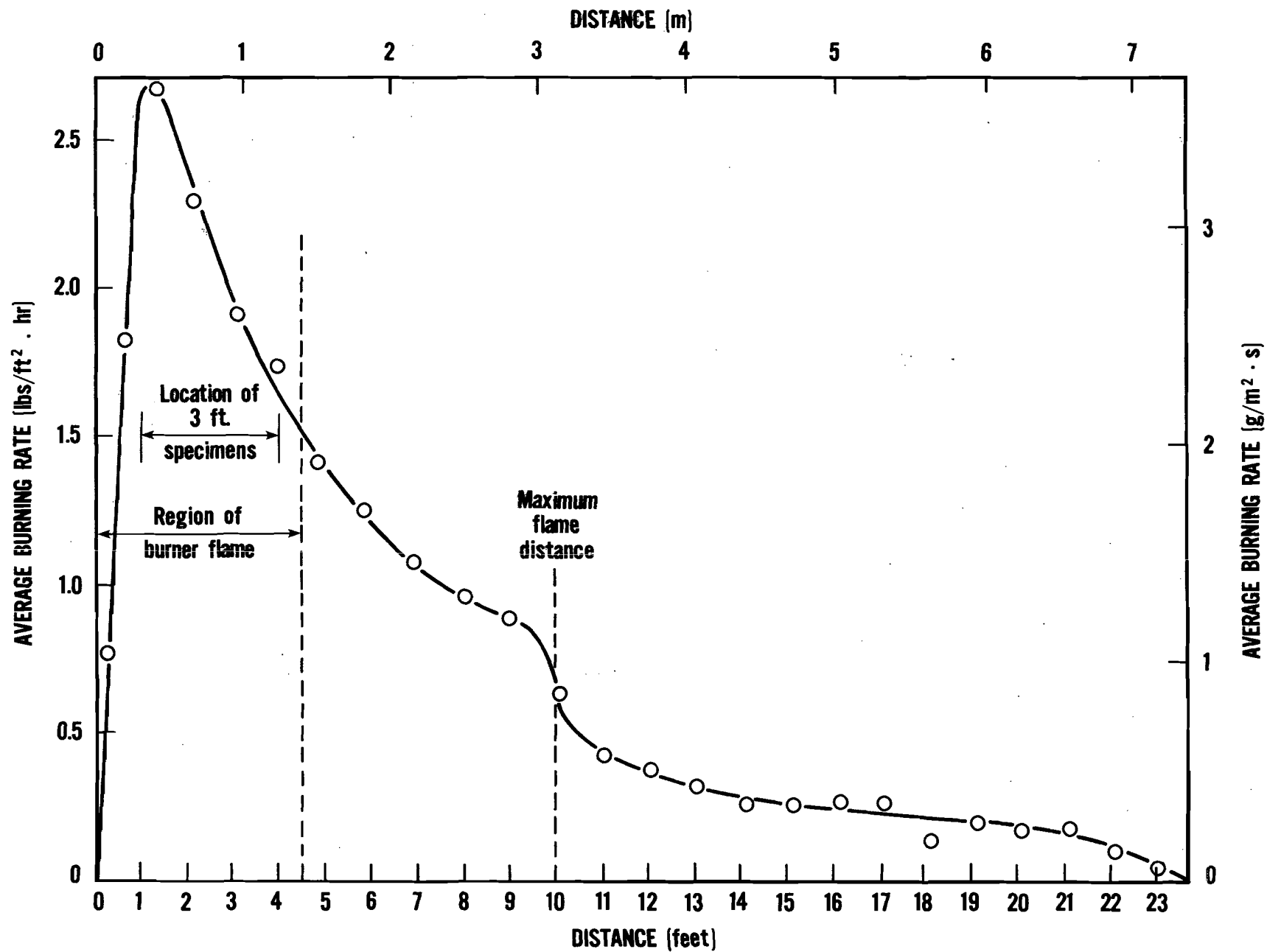
Figure 13. Average burning rate distribution along a type B specimen
