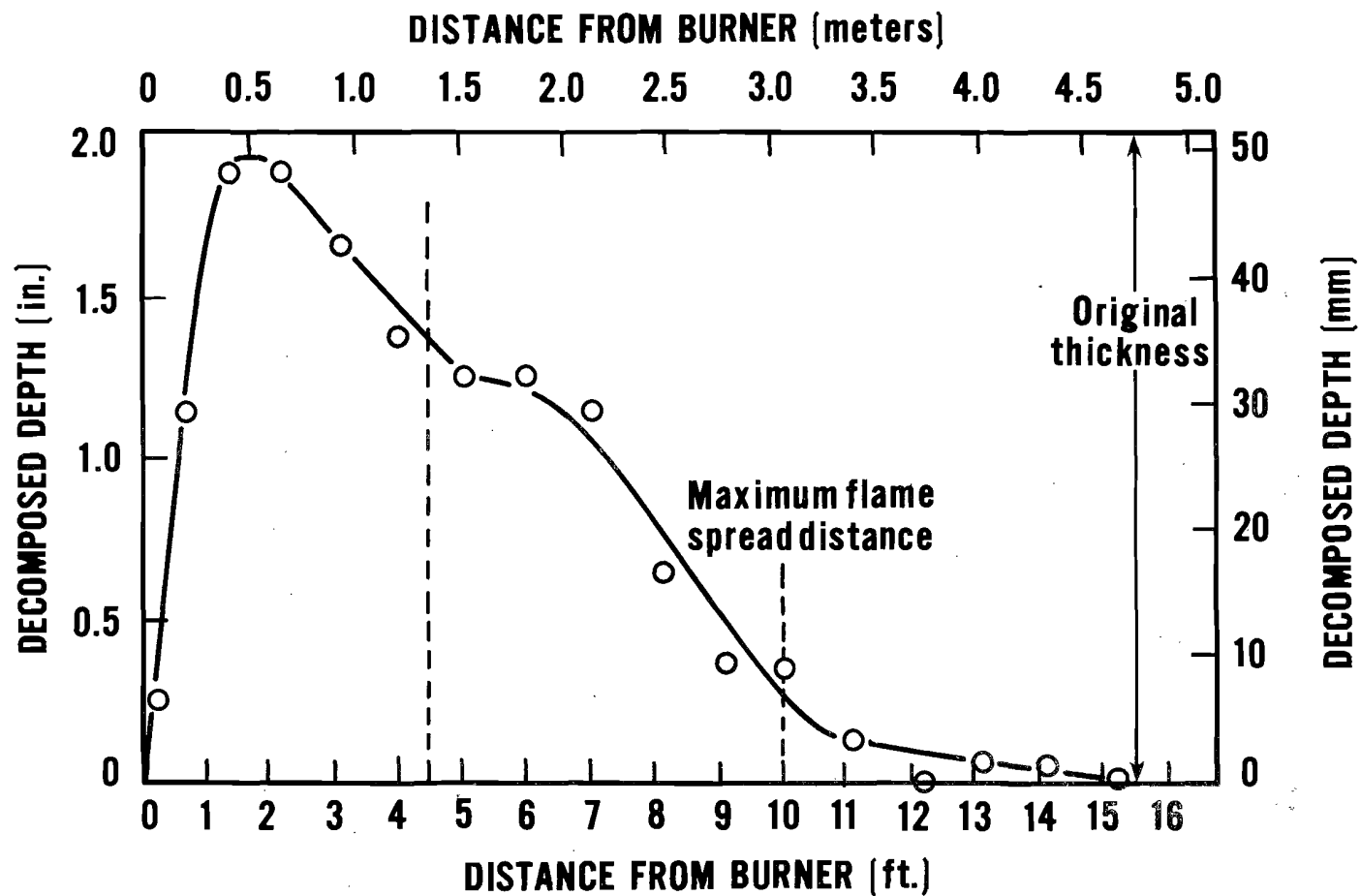
Figure 14. Decomposed depth versus distance for type B specimen.
