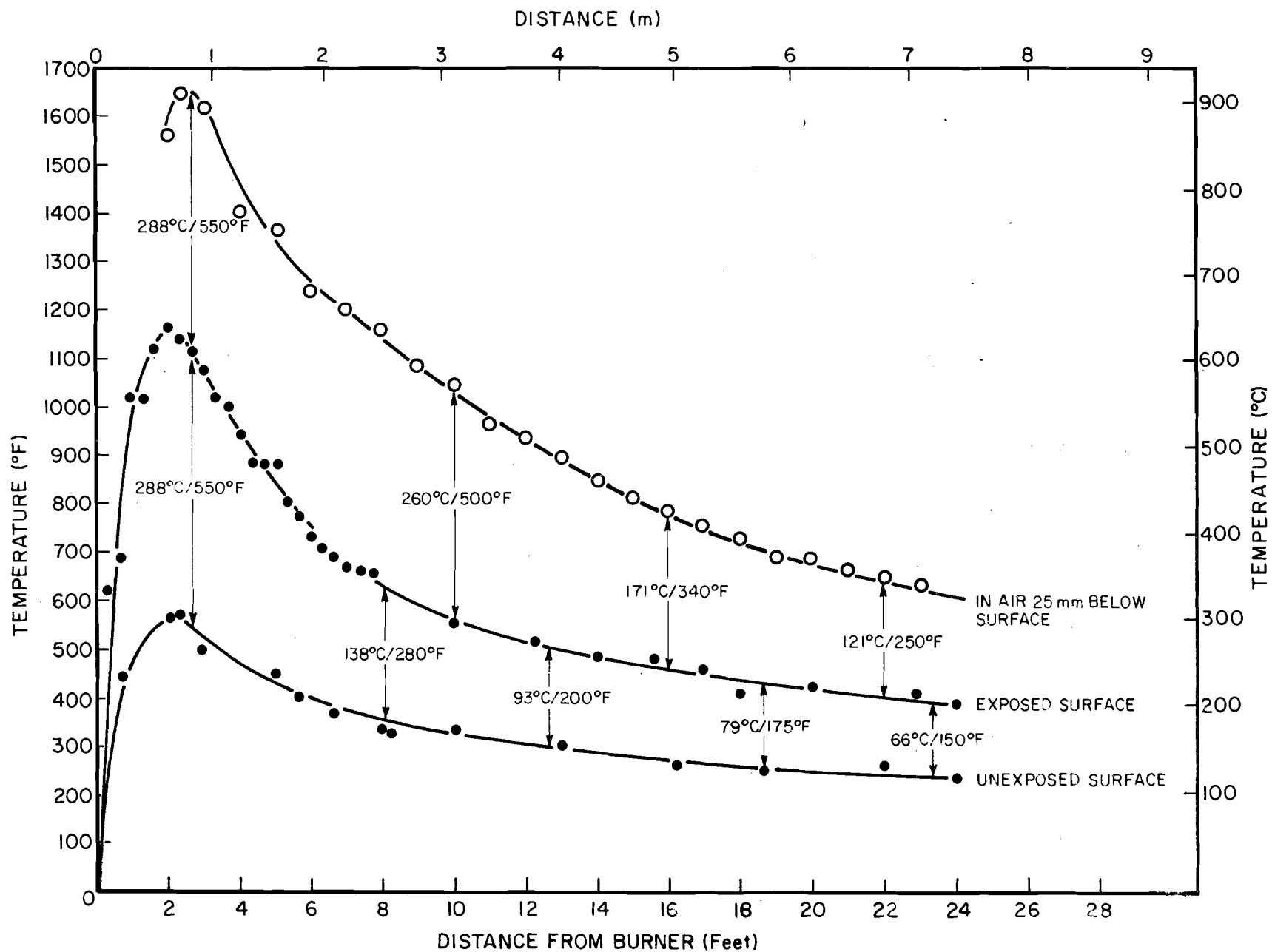
Figure 6. Temperature distribution along exposed and unexposed surfaces of AMB specimen
