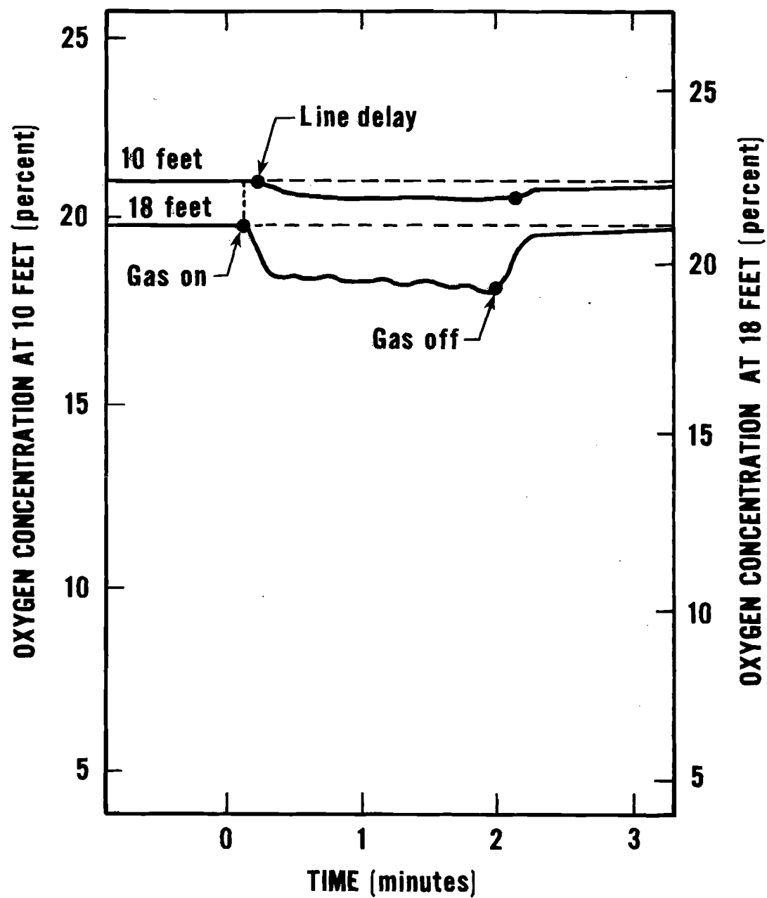
Figure 15. Chart record of oxygen concentration on the floor of the tunnel at 10 and 18 feet for a type B specimen (1 foot = 0.305 meters)
