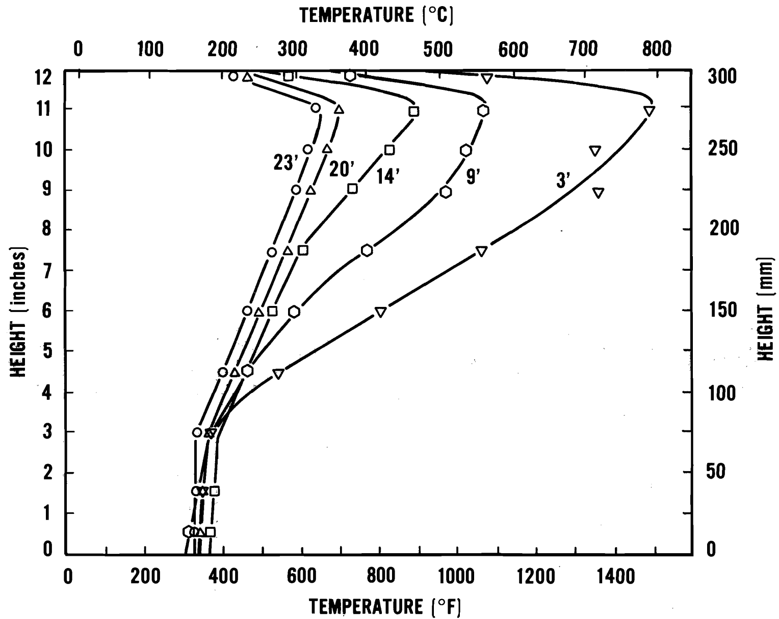
Figure 10. Centerline air temperature profiles at various distances in the tunnel for an ACB specimen at 10 minutes.
