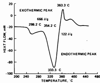
Figure 5: Differential Scanning Calorimetry of Vonar R 2
