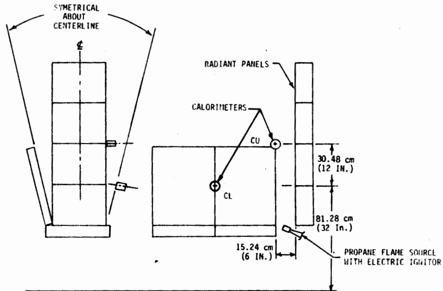
FIGURE 2. FUEL SOURCE AND CALORIMETER LOCATION
