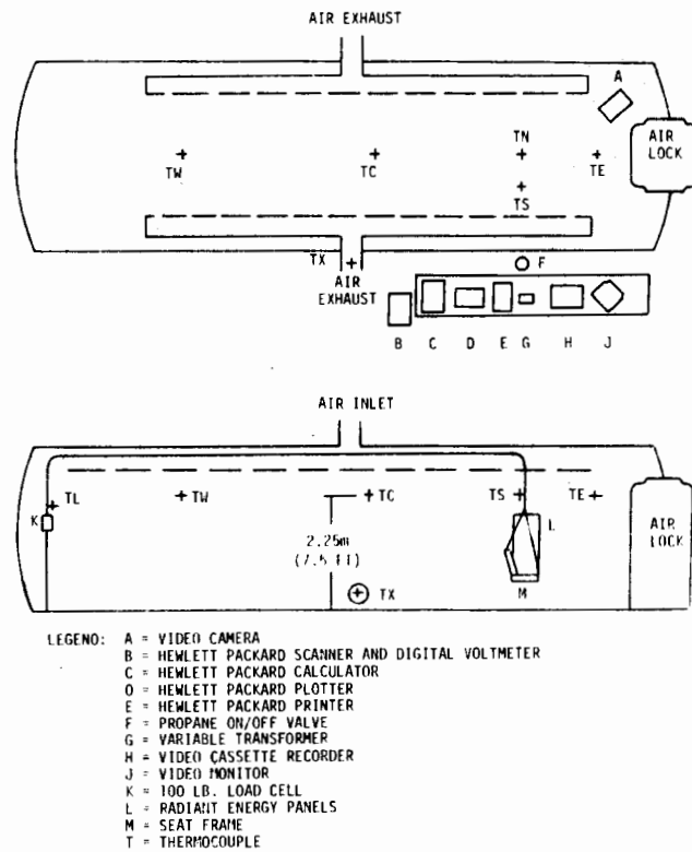
FIGURE 4. CFS INSTRUMENTATION
