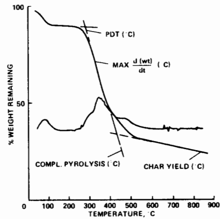
Figure 4: Typical Thermogram
