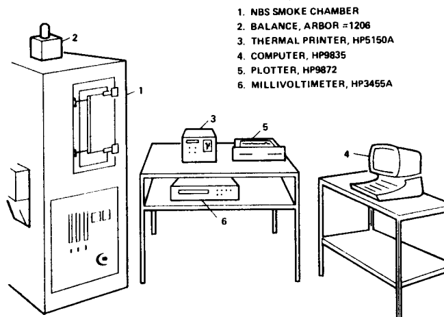
Figure 2: Equipment for Weight-Loss Data
