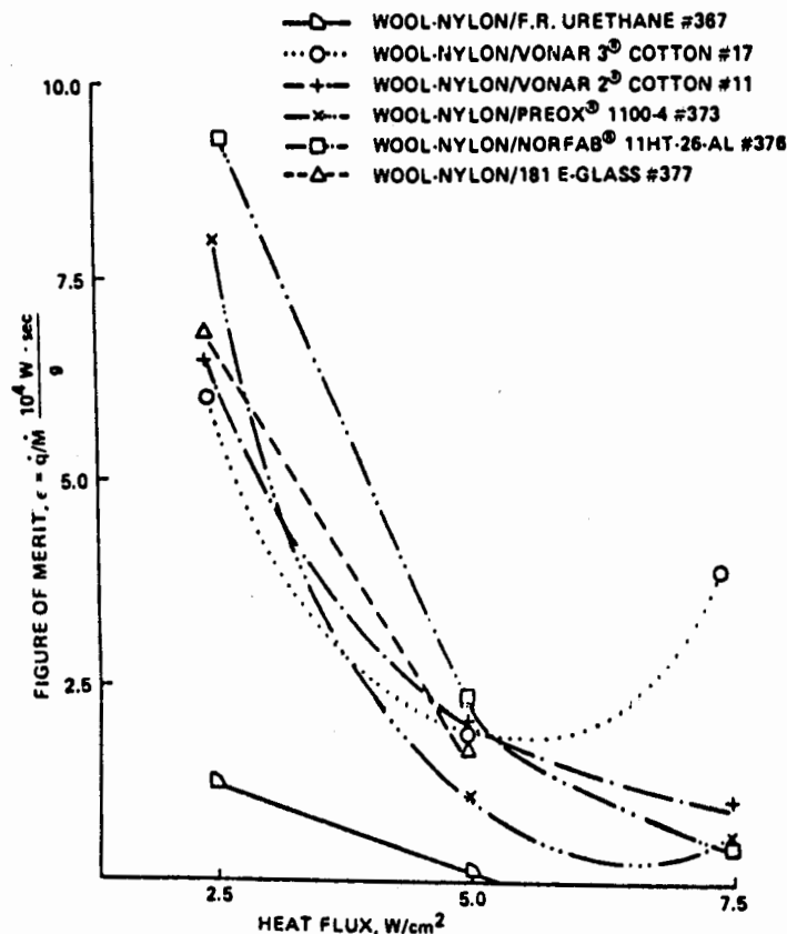
Figure 2: THERMAL EFFICIENCY COMPARISON OF HEAT BLOCKING LAYERS FOR FR URETHANE AS A FUNCTION OF HEAT FLUX AT 2 MINUTES ELAPSED TIME
