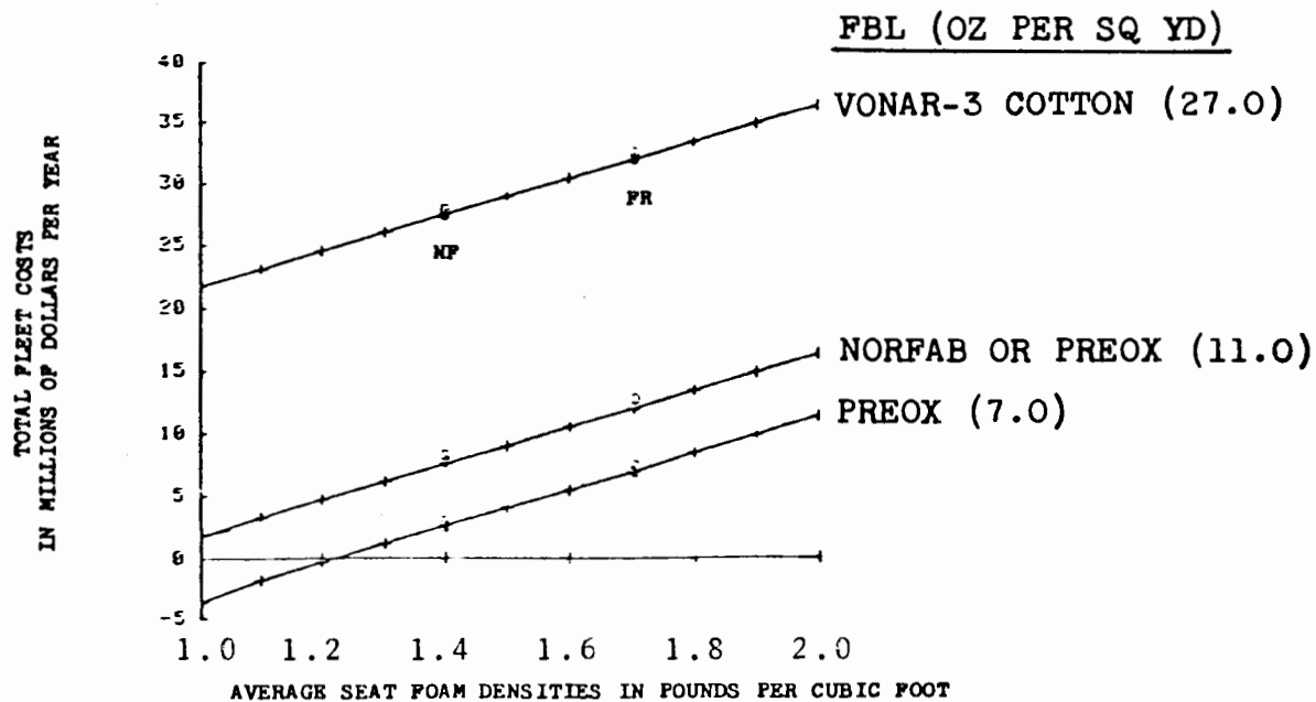
Figure 6: ALGORITHM COST EVALUATION OF CURRENTLY AVAILABLE FOAMS AND FIRE BLOCKING LAYERS AT EQUIVALENT FIRE PERFORMANCE AND COMFORT
