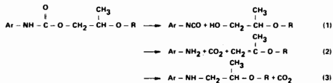
Figure 6: Thermal Degradation of Flexible Polyurethane Foams
