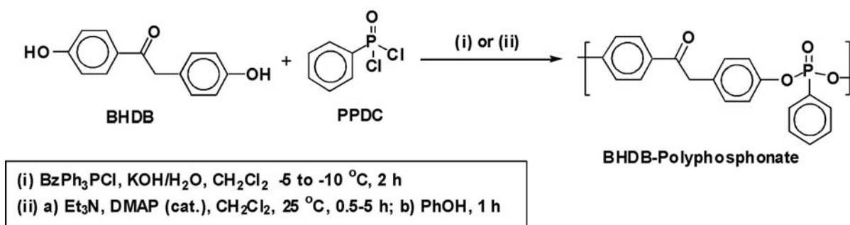
Figure 4. Synthetic Scheme for BHDB Polyphosphonates
