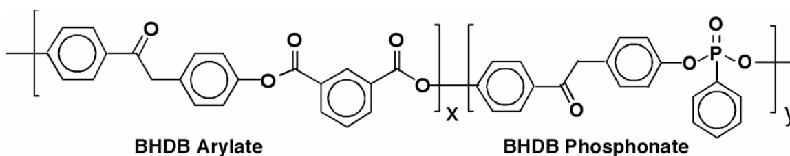
Figure 5. Structure of BHDB Arylate-Phosphonate Copolymers
