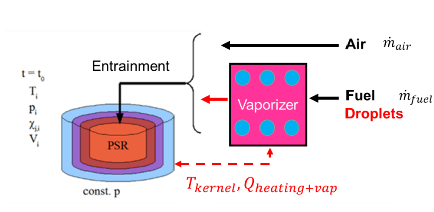
Figure 11. Conceptual model PSR modeling with droplet vaporization
