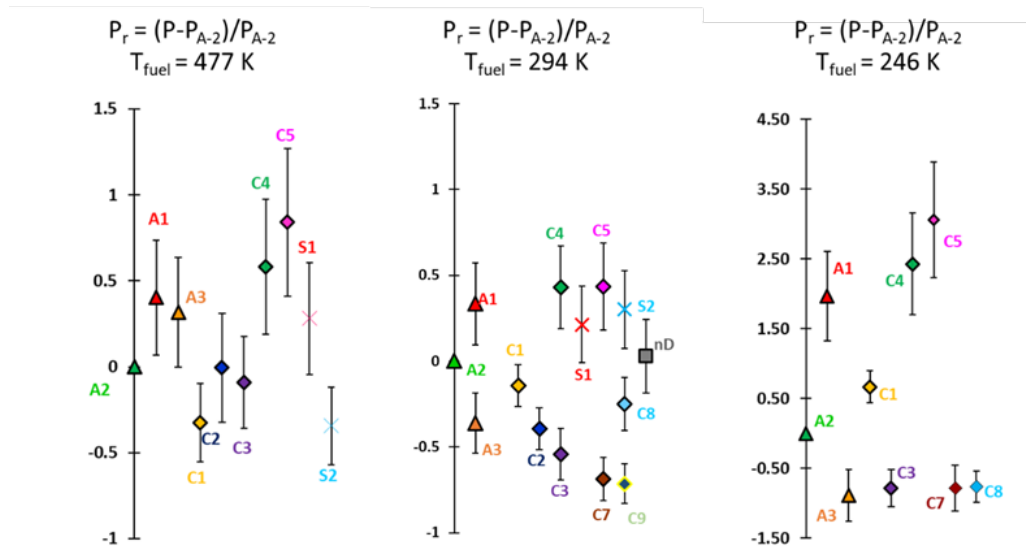
Figure 7. Ignition probability rankings, scaled with respect to A2 probability. Error bars show 68% uncertainty. Left: pre-vaporized fuel/air mixture; Middle: room temperature Liquid fuel spray; right: chilled liquid fuel spray.
