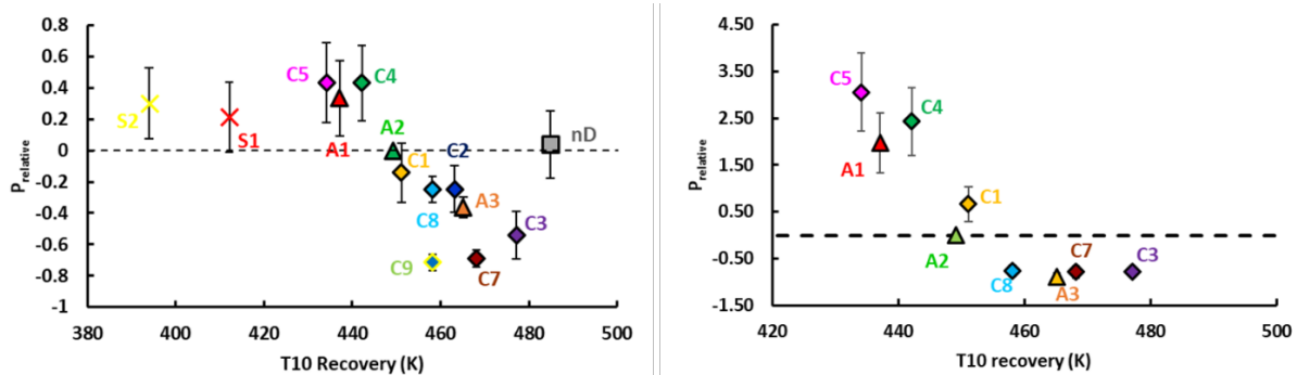
Figure 9. Relative probabilities versus 10% recovery temperature. Left: Probability results for room temperature fuel spray; right: probability results for chilled fuel sprays
