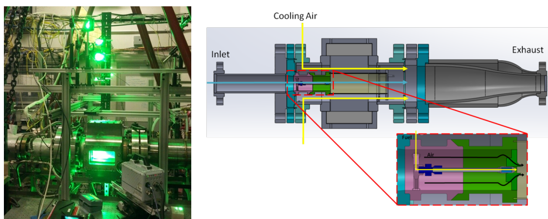
Figure 3. High shear swirl combustor, showing a) pressure vessel instrumented for high speed stereo PIV and OH PLIF, and b) a cross section with generic swirler holder/injector for illustrative purposes.
