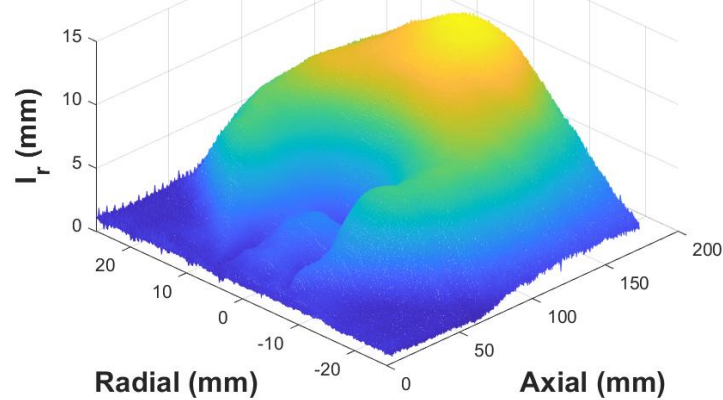
Figure 16. Radial integral length scale of visible light emissions from turbulent Bunsen burner flame burning A2 fuel. Such statistics have been considering as a marker of the onset of openings of the flame brush.
