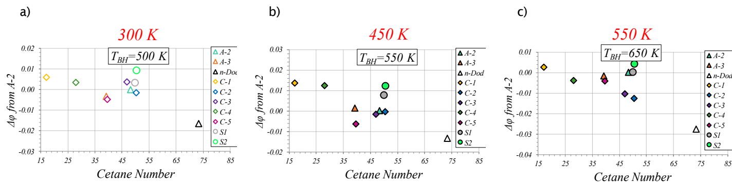
Figure 1. Sample of year 3 screening data at three different preheat temperatures and three different bulkhead temperatures, demonstrating the strong correlation of lean blowout with the cetane number. The correlation coefficients between blowout equivalence ratio and the Cetane number are -0.21 at 300 K, -0.79 at 450 K, and -0.76 at 550 K.
