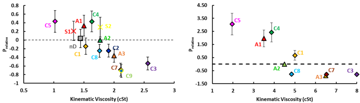
Figure 8. Relative probabilities versus relative viscosity for room temperature fuel spray; right: probability results for chilled fuel sprays.
