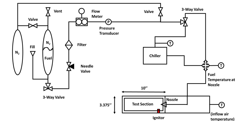
Figure 6. Schematic of the liquid fuel delivery system.
