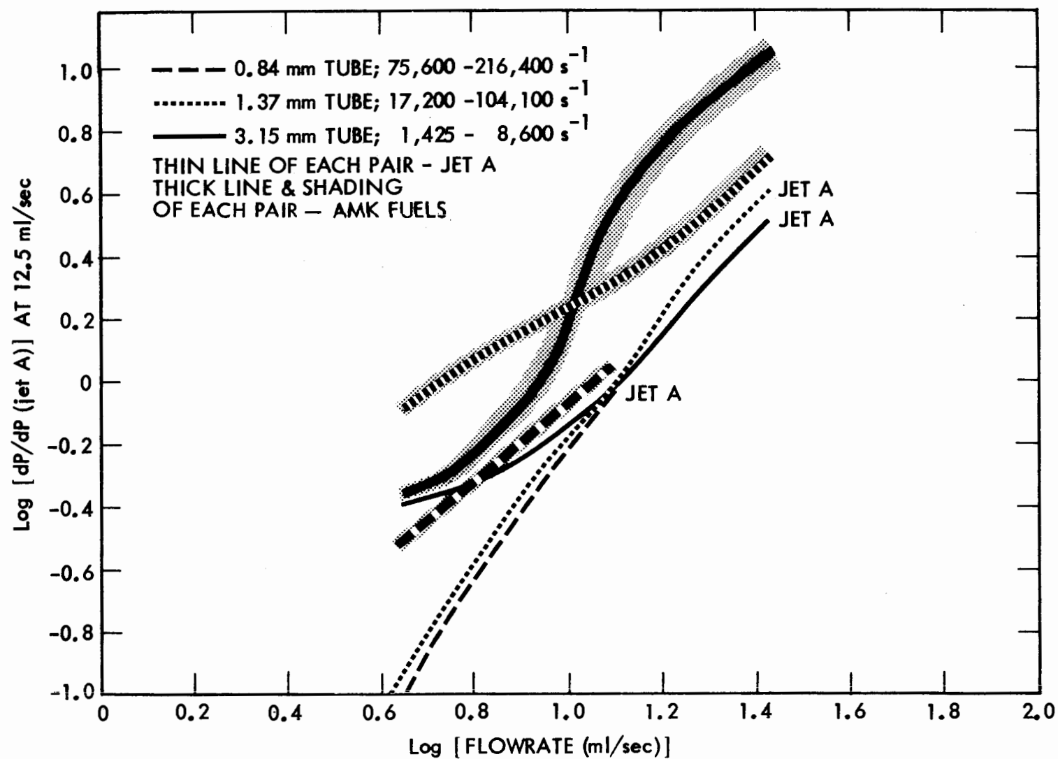
Figure 20. EFFECT OF TUBE EXIT SECTION DIAMETER AND SHEAR RATE ON THE SENSITIVITY OF THE PRESSURE DROP TEST.
