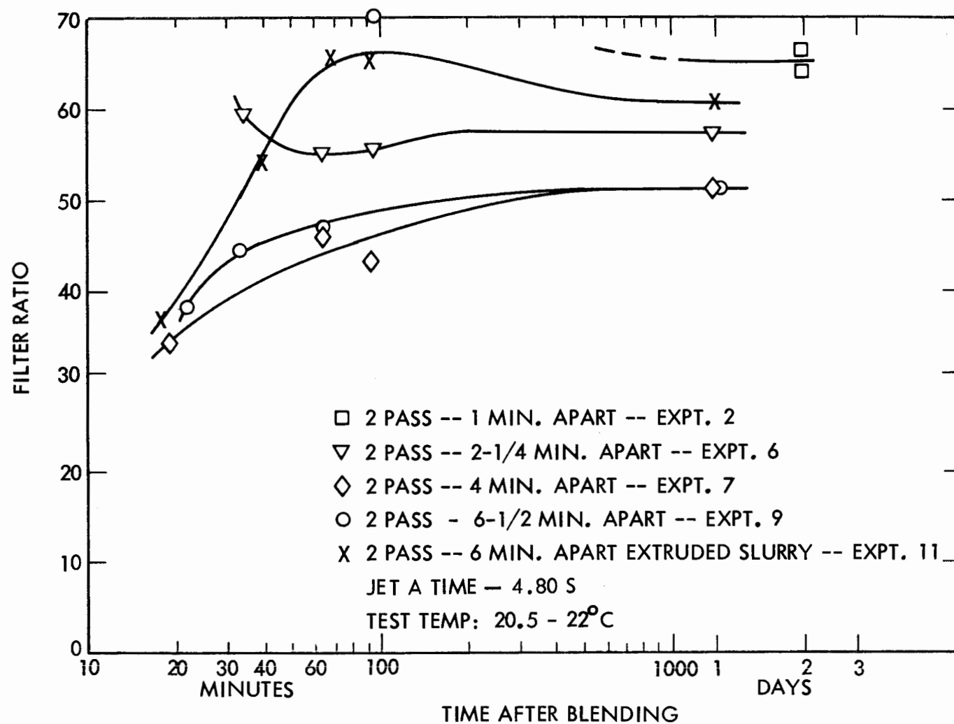
Figure 9. FILTER TEST RESULTS FOR AMK FUELS PREPARED BY IN-LINE BLENDING.
