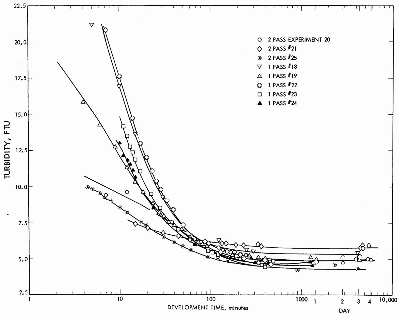
Figure 10. TURBIDITY MEASUREMENTS ON IN-LINE BLENDED AMK FUELS.
