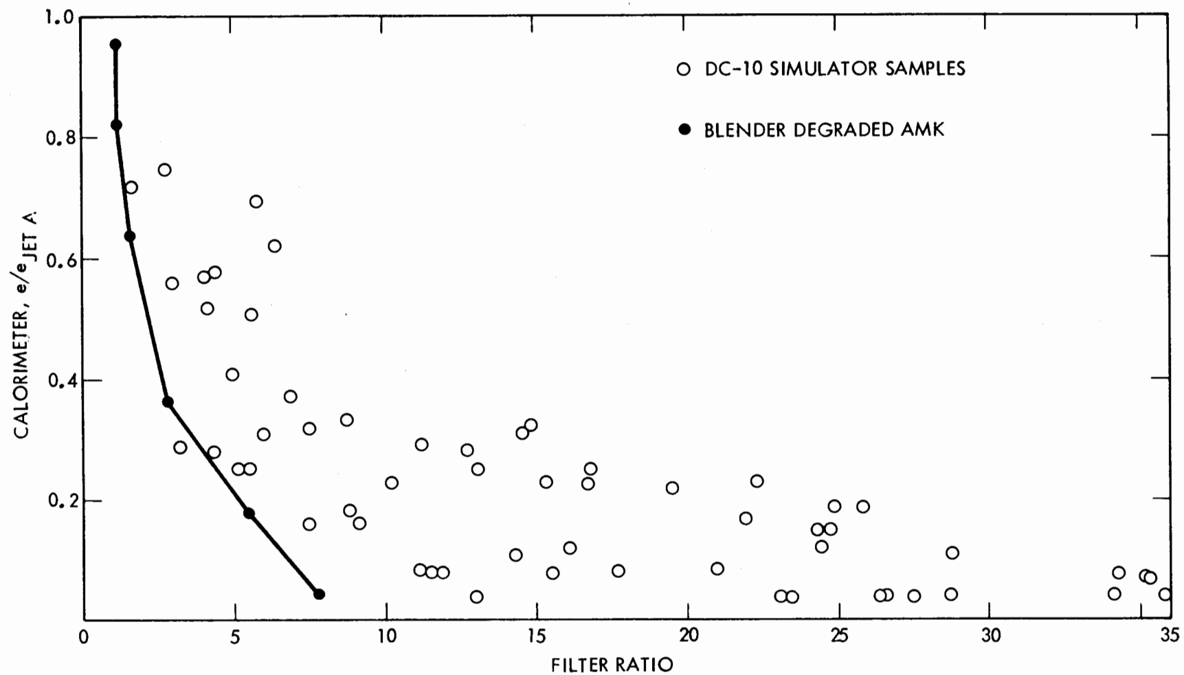
Figure 16. CORRELATION OF FILTER TEST AND FCTA CALORIMETER DATA FOR DC-10 FUEL SYSTEM SIMULATOR AND BLENDER DEGRADED SAMPLES.
