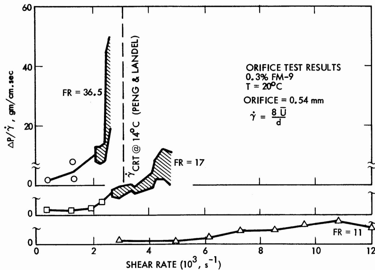
Figure 23. EXTENT OF DEGRADATION BY ORIFICE PRESSURE DROP TESTING.
