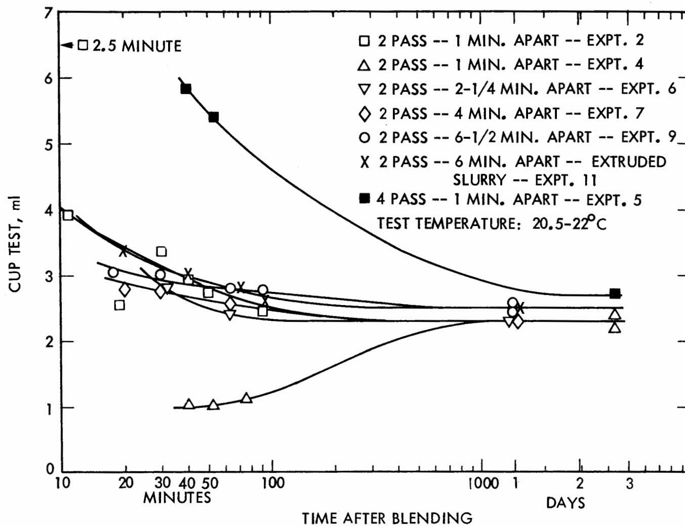
Figure 8. CUP TEST RESULTS FOR AMK FUELS PREPARED BY IN-LINE BLENDING.
