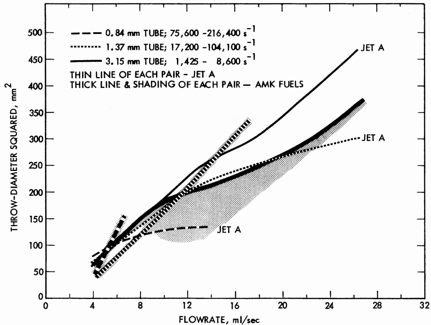
Figure 21. EFFECT OF TUBE EXIT SECTION DIAMETER AND SHEAR RATE ON THE SENSITIVITY OF THE TRAJECTORY ANALYSIS.
