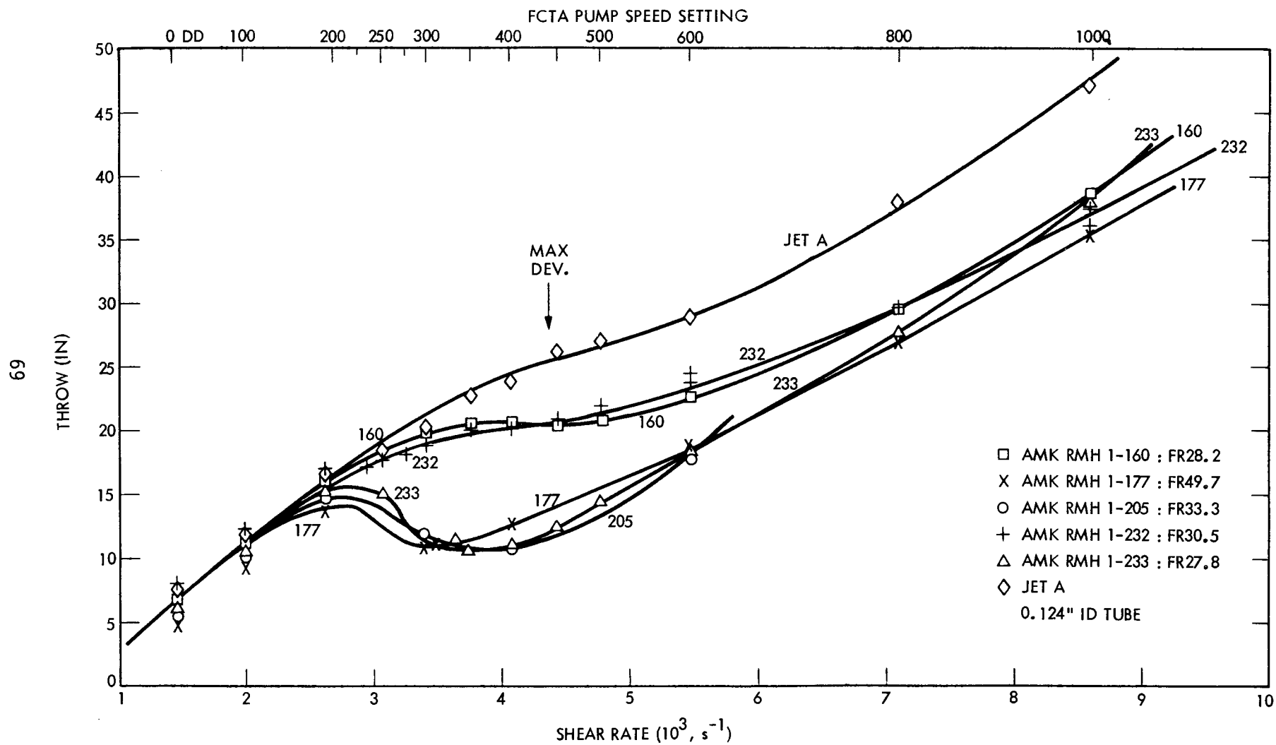
Figure 22. DISCRIMINATION OF EQUILIBRATED AMK FUELS BY TUBE TRAJECTORY ANALYSIS.
