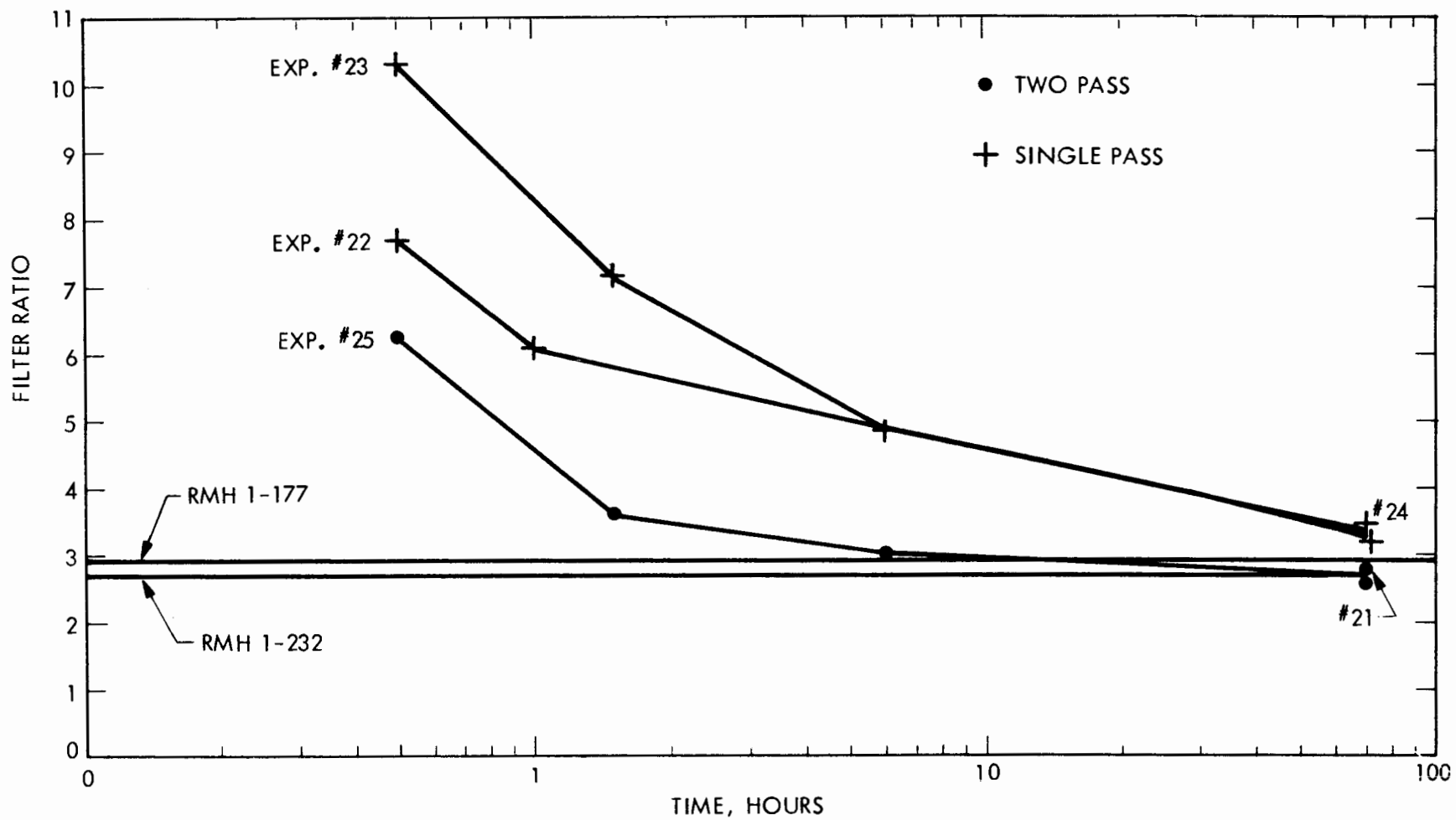
Figure 11. DEGRADABILITY OF IN-LINE BLENDED AMK FUELS.
