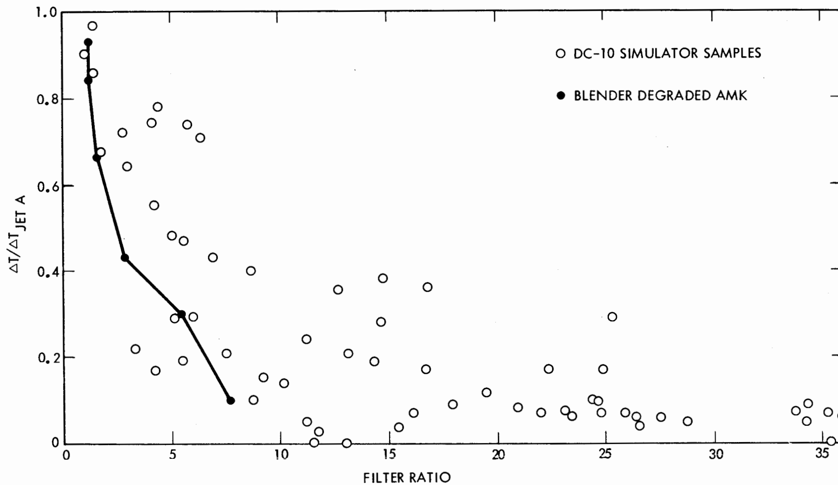
Figure 15. CORRELATION OF FILTER TEST AND FCTA THERMOCOUPLE DATA FOR DC-10 FUEL SYSTEM SIMULATOR AND BLENDER DEGRADED SAMPLES.
