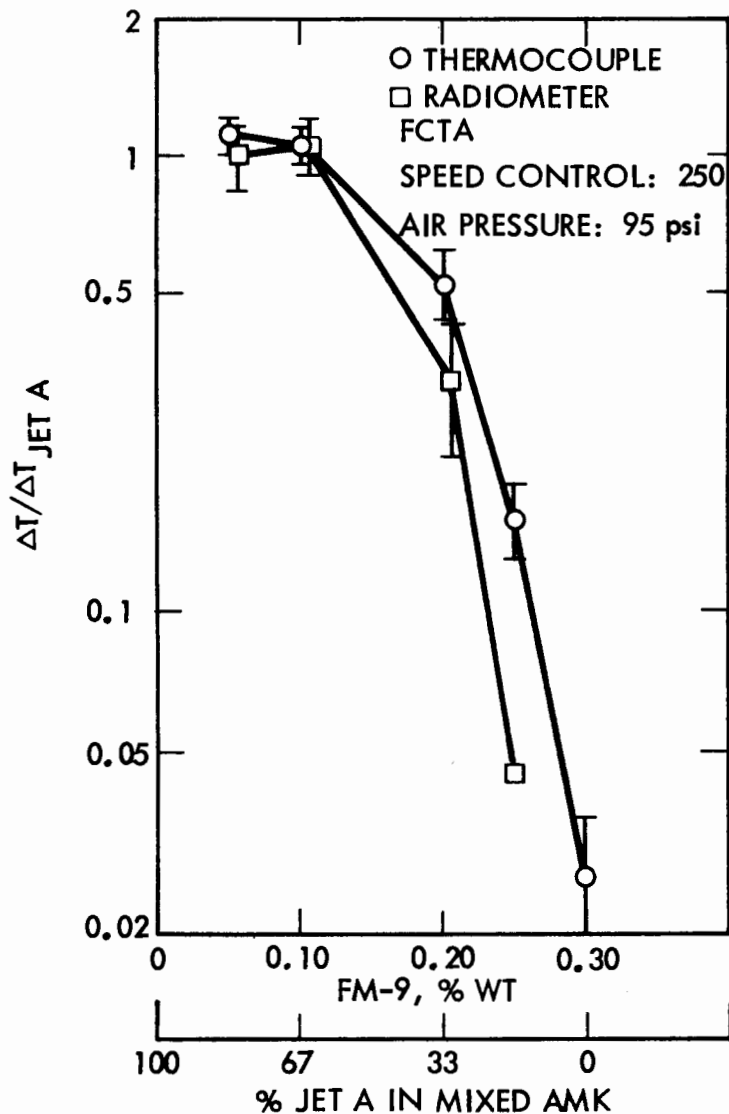
Figure 18. EFFECT OF DILUTION WITH JET A ON AMK FLAMMABILITY.
