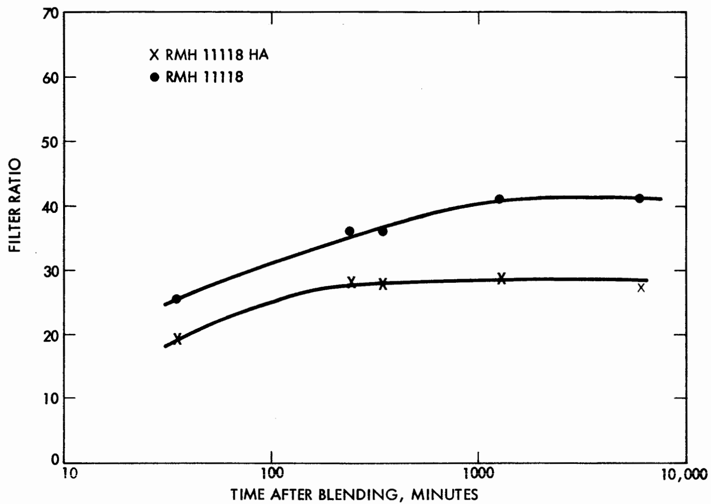
Figure 4. INFLUENCE OF BASE FUEL AROMATIC CONTENT ON FM-9 DISSOLUTION RATE.
