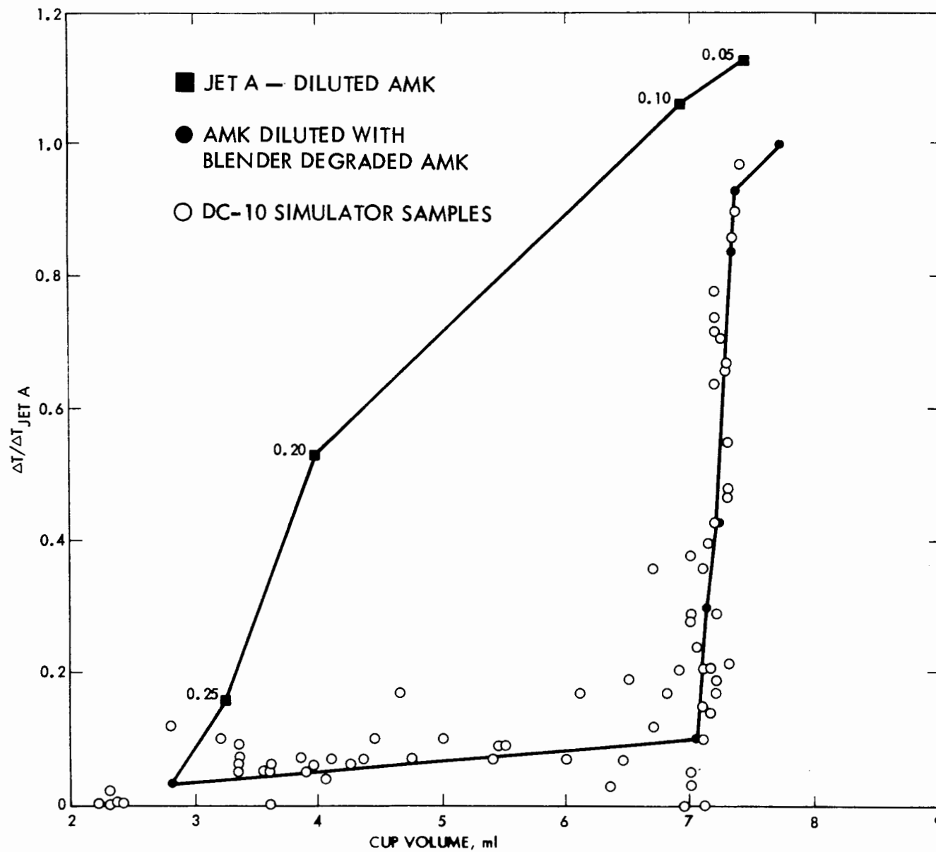
Figure 17. INFLUENCE OF DILUENT ON CORRELATION OF CUP TEST VOLUMES WITH FCTA FIRE TEST.
