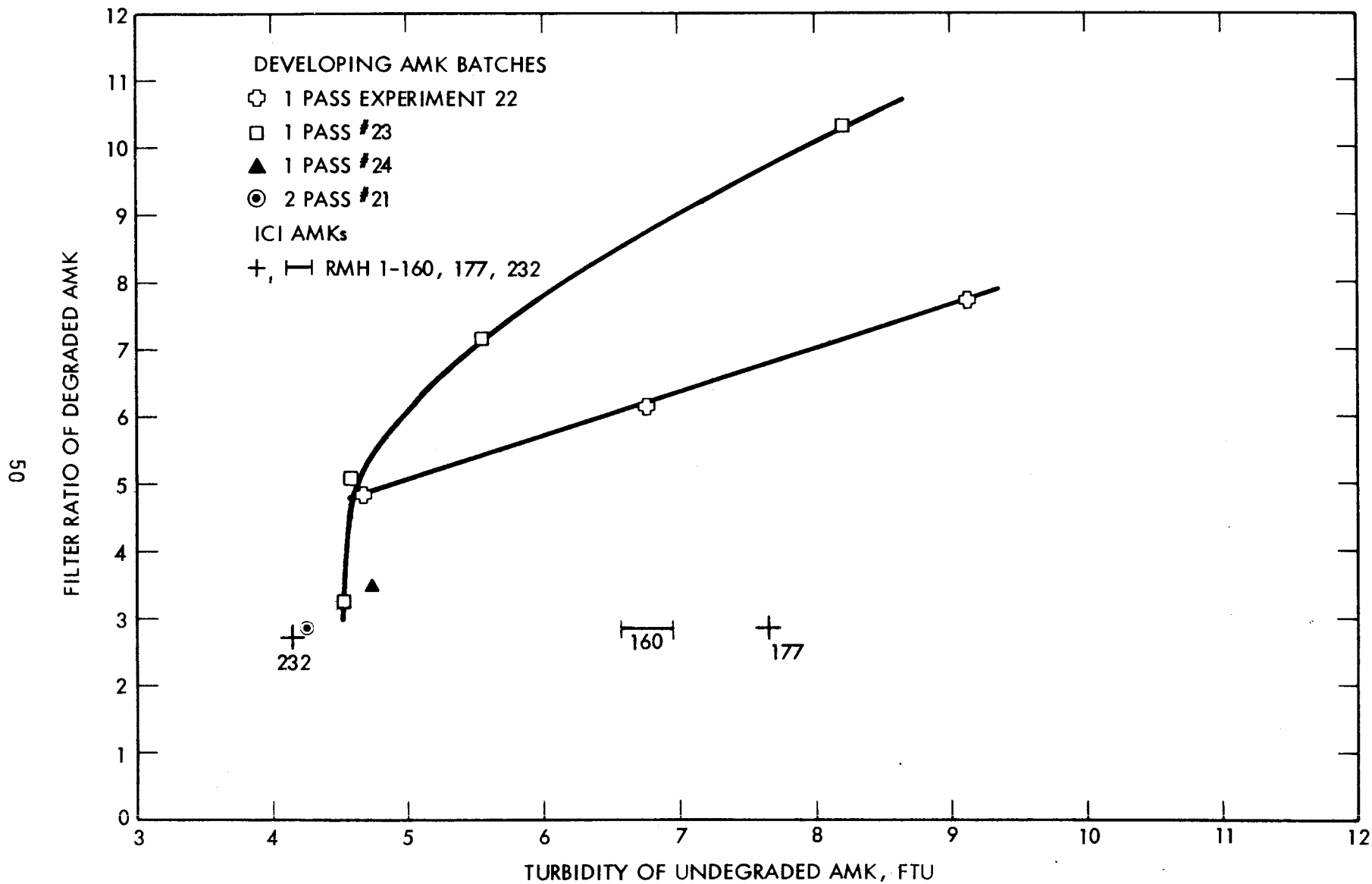
Figure 13. CORRELATION OF TURBIDITY AND DEGRADABILITY OF IN-LINE BLENDED AMK FUELS.
