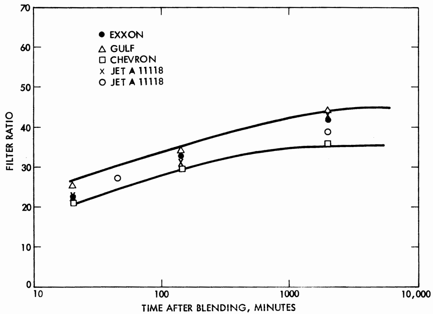
Figure 3. EFFECT OF BASE FUEL ON FILTER RATIO OF 0.3% AMK.
