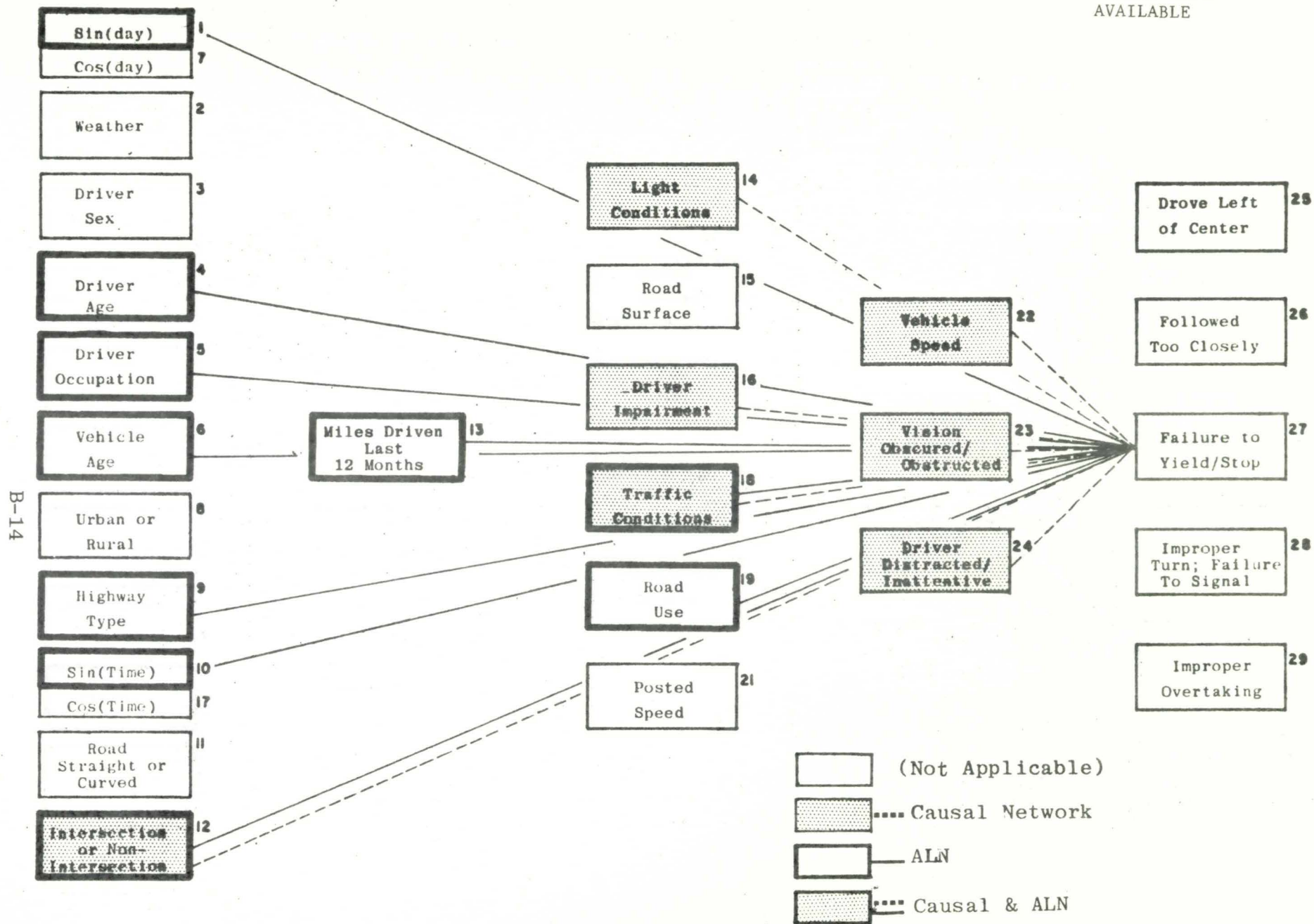
FIGURE B.13: RESTRUCTURED CAUSAL NETWORK: VARIABLE 27 - FAILURE TO YIELD/STOP
