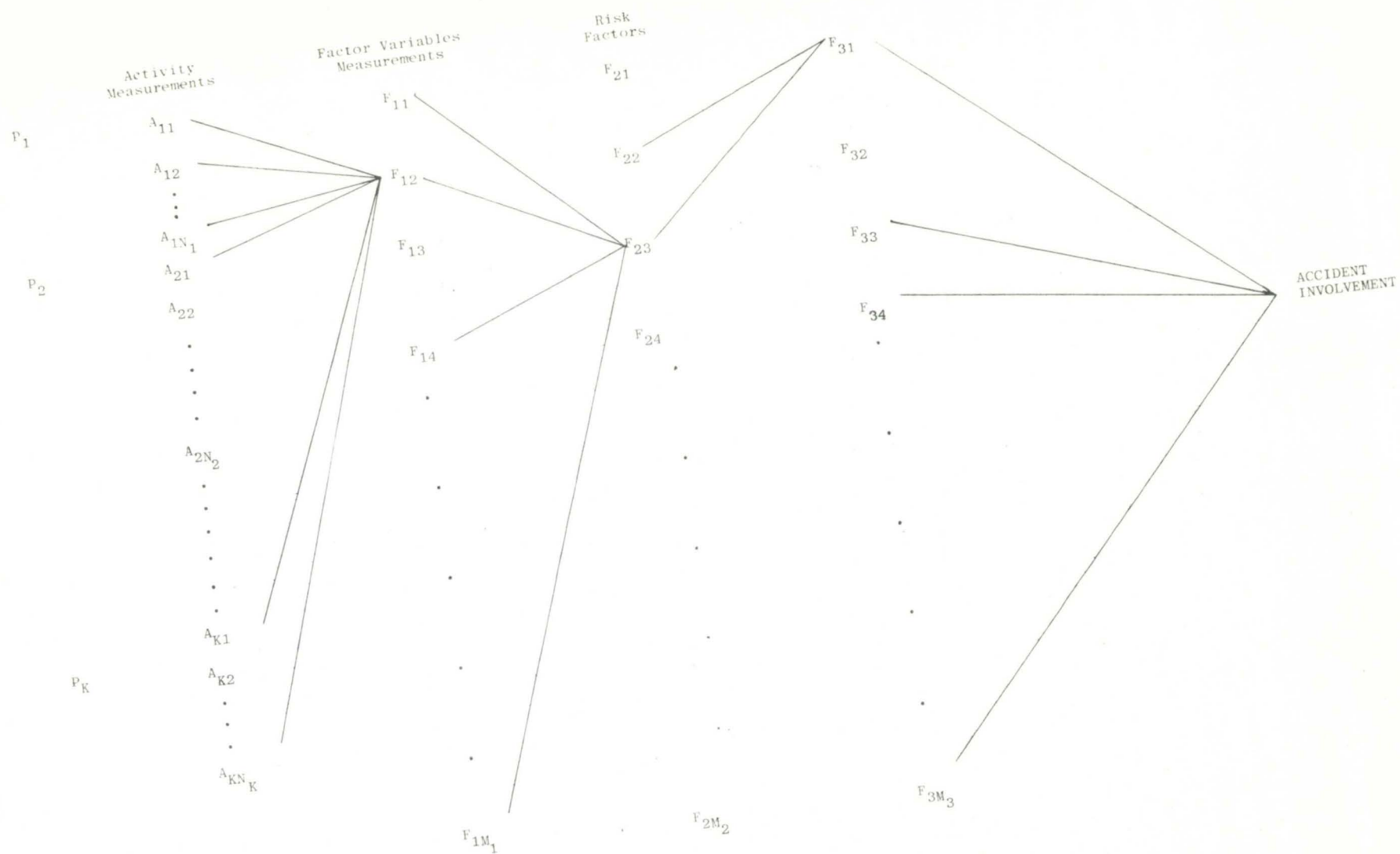
FIGURE 2.1: CONCEPTUAL CAUSAL NETWORK
