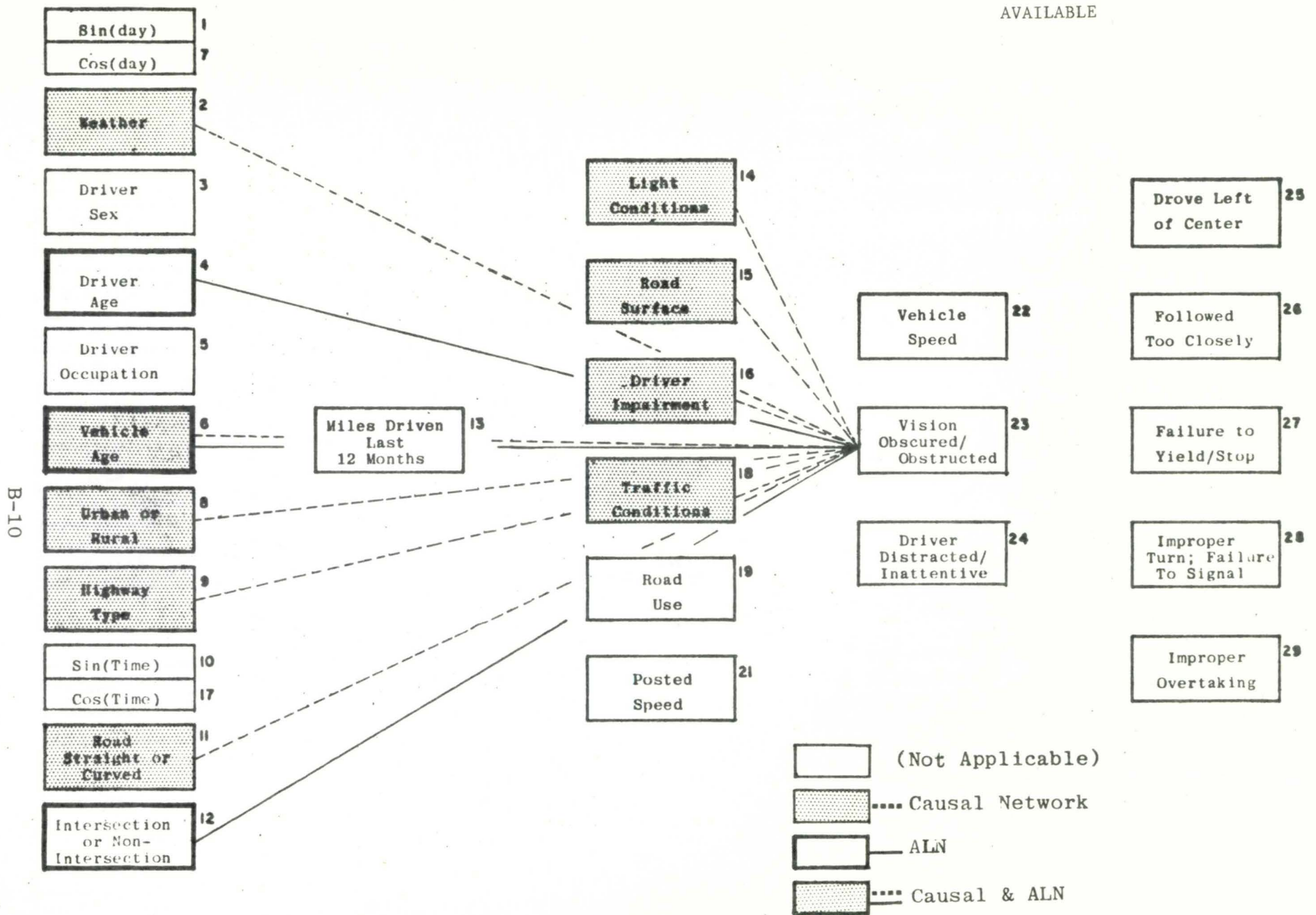
FIGURE B.9: RESTRUCTURED CAUSAL NETWORK: VARIABLE 23 - VISION OBSCURED/OBSTRUCTED
