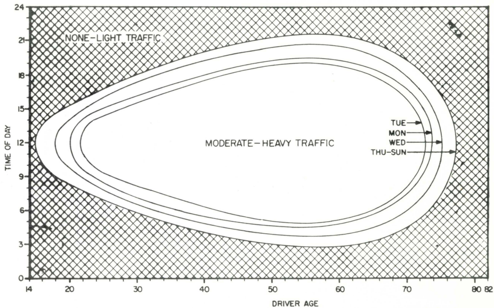
FIGURE 6.4: IMPORTANCE OF TRAFFIC CONDITIONS (FIG. 5.5)
