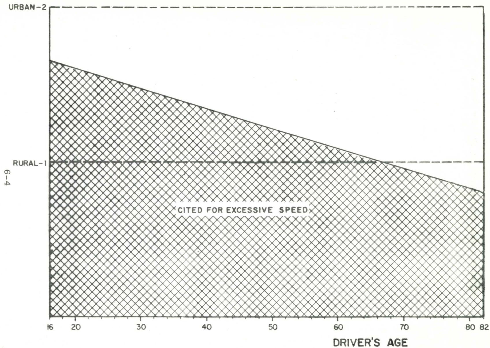
FIGURE 6.1: DECISION REGIONS FOR DEPENDENT VARIABLE 22 (EXCESSIVE SPEED -- FIG. 5-8)
