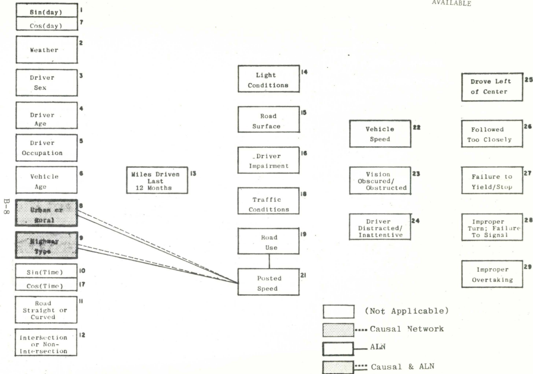
FIGURE B.7: RESTRUCTURED CAUSAL NETWORK: VARIABLE 21 - POSTED SPEED
