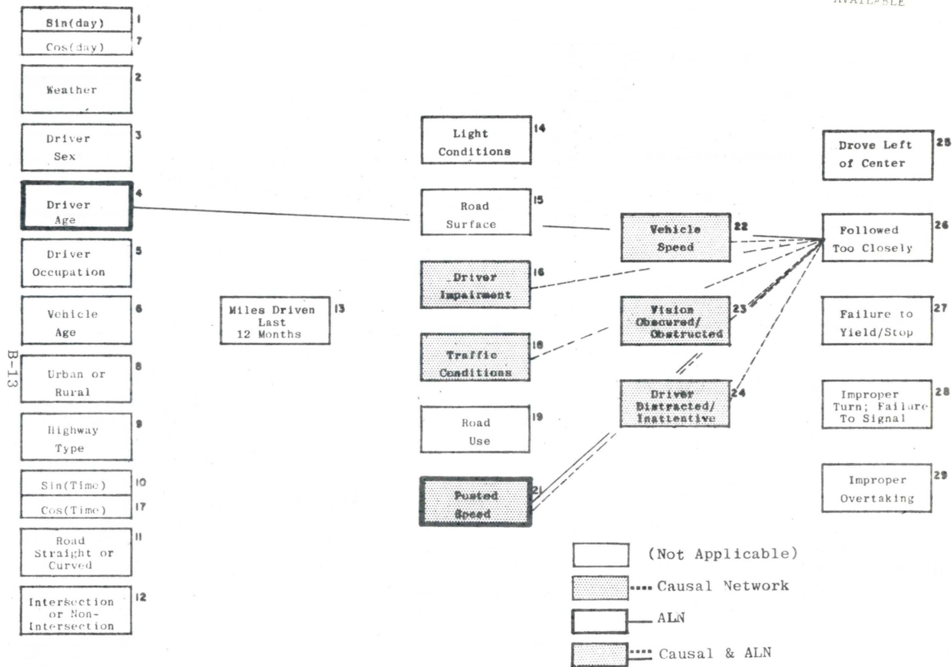
FIGURE B.12: RESTRUCTURED CAUSAL NETWORK: VARIABLE 26 - FOLLOWED TOO CLOSELY
