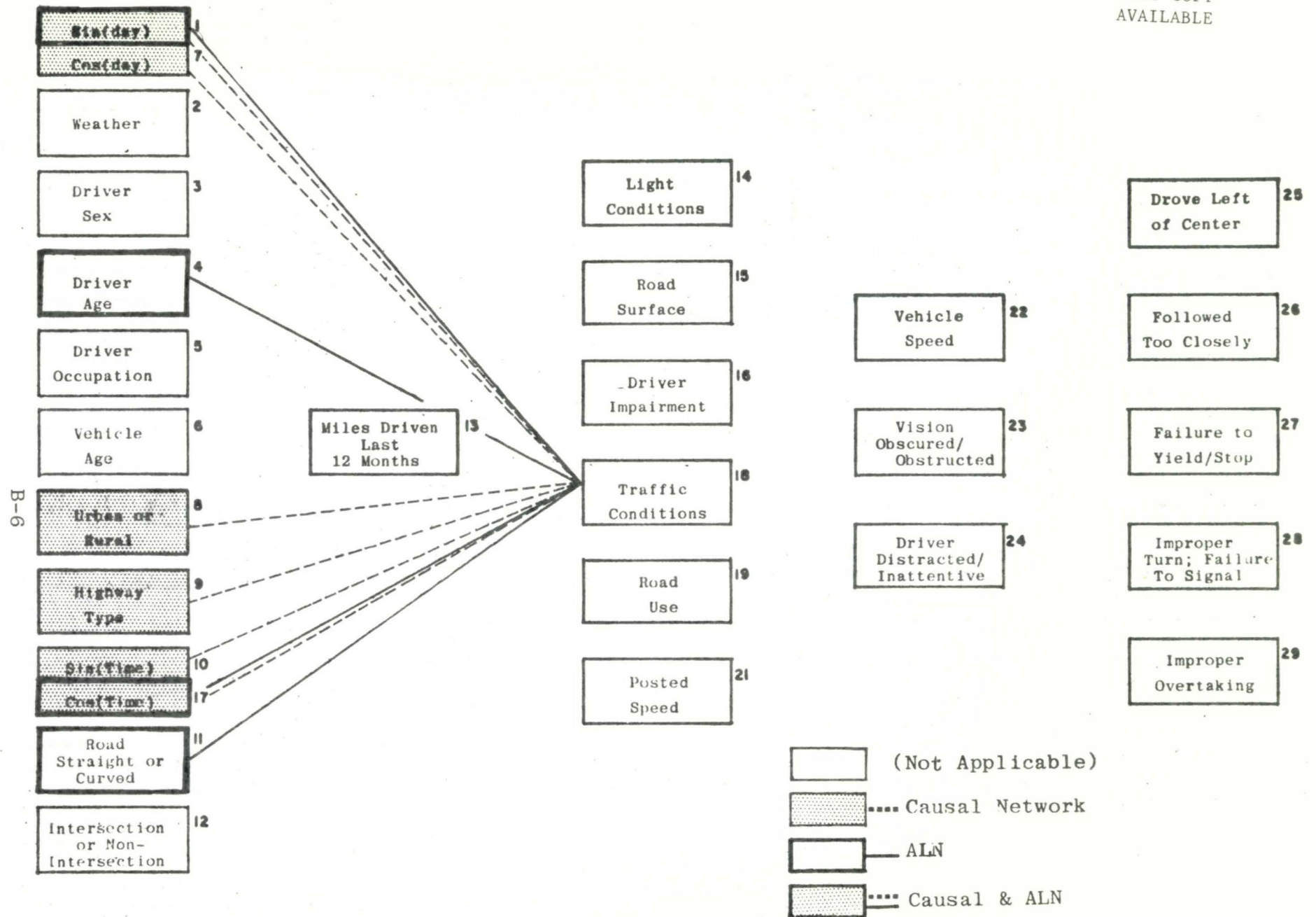
FIGURE B.5: RESTRUCTURED CAUSAL NETWORK: VARIABLE 18 - TRAFFIC CONDITIONS
