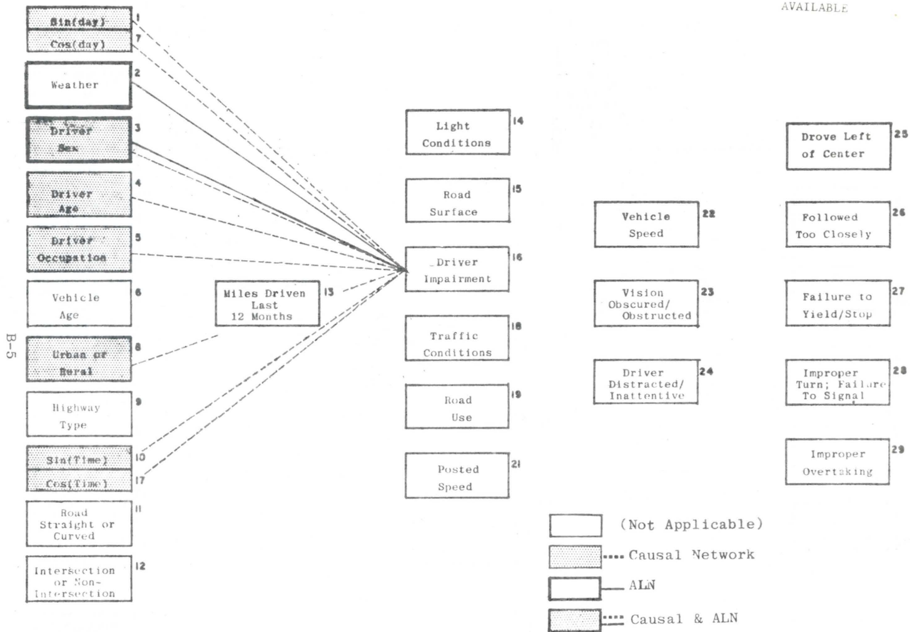
FIGURE B.4: RESTRUCTURED CAUSAL NETWORK: VARIABLE 16 - DRIVER IMPAIRMENT
