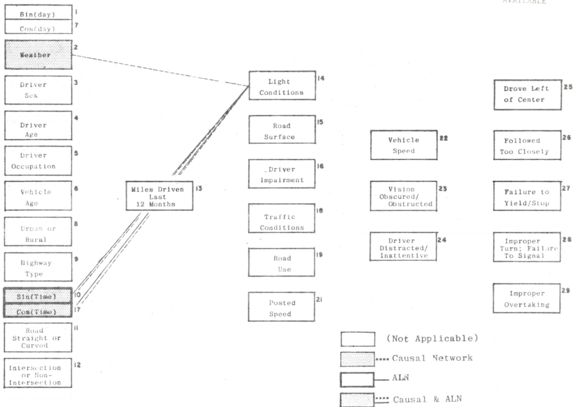
FIGURE B.2: RESTRUCTURED CAUSAL NETWORK: VARIABLE 14 - LIGHT CONDITIONS
