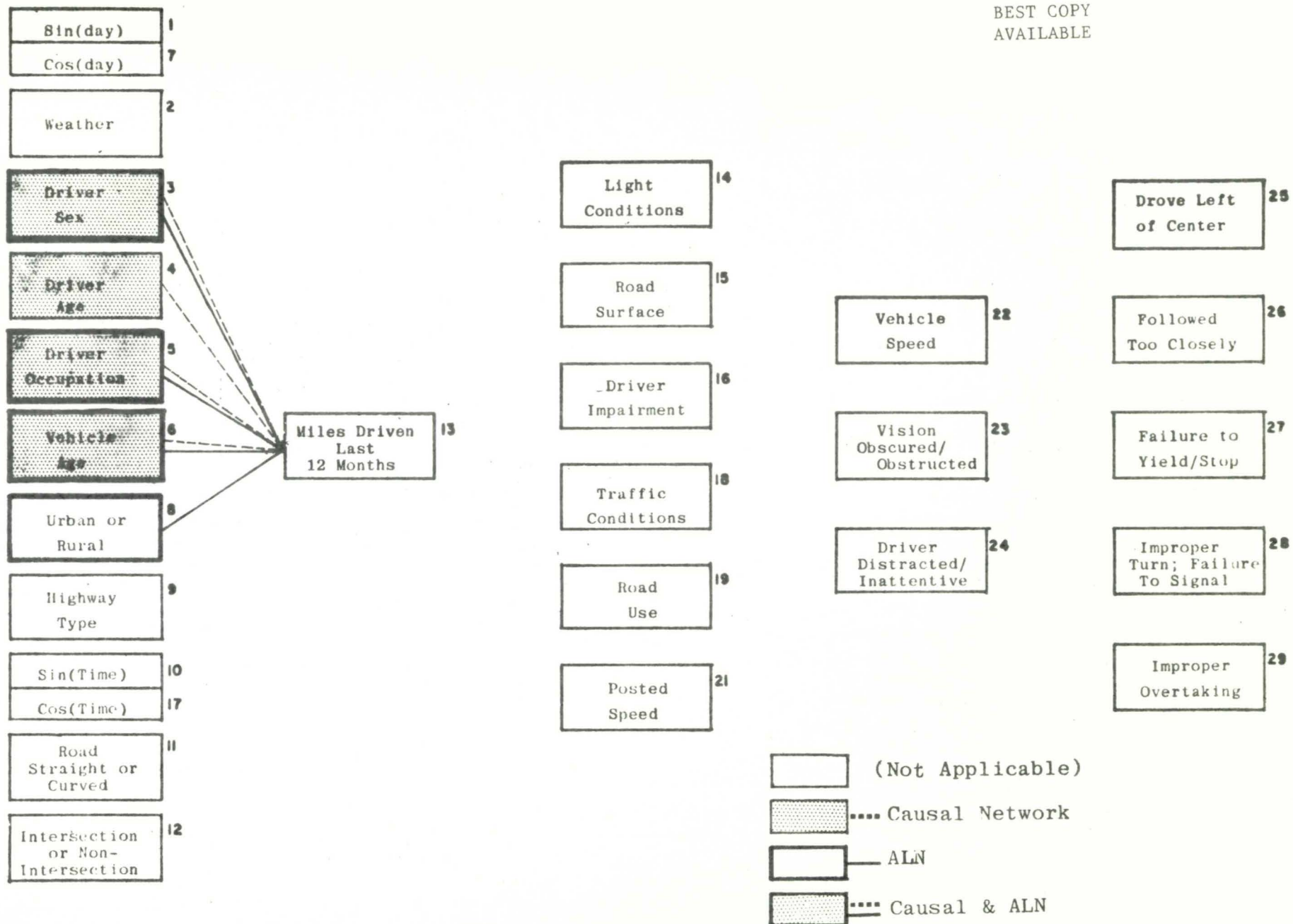
FIGURE B.1: RESTRUCTURED CAUSAL NETWORK: VARIABLE 13 - MILES DRIVEN LAST 12 MONTHS
