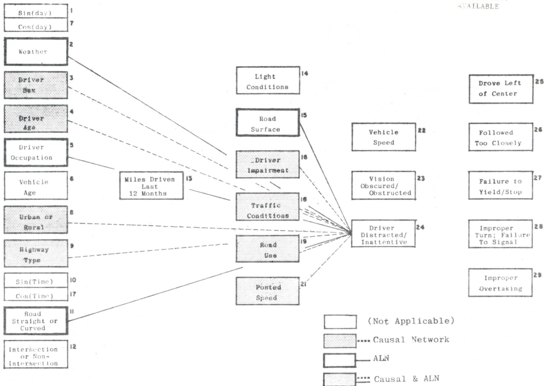
FIGURE B.10: RESTRUCTURED CAUSAL NETWORK: VARIABLE 24 - DRIVER DISTRACTED/INATTENTIVE
