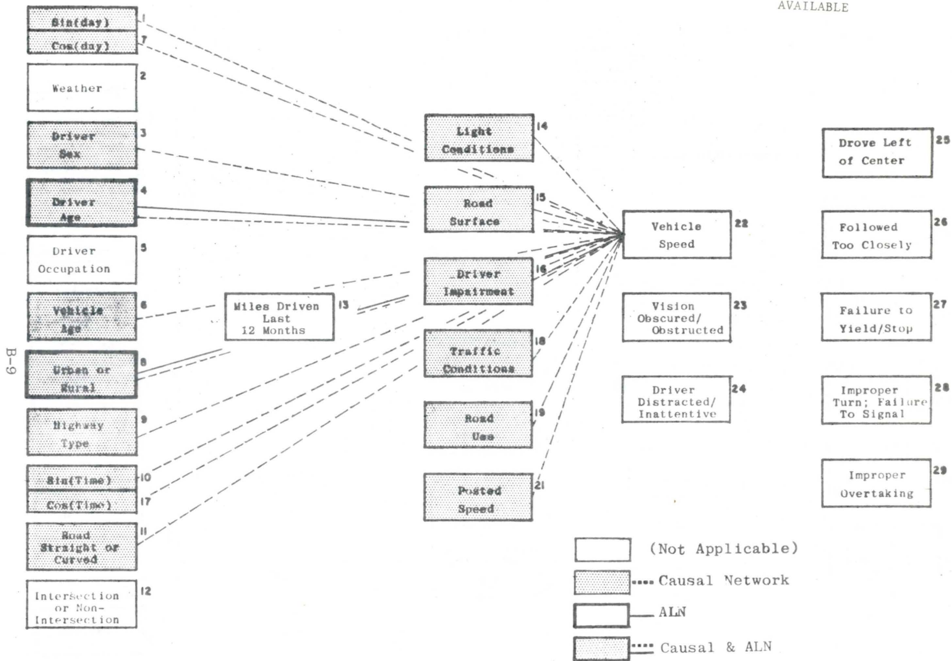
FIGURE B.8: RESTRUCTURED CAUSAL NETWORK: VARIABLE 22 - VEHICLE SPEED
