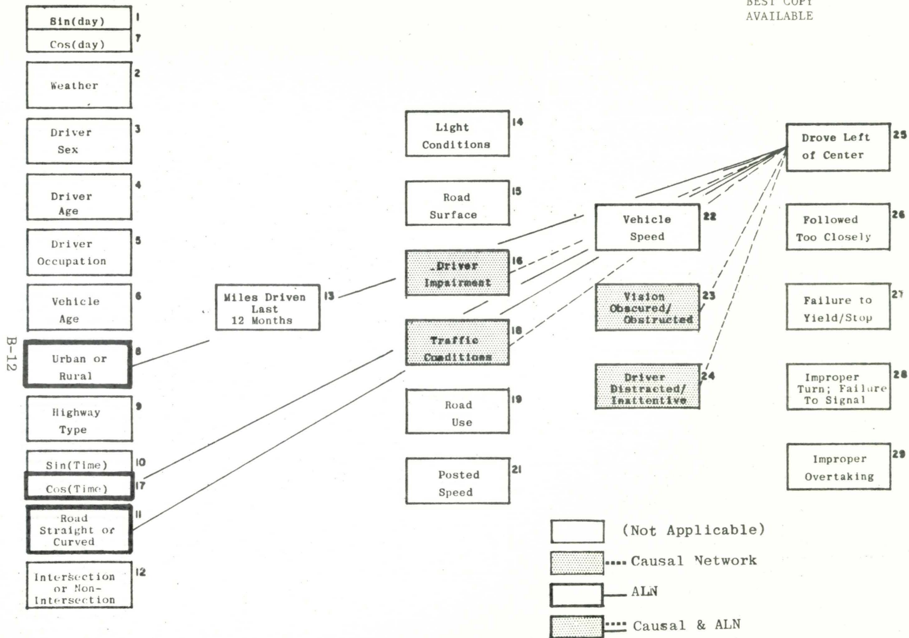
FIGURE B.11: RESTRUCTURED CAUSAL NETWORK: VARIABLE 25 - DROVE LEFT OF CENTER
