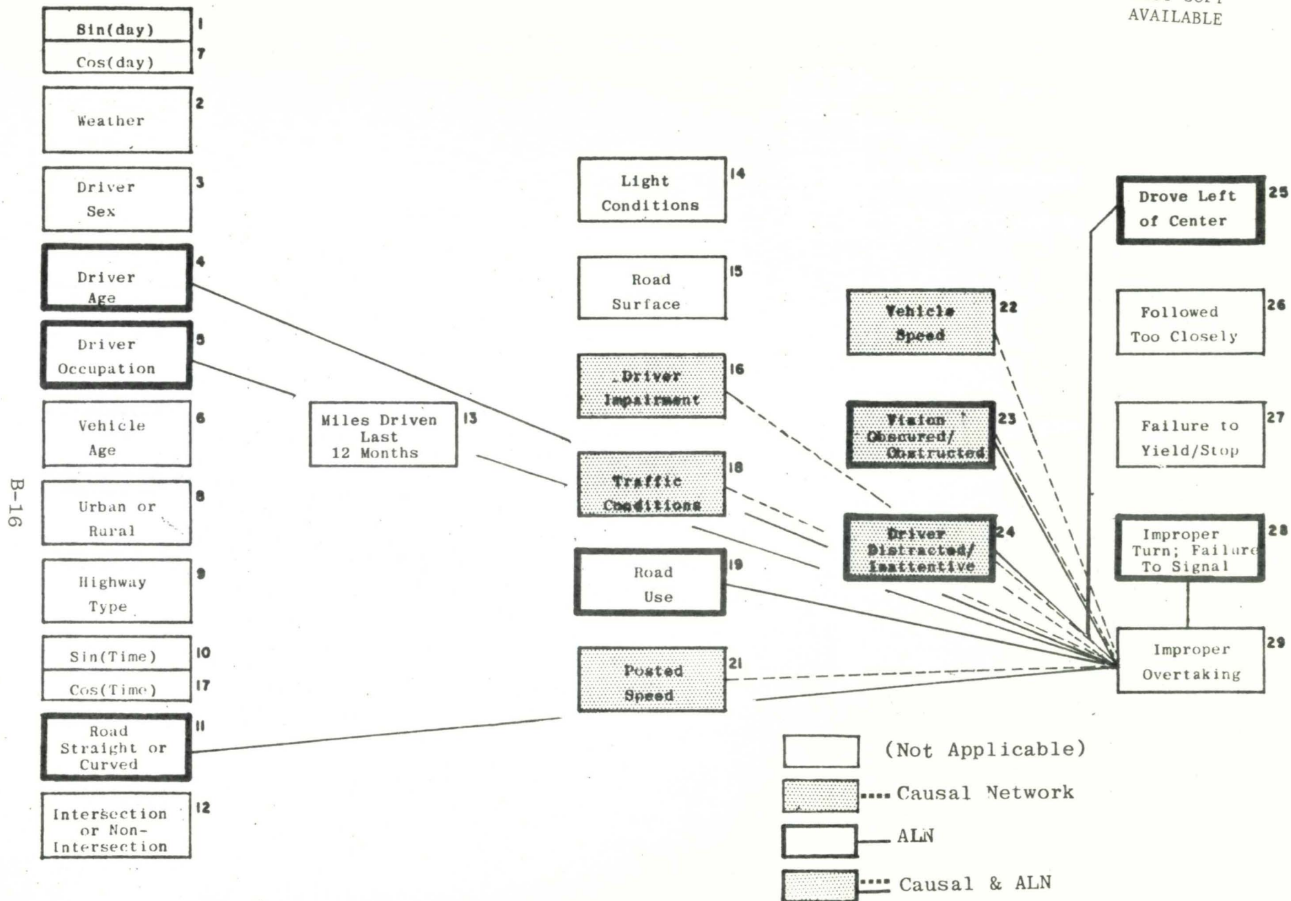
FIGURE B.15: RESTRUCTURED CAUSAL NETWORK: VARIABLE 29 - IMPROPER OVERTAKING
