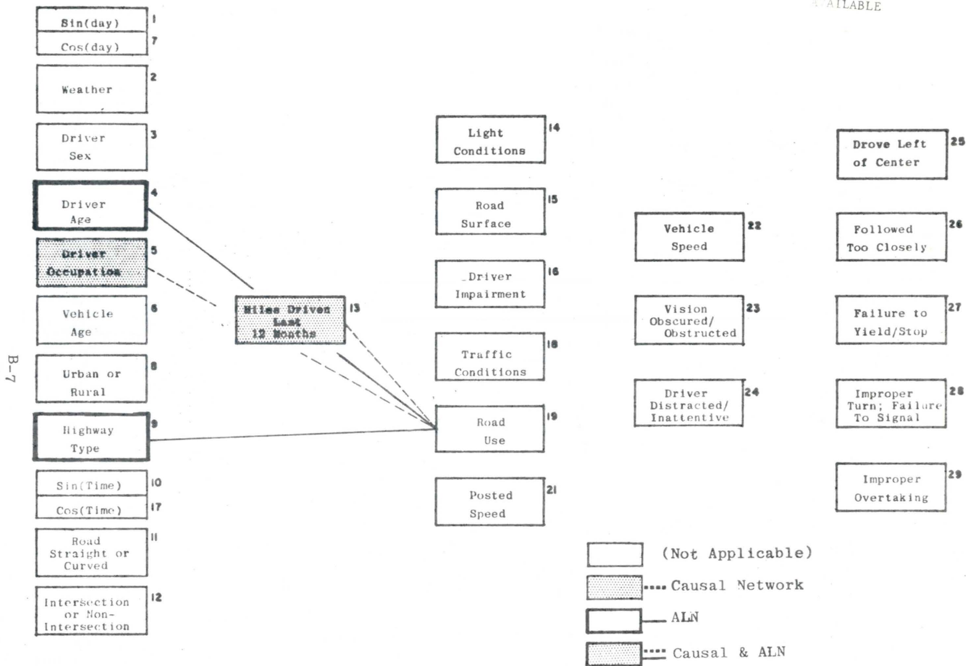
FIGURE B.6: RESTRUCTURED CAUSAL NETWORK: VARIABLE 19 - ROAD USE
