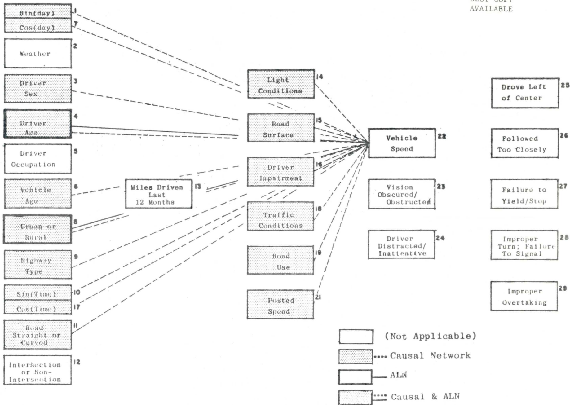
FIGURE 5.16: RESTRUCTURED CAUSAL NETWORK: VARIABLE 22 - VEHICLE SPEED
