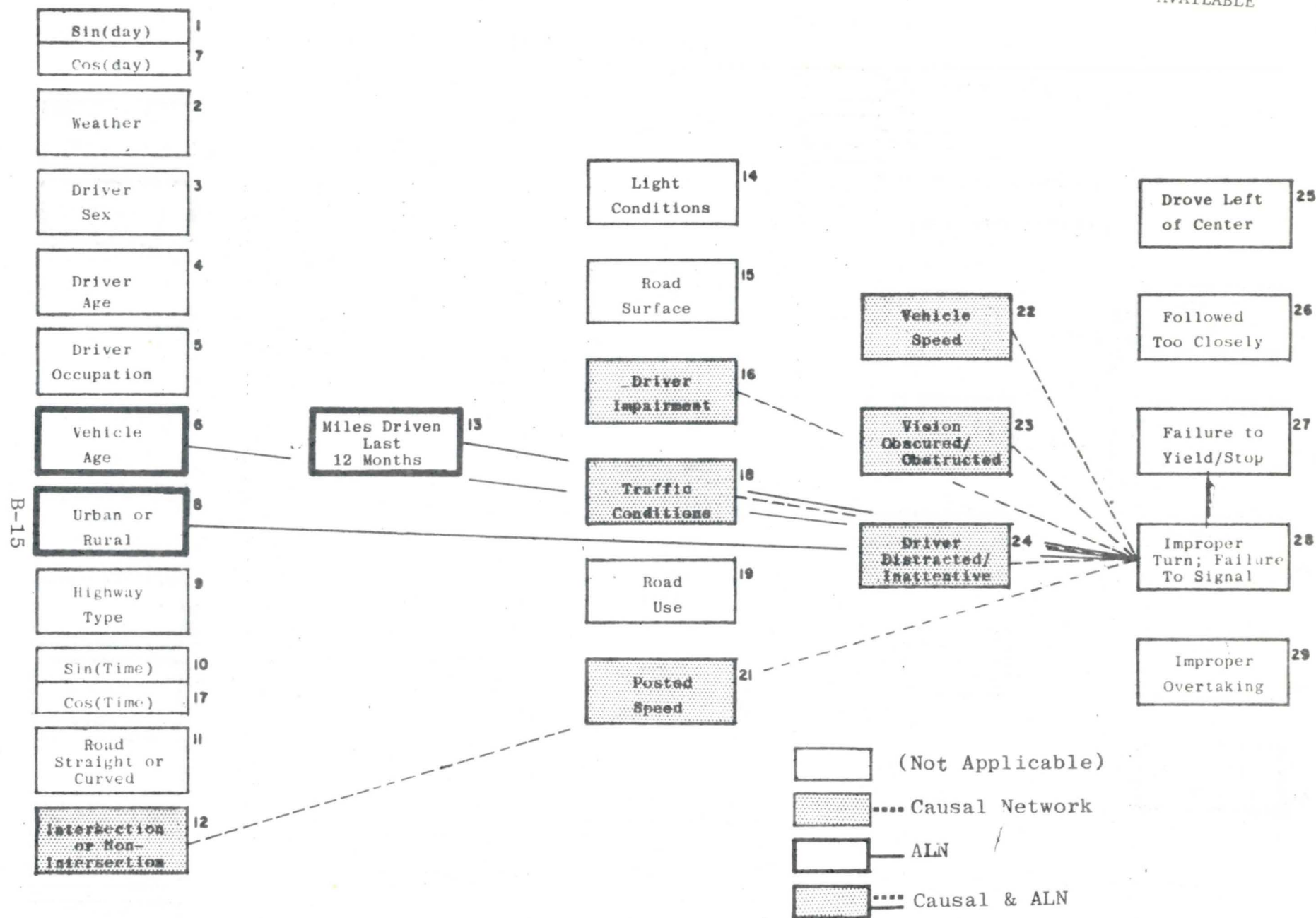
FIGURE B.14: RESTRUCTURED CAUSAL NETWORK: VARIABLE 28 - IMPROPER TURN; FAILURE TO SIGNAL
