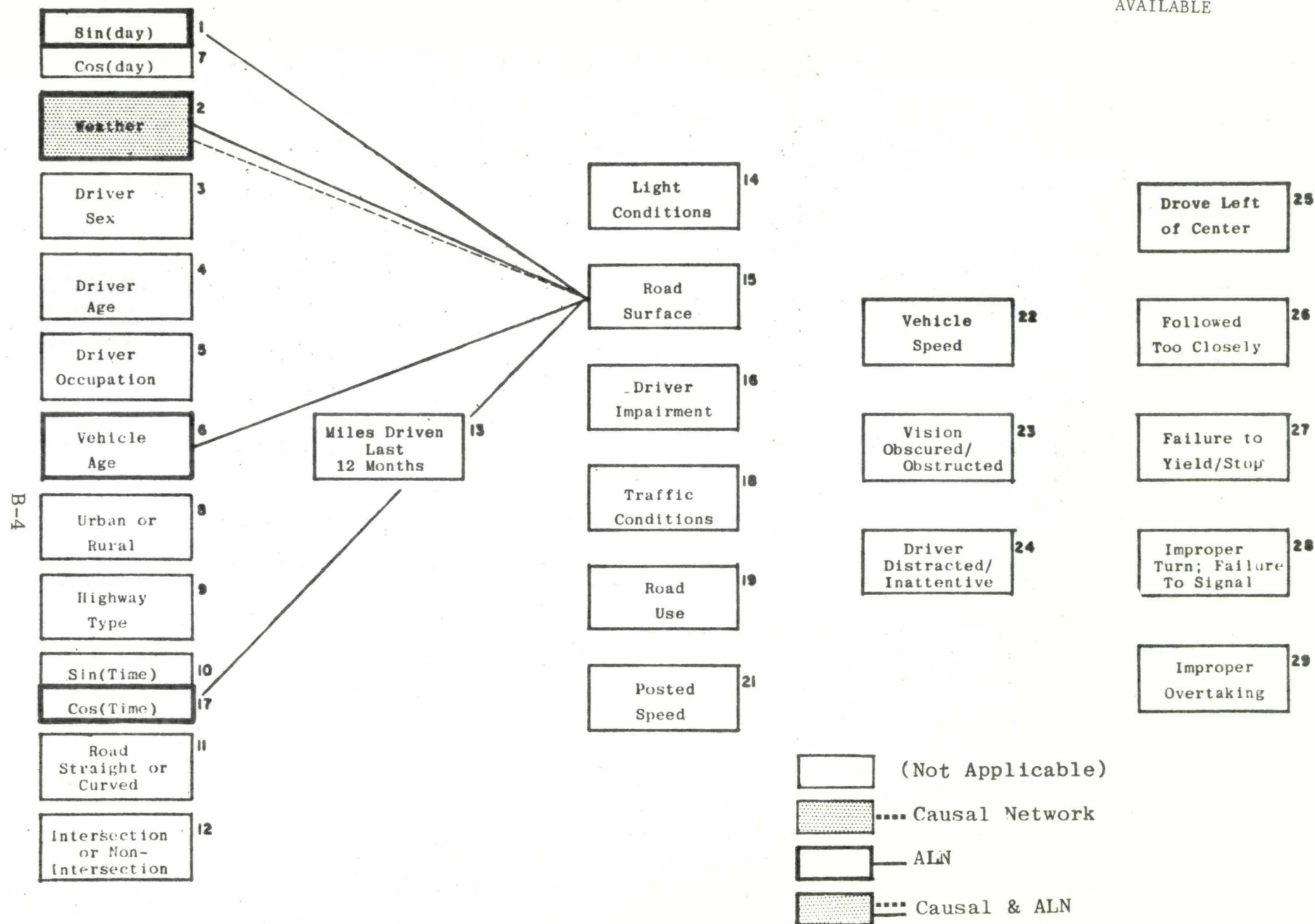
FIGURE B.3: RESTRUCTURED CAUSAL NETWORK: VARIABLE 15 - ROAD SURFACE
