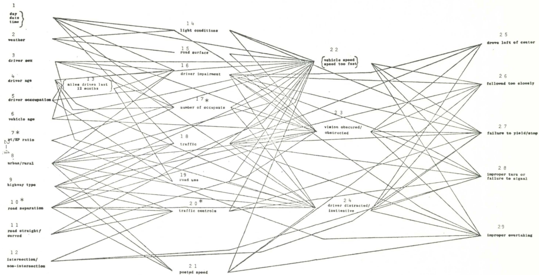
FIGURE 2.2: TYPICAL CAUSAL NETWORK
