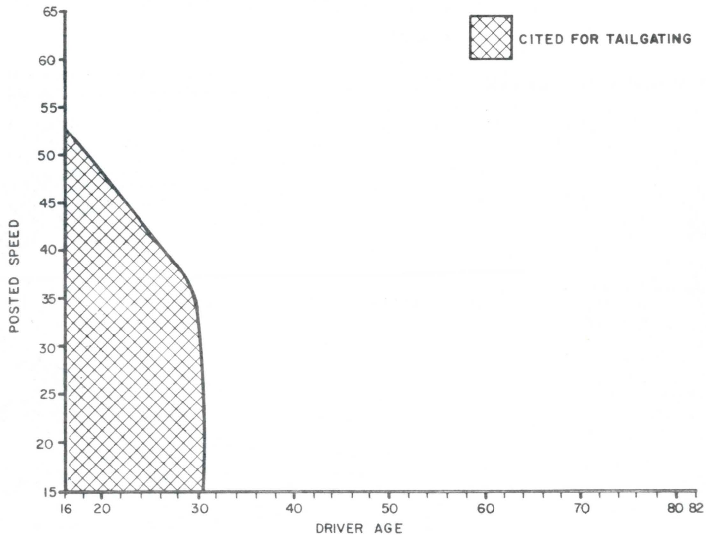
FIGURE 6.3: DECISION REGIONS FOR VARIABLE 26 (TAILGATING -- FIG. 5.12)
