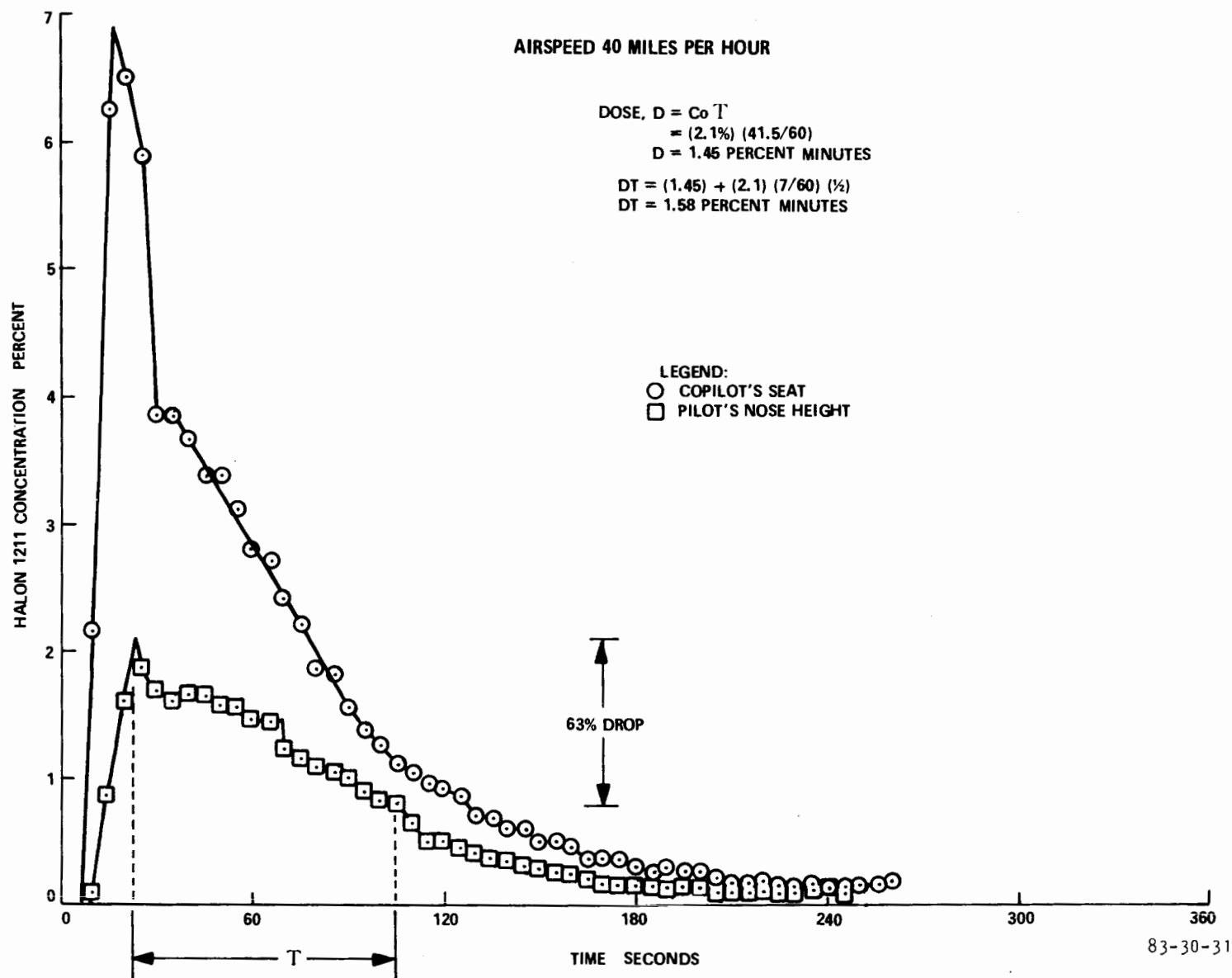
FIGURE 31. HALON 1211 CONCENTRATIONS - 2.5 POUND EXTINGUISHER DIRECTED TO THE COPILOT'S SEAT - AIRSPEED 40 MPH - OVERHEAD VENTS OPEN
