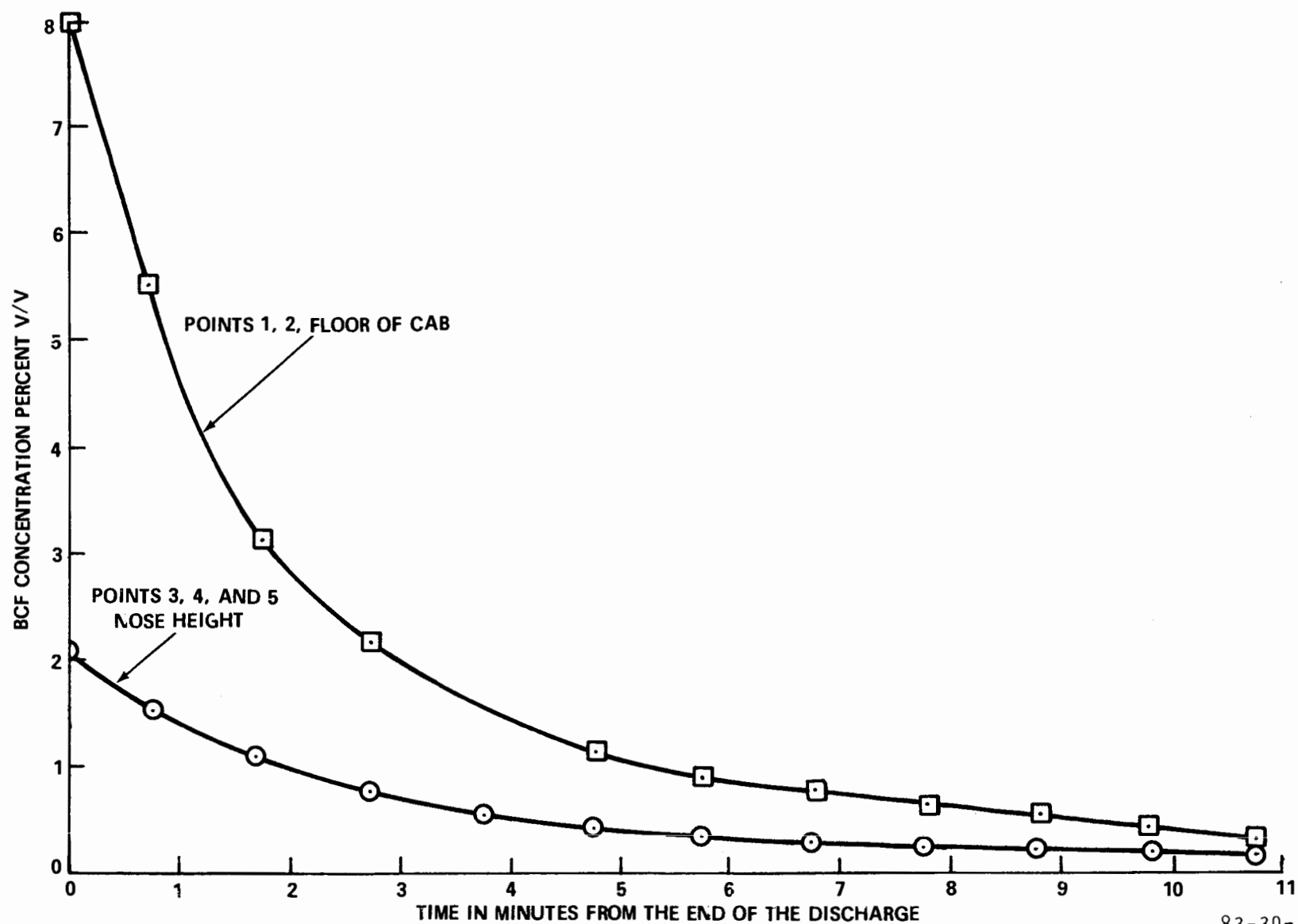
FIGURE 1. "BCF" CONCENTRATIONS - LORRY CAB, RUNS 1 AND 2, 3-1b (1.4 Kg) EXTINGUISHER (EXCERPTED FROM REFERENCE 2)
