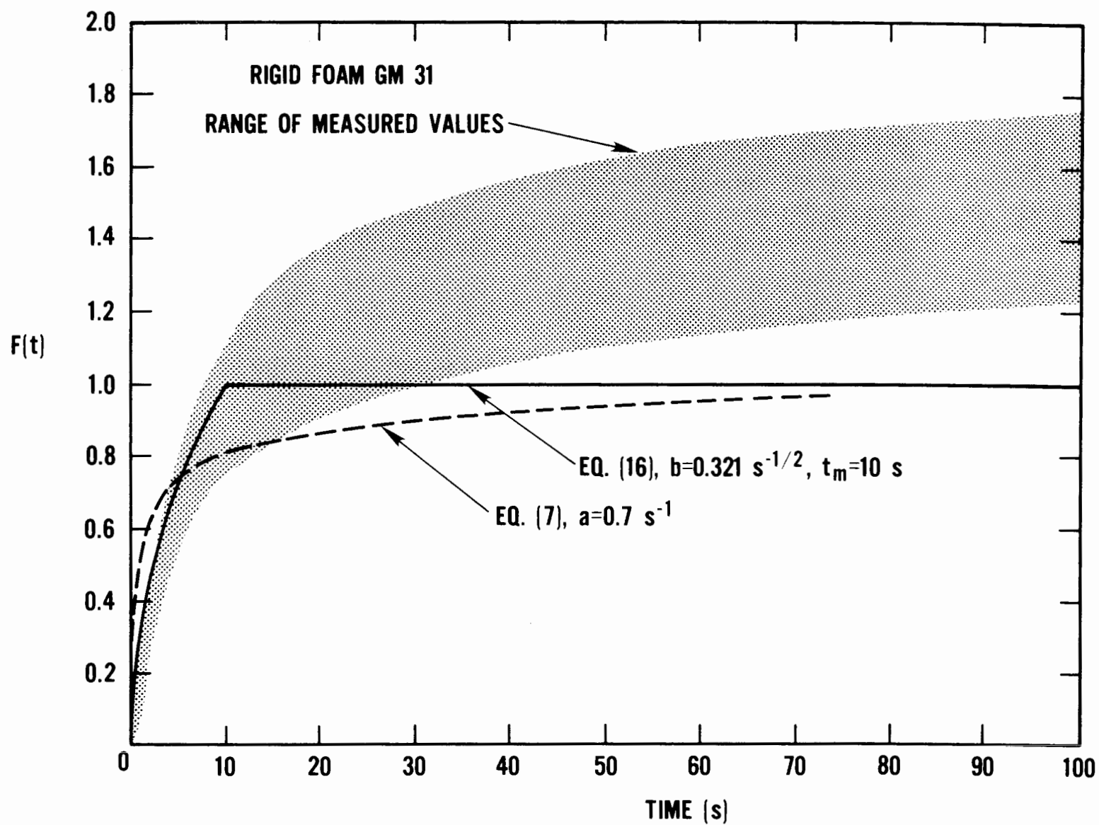
FIGURE 42. SURFACE TEMPERATURE PREDICTION FROM F(t) FOR RIGID FOAM
