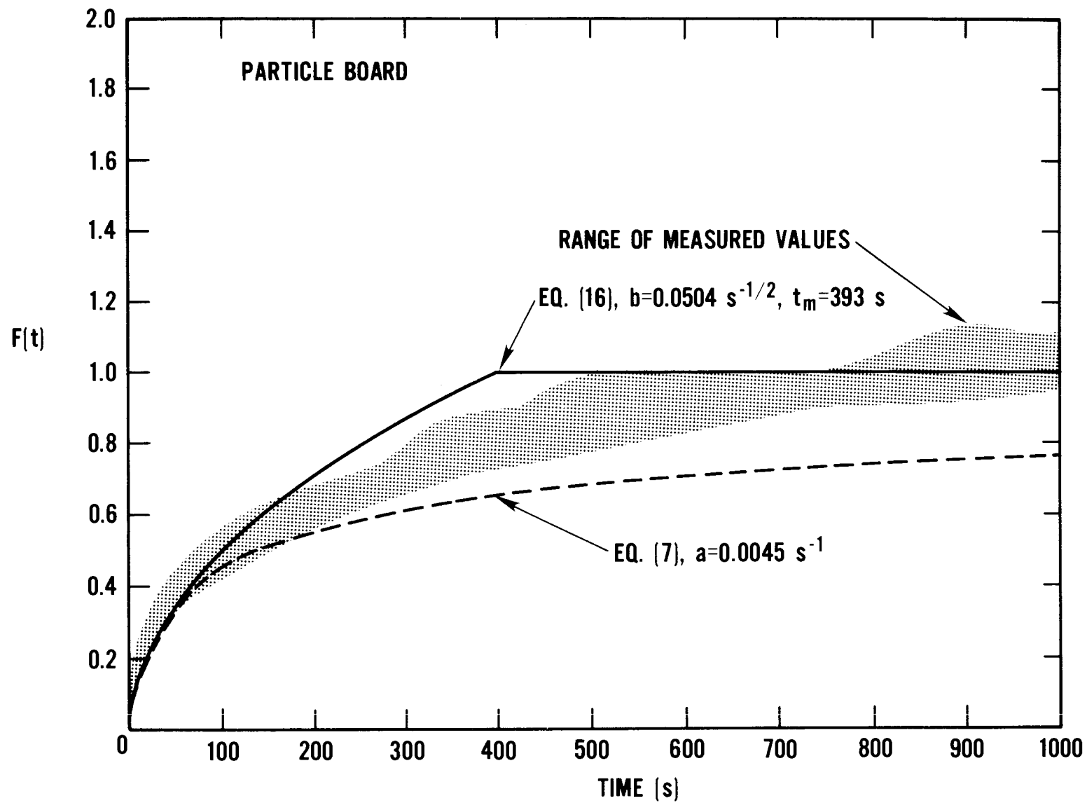
FIGURE 40. SURFACE TEMPERATURE PREDICTION FROM F(t) FOR PARTICLE BOARD
