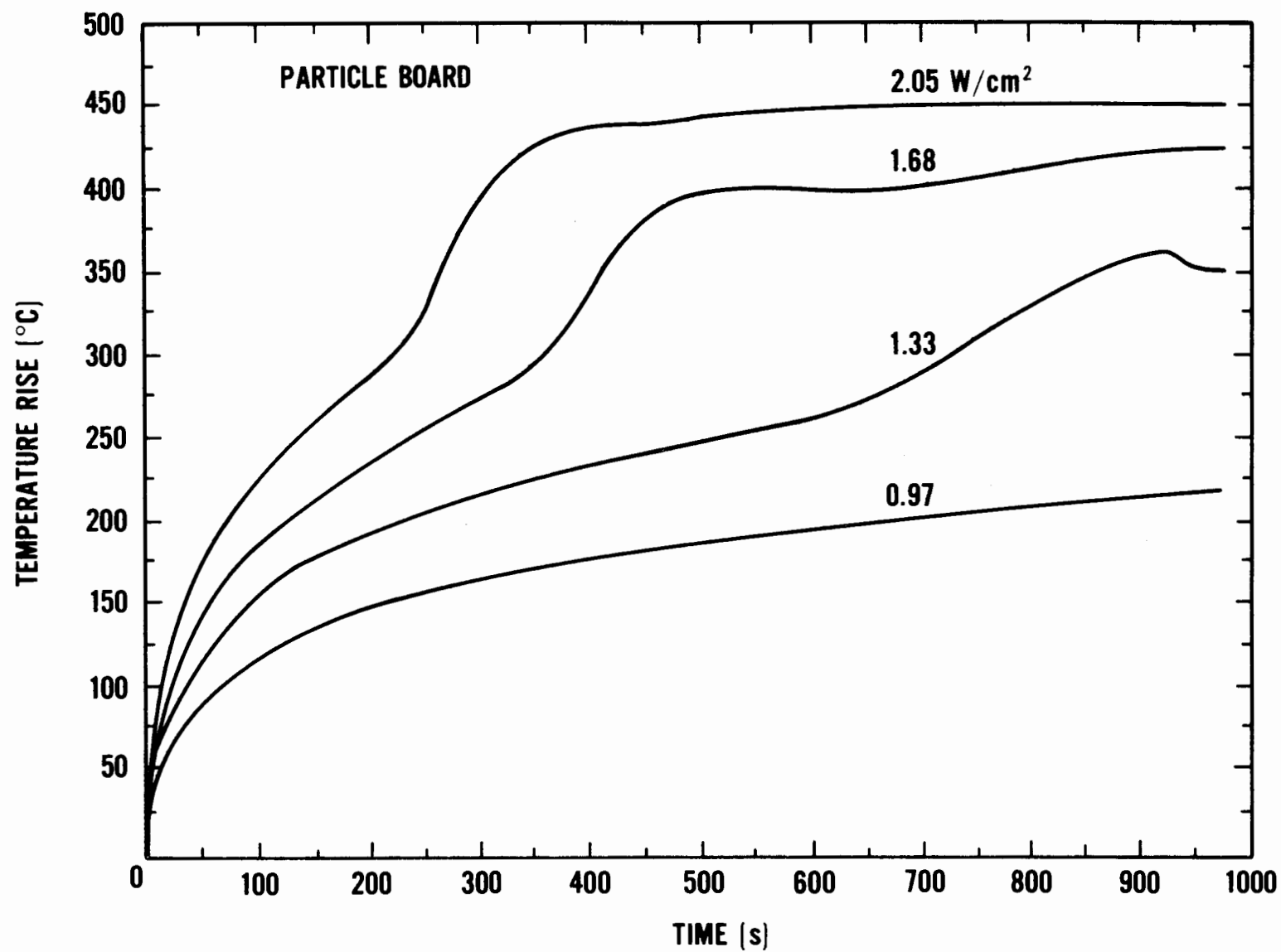
FIGURE 35. SURFACE TEMPERATURE RISE FOR PARTICLE BOARD
