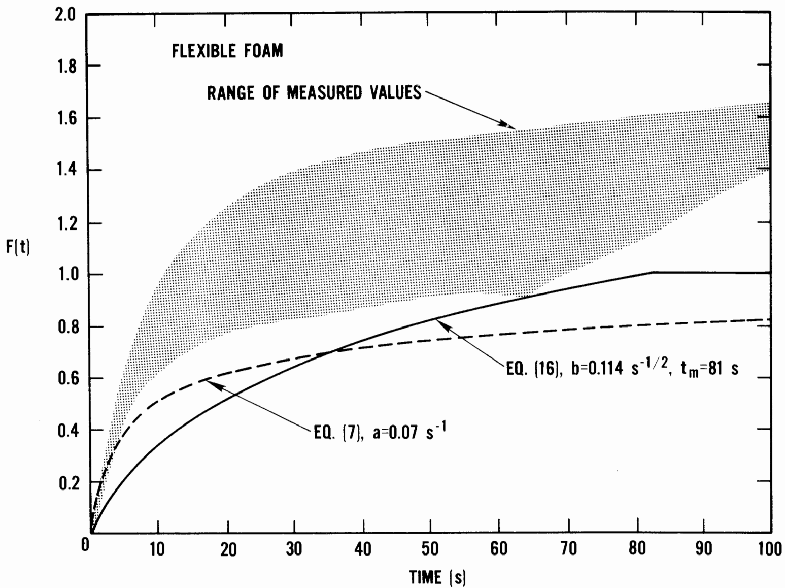
FIGURE 43. SURFACE TEMPERATURE PREDICTION FROM F(t) FOR FLEXIBLE FOAM
