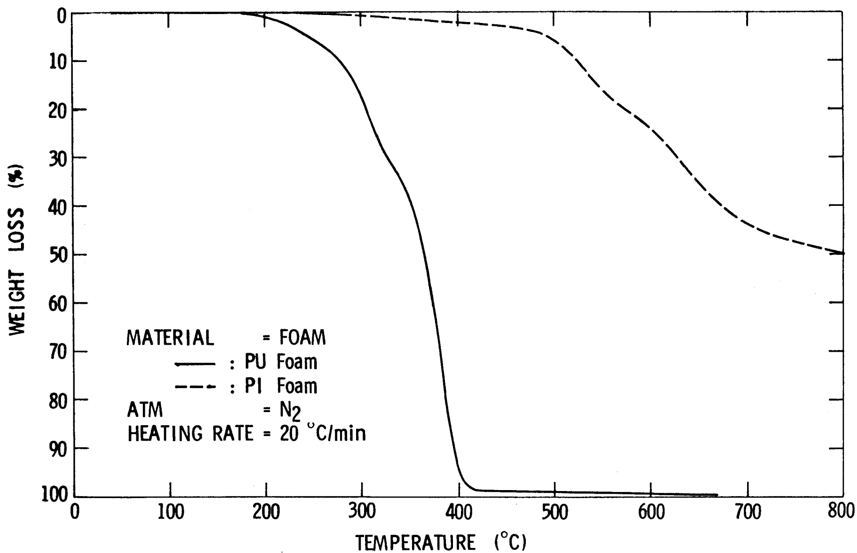
FIGURE 6. THERMOGRAVIMETRIC DIAGRAMS OF TWO FOAMS, POLYURETHANE FOAM AND POLYIMIDE FOAM.
