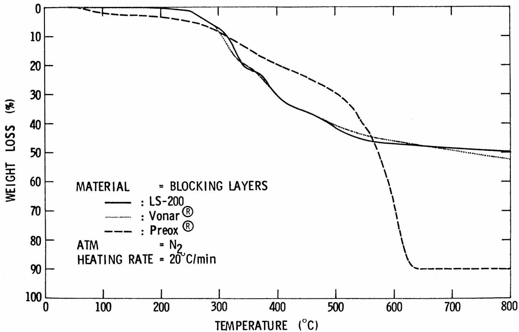
FIGURE 5. THERMOGRAVIMETRIC DIAGRAMS OF THREE FIRE BLOCKING LAYERS, LS-200, VONAR, AND PREOX.
