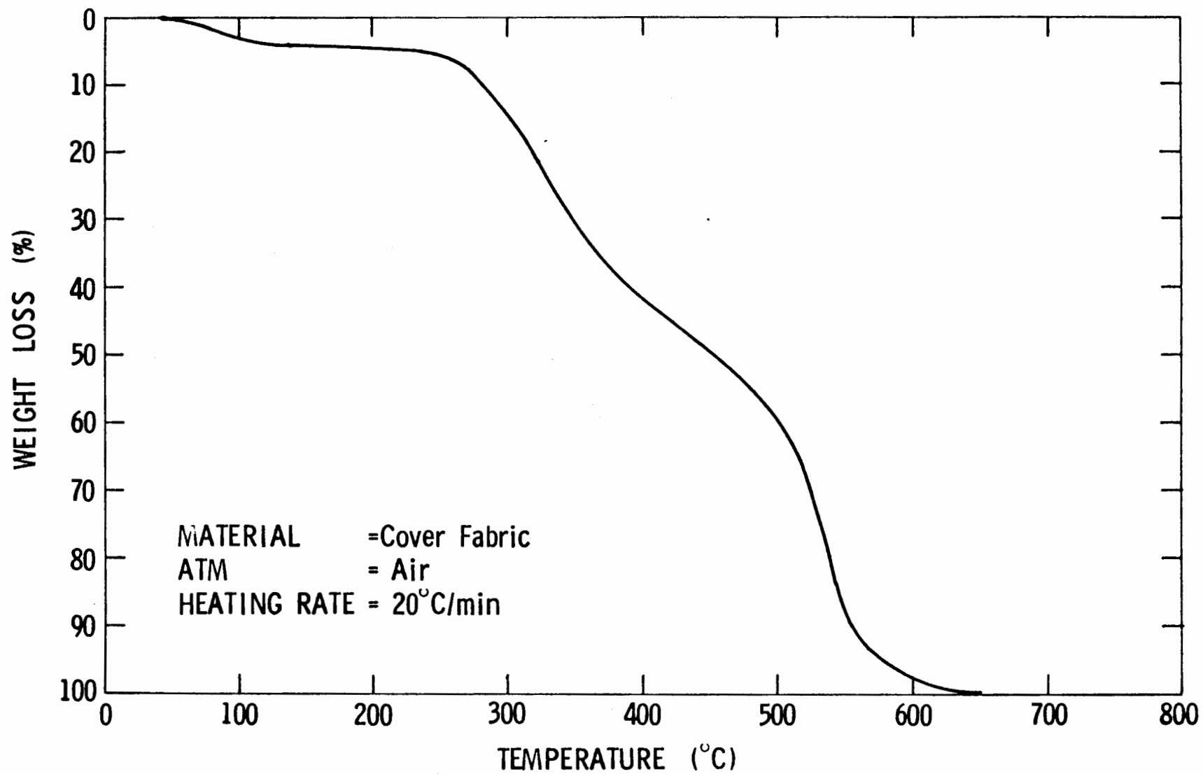
FIGURE 4. THERMOGRAVIMETRIC DIAGRAM OF SEAT CUSHION COVER FABRIC.
