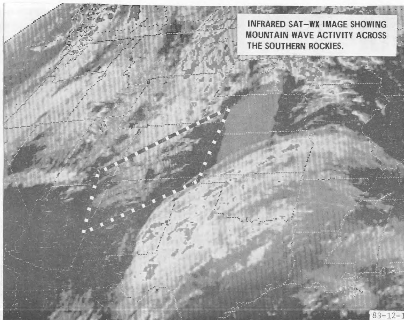
FIGURE 1. GOES SAT-WX IMAGE DEPICTING MOUNTAIN WAVE AND JET STREAM LOCATIONS
