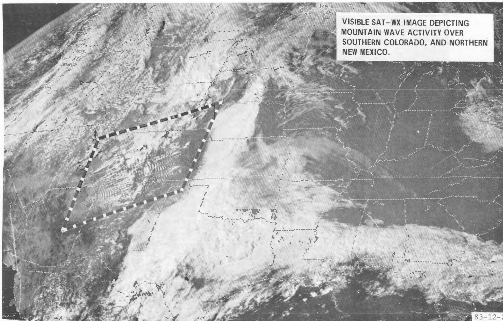
FIGURE 2. GOES SAT-WX IMAGE DEPICTING MOUNTAIN WAVE ACTIVITY
