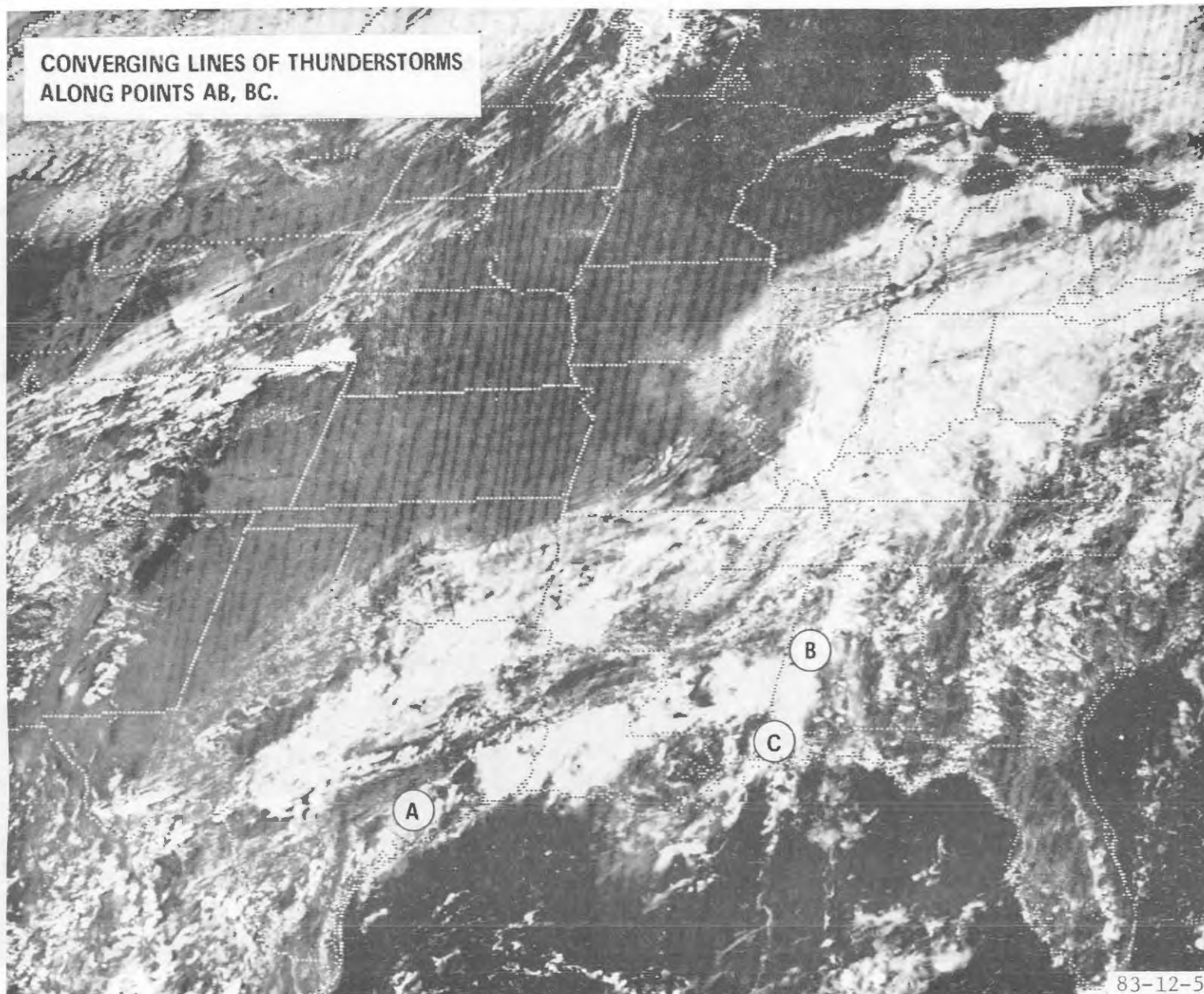
FIGURE 5. GOES SAT-WX IMAGE DEPICTING CONVERGING LINES OF THUNDERSTORMS
