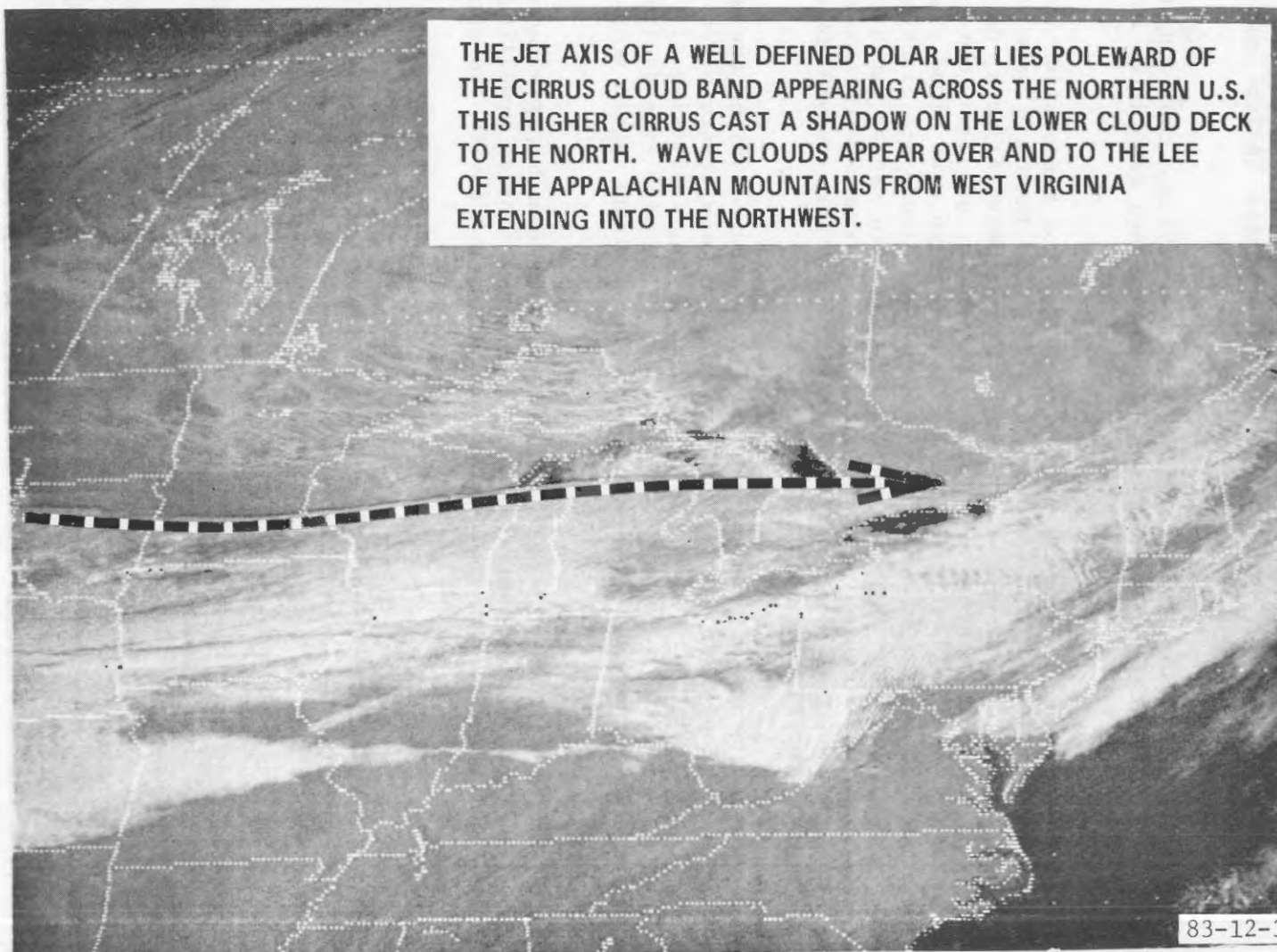
FIGURE 3. GOES SAT-WX IMAGE DEPICTING JET STREAM LOCATION
