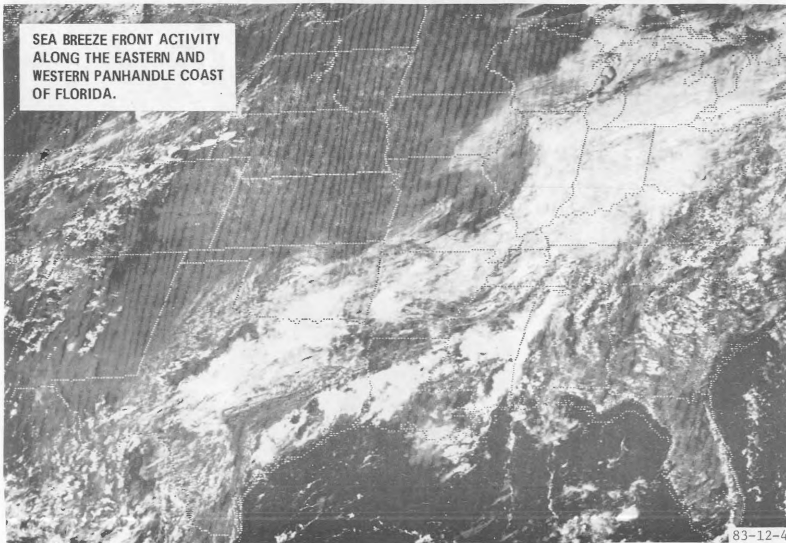
FIGURE 4. GOES SAT-WX IMAGE DEPICTING SEA BREEZE FRONT ACTIVITY
