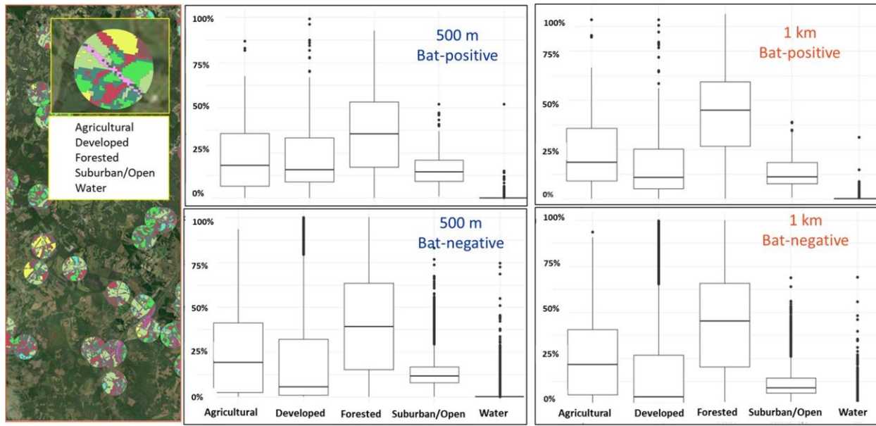
Figure 5. Land Cover Composition Surrounding Bat-Positive (n = 246) and Bat-Negative (n = 8,121) Bridges and Culvert Complexes in 500-m and 1-km Radii
