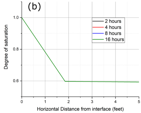
Figure 27. Spatial variation of degree of saturation near the pile face for site-1; (a) in vertical direction, (b) in horizontal direction.
